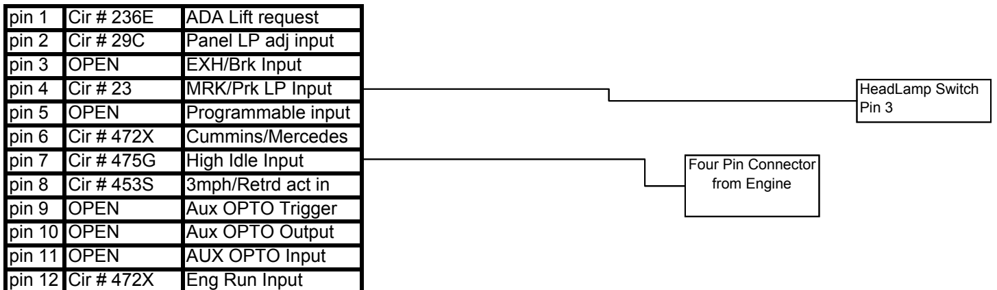
12 Pin Connector J3
