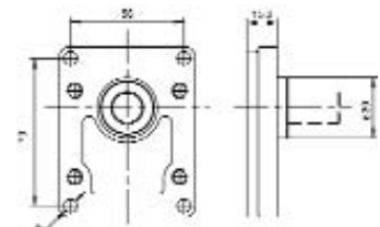
D2 Italian/European 4 Bolt 30mm Pilot
