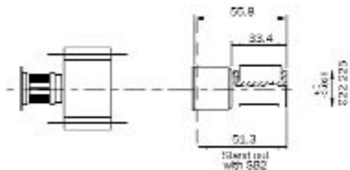
P2 Long SAE B 7/8" Parallel
