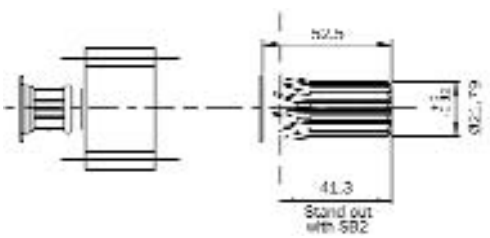
S2 SAE B 13 Tooth Spline
