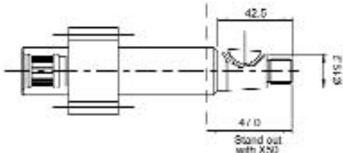
T2 1:8 Taper with M14 X 1.5mm Thread & 4mm Wide Key
