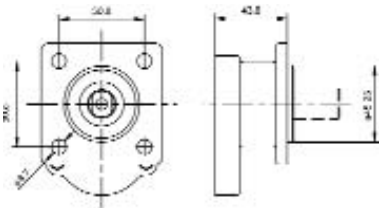
A1 2" x 2" 4 Bolt Shallow Shaft Seal
