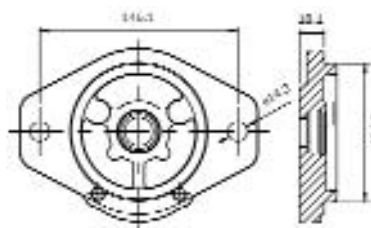
SB2W SAE B 2 Bolt
