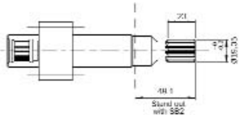
Q3 SAE 11 Tooth Spline
