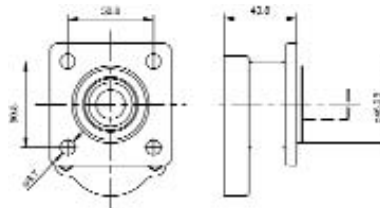
A2A1 2" x 2" 4 Bolt Deep Shaft Seal
