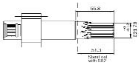
S3 Long SAE B 13 Tooth Spline
