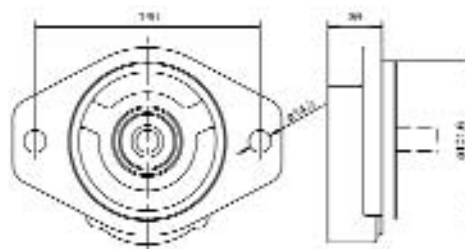
CSB2 Continental SAE B 2 Bolt
