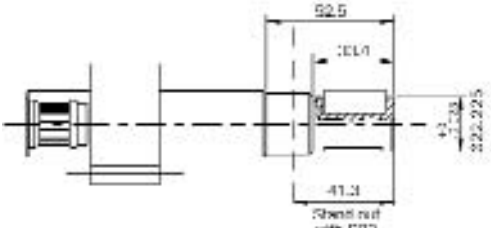
P1 SAE B 7/8" Parallel
