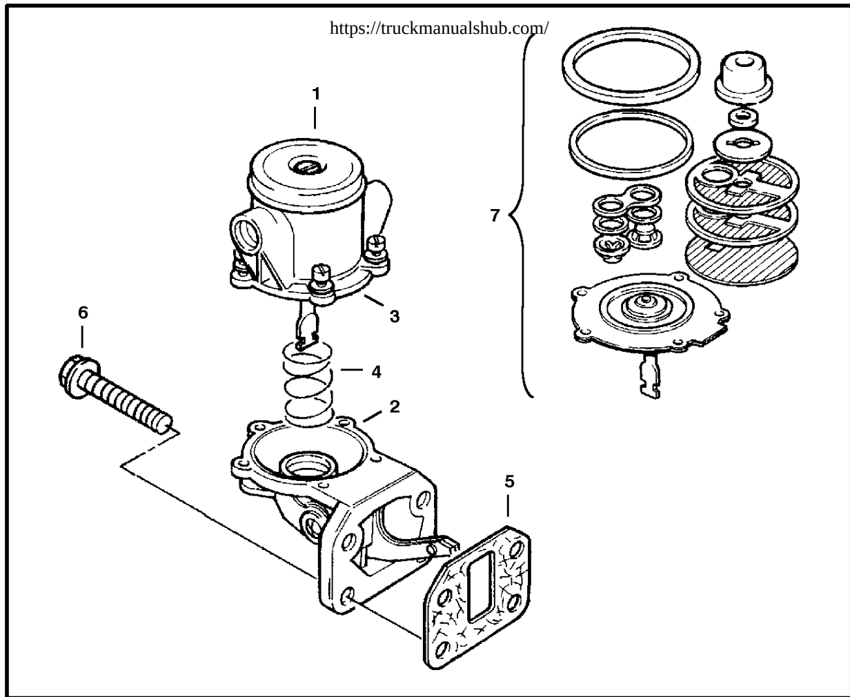
FUEL PUMP
