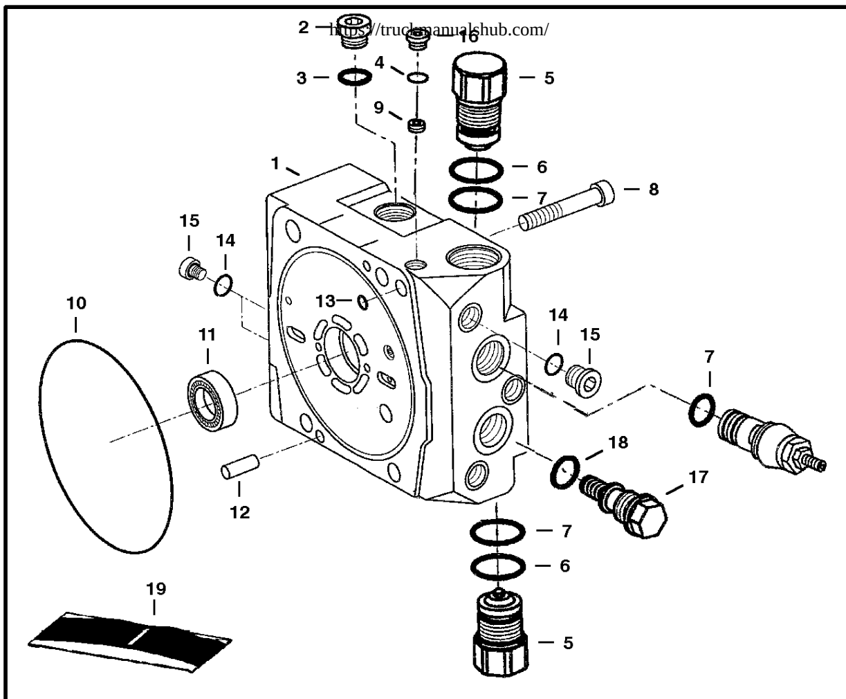
PORT BLOCK
