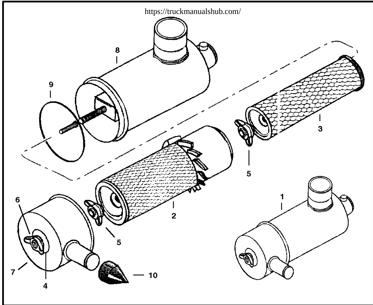
AIR CLEANER
