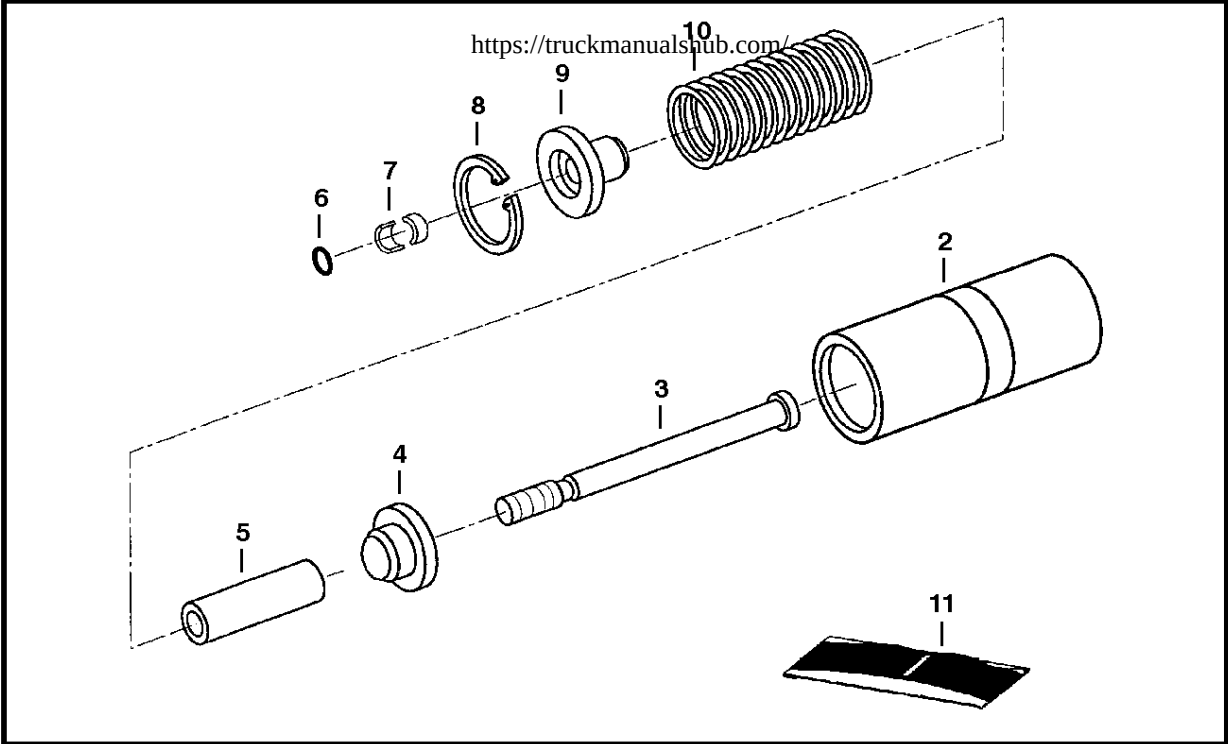
PISTON ASSY
