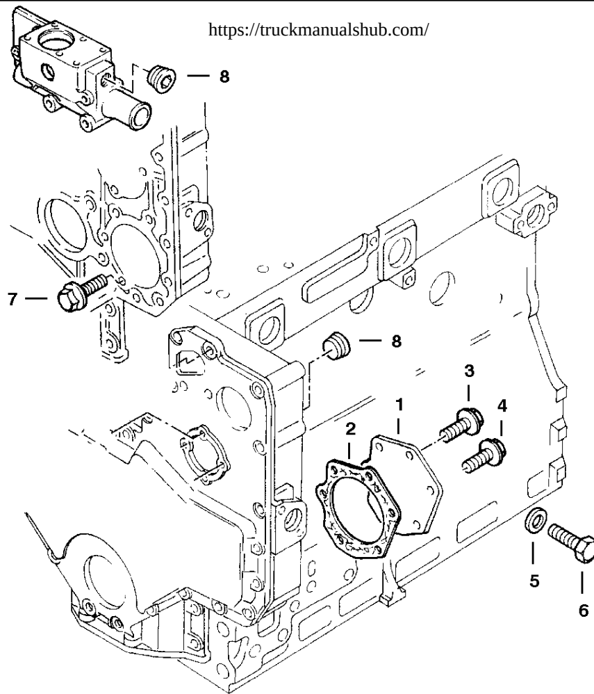
PLATE EXTERNAL
