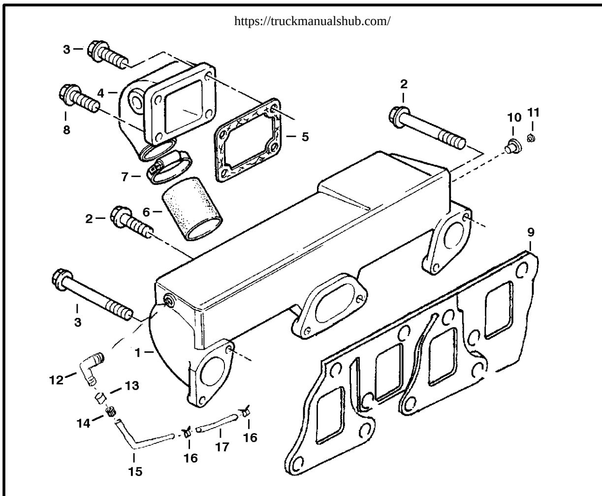
MANIFOLD
