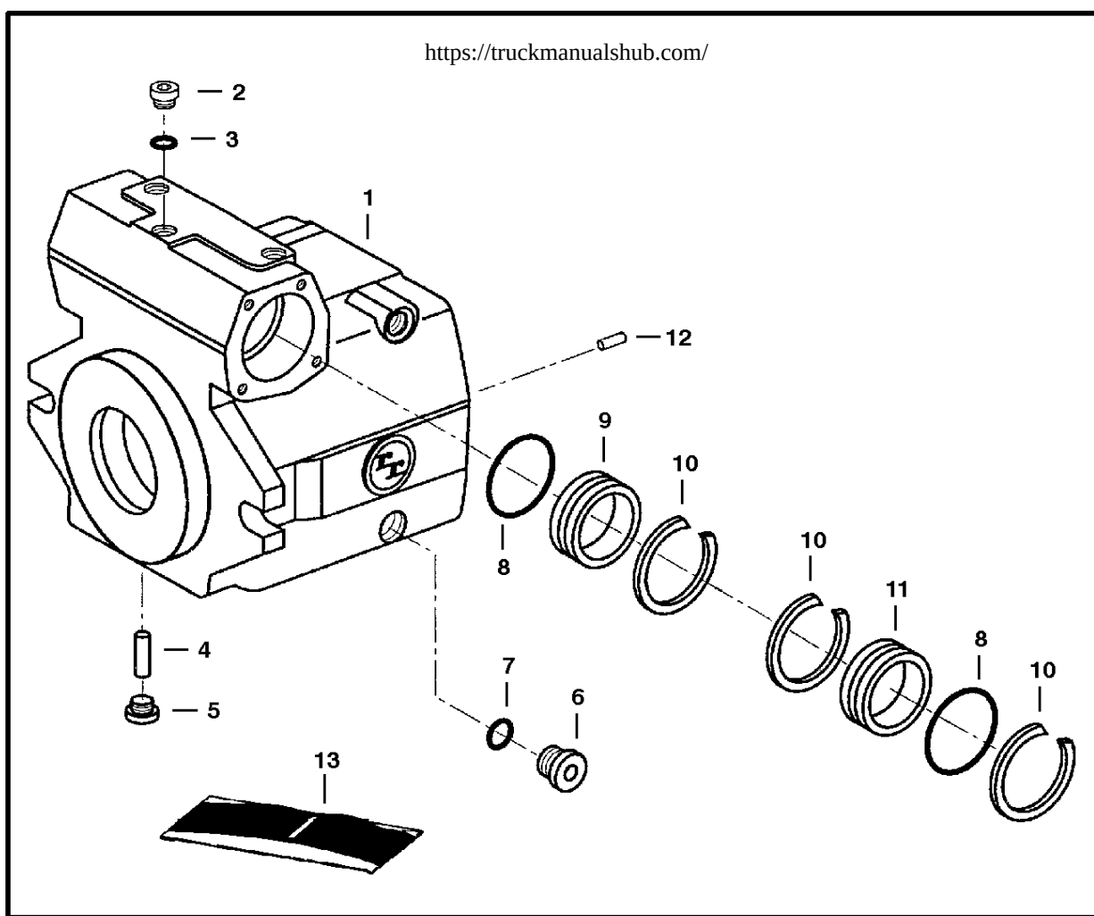
HOUSING ASSY
