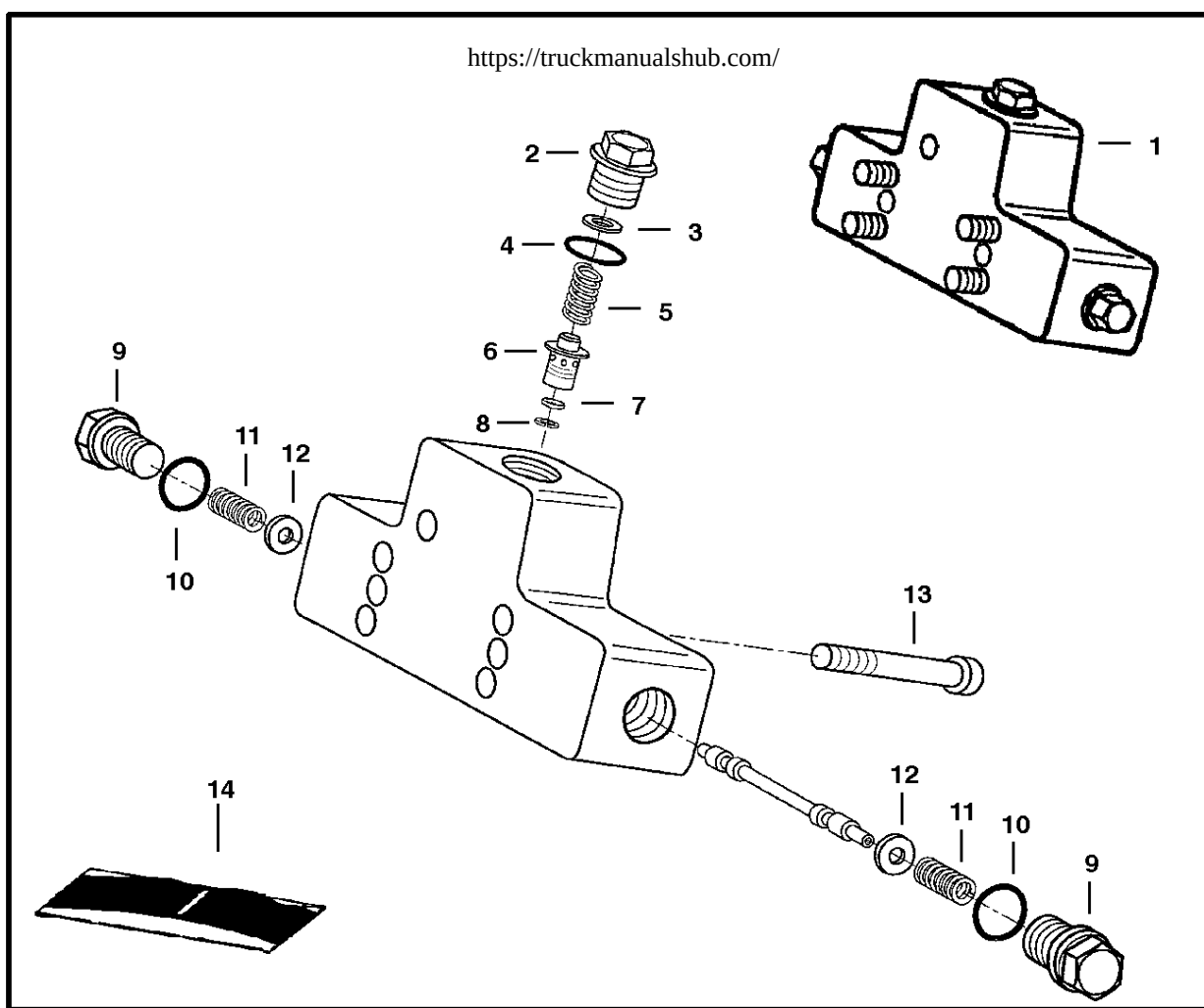
FLUSHING VALVE
