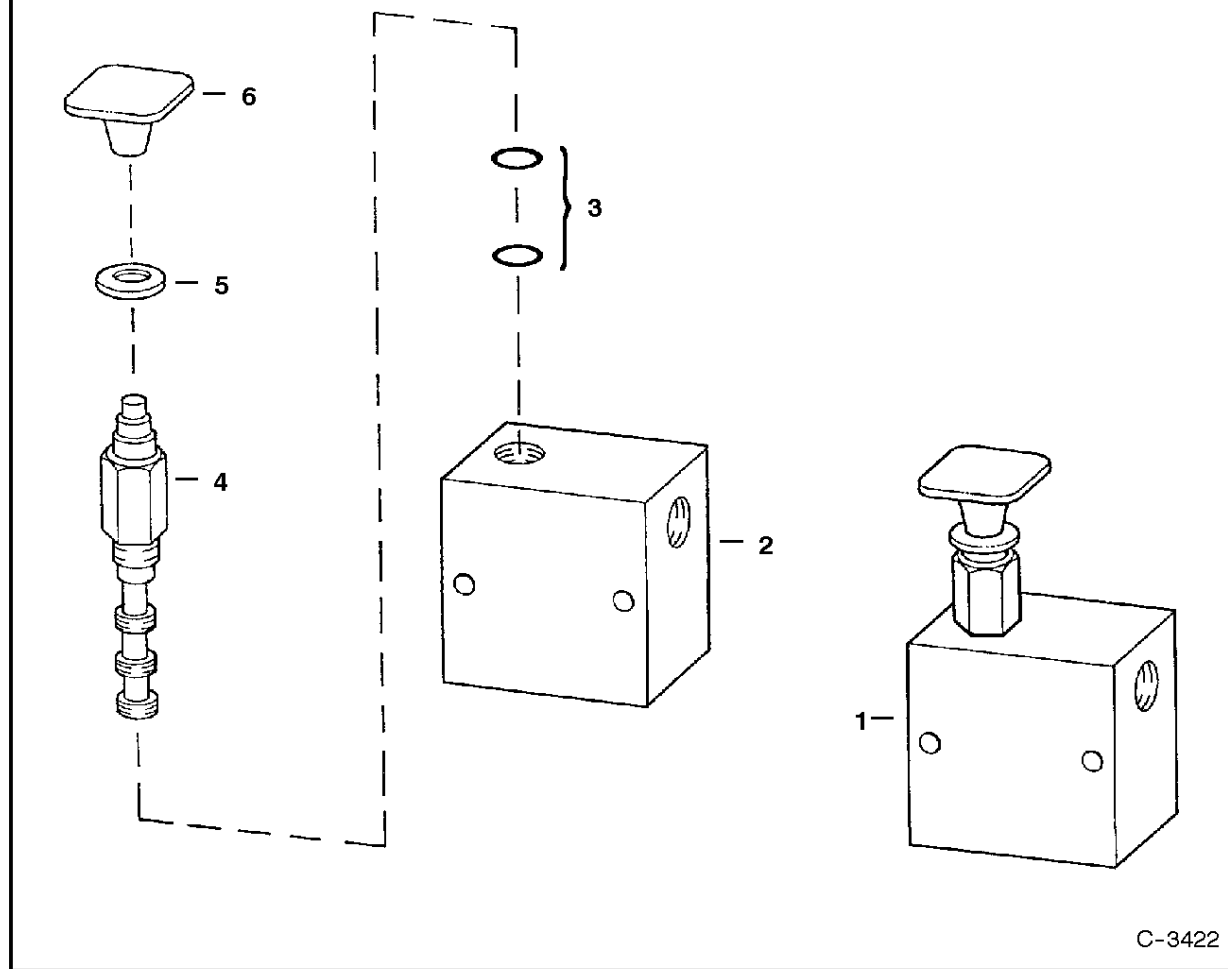
MANUAL LIFT RELEASE VALVE
