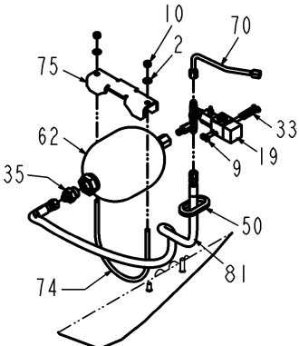
DETAIL D
