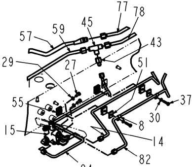
VIEW E-E
