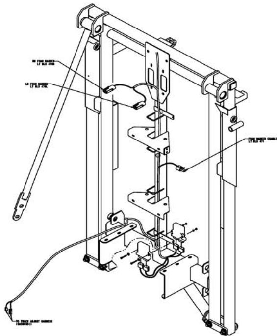
VIEW G-G
