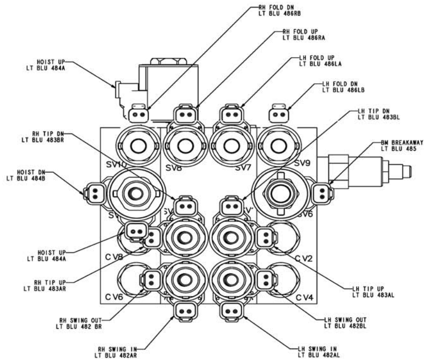
VIEW C-C
