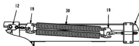
VIEW F-F
