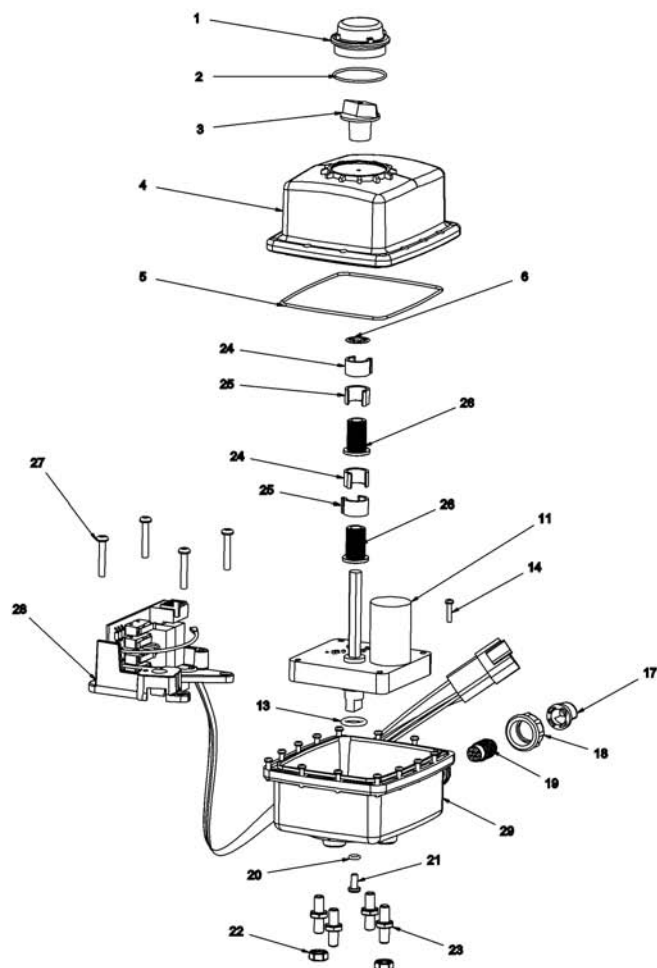
Parts Breakdown Units After Serial #86501
