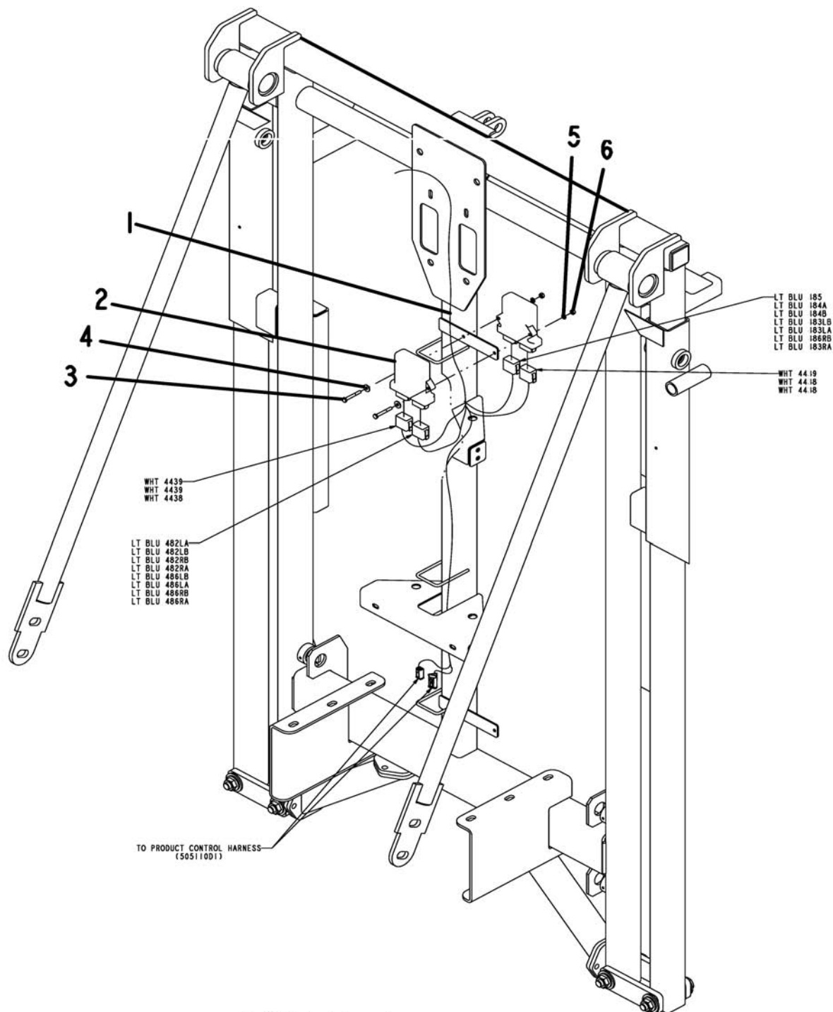
DETAIL A
