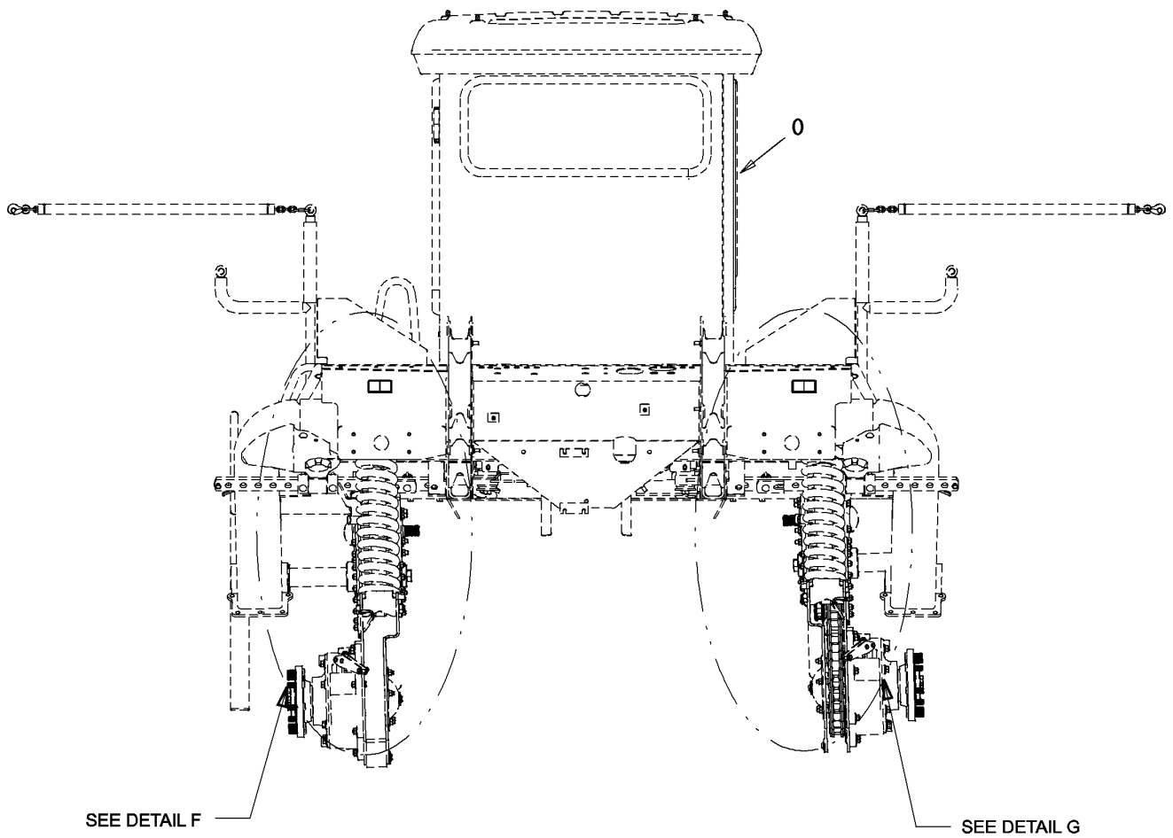
REAR VIEW
