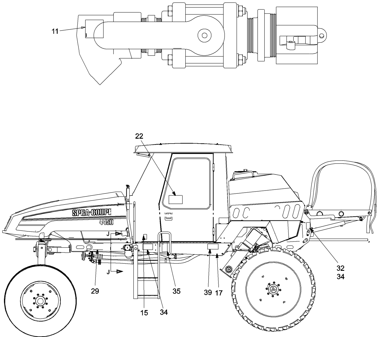
VIEW J-J
