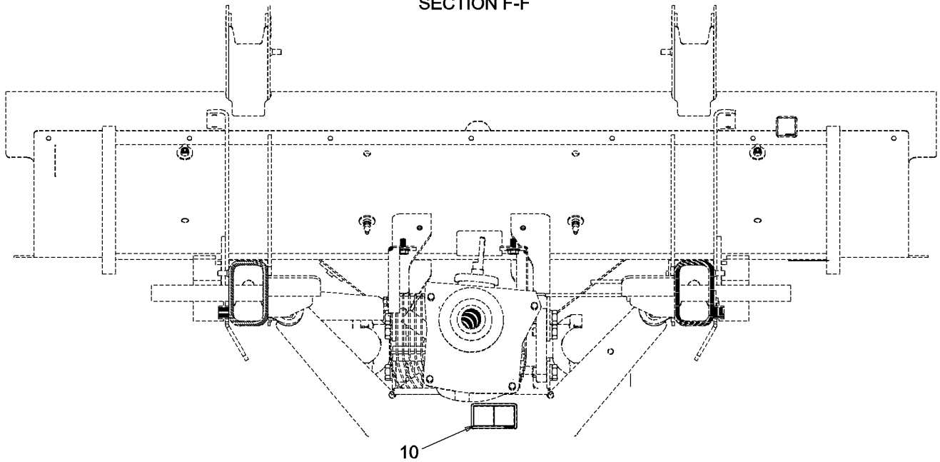
SECTION F-F
