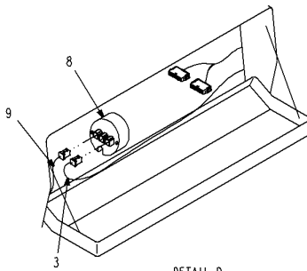
DETAIL D
