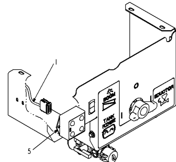
DETAIL C
