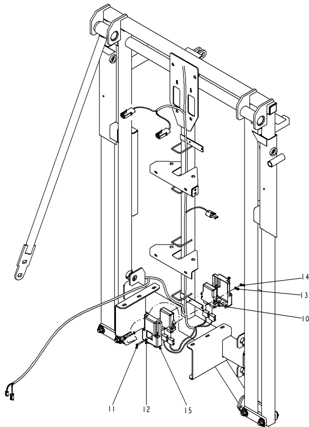
VIEW G-G
