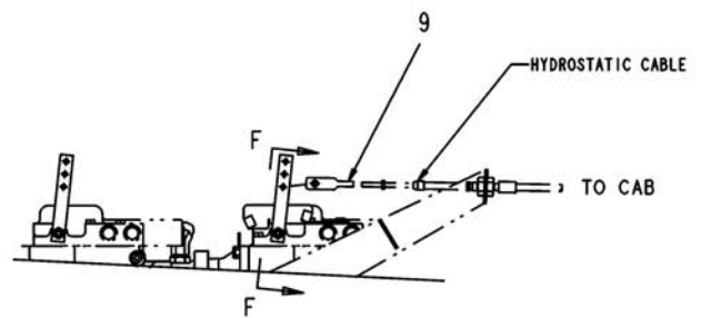
VIEW D-D
