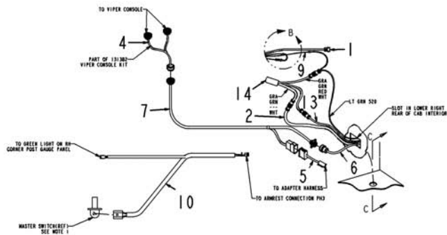
VIEW A
