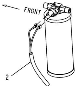
DETAIL R
