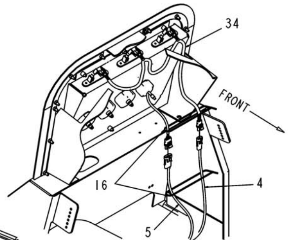
DETAIL Q
