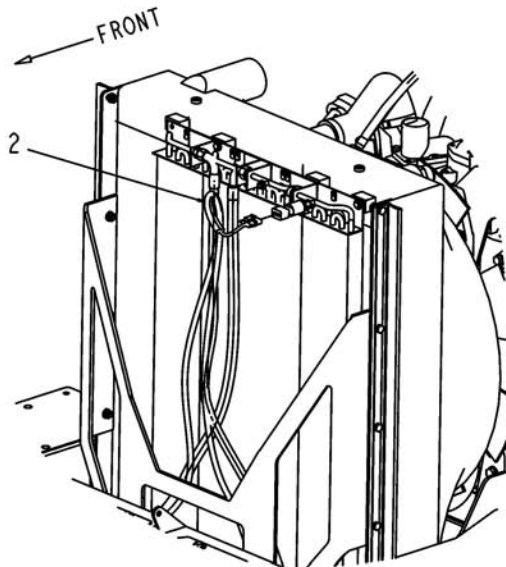
DETAIL P
