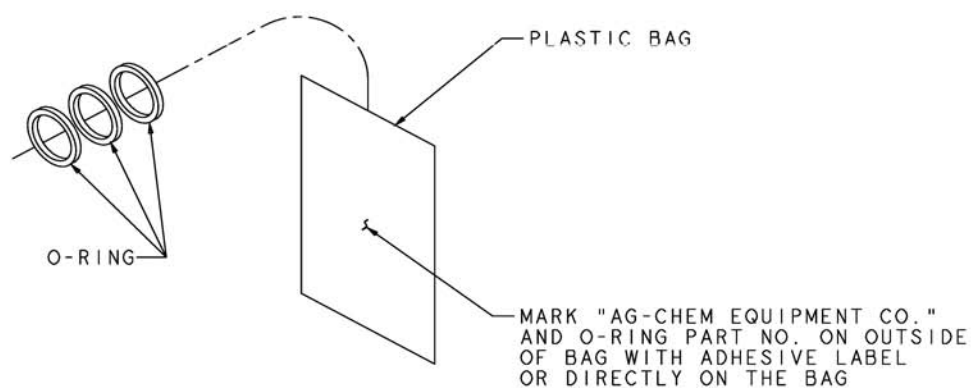
DETAIL A
