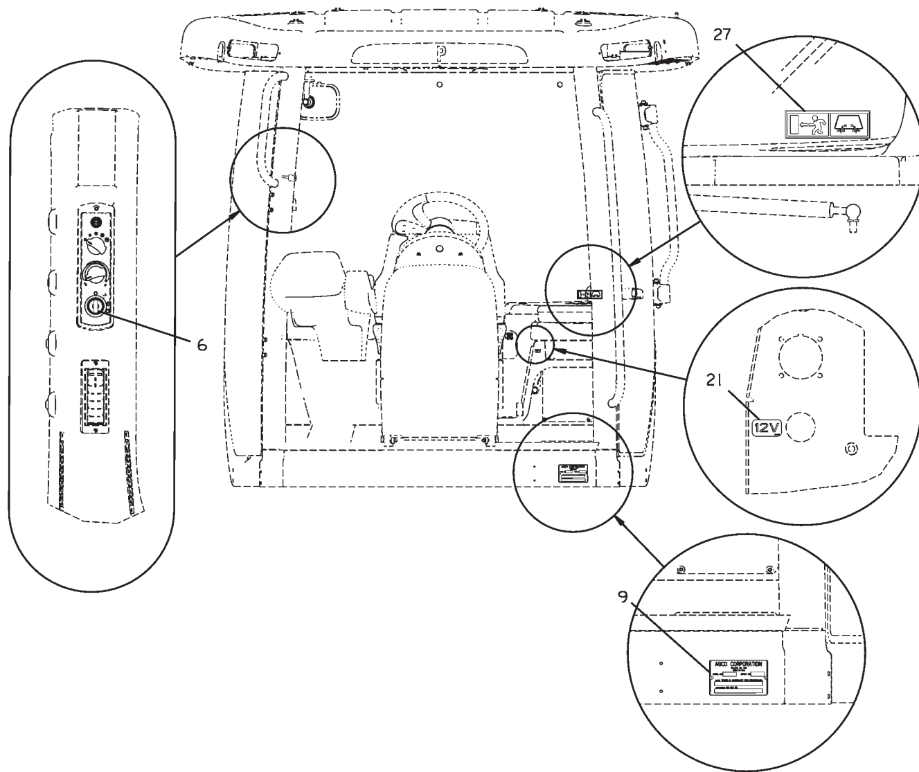
FRONT VIEW OF CAB
