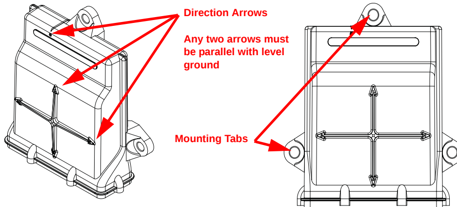
FIGURE 2. Node Mounting
