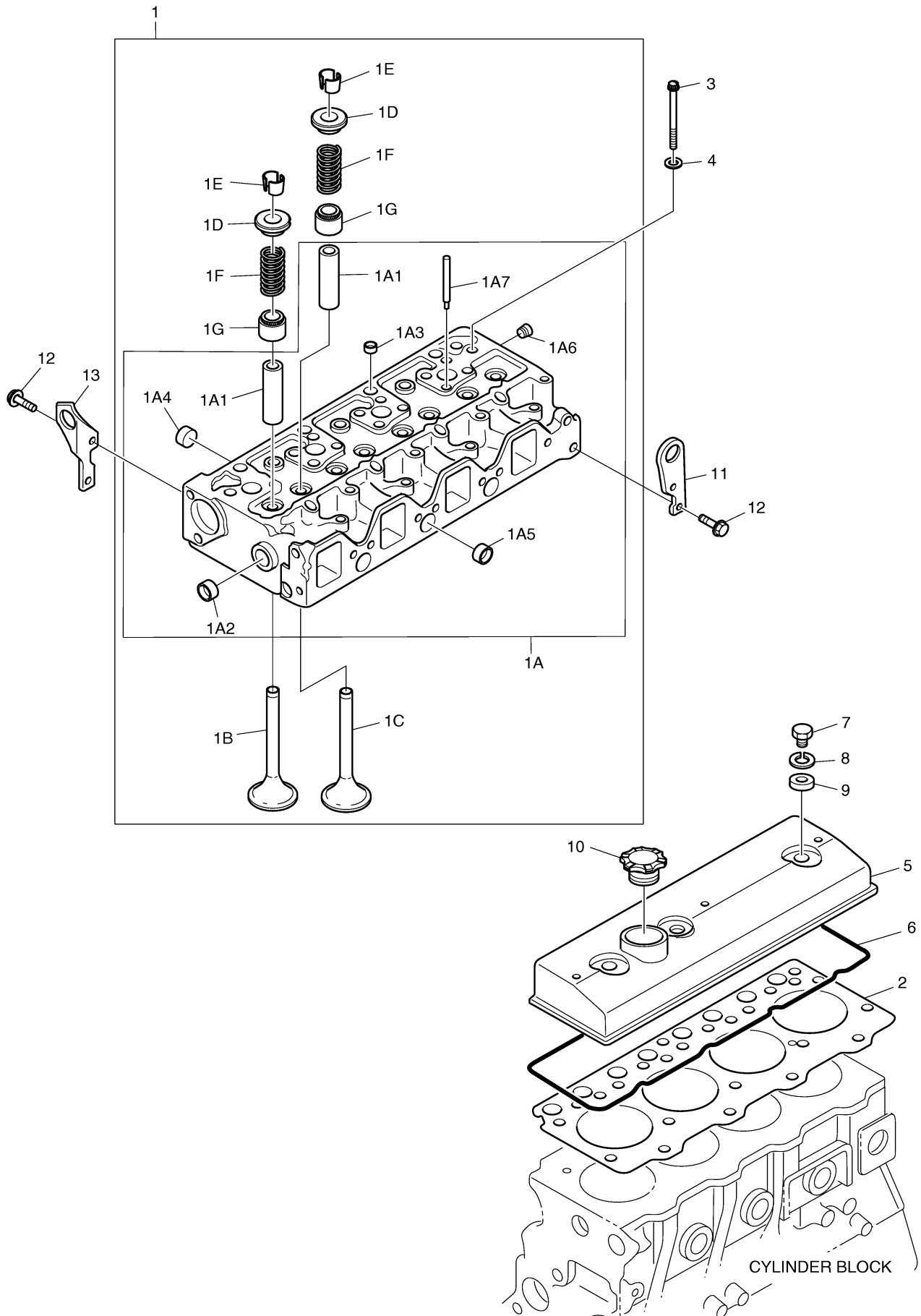
Fig. 001 CYLINDER HEAD & COVER
