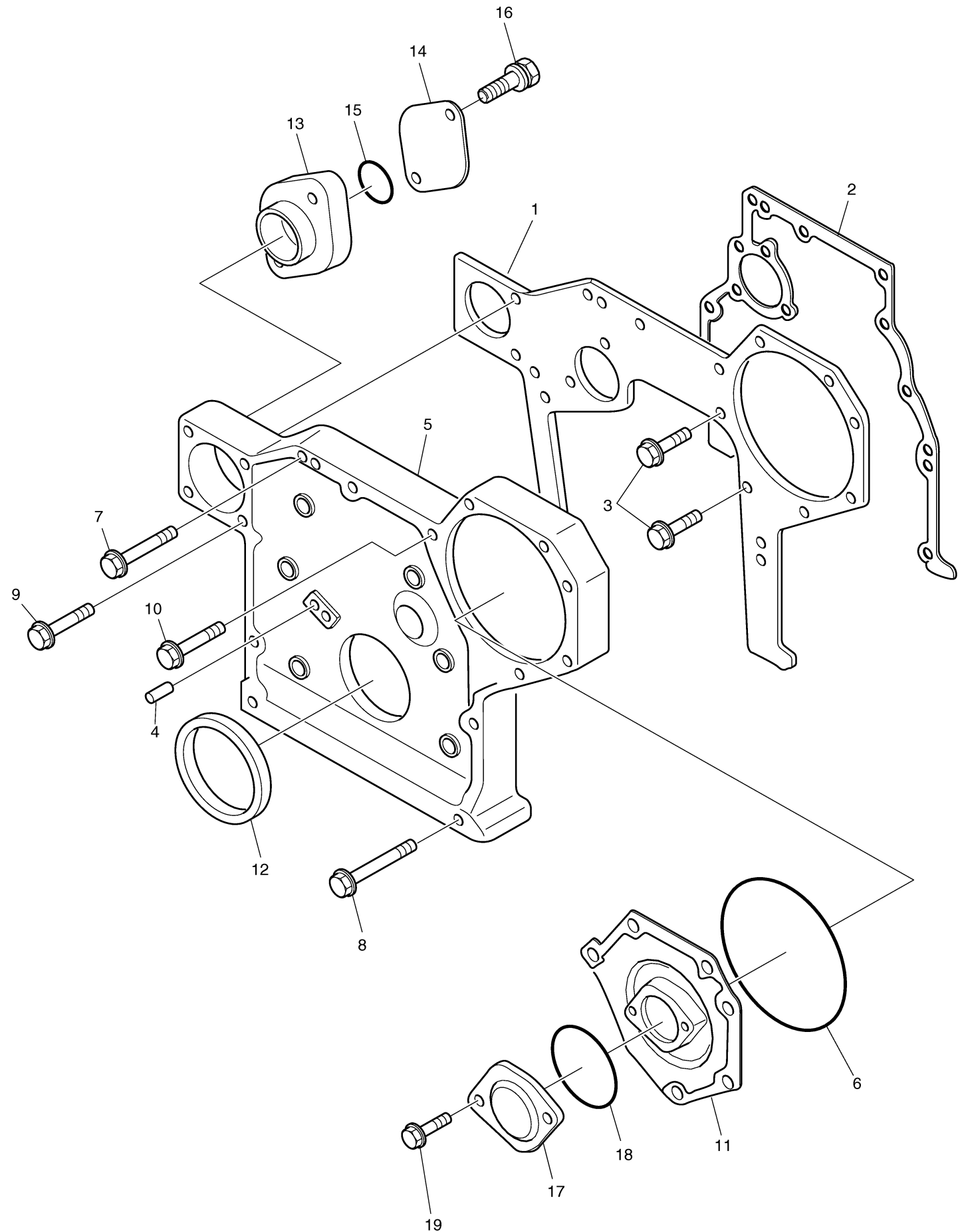
Fig. 003 TIMING GEAR CASE
