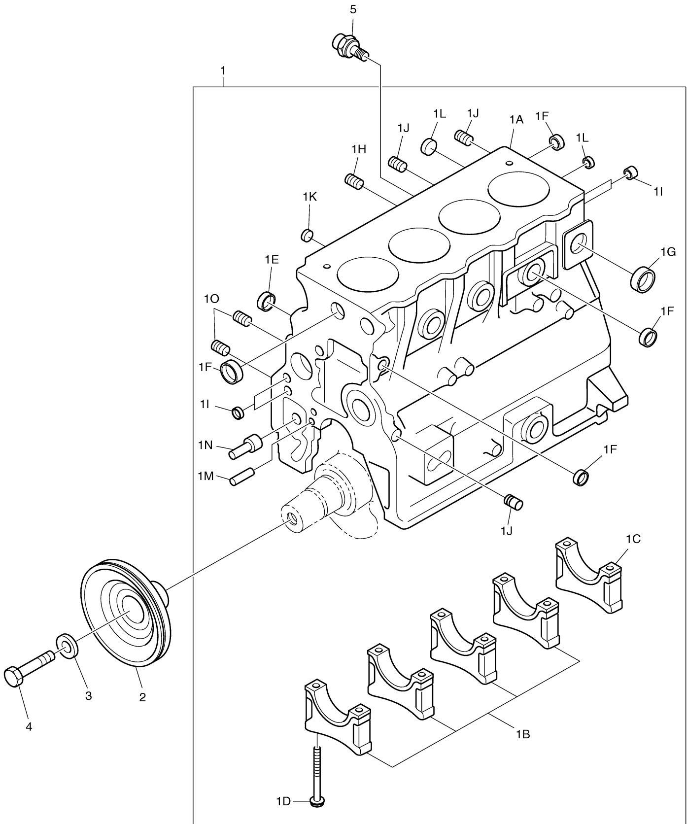
Fig. 002 CYLINDER BLOCK
