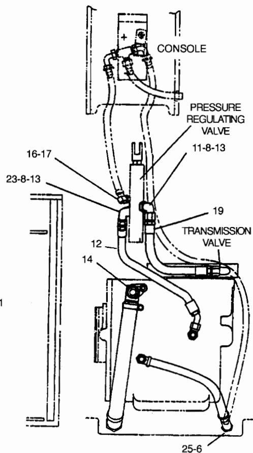
REAR VIEW
