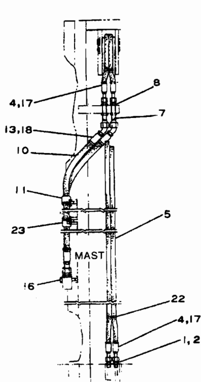
REAR VIEW
