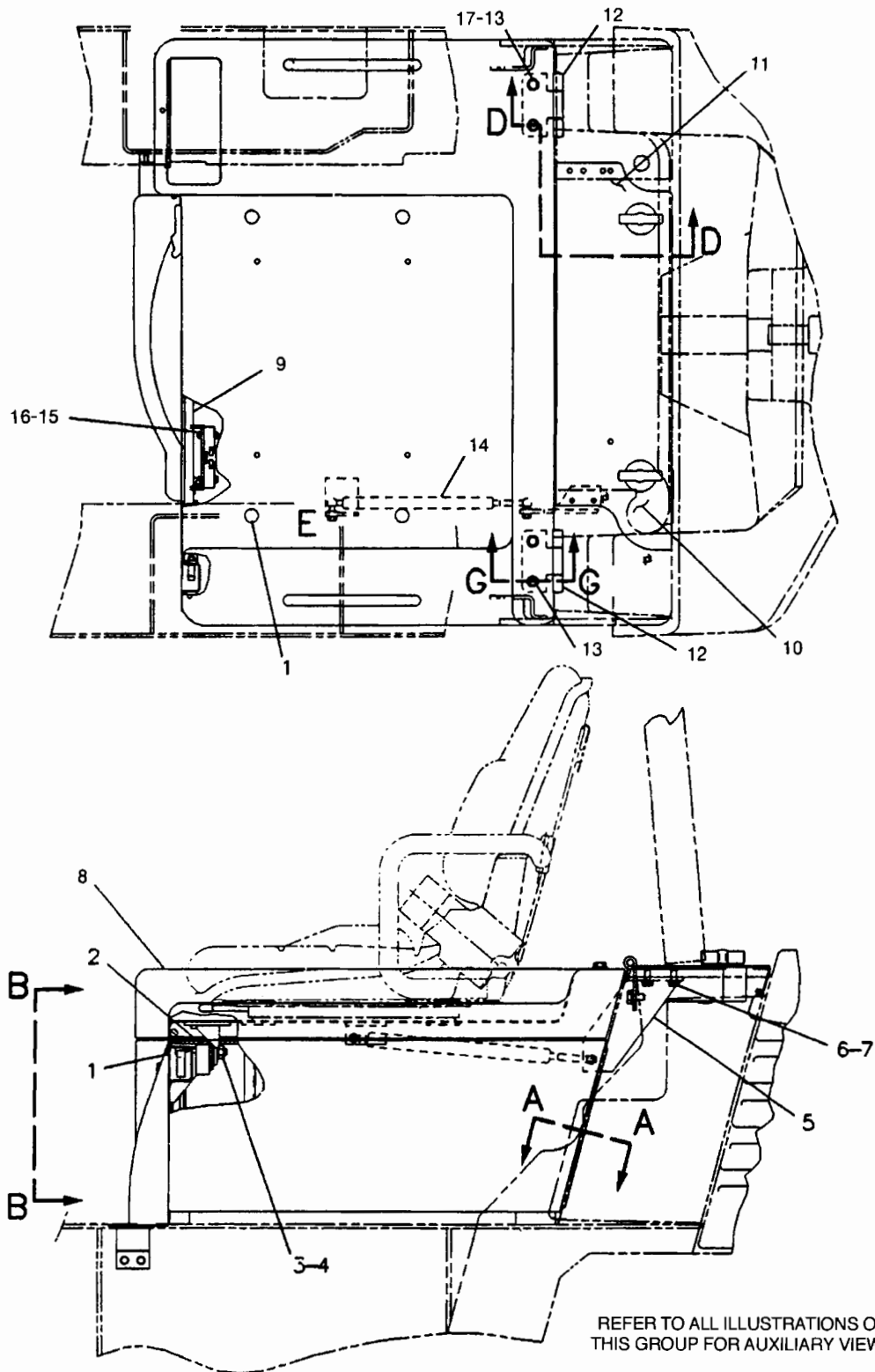
D130694 PANEL GP - TOP - PART 1 OF 2
