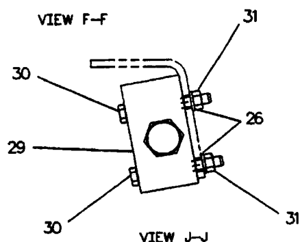
VIEW J-J
