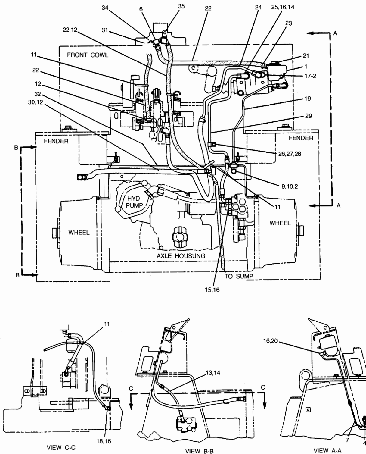
D130534-01 LINES GP - BRAKE (DISC) Refer To Fig.9.09
