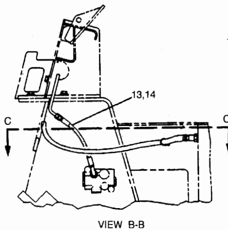
D130535-01 LINES GP - SERVICE BRAKE (SHOE) Refer To Fig.9.10
