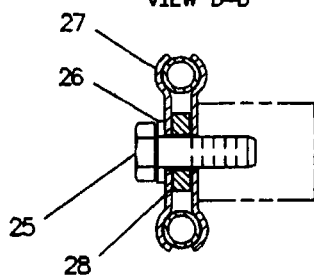
SECTION E-E
