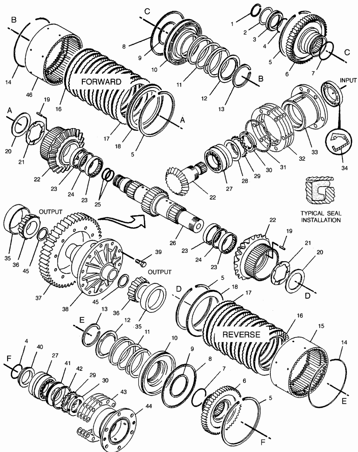
D141127 GEAR GP - FORWARD & REVERSE Part Of D141132 Transmission Ar
