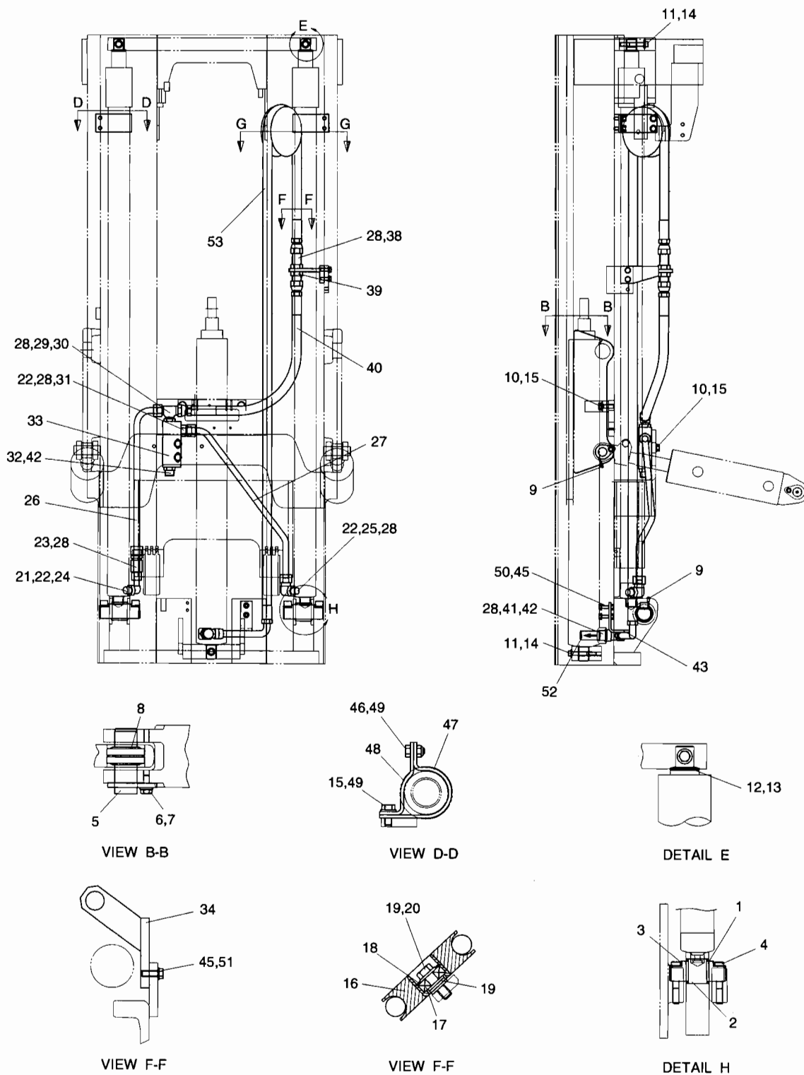
A216101 MOUNTING GP - LIFT & TILT(FFT) Refer To Type1 - Fig.12.25, Fig.12.26
