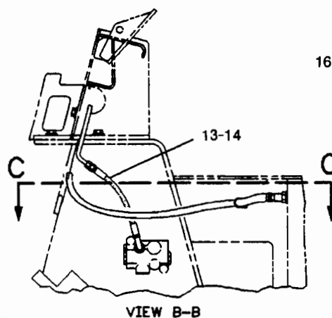
D130535 LINES GP - SERVICE BRAKE (SHOE) Refer To Fig.9.101
