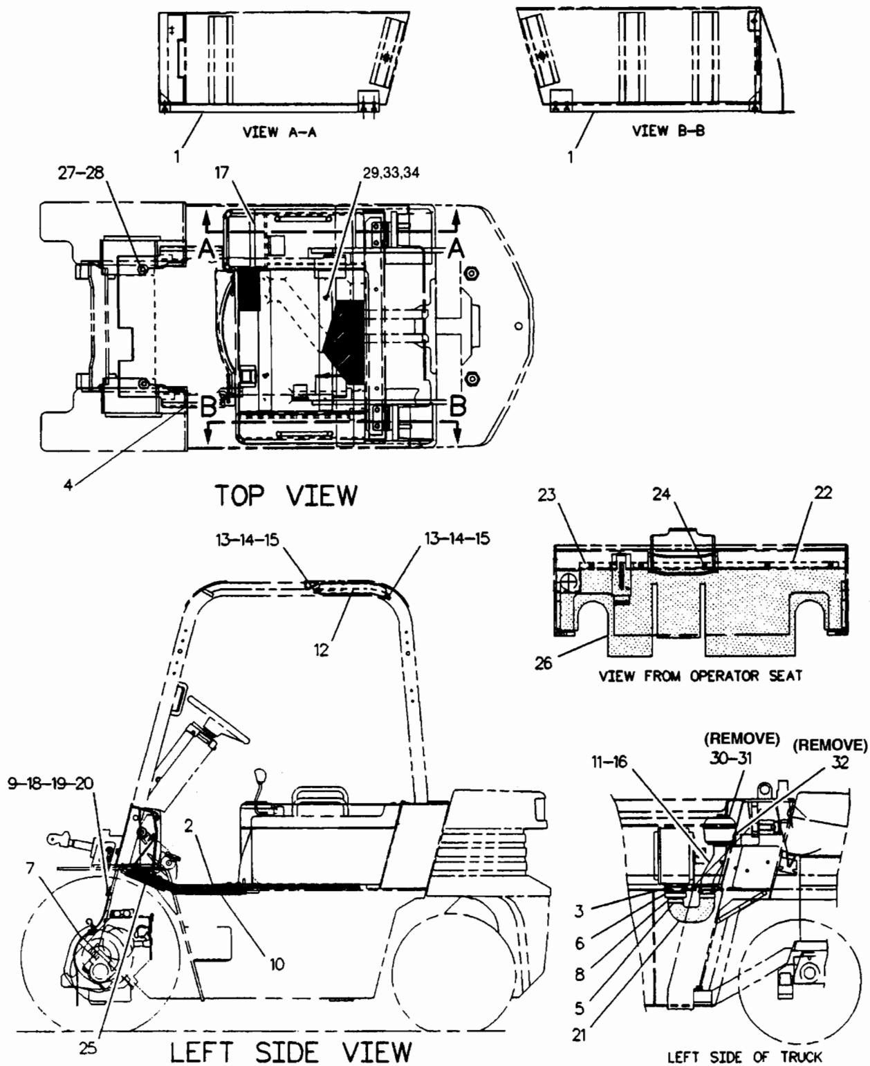
D130954 CHANGEOVER AR - SOUND SUPPRESSION An Attachment
