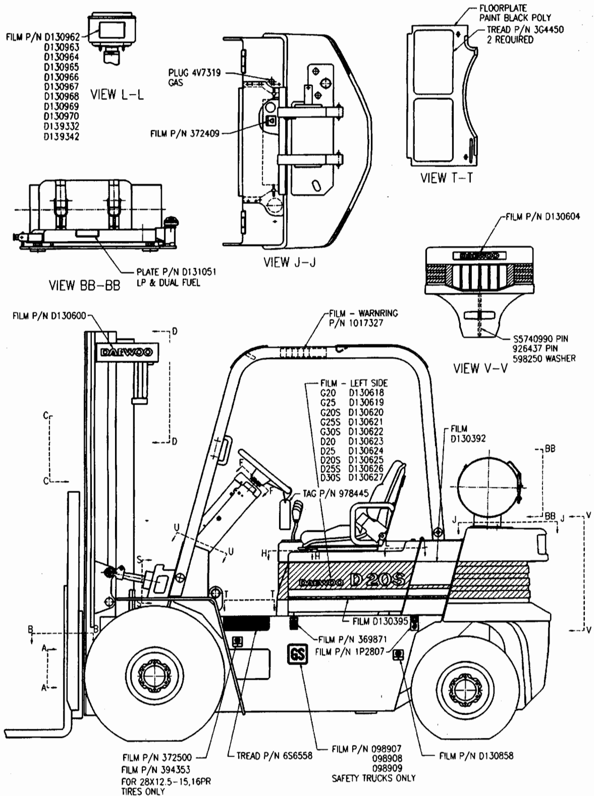
D130486-01 PAINT & LUBRICANT GP - PART 1 OF 4
