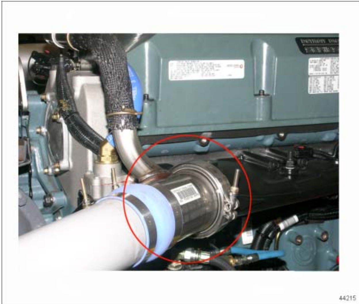
Figure 2-14 EGR Mixer
