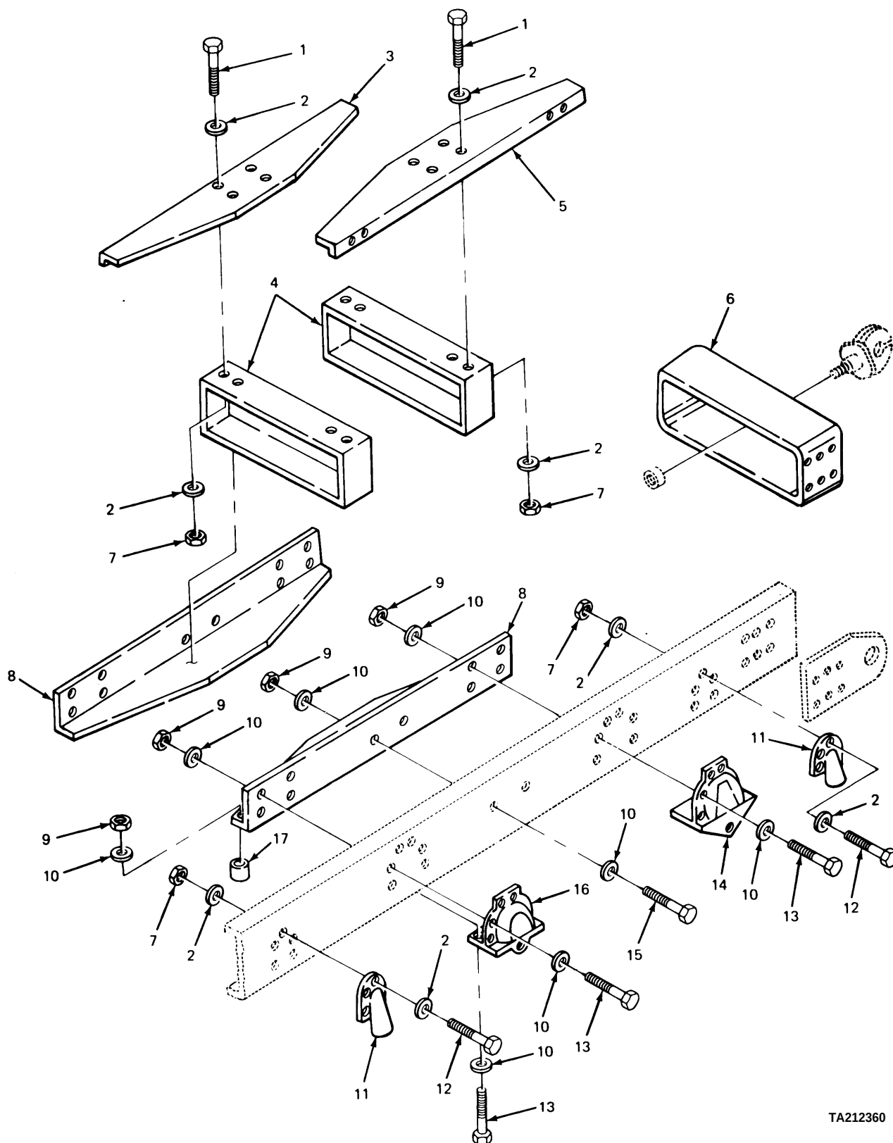
FIGURE 233. CROSSMEMBER, GUSSETS AND RELATED PARTS.
