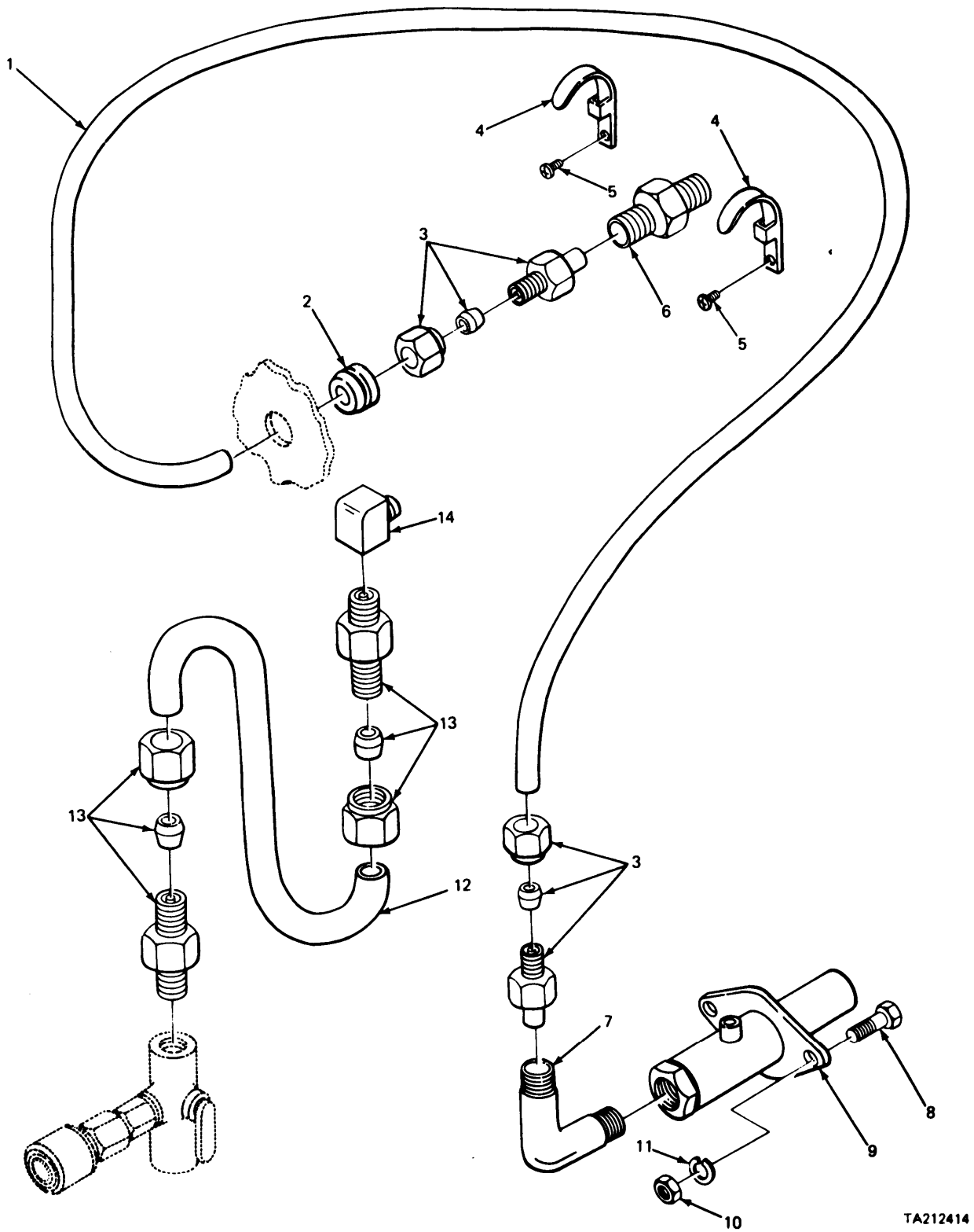
FIGURE 288. SUPPLY VALVE AIR CONNECTORS AND RELATED PARTS.
