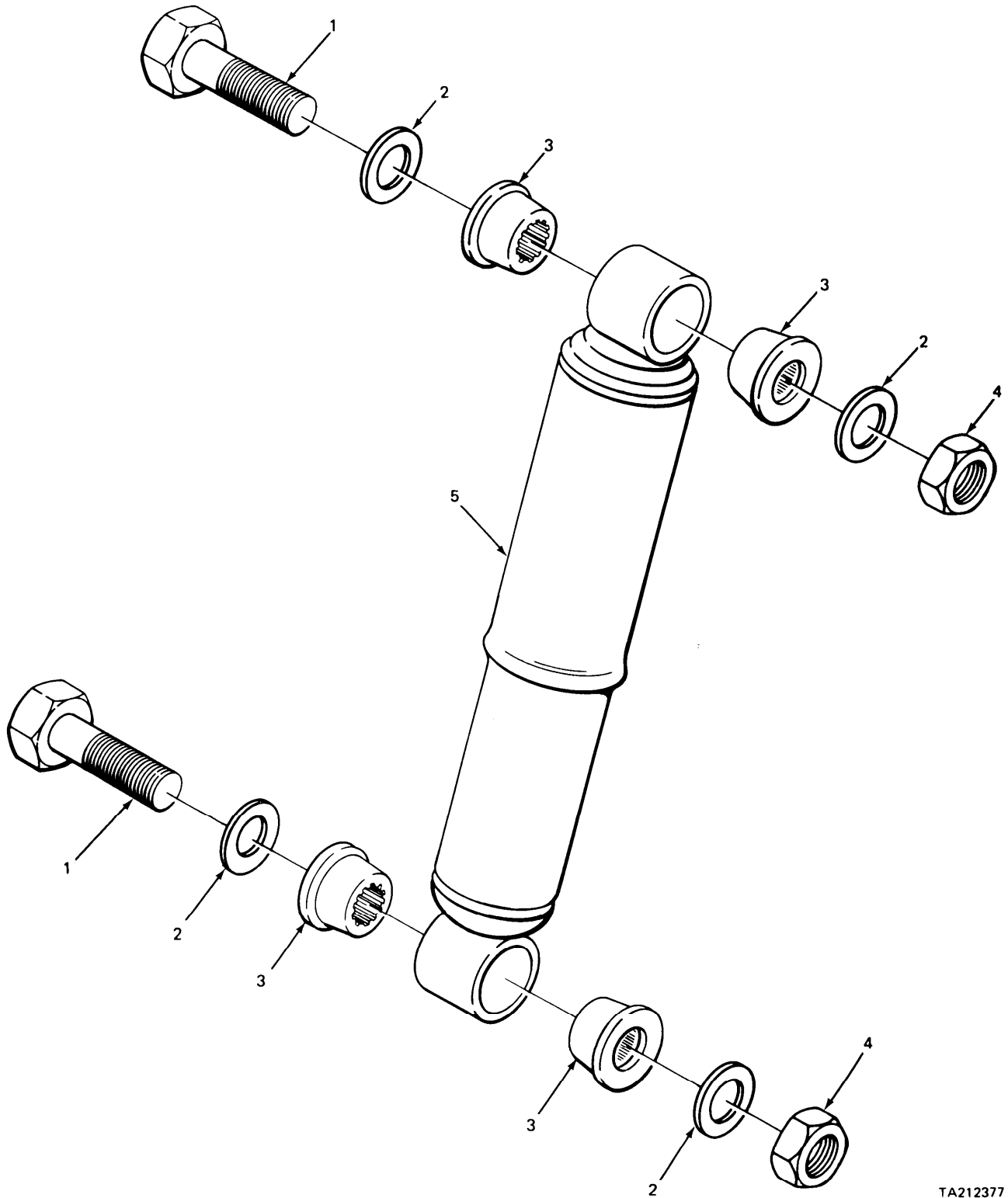
FIGURE 249. SHOCK ABSORBER.
