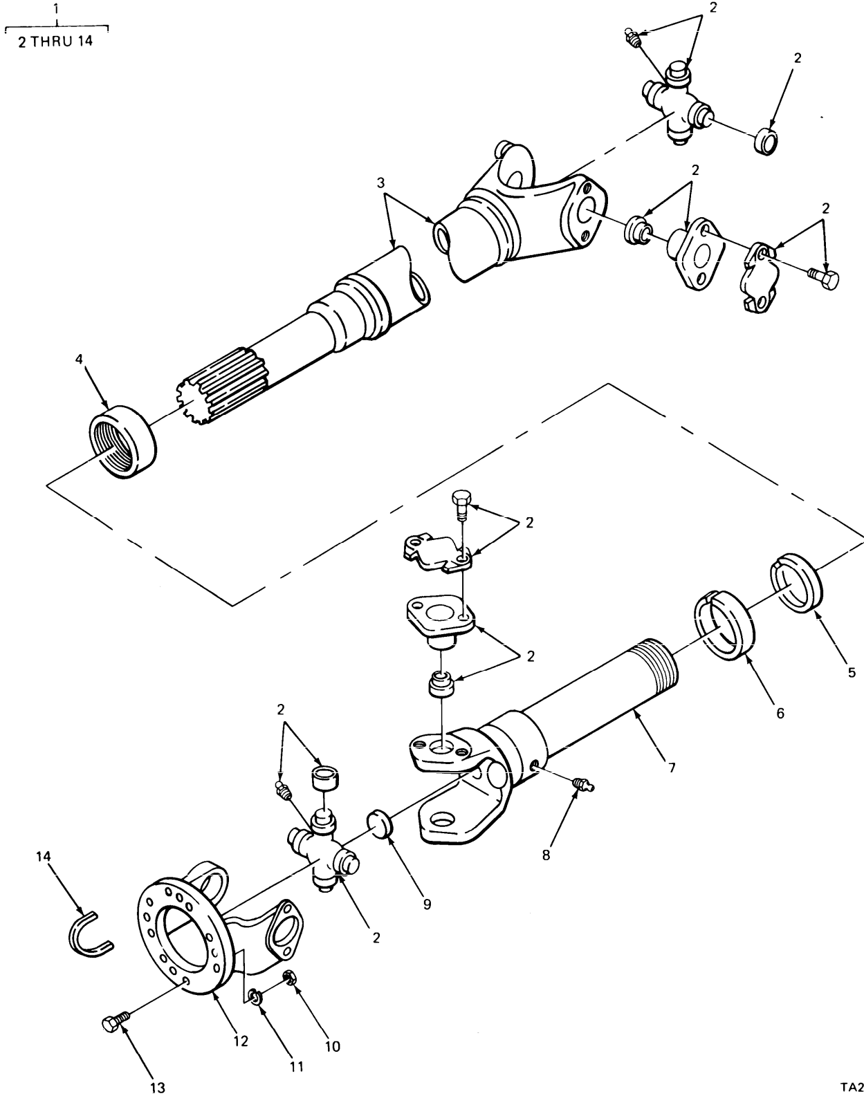
FIGURE 144. PROPELLER SHAFTS AND RELATED PARTS.
