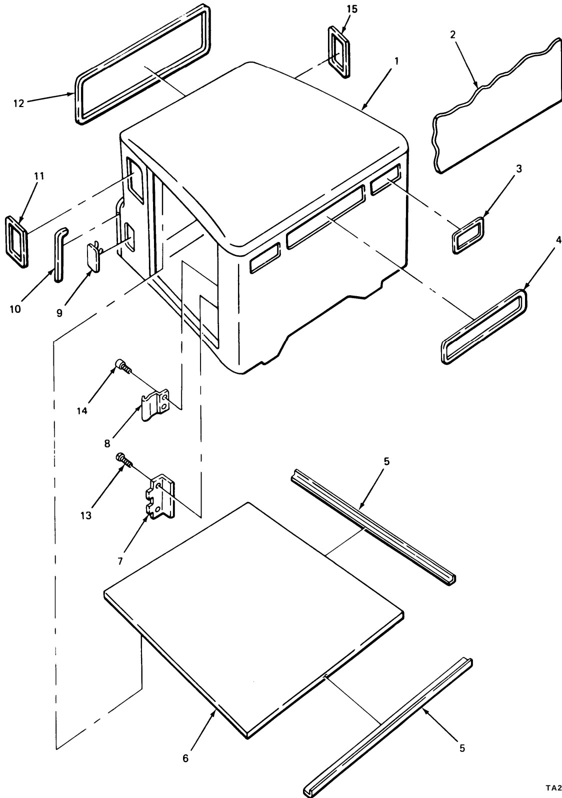
FIGURE 255. CAB ASSEMBLY.
