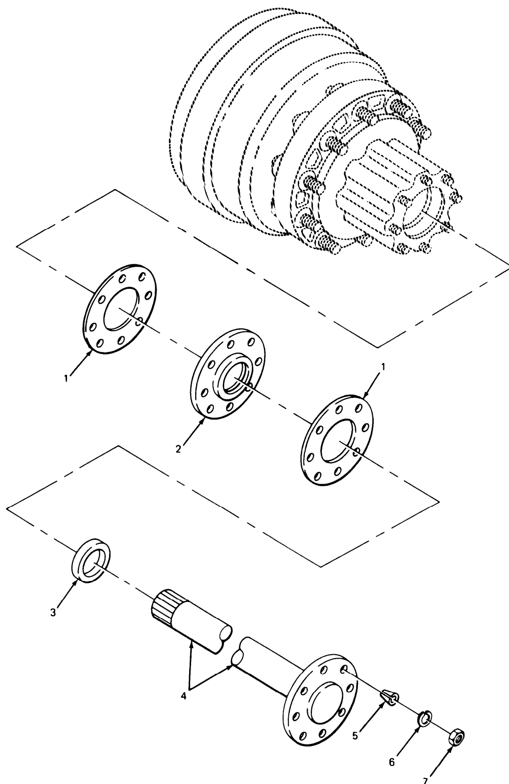
FIGURE 151. AXLE SHAFT AND RELATED PARTS.
