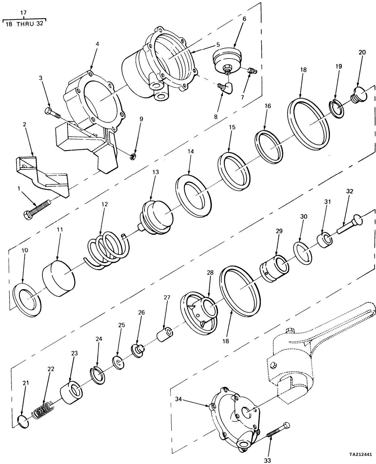
FIGURE 246. VALVE HANDLE EXPLODED VIEW.
