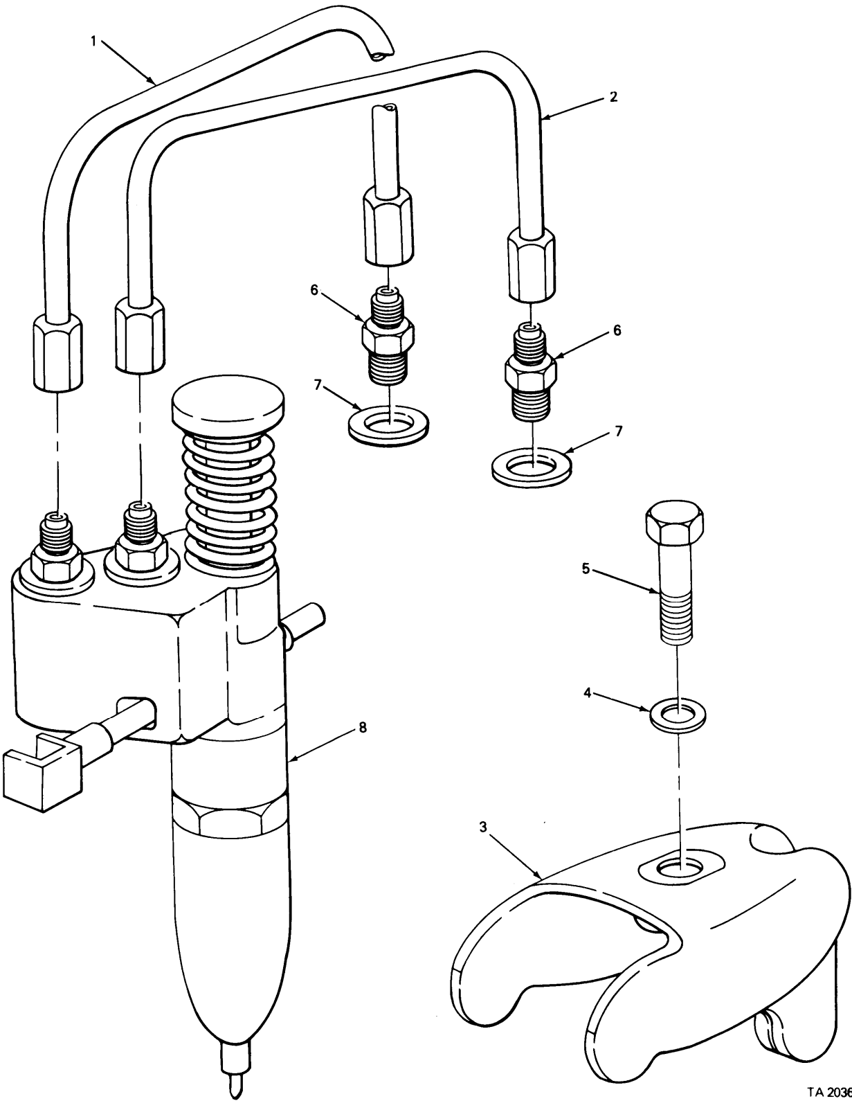
FIGURE 33. FUEL INJECTOR ASSEMBLY.
