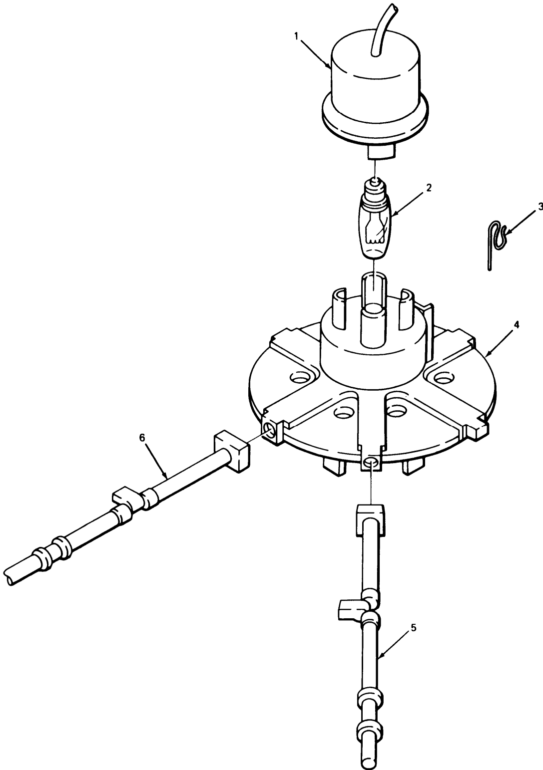
FIGURE 98. LAMPHOLDER, OPTICAL RIBBON, AND RELATED PARTS.
