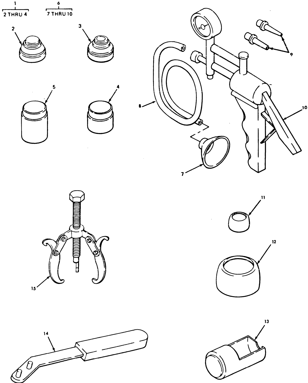
FIGURE 309. GENERAL SUPPORT SPECIAL TOOLS.
