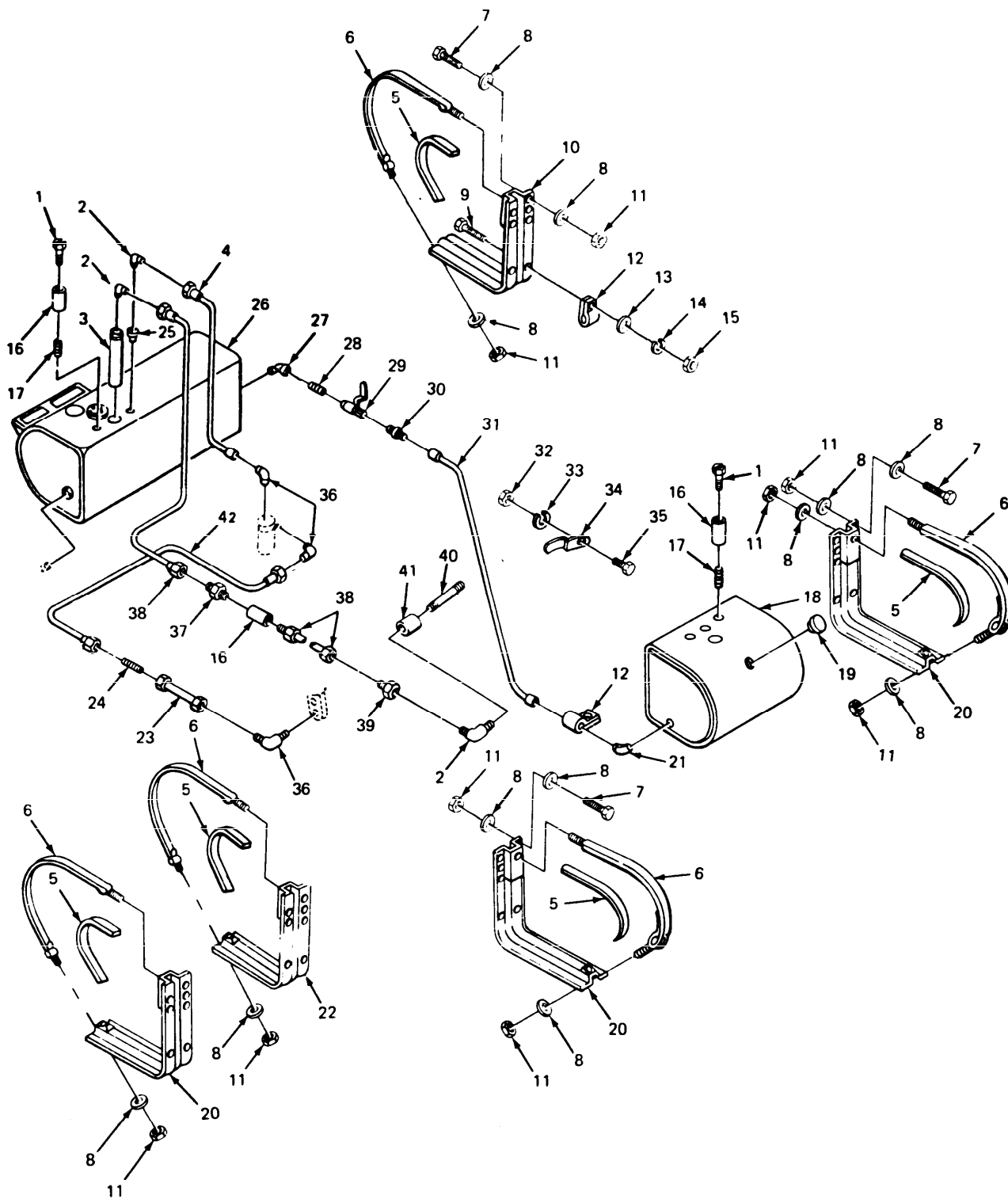
FIGURE 45. FUEL TANK, LINES AND FITTINGS.
