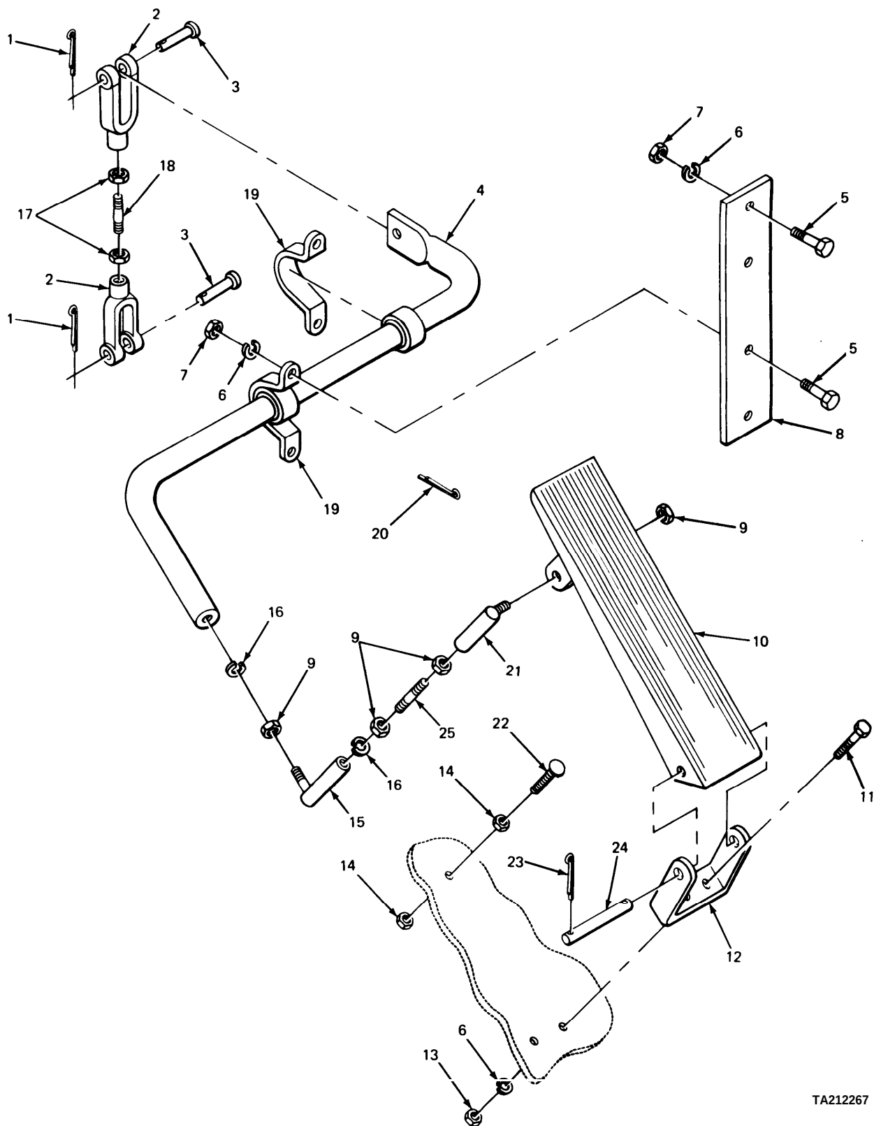
FIGURE 125. TRANSMISSION RETARDER CONTROL PEDAL AND RELATED PARTS.
