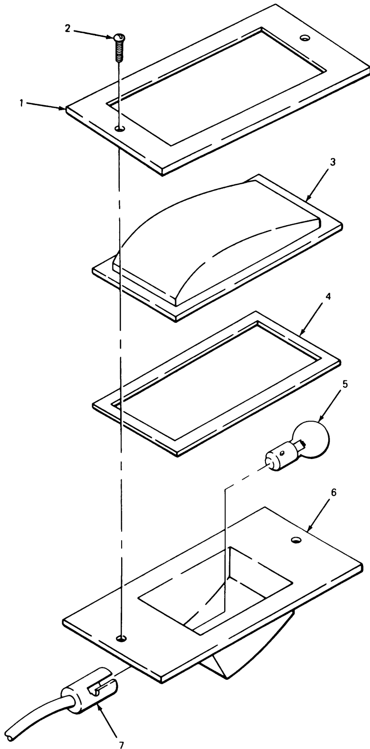
FIGURE 82. DOME LIGHT.
