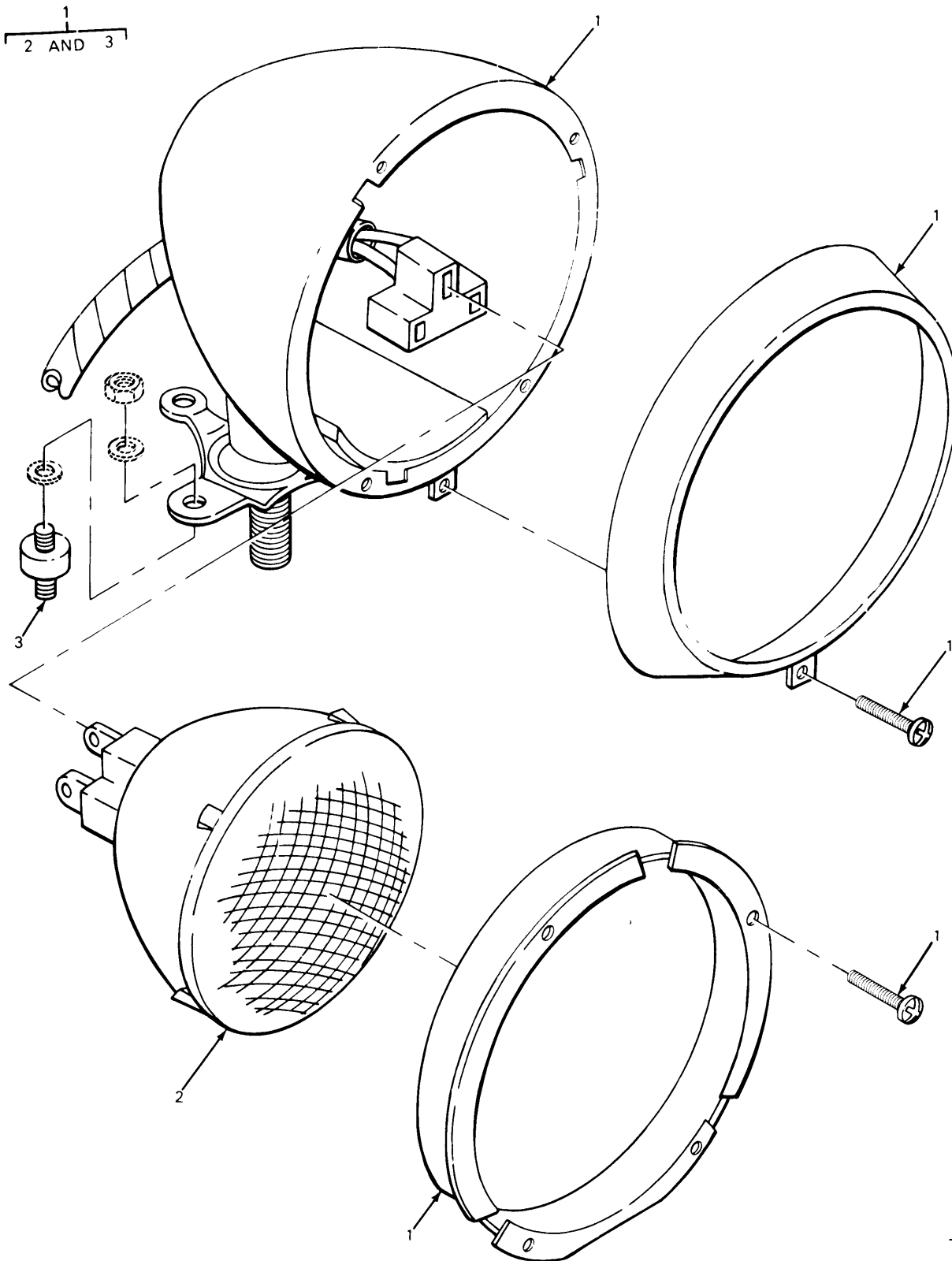
FIGURE 85. HEADLIGHT ASSEMBLY.
