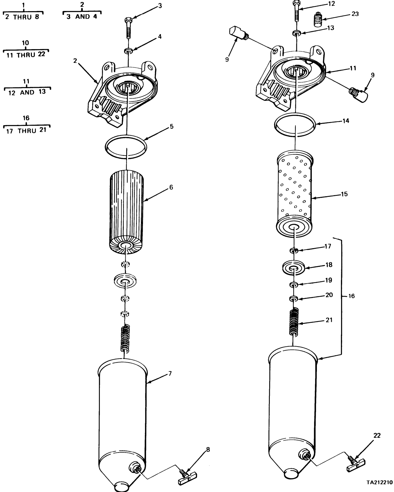
FIGURE 54. PRIMARY AND SECONDARY FUEL FILTERS (REPLACEABLE ELEMENT TYPE).
