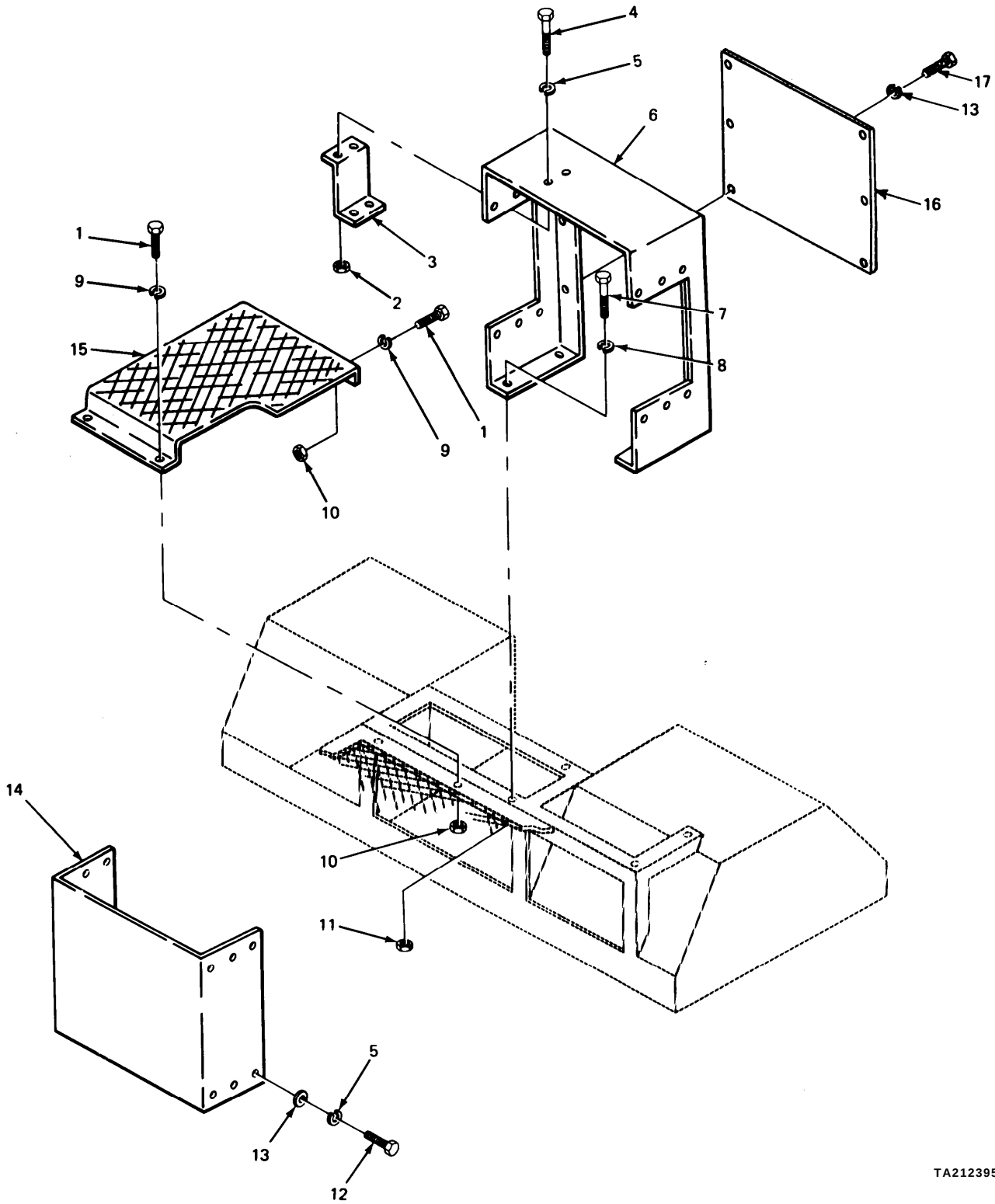
FIGURE 269. CONSOLE PANEL AND RELATED PARTS.
