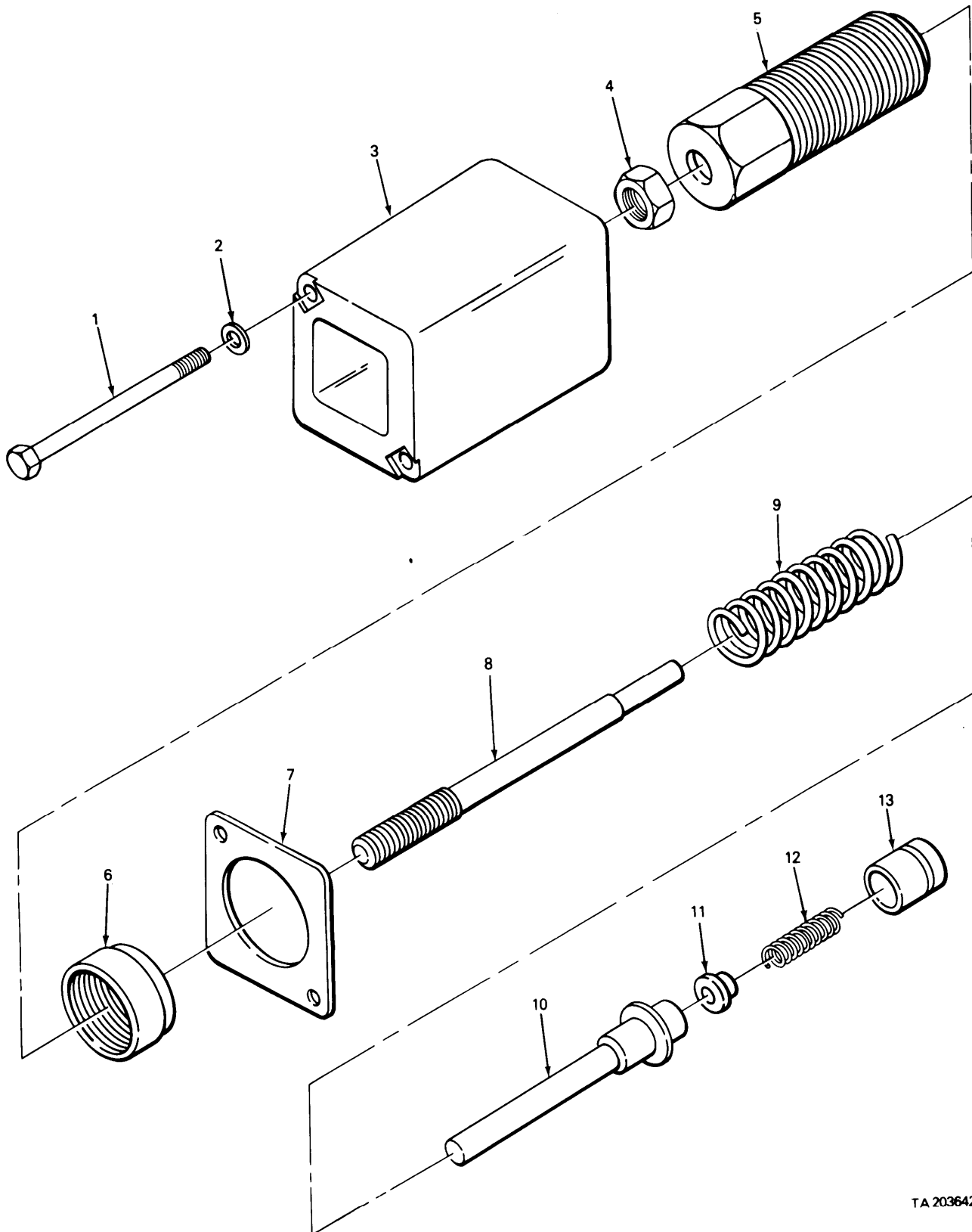
FIGURE 51. GOVERNOR SPRING AND RELATED PARTS.
