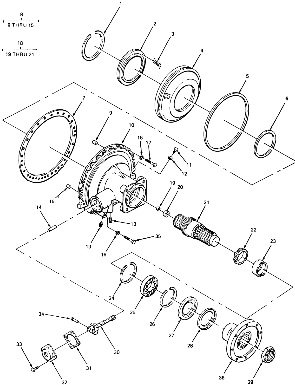
FIGURE 118. FIRST CLUTCH AND RELATED PARTS.
