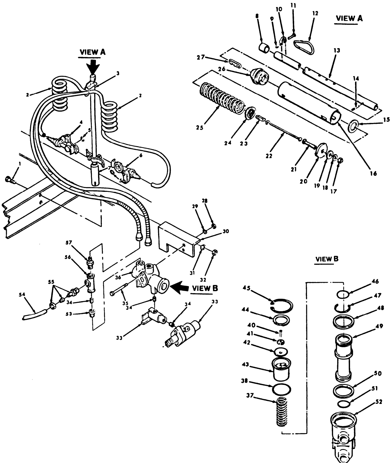
FIGURE 203. TRAILER HOSE ASSEMBLY.
