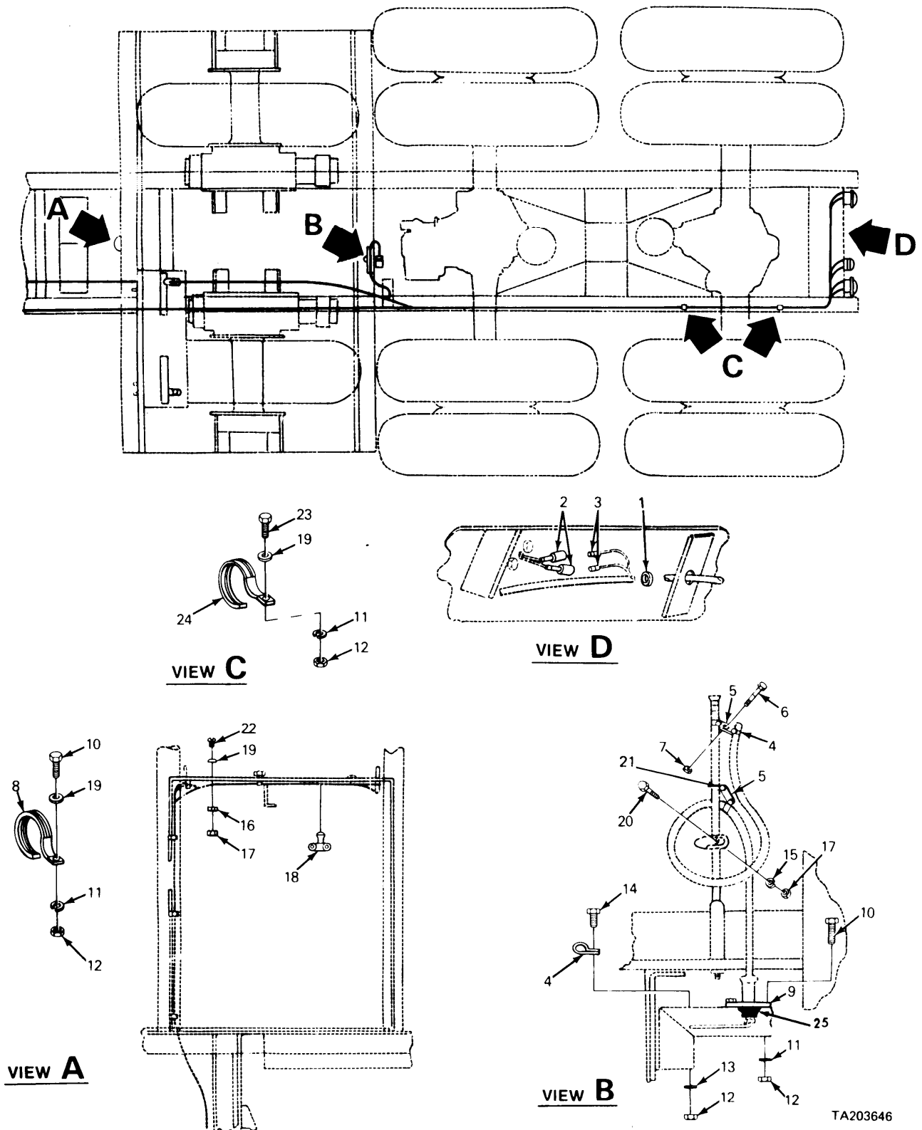
FIGURE 101. CHASSIS WIRING HARNESS (REAR SECTION).
