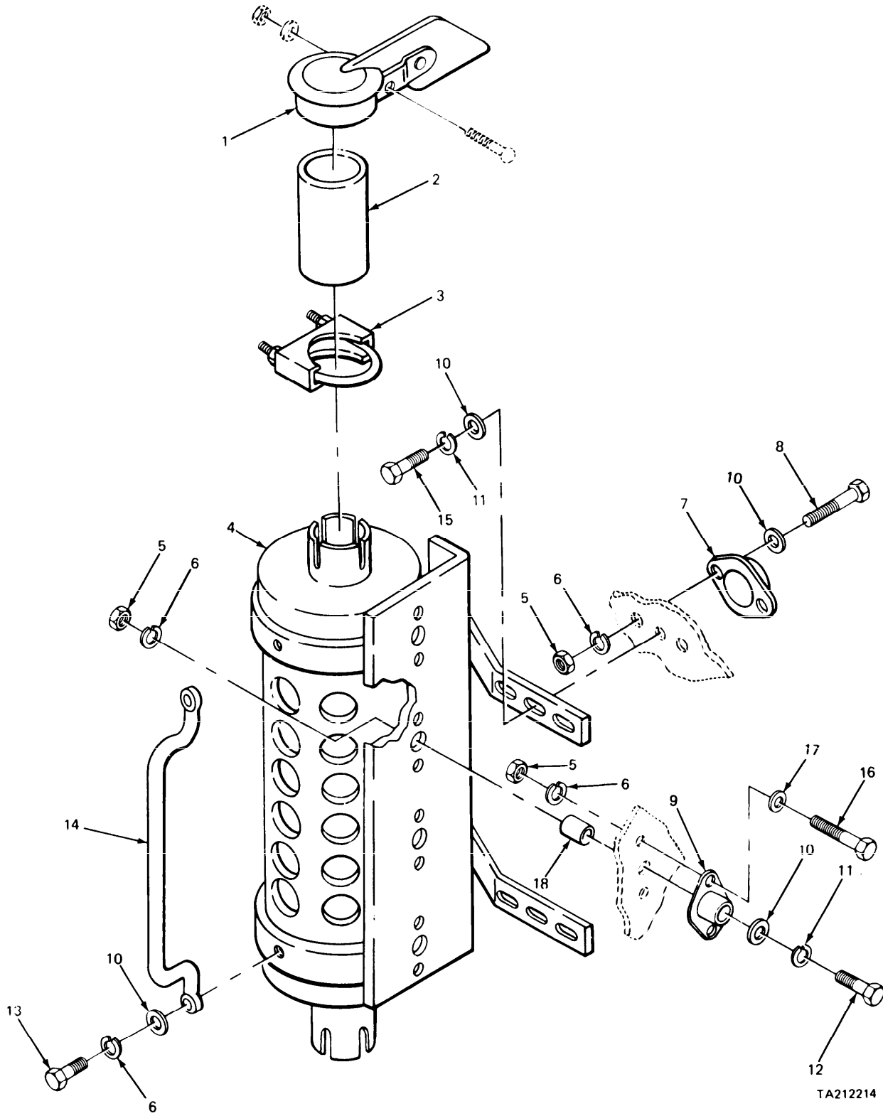
FIGURE 58. MUFFLER AND RELATED PARTS.
