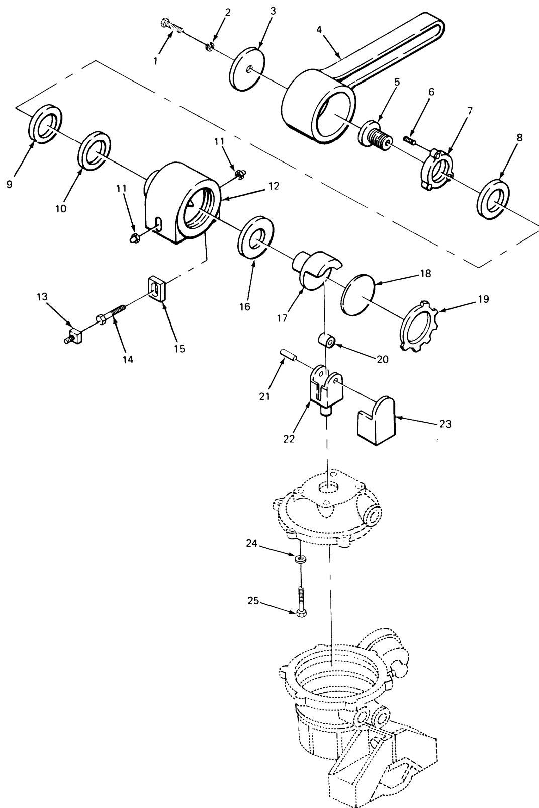
FIGURE 245. VALVE HANDLE AND RELATED PARTS.
