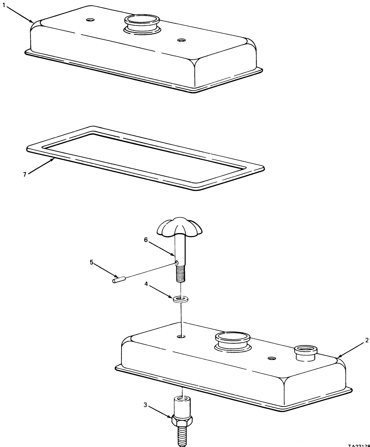
FIGURE 19. ROCKER COVERS AND RELATED PARTS FOR THE EARLY T ENGINE.
