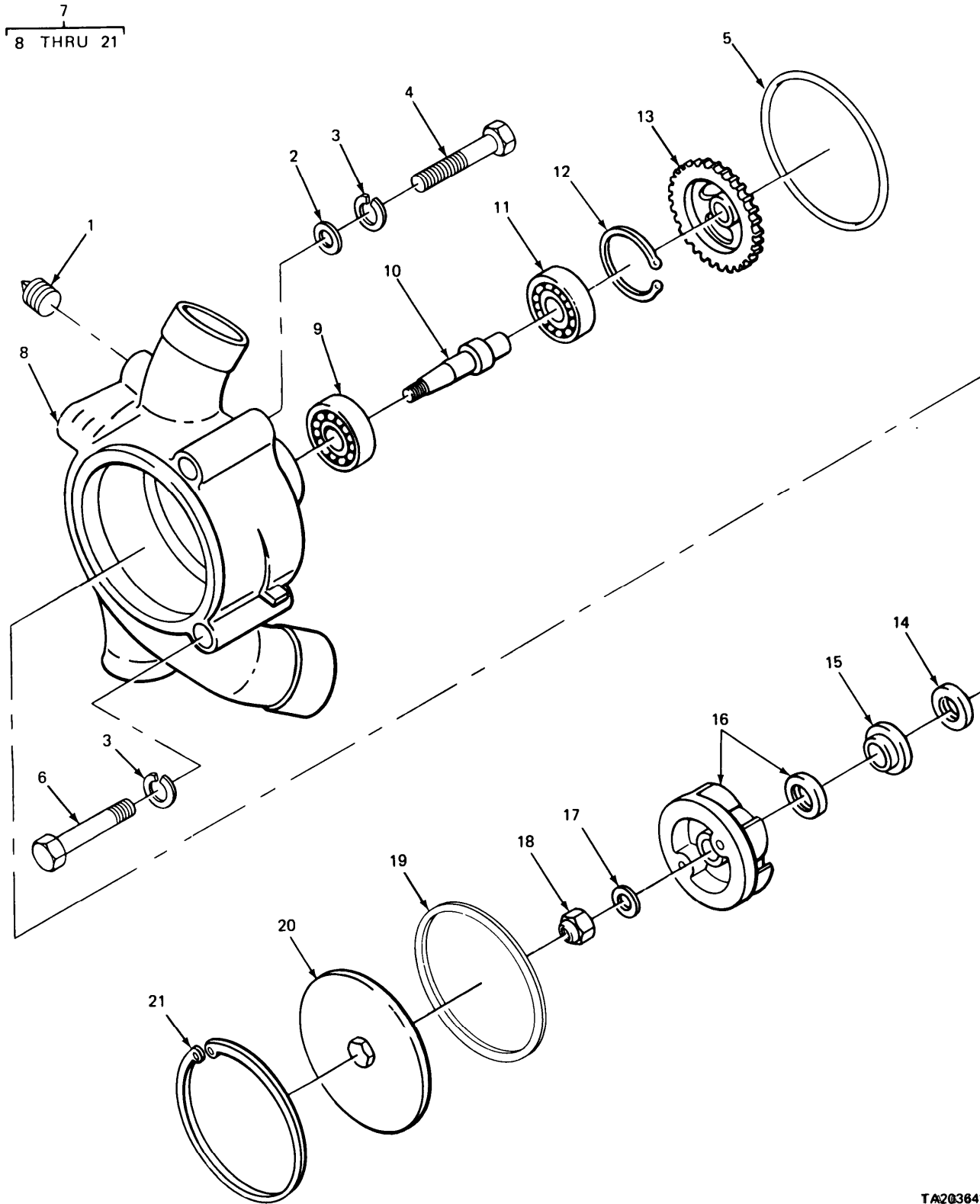
FIGURE 67. WATER PUMP.
