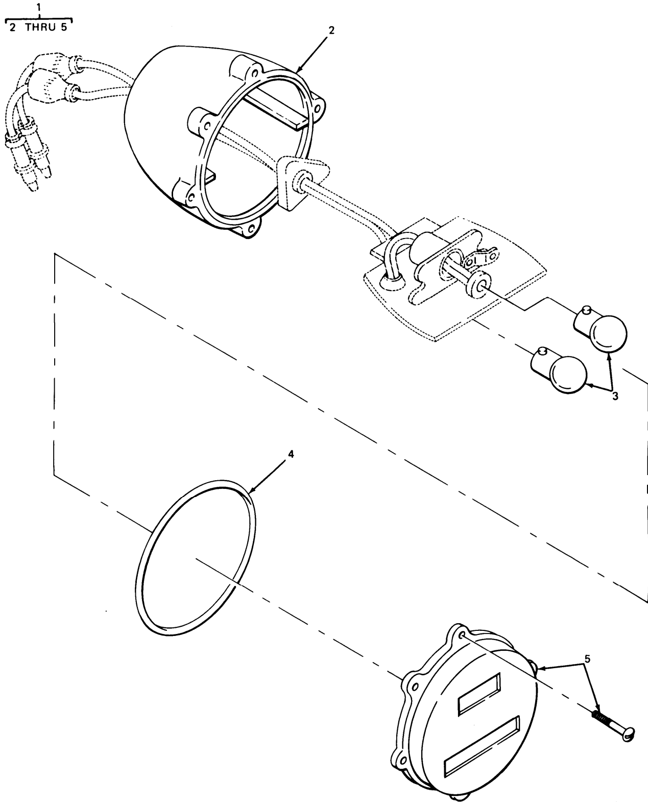
FIGURE 91. BLACKOUT TAILLIGHT.
