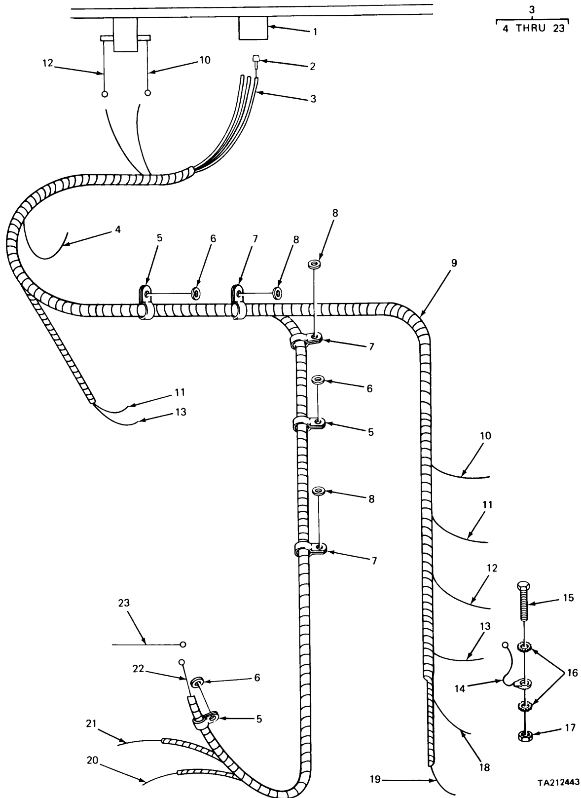
FIGURE 99. ENGINE WIRING HARNESS.
