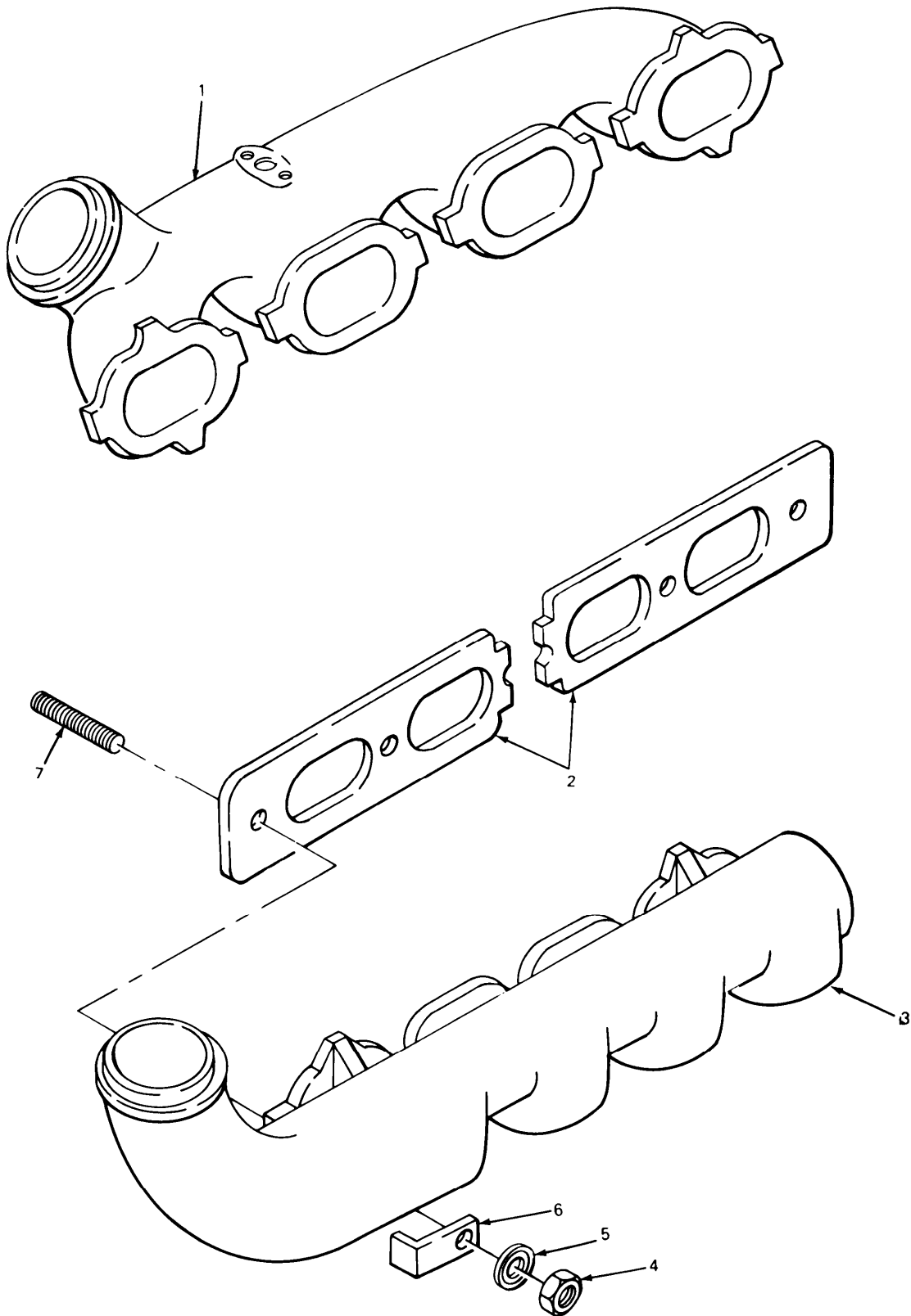
FIGURE 28. EXHAUST MANIFOLDS.
