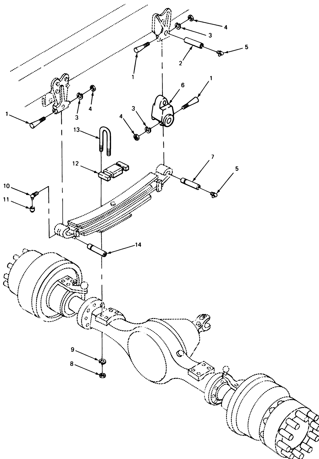
FIGURE 241. SPRING LINK AND PRESSURE PLATE FOR SPRINGS.
