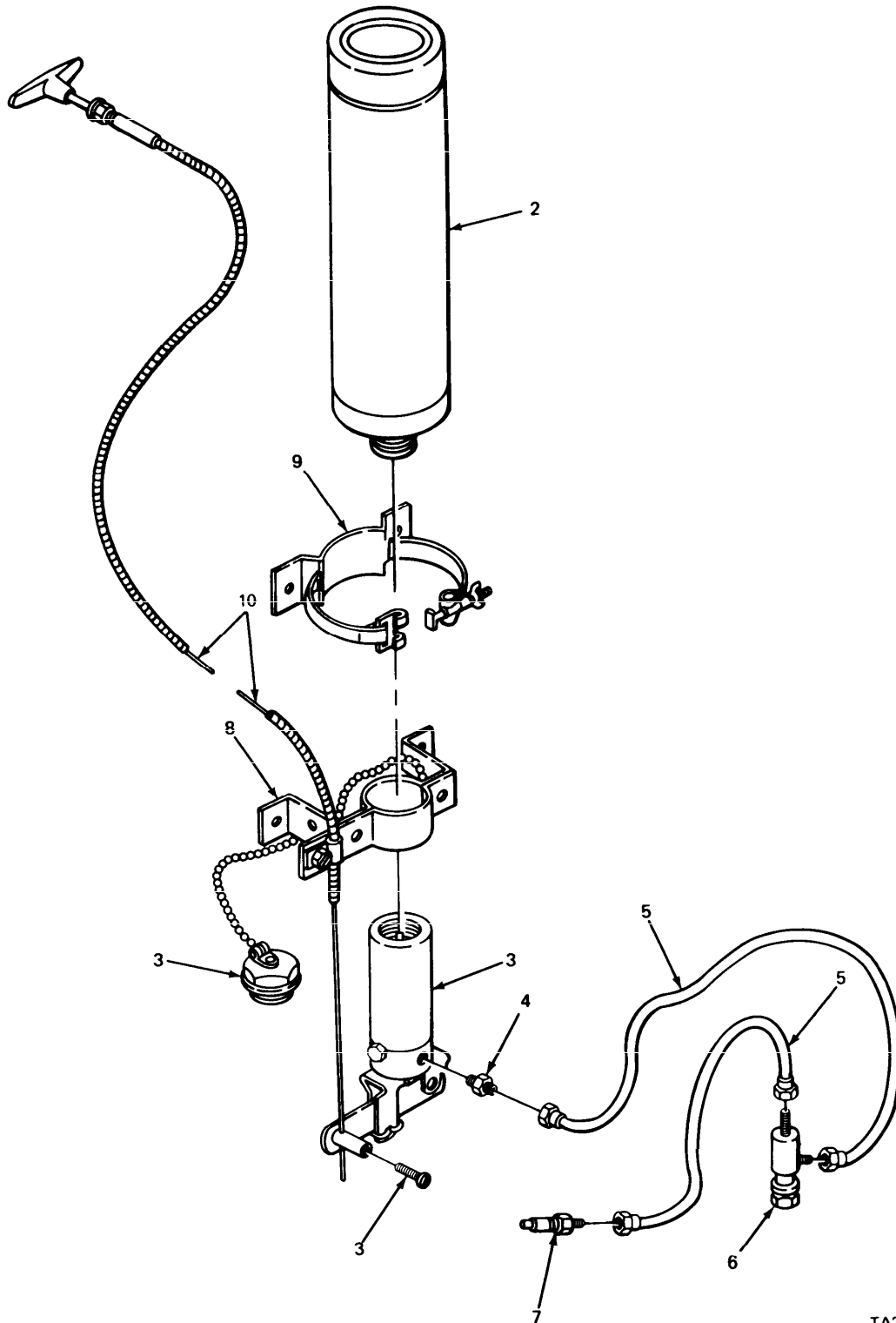
FIGURE 55. ENGINE FUEL PRIMER AND RELATED PARTS.
