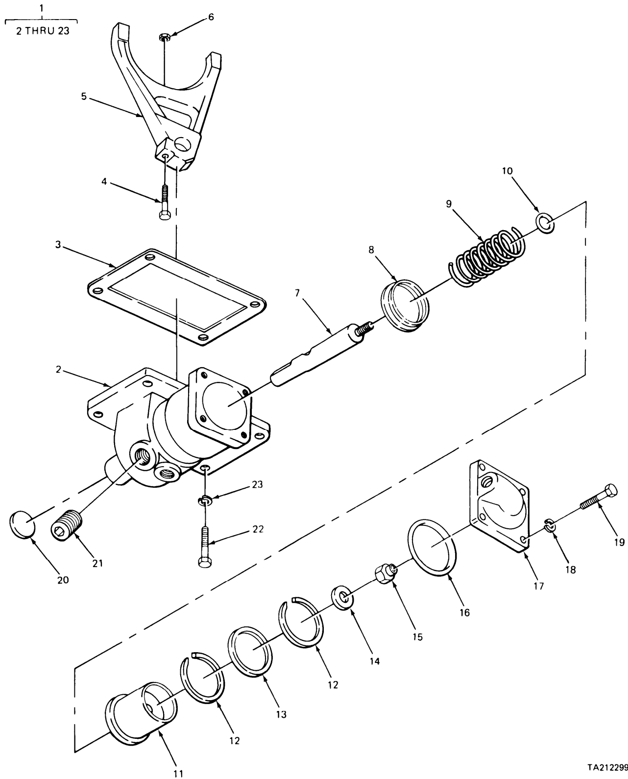
FIGURE 163. SHIFTER FORK AND RELATED PARTS.
