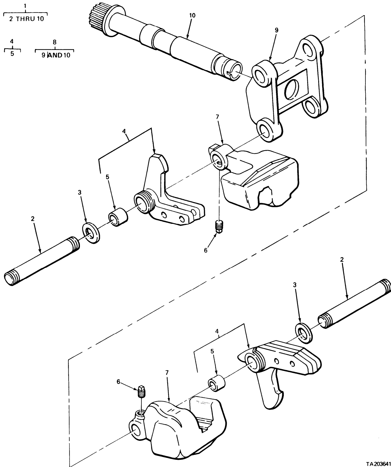
FIGURE 50. GOVERNOR WEIGHTS AND RELATED PARTS.
