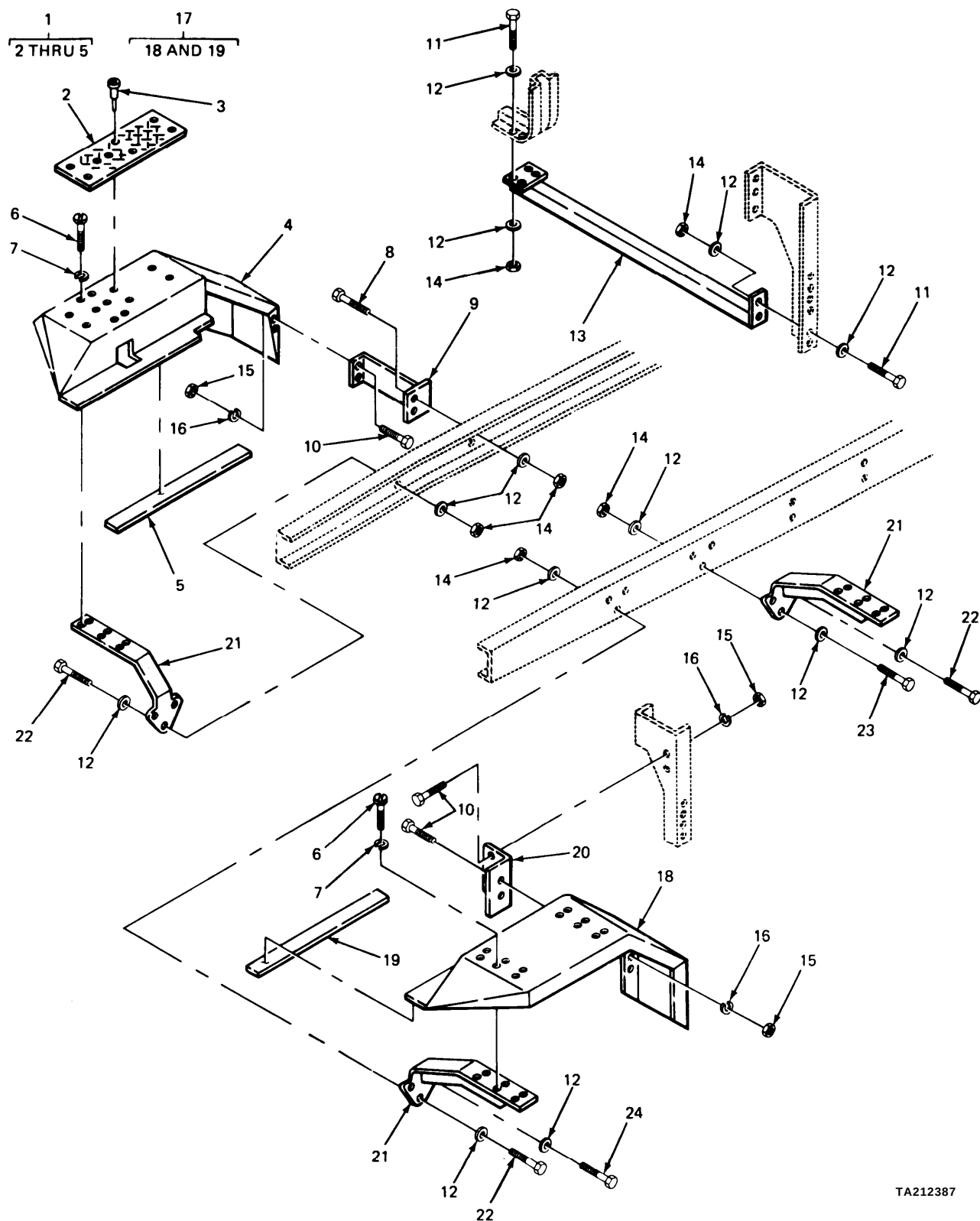
FIGURE 260. FENDER AND RELATED PARTS.
