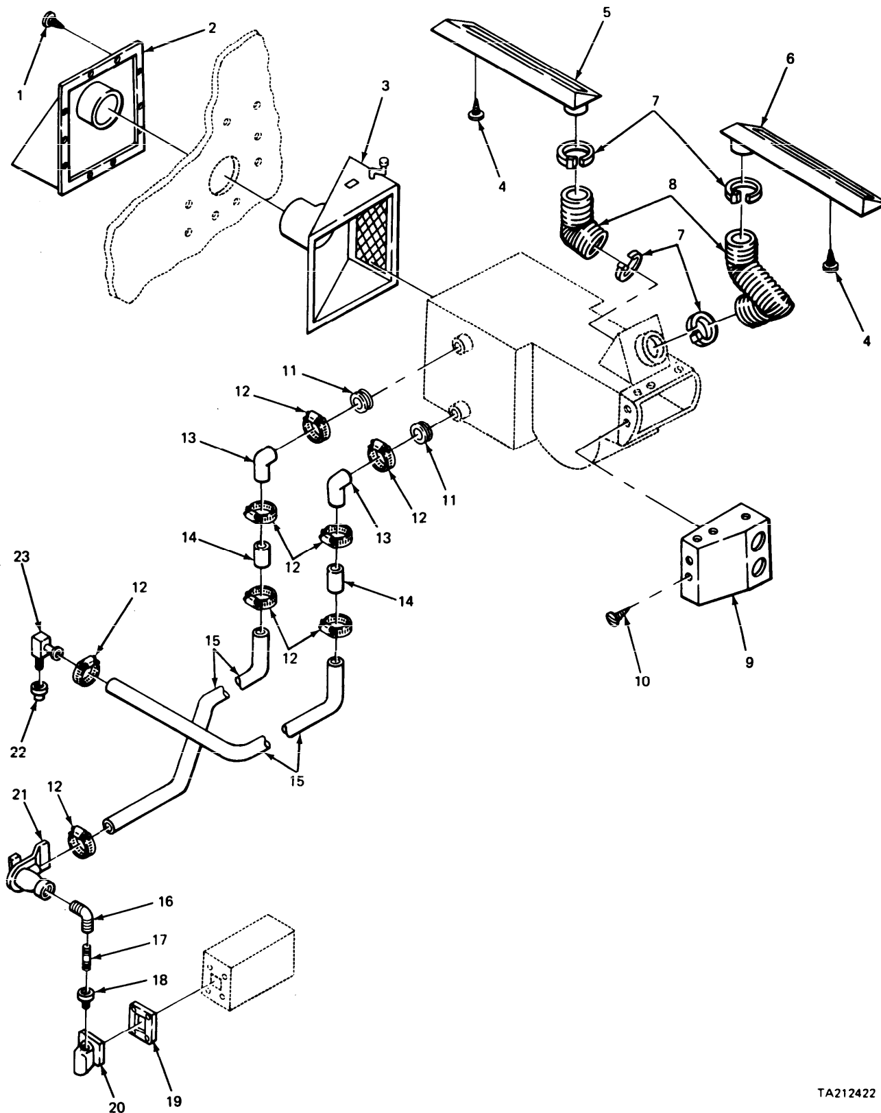
FIGURE 296. DEFLECTOR HEATER AND RELATED PARTS.
