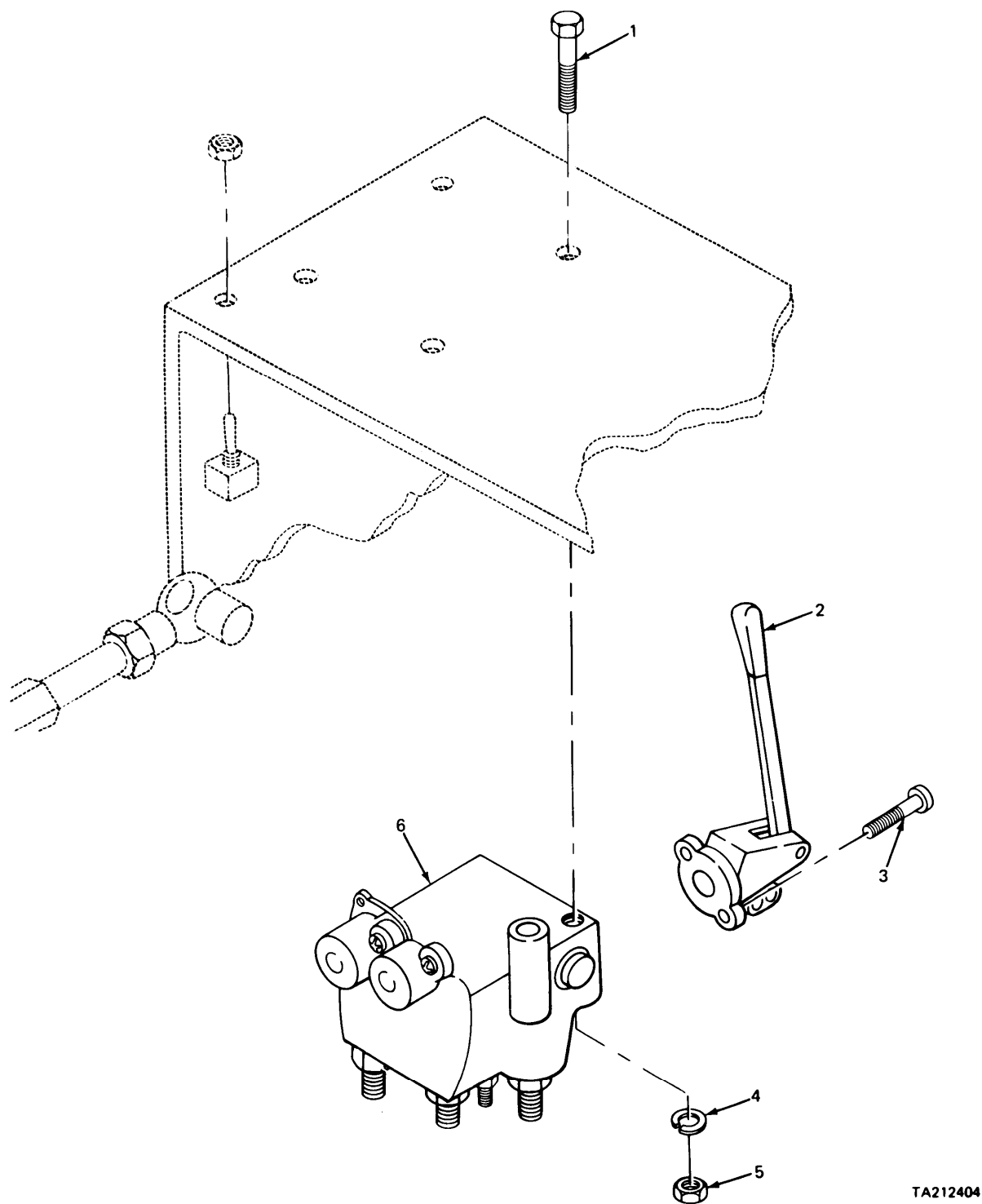
FIGURE 278. WINCH CONTROL.
