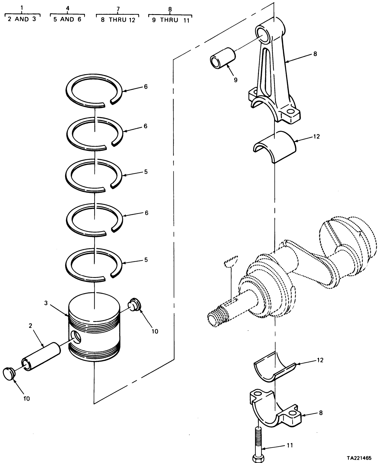
FIGURE 200. AIR COMPRESSOR PISTON AND CONNECTING ROD.
