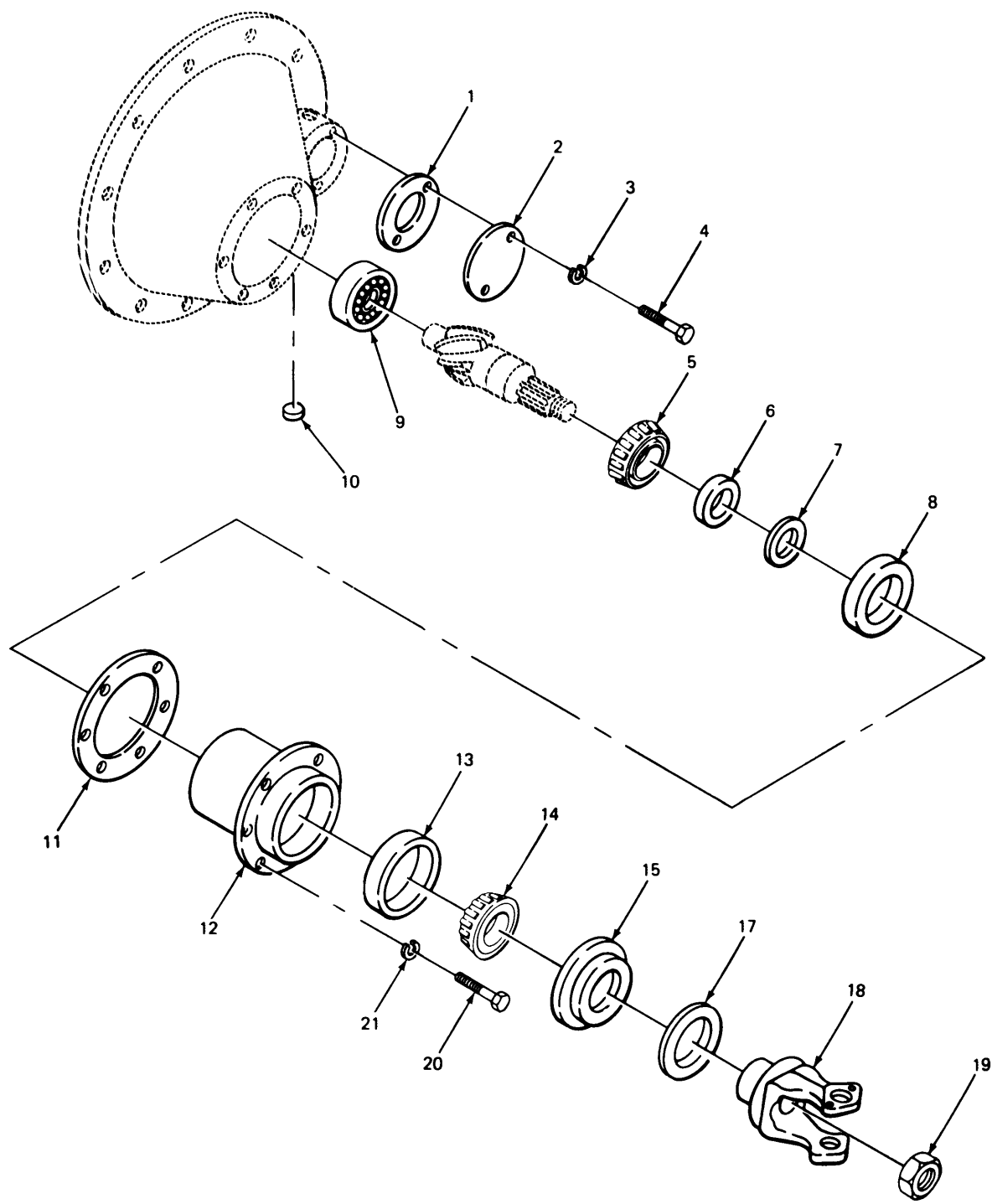
FIGURE 162. REAR YOKE AND RELATED PARTS.
