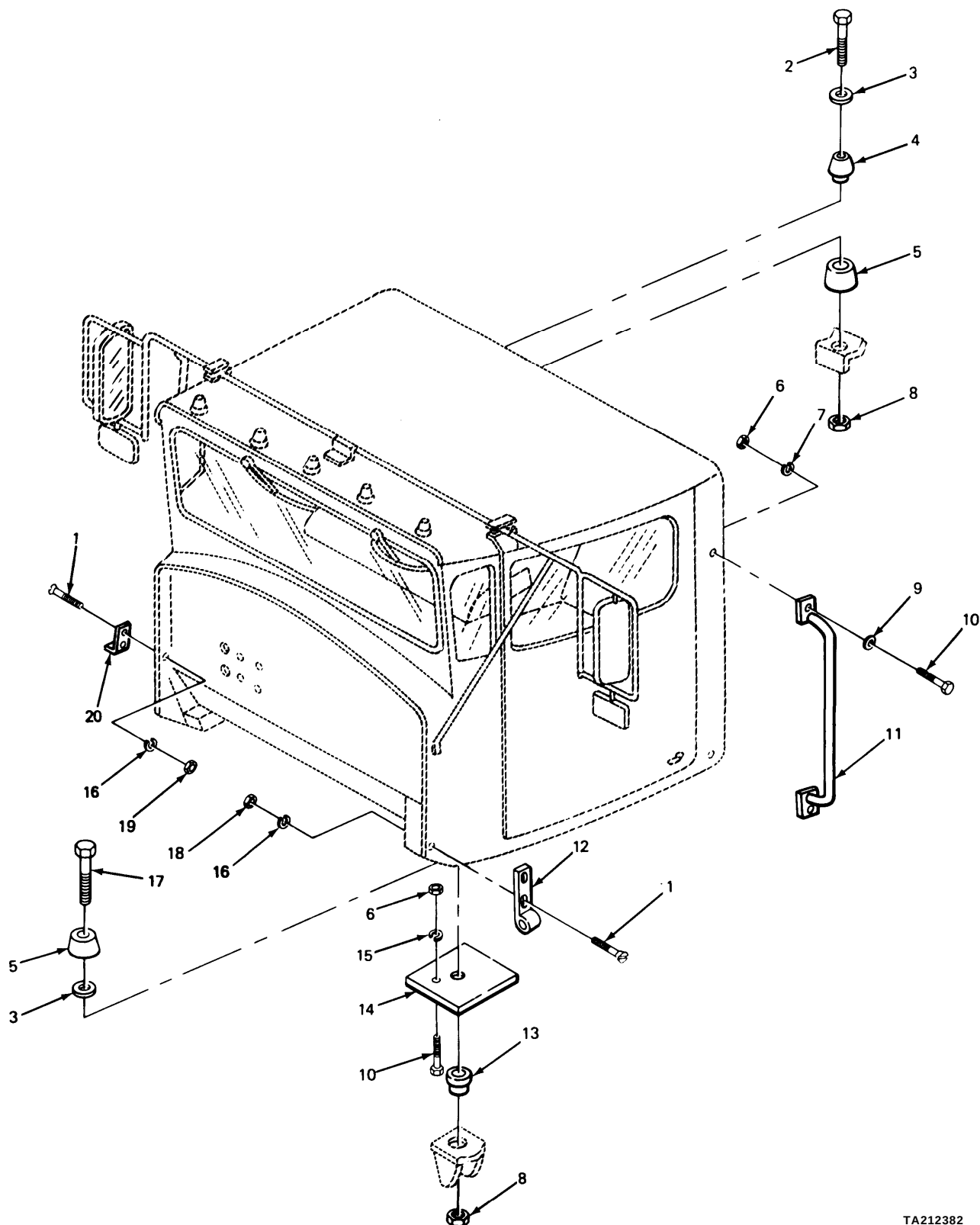
FIGURE 254. CAB MOUNT PLATE AND RELATED PARTS.
