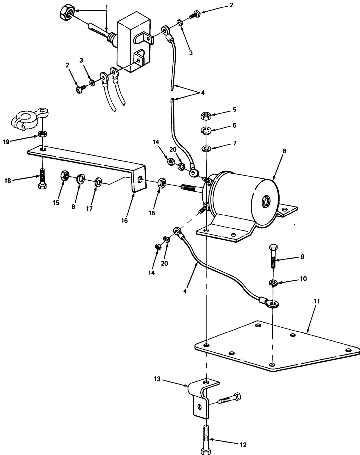
FIGURE 75. ENGINE SHUT DOWN AND RELATED PARTS.
