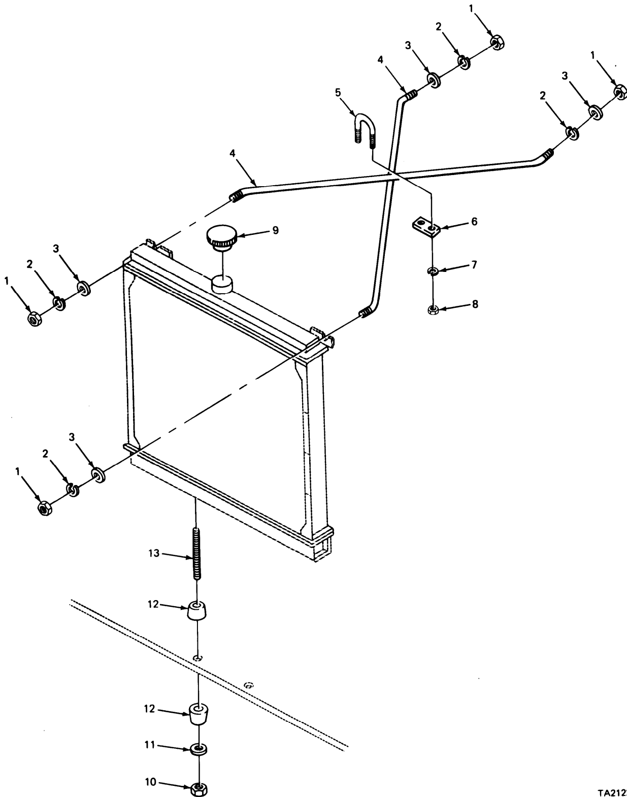
FIGURE 60. RADIATOR TIE RODS AND
