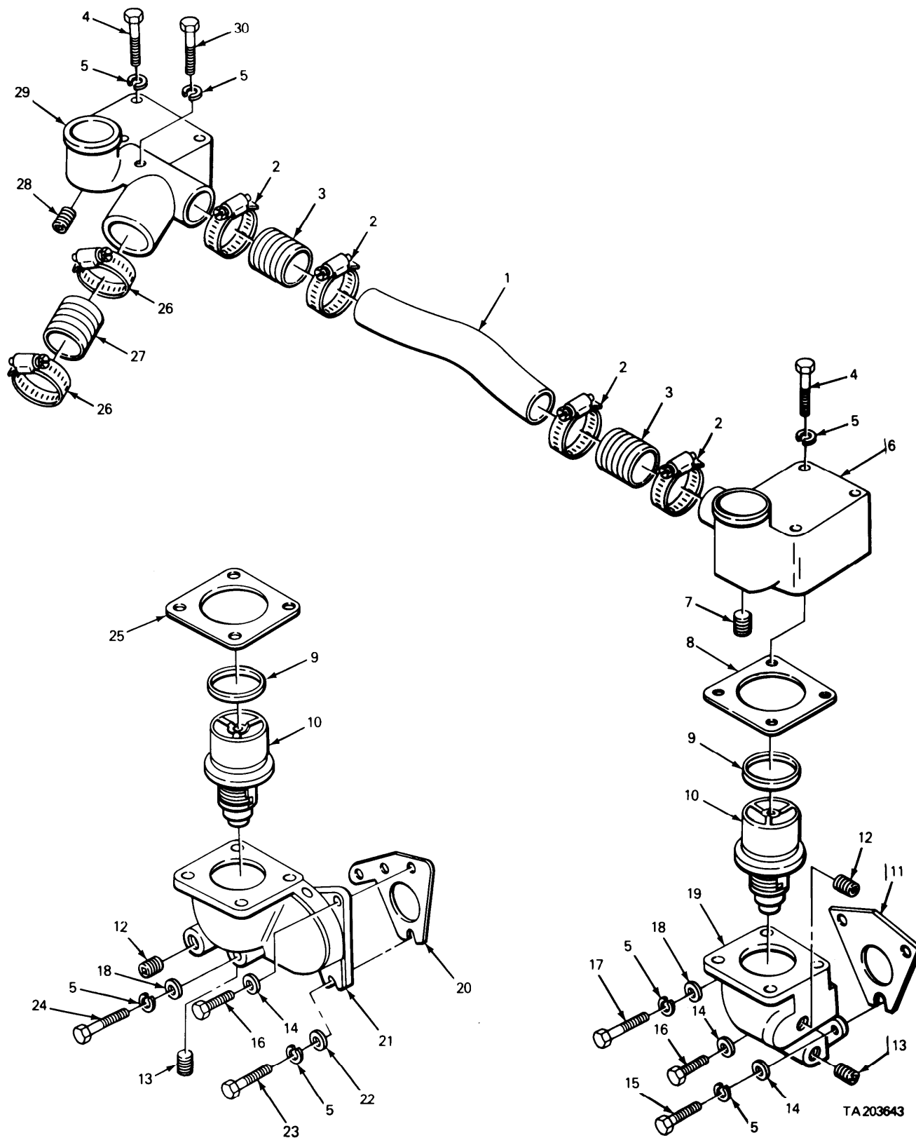
FIGURE 64. THERMOSTAT, HOUSINGS AND RELATED PARTS.
