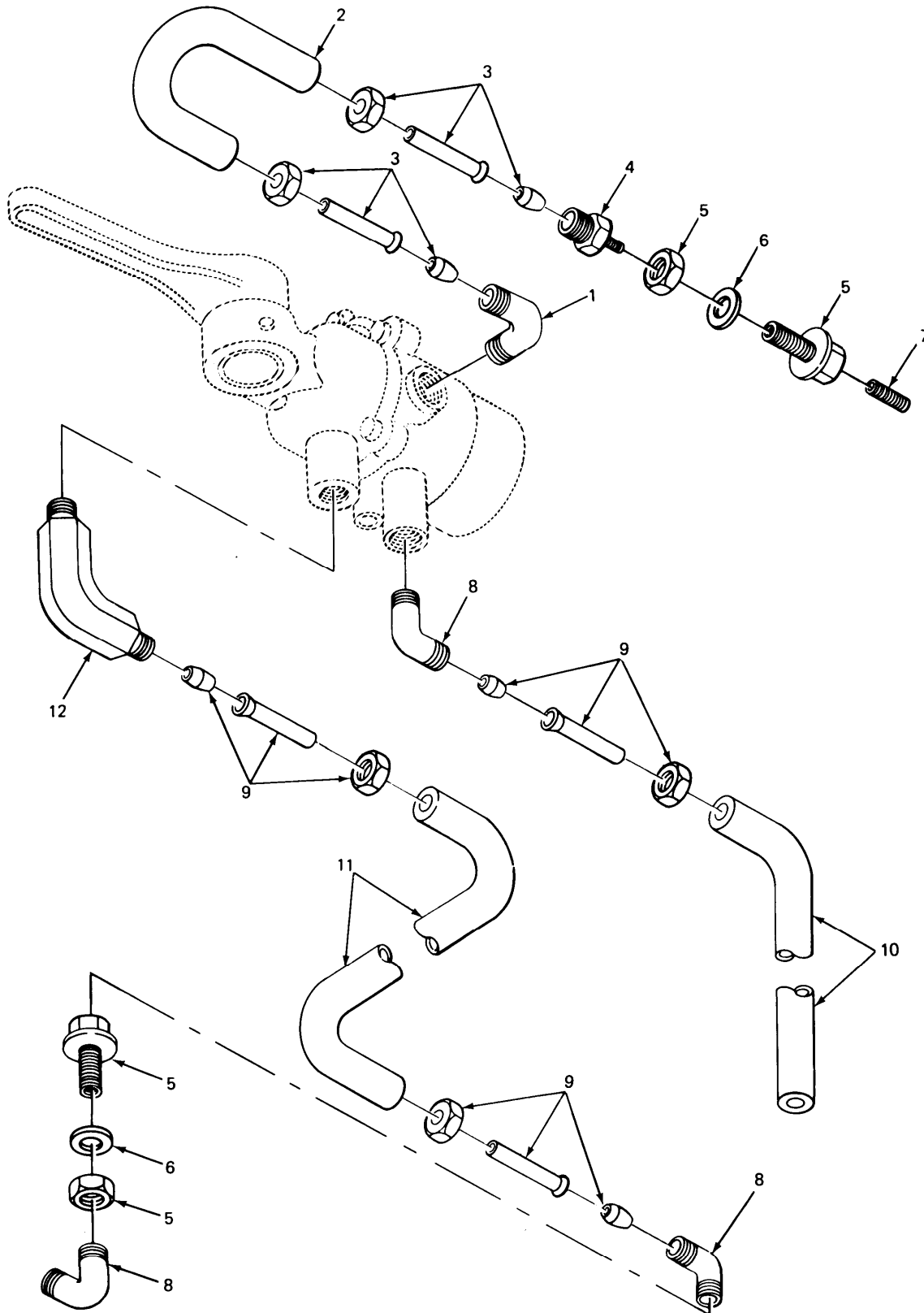
FIGURE 184. TRAILER BRAKE CONTROL AND AIR PRESSURE GAGE LINES AND FITTINGS.
