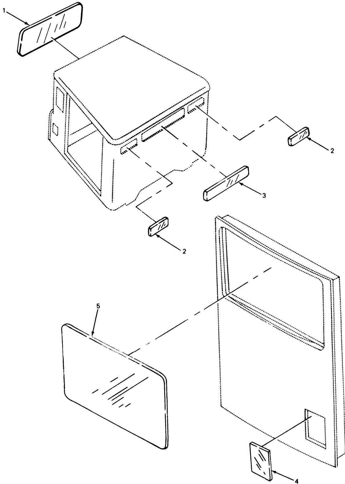
FIGURE 259. CAB WINDSHIELD AND ASSORTED GLASS.
