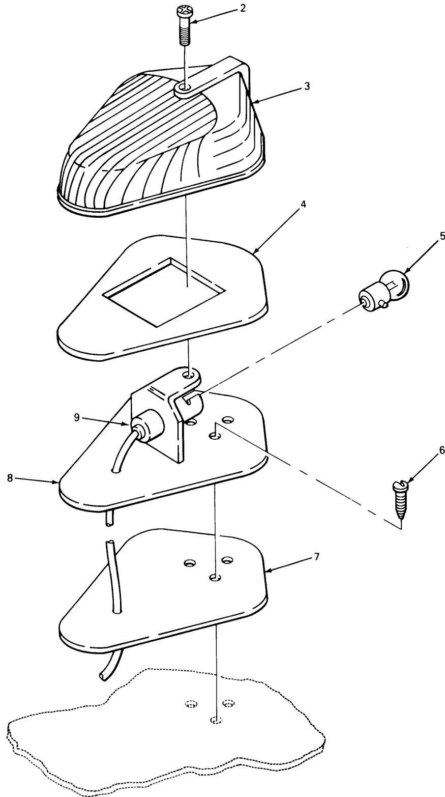
FIGURE 84. CLEARANCE LIGHT.
