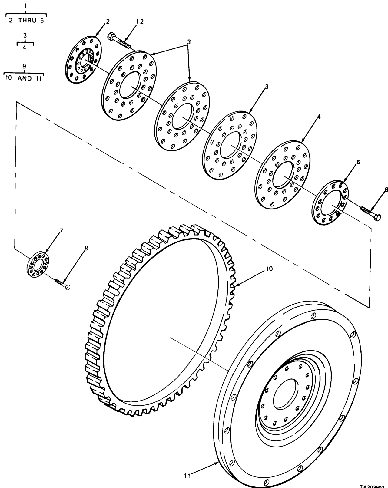
FIGURE 10. FLEXIBLE COUPLING AND FLYWHEEL.
