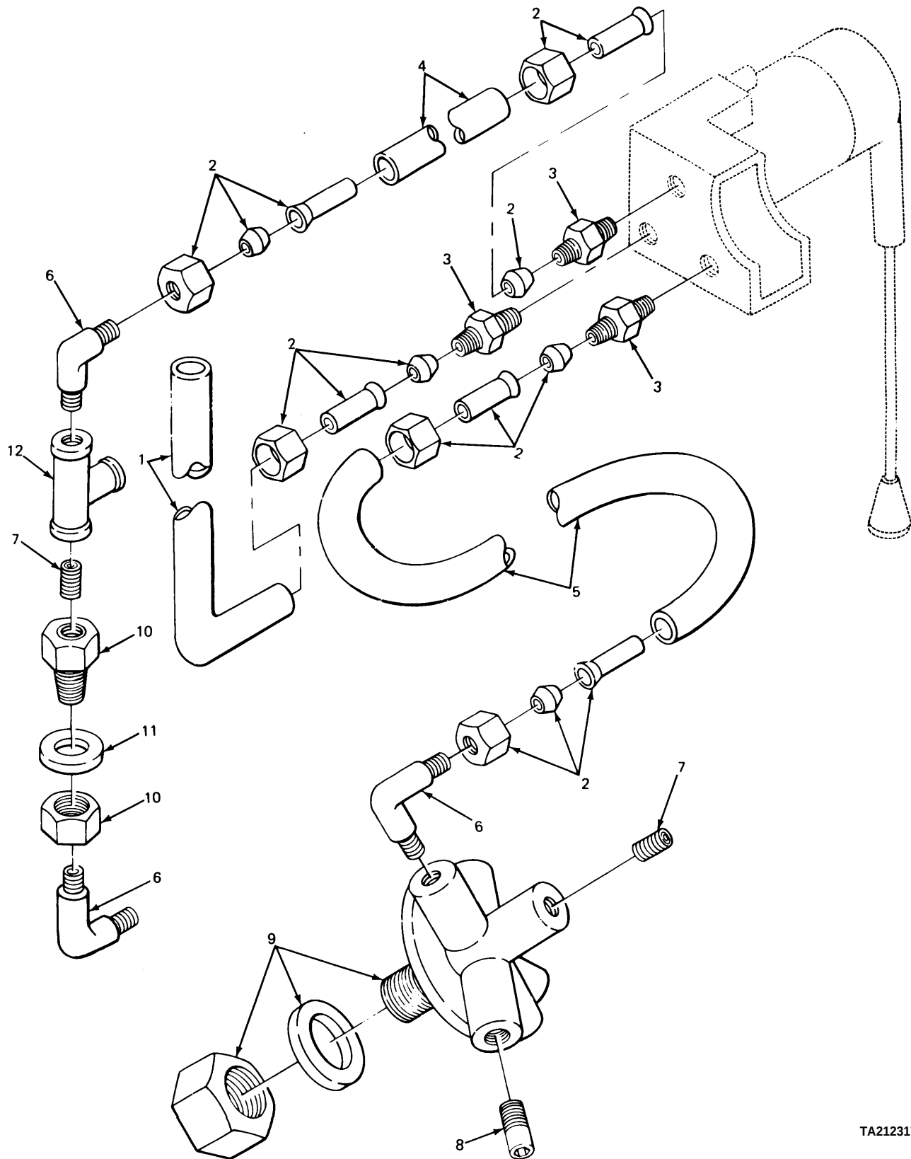
FIGURE 183. BULKHEAD FITTING AND RELATED PARTS.
