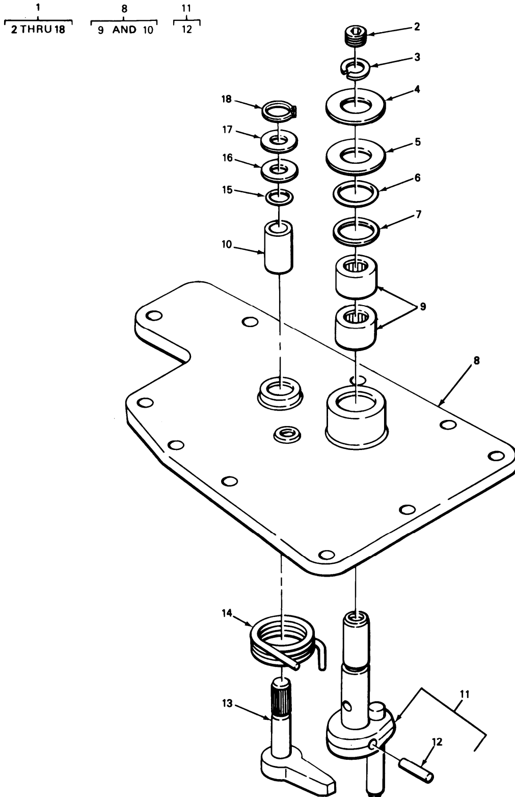
FIGURE 49. GOVERNOR COVER AND RELATED PARTS.
