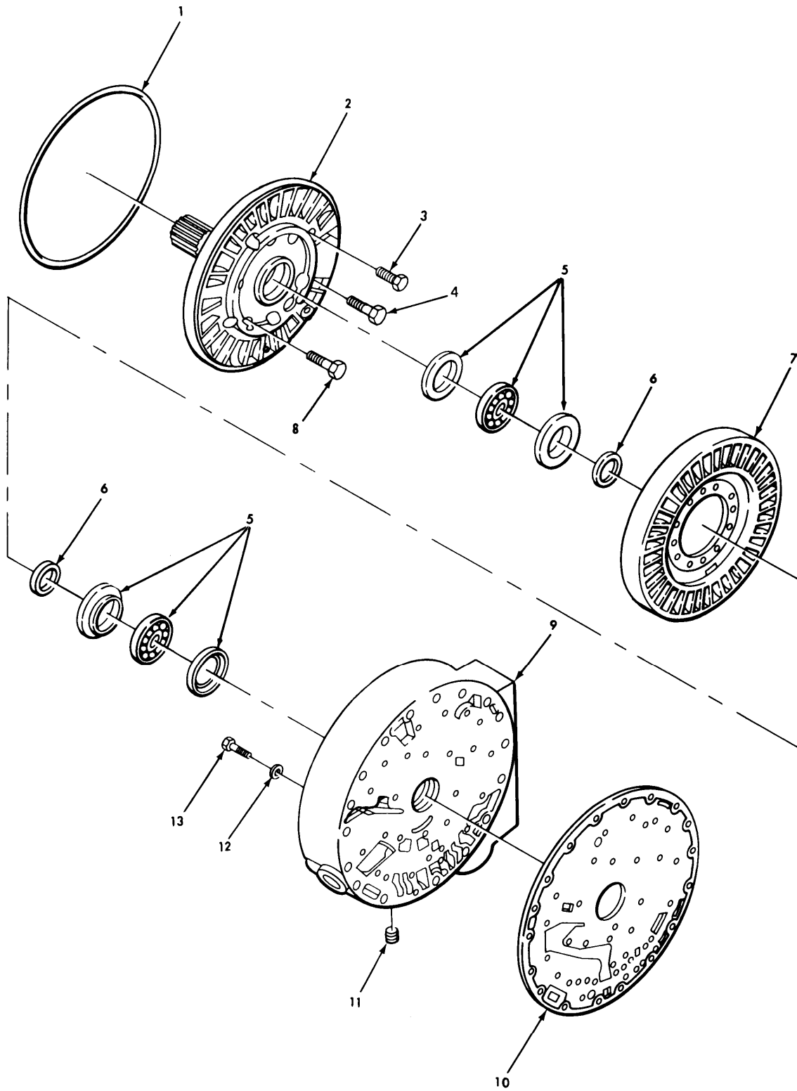
FIGURE 120. RETARDER HOUSING AND RELATED PARTS.
