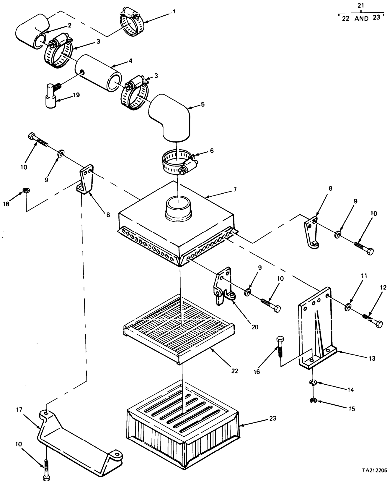
FIGURE 38. AIR INTAKE FILTER AND RELATED PARTS.
