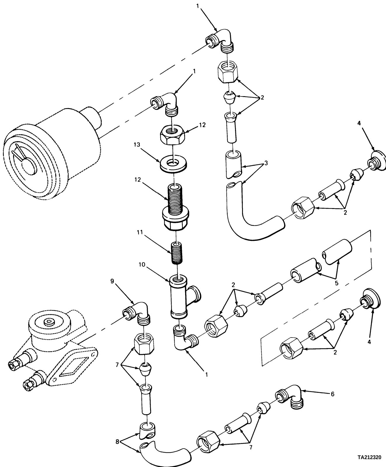
FIGURE 187. AIR PRESSURE GAGE'S LINES AND FITTINGS.
