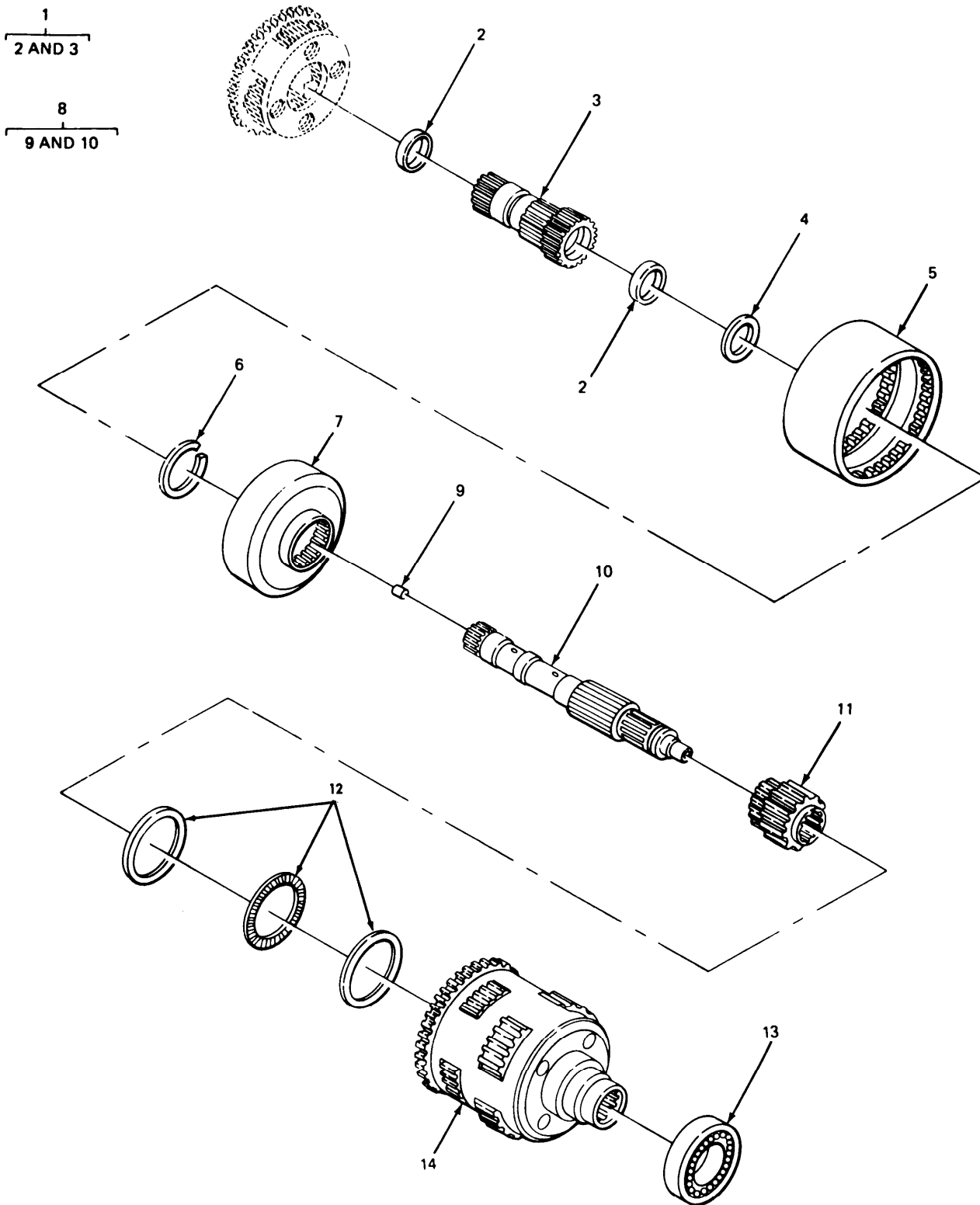
FIGURE 116. CARRIER ASSEMBLY MAIN SHAFT AND RELATED PARTS.
