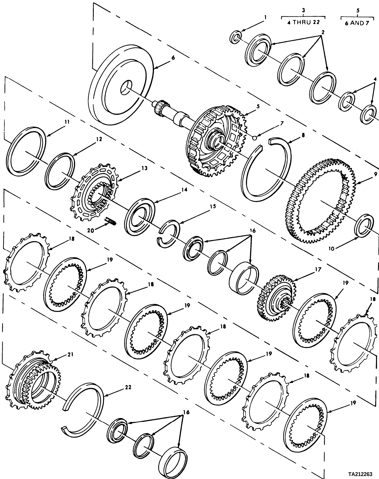
FIGURE 121. FORWARD CLUTCH AND RELATED PARTS.
