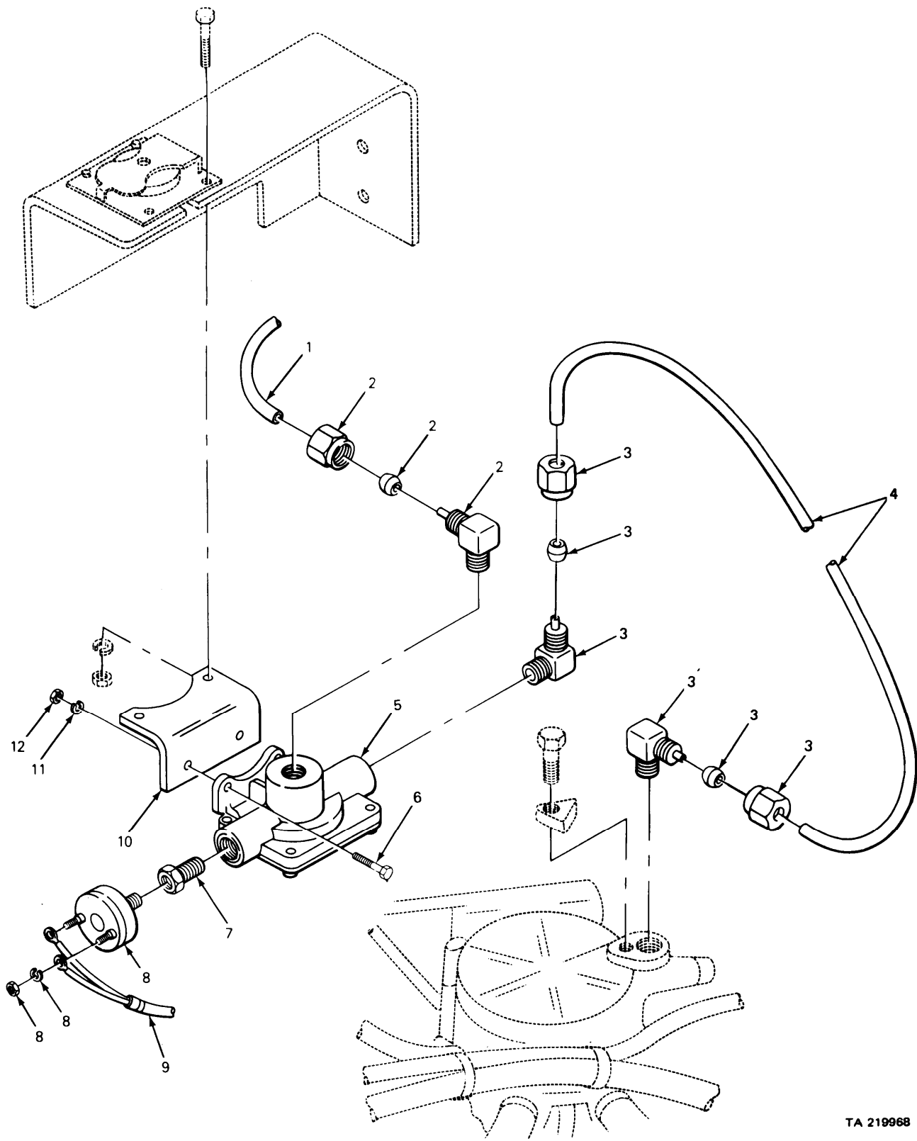
FIGURE 208. QUICK RELEASE VALVE AND ATTACHING PARTS.
