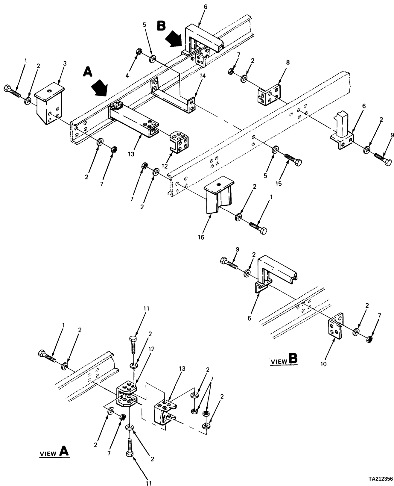
FIGURE 229. AUXILIARY TRANSMISSION SUPPORT AND RELATED PARTS.
