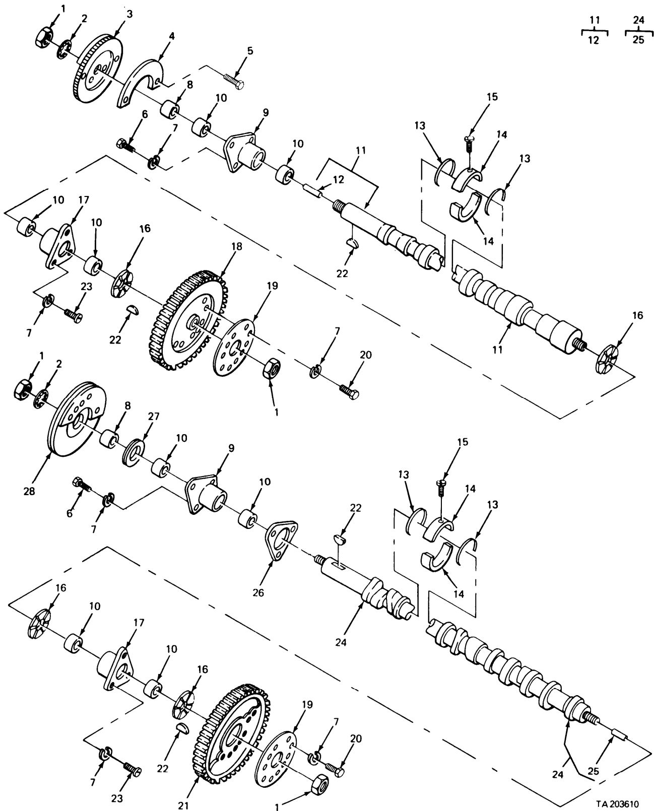
FIGURE 14, CAMSHAFT, BEARINGS, GEARS, AND RELATED PARTS.
