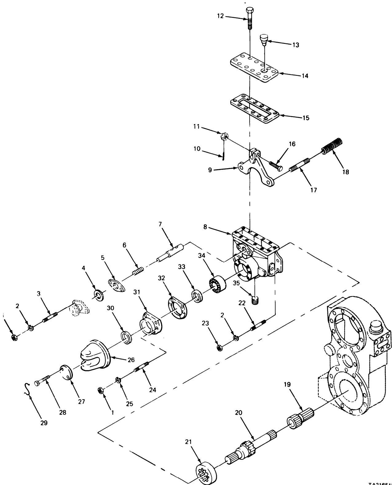
FIGURE 140. SHIFTER FORK AND UNIVERSAL YOKE EXPLODED.
