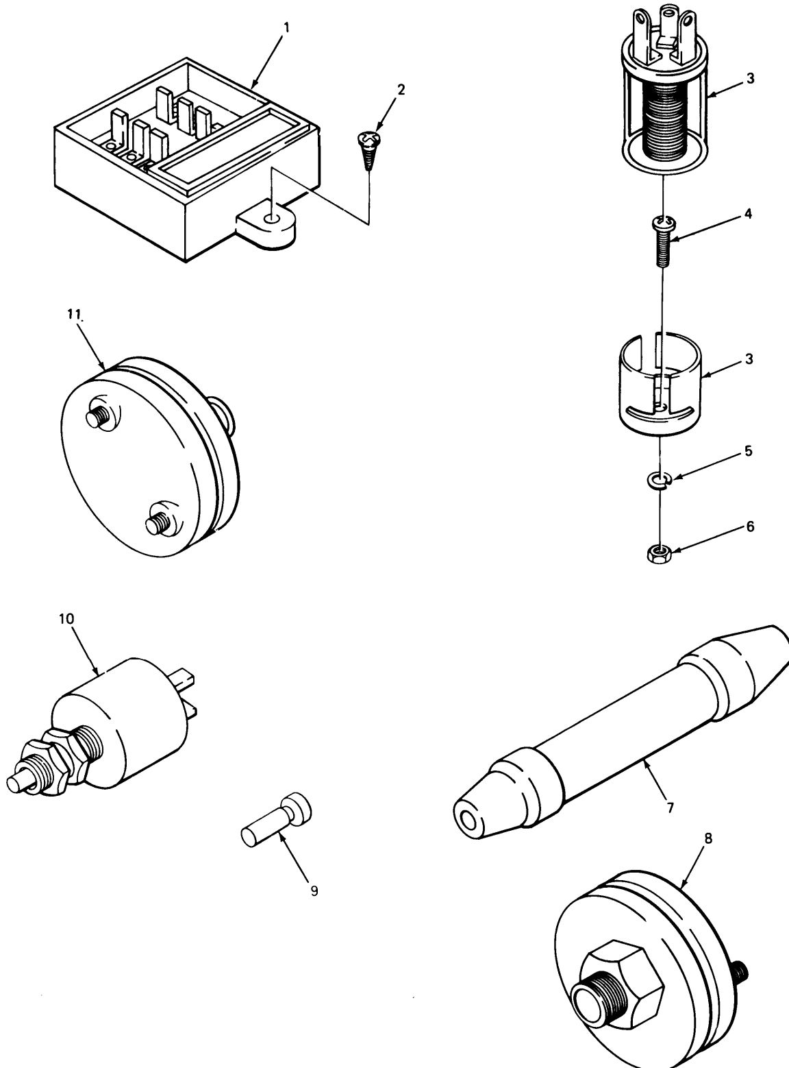
FIGURE 80. SENDING SWITCHES AND RELATED PARTS (INCLUDES NEUTRAL SAFETY SWITCH AND PIN).
