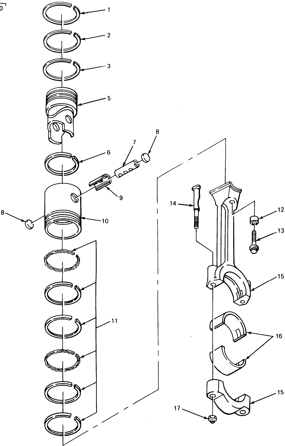
FIGURE 13. PISTON, RINGS, CONNECTING ROD AND RELATED PARTS.
