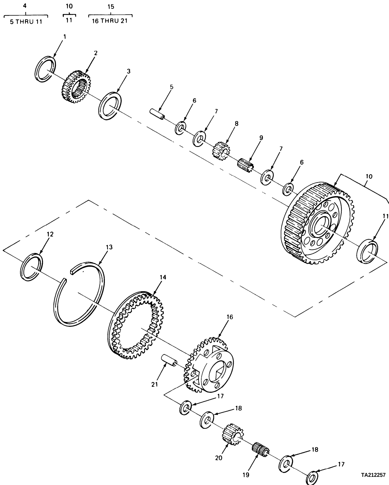
FIGURE 115. CARRIER ASSEMBLY AND RELATED PARTS.
