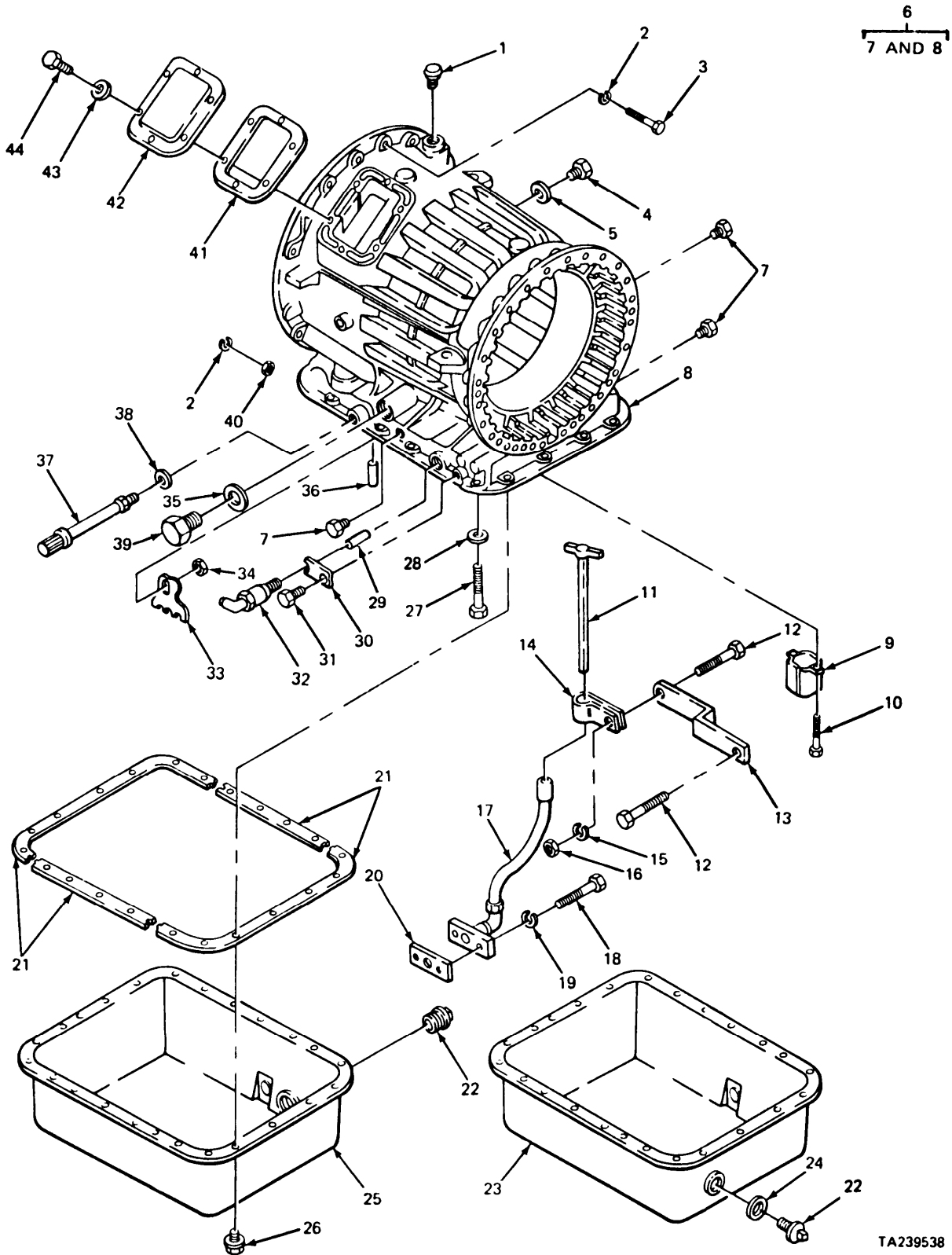
FIGURE 114. TRANSMISSION EXPLODED VIEW.
