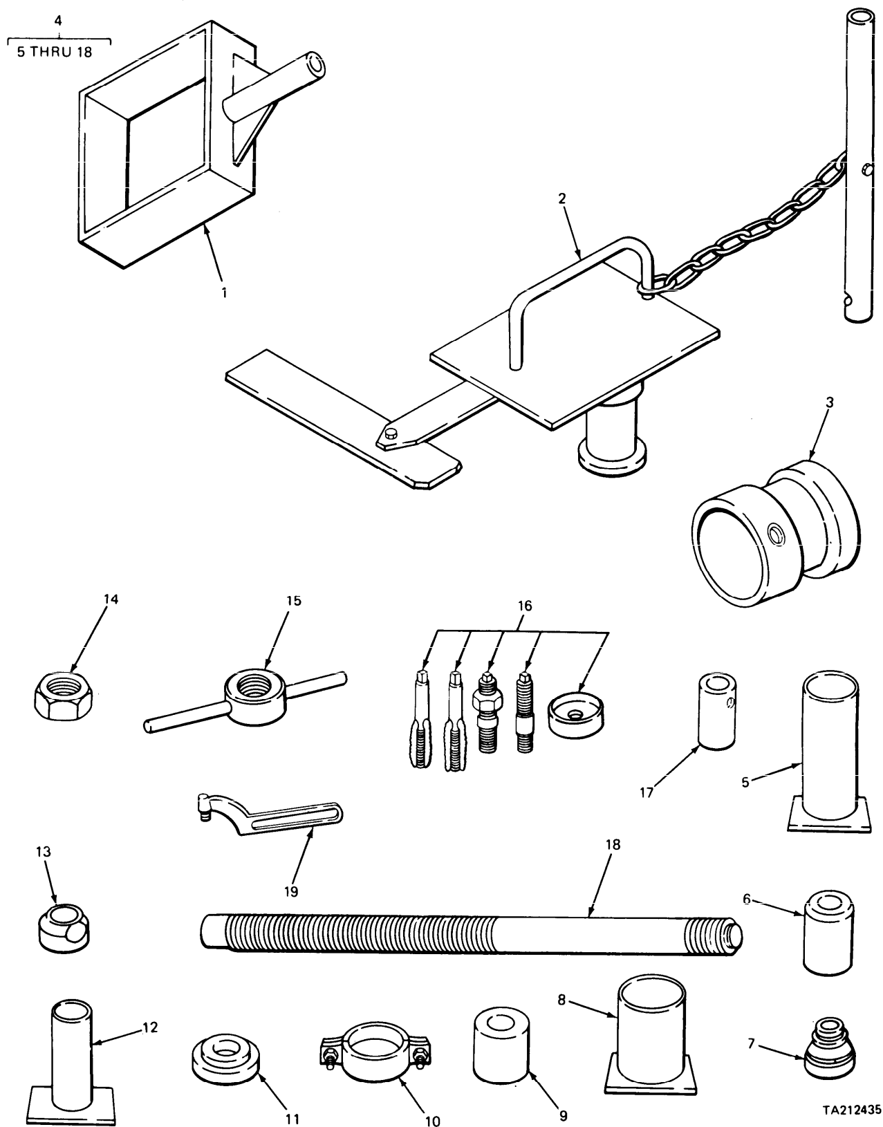
FIGURE 310. GENERAL SUPPORT SPECIAL TOOLS.
