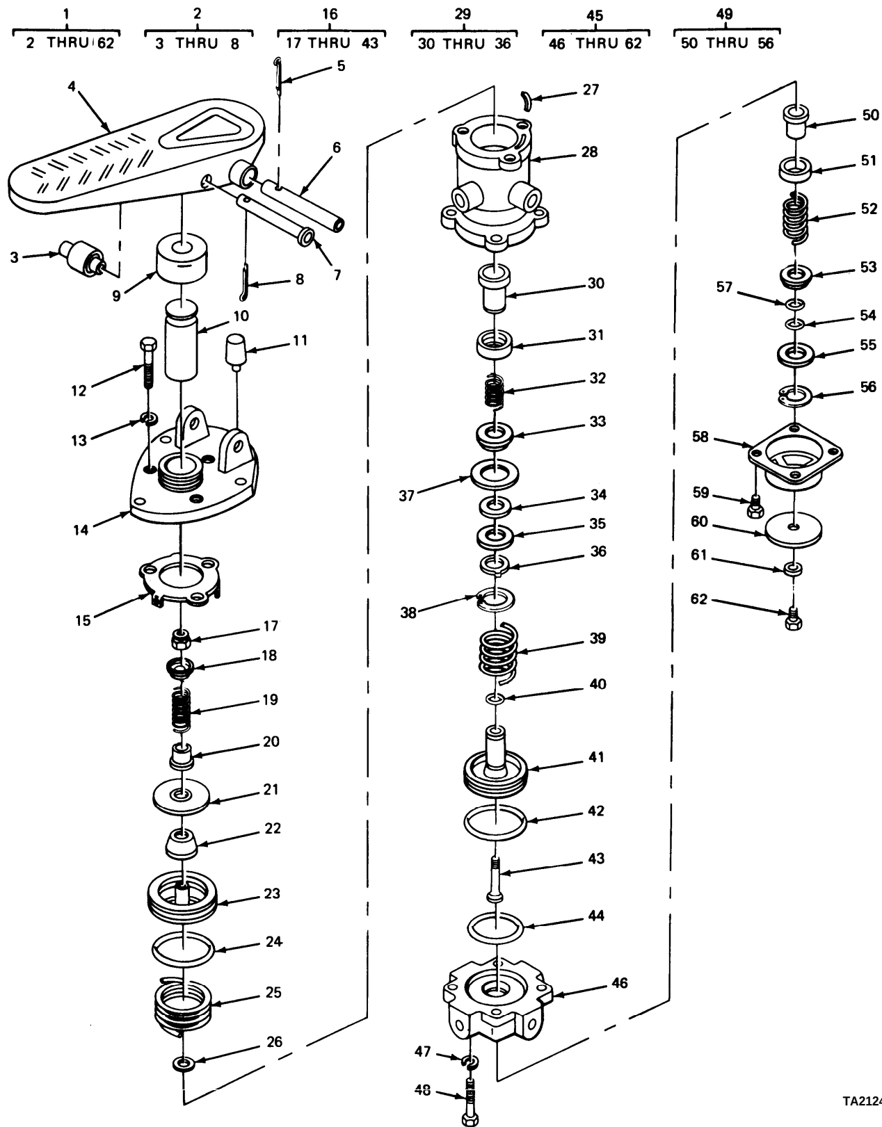
FIGURE 176. BRAKE TREADLE VALVE ASSEMBLY.
