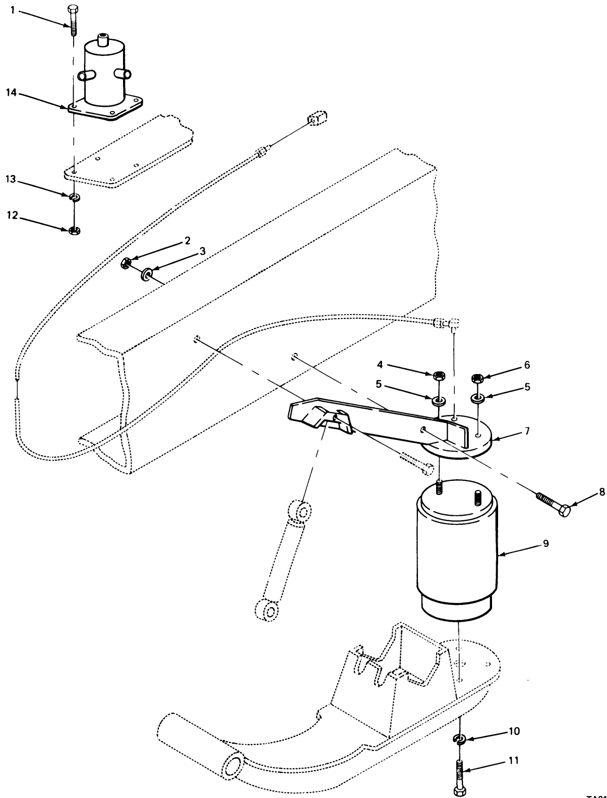
FIGURE 243. PUSHER AXLE SHOCK ABSORBER AND RELATED PARTS.
