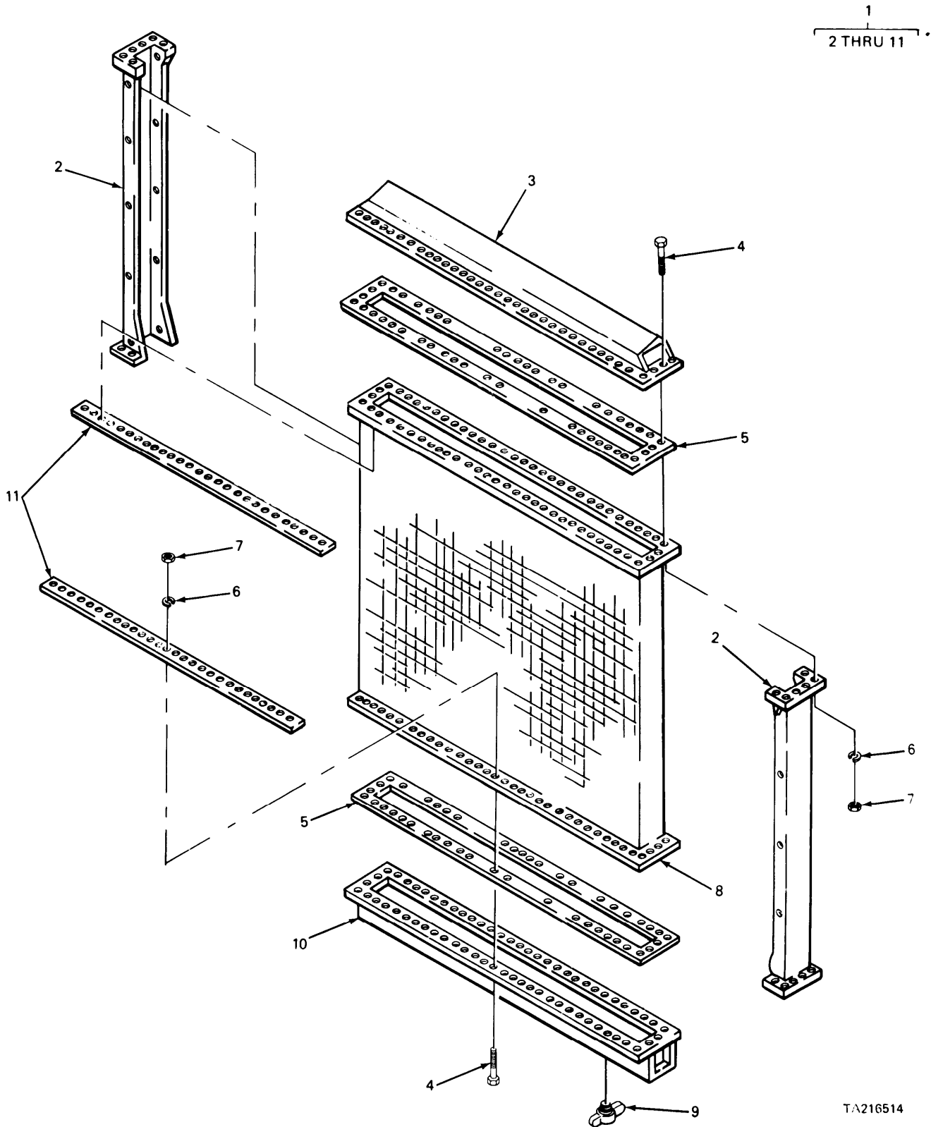
FIGURE 61. RADIATOR CORE AND RELATED PARTS.
