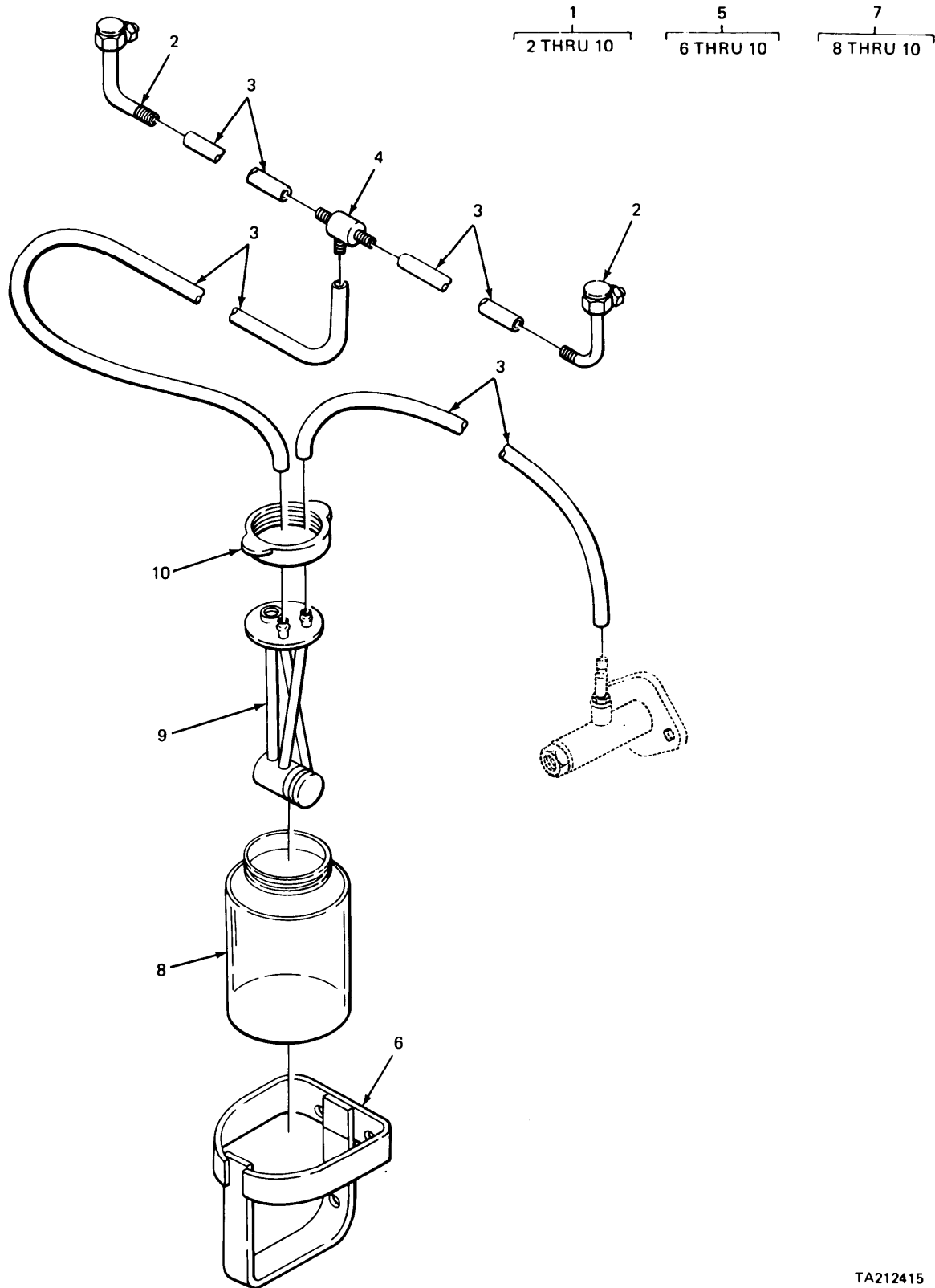
FIGURE 289. WINDSHIELD WASHER ASSEMBLY.
