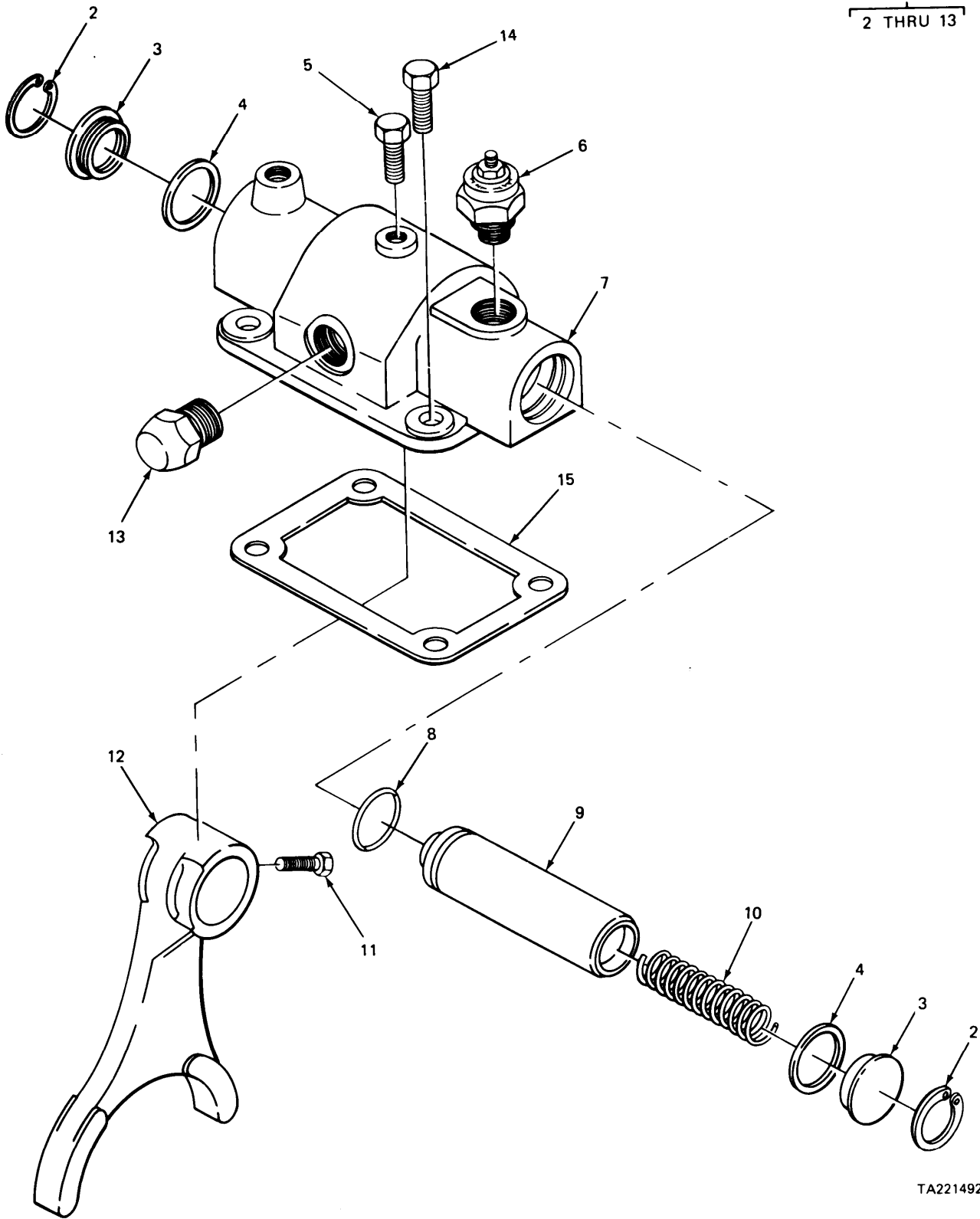
FIGURE 285. AIR SHIFT ASSEMBLY, P. T. O..
