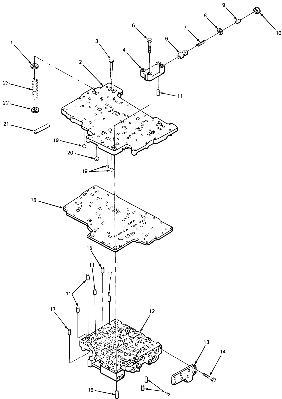
FIGURE 130. CONTROL VALVE AND RELATED PARTS.
