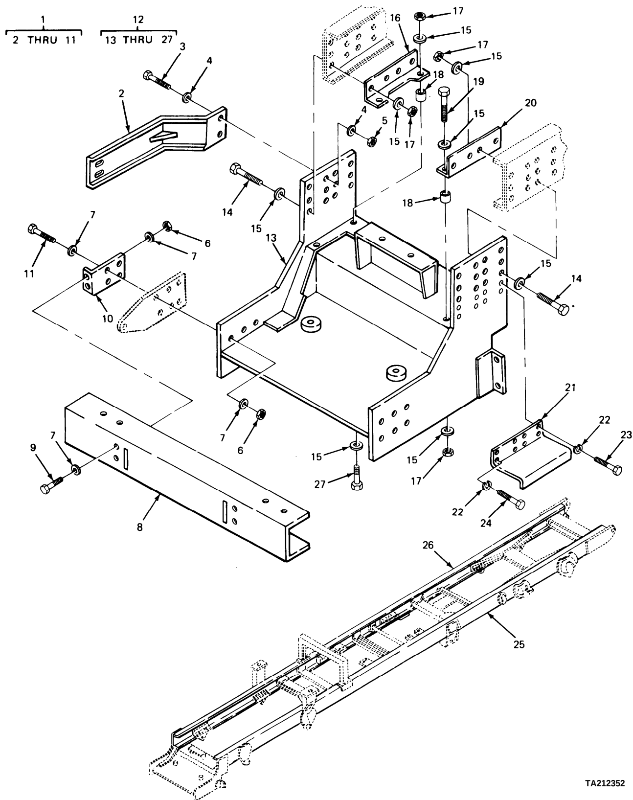
FIGURE 227. BUMPER AND FRAME ASSEMBLY.
