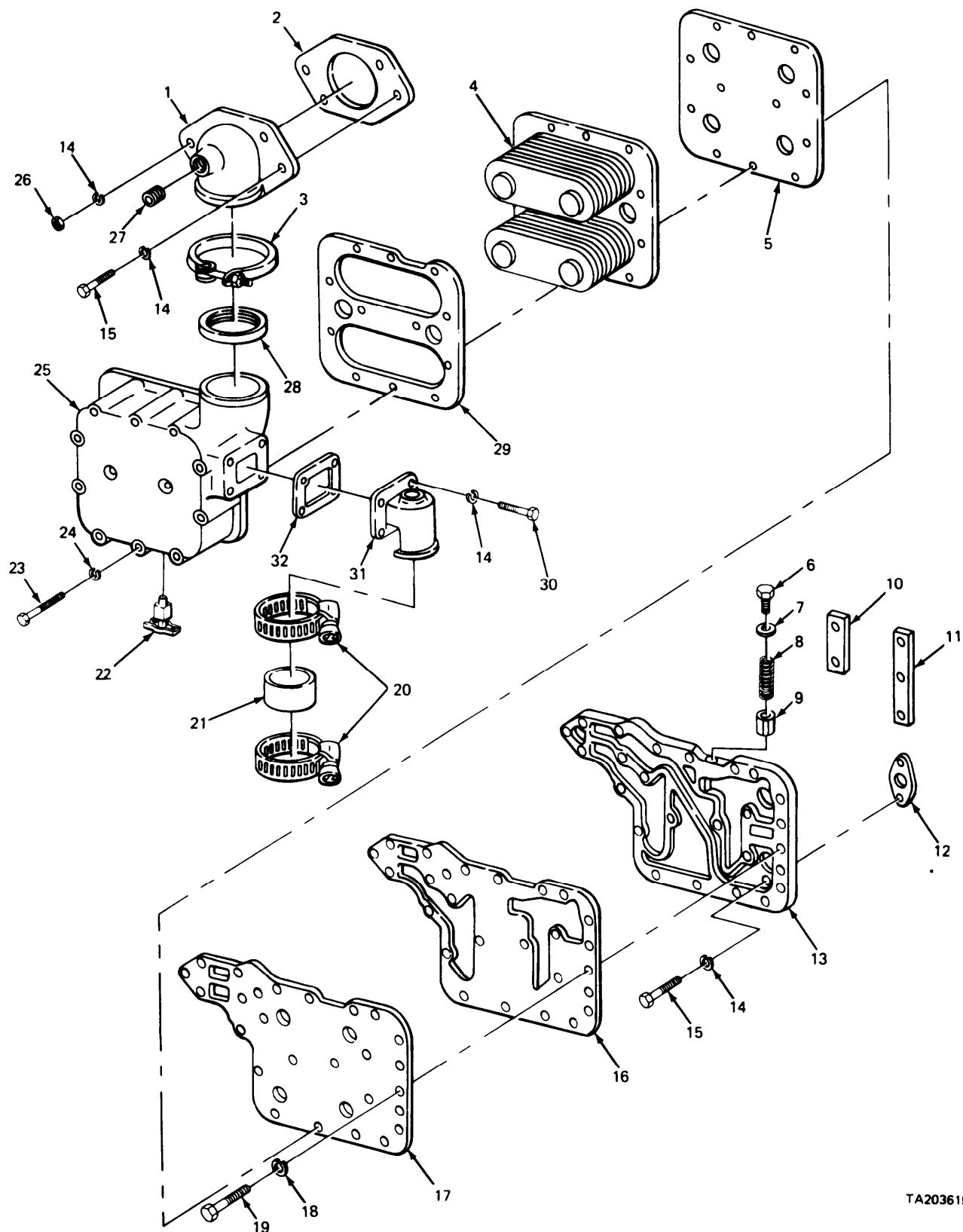
FIGURE 24. OIL COOLER EXPLODED VIEW.
