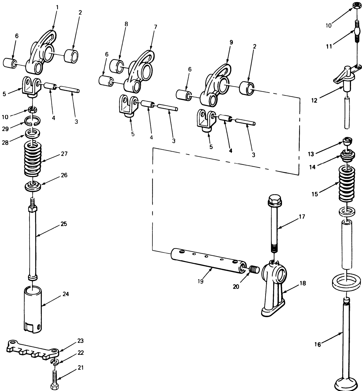
FIGURE 15. VALVES, TAPPETS, ROCKER ARMS, AND RELATED PARTS.
