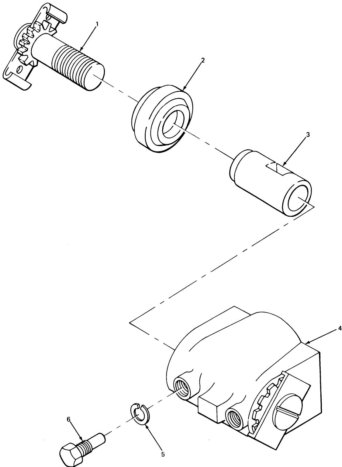
FIGURE 168. FRONT BRAKE ACTUATOR HOUSING AND ADJUSTING BOLT ASSEMBLY.
