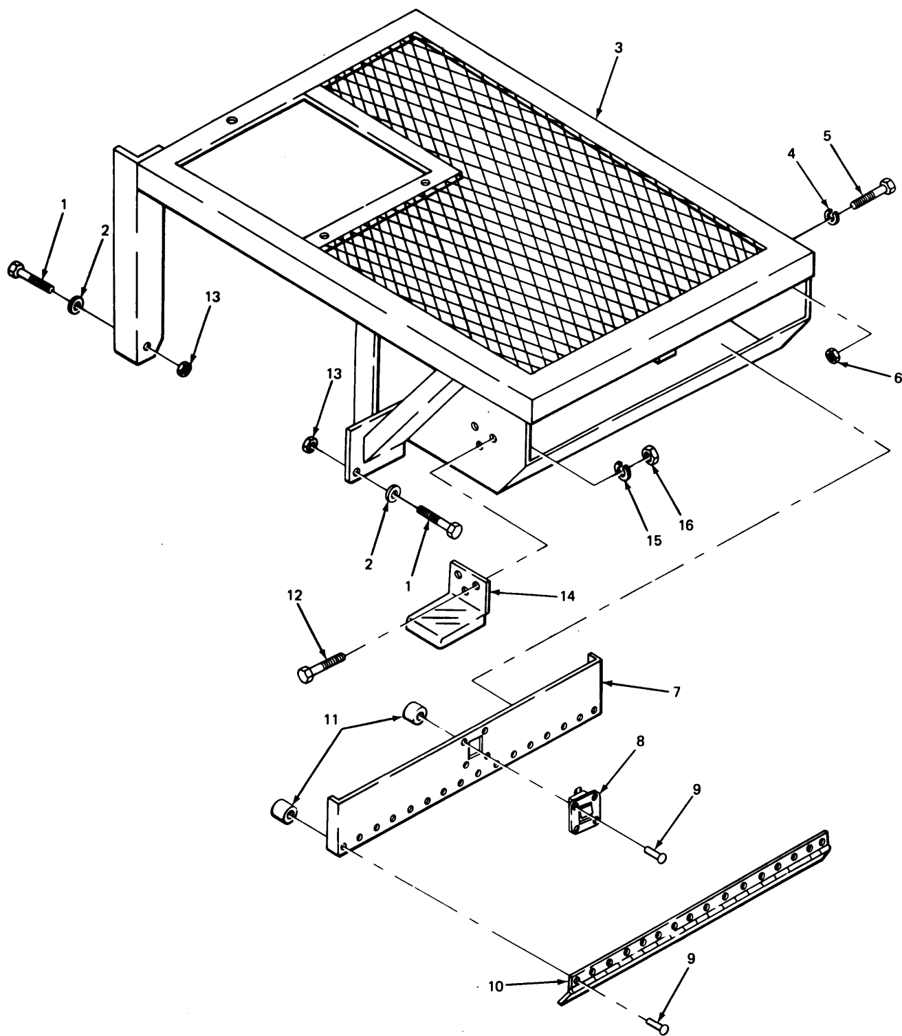
FIGURE 268. WINCH PLATFORM AND RELATED PARTS.
