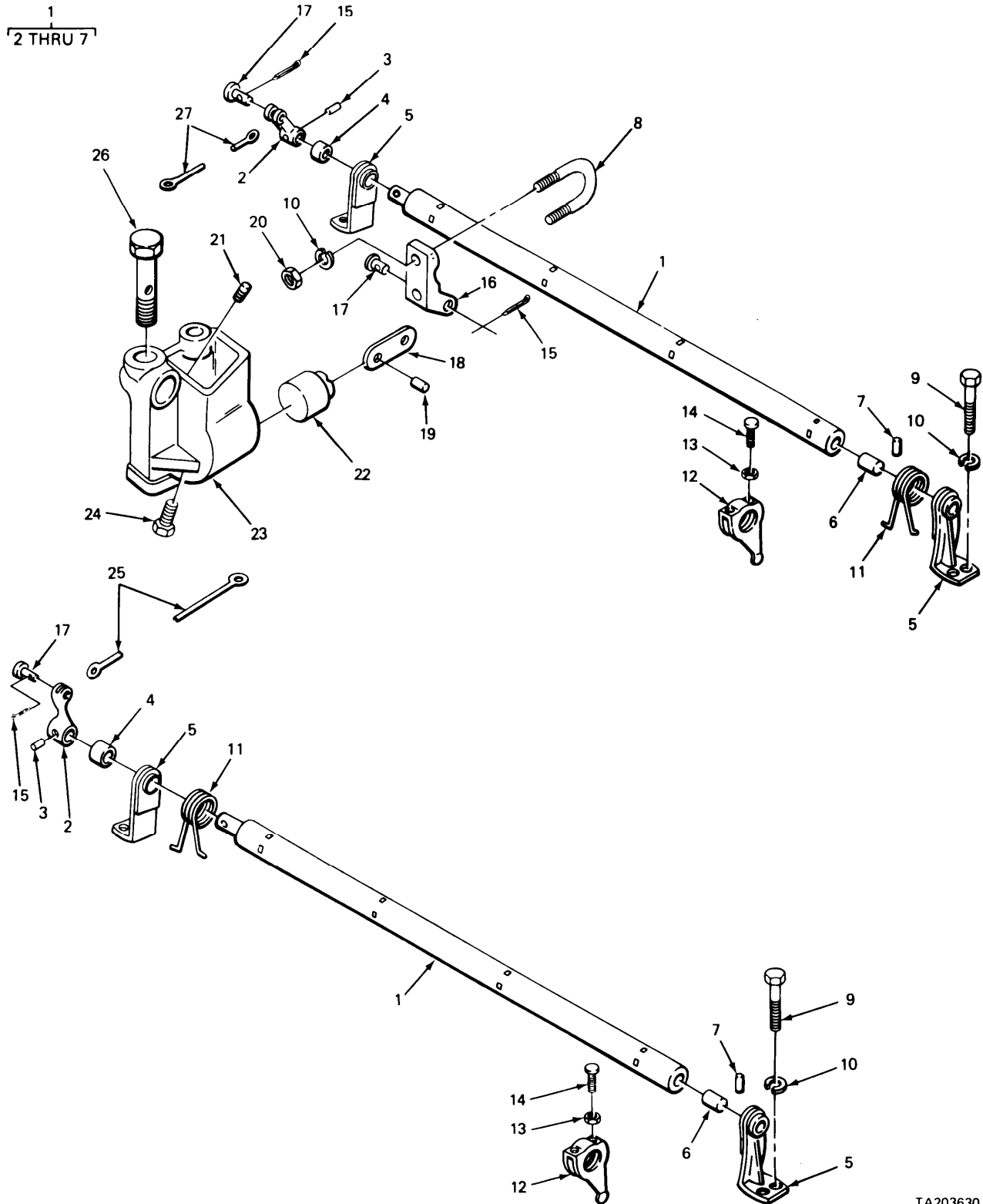
FIGURE 35. FUEL CONTROL TUBES AND RELATED PARTS.
