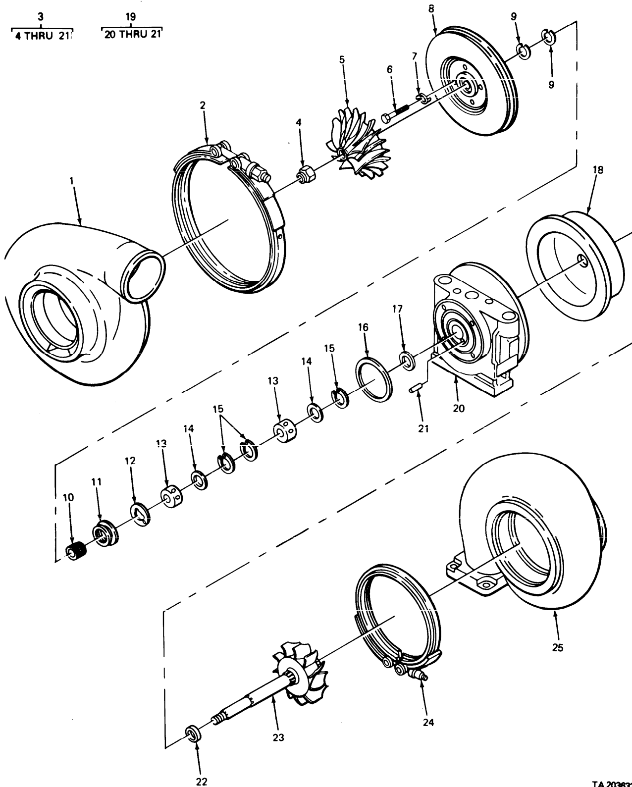
FIGURE 41. TURBOCHARGER EXPLODED VIEW.
