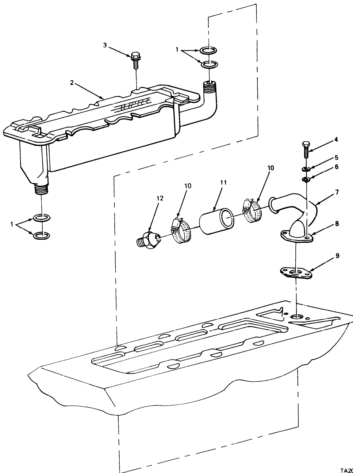
FIGURE 42. AFTERCOOLER AND RELATED PARTS FOR THE 8V92TA ENGINE.
