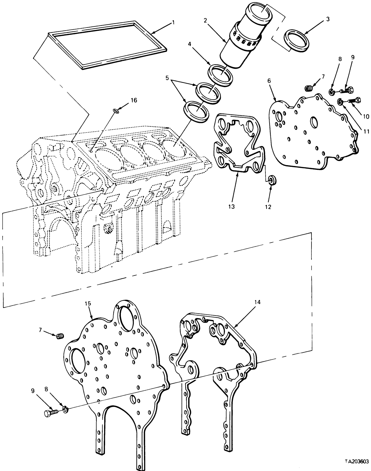
FIGURE 6. ENGINE BLOCK CYLINDER LINERS, AND RELATED PARTS.
