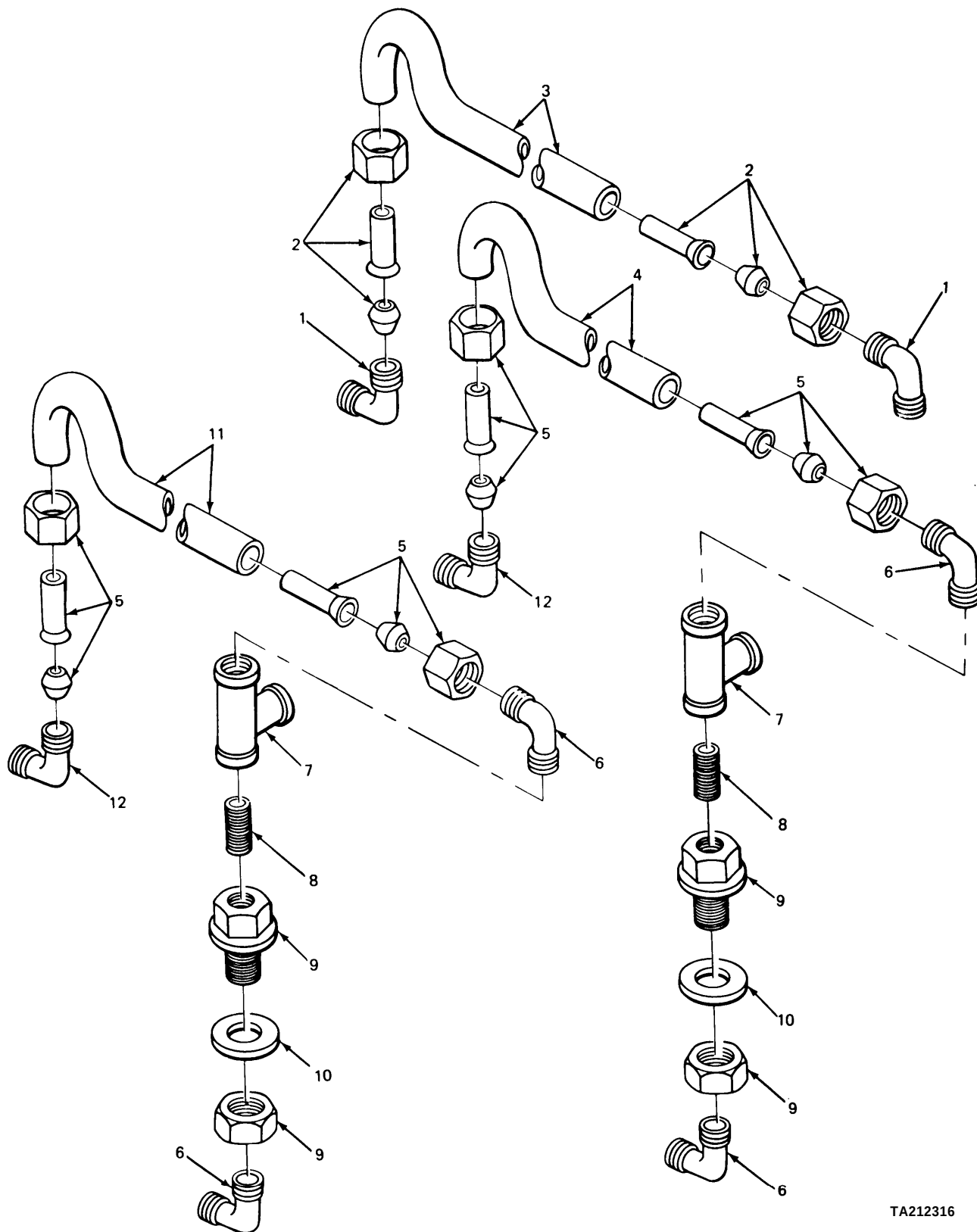
FIGURE 182. CONNECTORS AND RELATED PARTS.
