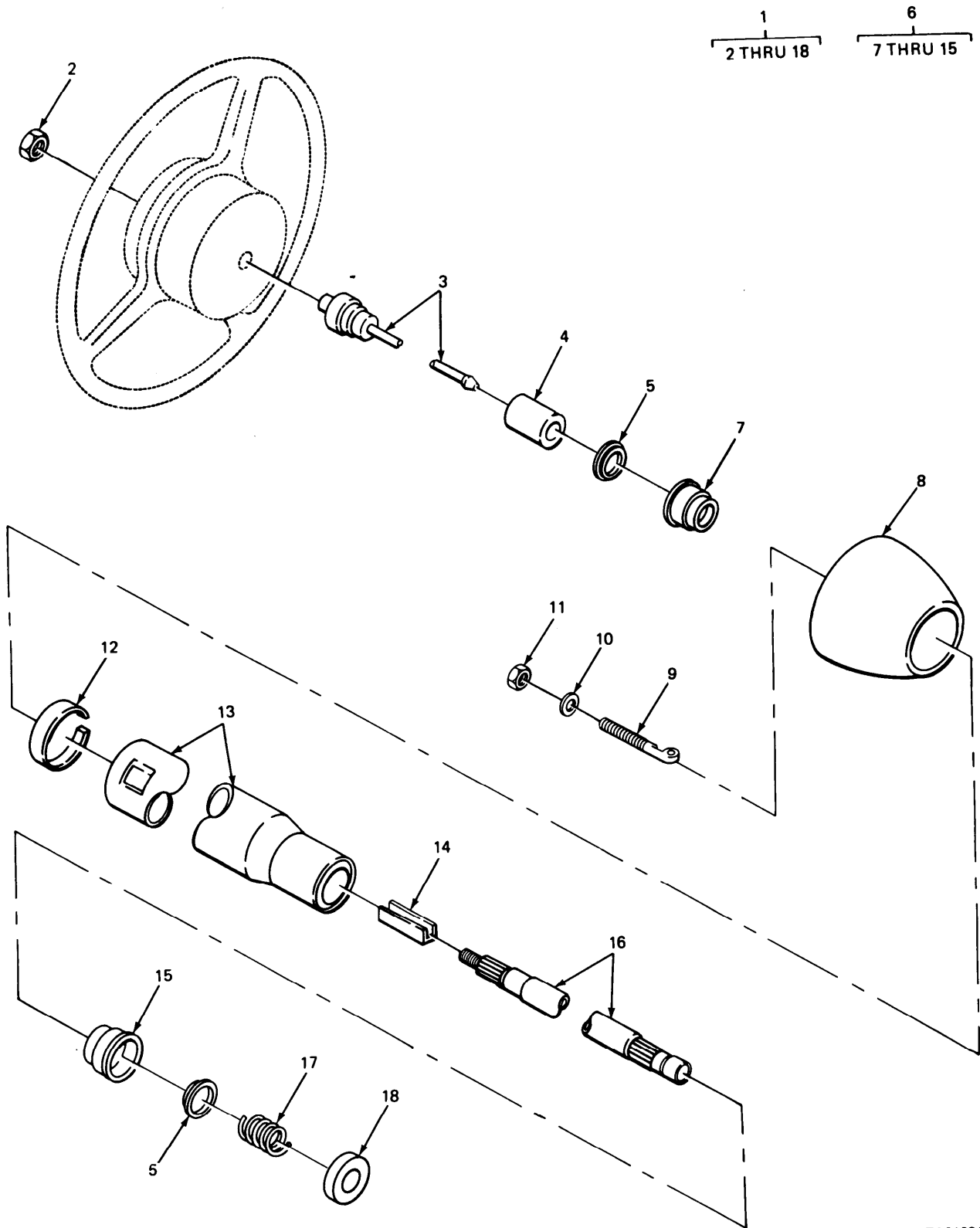
FIGURE 215. STEERING WHEEL JACKET AND RELATED PARTS.
