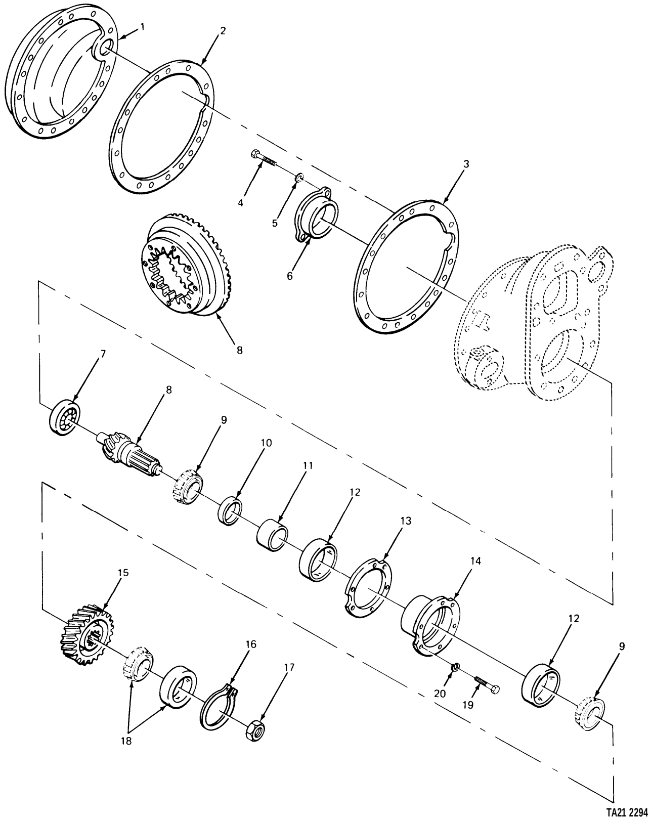
FIGURE 158. AXLE HOUSING COVER AND RELATED PARTS.
