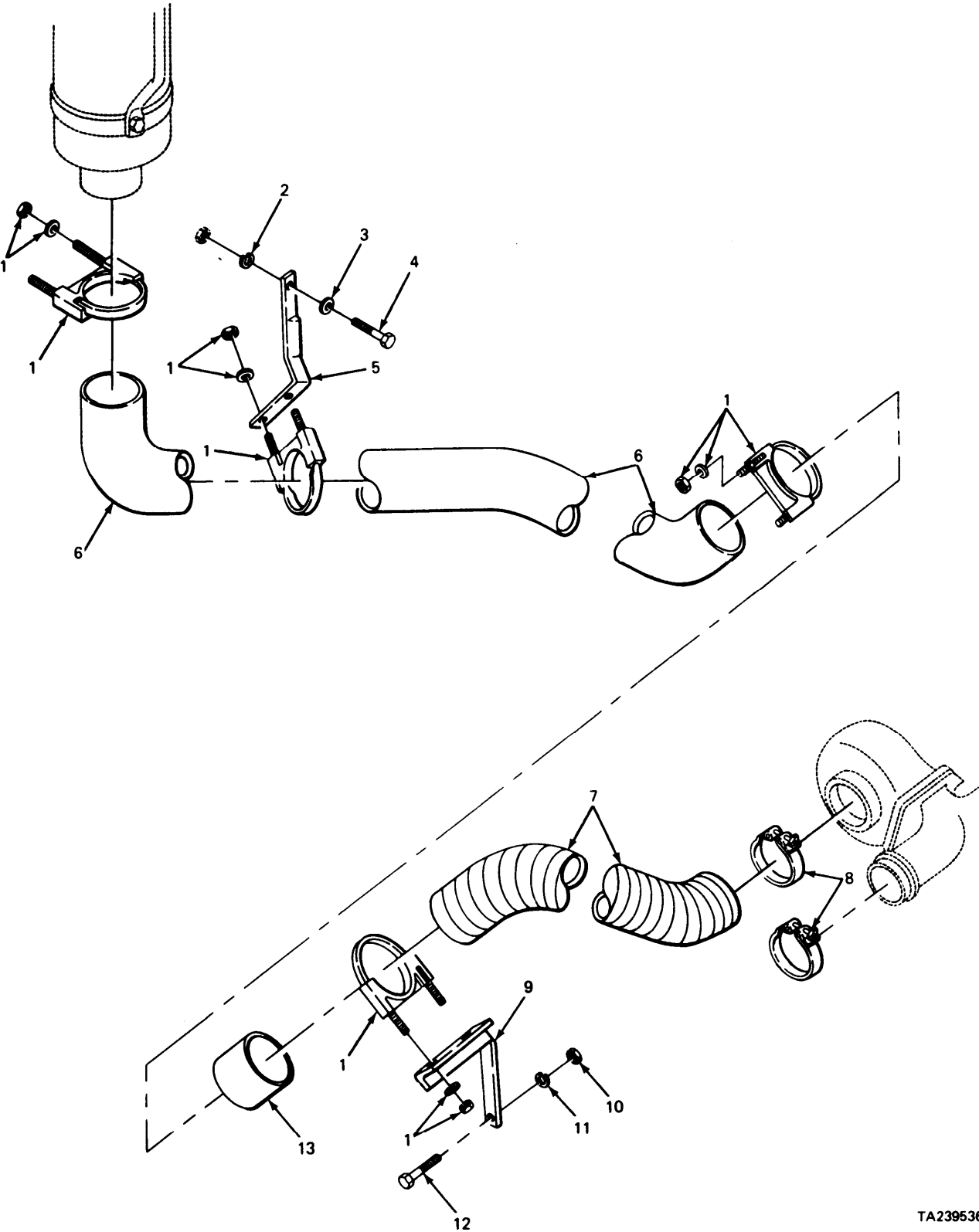
FIGURE 59. EXHAUST PIPE AND RELATED PARTS.
