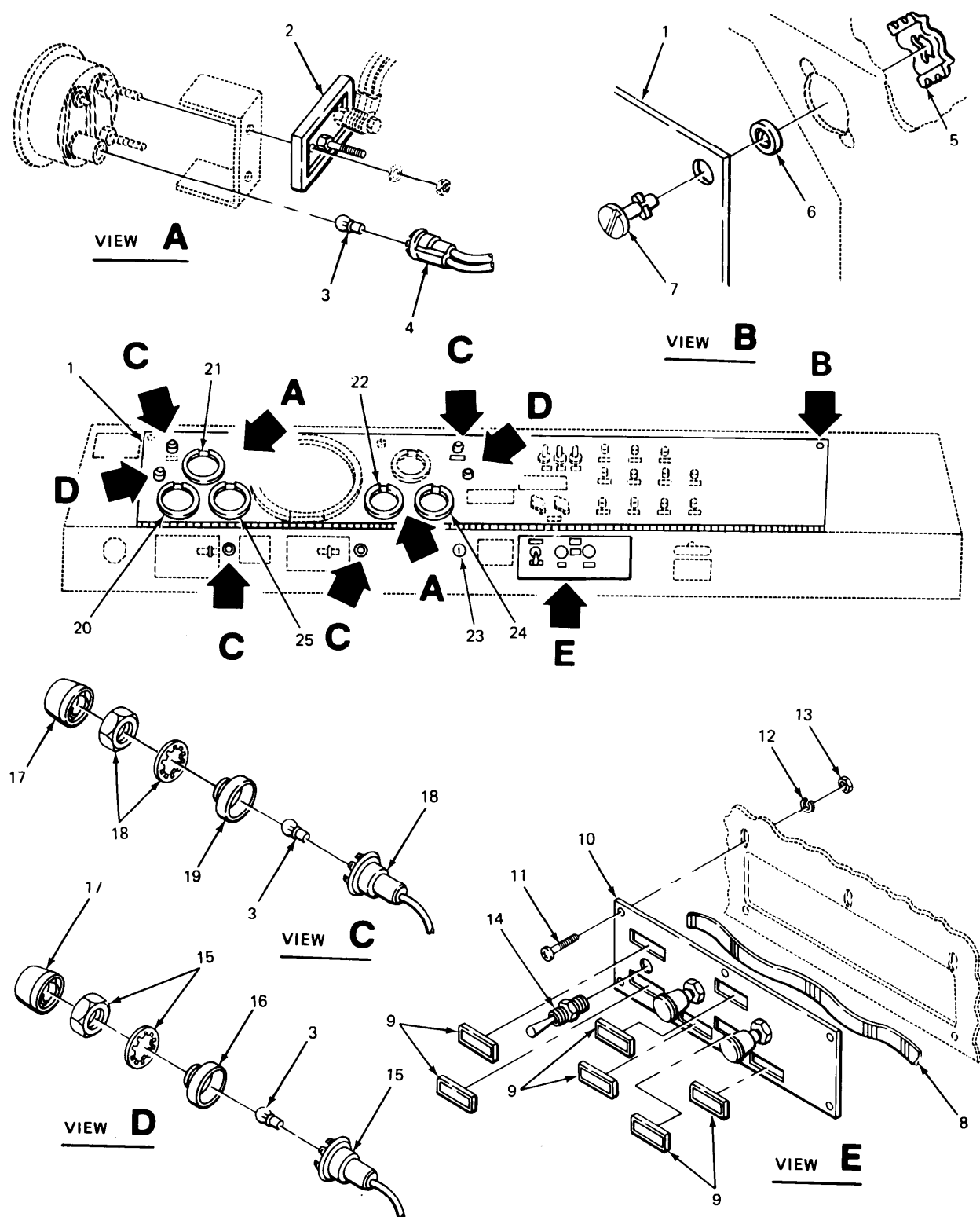
FIGURE 76. INSTRUMENT PANEL AND RELATED PARTS.
