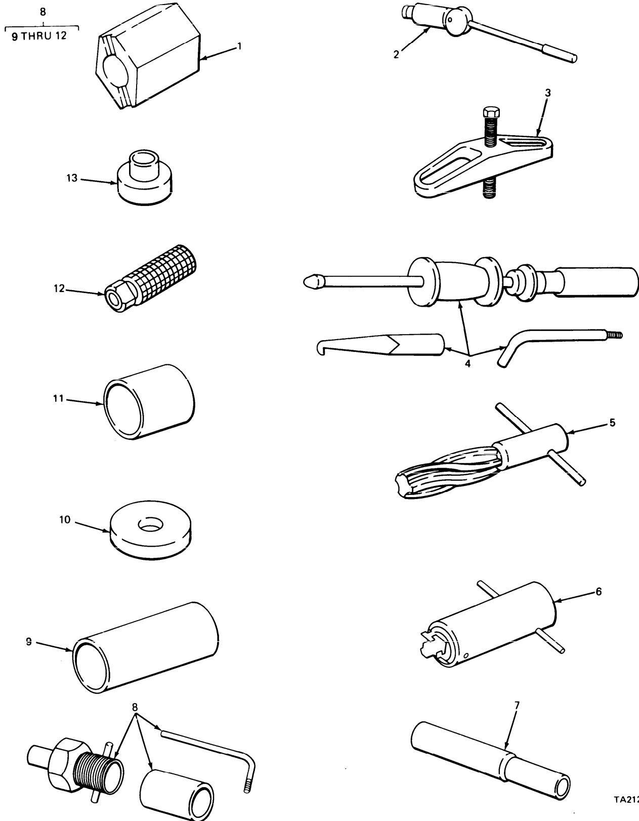
FIGURE 304. DIRECT SUPPORT SPECIAL TOOLS.
