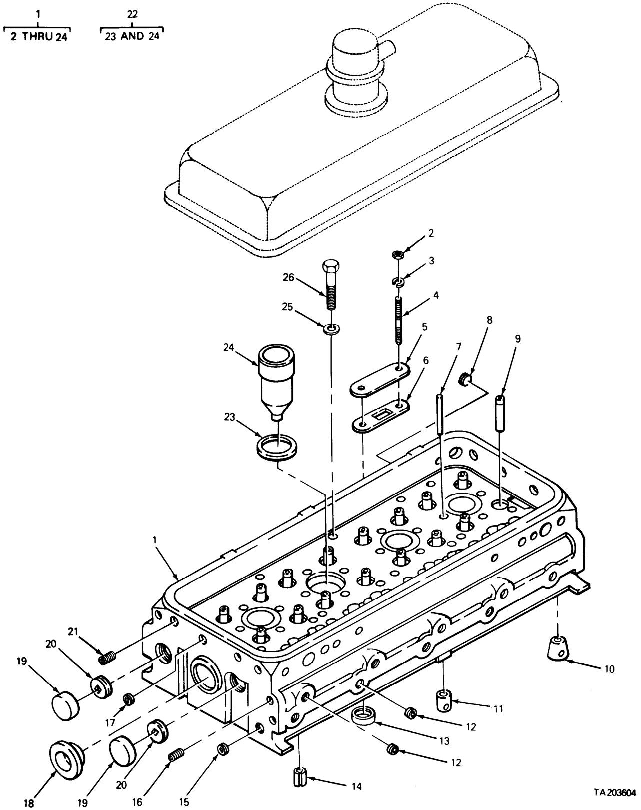
FIGURE 7. CYLINDER HEAD AND RELATED PARTS.
