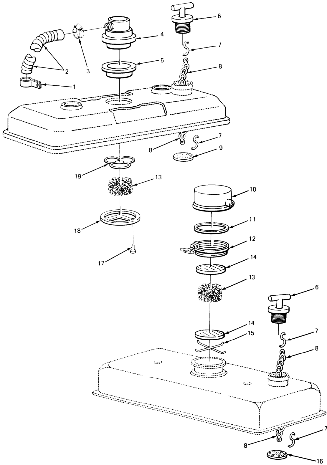
FIGURE 20. OIL FILTER, BREATHER, AND RELATED PARTS.
