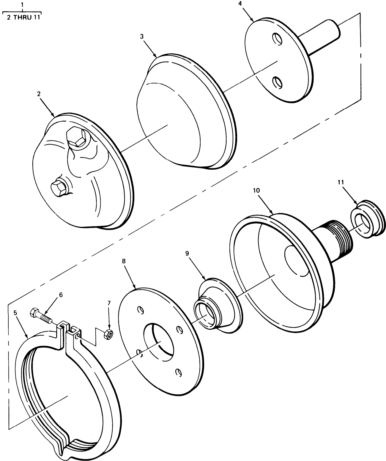
FIGURE 174. PUSHER AXLE AIR BRAKE CHAMBER.
