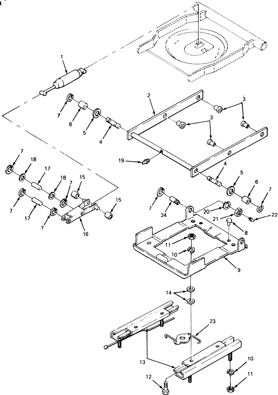
FIGURE 267. BASE ASSEMBLY AND RELATED PARTS.
