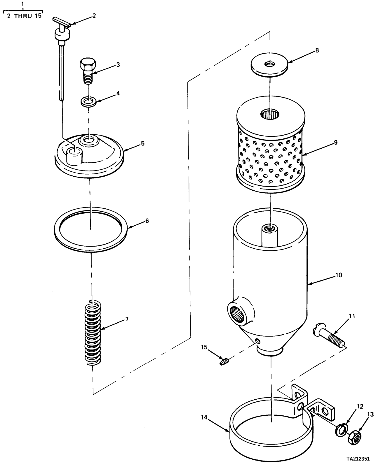
FIGURE 226. RESERVOIR AND FILTER ASSEMBLY.
