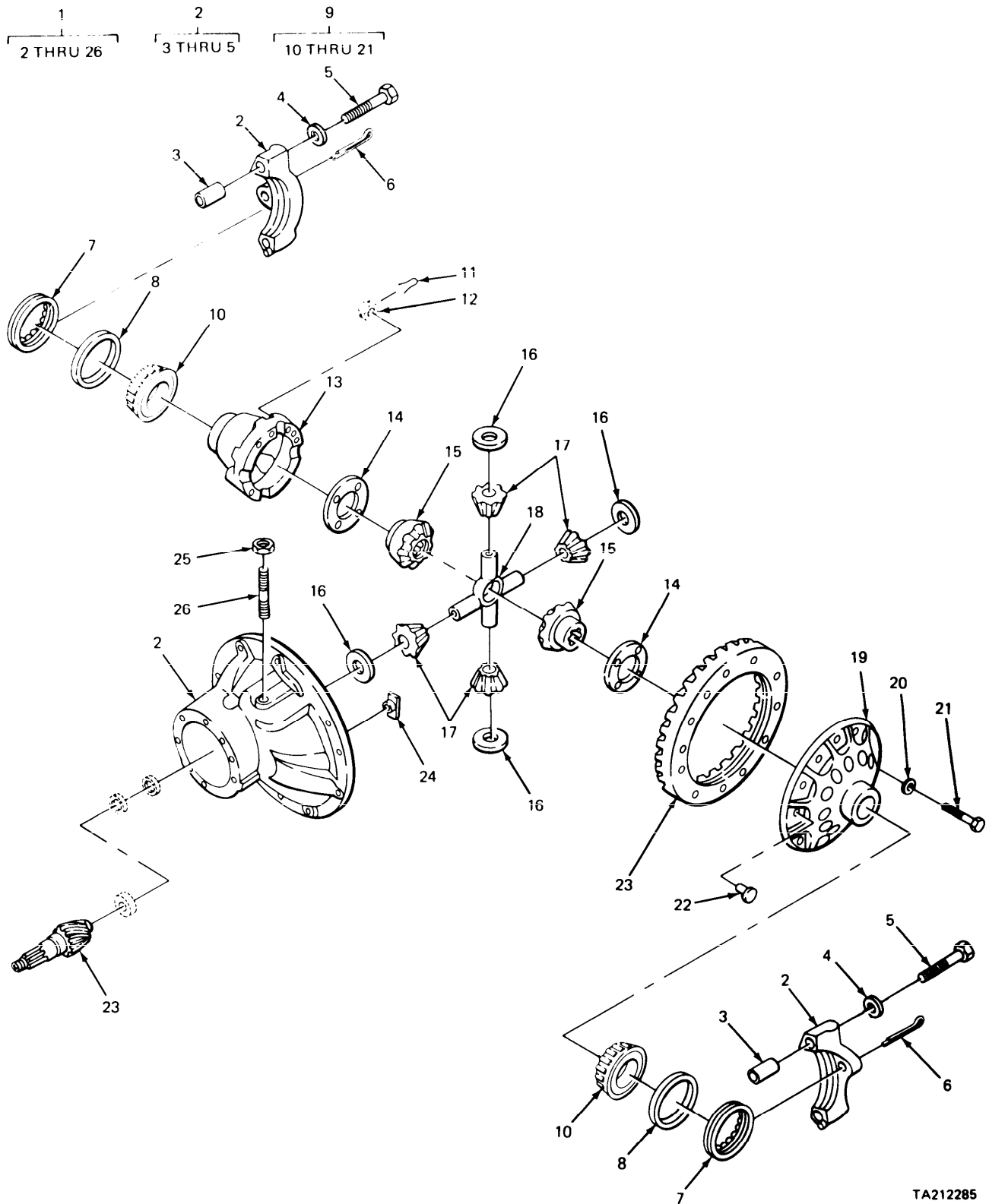
FIGURE 146. FRONT CARRIER ASSEMBLY AND RELATED PARTS.
