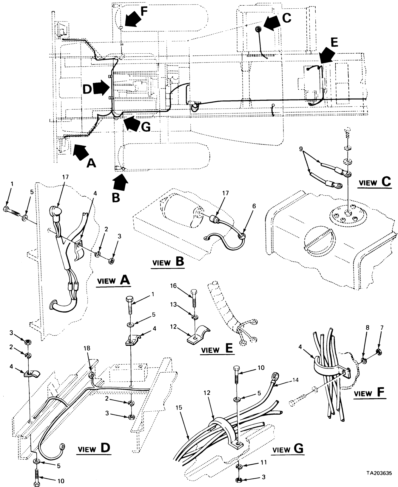
FIGURE 100. CHASSIS WIRING HARNESS (FRONT SECTION).
