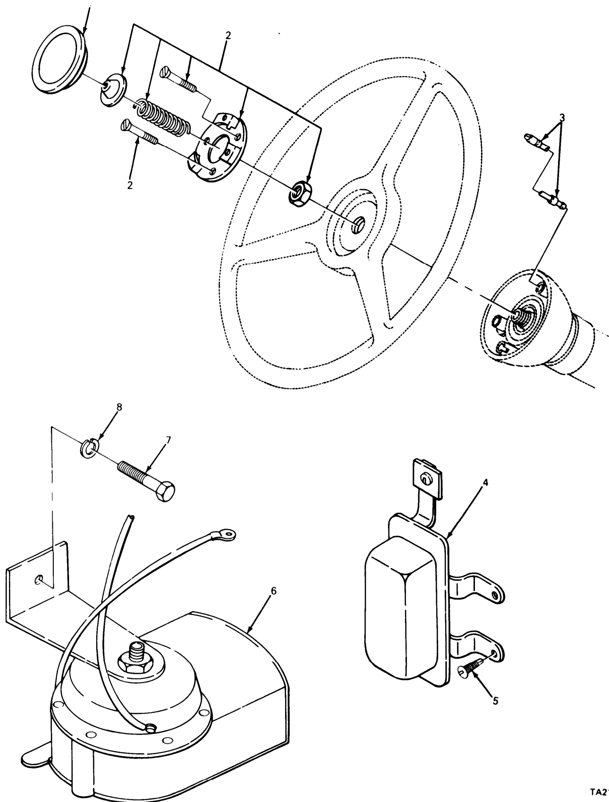
FIGURE 94. HORN AND RELATED PARTS.
