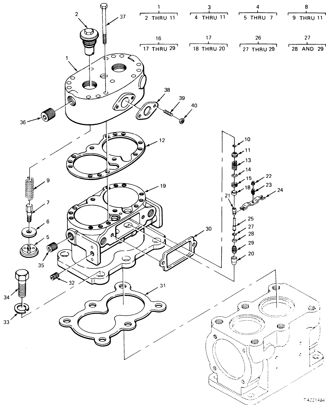
FIGURE 198. AIR COMPRESSOR HEAD AND LOCK.
