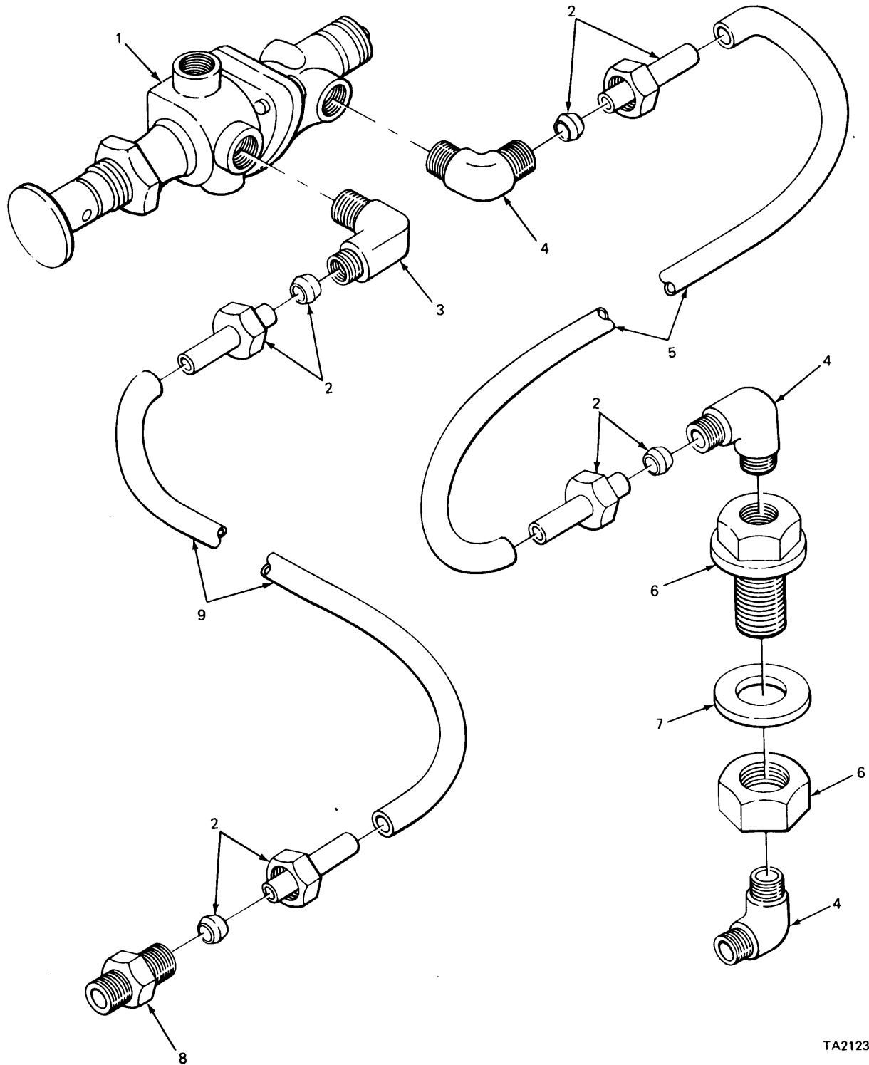
FIGURE 204. SERVICE AND DELIVERY VALVE ASSEMBLY.
