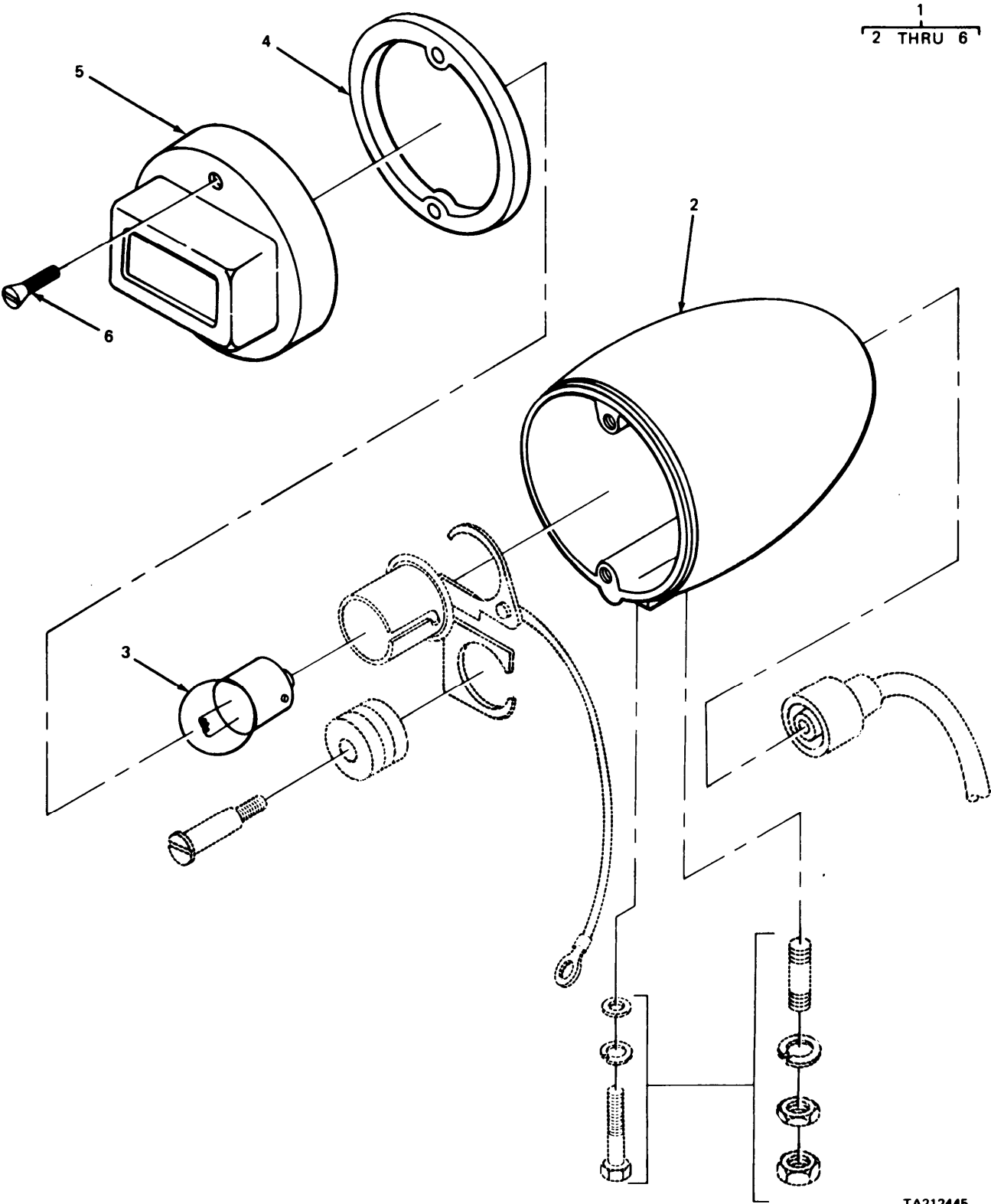
FIGURE 90. BLACKOUT CLEARANCE LIGHT.
