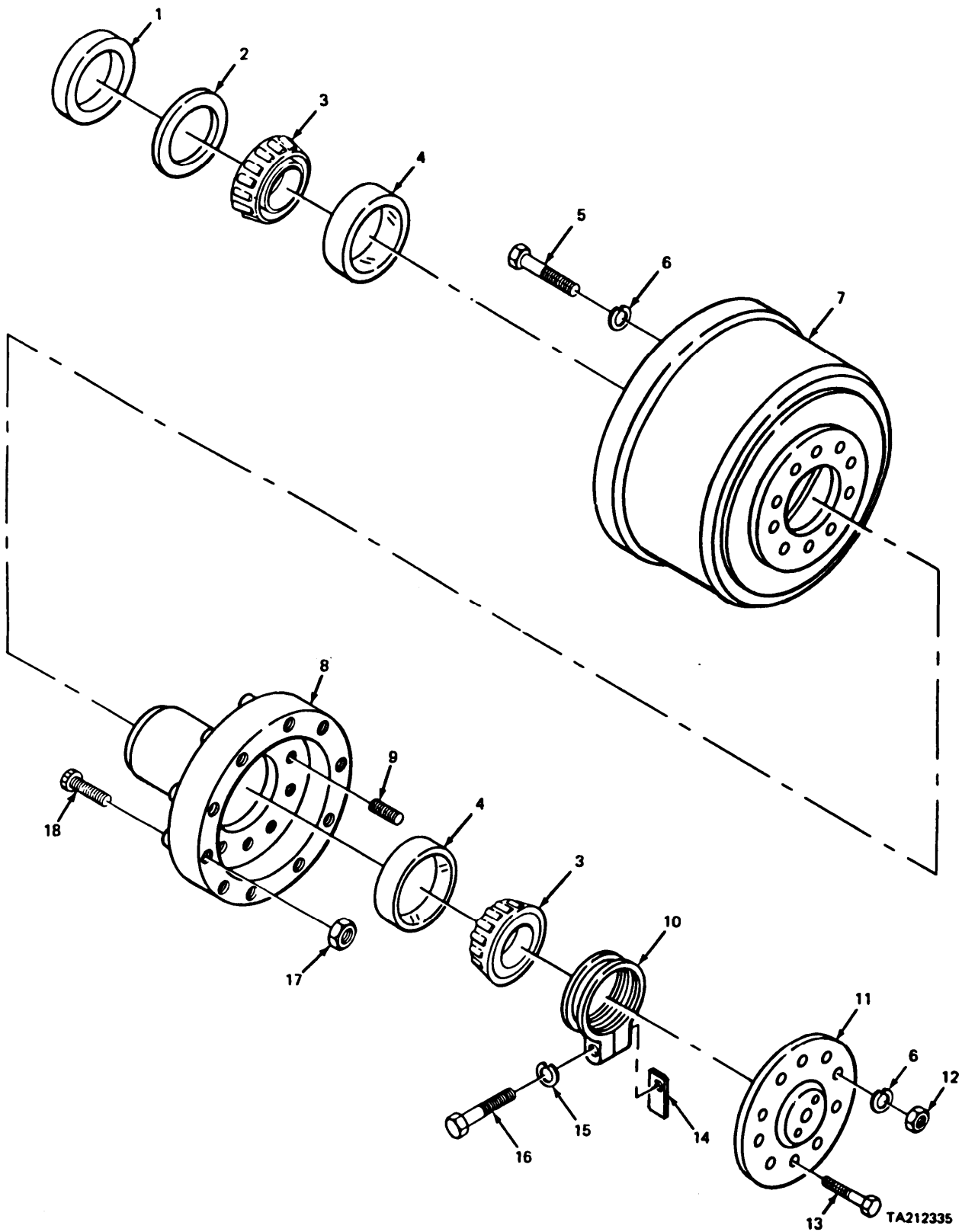
FIGURE 209. FRONT BRAKE DRUM AND HUB ASSEMBLY.
