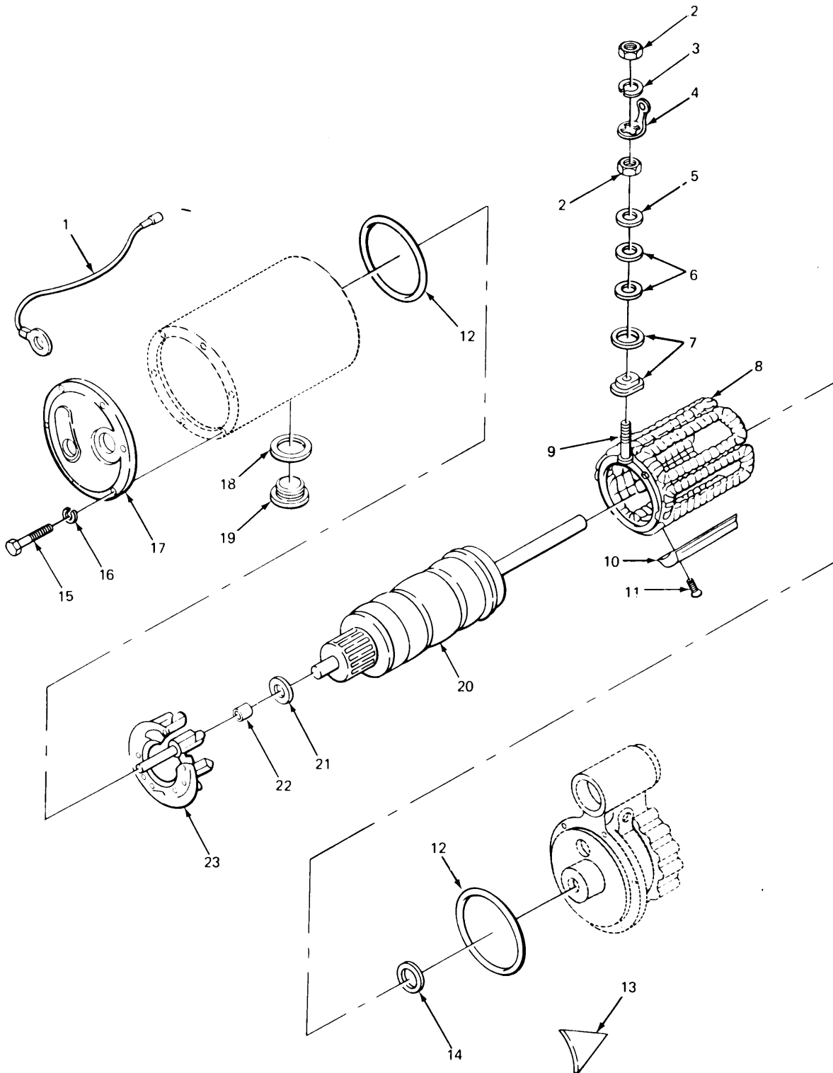
FIGURE 73. STARTER ARMATURE AND RELATED PARTS.
