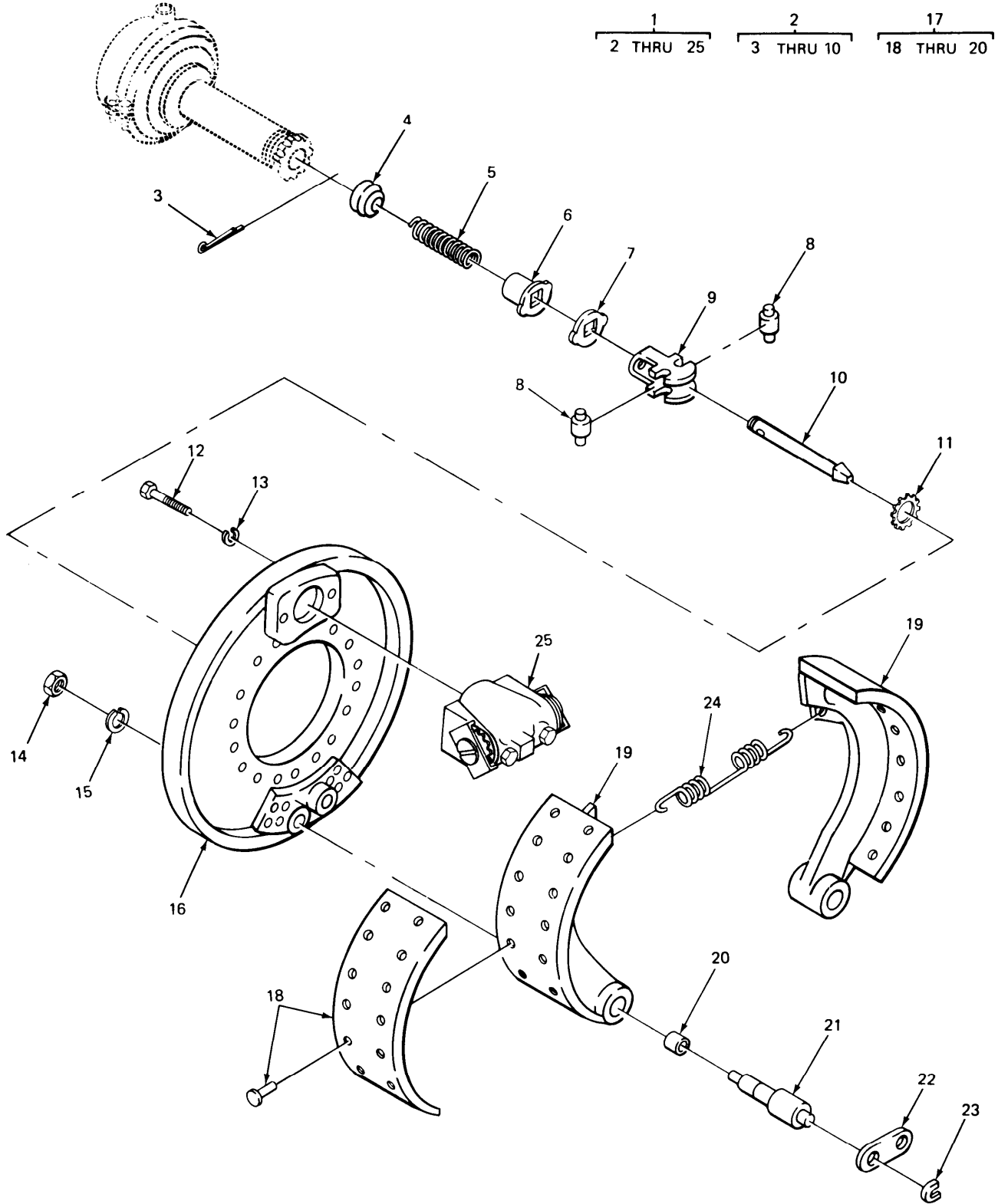
FIGURE 167. FRONT BRAKE ASSEMBLY,
