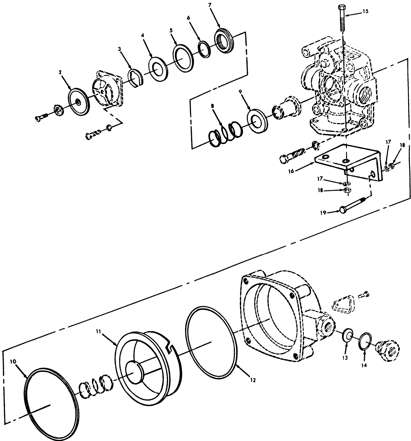
FIGURE 188. RELAY VALVE.
