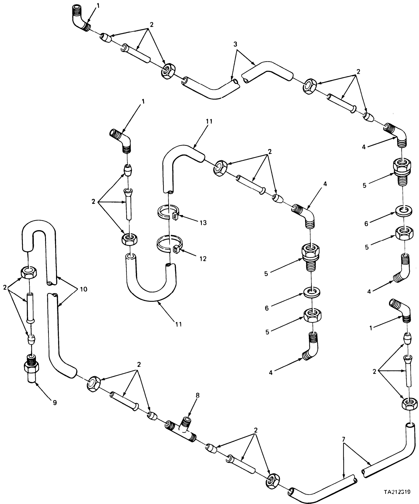
FIGURE 186. AIR TANK LINES AND FITTINGS.
