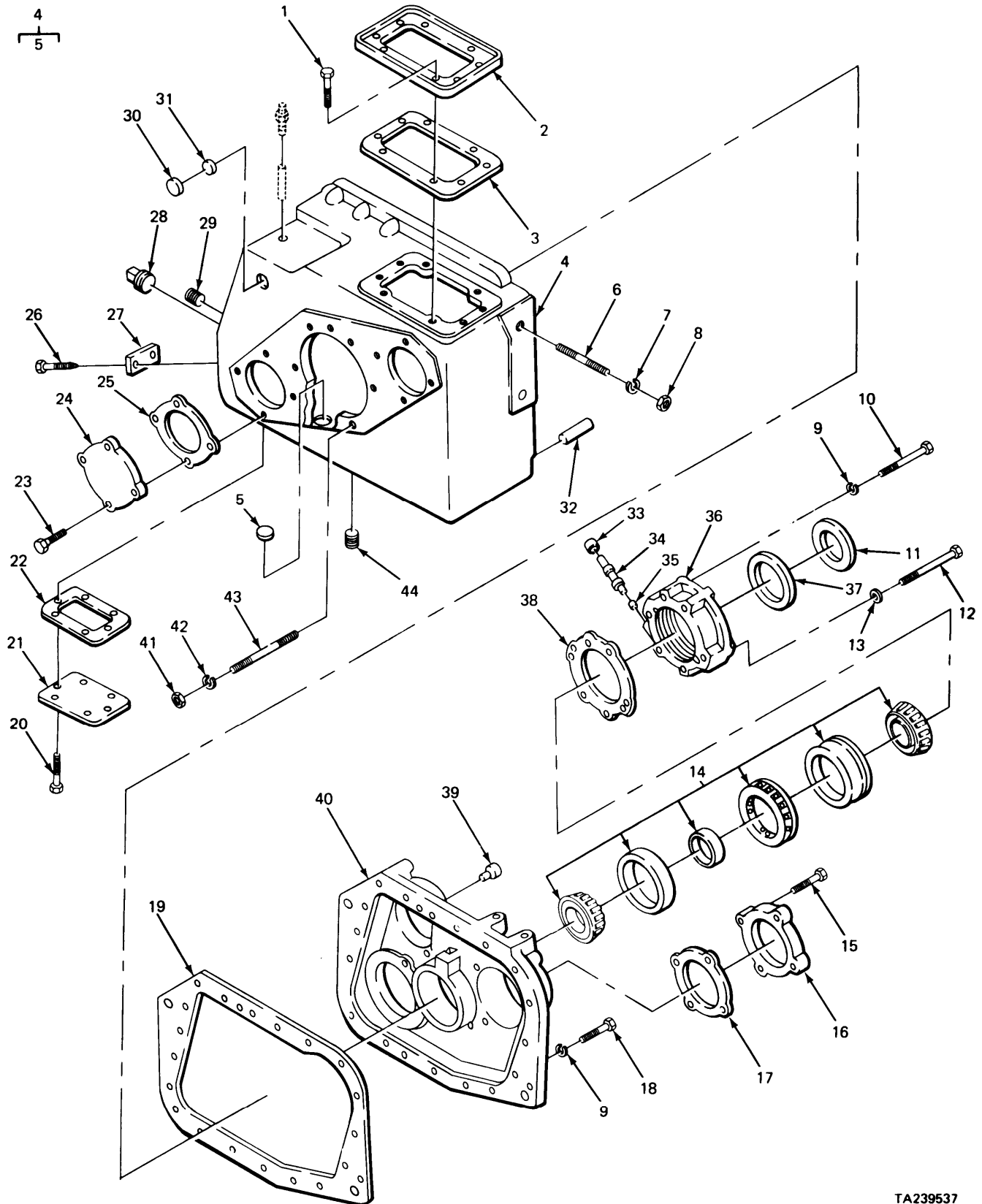
FIGURE 107. AUXILIARY TRANSMISSION EXPLODED VIEW.
