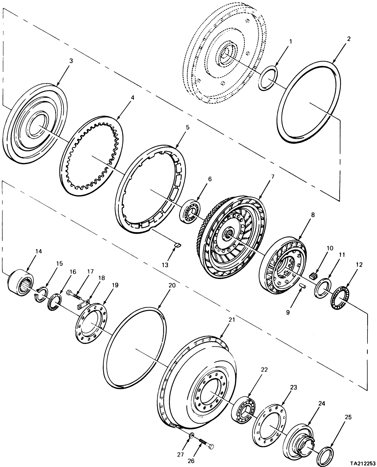
FIGURE 111. TORQUE CONVERTER AND RELATED PARTS.
