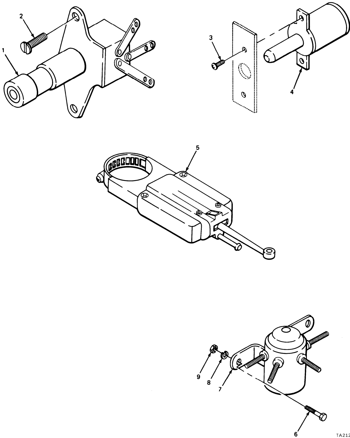
FIGURE 79. SENDING SWITCHES.
