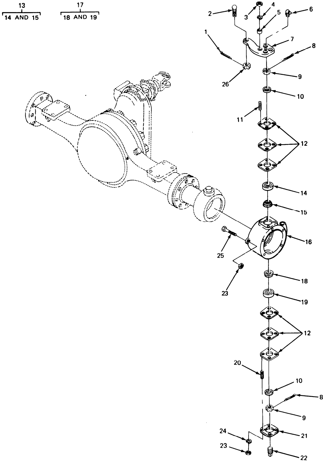
FIGURE 148. AXLE BALL AND RELATED PARTS.
