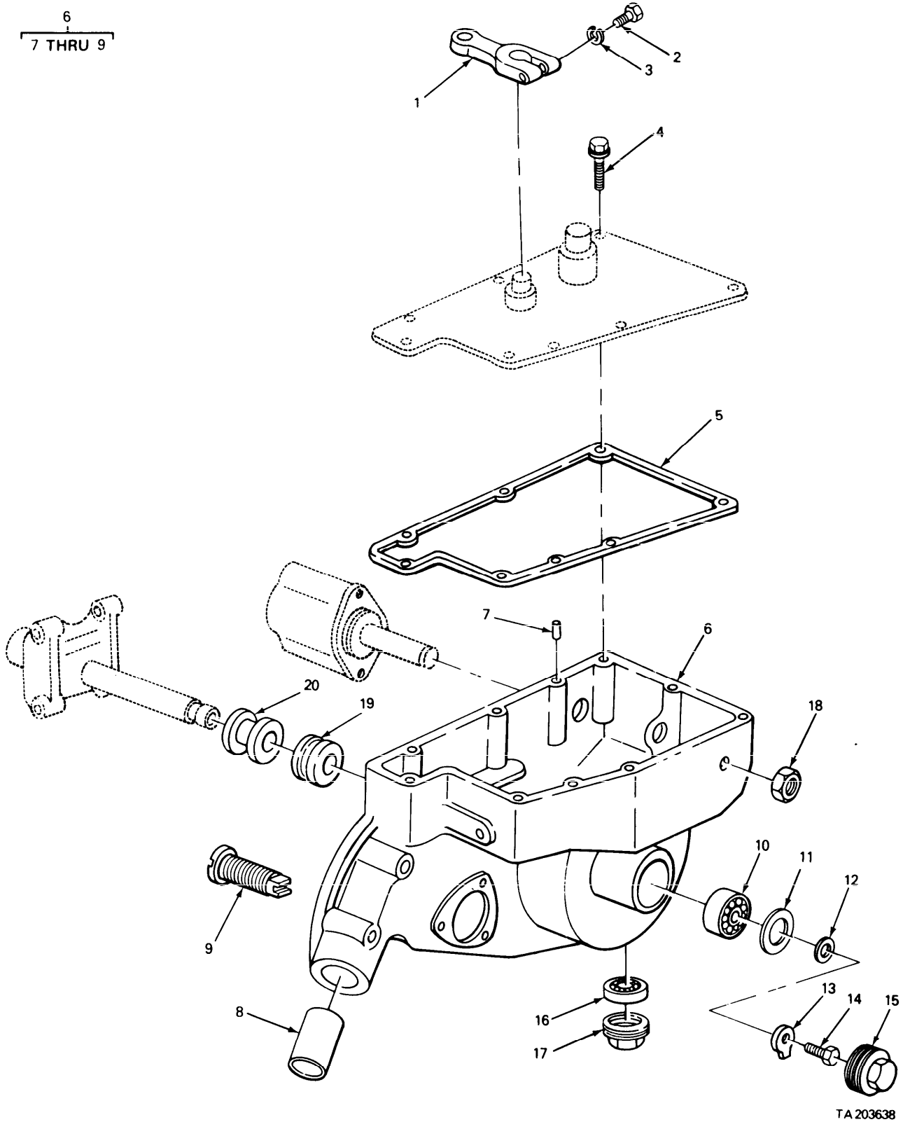
FIGURE 47. GOVERNOR EXPLODED VIEW.
