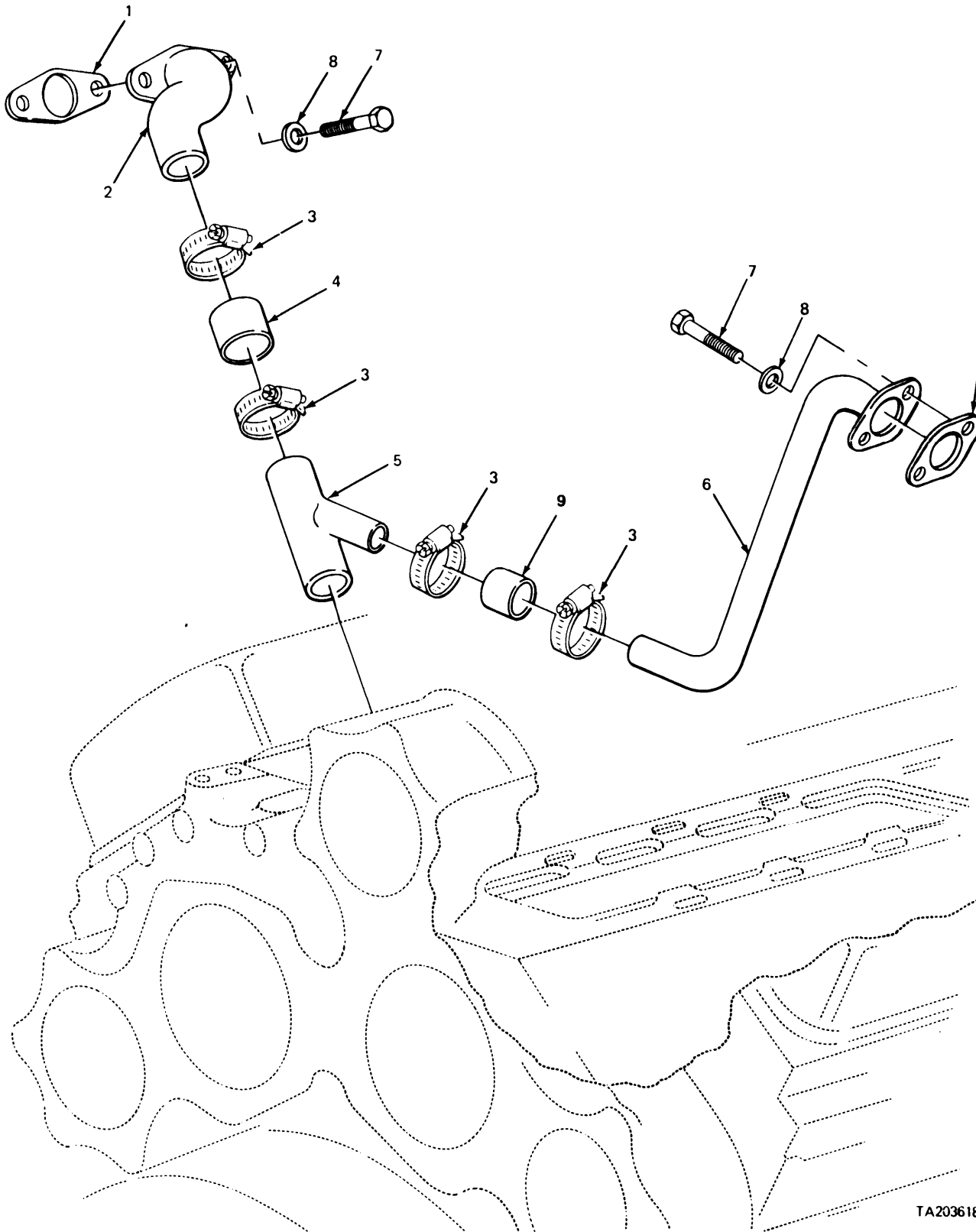
FIGURE 23. BREATHER TUBES AND RELATED PARTS.
