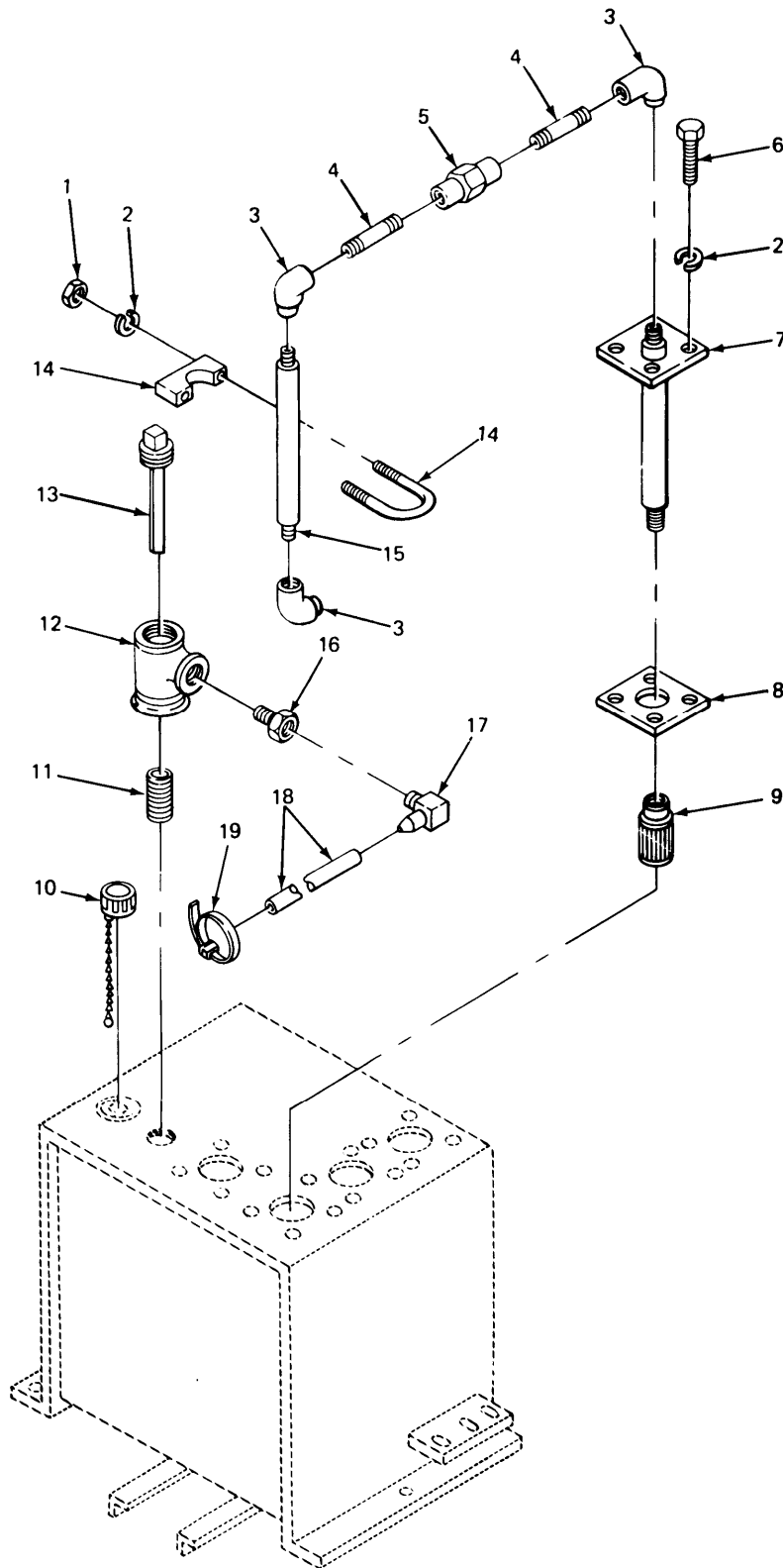
FIGURE 282. RESERVOIR ASSEMBLY EXPLODED VIEW.
