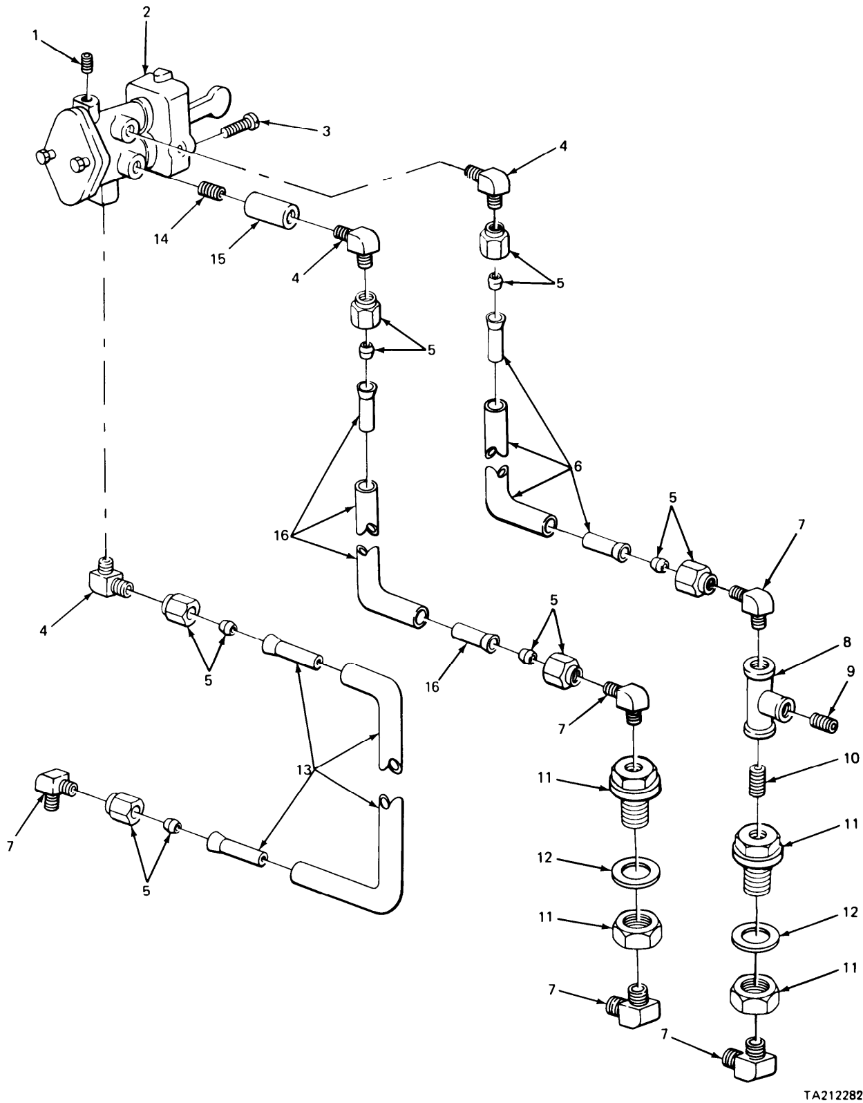
FIGURE 143. TRANSFER CASE LOCKUP VALVE AND RELATED PARTS.
