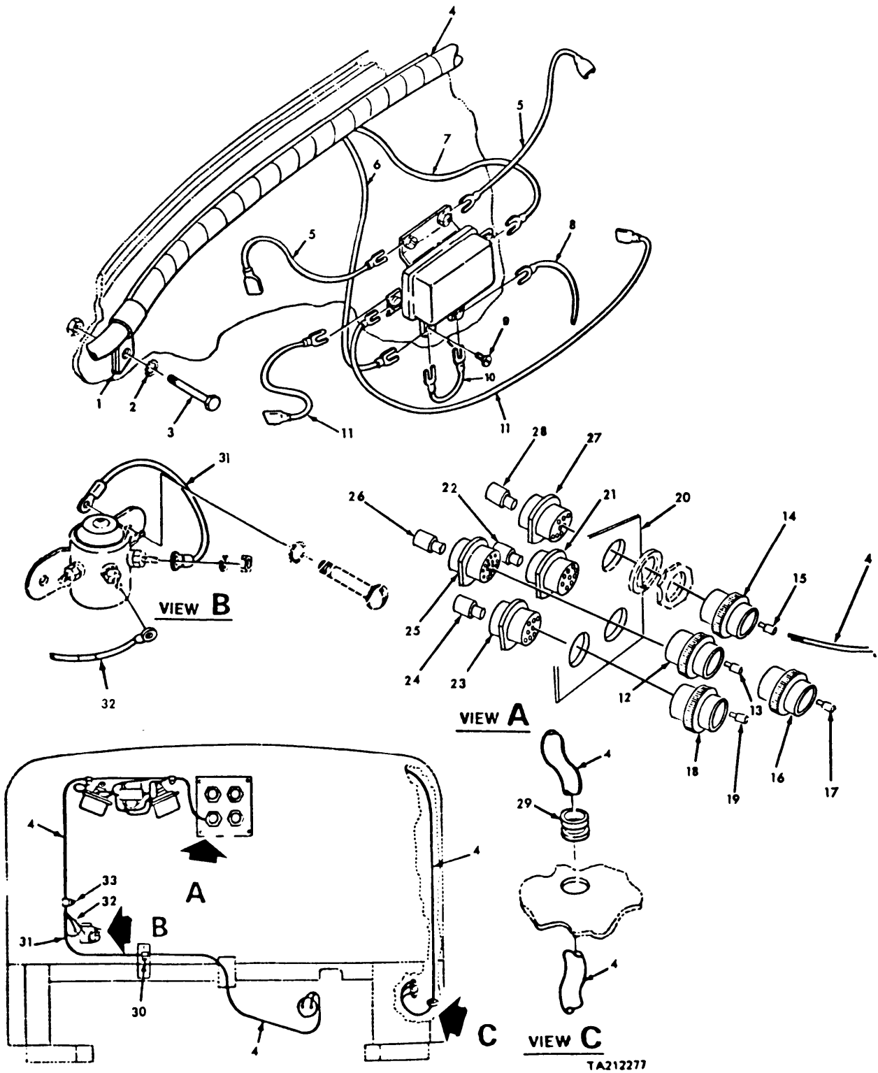
FIGURE 103. CAB WIRING (FIREWALL SECTION).
