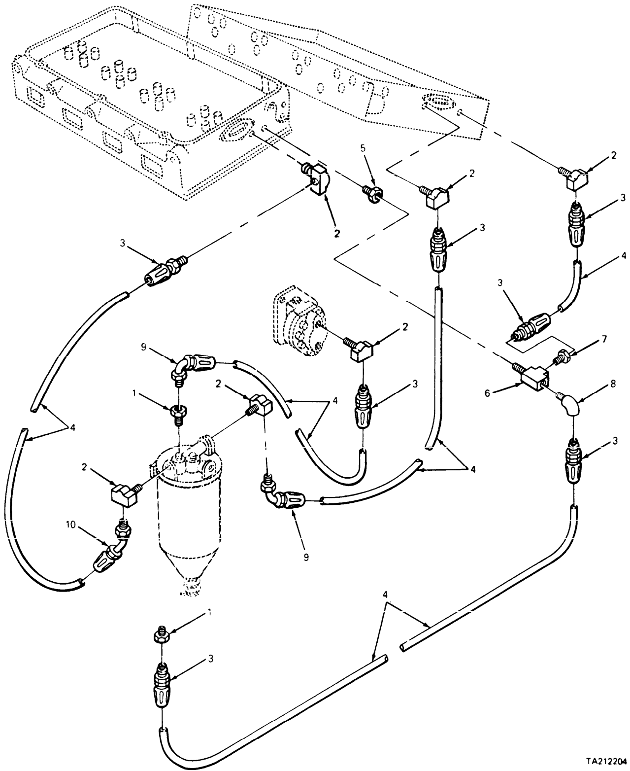
FIGURE 37. FUEL LINES AND FITTINGS.
