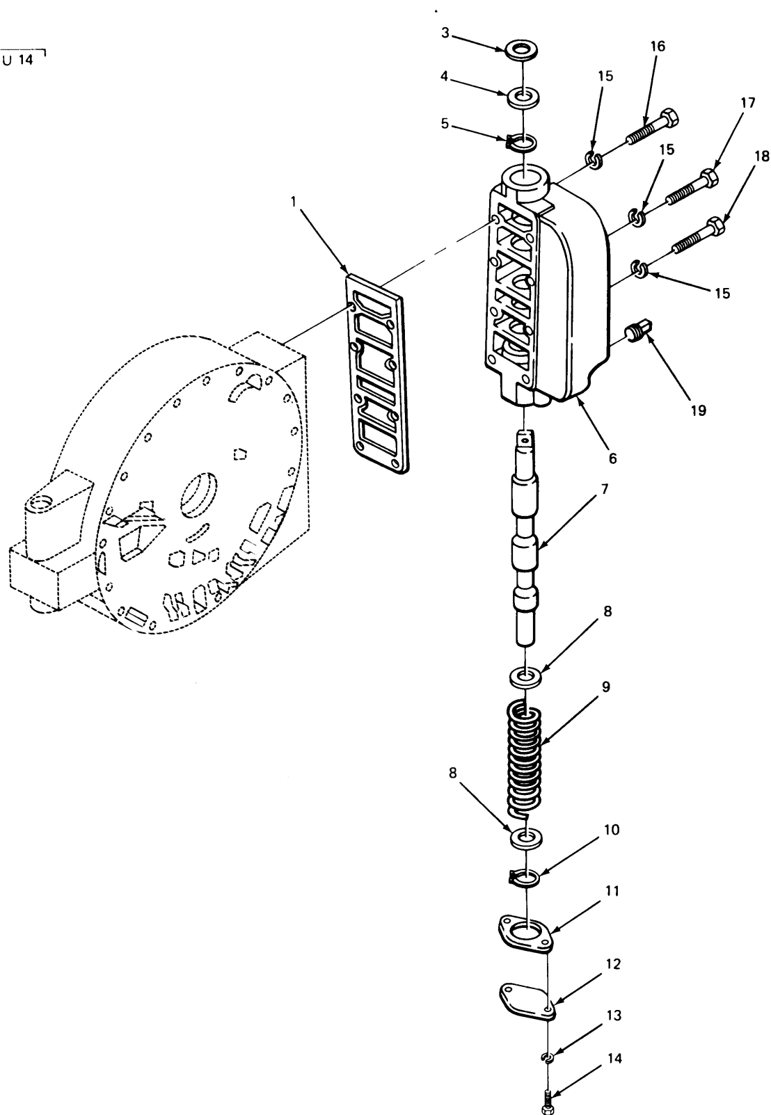
FIGURE 126. RETARDER CONTROL VALVE AND RELATED PARTS.
