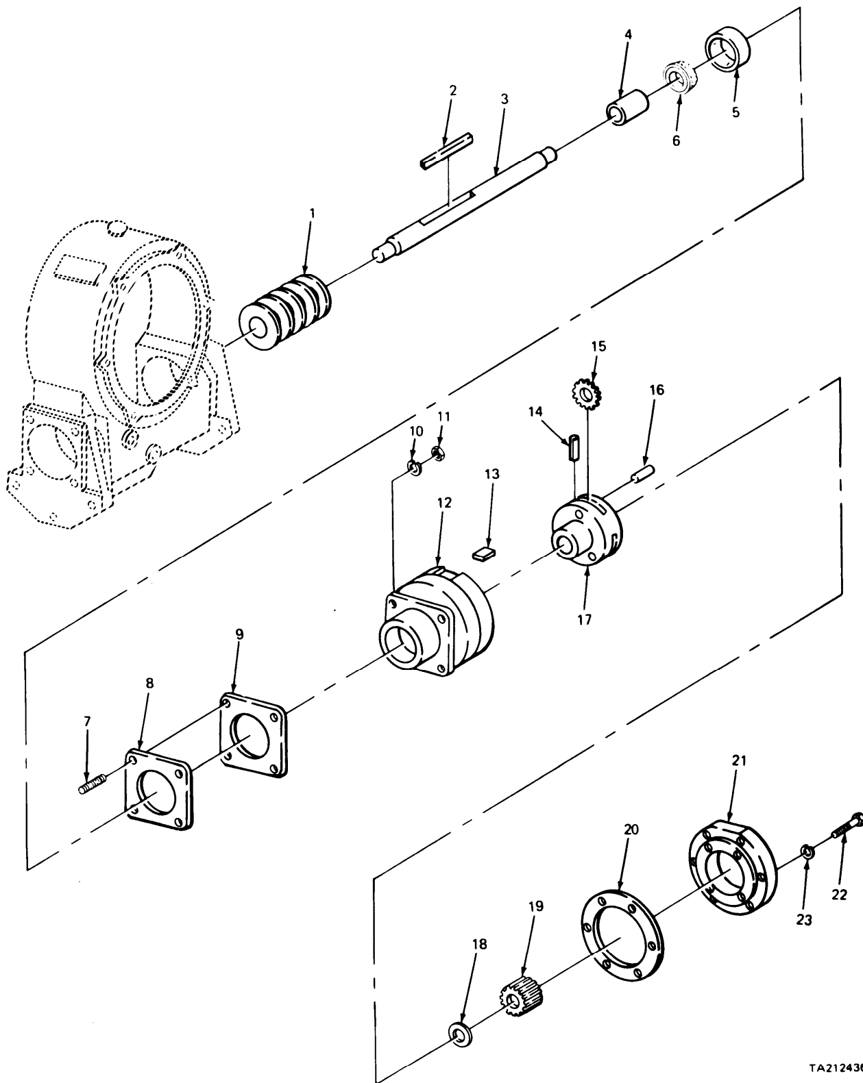
FIGURE 272. WINCH ASSEMBLY EXPLODED VIEW.
