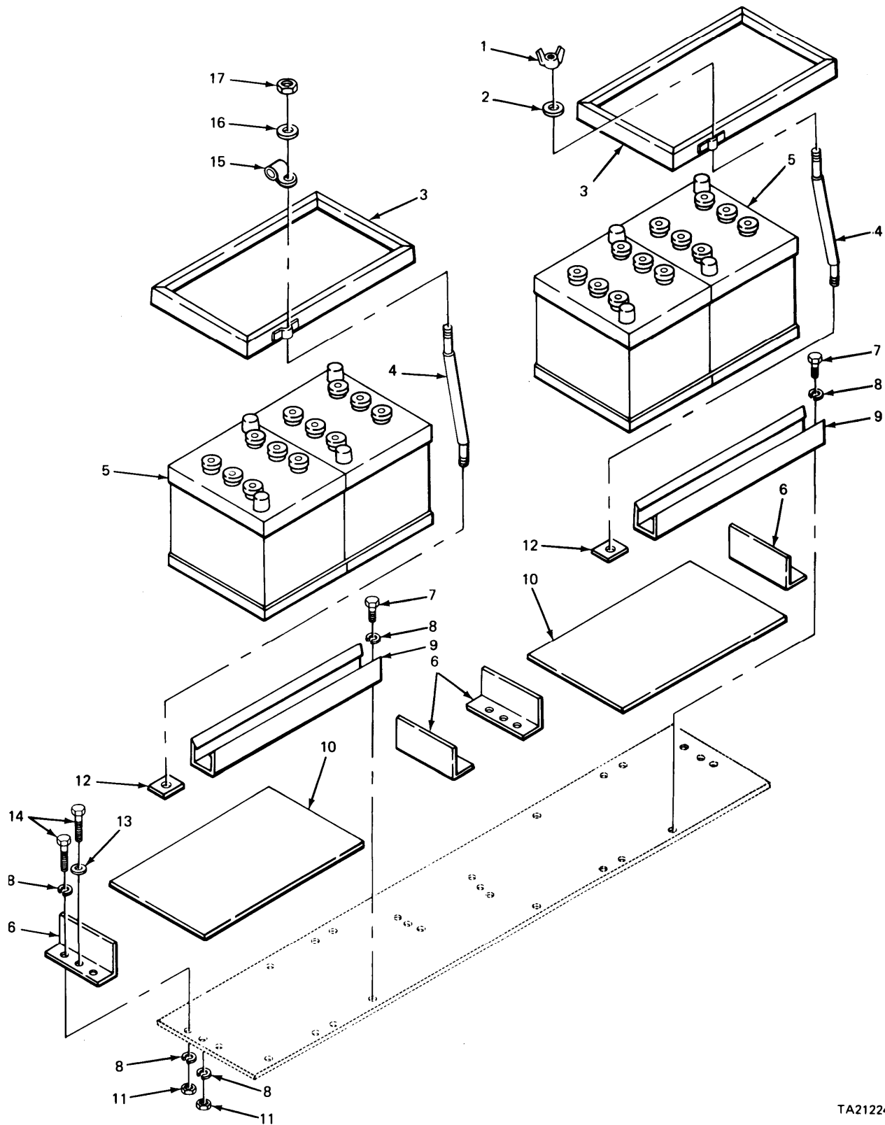
FIGURE 96. BATTERY AND RETAINER ASSEMBLY.
