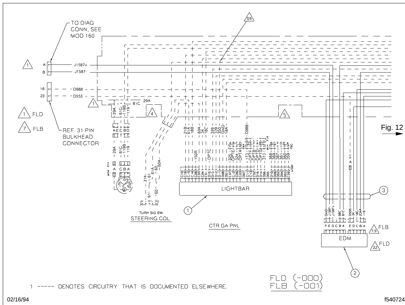
Fig. 11, Electronic Data Monitor (EDM) Wiring Diagram, Detroit Diesel Series 50 and 60 Engines With DDEC III (enlarged portion of Figure 10)
