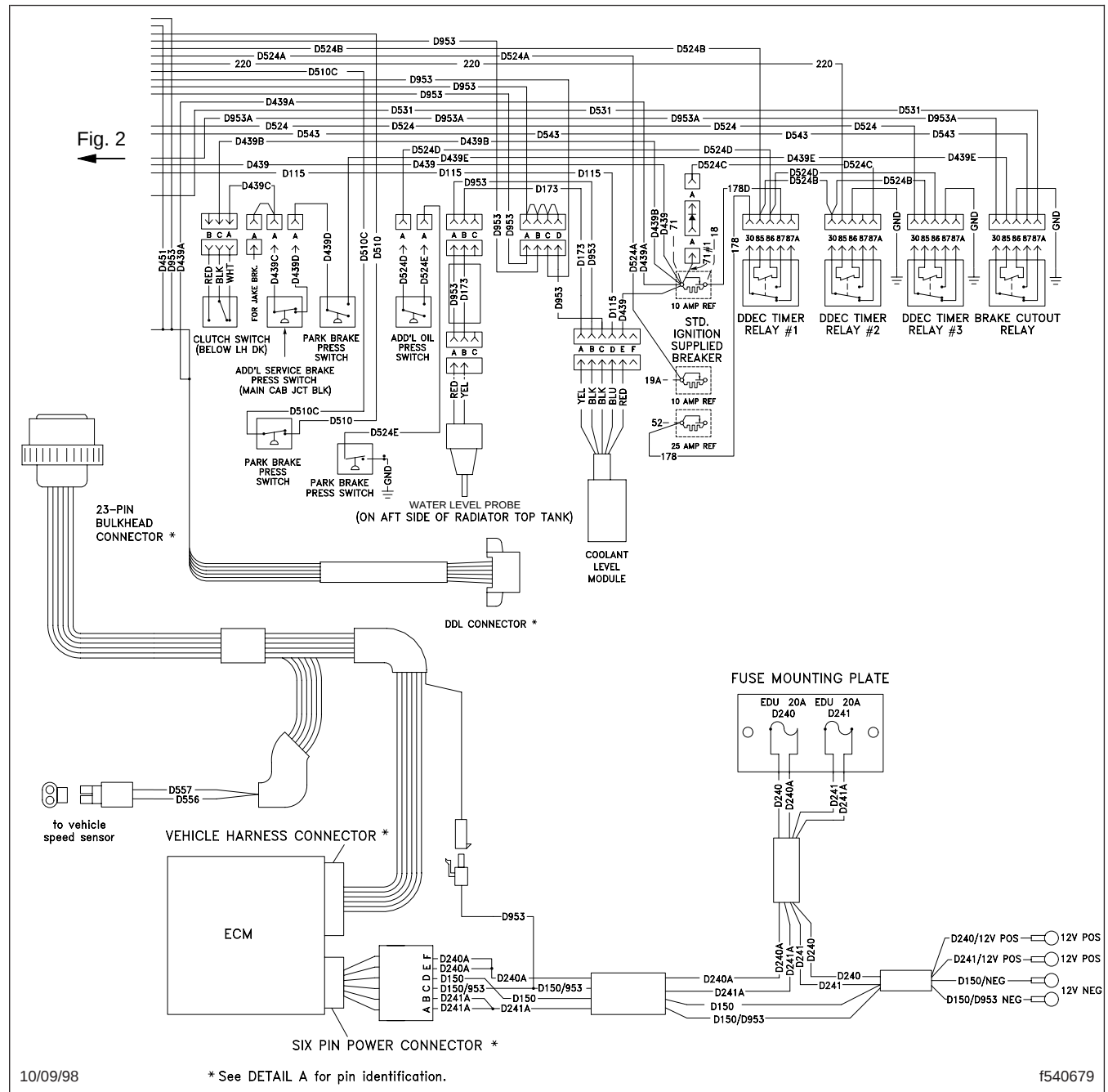
Fig. 3, DDEC II Wiring Diagram (enlarged portion of Figure 1)
