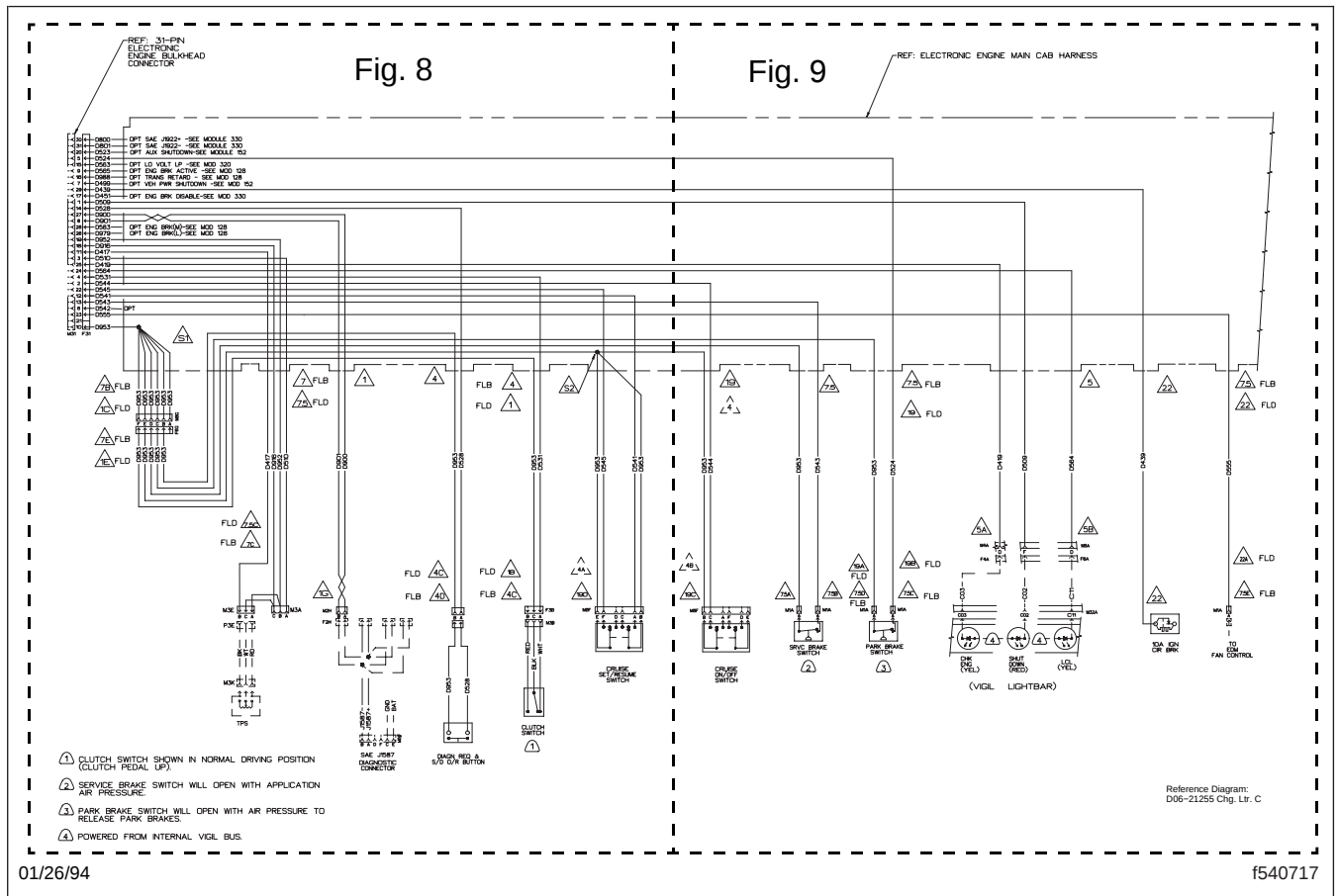
Fig. 7, Detroit Diesel Series 50 and 60 Engines With DDEC III Wiring Diagram (cab-harness side)
