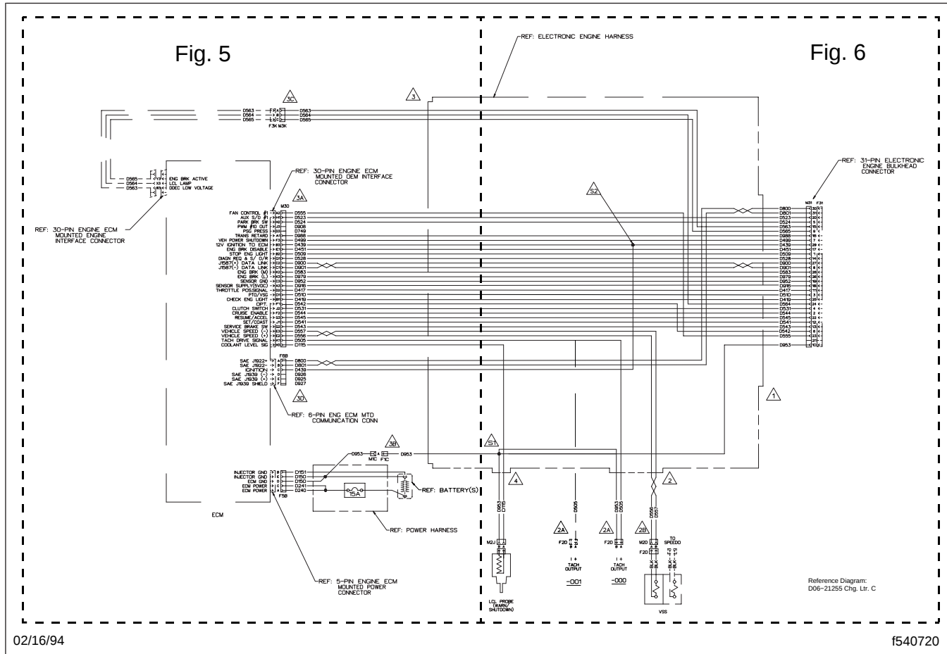
Fig. 4, Detroit Diesel Series 50 and 60 Engines With DDEC III Wiring Diagram (engine-harness side)
