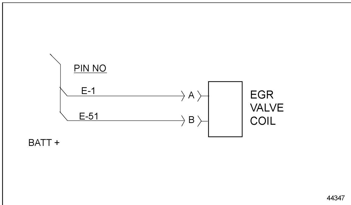
Figure 9-1 EGR Valve Coil Wiring
