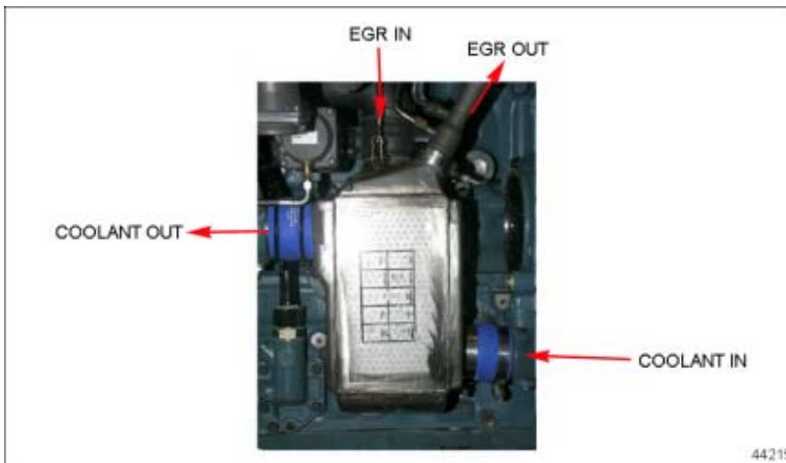
Figure 2-10 EGR Cooler (Bar and Fin Design)
