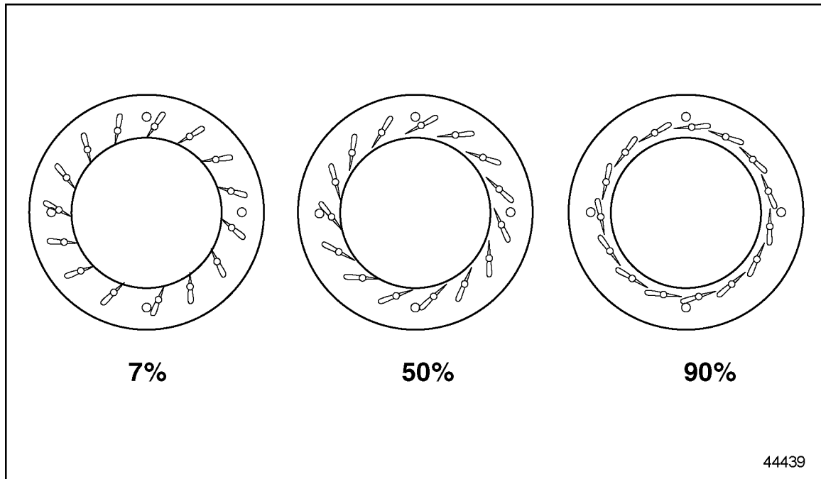
Figure 2-7 VNT Vane Position
