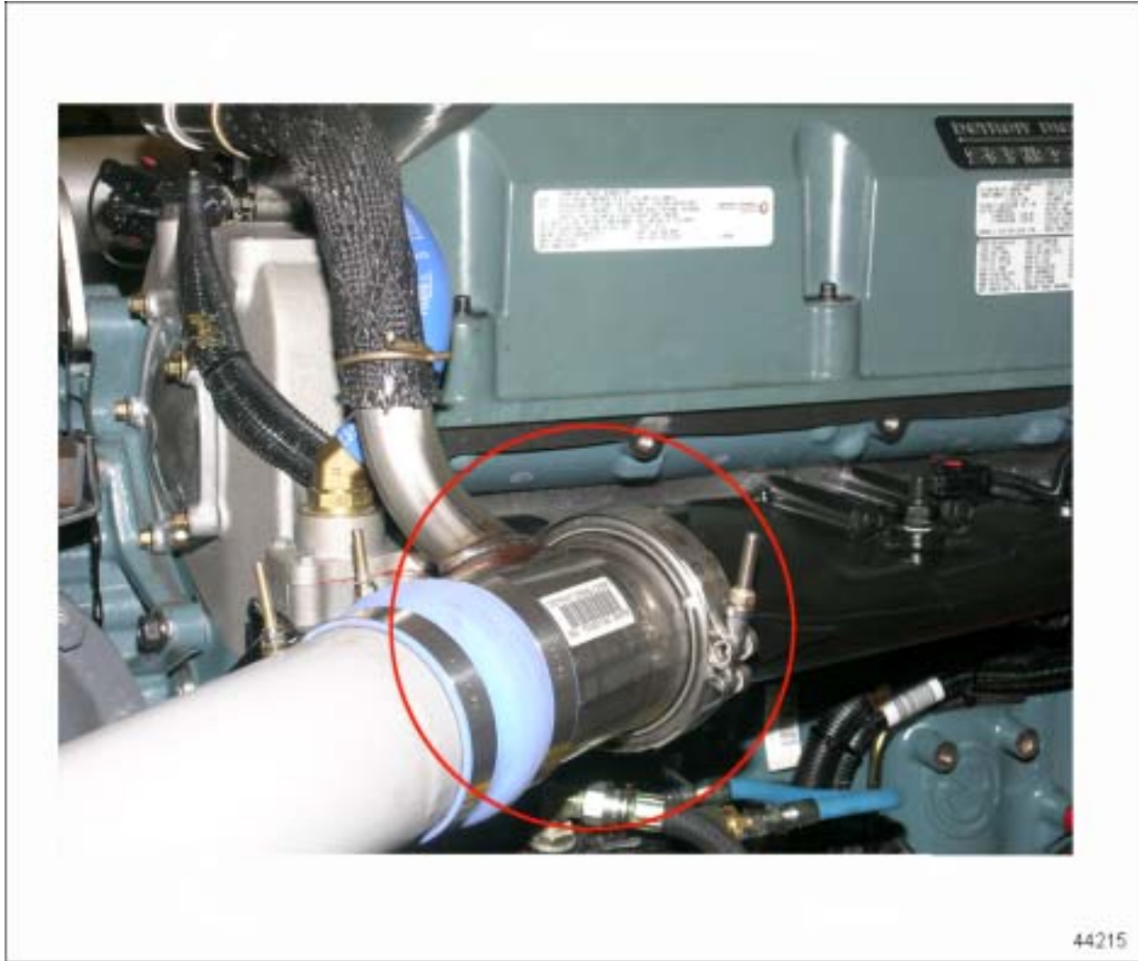
Figure 2-14 EGR Mixer
