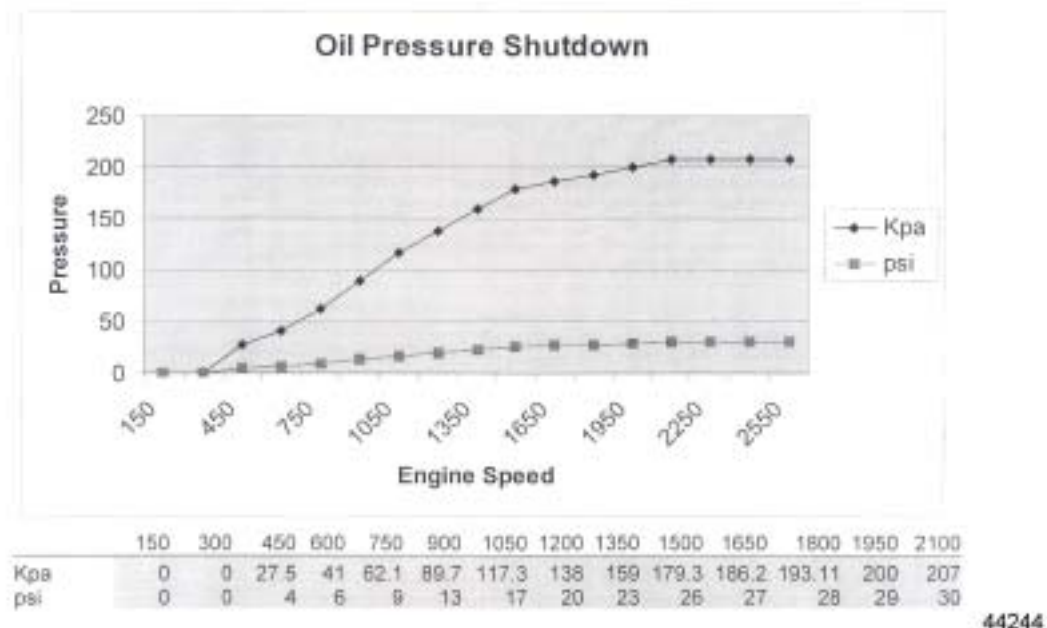
Figure 4-1 Oil Pressure Shutdown
