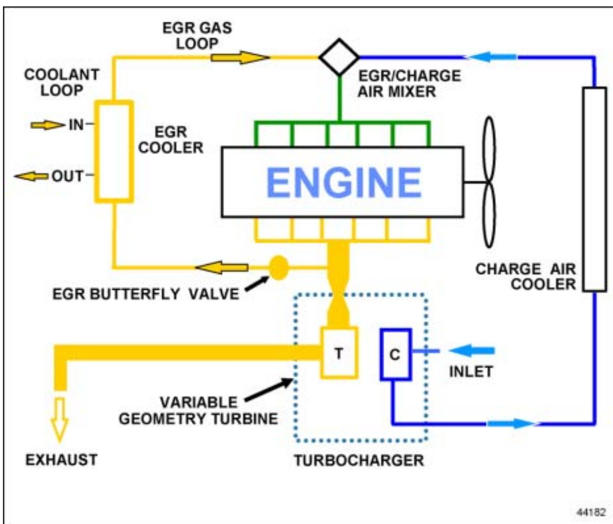
Figure 2-1 EGR System
