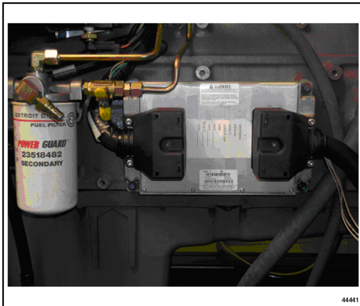
Figure 8-1 DDEC V ECU
