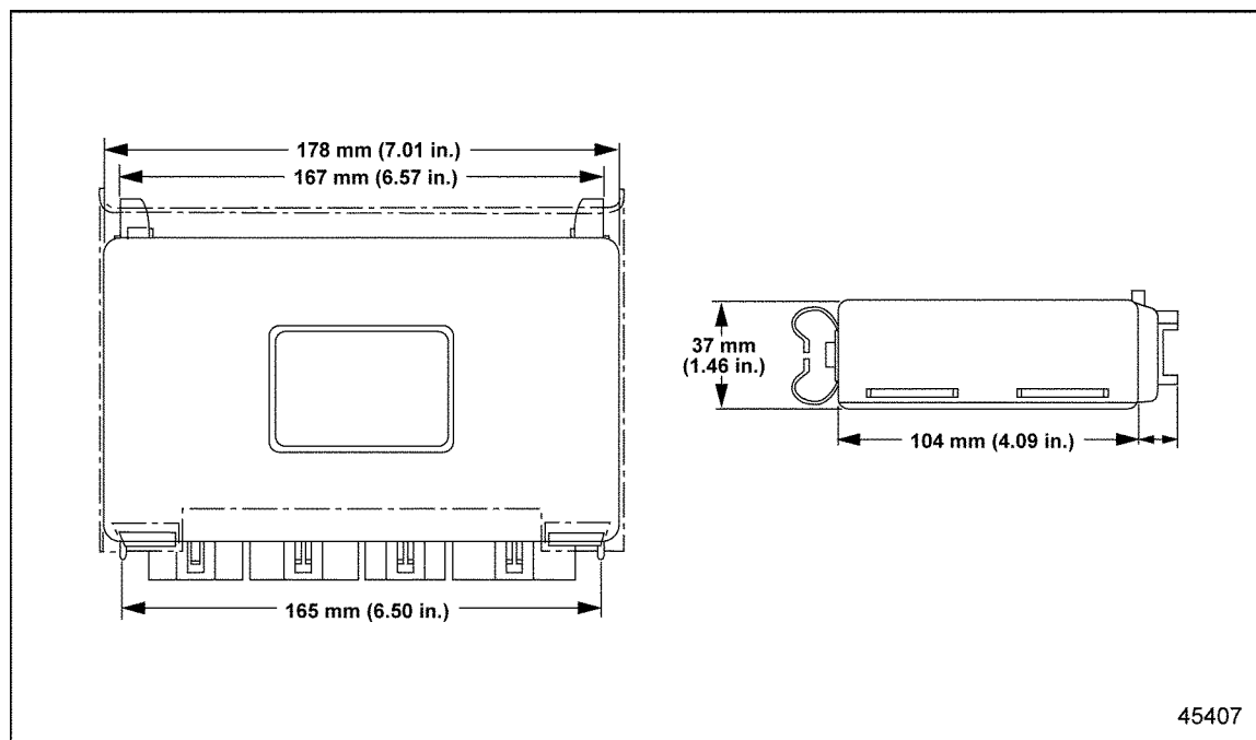
Figure 2-4 CPC Dimensions
