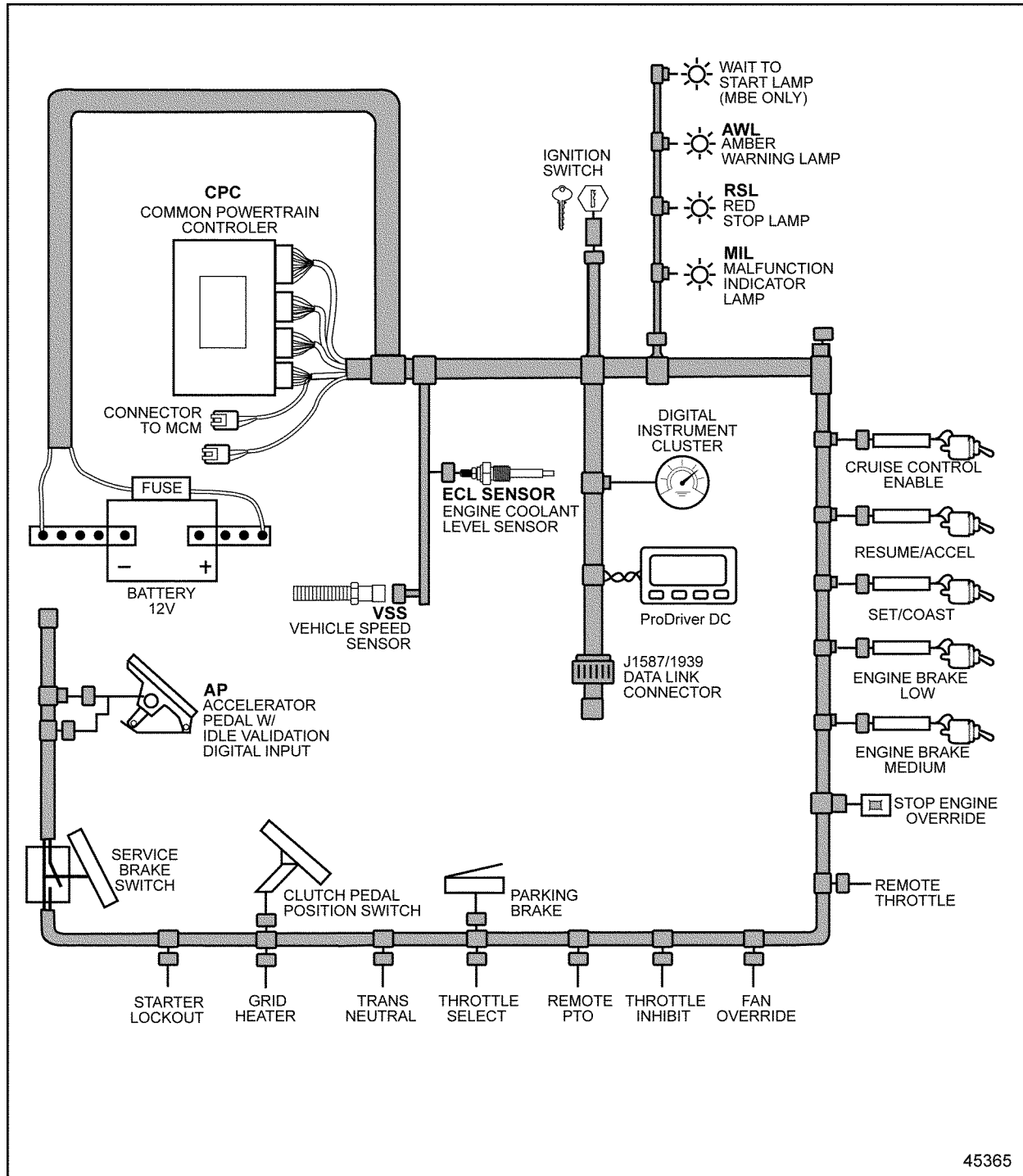
Figure 2-6 Vehicle Interface Harness
