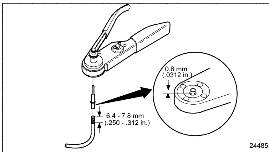
Figure 2-9 Setting Wire Gage Selector and Positioning the Contact
