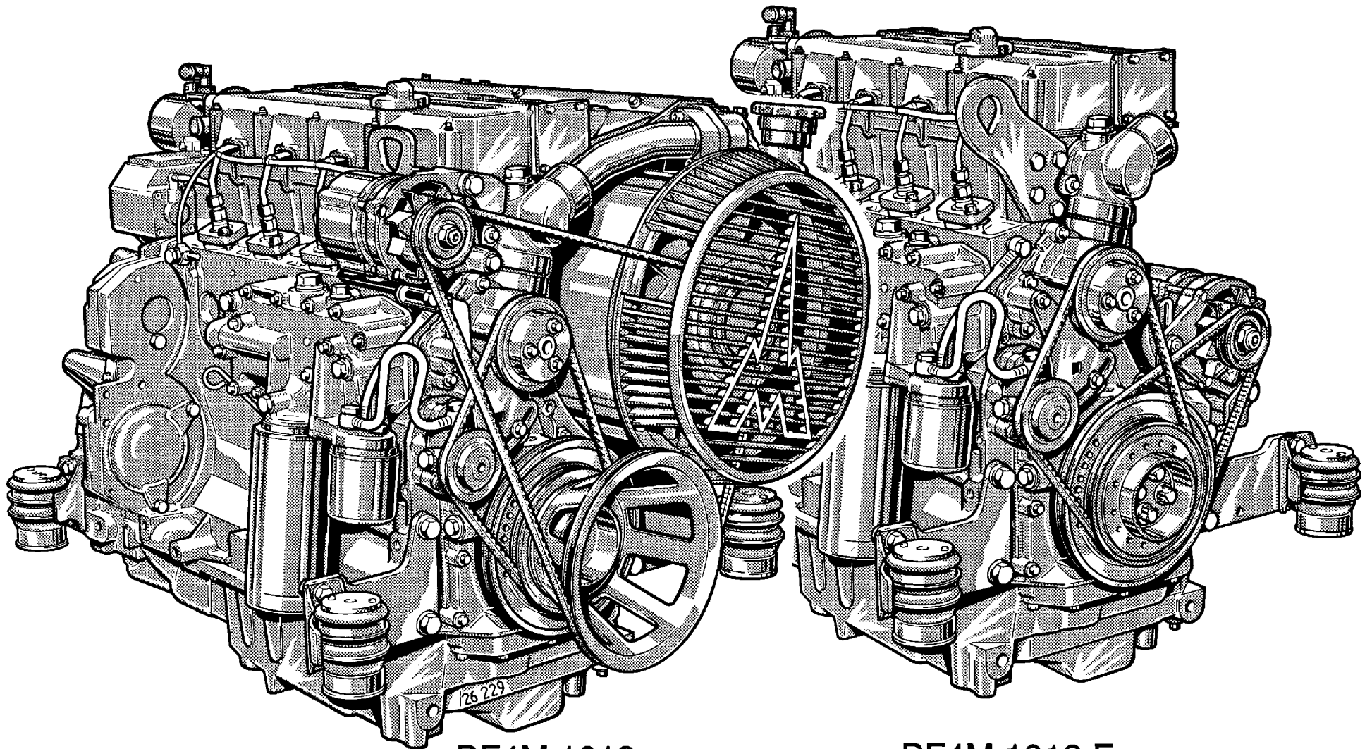
BF4M 1012
