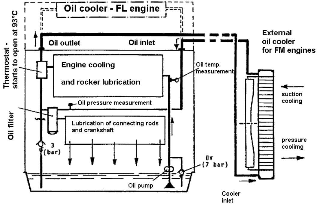
FIG. 1-23 Oil circuit schematic in B/FL/FM 1011F / 2011
