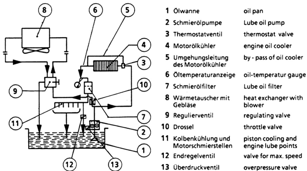
Sub-flow system
