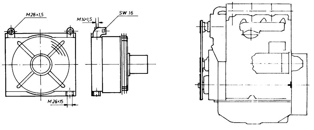
FIG. 1 - 36 Separate cooler system with electric fan drive
