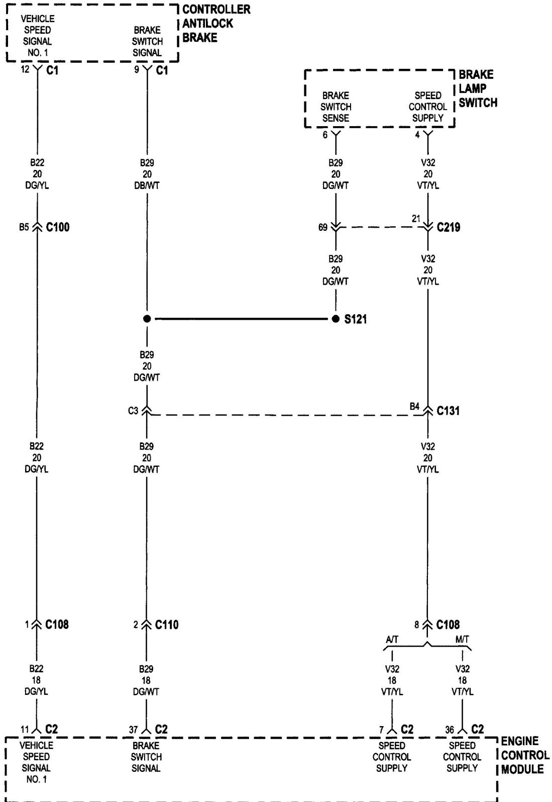
Figure C126-16 Brake lamp switch and ABS controller
