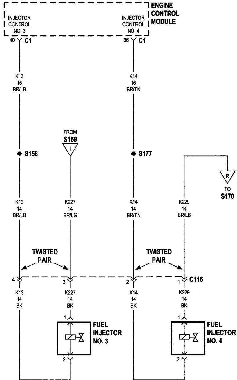
Figure C126-2 Fuel injectors, late build (sheet 2 of 3)
