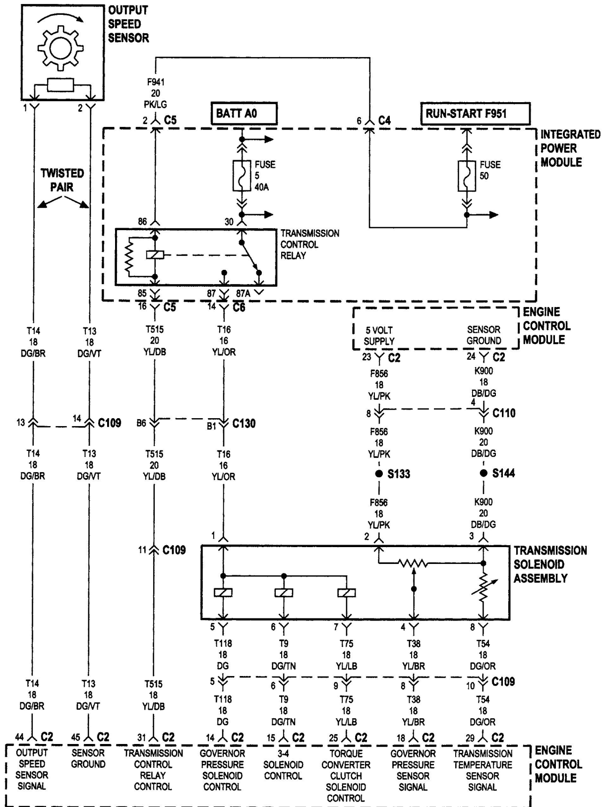
Figure C126-20 Transmission solenoid assembly
