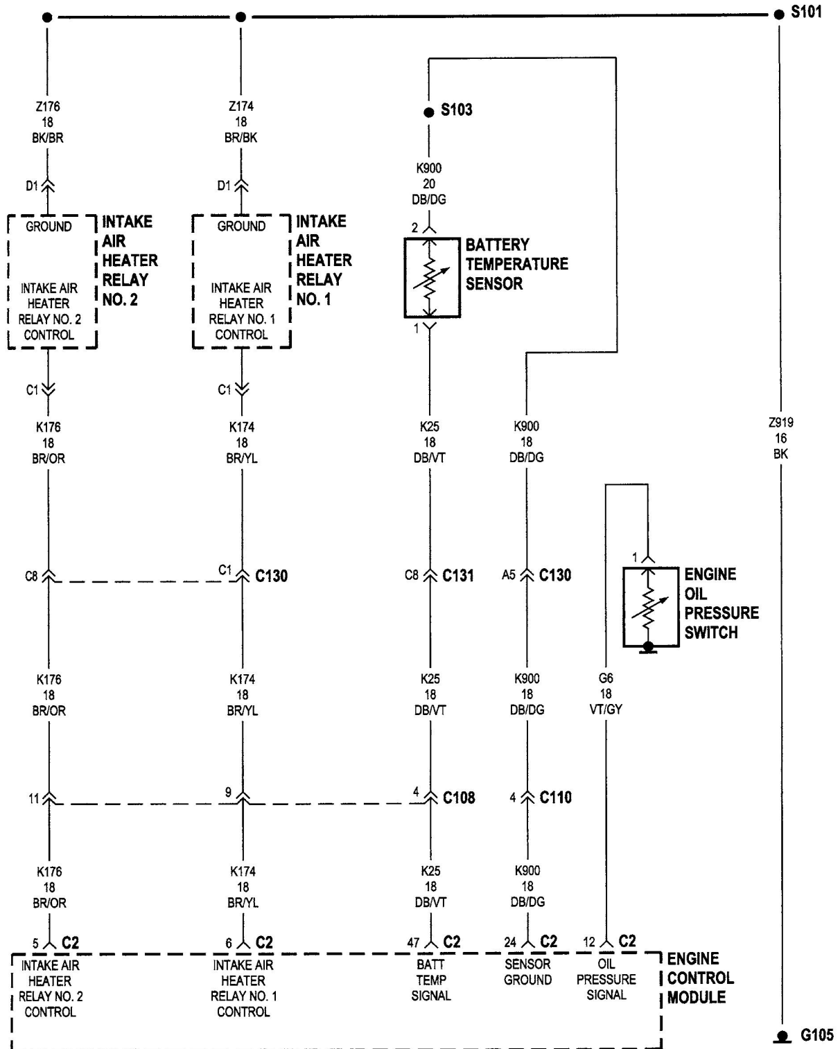
Figure C126-15 Battery temperature sensor and intake air heater relays
