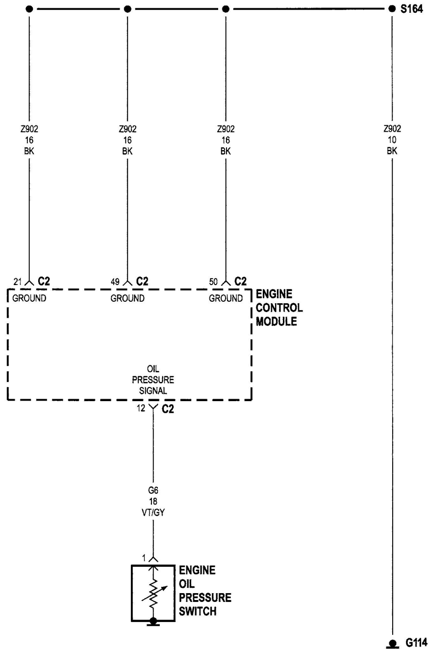
Figure C126-11 Engine oil pressure switch
