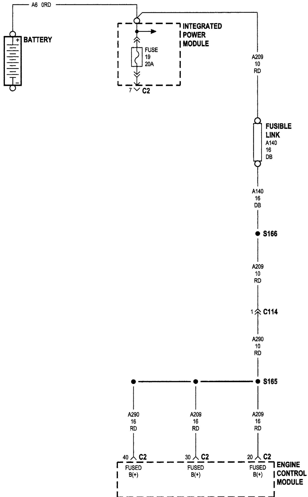
Figure C126-10 ECM power supply
