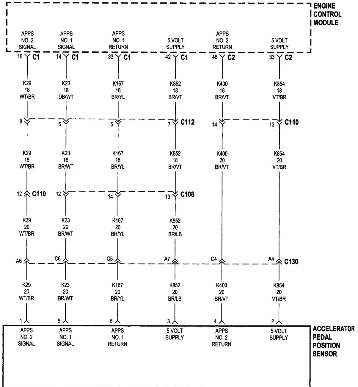
Figure C126-23 APP sensor with manual transmission
