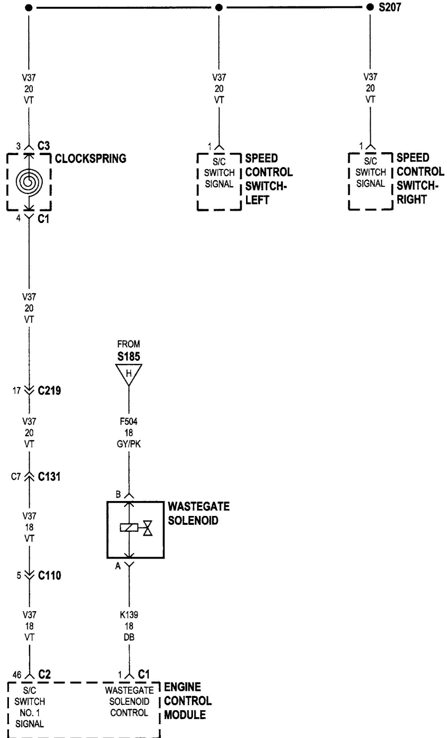
Figure C126-18 Wastegate solenoid and speed control switches
