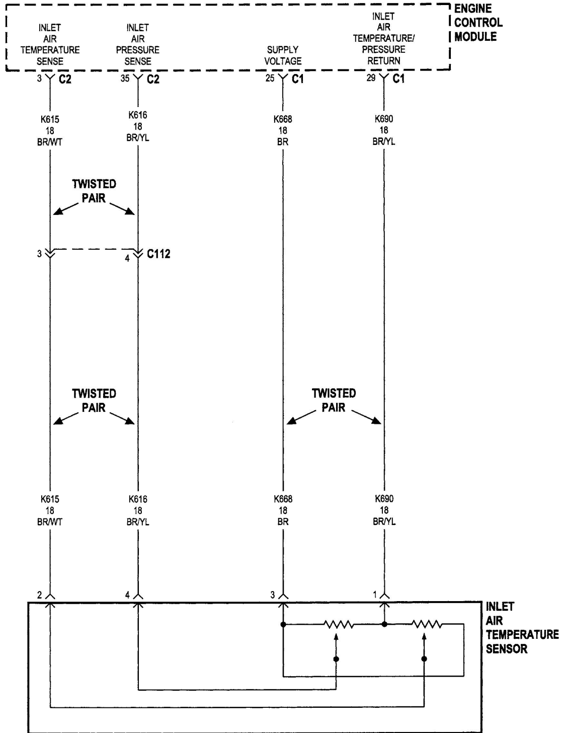
Figure C126-6 IAT sensor, early build with manual transmission
