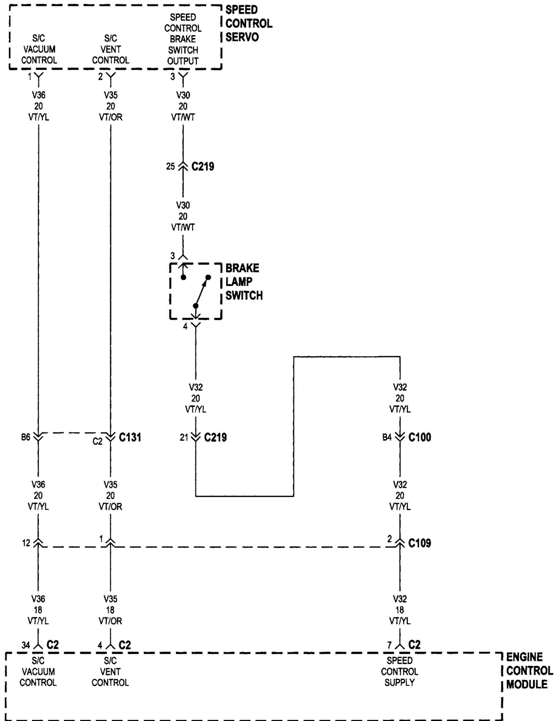
Figure C126-21 Speed control servo
