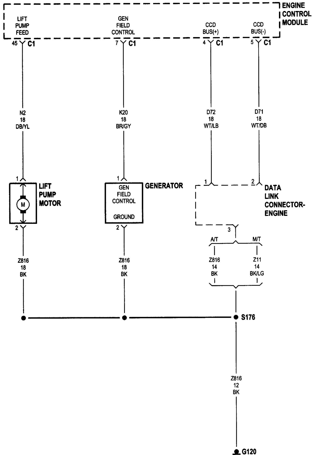
Figure C126-9 Generator and lift pump motor
