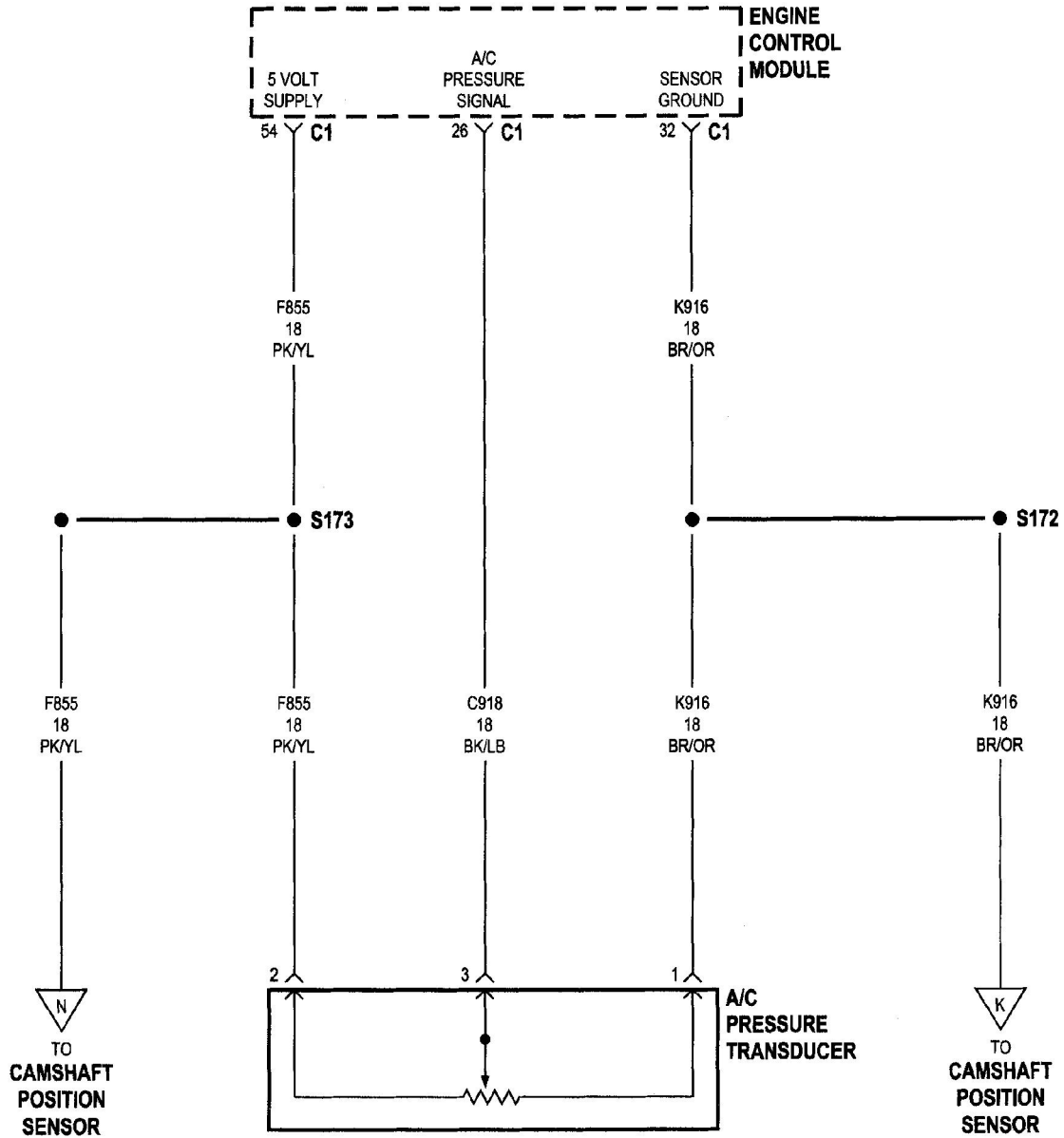
Figure C126-3 A/C pressure transducer
