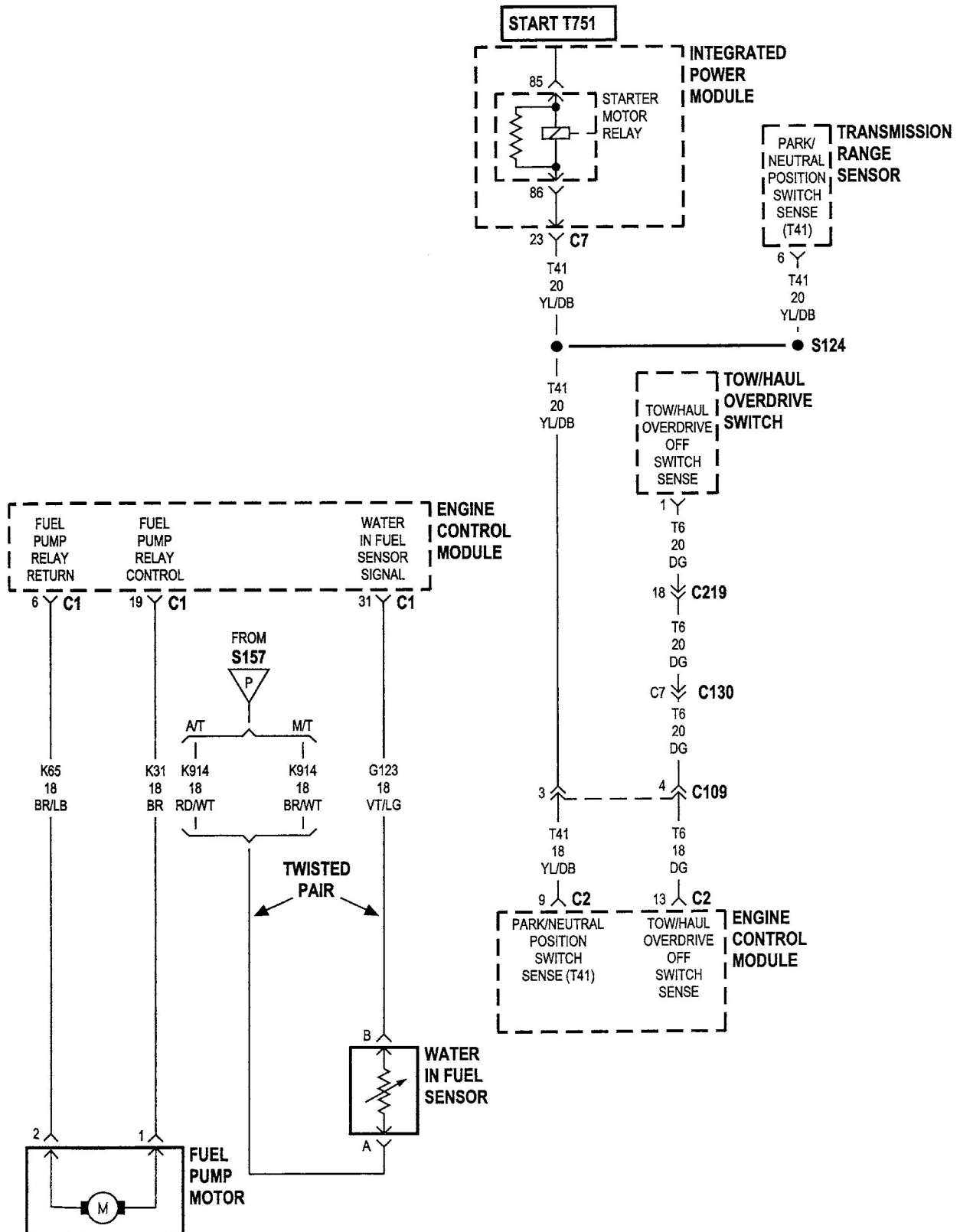
Figure C126-5 Fuel pump, water-in-fuel sensor, TR sensor, and tow/haul OD switch
