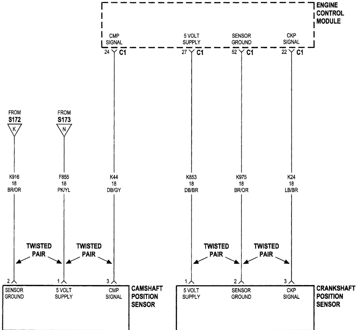
Figure C126-4 CMP sensor and CKP sensor
