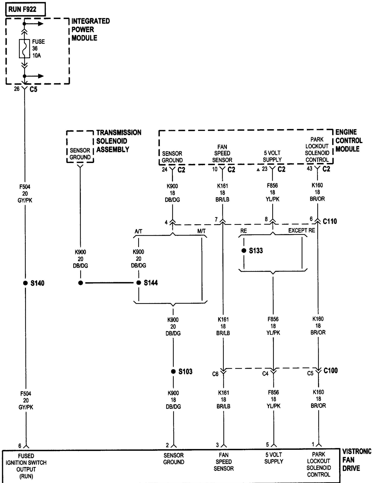
Figure C126-12 Vistronic fan drive, early build
