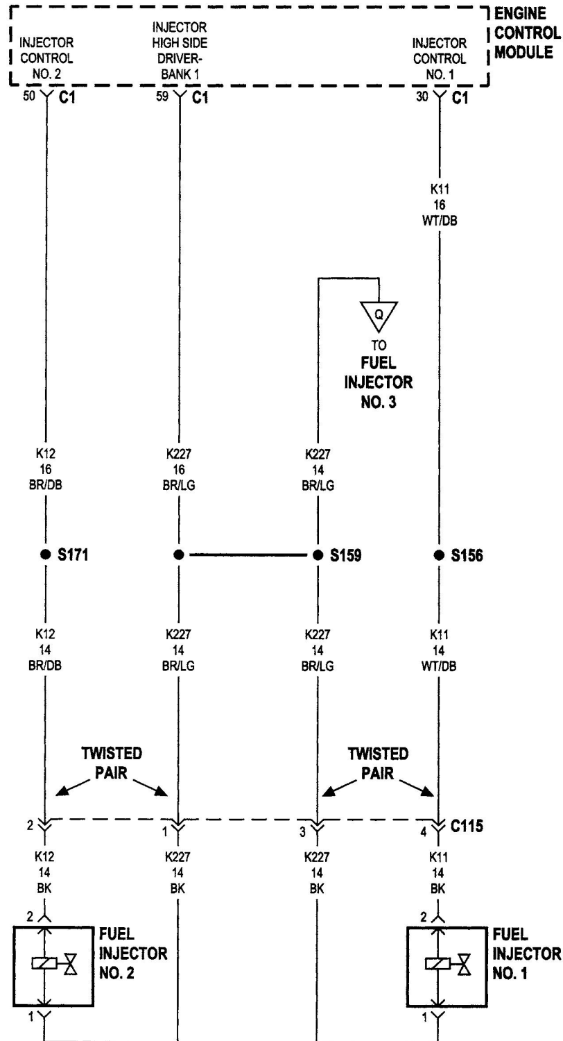
Figure C126-1 Fuel injectors, early build (sheet 1 of 3)
