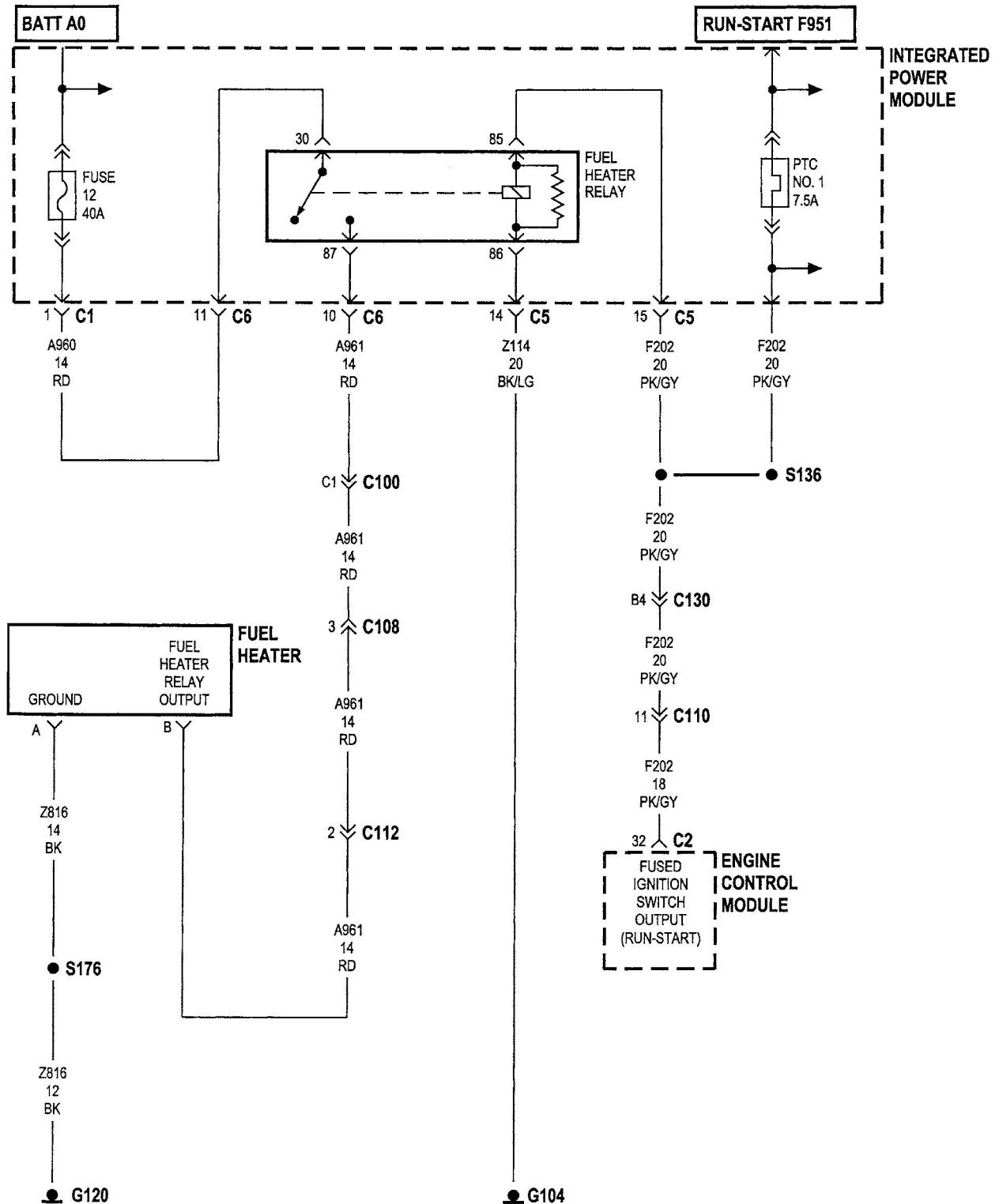
Figure C126-19 Fuel heater
