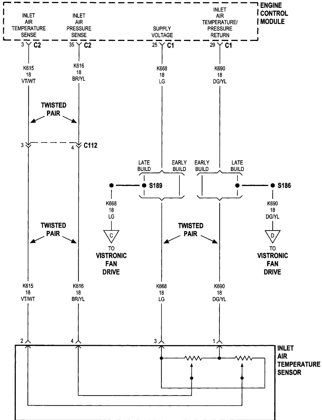
Figure C126-7 IAT sensor, except early build with manual transmission
