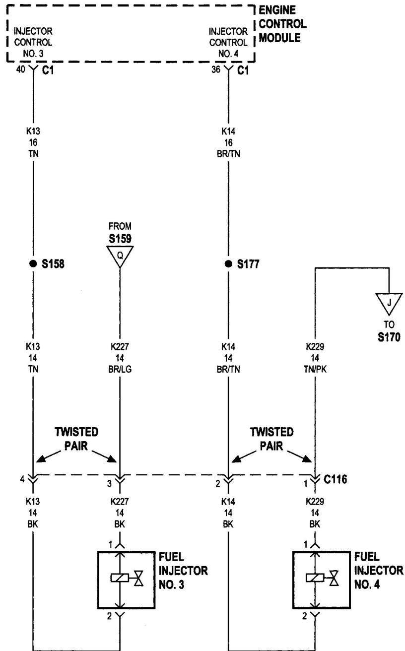
Figure C126-1 Fuel injectors, early build (sheet 2 of 3)
