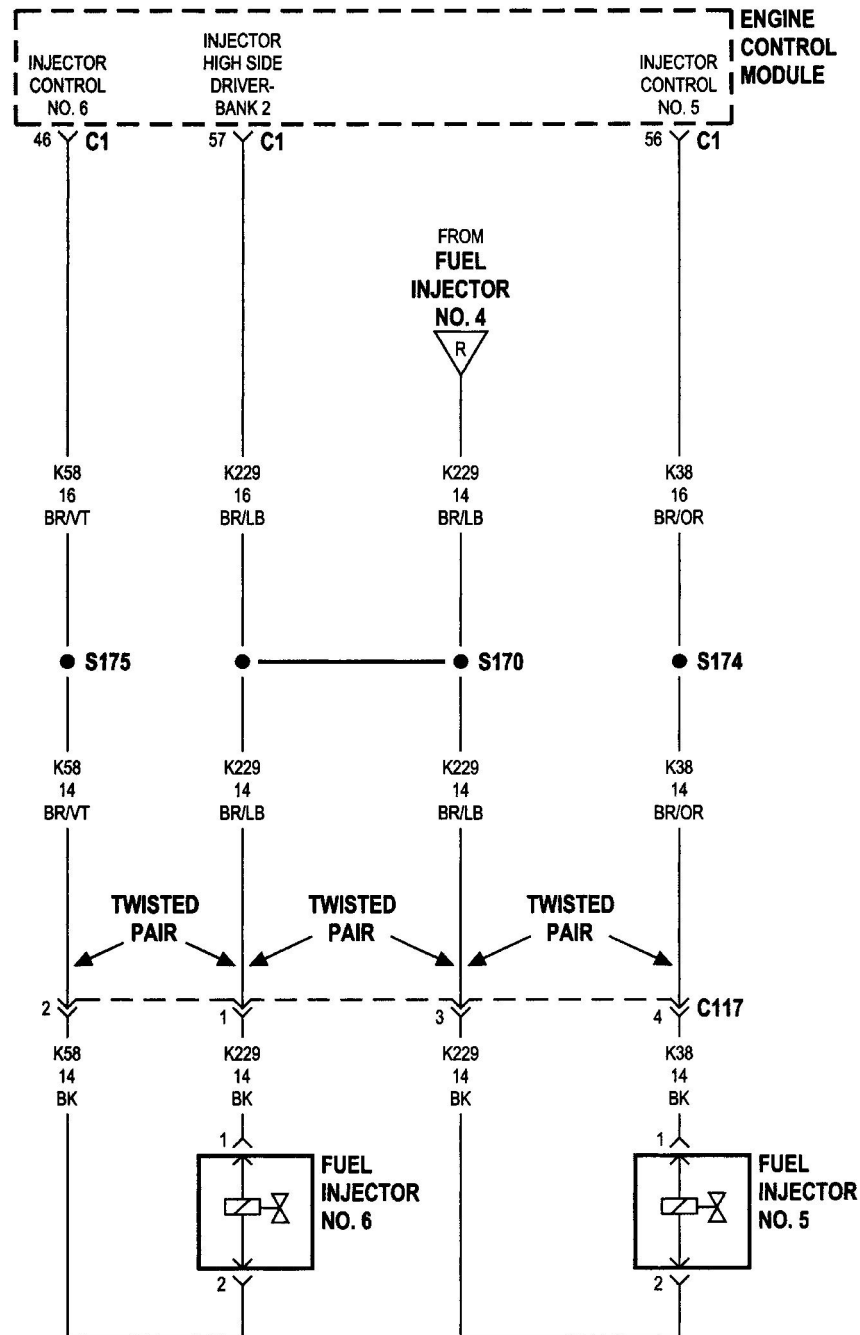
Figure C126-2 Fuel injectors, late build (sheet 3 of 3)
