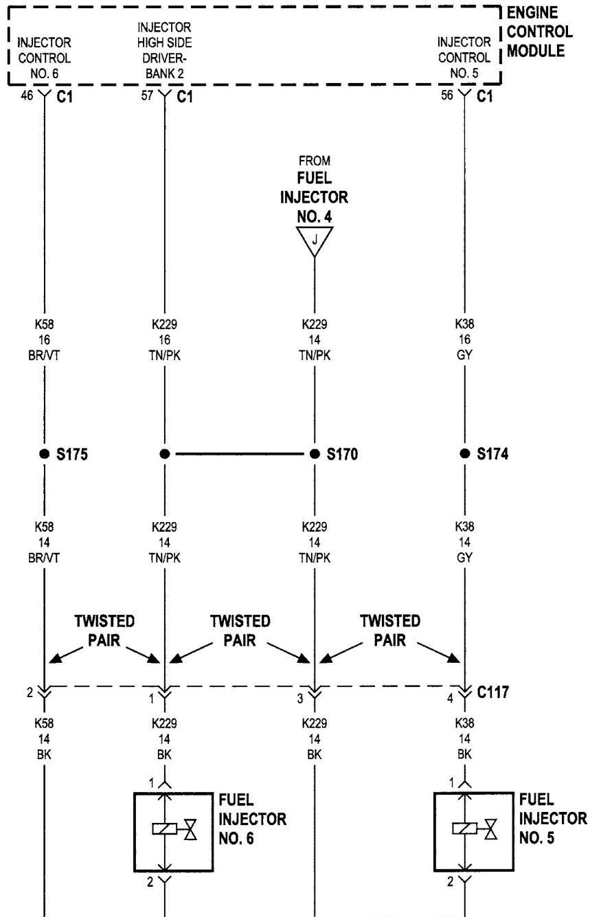
Figure C126-1 Fuel injectors, early build (sheet 3 of 3)
