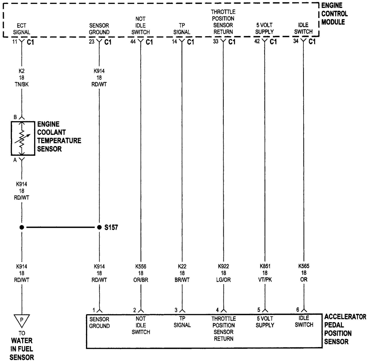
Figure C126-22 APP sensor with automatic transmission
