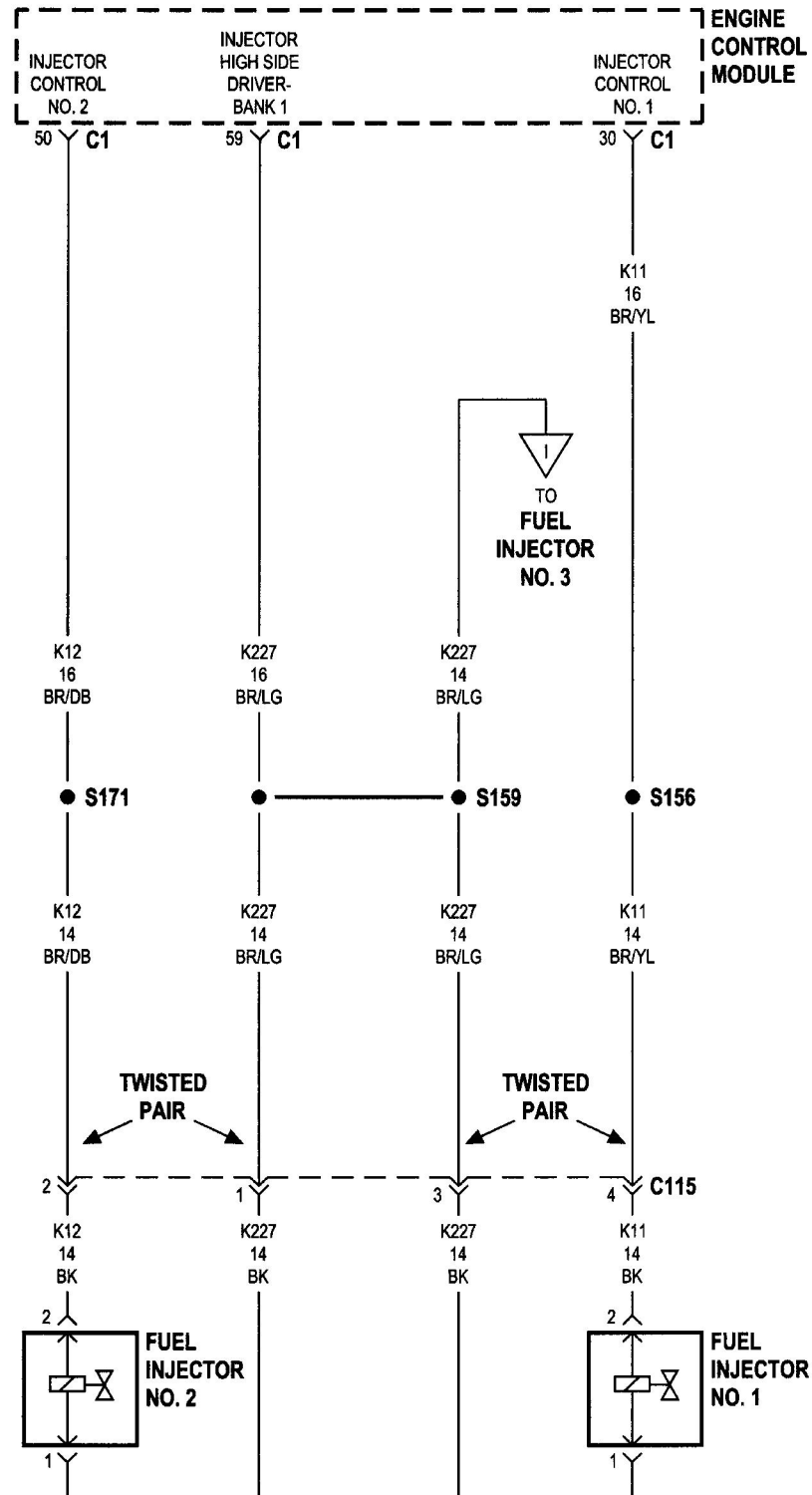
Figure C126-2 Fuel injectors, late build (sheet 1 of 3)
