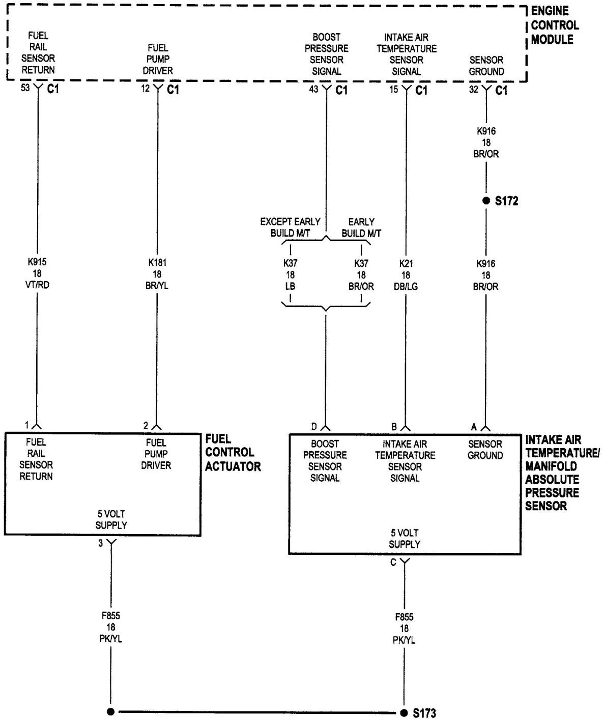
Figure C126-8 Fuel control actuator and IAT/MAP sensor
