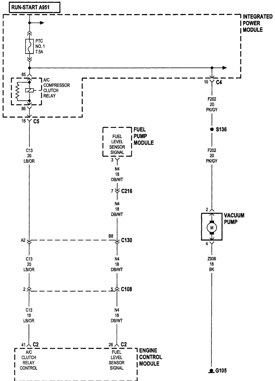
Figure C126-17 Fuel pump module and vacuum pump
