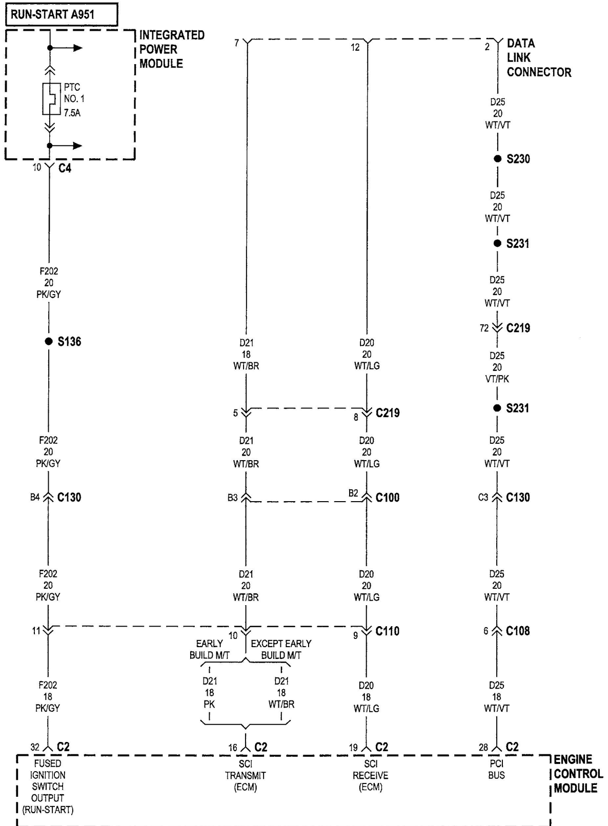
Figure C126-14 PCI bus and SCI bus
