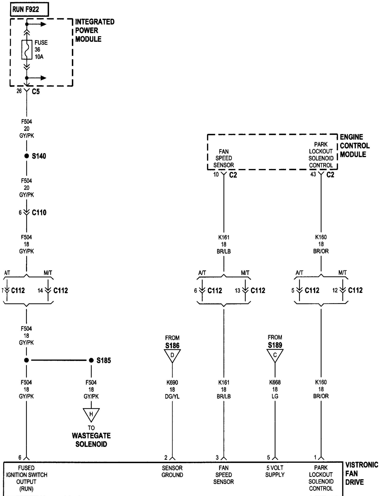
Figure C126-13 Vistronic fan drive, late build
