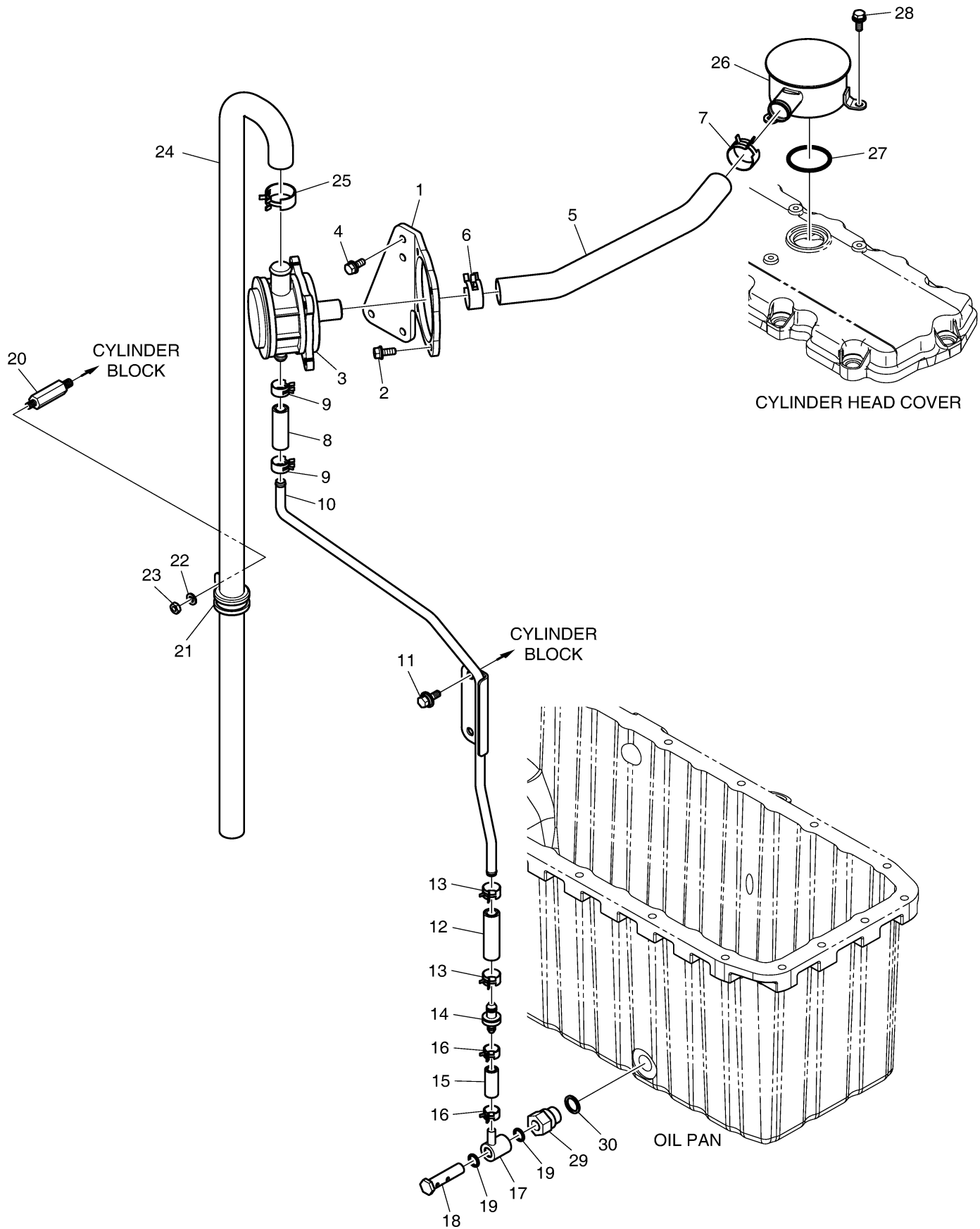
Fig. 006 BREATHER SYSTEM
