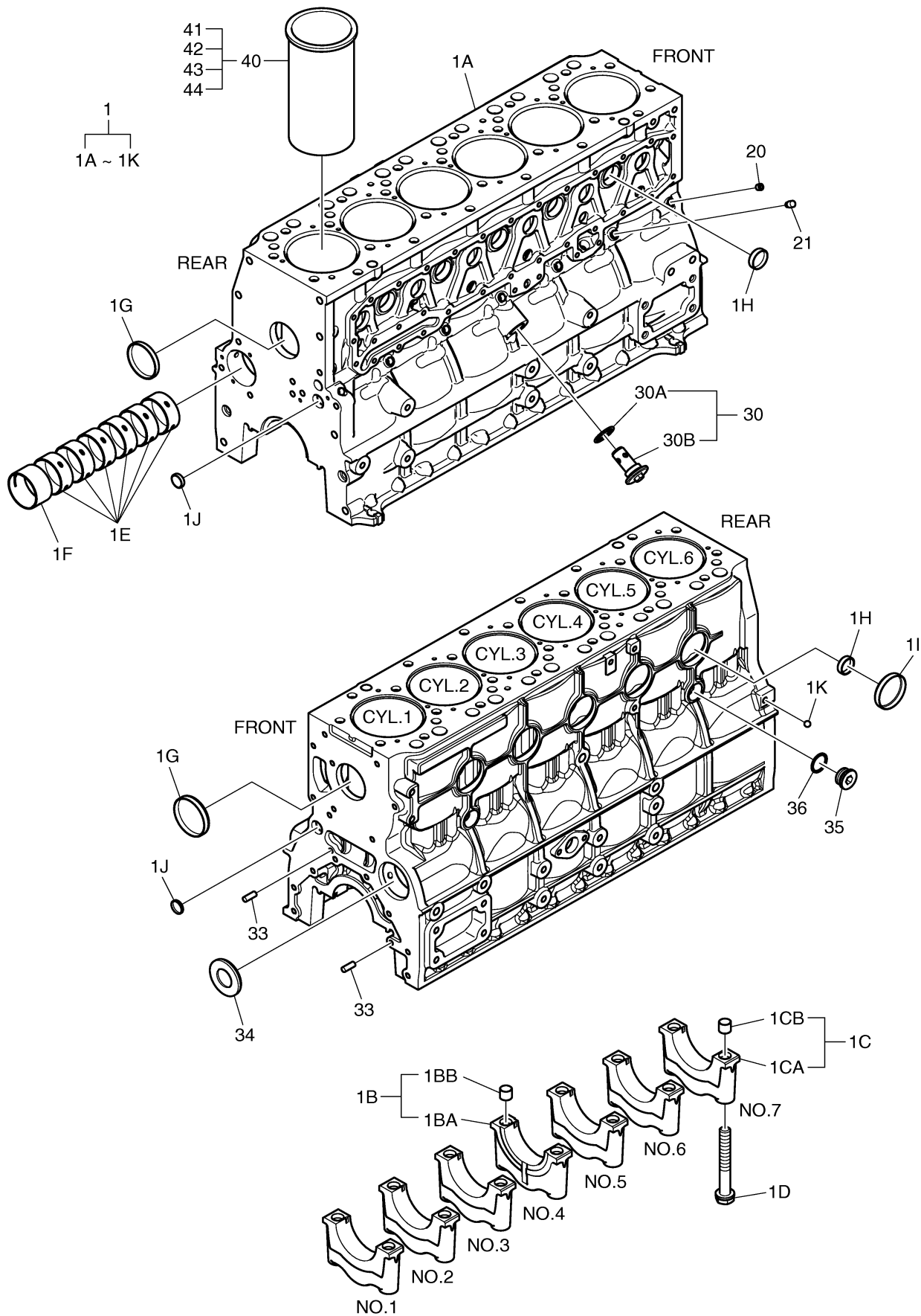
Fig. 001 CYLINDER BLOCK
