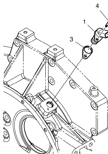
THERMOSTAT HOUSING
