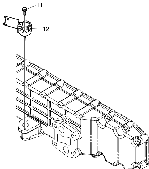
OIL COOLER HOUSING
