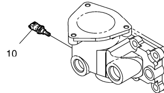
THERMOSTAT HOUSING
