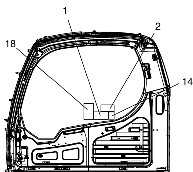
RIGHT SIDE VIEW OF CABIN INSIDE
