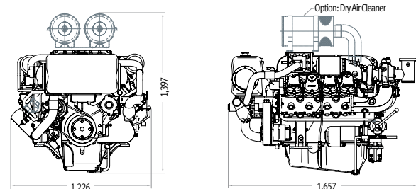
Engine Dimension
