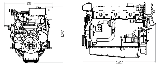
Engine Dimension
