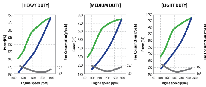
Performance Curve
