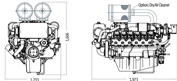
Engine Dimension
