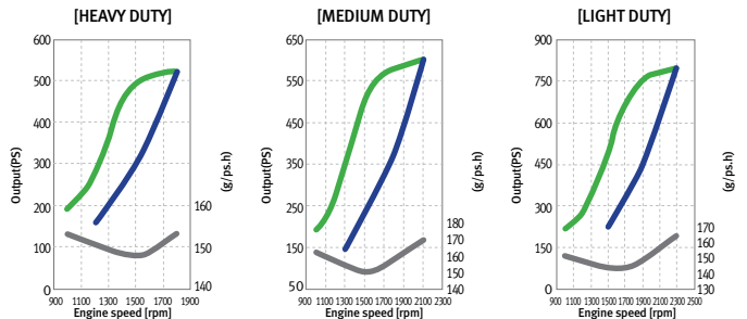
Performance Curve
