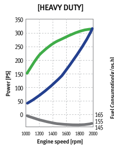
Performance Curve
