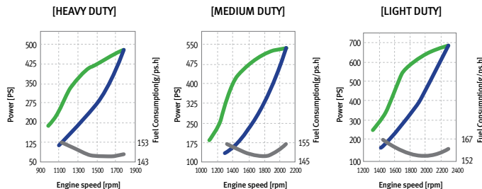
Performance Curve
