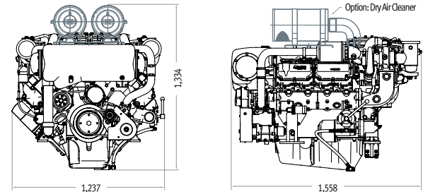
Engine Dimension
