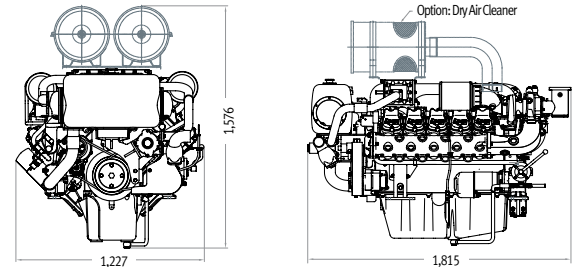
Engine Dimension
