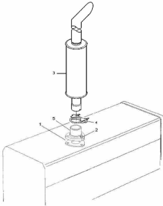
MUFFLER VERTICAL
