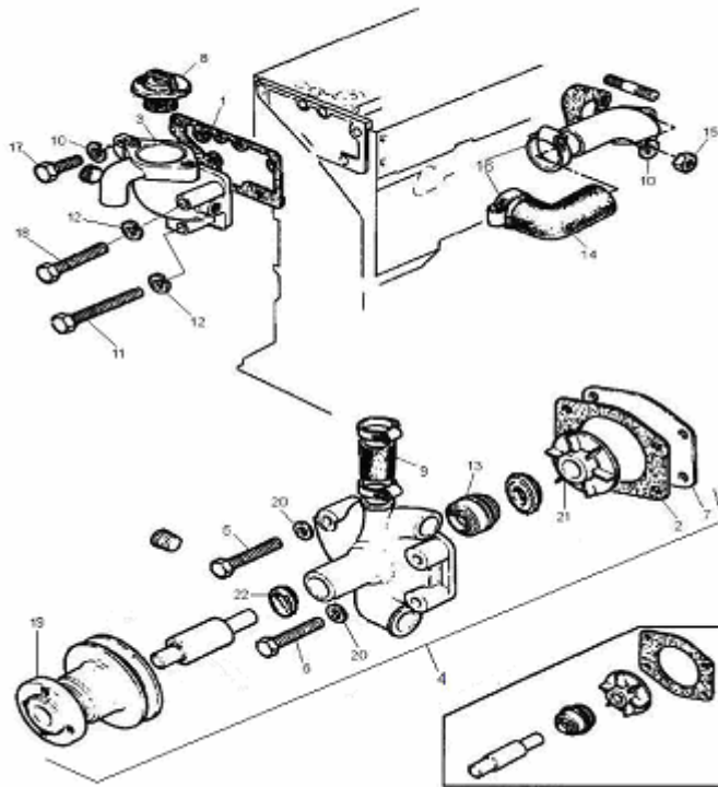
WATER PUMP THERMOSTATE & HEAT EXCHANGER
