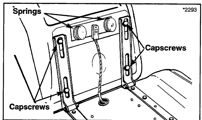
Figure 22 Seat Adjustment
