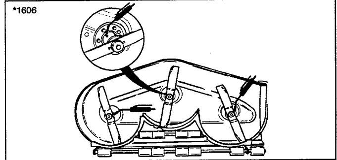
Figure 12. Mower Arbor
