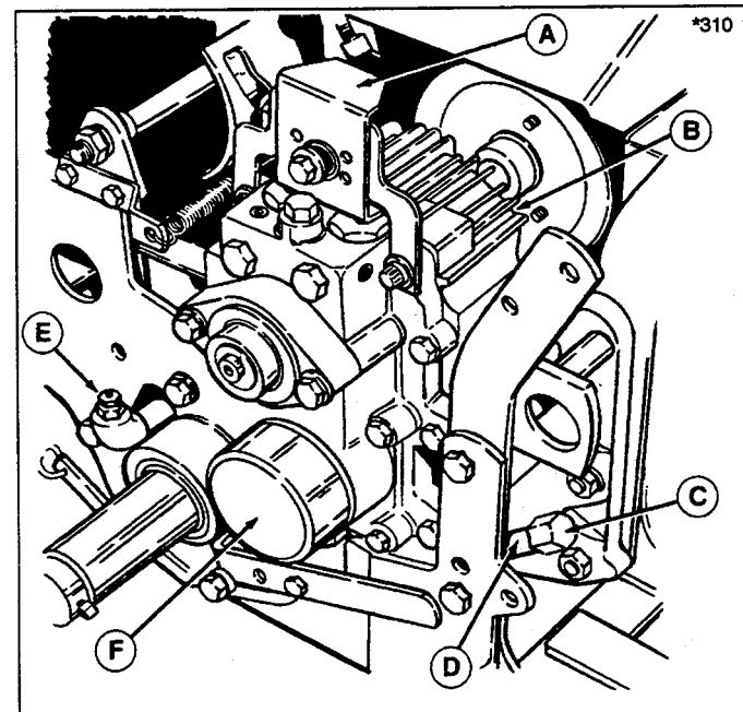
Figure 14. Hydrostatic Transmission
