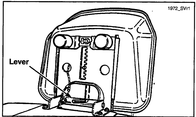
Figure 21 Seat Adjustment
