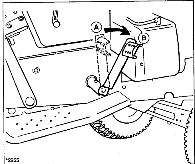
Figure 6. Clutch/Brake Pedal
