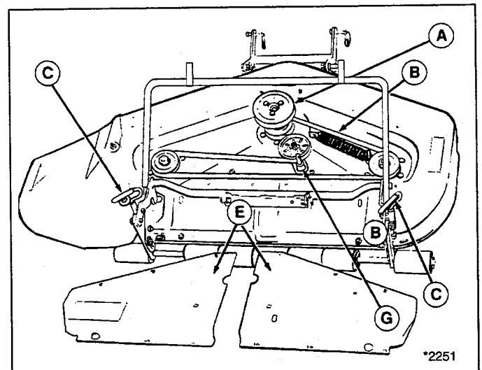
Figure 28. Mower Belt
