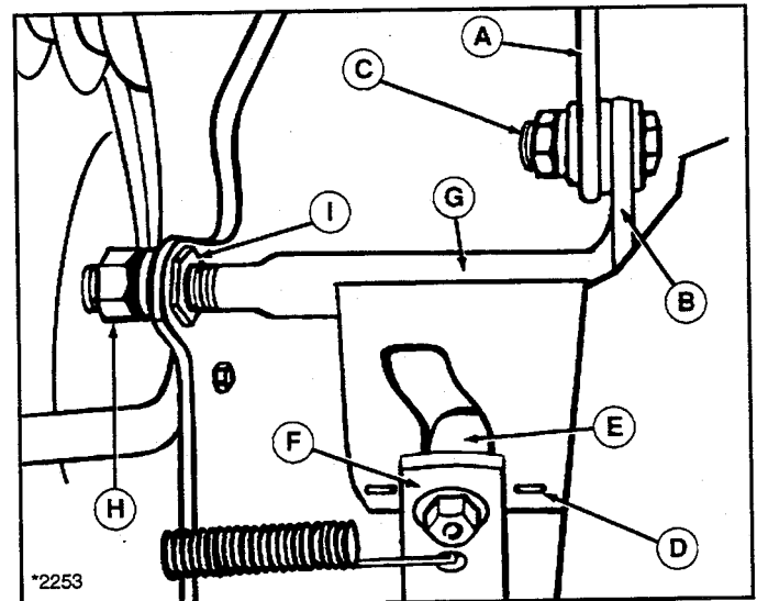
Figure 25. Neutral Adjustment
