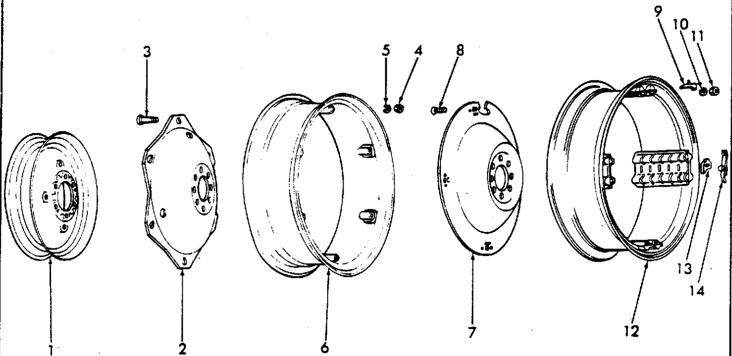
Fig. 1 Wheels &amp; Weights
