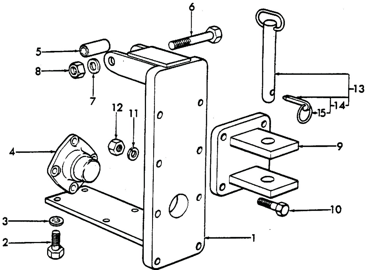
Fig. 57 Drawbar Bracket &amp; Towing Hitch Assy.
