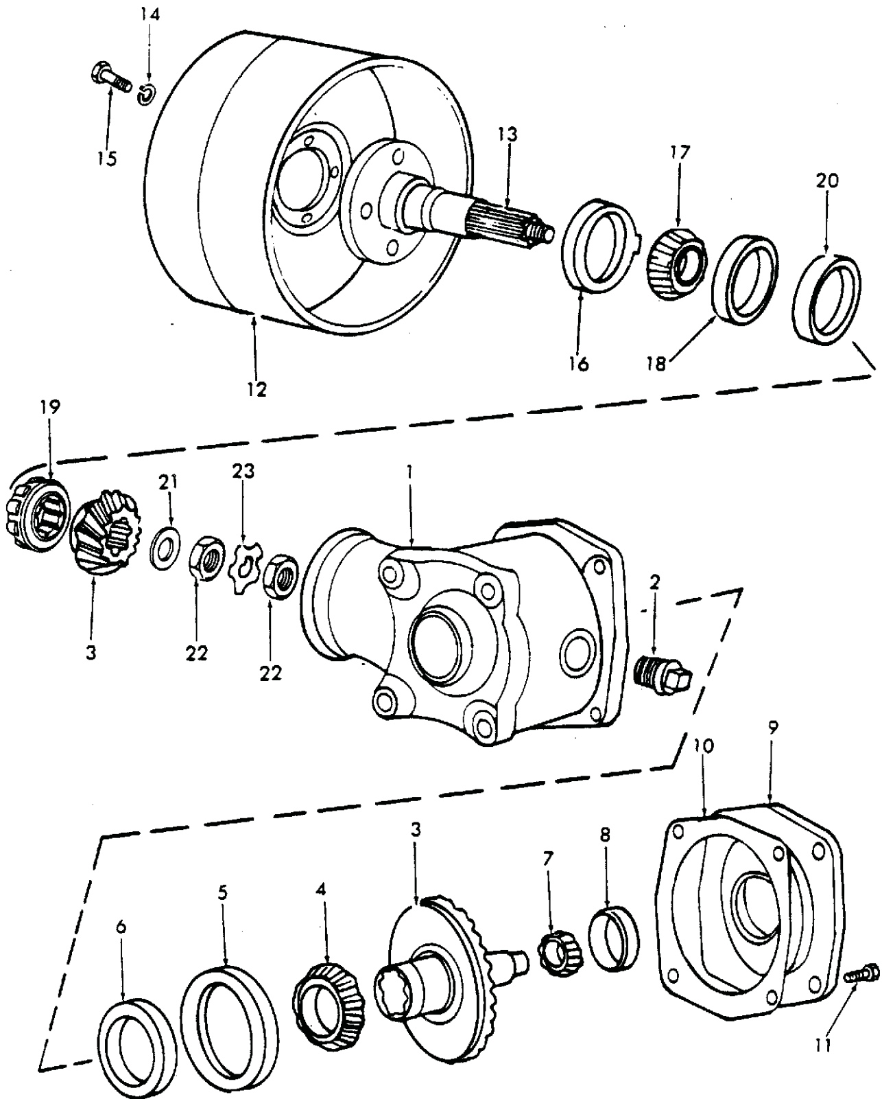
Fig. 33 Pulley Assy.
