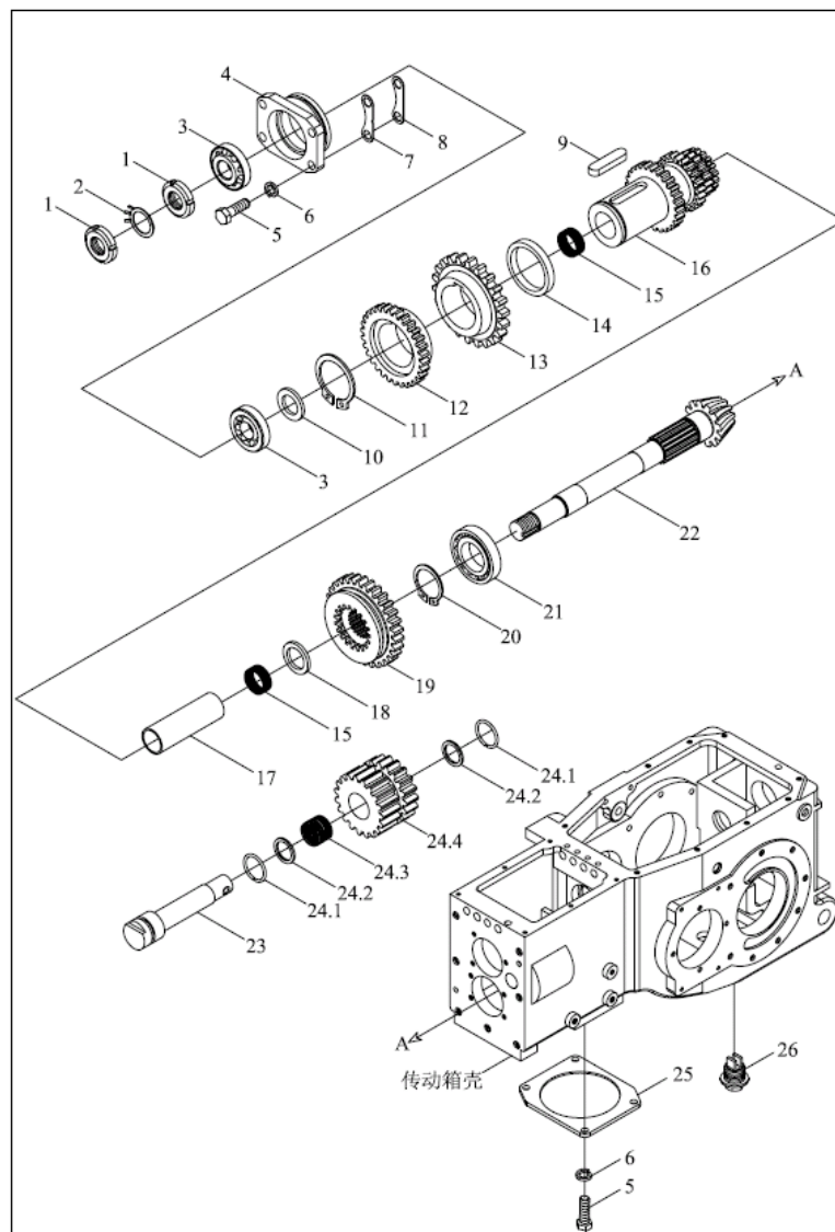
TE250.371E 传动箱总成-2
