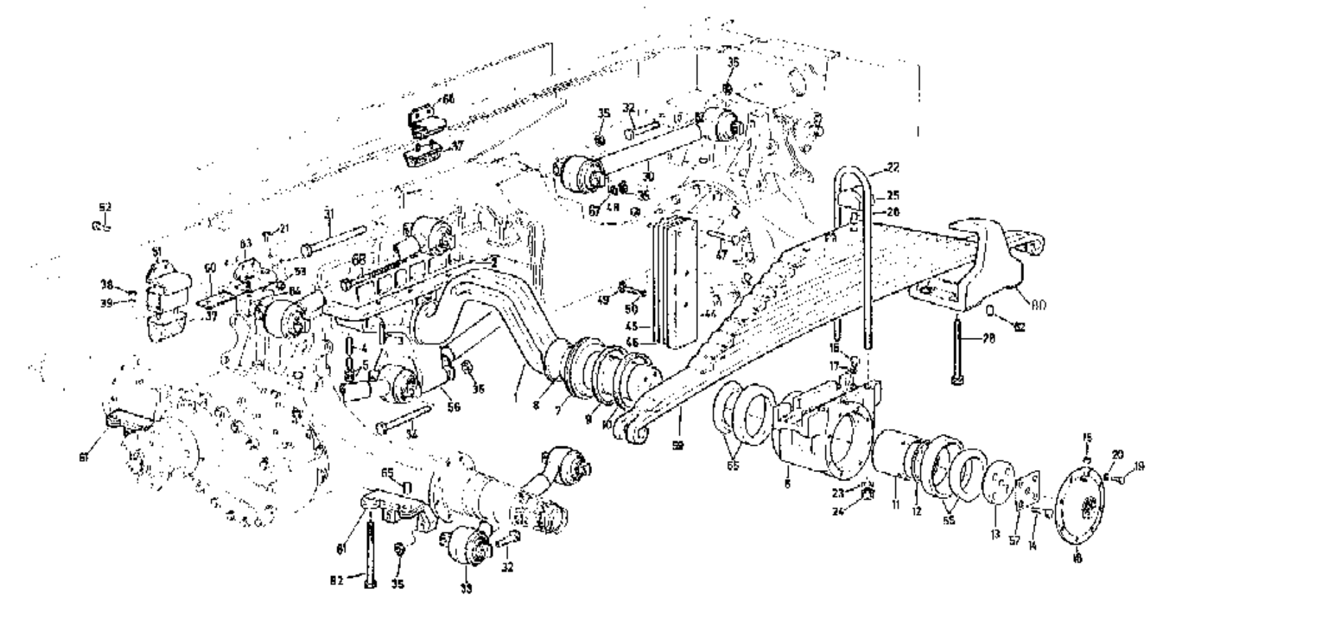
C8-4 6×4, 8×4 SWIVEL SPRING AND SUSPENSION/6×4, 8×4平衡悬架
