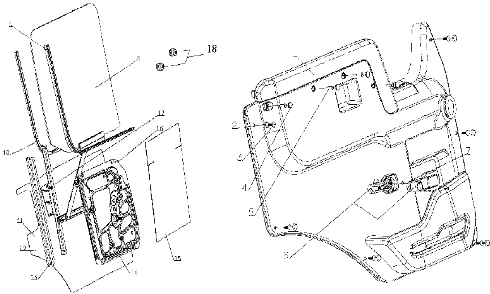
DOOR, GLASS AND FITTINGS/车门，玻璃及附件
