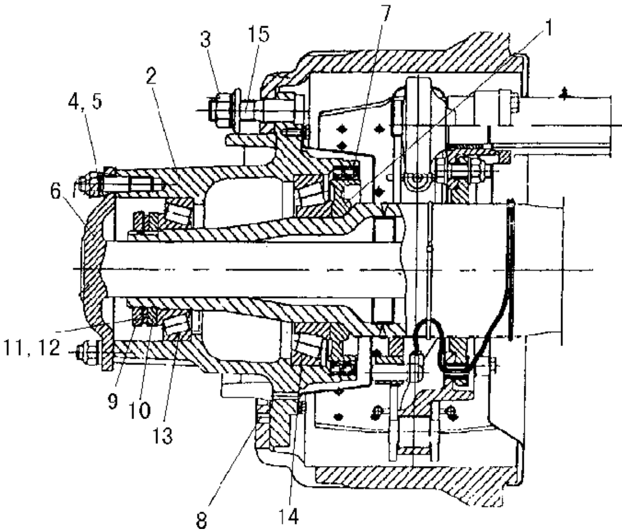
WHEEL HUB OF TRAILING AXLE/支承轴轮毂
