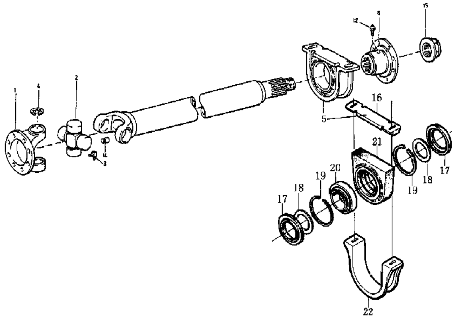
INTERMEDIATE SHAFTS/中间传动轴
