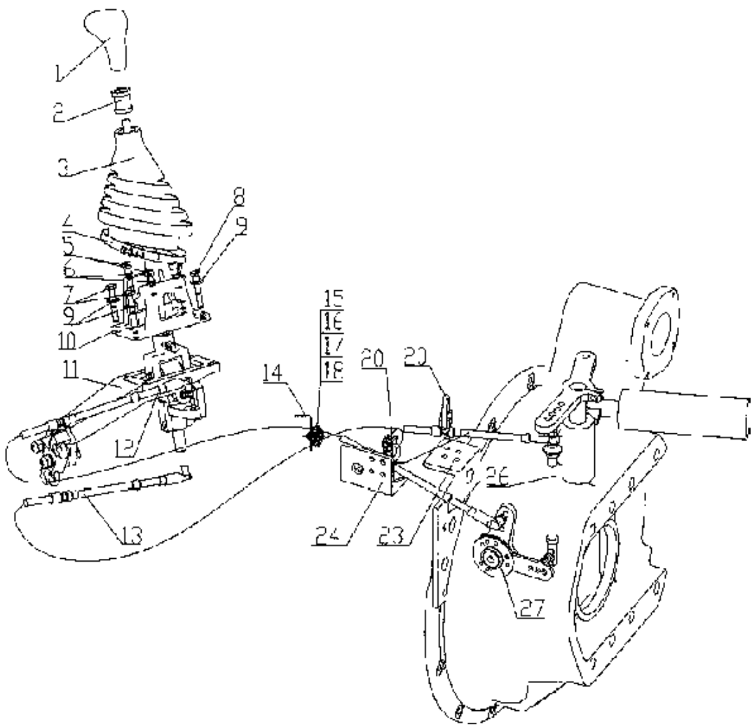
C3-1 GEARBOX GEAR CHANGE SYSTEM/变速器换档操纵装置 Fig. C3-1
