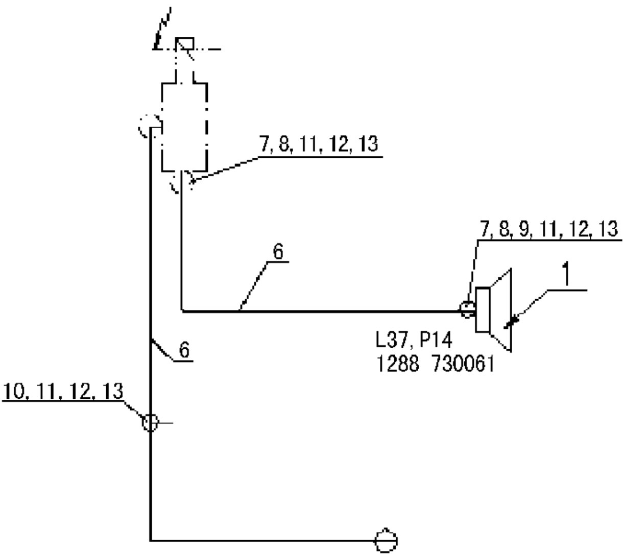
DOUBLE VOICE PENUMATIC HORN/双音气喇叭操纵管路
