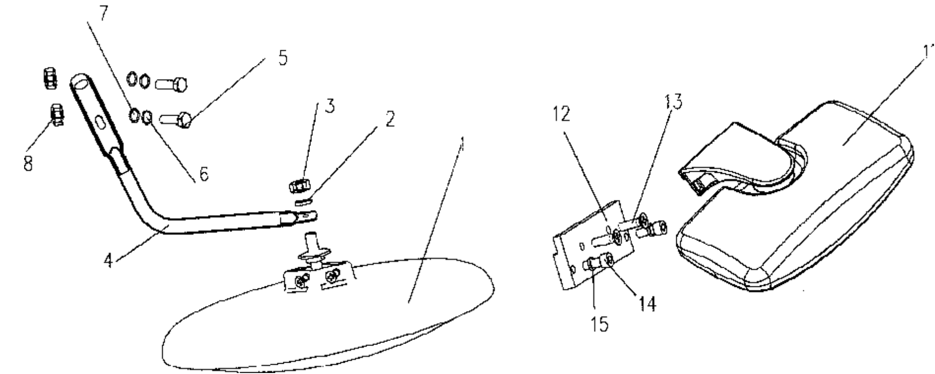
C12-25 DOWN VIEW MIRROR, SIDE MIRROR/下视镜，路面镜 Fig. C12-28
