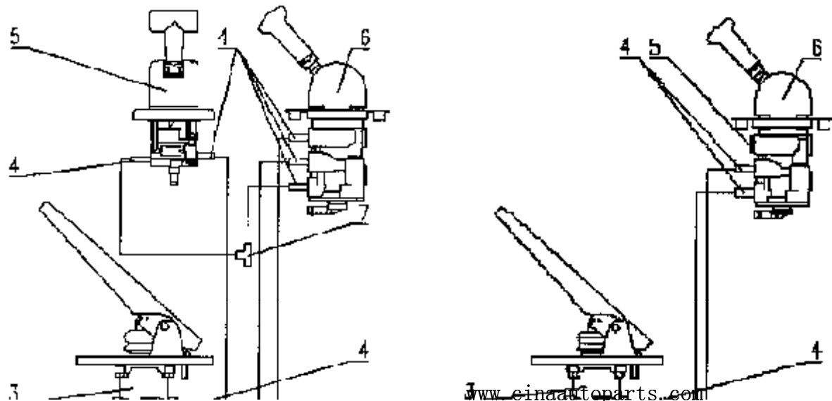
C10-1 BRAKE MECHANISM IN CAB/驾驶室制动操纵机构 Fig.C10-1
