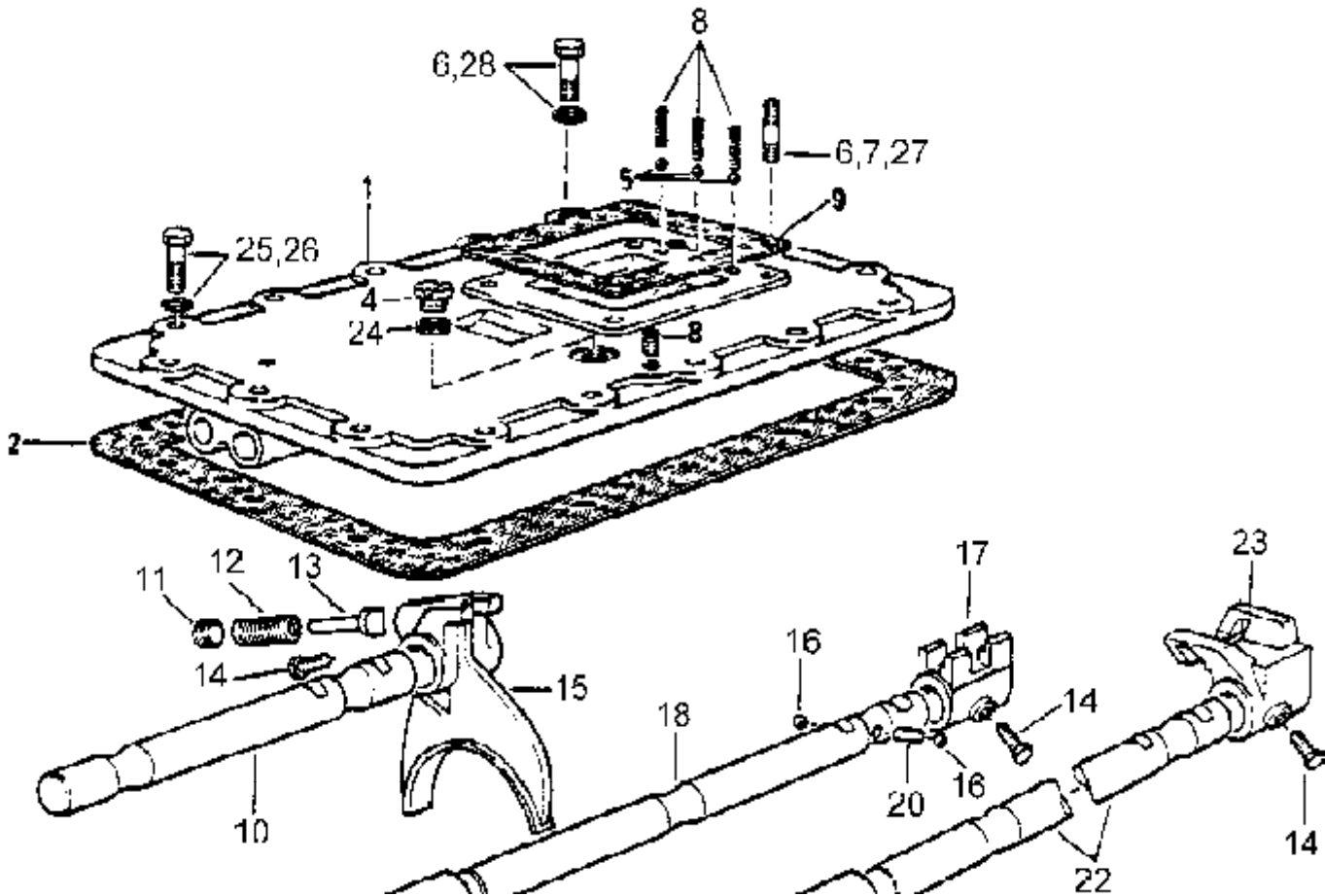
C4-6 9JS150T SWITCH GEAR/换档机构 Fig. C4-6
