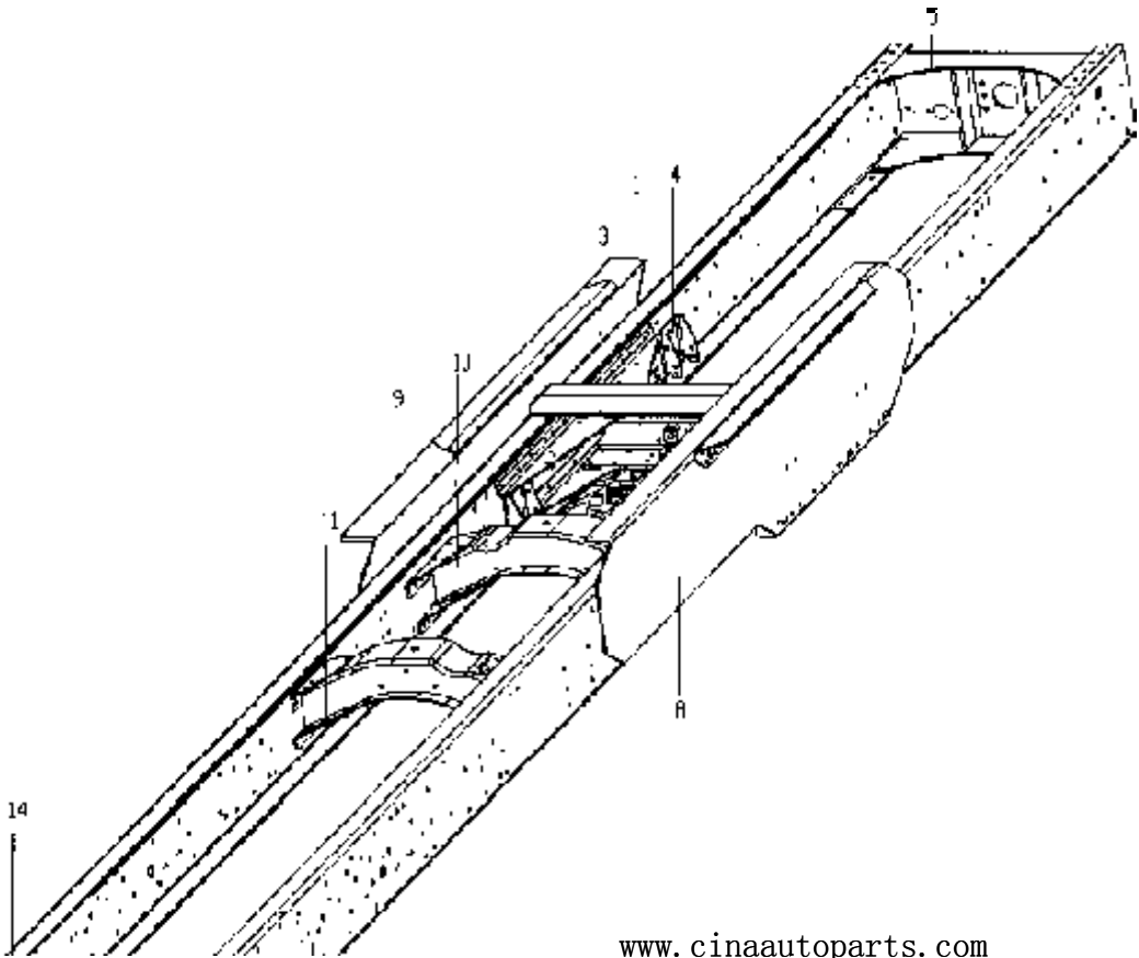
C7-5 CHASSIS FRAME FOR 6×4 TRACTOR TRUCK/6×4牵引车车架 Fig. C7-5
