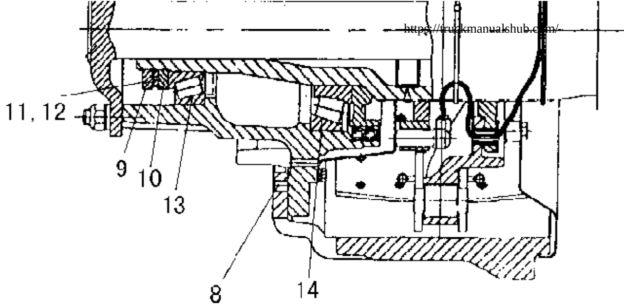
C13-4 WHEEL HUB OF TRAILING AXLE/支承轴轮毂
