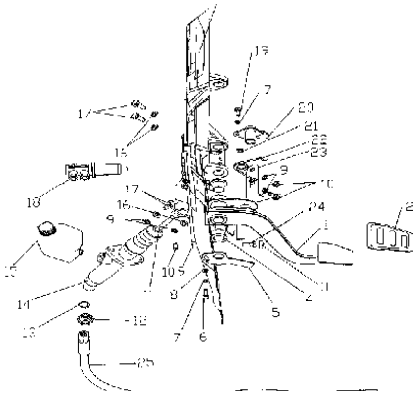
Combination pedal bracket 组合踏板支架
