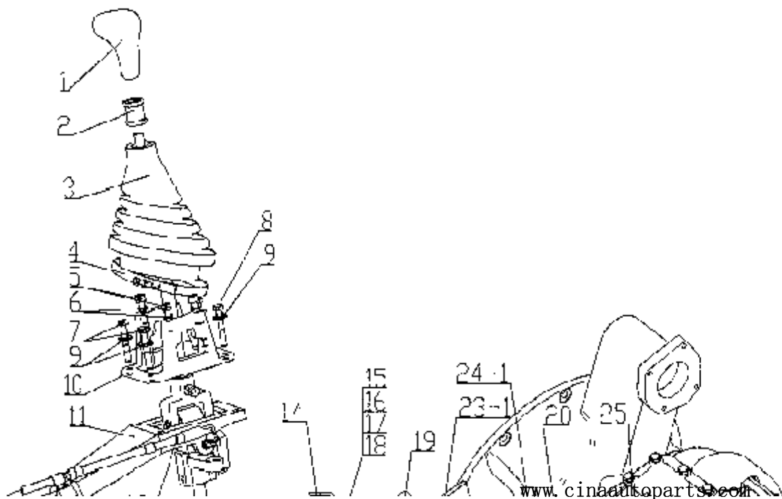
C3-1 GEARBOX GEAR CHANGE SYSTEM/变速器换档操纵装置
