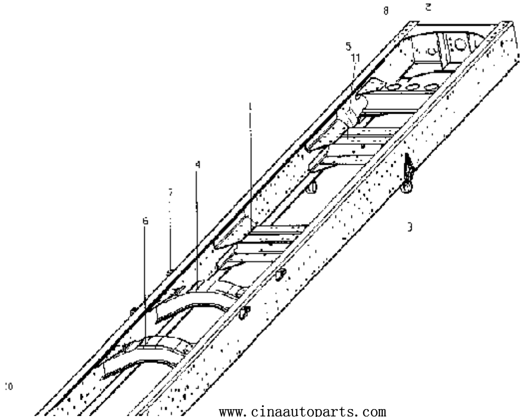
C7-3 CHASSIS FRAME FOR 4×2 CARGO TRUCK/4×2载货车车架 Fig.C7-3
