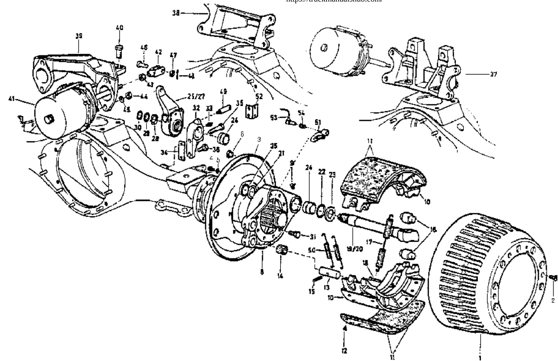
C13-5 BRAKE OF TRAILING AXLE/支承轴制动器
