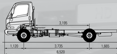
Standard Cab Long Wheelbase
