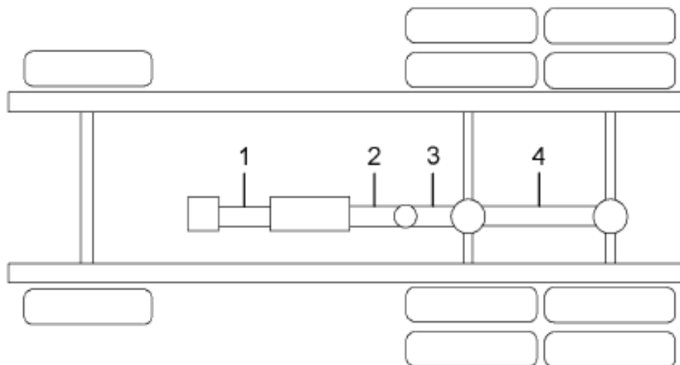
6X4, W/AUXILIARY TRANSMISSION AND ONE CENTER BEARING
