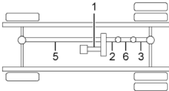
4X4, SEPERATE TRANSFER CASE AND TWO CENTER BEARINGS
