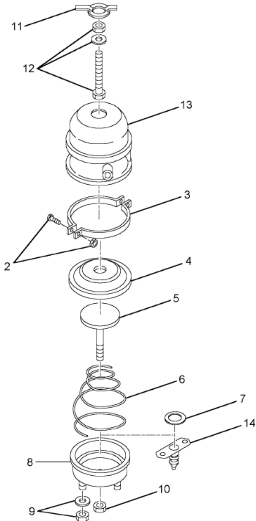
https://truckmanualshub.com/ Figure 1688941C91 CHAMBER, BRAKE
