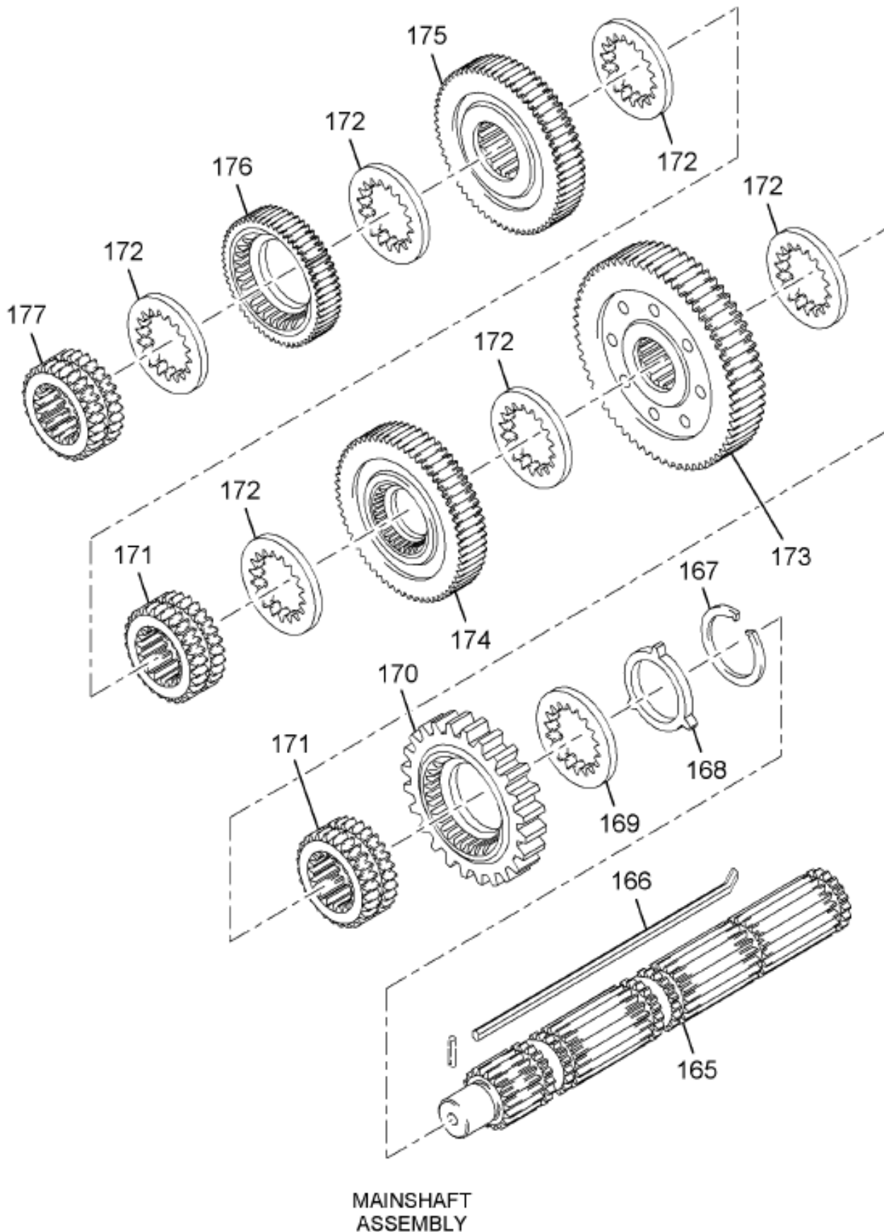
https://ruclmanualshub.com/ Figure 3505487C91 TRANSMISSION, W/HSG 13GHS
