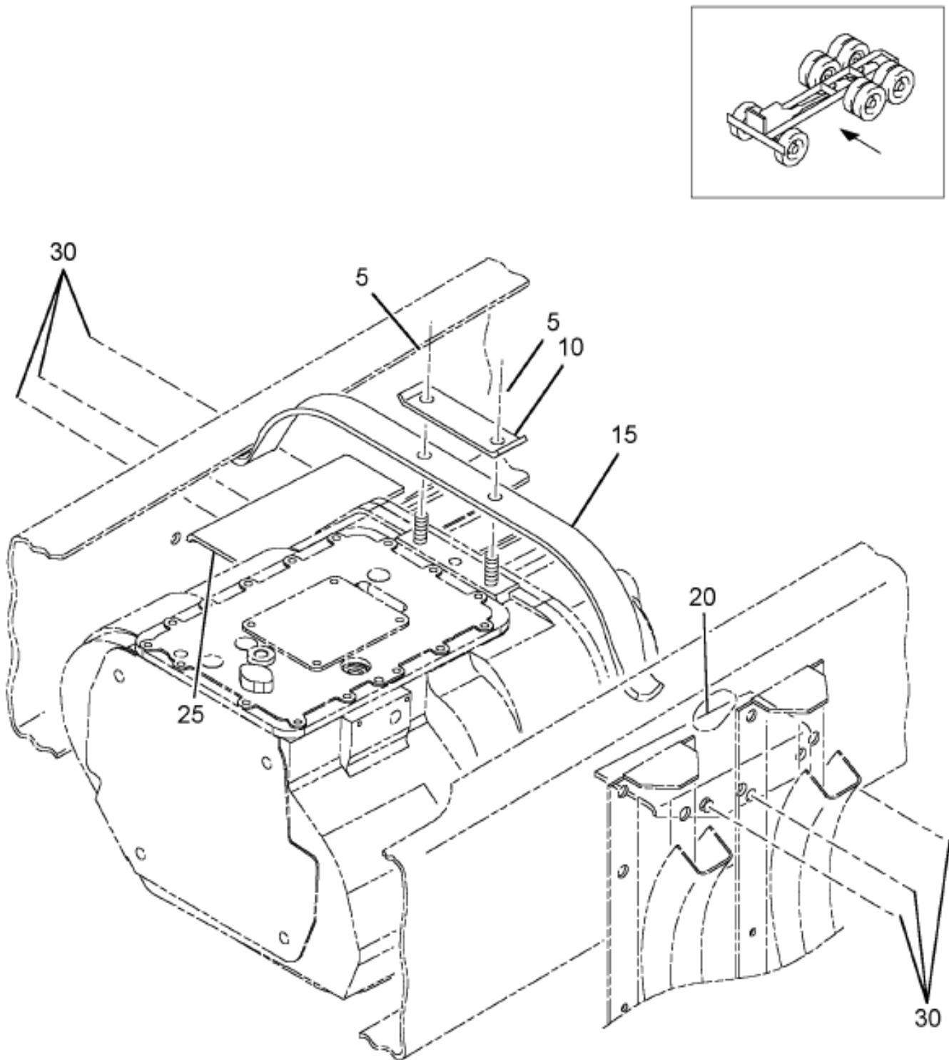
https://truckmanualshub.com/ Figure 0GW09 TRANSMISSION MTG, REAR
