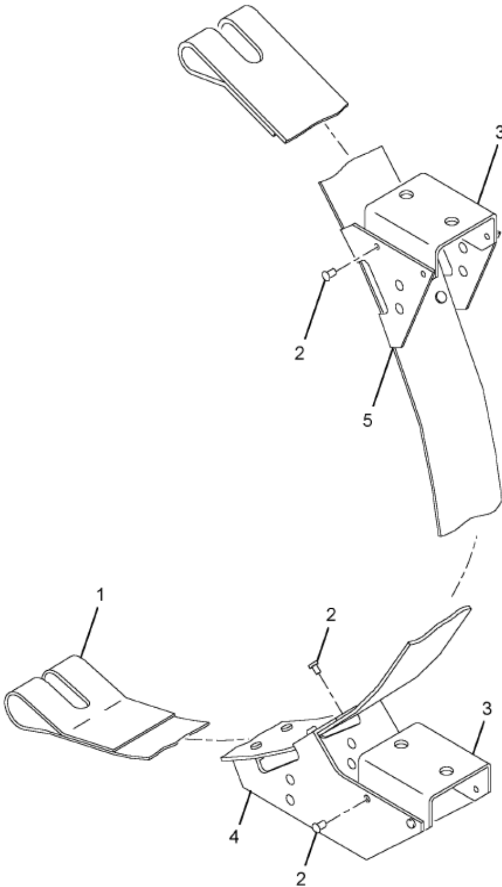
https://truckmanualshub.com/ Figure 3566480C1 STRAP, FUEL TANK MTG*
