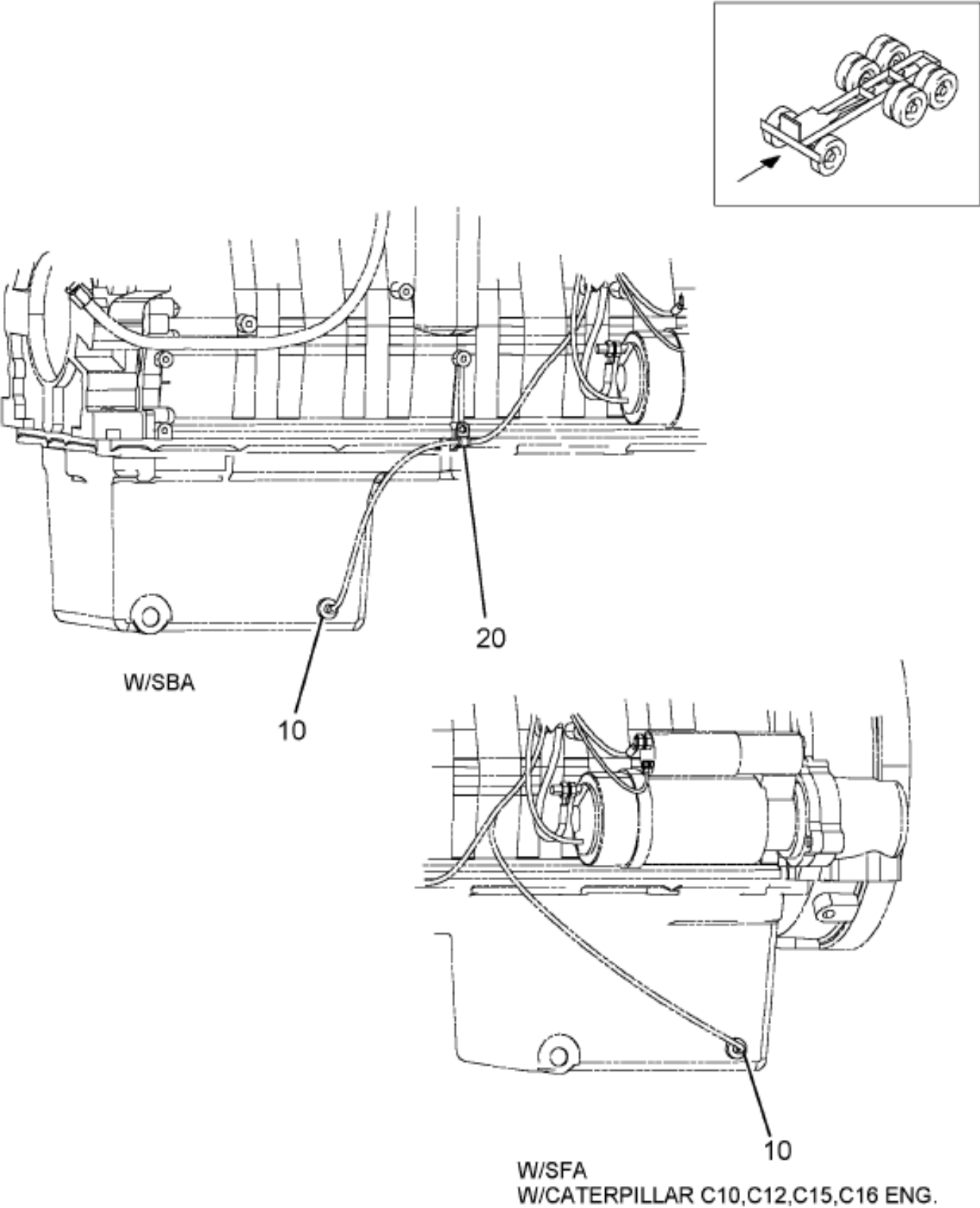
https://trackmanualshub.com/ Figure 0GXPB ENGINE OIL TEMP GAUGE WIRING
