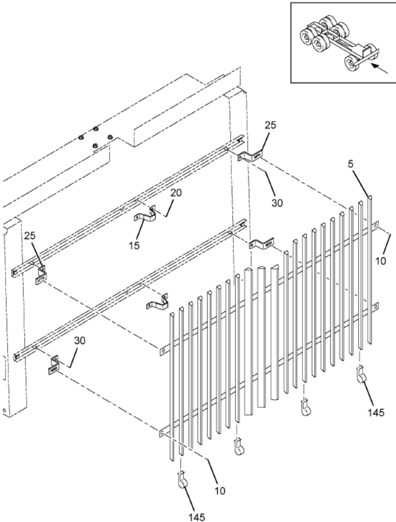
https://truckmanualshub.com/ Figure 086KT GRILLE INSTL; FRONT
