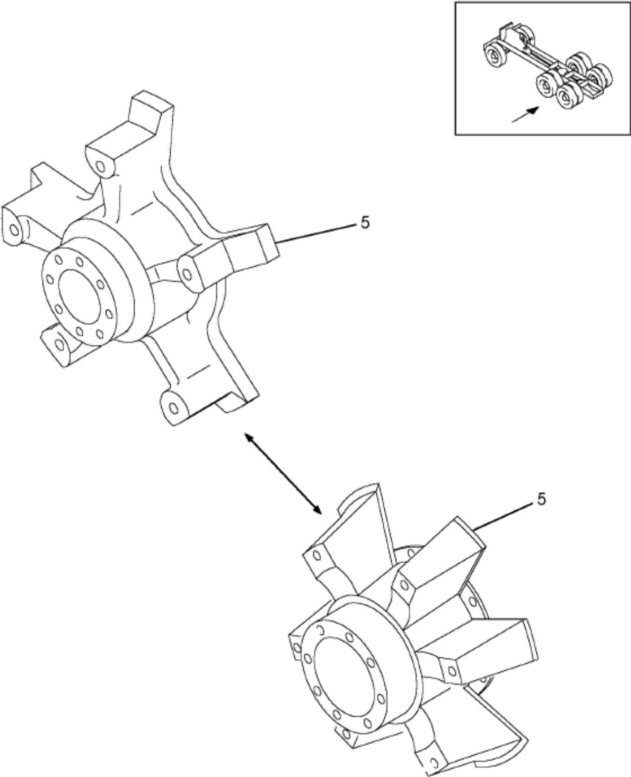
Figure 00QSR WHEEL ASM, REAR CAST
