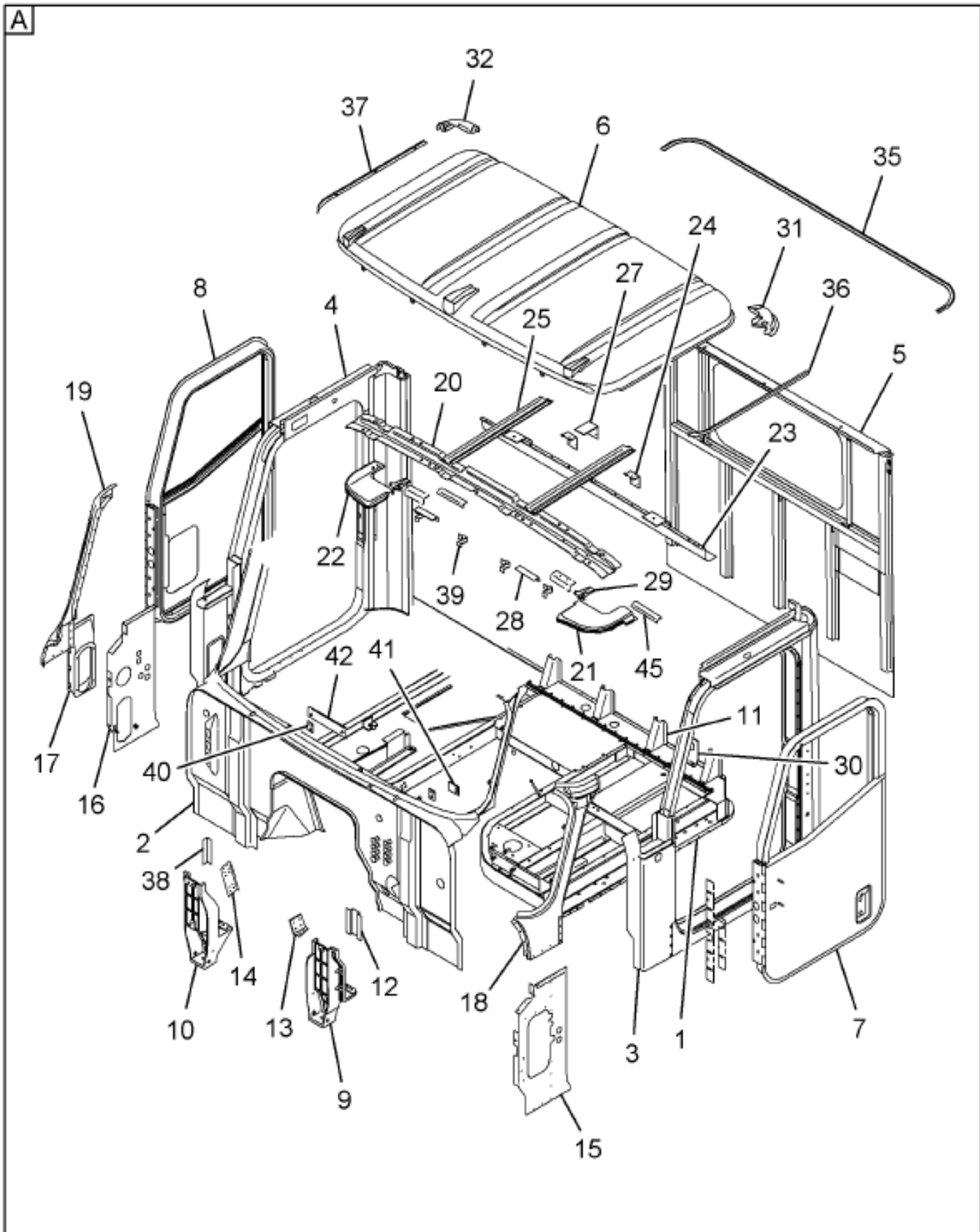
https://truckmanualshub.com/ Figure 3570699C94 CAB, REGULAR PARTIAL UNFINISHED
