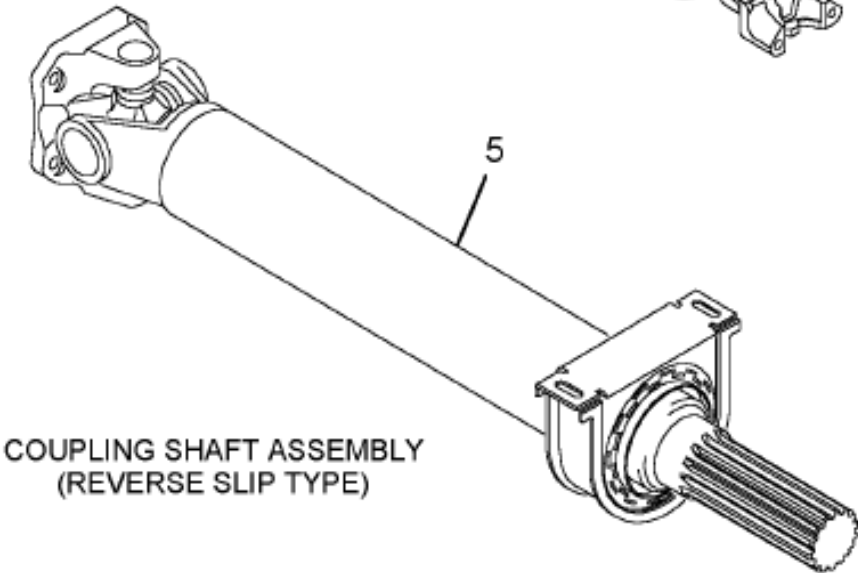
COUPLING SHAFT ASSEMBLY (FIXED END YOKE)
