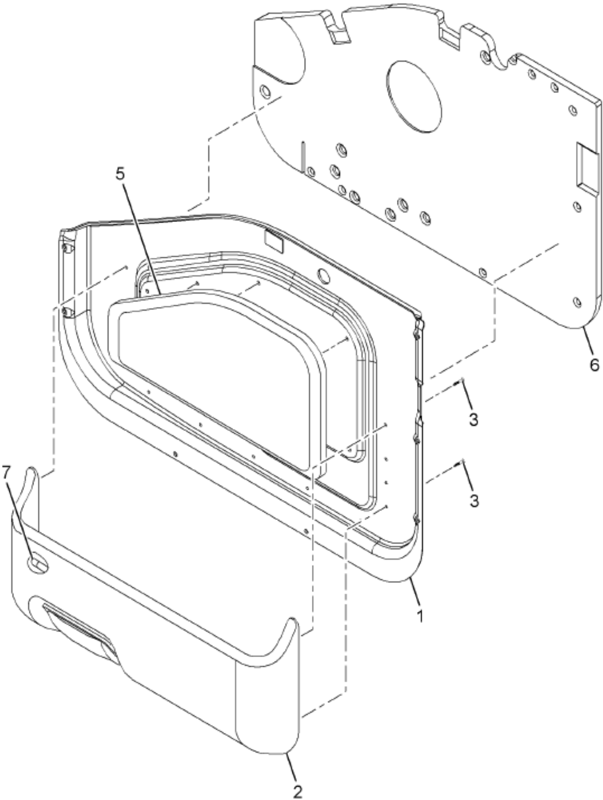
https://truckmanualshub.com/ Figure 3575492C92 PANEL,DR TRM LWR LH TAN E/WNDW
