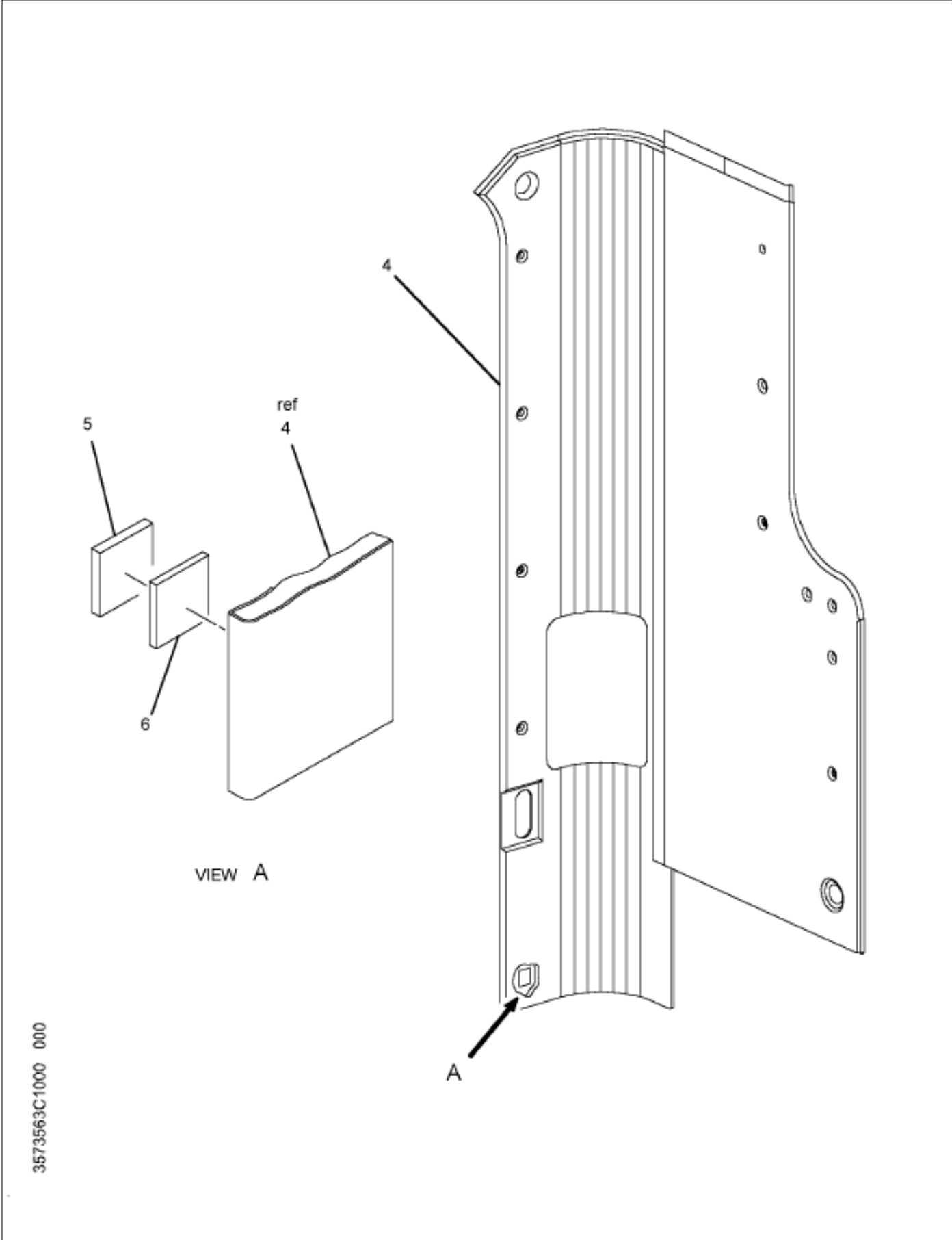
https://truckmanualshub.com/ Figure 3573563C1 PANEL, TRM RR CRNR RH MED TAN
