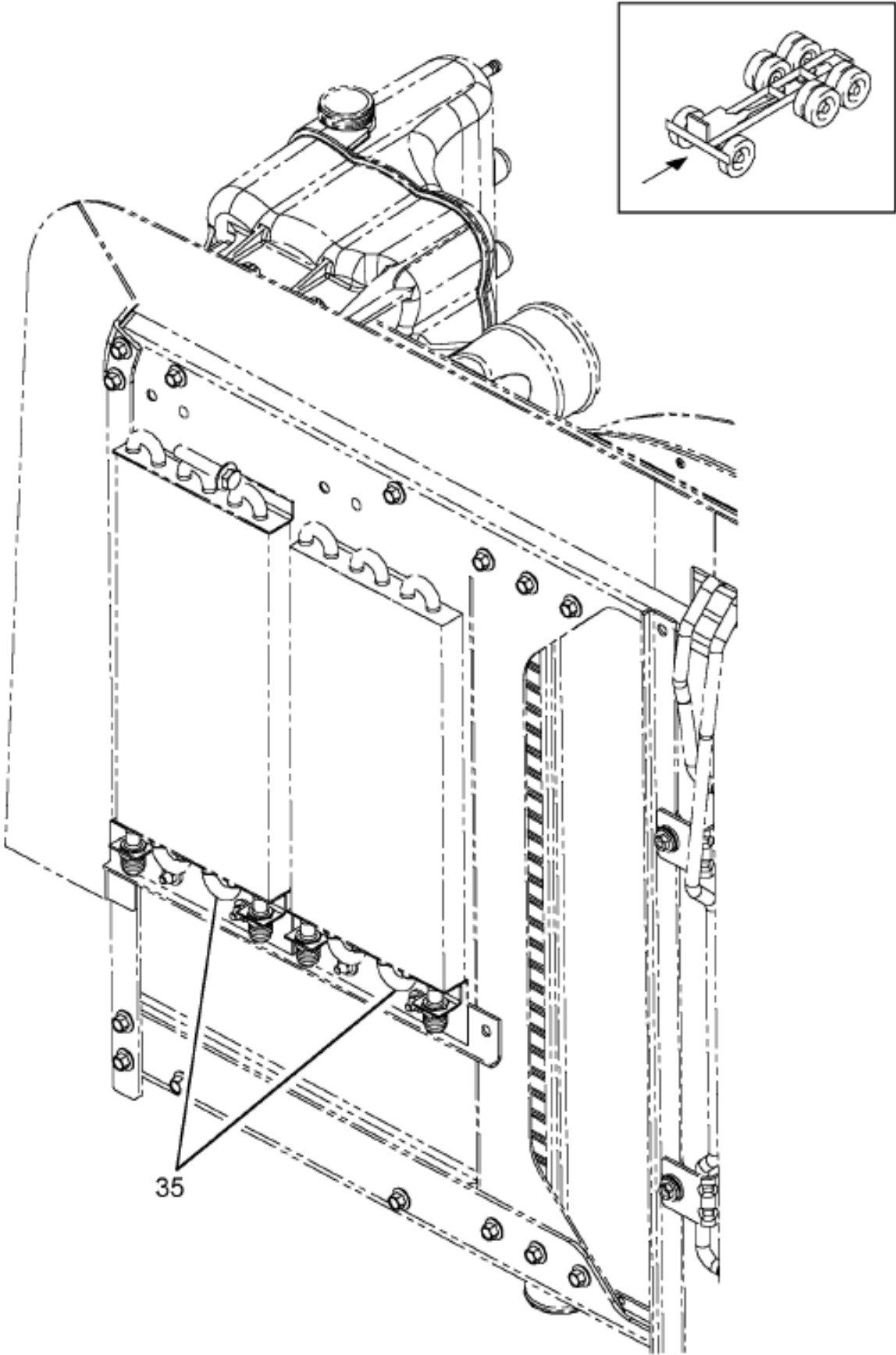
Figure 06XDK OIL COOLER, TRANS; MANUAL
