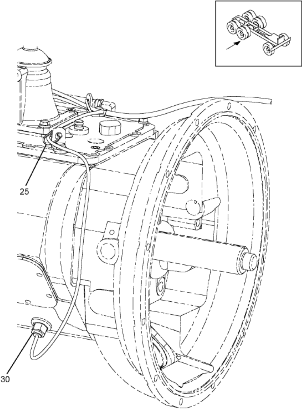
Figure 0GXF7 TRANSMISSION OIL TEMP COMPONENTS
