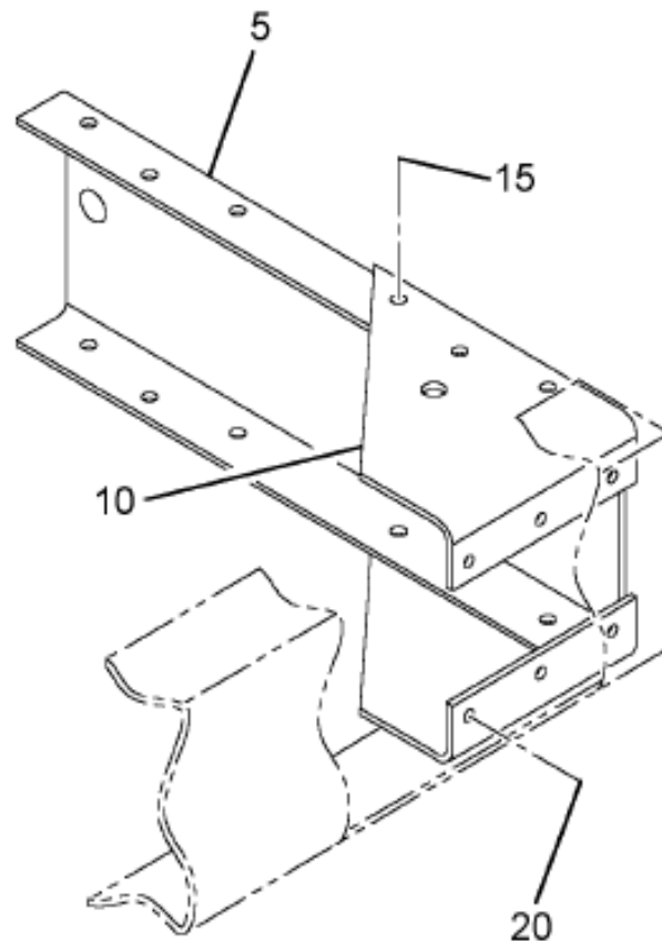
FLUSHED MOUNTED
