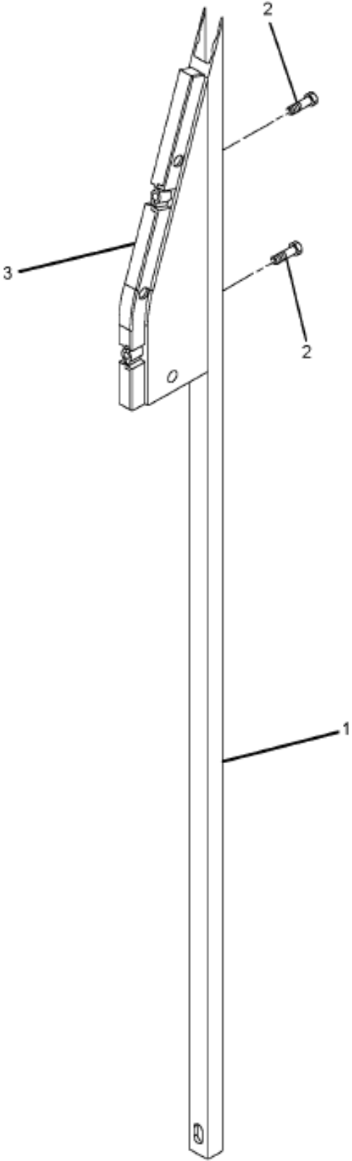
Figure 3516218C93 RETAINER, DOOR GLASS CHANNEL
