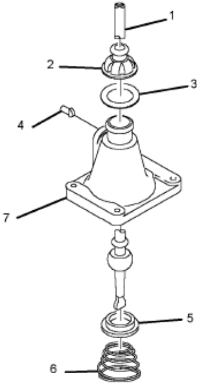
Figure 557069C91 HOUSING, CONTROL W/LEVER
