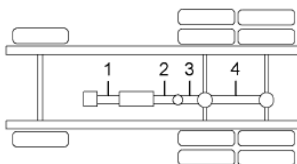
6X4, W/AUXILIARY TRANSMISSION AND ONE CENTER BEARING
