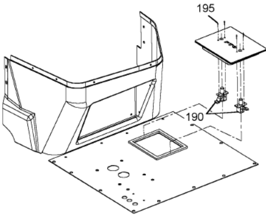
https://trackmanualshub.com/ Figure 0GVYC COVER INSTL, TRANS
