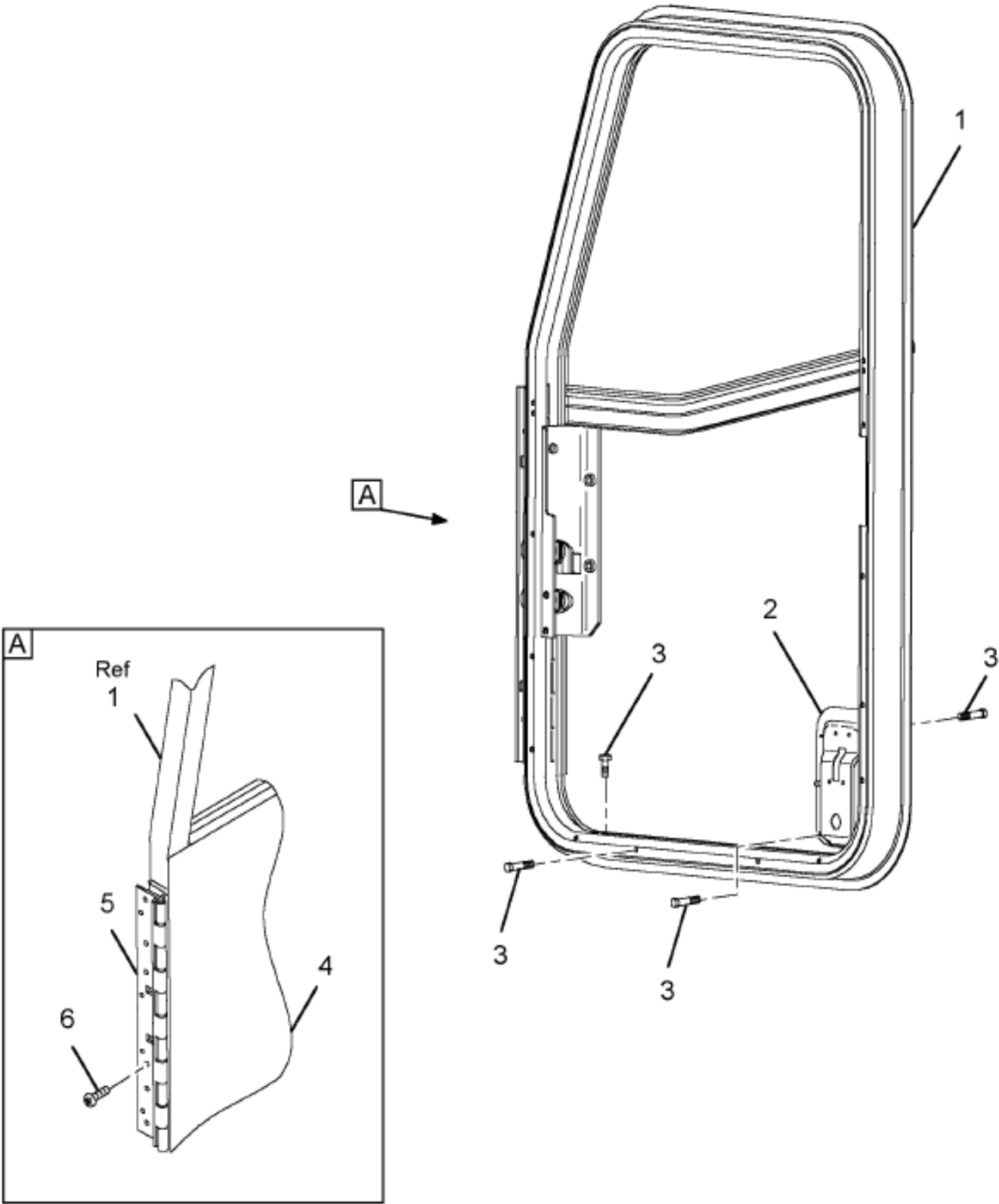
Figure 3544586C95 DOOR, CAB LT (SHELL)
