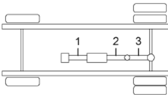
4X2, W/ AUXILIARY TRANSMISSION AND ONE CENTER BEARING
