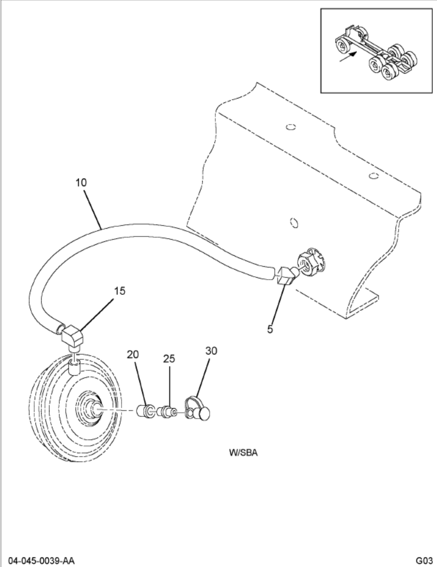
Figure 0G59X HOSING, FRONT AXLE
