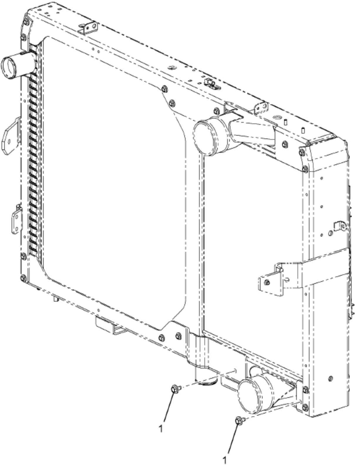
https://truckmanualshub.com/ Figure 2509897C91 KIT, ISOLATOR CAC
