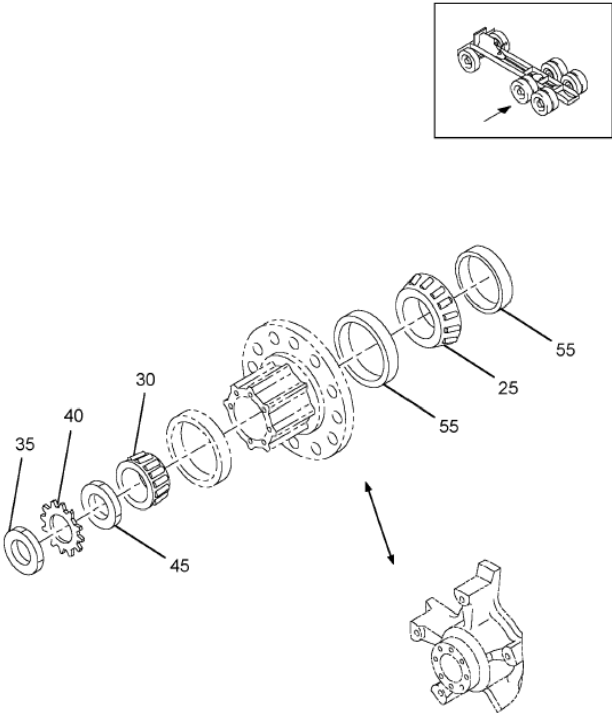
Figure 00QGT SEALS & BEARINGS; WHEELS, REAR AXLE
