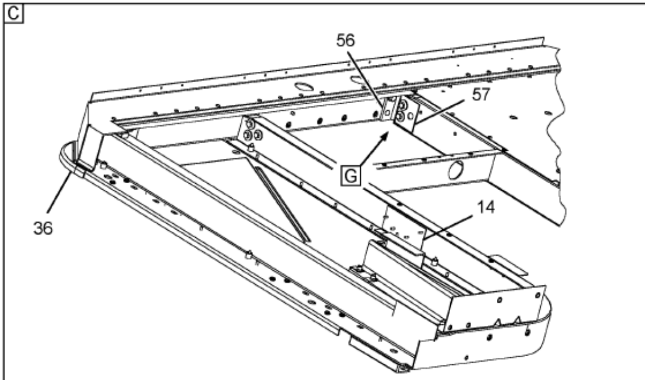
https://truckmanualshub.com/ Figure 3547334C95 UNDERBODY, ASM DAYCAB
