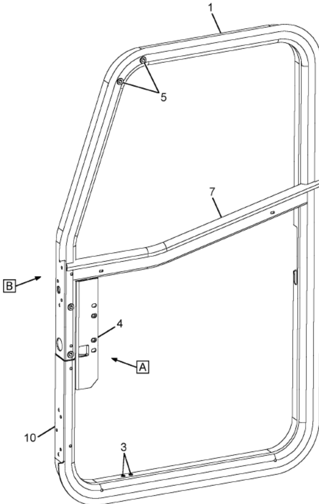
https://truckmanualshub.com/ Figure 3544816C2 FRAME, ASSY DOOR LH
