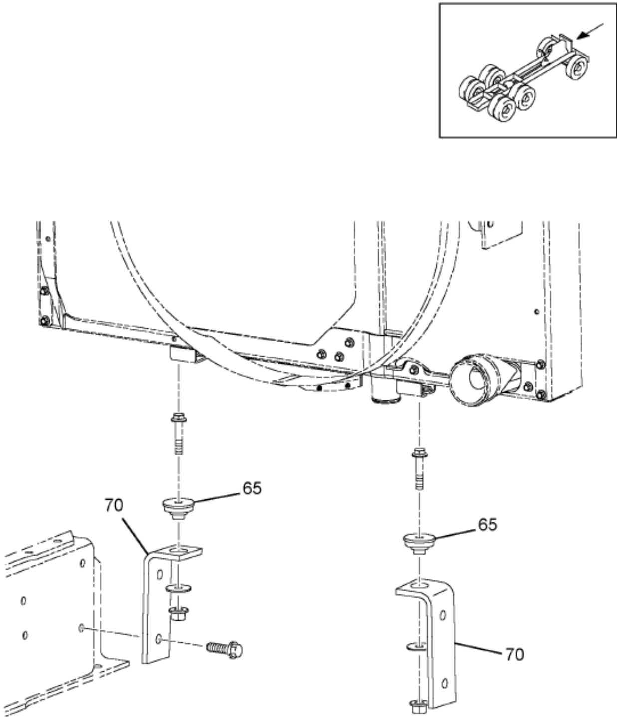
https://trackmanualshub.com/ Figure 0GXGD RADIATOR MTG
