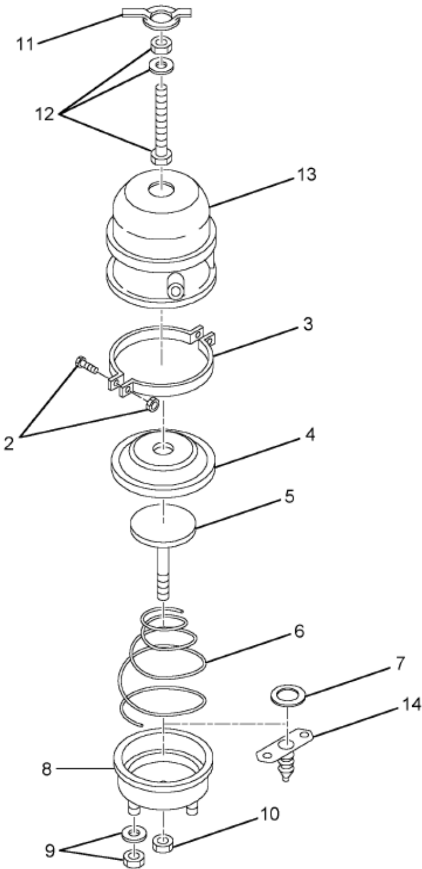
Figure 1688940C91 CHAMBER, BRAKE
