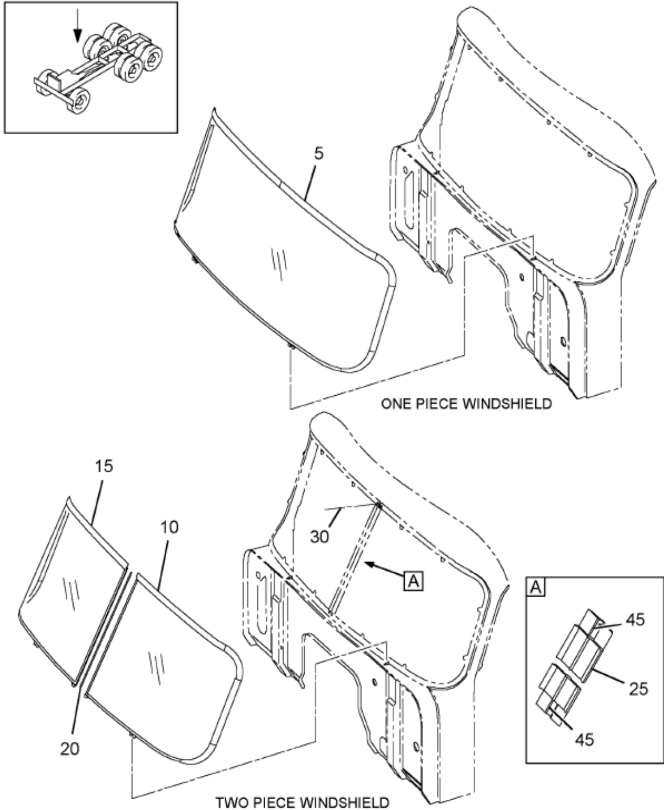
Figure 05673 WINDSHIELD INSTL
