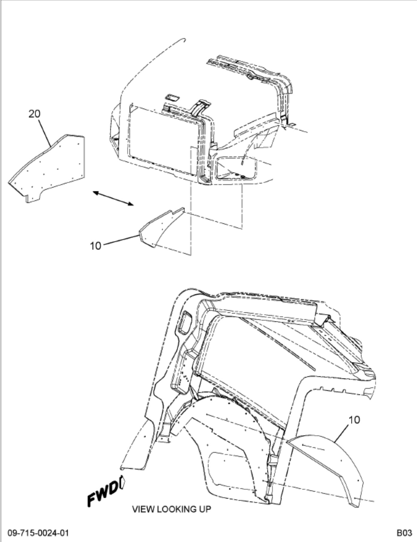
https://truckmanualshub.com/ Figure 0K26M INSULATOR, FRONT END; SPLASH GUARD
