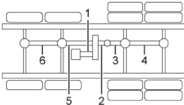
8X8, W/ONE CENTER BEARING
