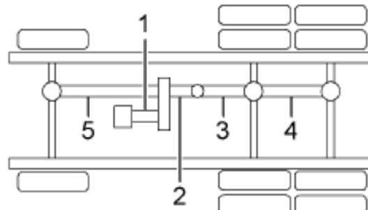
6X6, W/ONE CENTER BEARING
