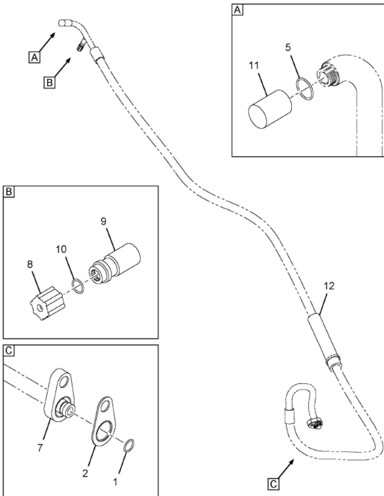
https://trucksmanualshub.com/ Figure 35654/3C93 HOSE, A/C EVAP TO COMPR
