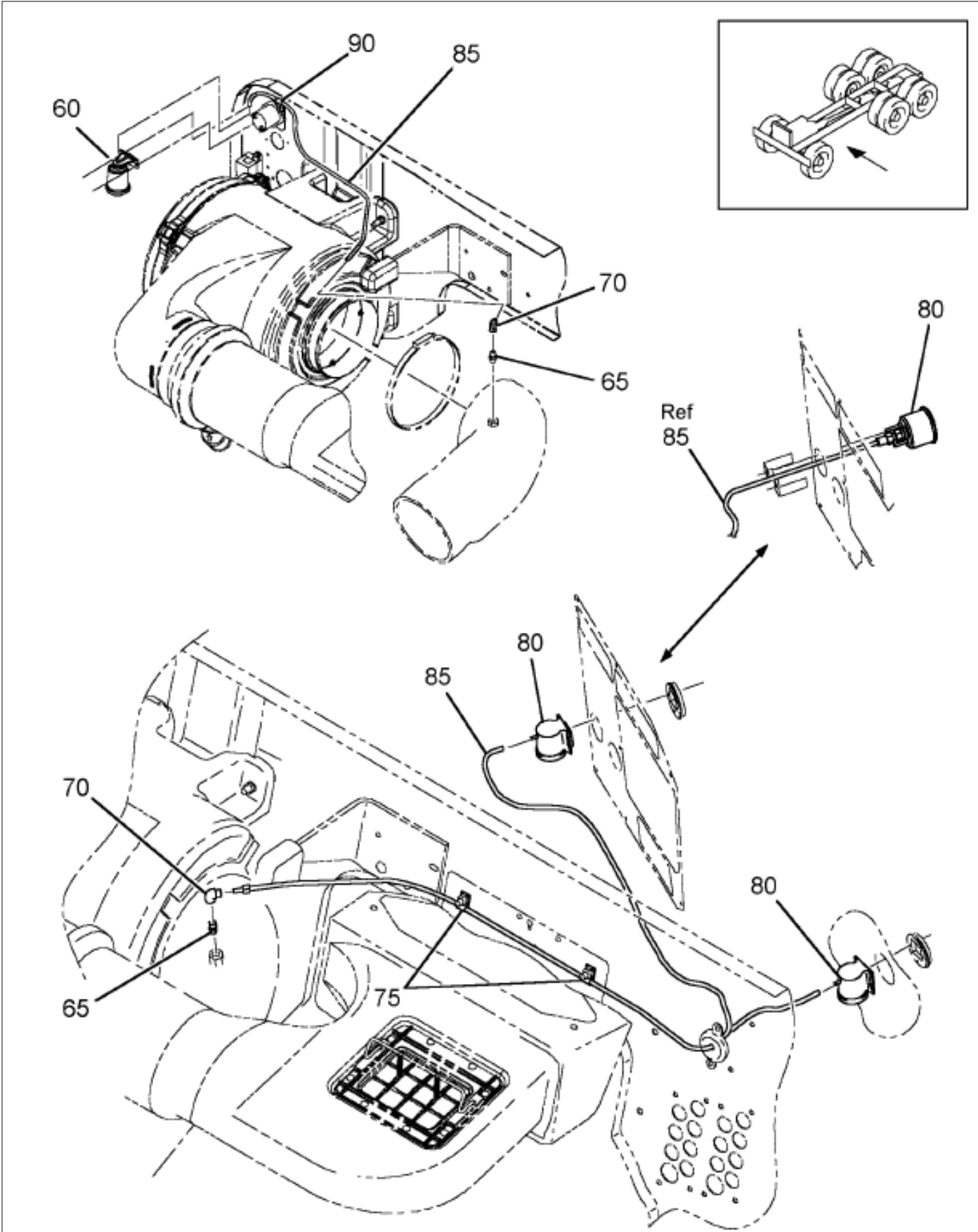
Figure 05VW4 AIR RESTRICTION GAUGE INSTL
