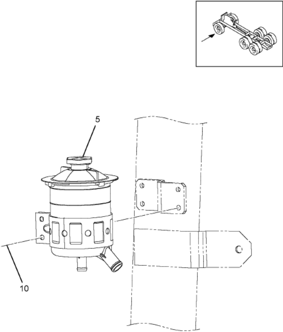
Figure 0GX5F POWER STEERING RESERVOIR & MTG
