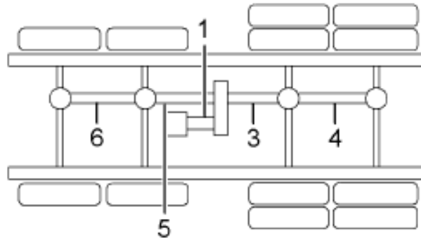
8X8, W/O CENTER BEARING
