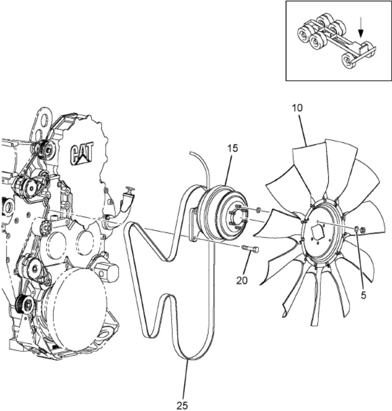
Figure 01102 FAN DRIVE & MTG; HORTON, BORG WARNER
