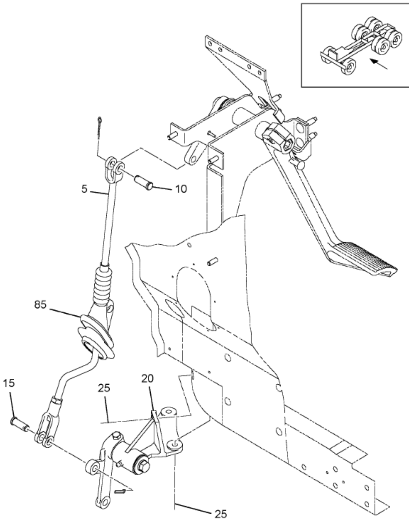
https://trucksmanualshub.com/ Figure 06TH7 CLUTCH CONTROL, UPPER
