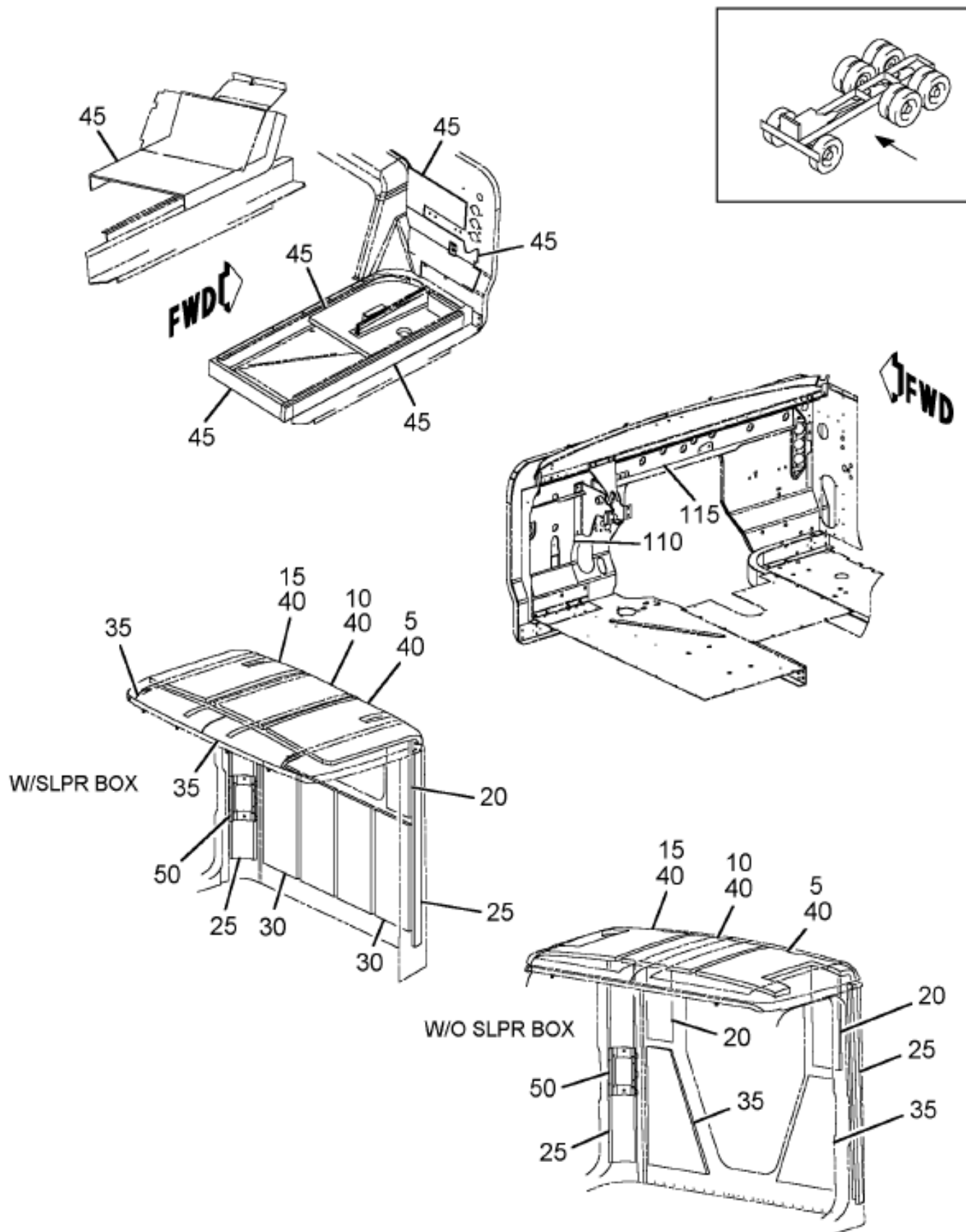
https://truckmanualshub.com/ Figure 052ZR INSULATOR INSTL, CAB
