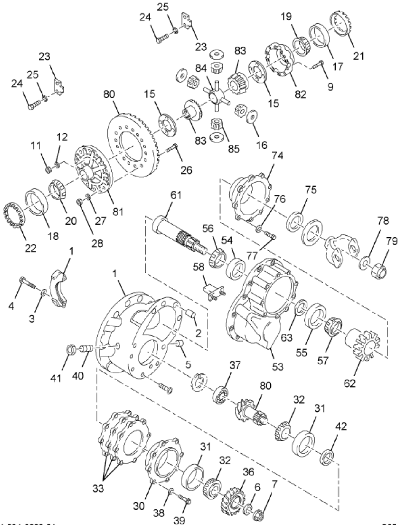
https://truckmanualshub.com/ Figure 1668175C91 DIFFERENTIAL, RR RR 6.07
