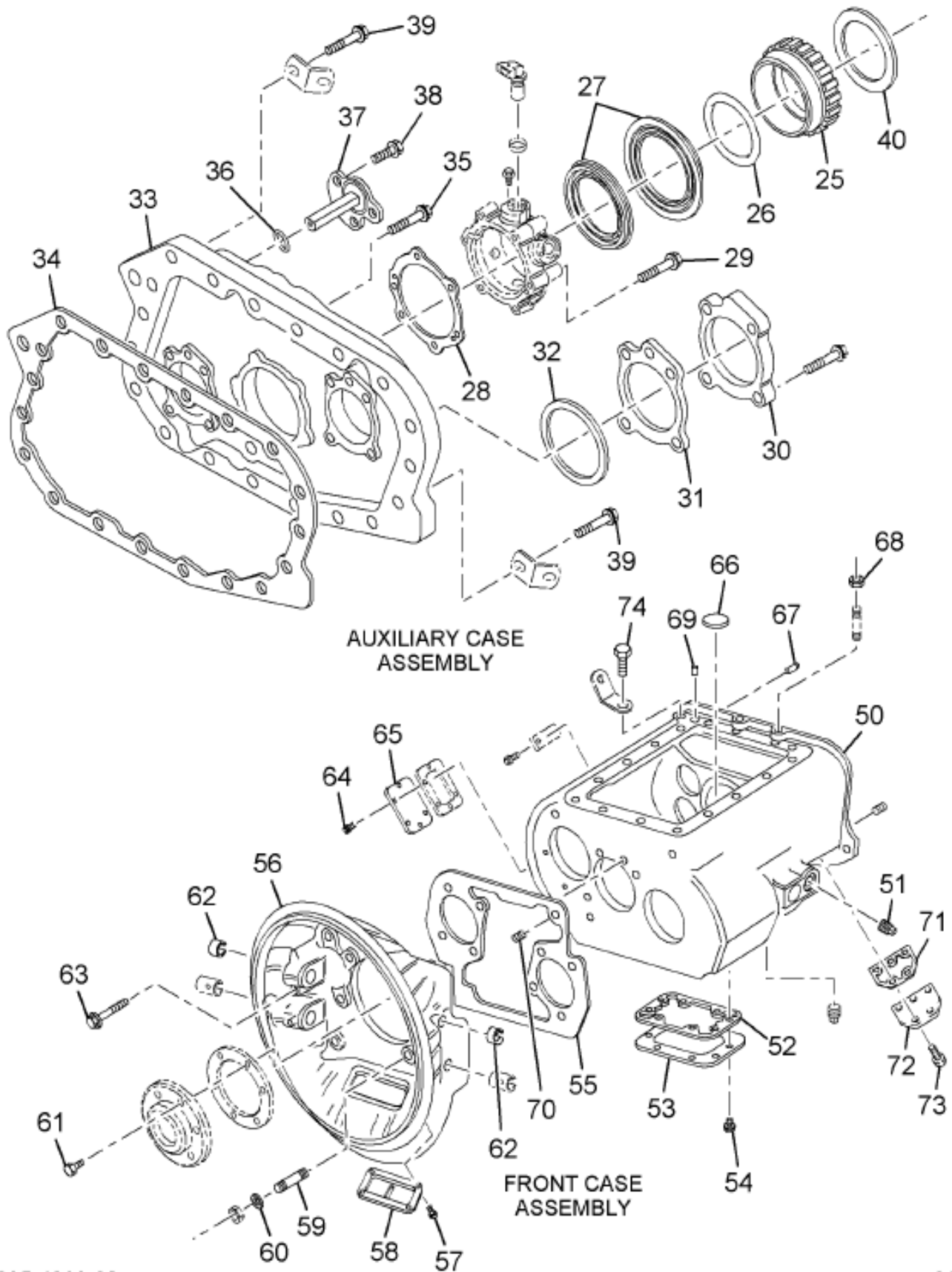
https://ruclmanualshub.com/ Figure 3505487C91 TRANSMISSION, W/HSG 13GHS
