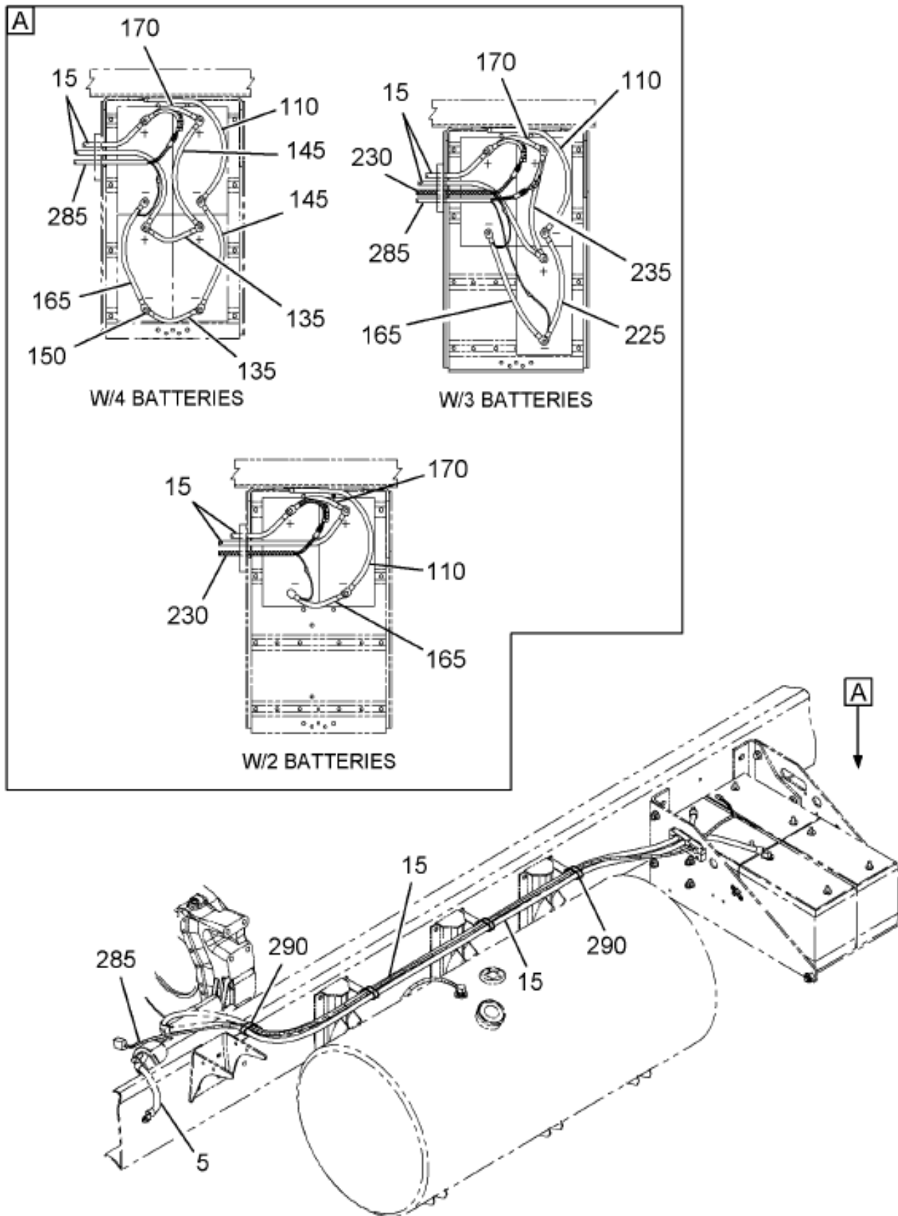
https://truckmanualshub.com/ Figure 01HDS0 BATTERY CABLES
