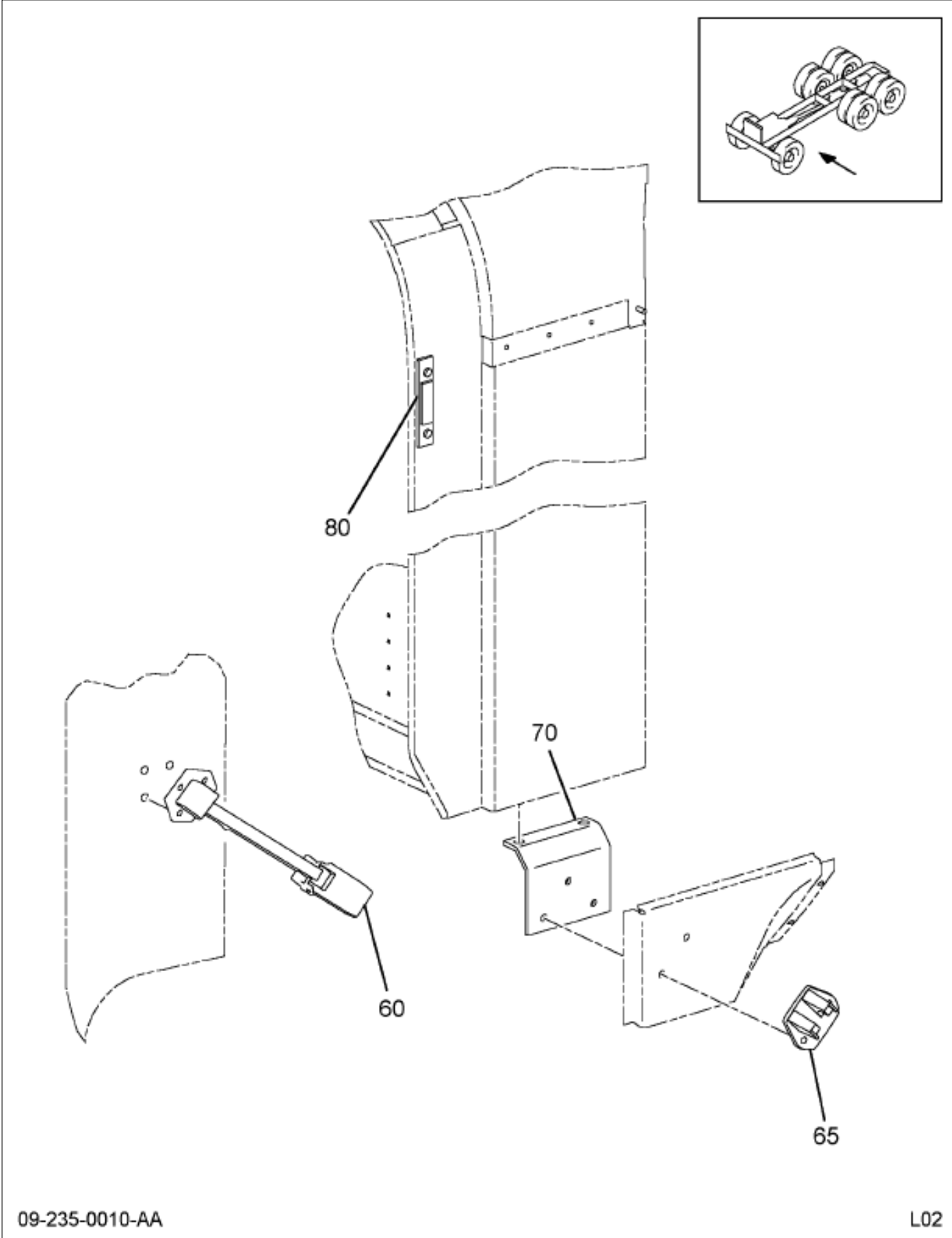
Figure 05558 MTG LATCH INSTL, HOOD; 9100/9200/94
