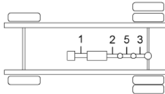
4X2, W/ AUXILIARY TRANSMISSION AND TWO CENTER BEARINGS
