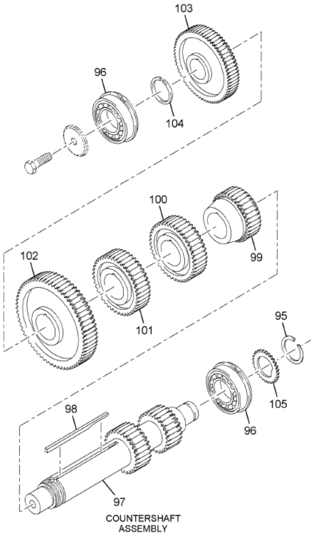
https://ruclmanualshub.com/ Figure 3505487C91 TRANSMISSION, W/HSG 13GHS
