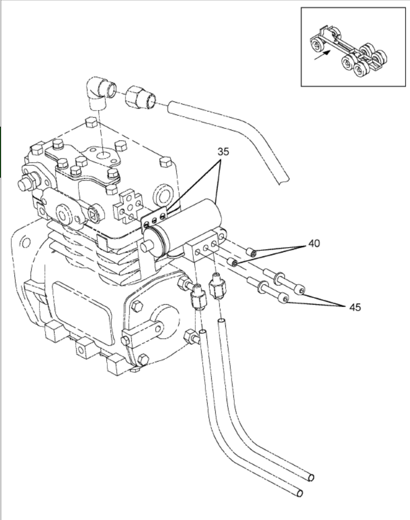
https://truckmanualshub.com/ Figure 0GZVL GOVERNOR INSTL
