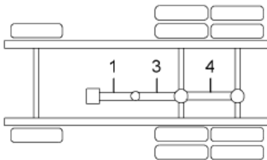
6X4, W/ONE CENTER BEARING
