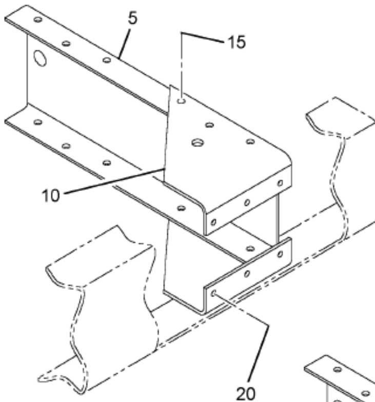
STANDARD LOCATION
