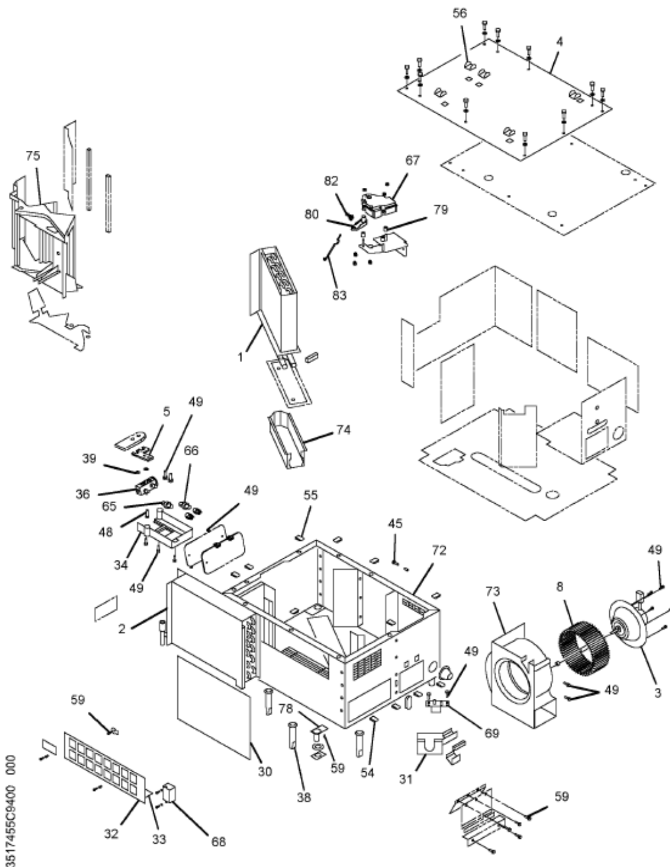
https://trucksmanualshub.com/ Figure 3517455C94 HEATER, A/C DAYCAB
