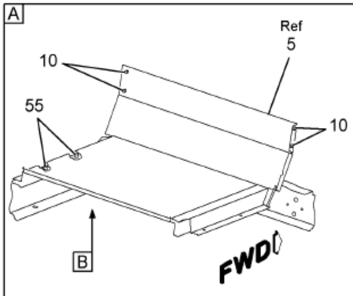
https://truckmanualshub.com/ Figure 052FM FLOOR PANEL, RT FRONT
