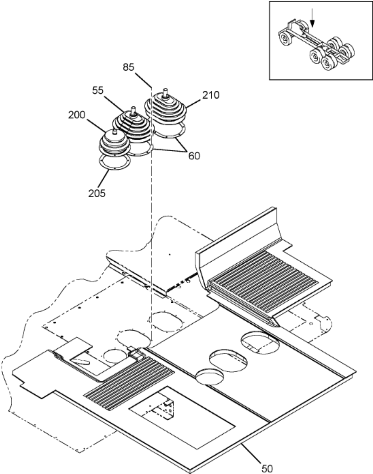
https://truckmanualshub.com/ Figure 0HBHY FLOOR MAT FOR 5000I
