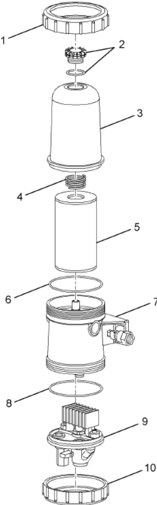
https://buckmanualshub.com/ Figure 3526573C92 FILTER, FUEL *DAVCO 382030CMDVNA
