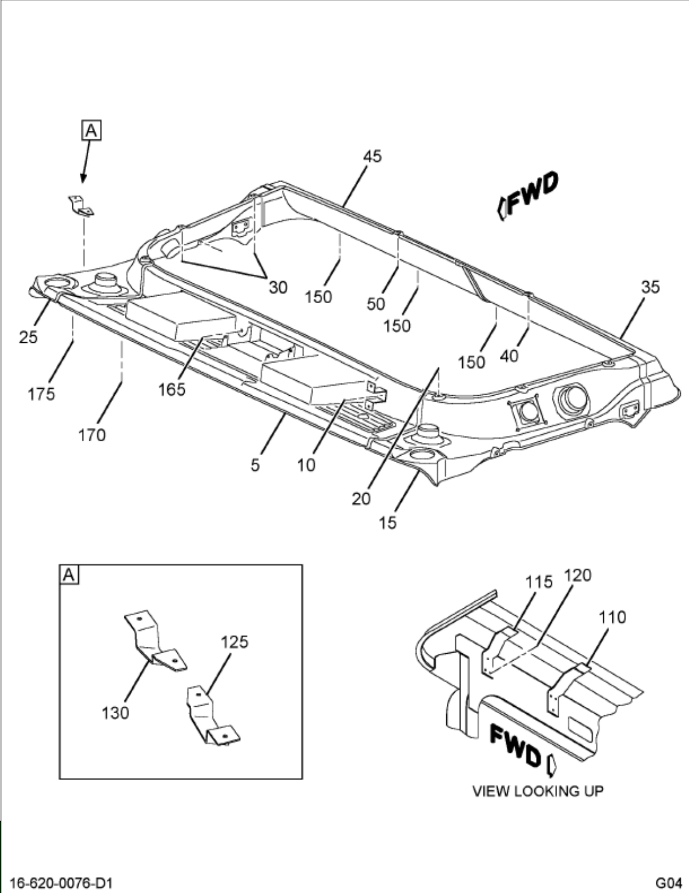
https://truckmanualshub.com/ Figure 015R7 PANELS, TRIM; ROOF HEADER & COVE
