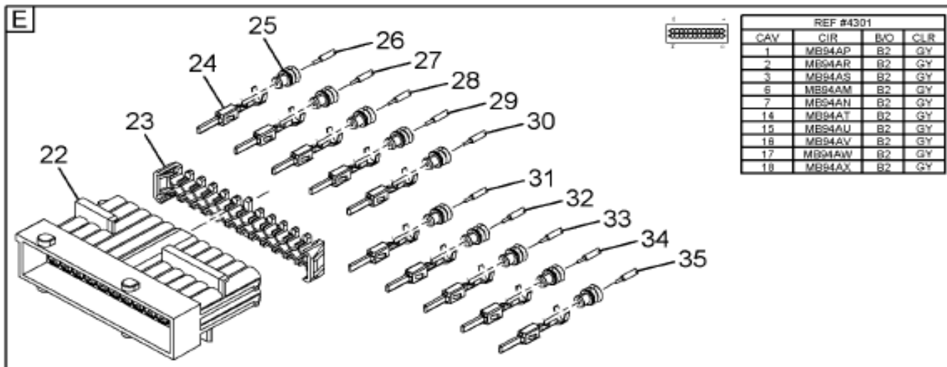
Figure 358186C91 HARNESS, DASH WRG, AIR ABS N/ATC
