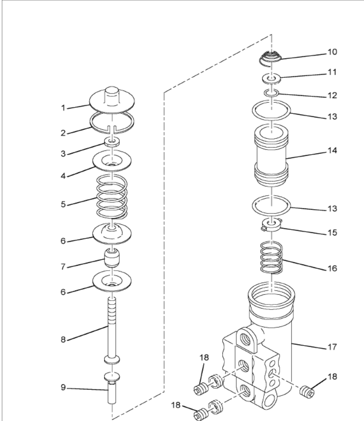
Figure 410986C92 GOVERNOR, ASSY D-2
