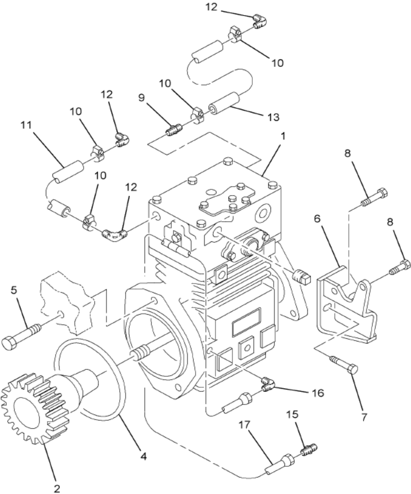
Figure 641016L002 COMPRESSOR, AIR
