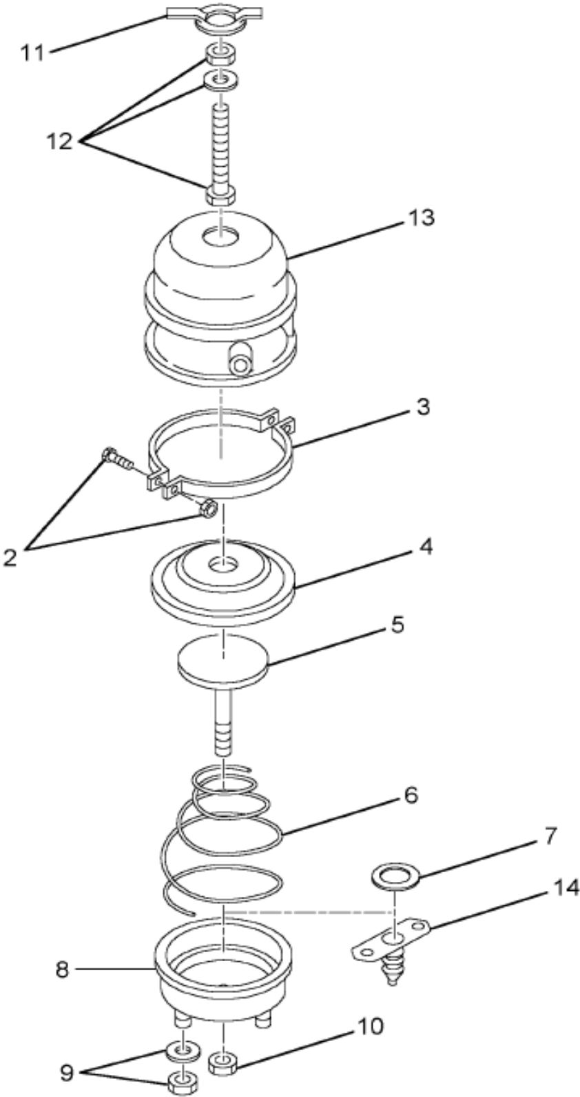
Figure 350654C91 CHAMBER, BRAKE*MGM TR3030LP3HD
