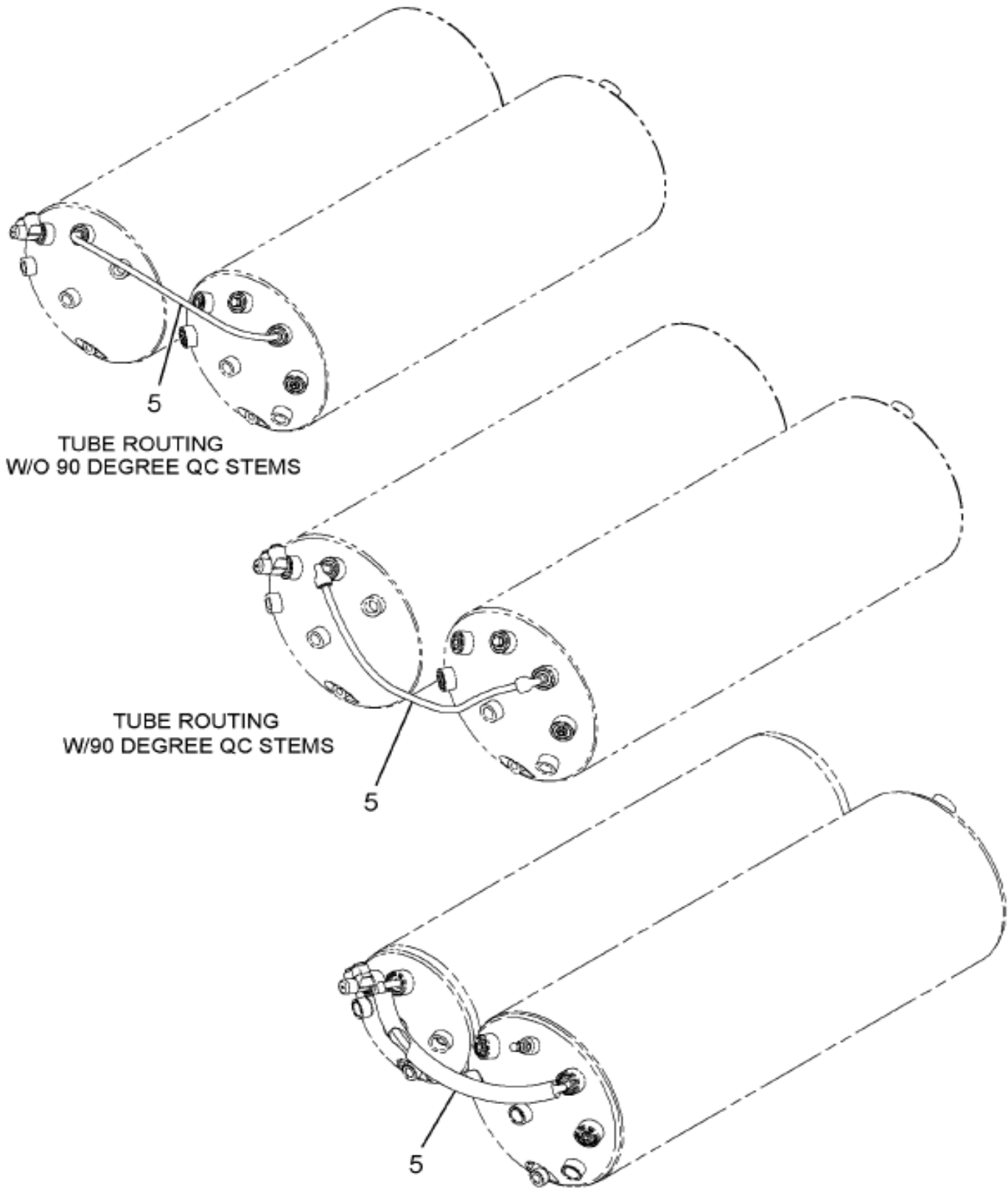
https://truckmanualshub.com/ Figure 011WFB AIR TANK TUBING; PRIMARY TANK
