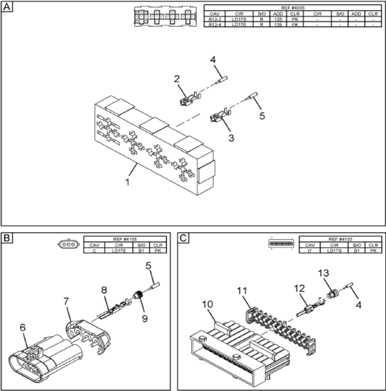
https://truckmanualshub.com/ Figure 3588674C91 HARNESS, DASH START W/ INTL ENG
