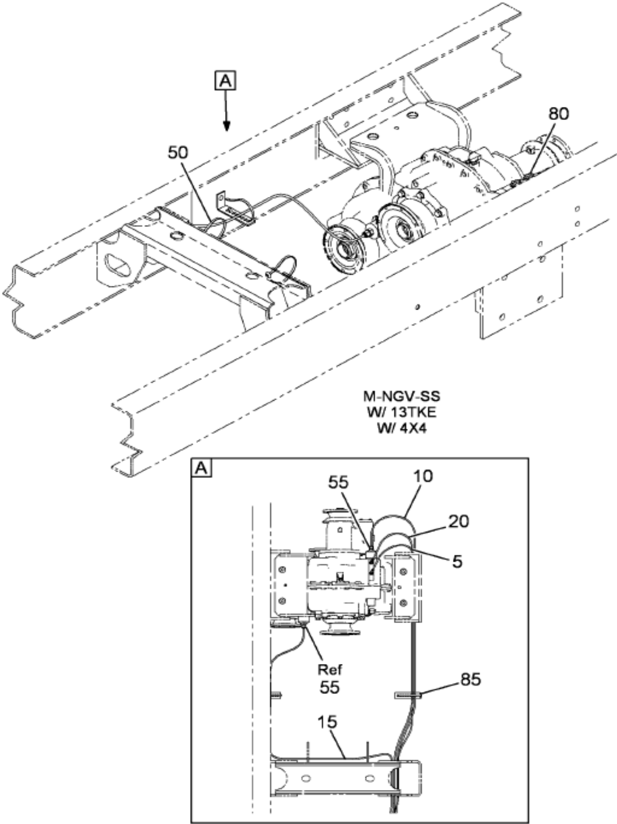
https://www.manualshub.com/ Figure 07VRS TRANSFER CASE CONTROL INSTL
