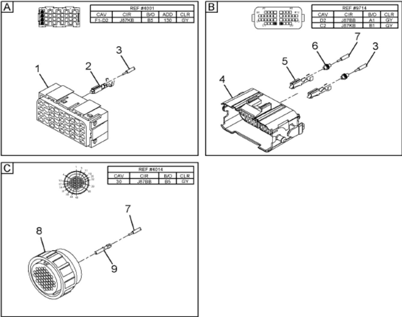
Figure 3568510C91 https://truckmanualshub.com/ HARNESS, CHASSIS WIRING*WASHER
