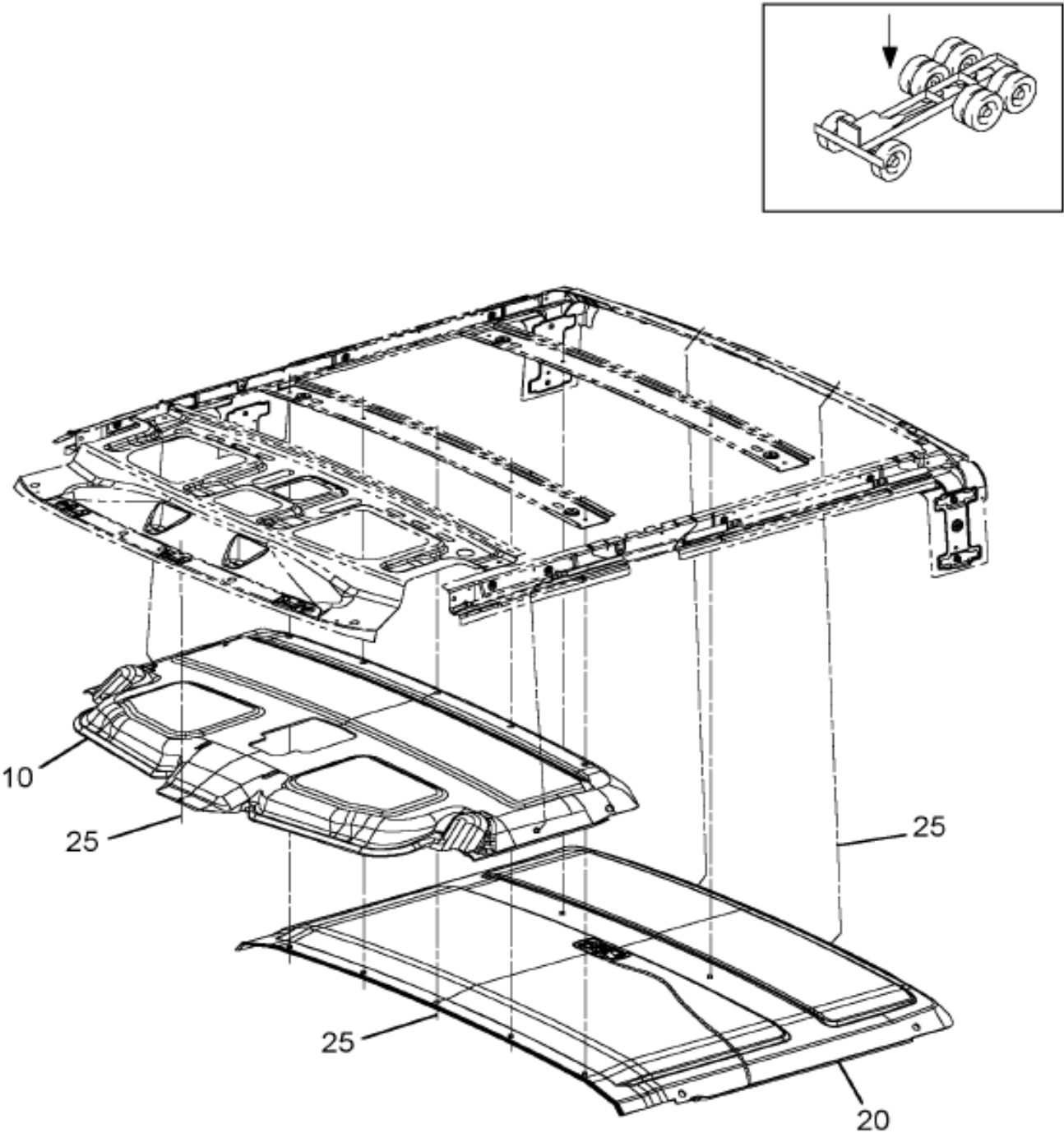
Figure 06SH0 INTERIOR TRIM; HEADLINER
