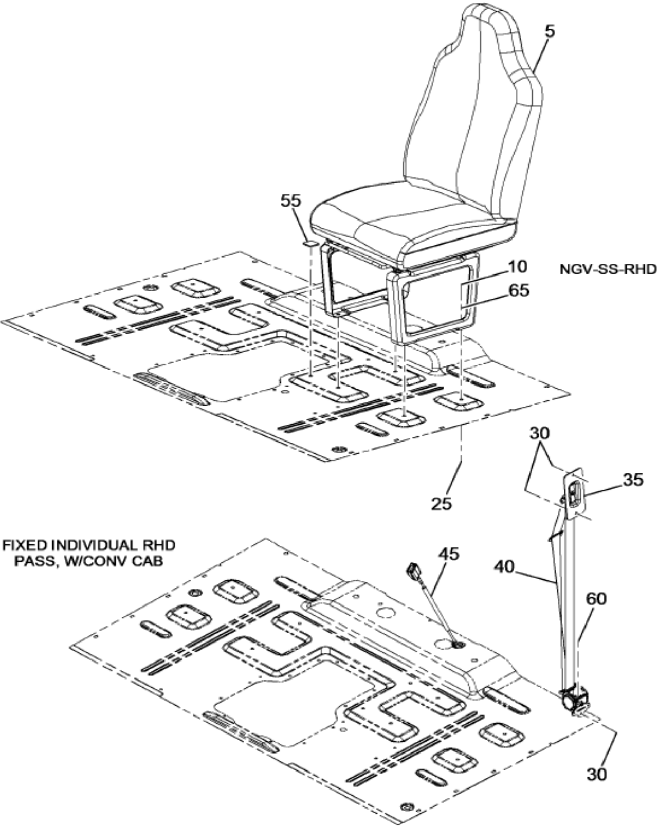
https://truckmanualshub.com/ Figure 06WJ7 PASS SEAT INSTL; W/ BELT
