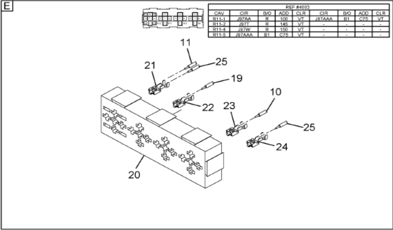
Figure 3568513C91 HARNESS, ENGINE*CEC I6 ENGINE
