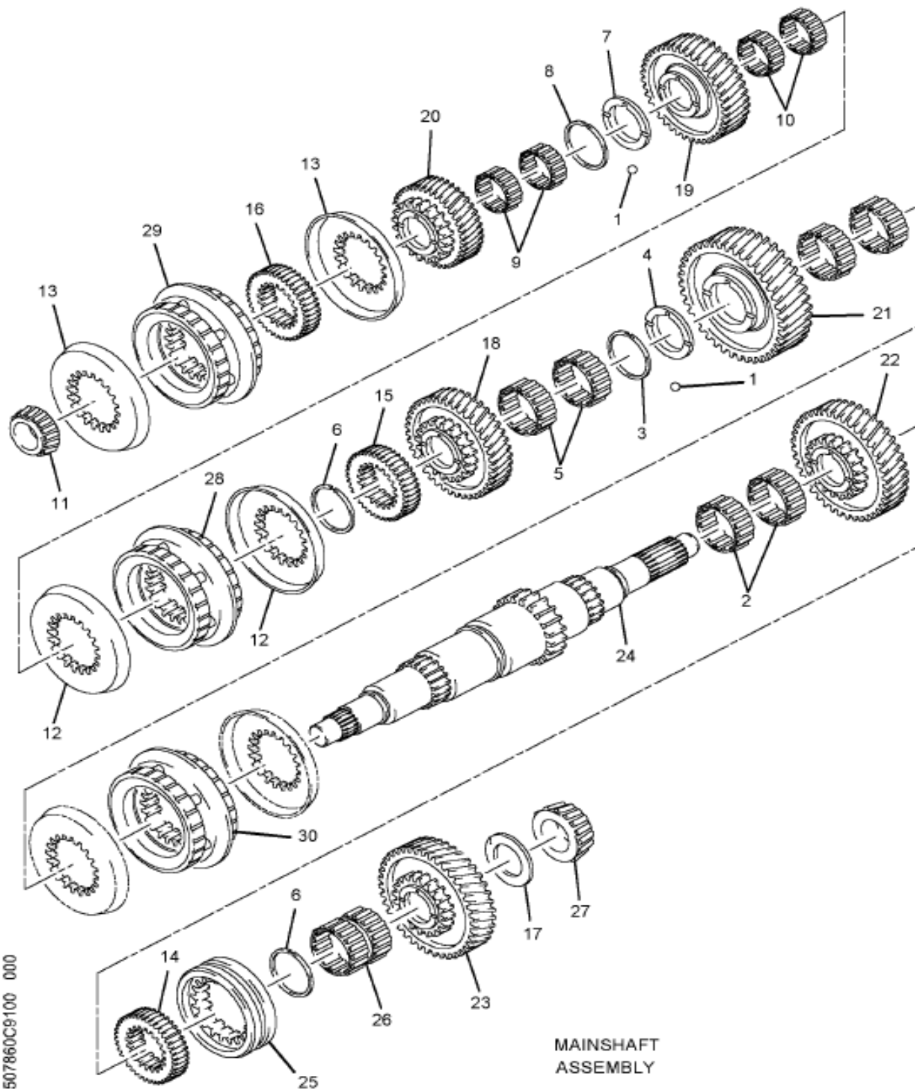
https://www.manualshub.com/ Figure 2507860C91 SHAFT, TRANS MAIN
