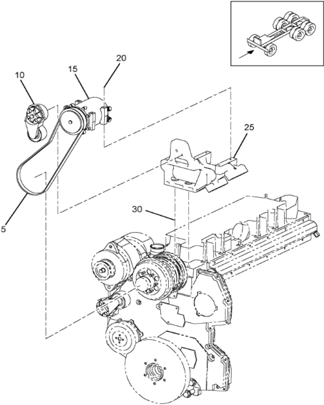
https://truckmanualshub.com/ Figure 00132 A/C COMP SR INSTL; EATON
