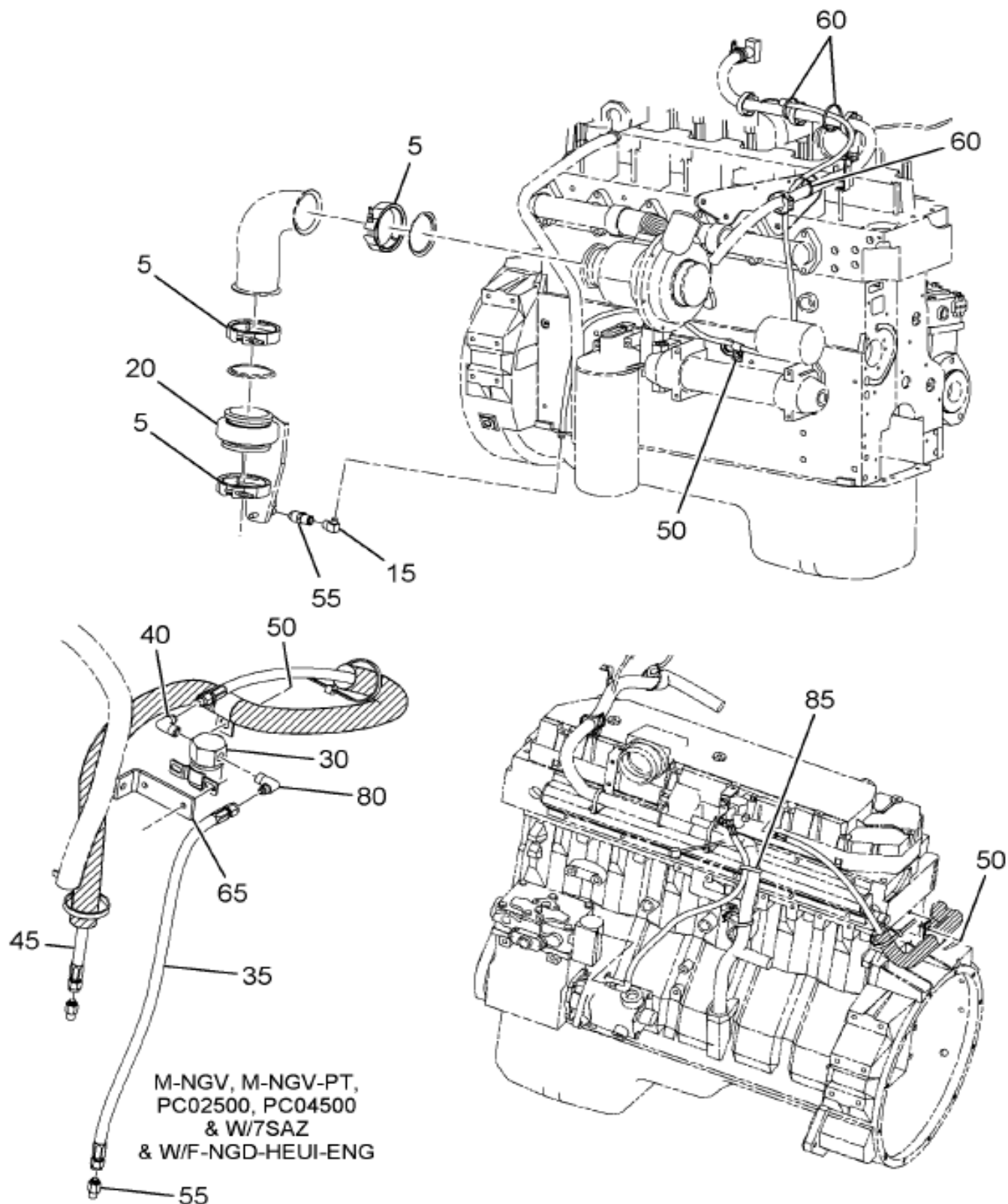
https://truckmanualshub.com/ Figure 0HGRZ EXH BRK INSTL; PACBRAKE
