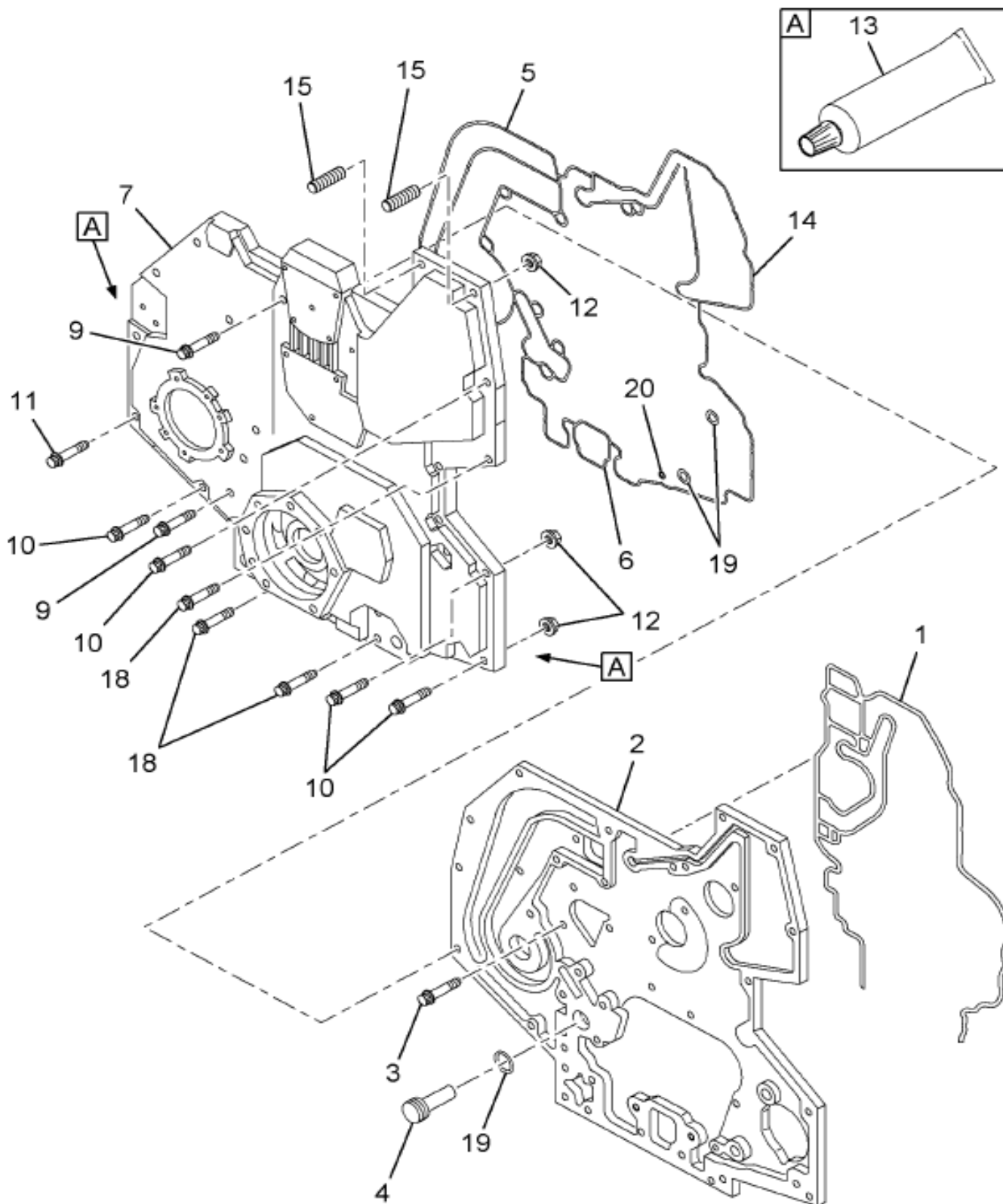
Figure 641006B009 COVER, FRONT (I-308)
