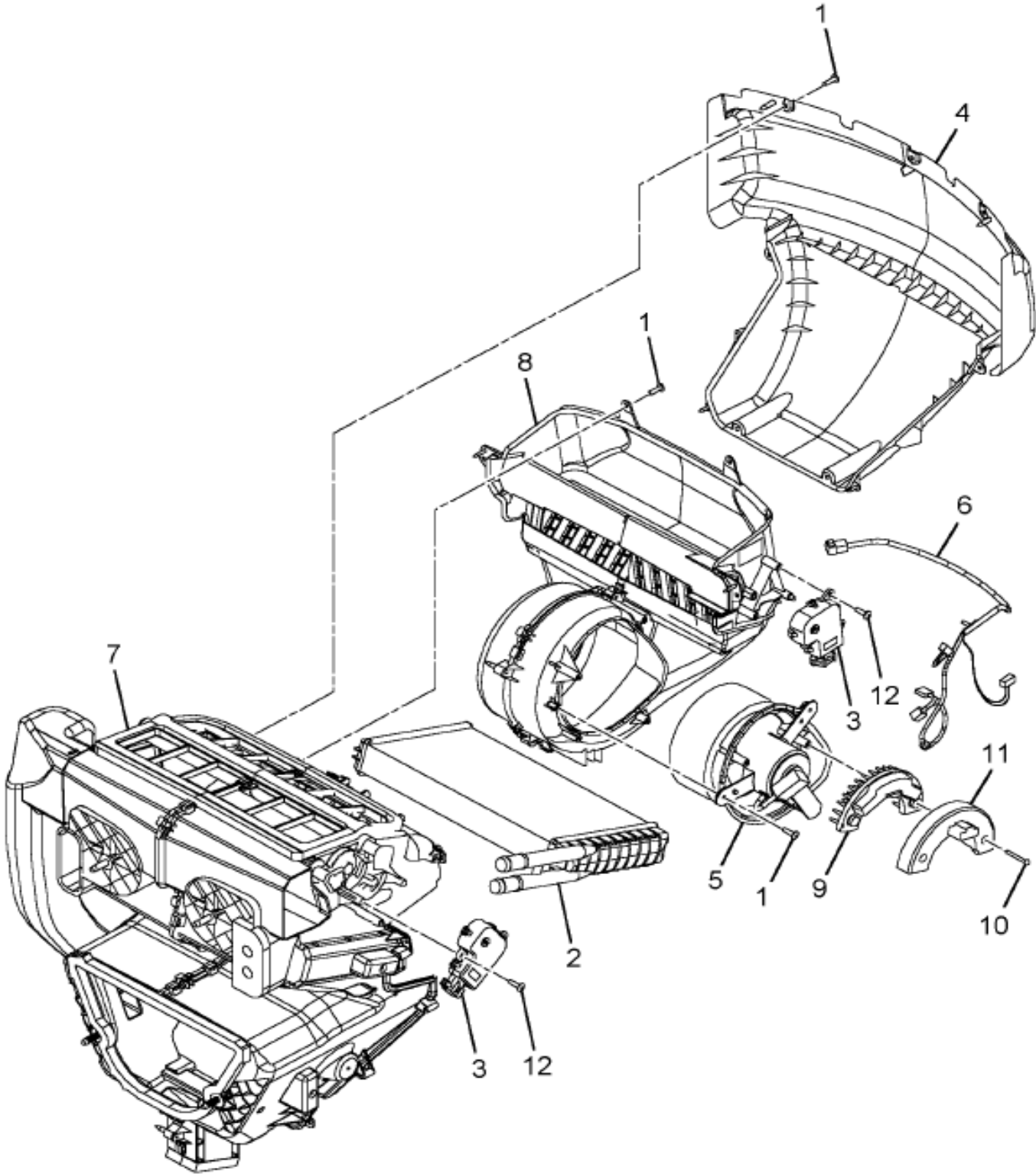
Figure 3545211C93 HEATER, ASSY FRESH AIR LHD CONV
