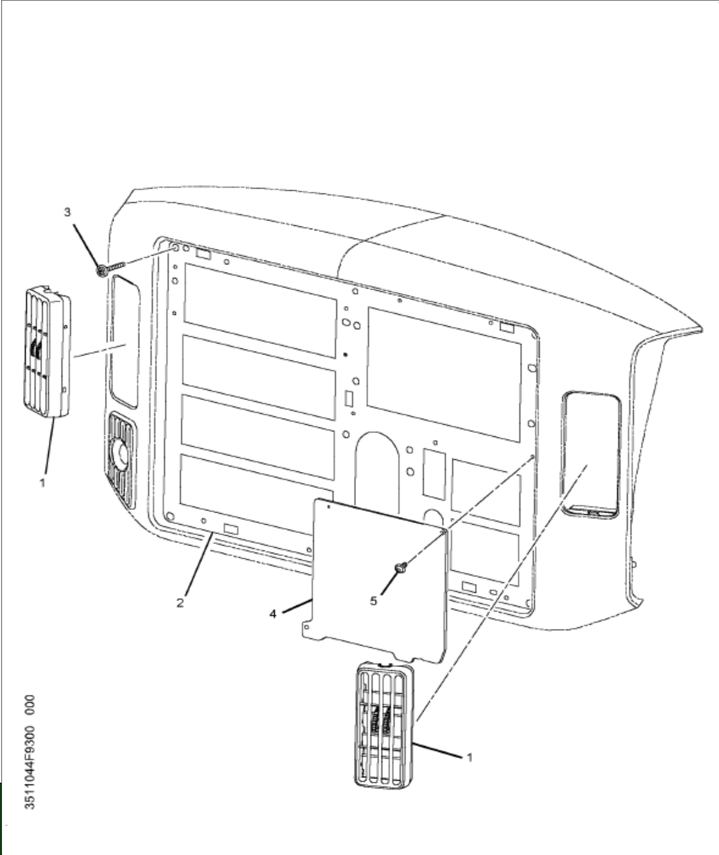
Figure 3511044F93 INST PNL FLT CTR ASSY LHD
