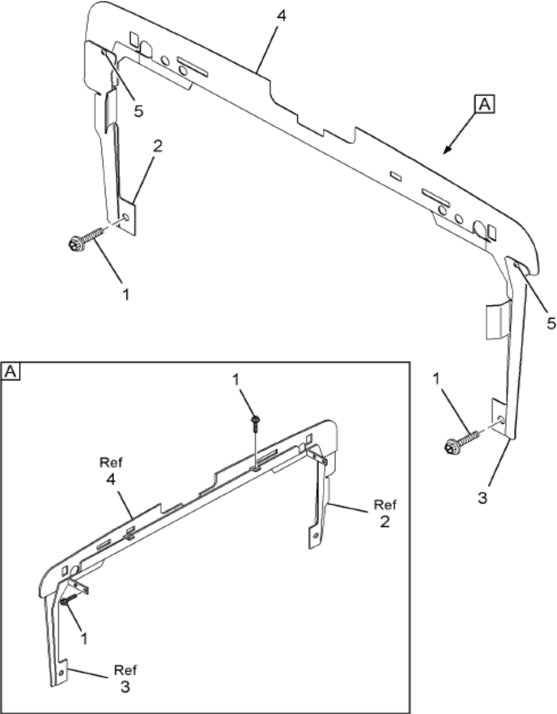
Figure 2507472C92 SEAL, COOLING RECIRC ASSY
