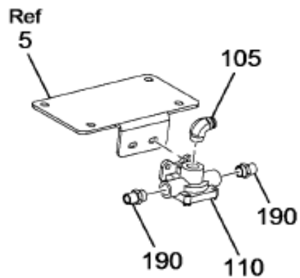
QUICK RELEASE VALVE MTG W/04091 W/12" RAILS N/01UAA
