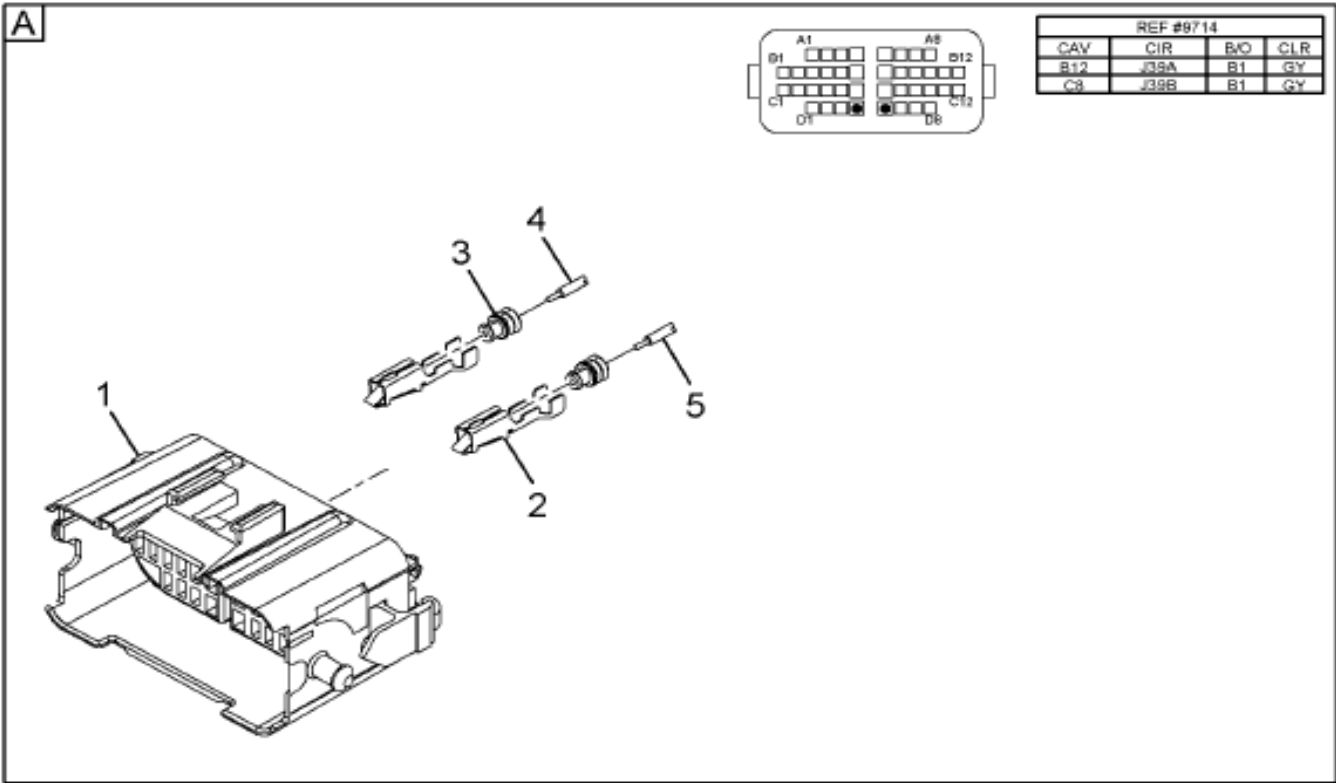
Figure 3549551C92 HARNESS, ELEC; AIR DRYER
