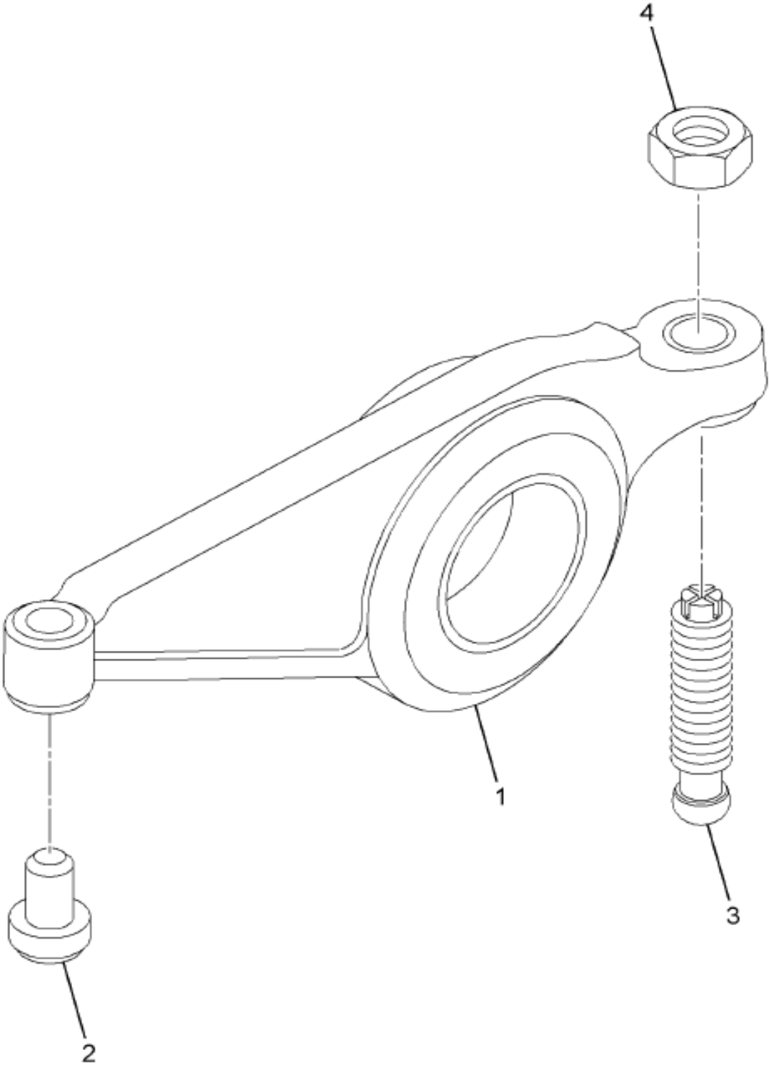
https://truckmanualshub.com/ Figure 1827155C95 ARM ASSY,ROCKER (RATIO 1:66)
