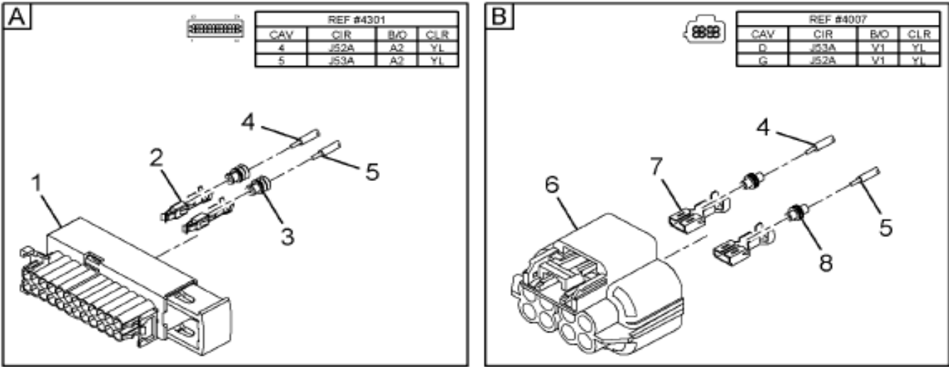
Figure 3560260C91 HARNESS, HEAD LIGHT WIRING *HEA
