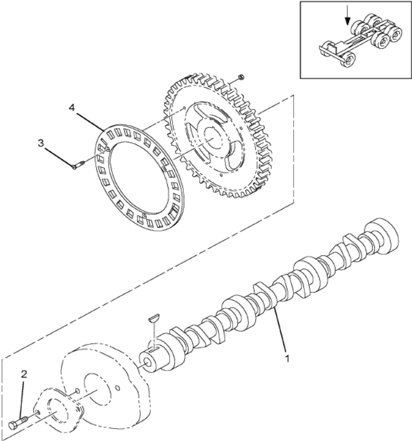
Figure 641003A004 CAMSHAFT
