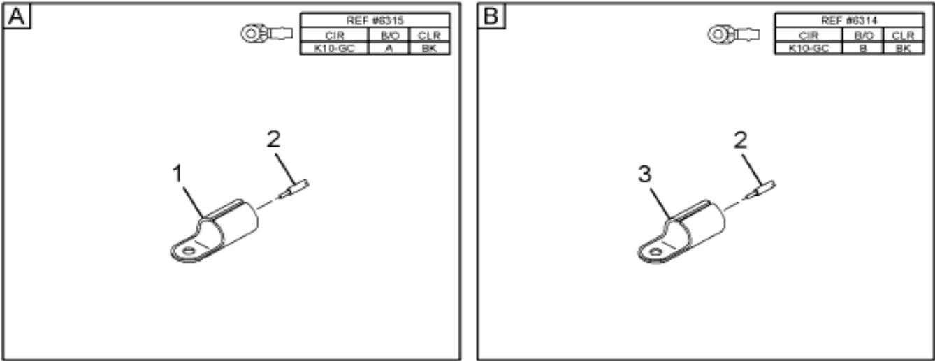
Figure 3565992C91 https://truckmanualshub.com/ HARNESS,ELEC; ENG BLOCK GRD
