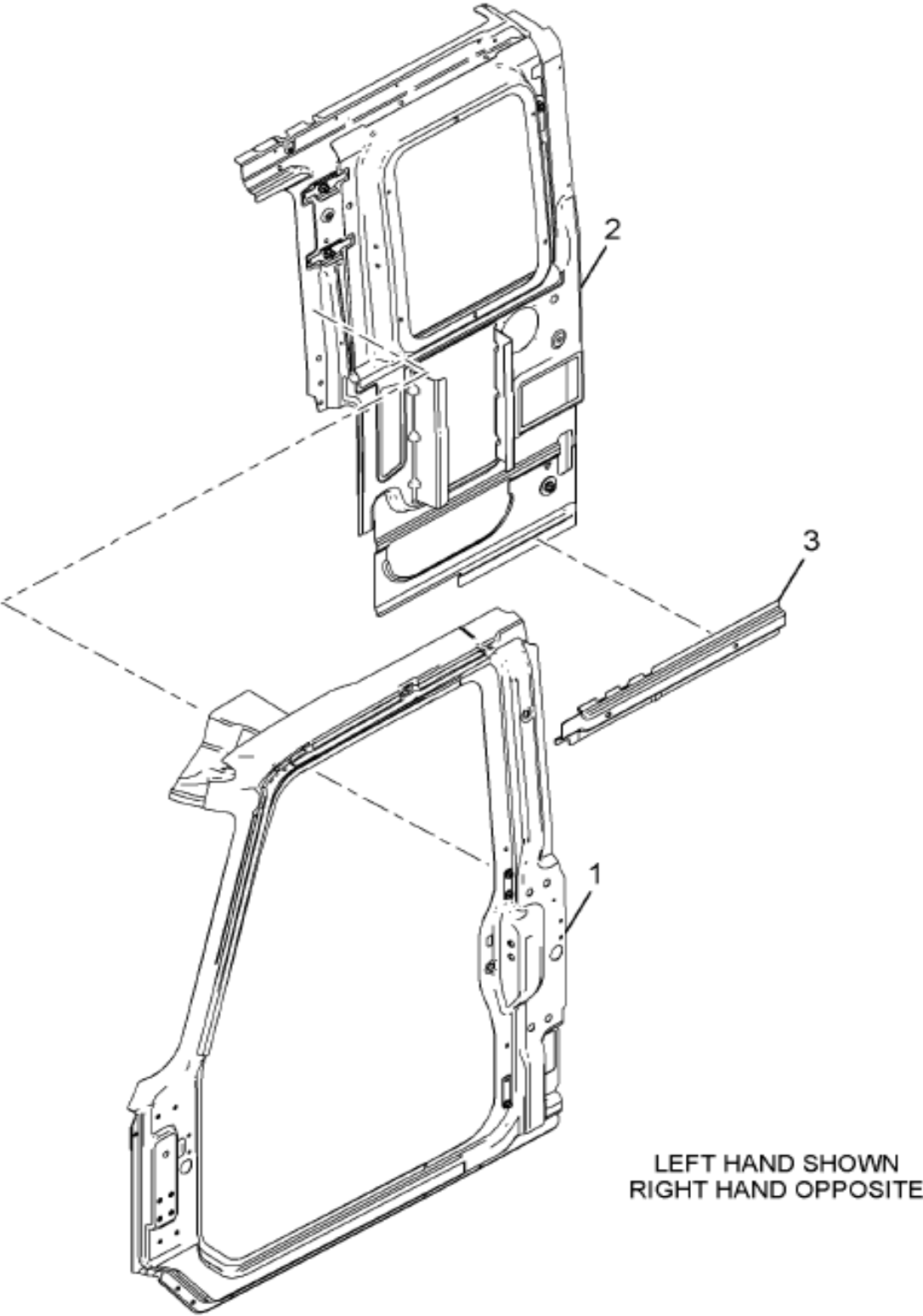
Figure 3548070C3 https://truckmanualshub.com/ PANEL, SIDE BODY SUB ASSY LH
