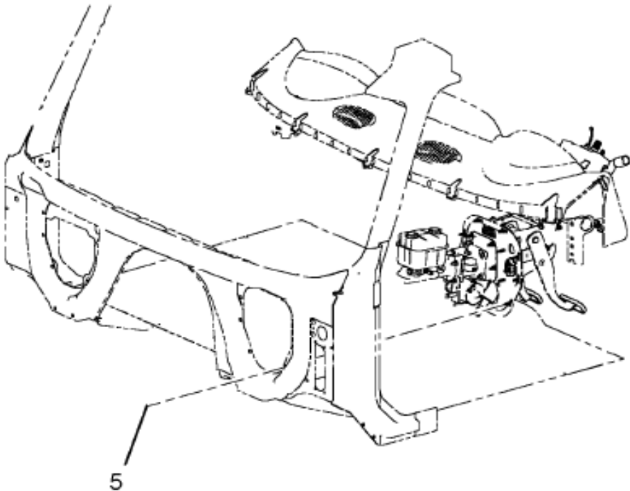
https://www.manualshub.com/ Figure 06Q53 DCM MOUNTING HARDWARE
