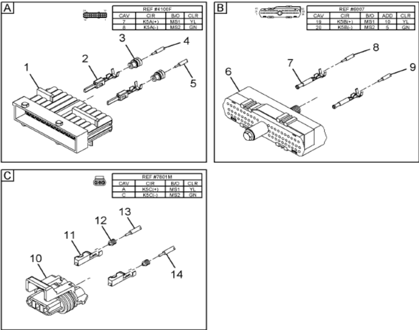
Figure 3577574C91 HARN,ELEC,J1939 O/L W/ALLSN&I6
