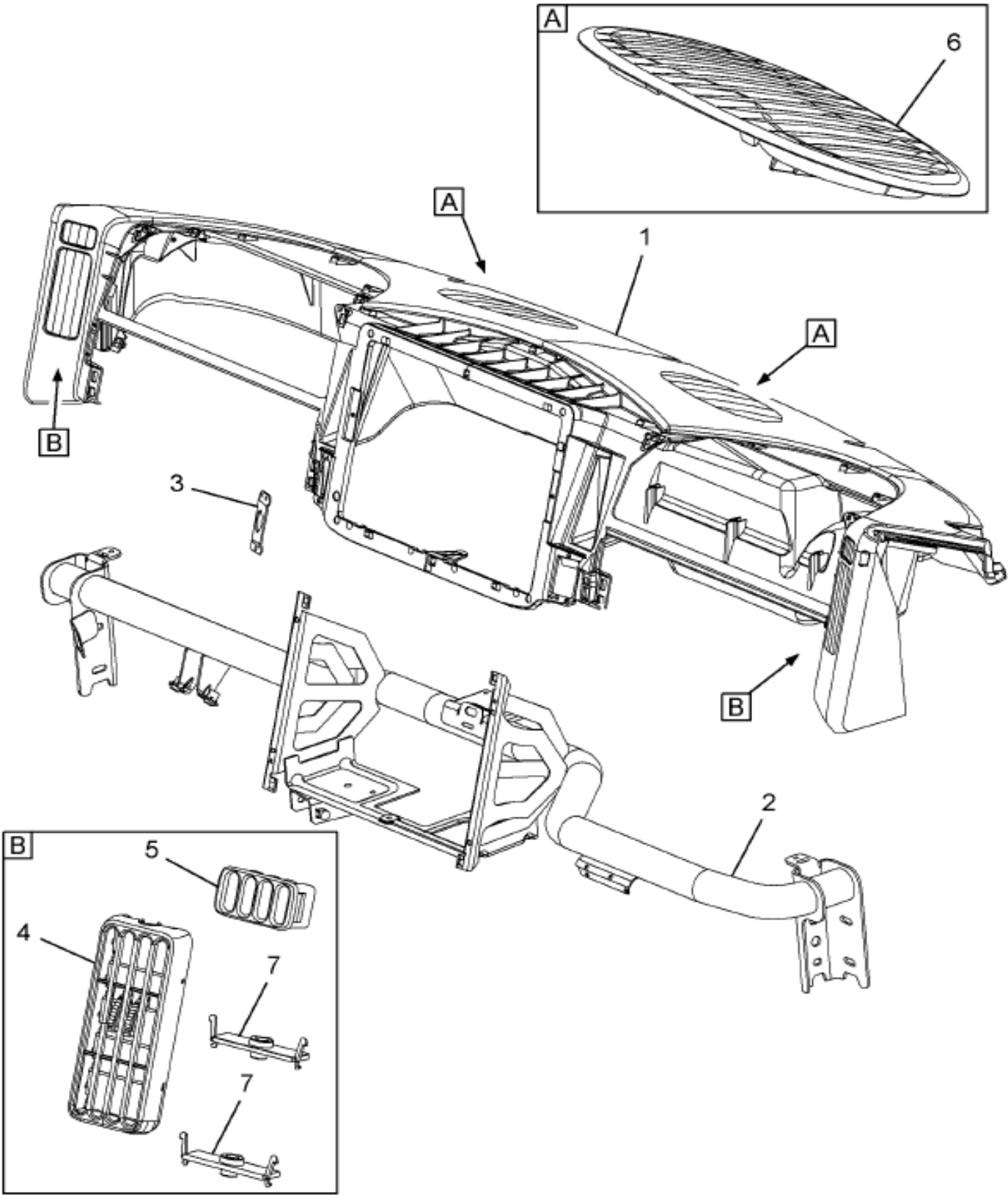
Figure 3511018P93 INST PANEL MAIN CARRIER LHD
