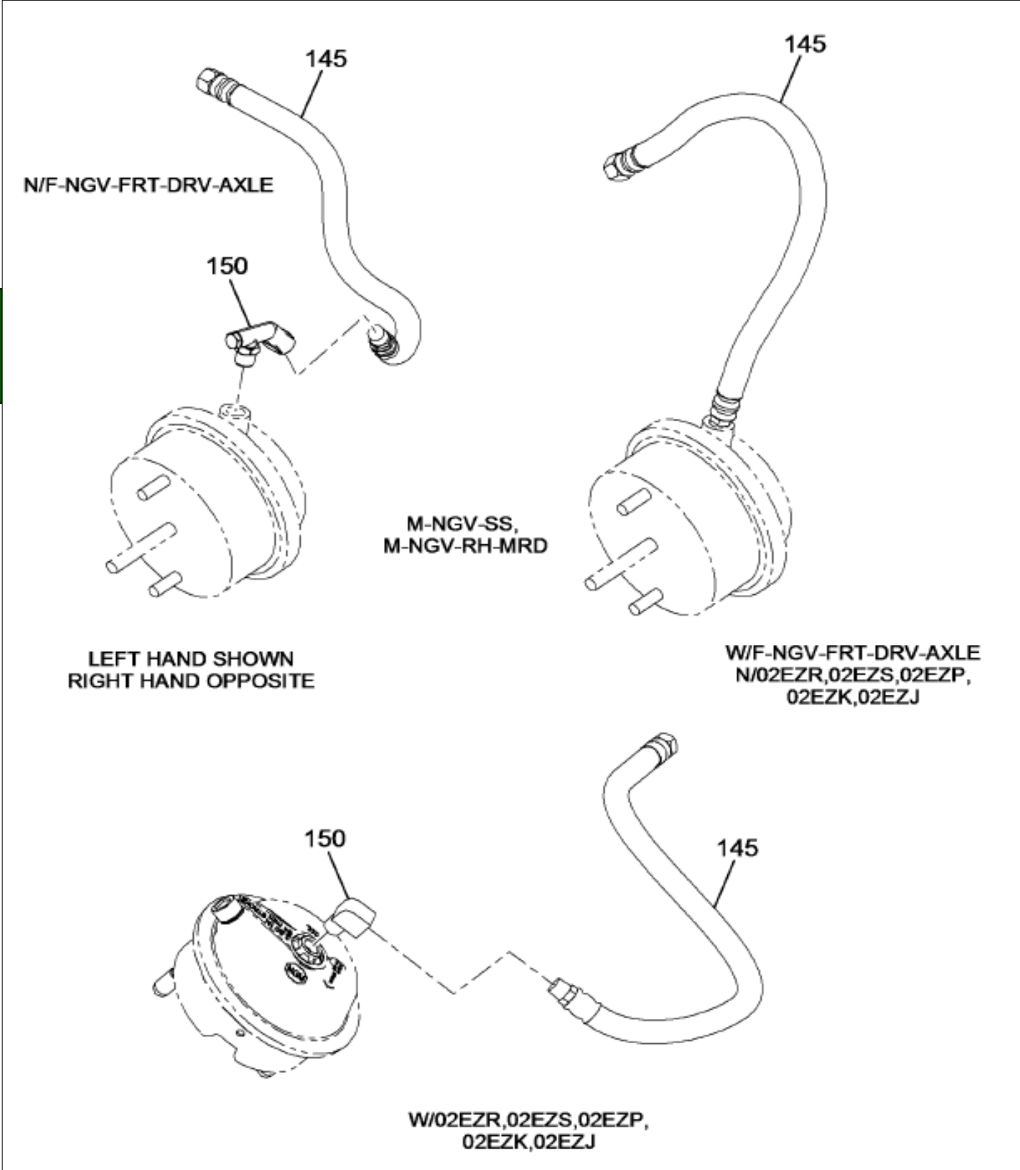
Figure 0H75K FRT AXLE HOISING
