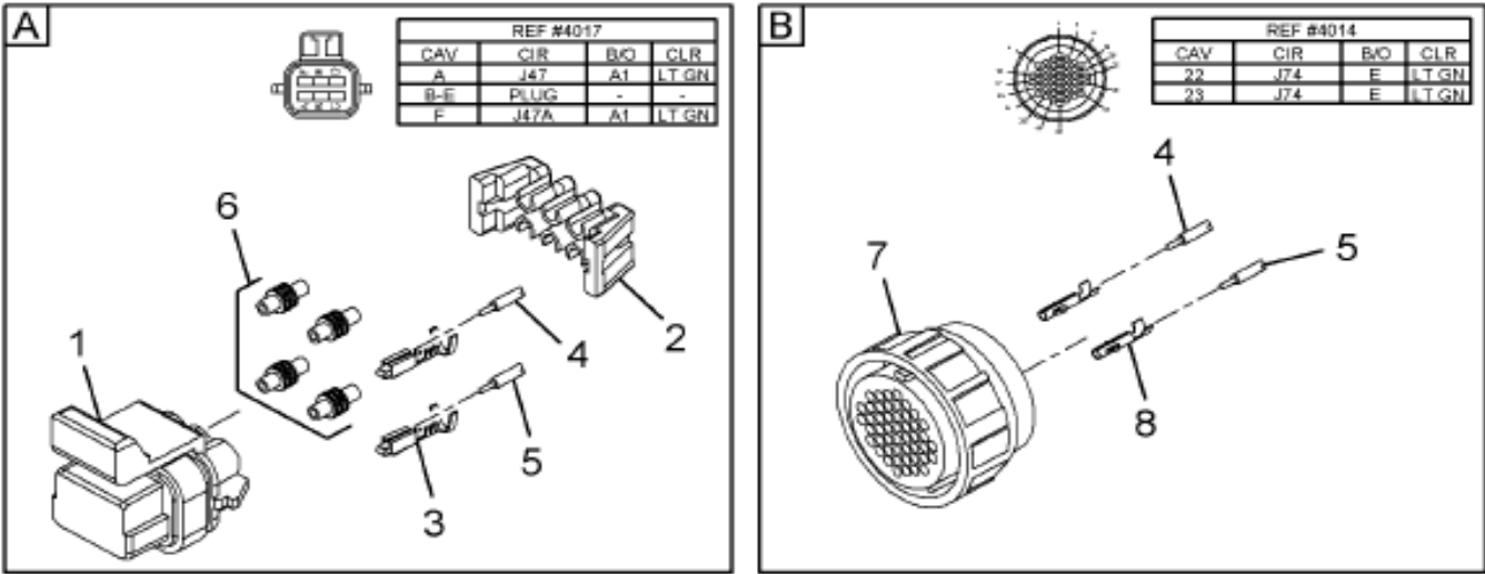
https://truckmanualshub.com/ Figure 3568458C91 HARNESS,ELEC; HEATER RECIRC
