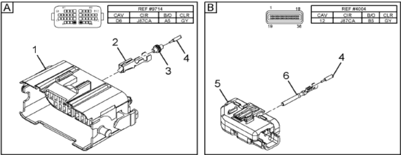
Figure 3535306C1 https://trucksmanualshub.com/ HARNESS, CHASSIS WIRING*WASHER
