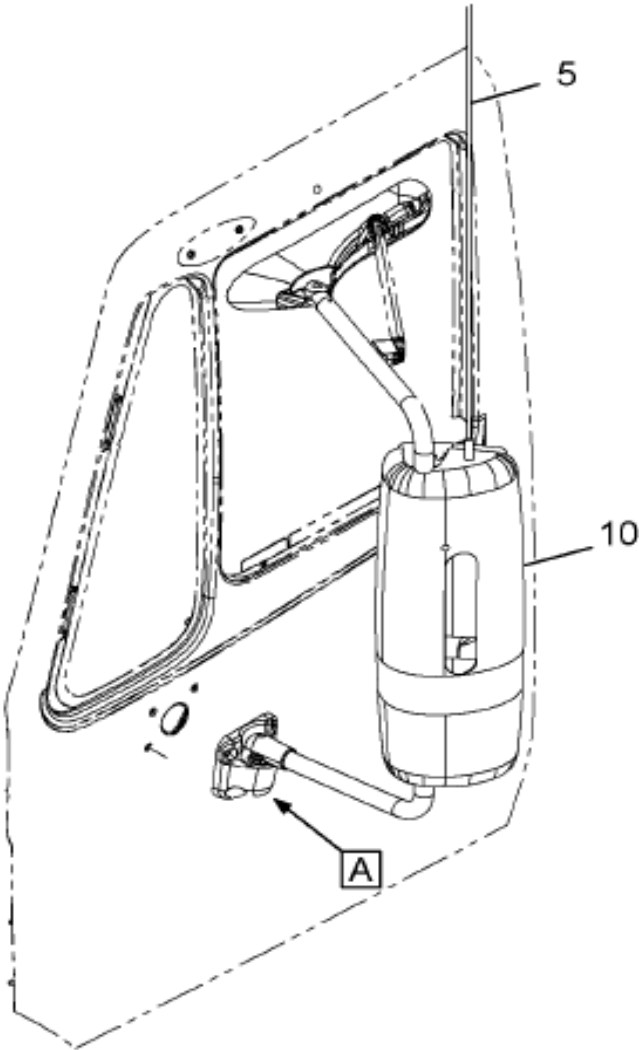
https://www.manualshub.com/ Figure 0M72R MIRROR ASM & MTG; REAR VIEW
