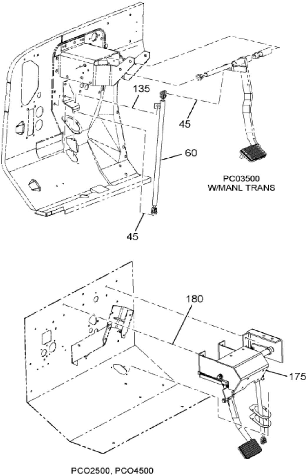
https://truckmanualshub.com/ Figure 00VKH INTMD CLUTCH CONTROLS; (LHD)
