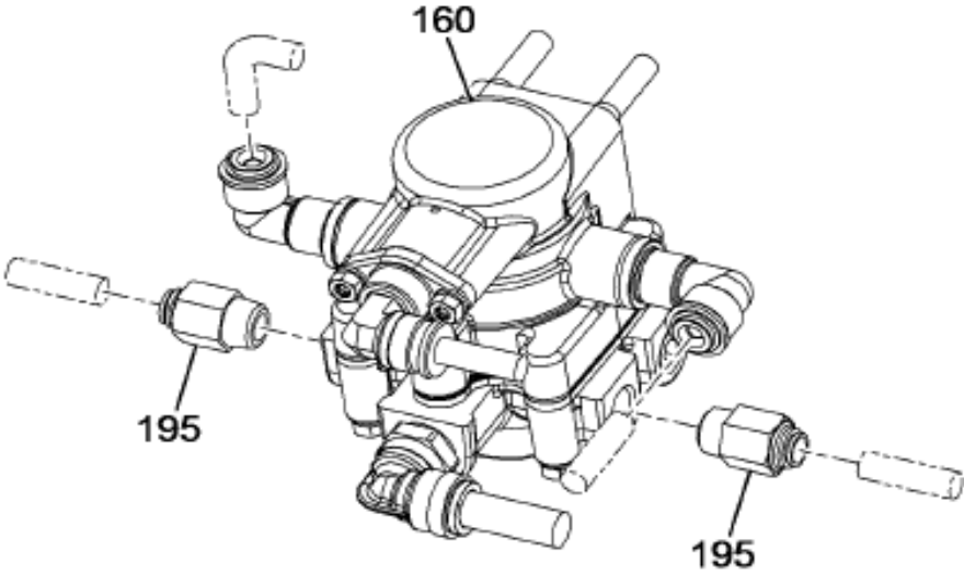
SPRING BRAKE CONTROL VALVE W/04091 W/504061
