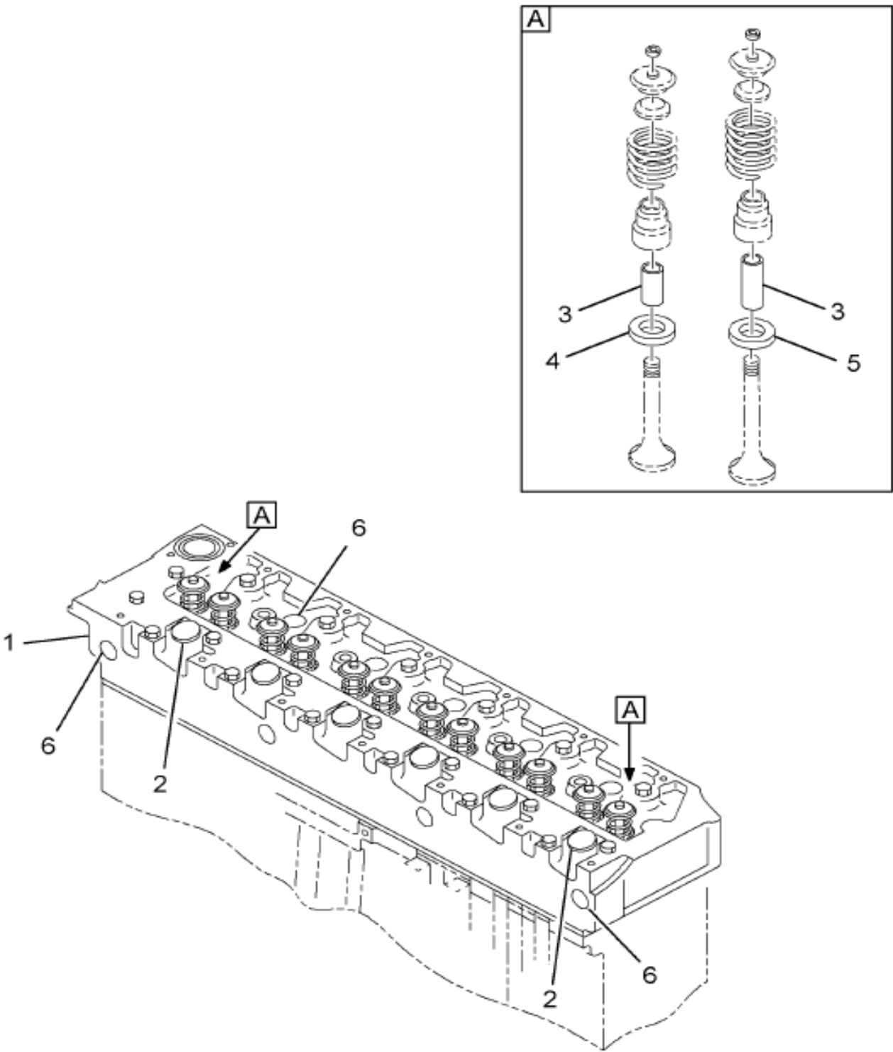
Figure 1830345C93 HEAD ASSY., CYLINDER
