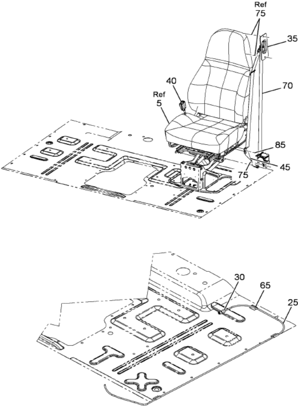
Figure 0FVYN DRIVERS SEAT INSTL; W/BELT, NATIONAL
