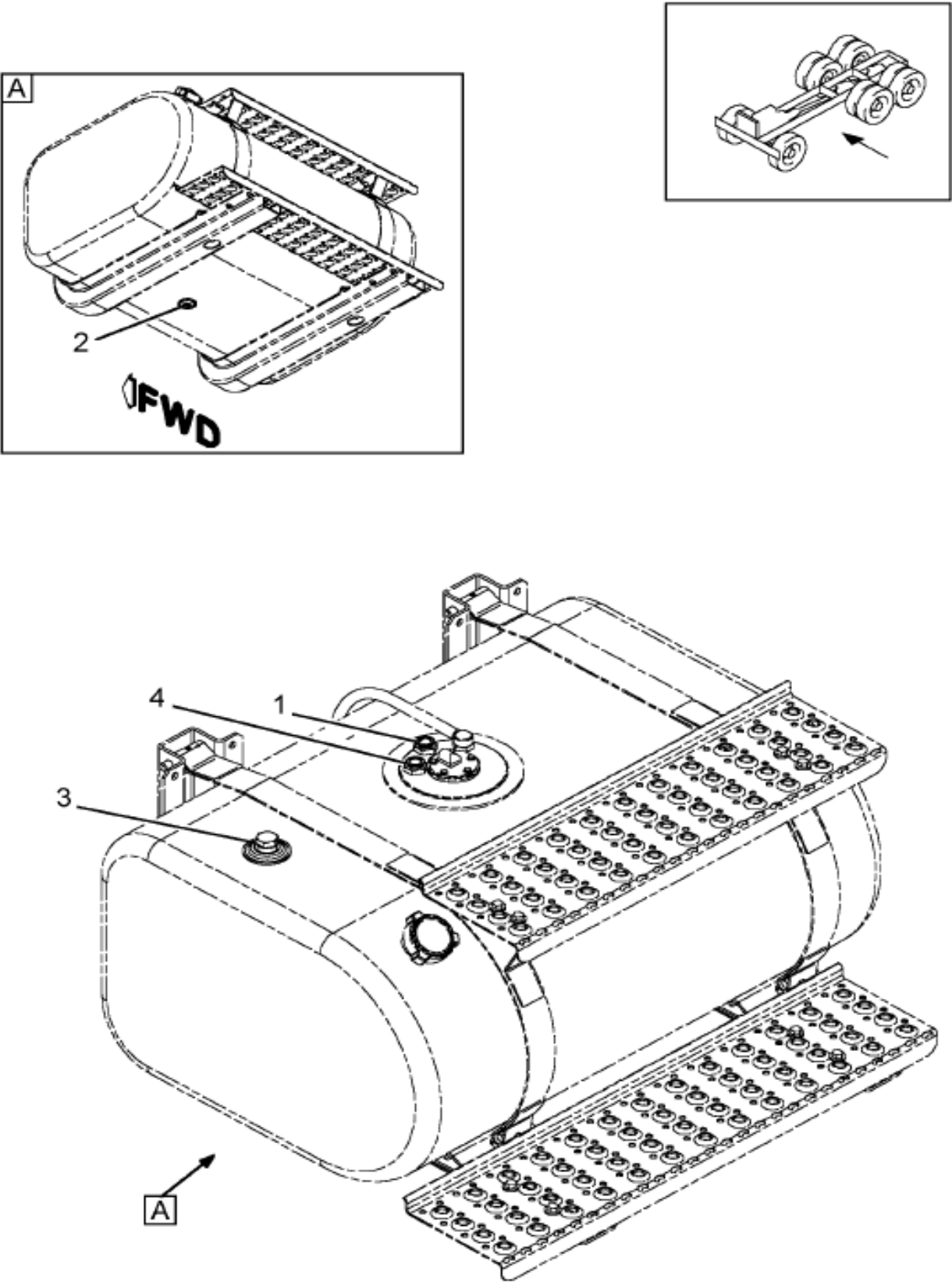
https://truckmanualshub.com/ Figure 3548119F92 TUBE, FUEL TANK INLET OR OUTLET
