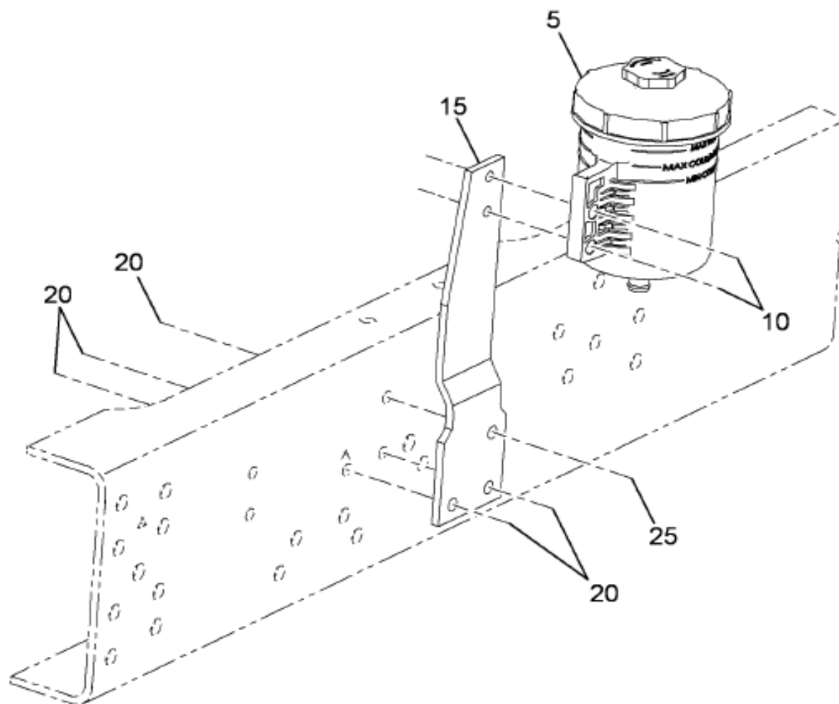
SA61500 W/0012NTP,0012NTR 1.5 QT CLEAR PLASTIC RESERVOIR
