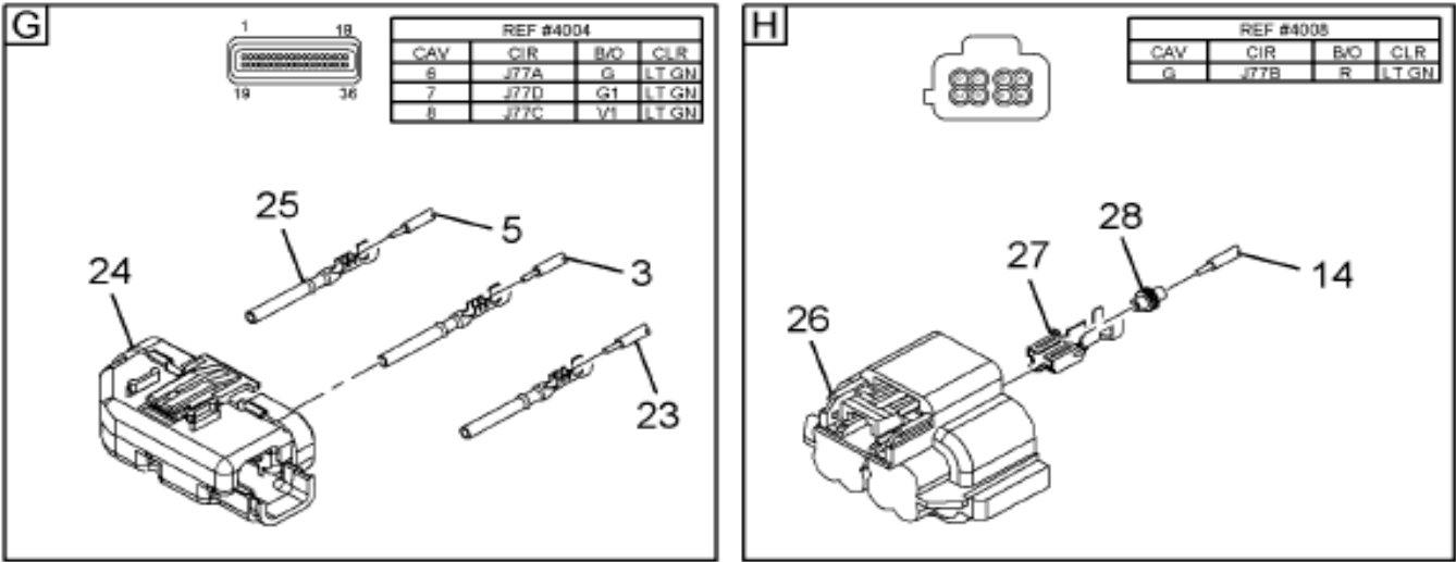
Figure 3560276C91 HARNESS, ELEC; CHAS WI
