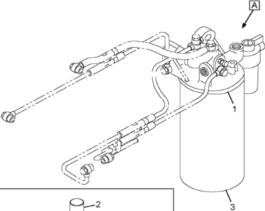
Figure 1836409C1 https://truckmanualshub.com/ HEADER ASSY, FUEL FILTER
