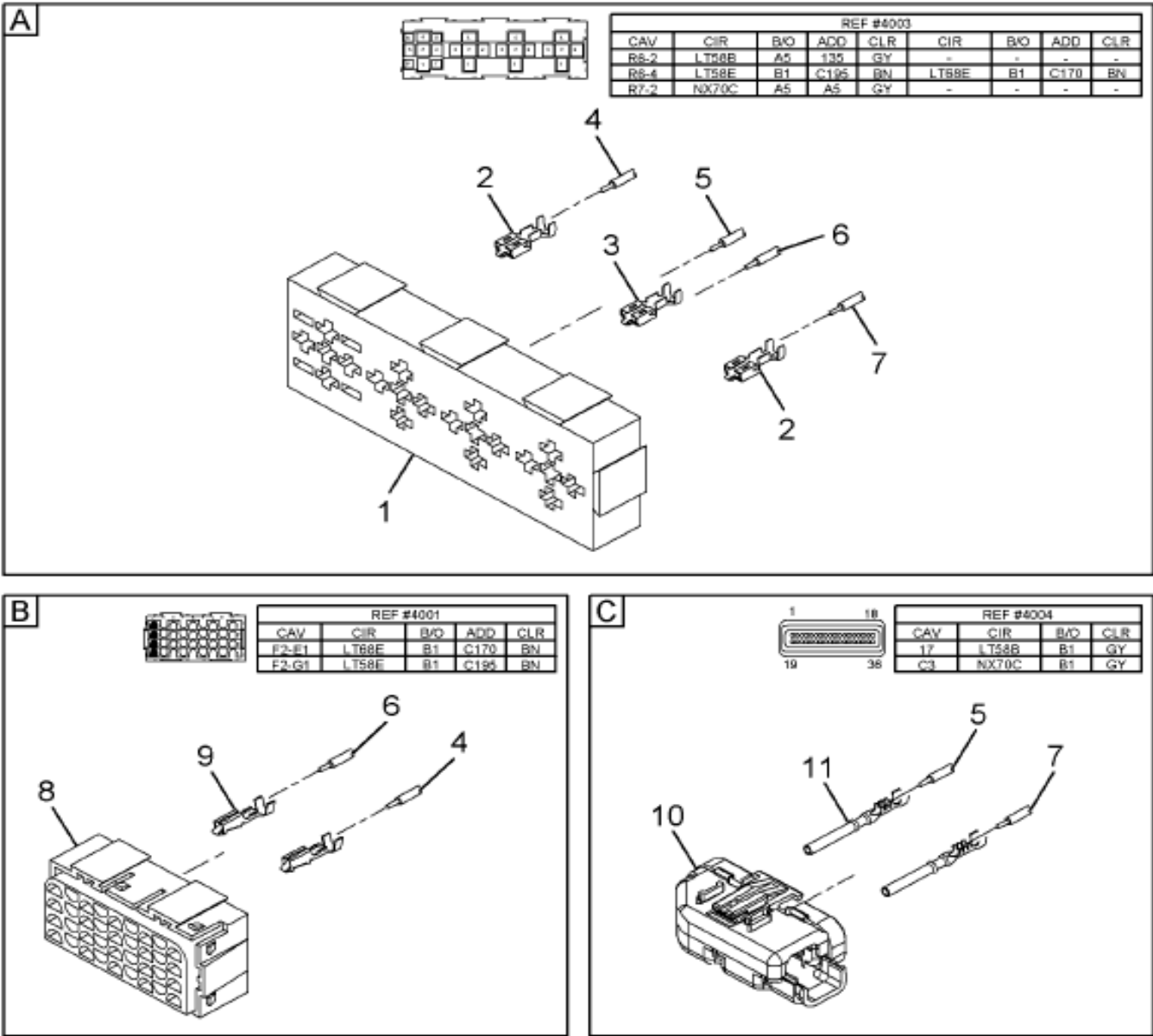
https://truckmanualshub.com/ Figure 3581900C91 HARNESS, DASH W/TRLR OR BB CONN
