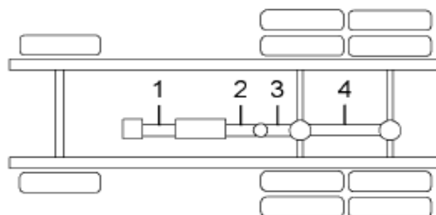
6X4, W/AUXILIARY TRANSMISSION AND ONE CENTER BEARING
