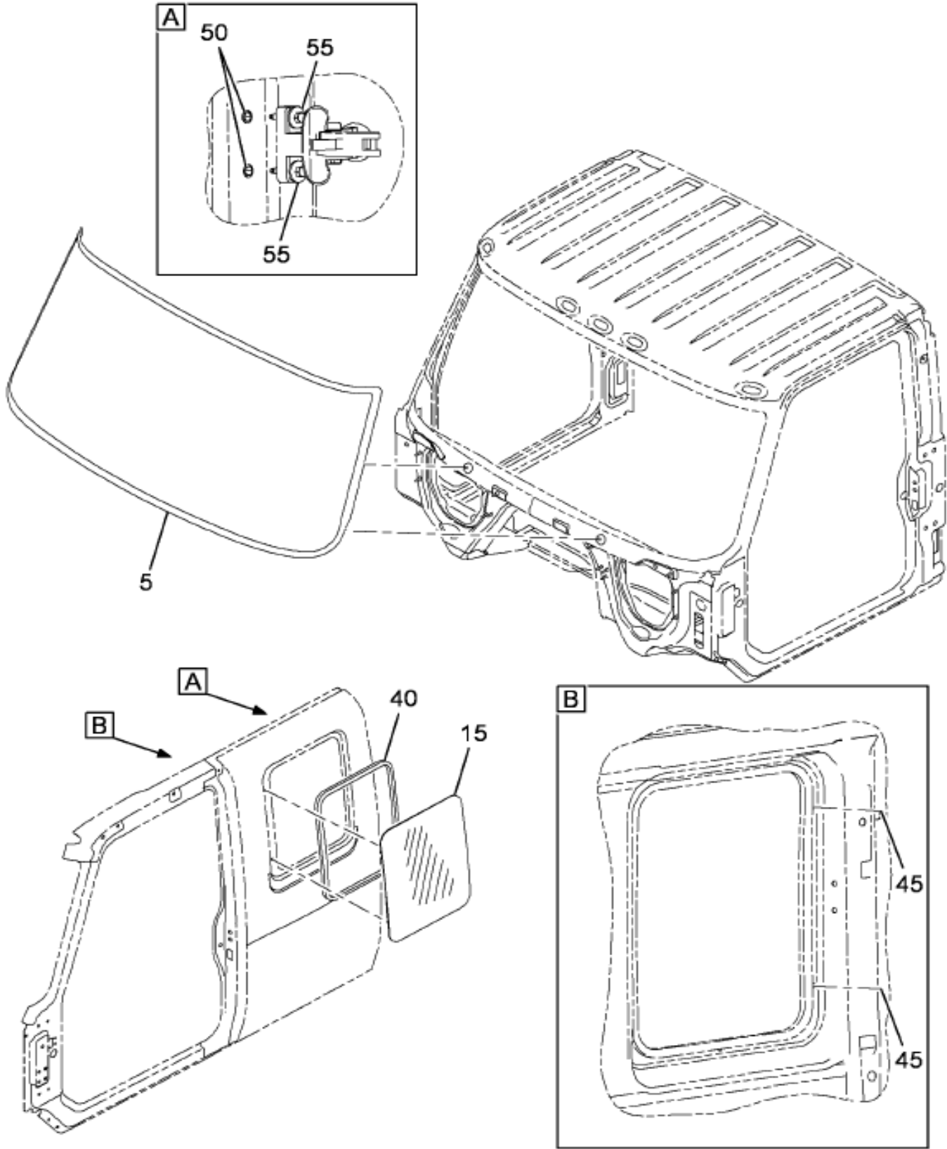
Figure 06MXXR WINDSHIELD INSTL; W/REAR SIDE QTR WINDOW
