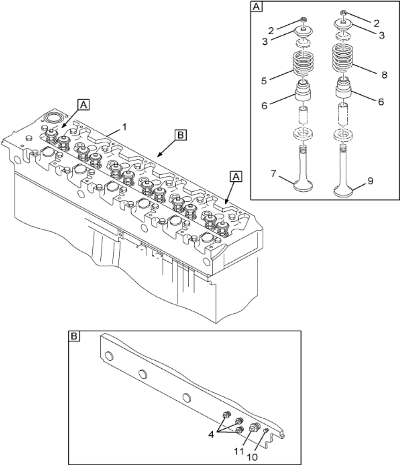
https://truckmanualshub.com/ Figure 1830345C93 HEAD ASSY, CYLINDER, W/VALVES
