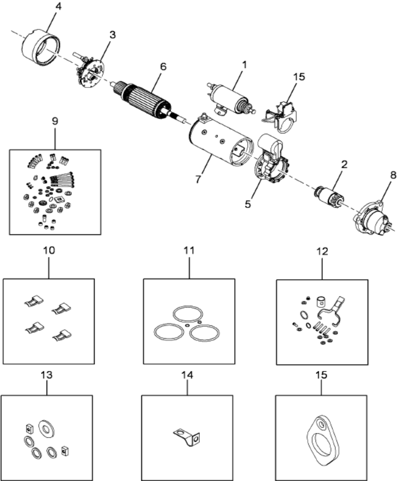
Figure 3610516C91 MOTOR, START 24V, L/N N/MAG SW
