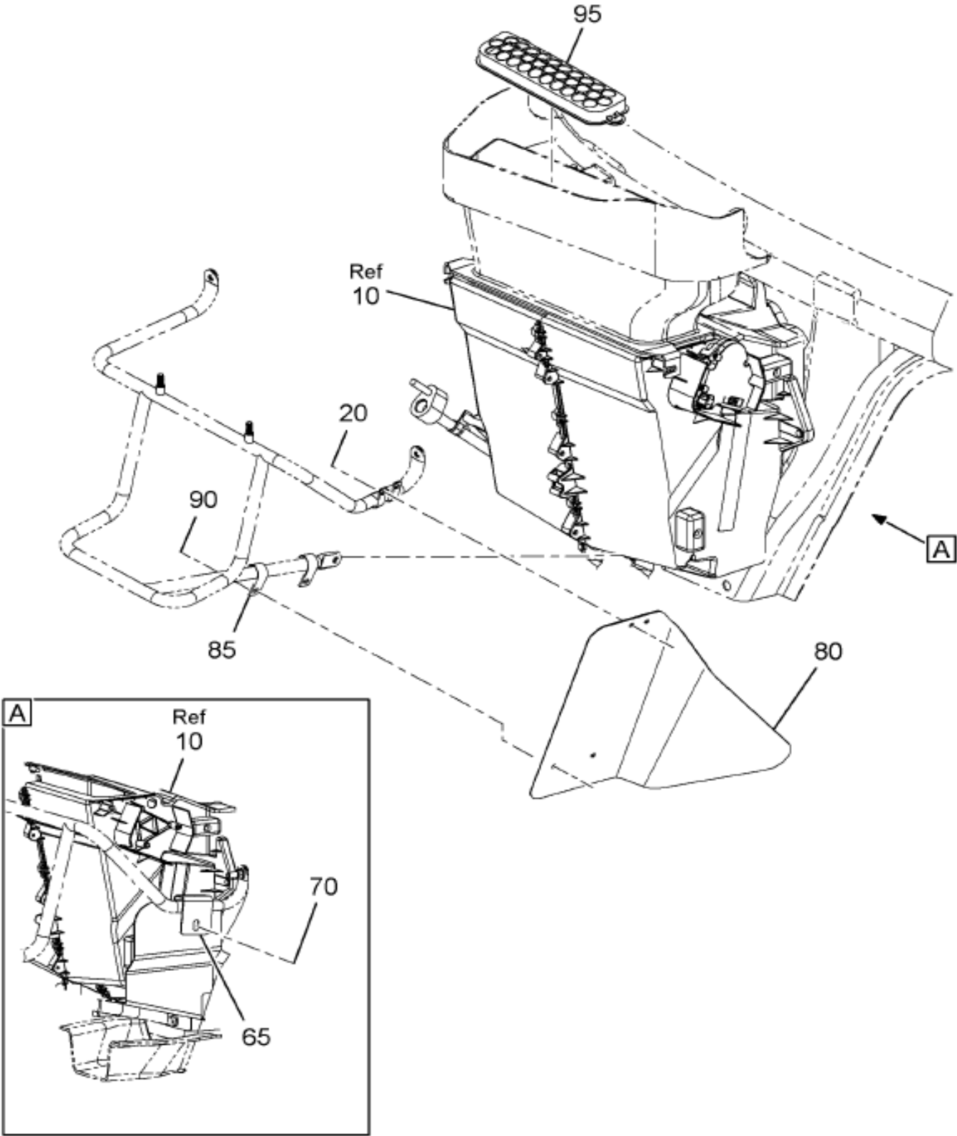
https://truckmanualshub.com/ Figure 0LV7L HTR & A/C UNIT INSTL; W/ DUCT
