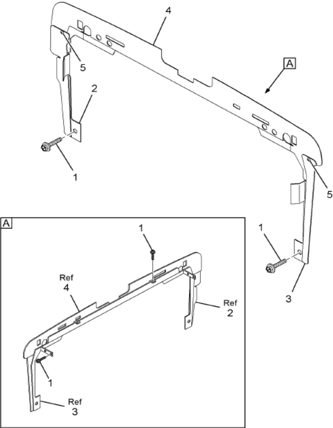
https://truckmanualshub.com/ Figure 2507472C92 SEAL, COOLING RECIRC ASSY
