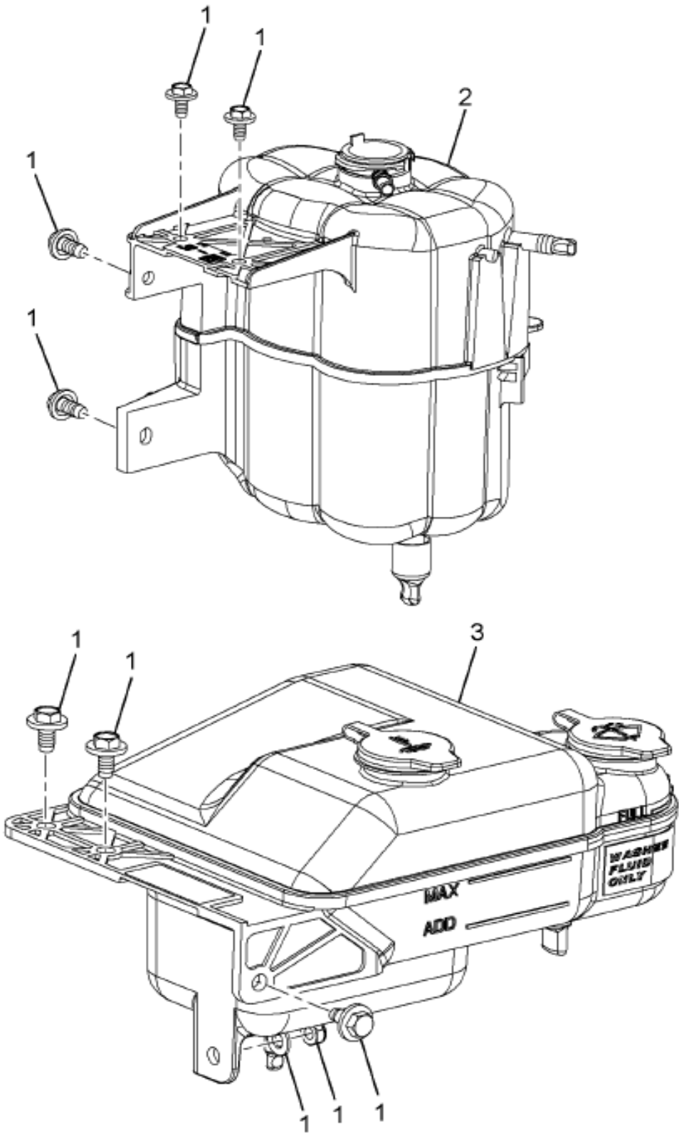
https://truckmanualshub.com/ Figure 3551079F94 TANK, RAD SURGE OR COOLANT*
