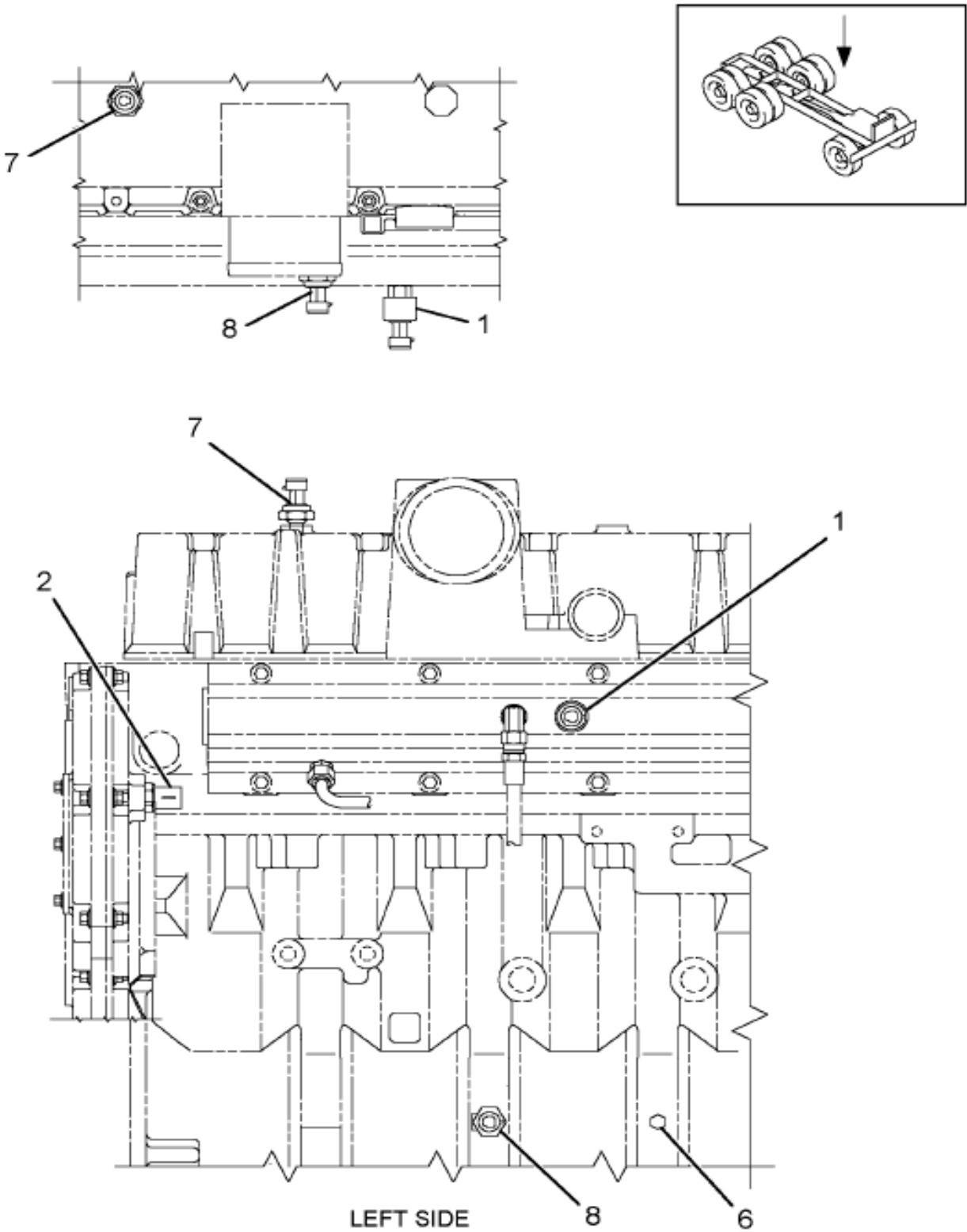
Figure 641005B005 SENSORS, ELECTRONIC NGV
