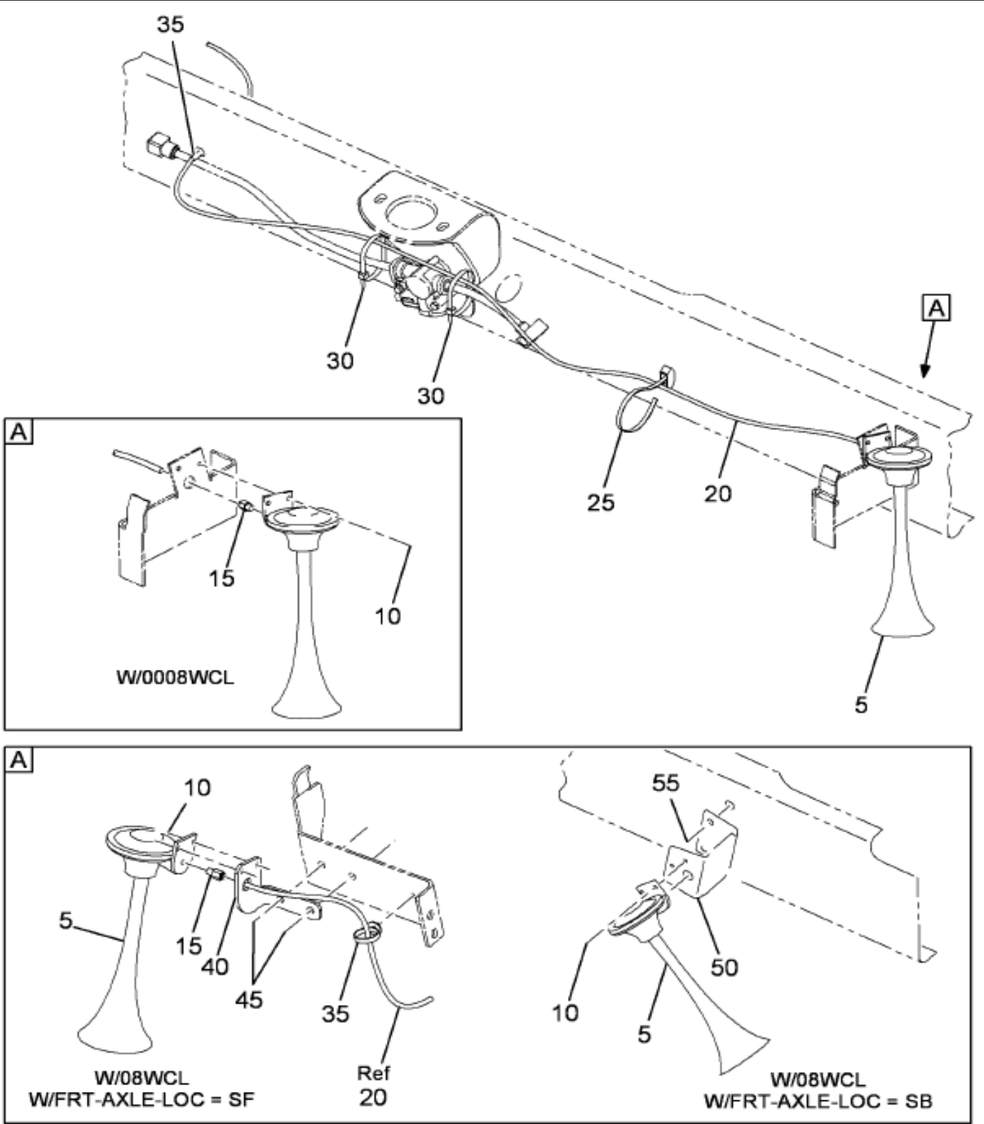
Figure 0G9F8 AIR HORN INSTL; MTD RIGHT FRAME RAIL
