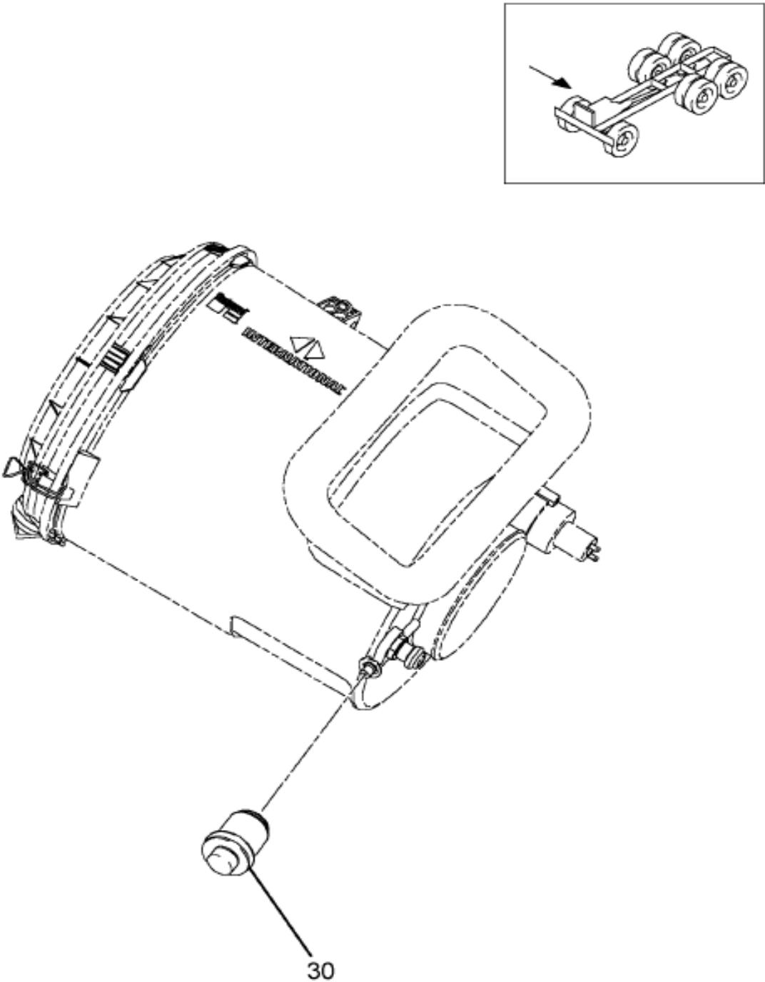
Figure 07V17 AIR RESTRICTION GAUGE INSTL
