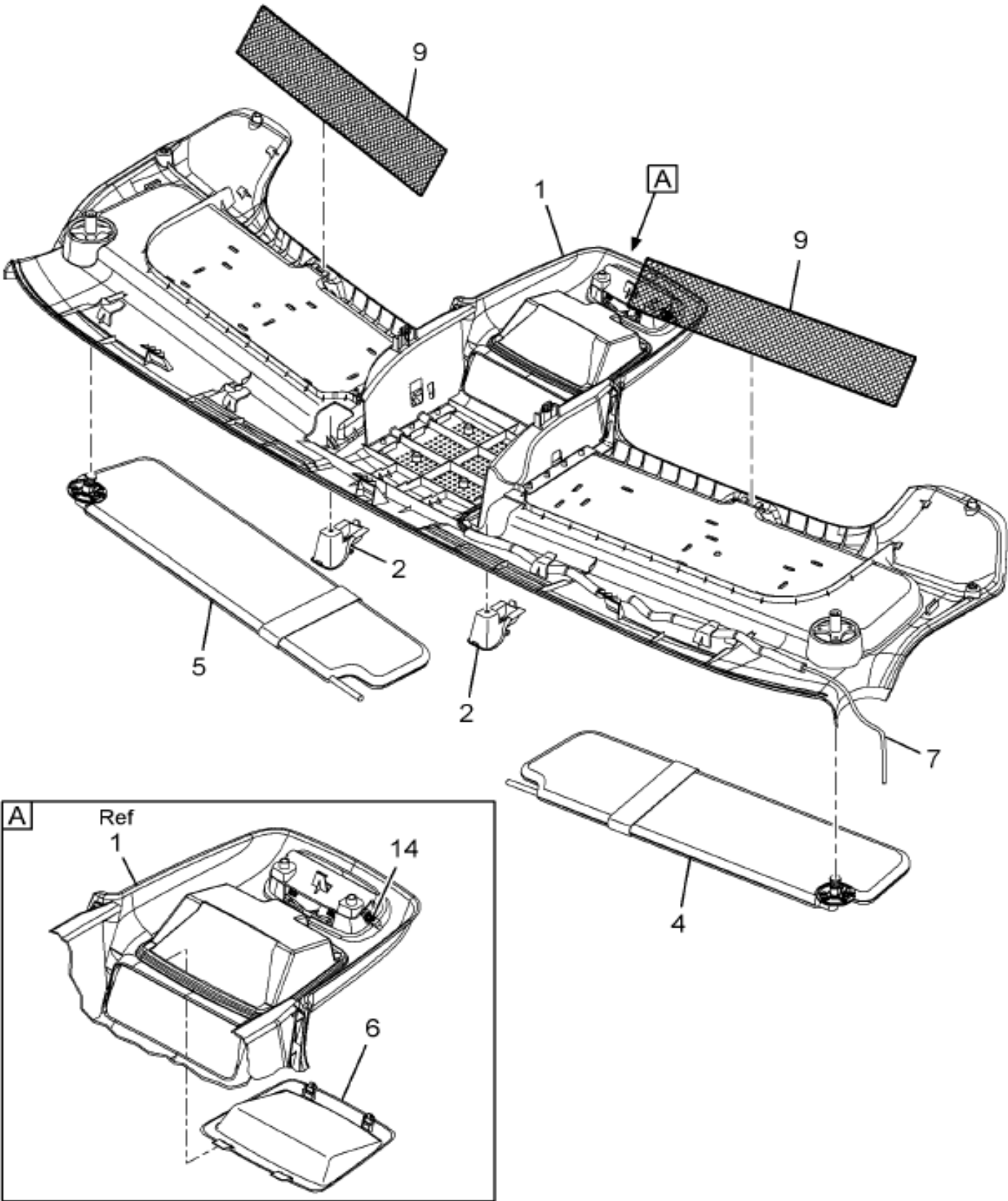
https://truckmanualshub.com/ Figure 3546500C95 PANEL, OVRHD CNSL STD
