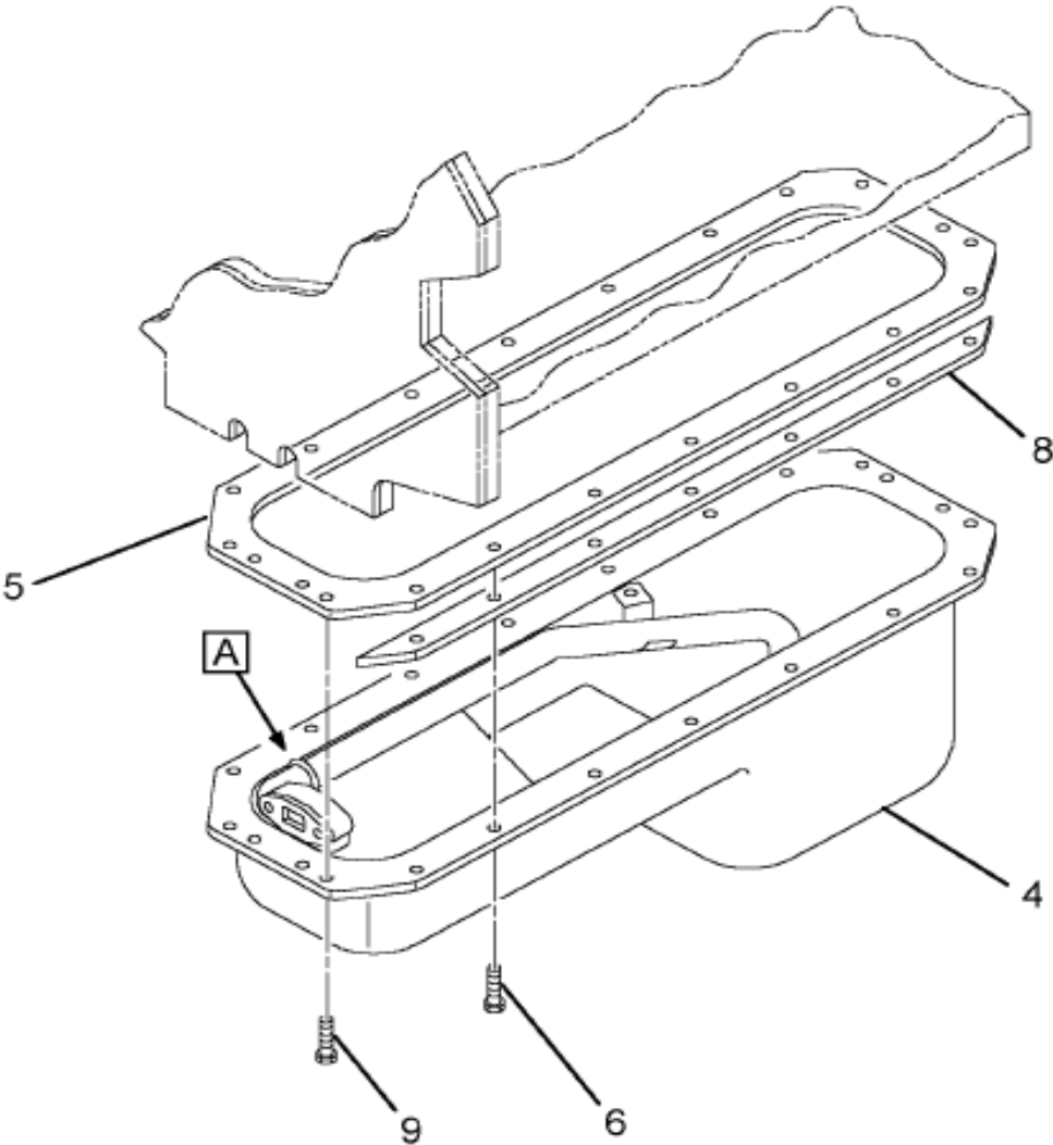
Figure 641006L001 PAN, OIL
