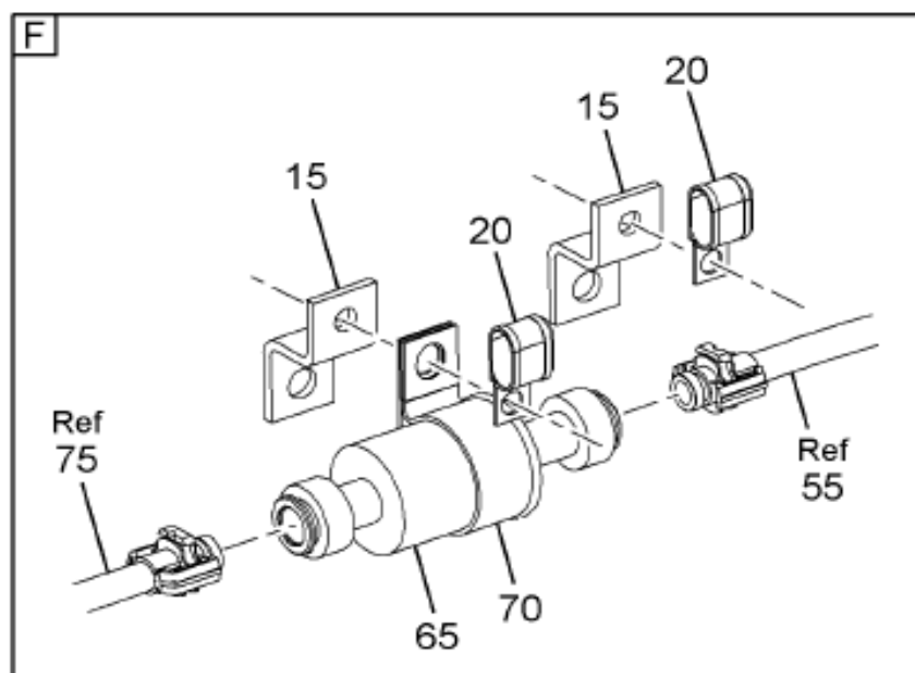
https://truckmanualshub.com/ Figure 01F3C3 FUEL HOSEING INSTL
