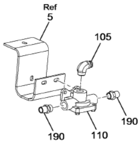
QUICK RELEASE VALVE MTG W/04091 W/12" RAILS W/01UAA
