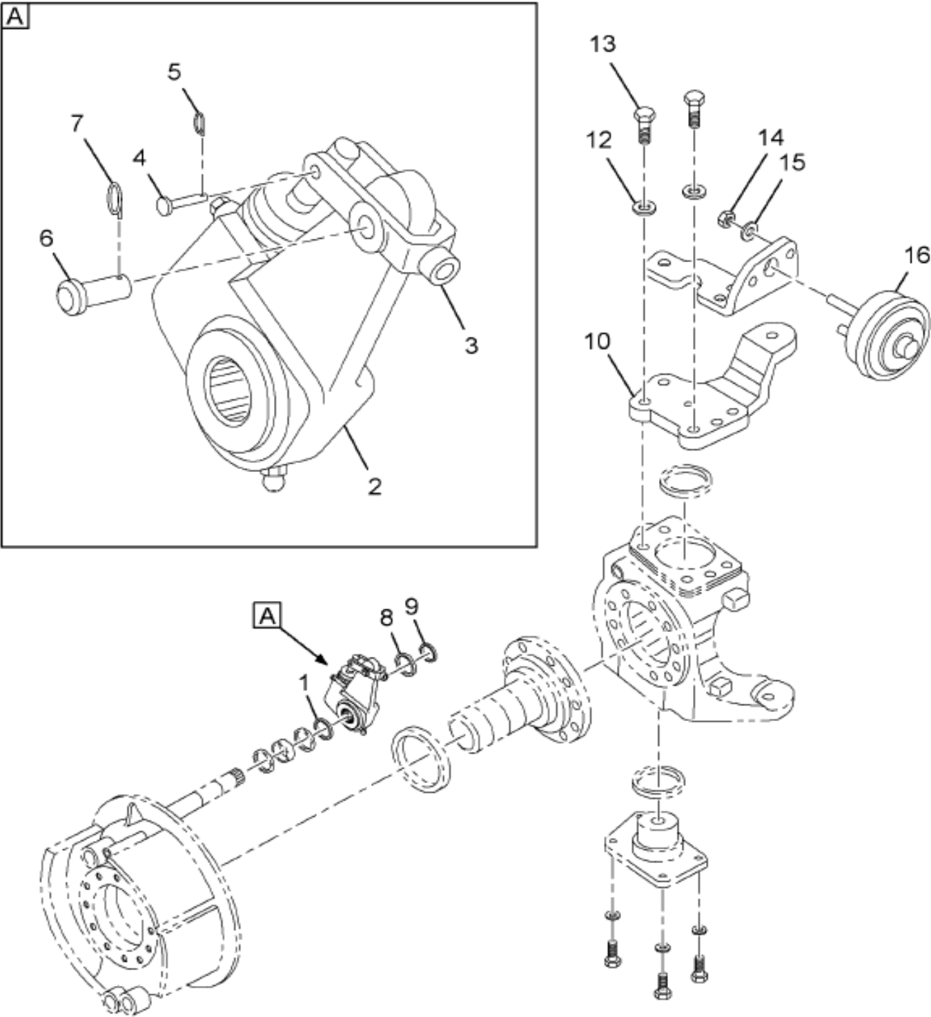
Figure 3356963P91 ADJUSTER, BRK SLACK 5.5" FC#6
