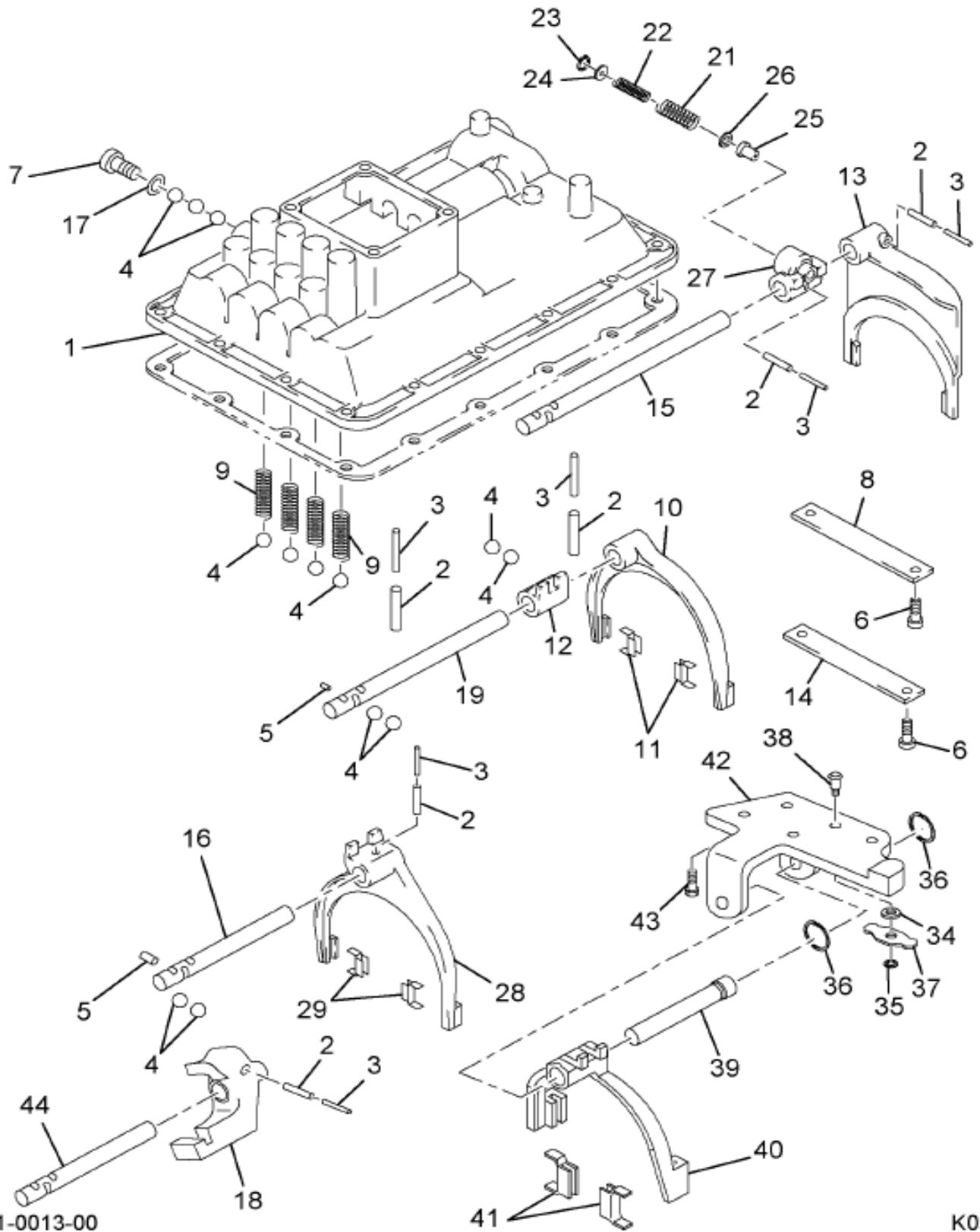
Figure 3368552F91 HOUSING, SHIFT BAR*STD SHIFT CN
