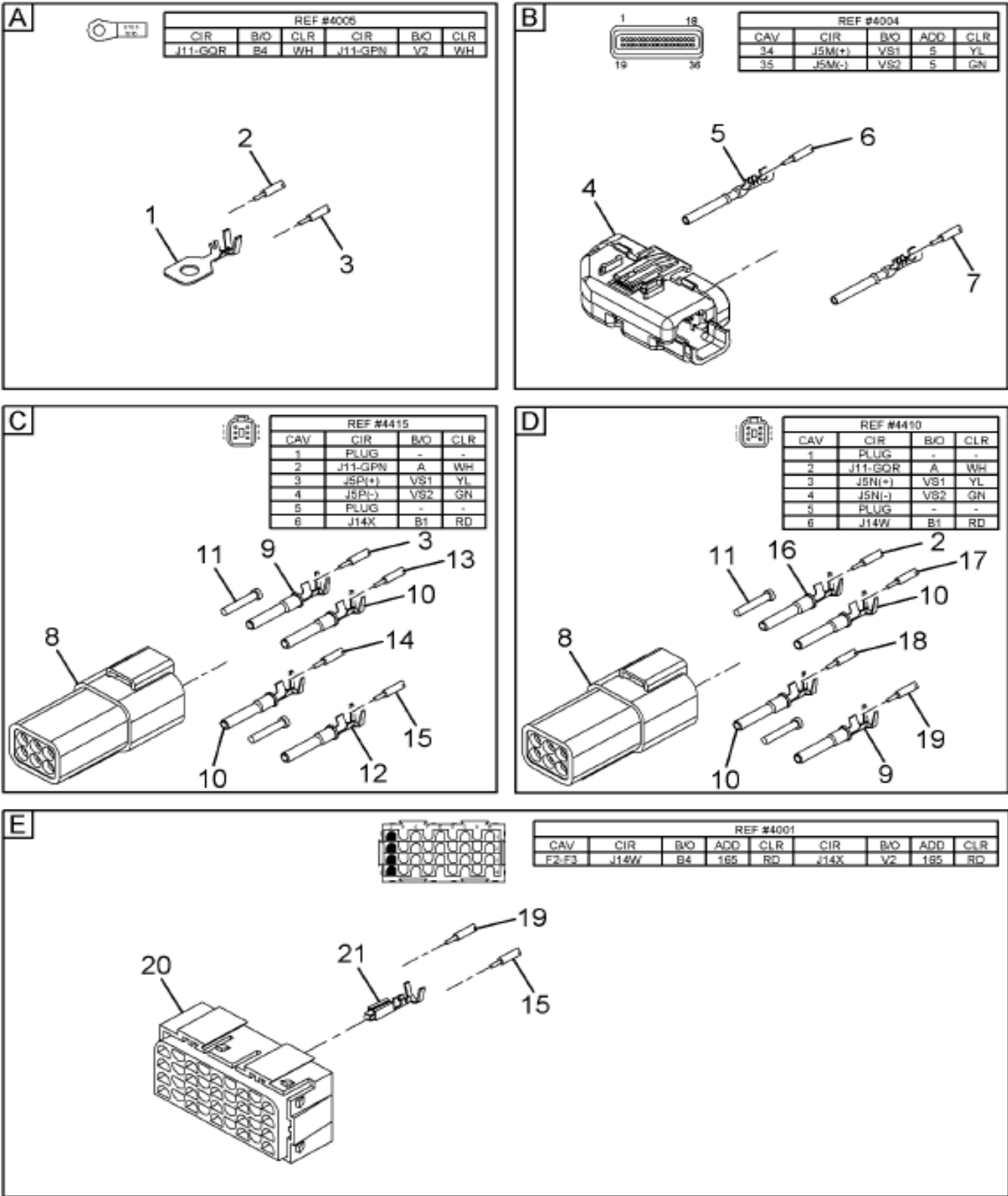
Figure 3372525C91 HARN,DASH WRG,BB DLINK,PWR&GND
