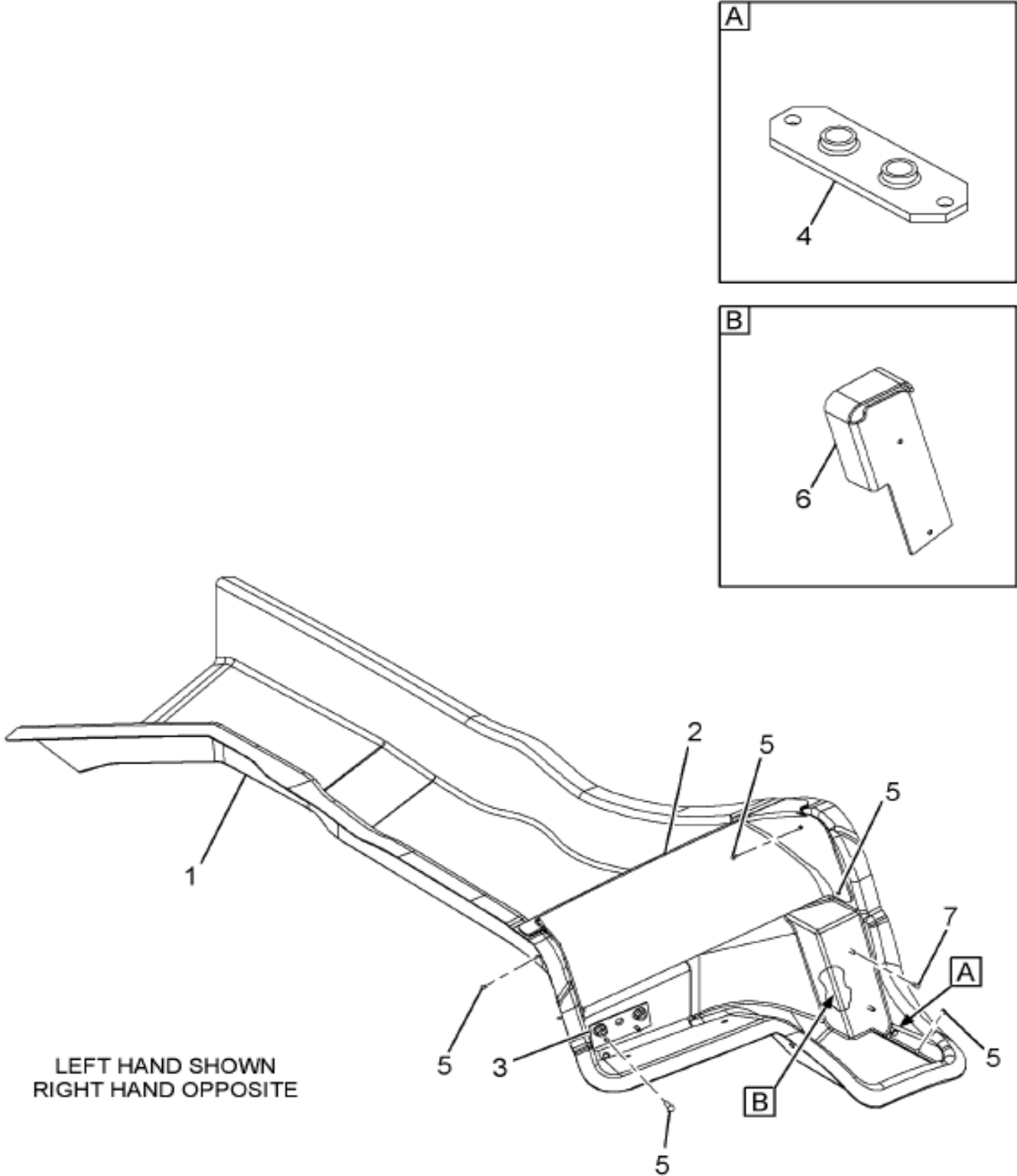
https://trucksmanualshub.com/ Figure 3552425C3 REINFORCEMENT, ASSY HOOD LH RR
