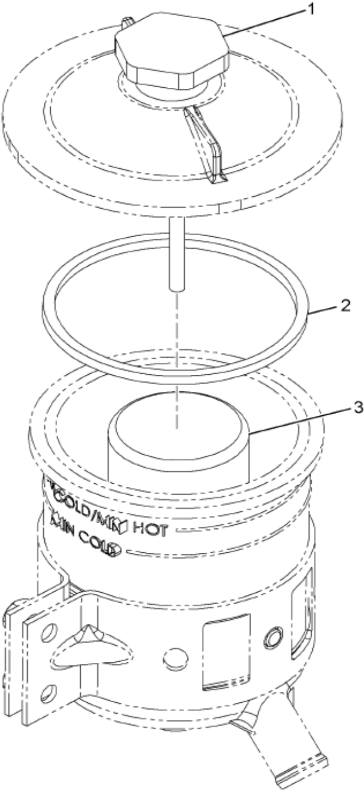
https://truckmanualshub.com/ Figure 3558153C93 RESERVOIR, POWER STRG PUMP, 1.5L
