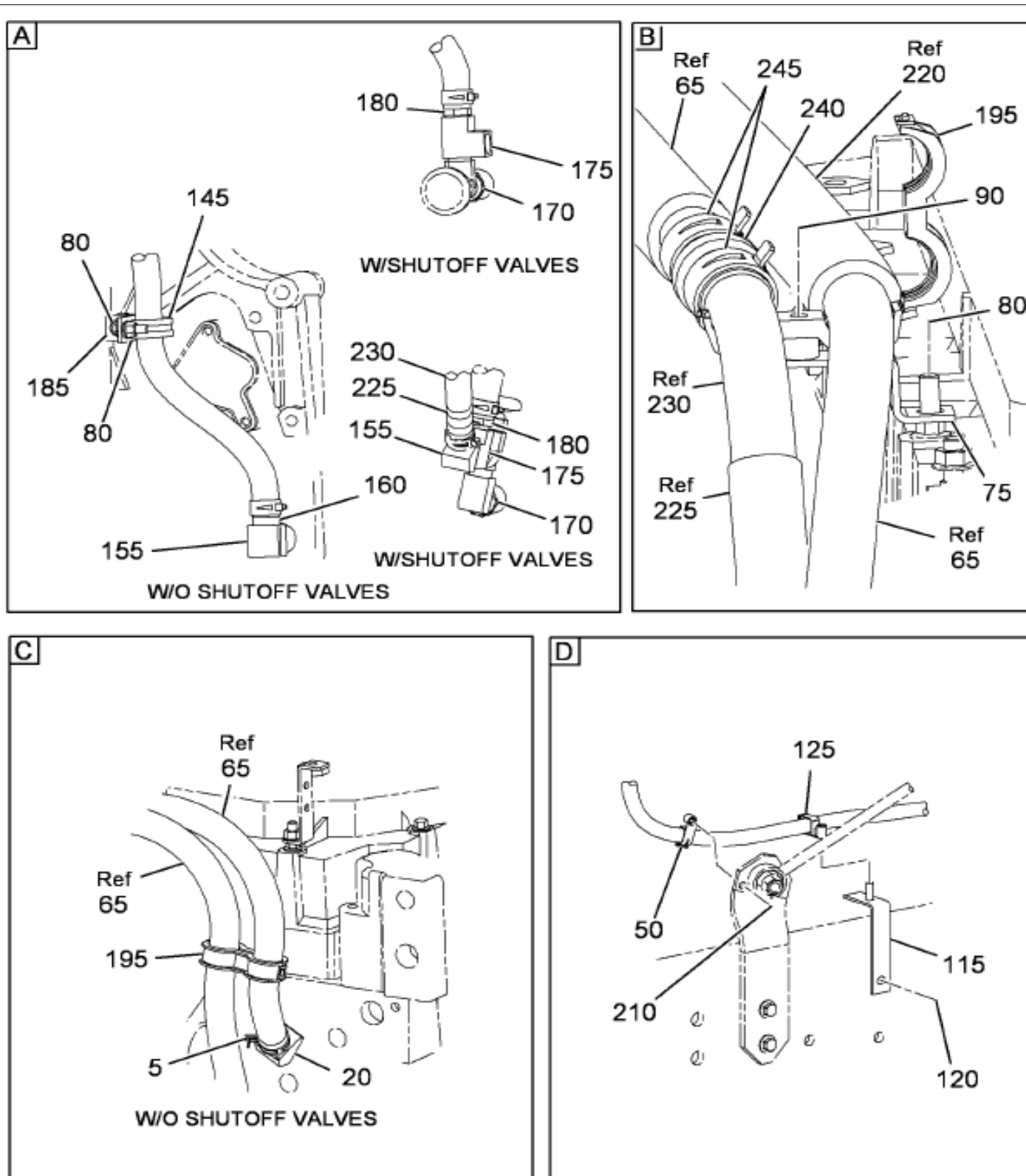
https://bookmanualshub.com/ Figure 07TDR HTR & A/C HOSE ROUTING
