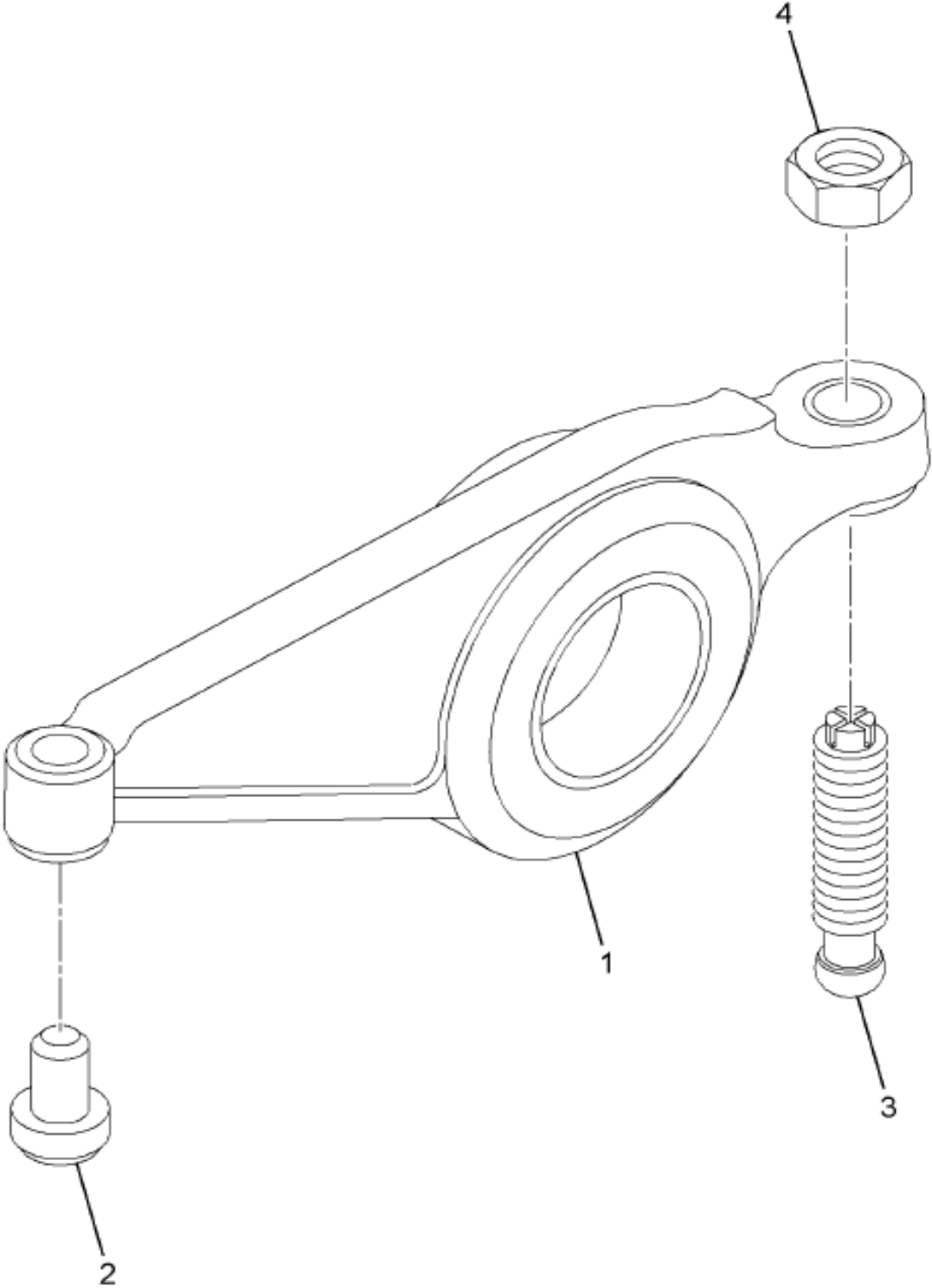
Figure 187255C91 ARM, VALVE ROCKER ASSY
