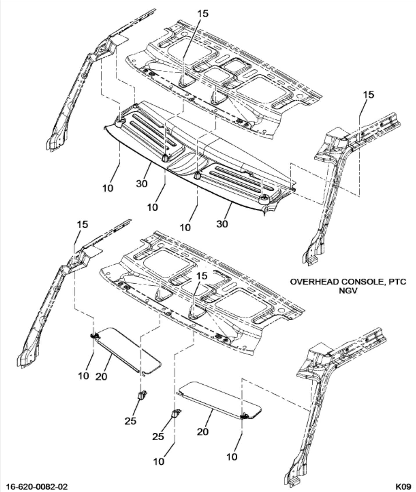
Figure 00927 HEADER PANEL INSTL; FRONT
