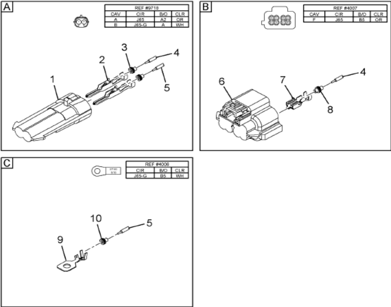
Figure 3543544C92 https://truckmanualshub.com/ HARNESS, FLOOD LIGHT WIRING*WOR
