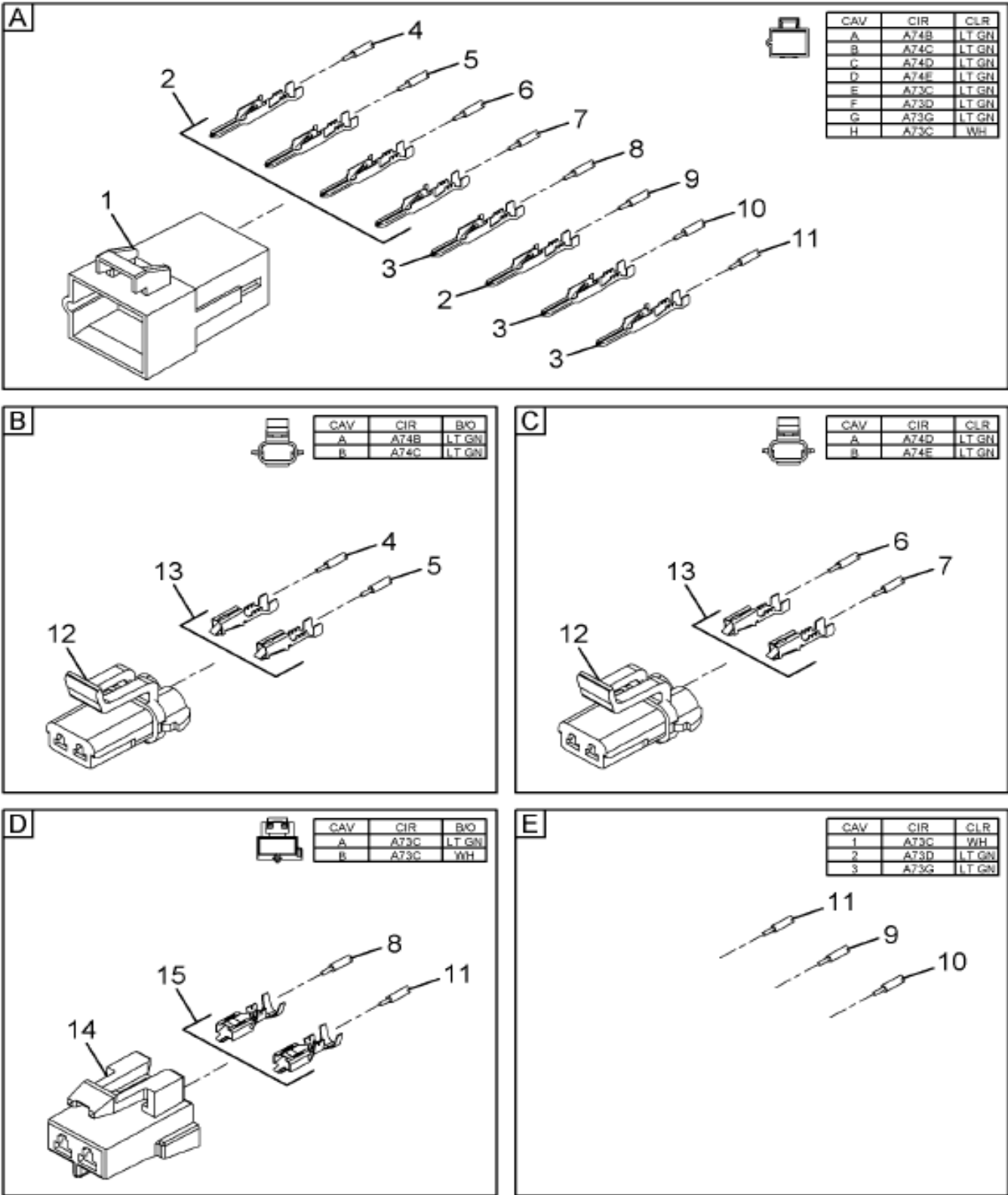
Figure 3549211C93 HARNESS, CAB/PLATFORM WIRING BA
