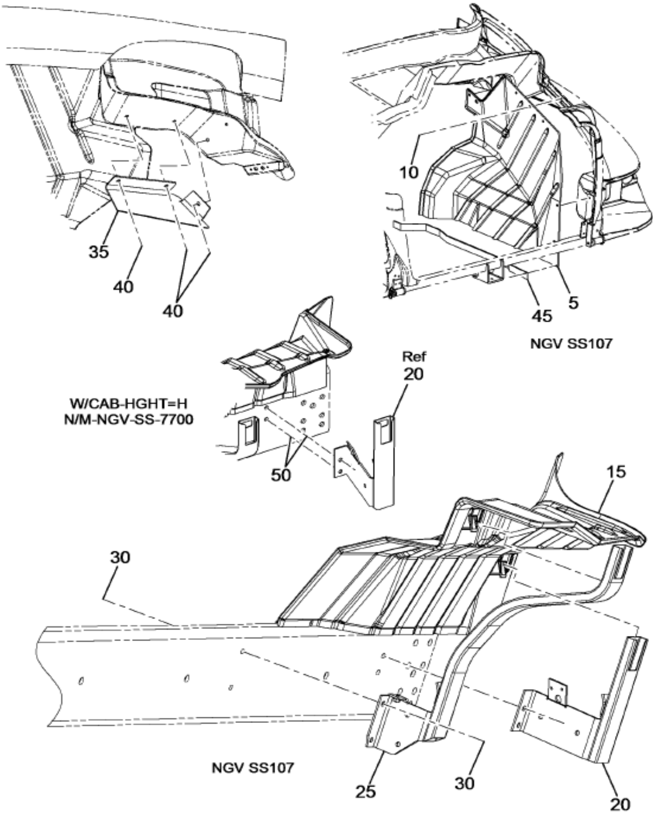
https://manualshub.com/ Figure 0DDTF SPLASH PANEL INSTL; (FRONT END)
