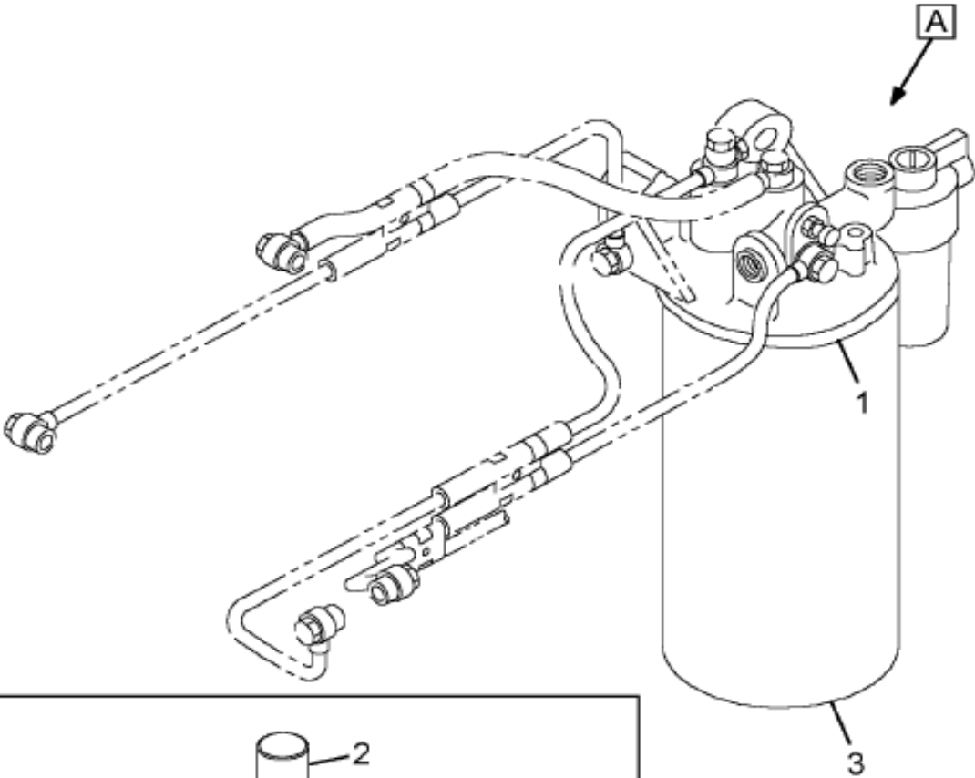
Figure 1836287C91 https://truckmanualshub.com/ HEADER ASSY, FUEL FILTER
