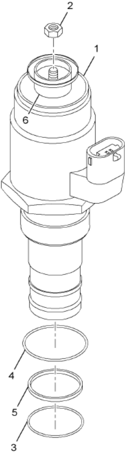
Figure 1825349C1 VALVE ASSY, IPR
