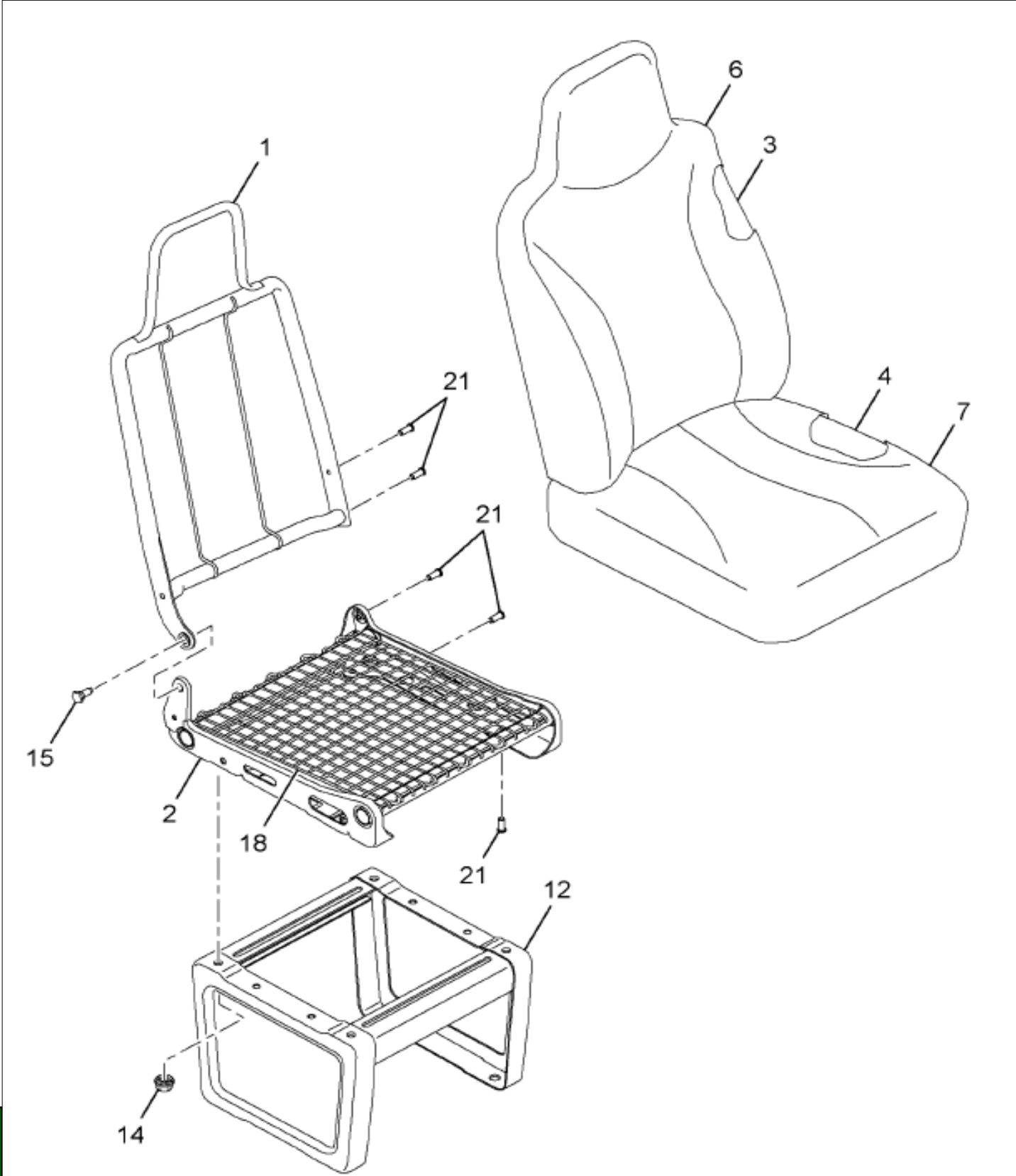
https://truckmanualshub.com/ Figure 35/9748C93 SEAT, DRS 1/3 HI BCK VINYL
