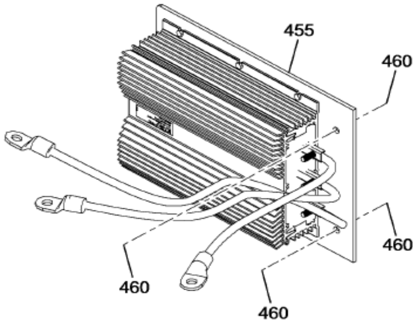
https://www.manualshub.com/ Figure 0MSPZ BATTERY EQUALIZER MODULE; 12/24V
