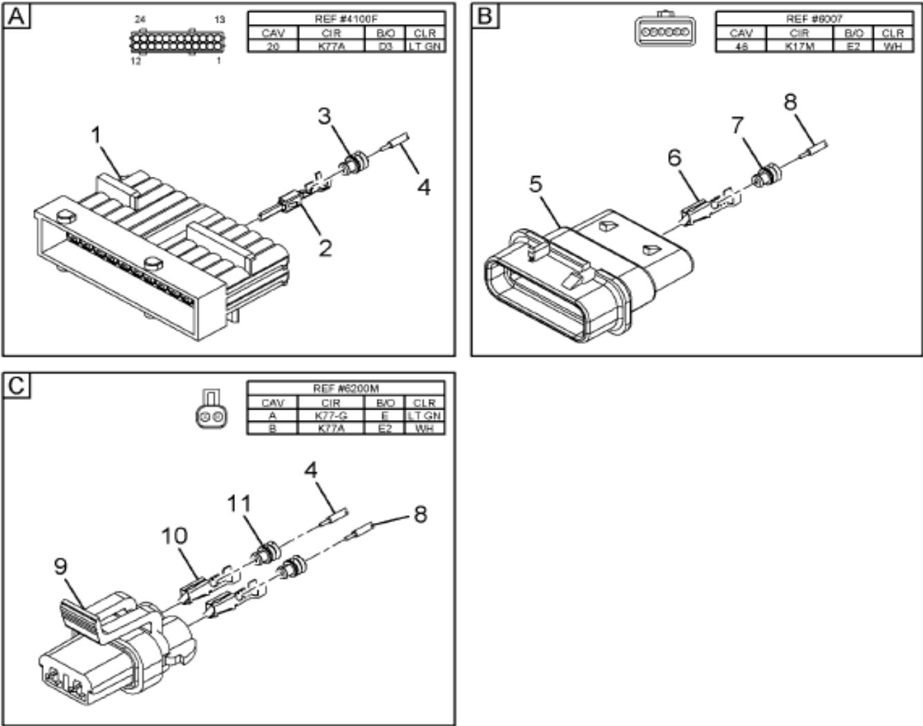
Figure 3560343C91 https://truckmanualshub.com/ HARNESS, ELEC A/C COMPR
