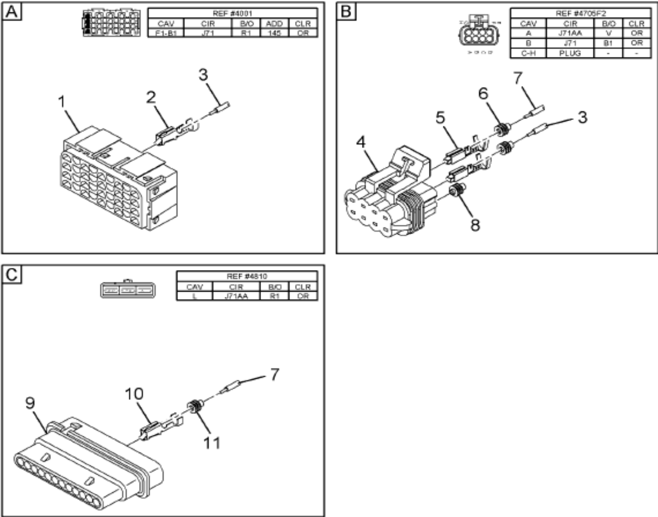
Figure 3561092C91 https://www.manualshub.com/ HARNESS, ELEC; XMSN WIRIN
