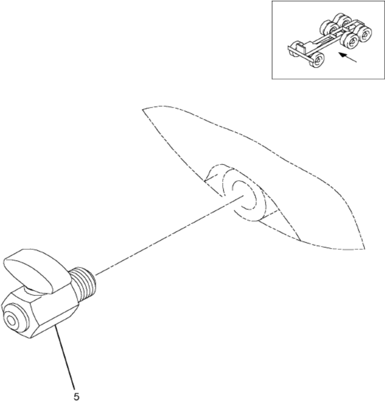
https://truckmanualshub.com/ Figure 0FLMS DRAIN VALVE; AIR TANK
