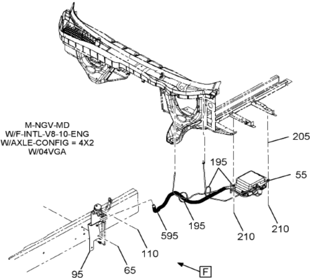
Figure 06191 WINDSHIELD WASHER INSTL
