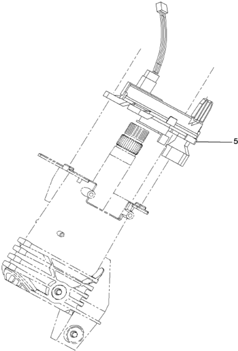
https://truckmanualshub.com/ Figure 0DC9Y DCM; CLOCK SPRING, ELECTRICAL
