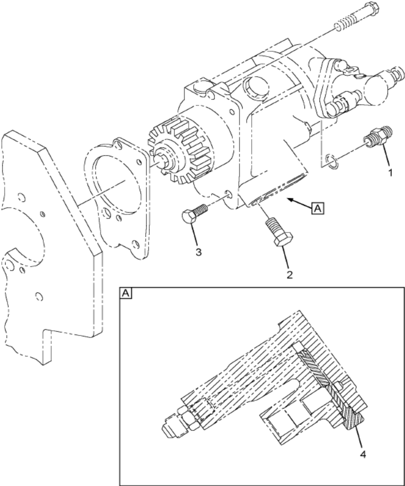
https://trucksmanualshub.com/ Figure 1830192C2 PUMP, HIGH PRESSURE OIL
