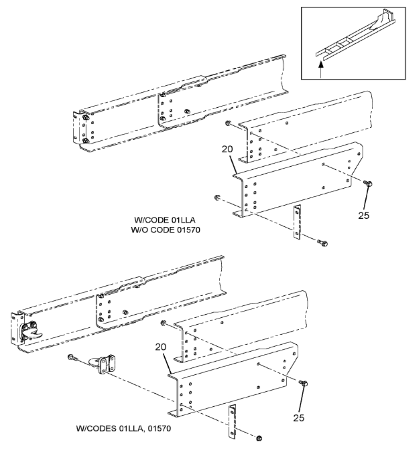
https://truckmanualshub.com/ Figure 07VHX BOLT-ON FRAME EXTENSION; W/XMBR
