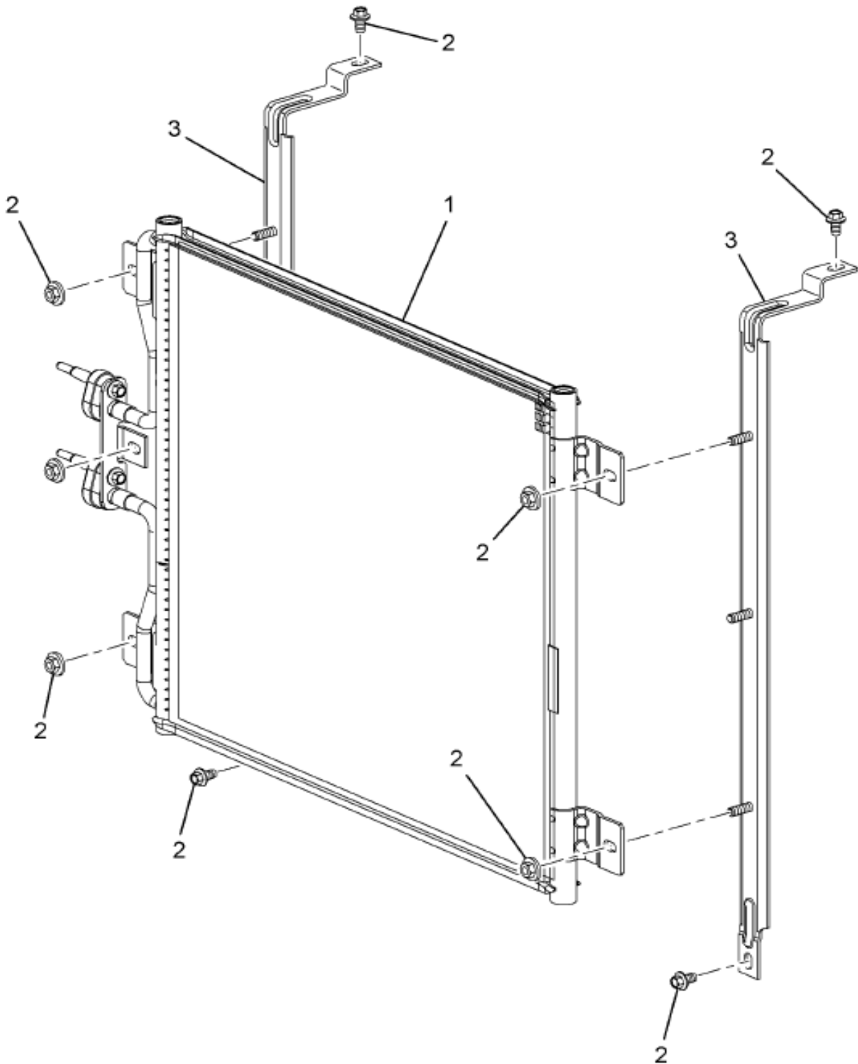
https://truckmanualshub.com/ Figure 3551081F92 CONDENSER,AIR COND PF CONDENSO
