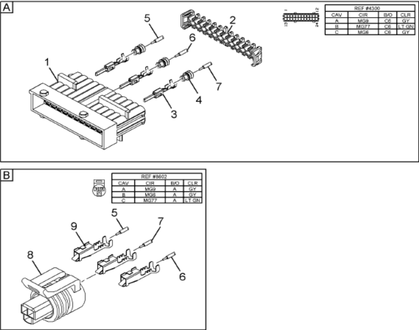
Figure 3372242F91 MODULE, A/C PRESS TRANSDUCER
