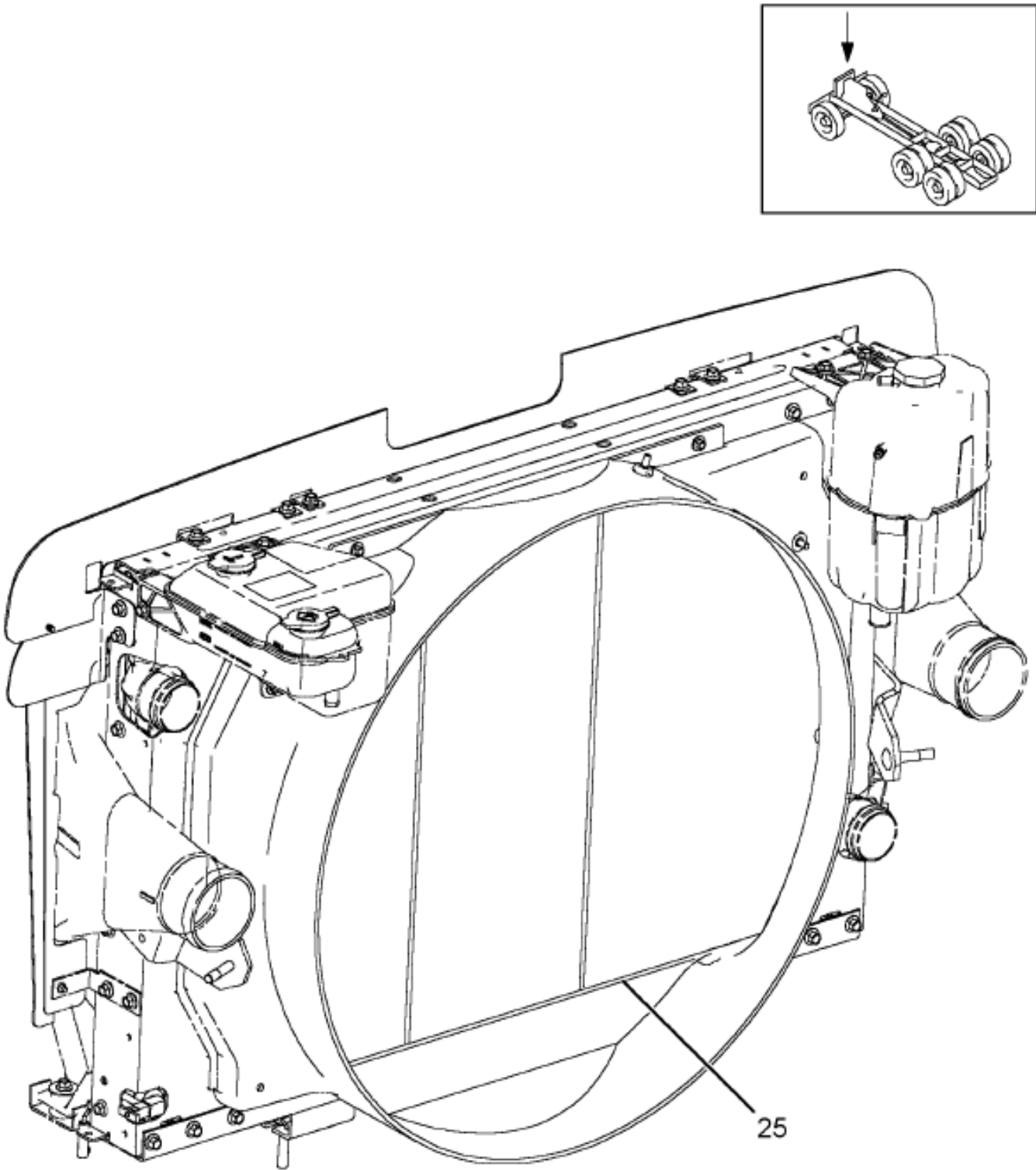
https://truckmanualshub.com/ Figure 0K2VF COOLING PACKAGE, A/C CONDENSER
