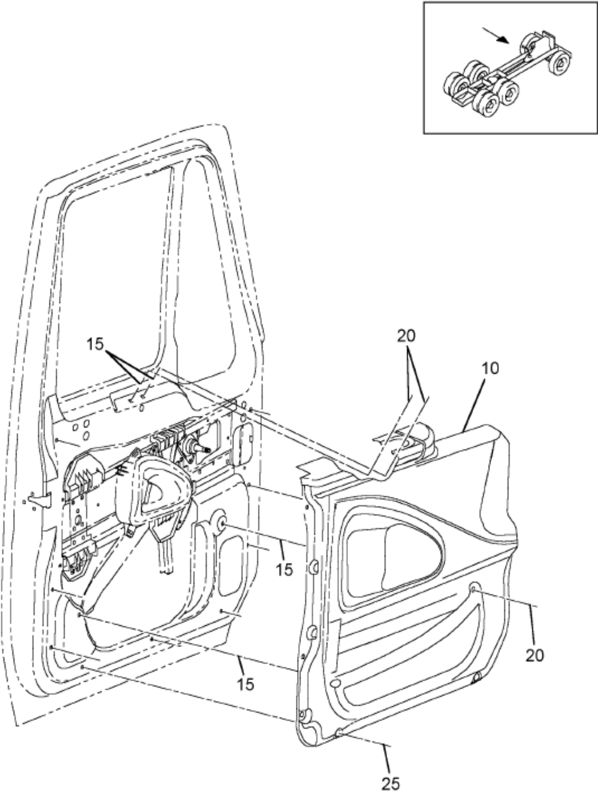
Figure 06QG0 PANEL, DOOR TRIM RIGHT
