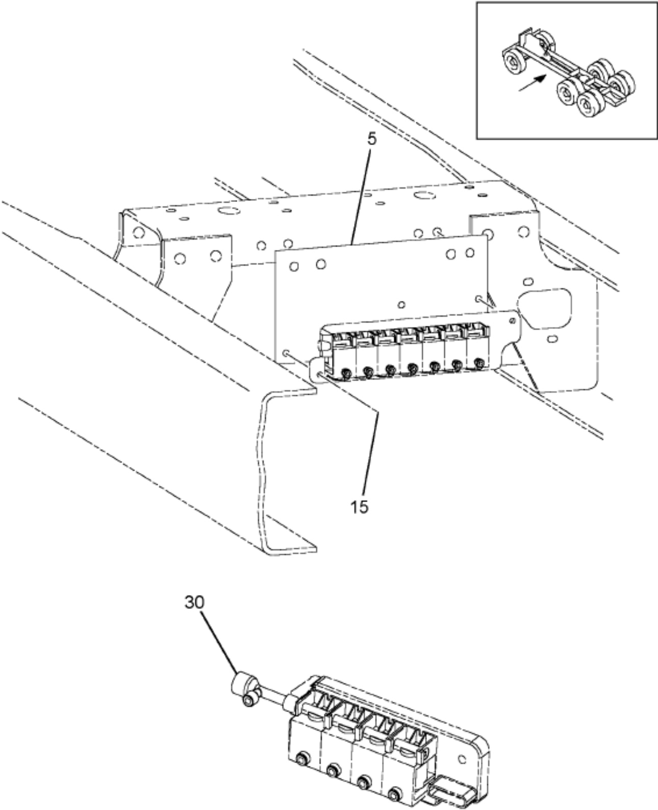
Figure 0CBKD BRACKET MTG; SOLENOID PACK
