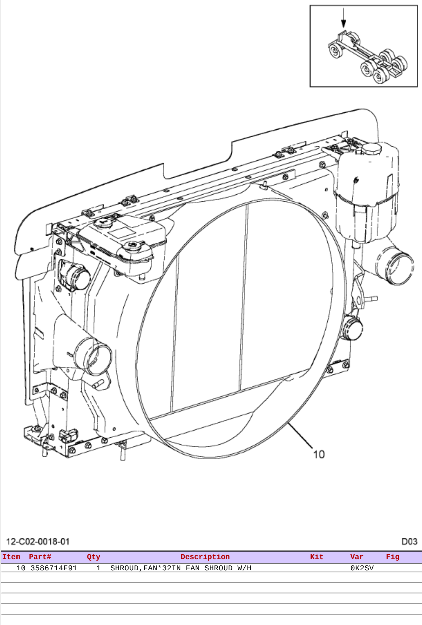
Figure 0K2RQ FAN SHROUD INSTL; COOLING PACKAGE
