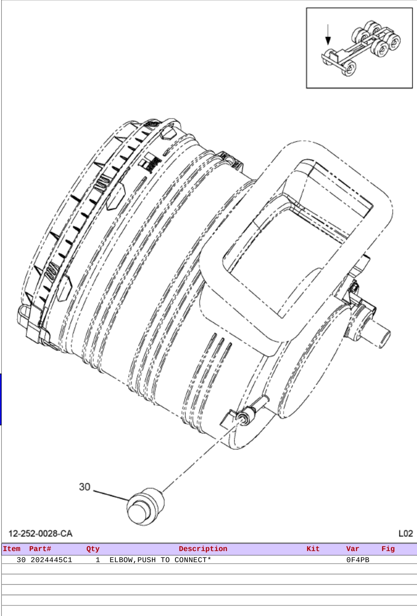
Figure 0F4N7 AIR RESTRICTION GAUGE INSTL
