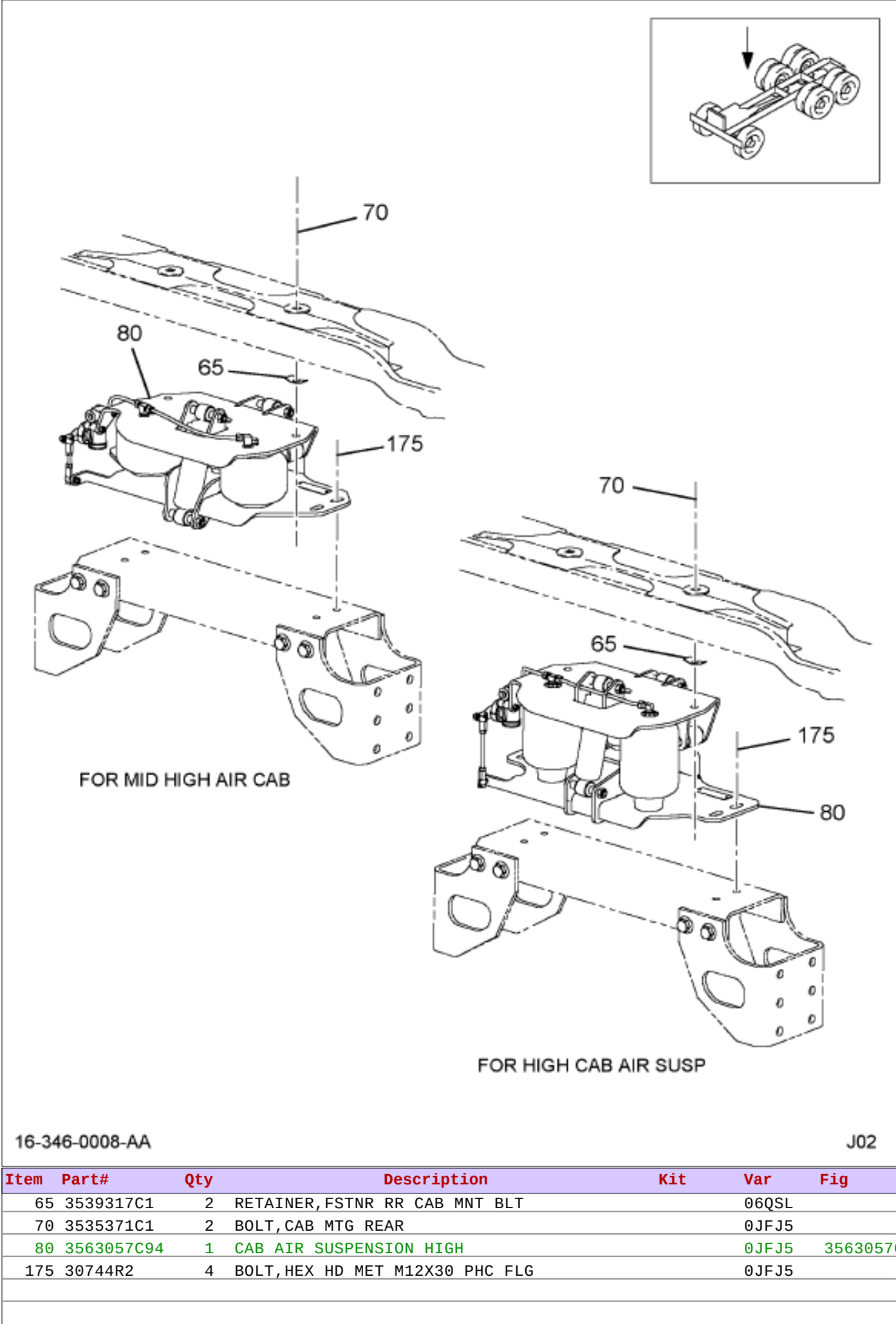
https://truckmanualshub.com/ Figure 06QSL CAB MTG, REAR; W/SUSP MTG
