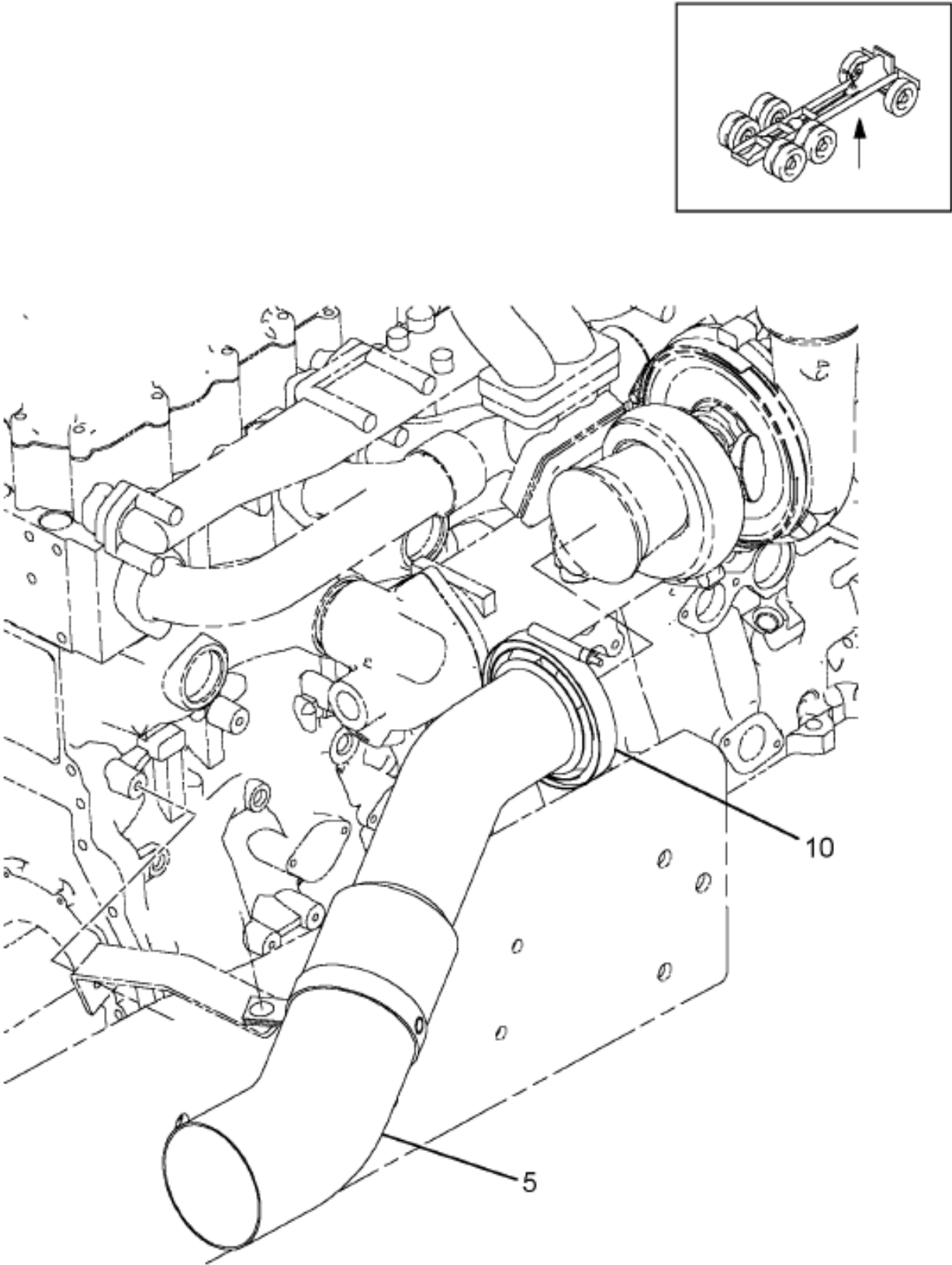
Figure 0G8JL TURBOPIPE, W/HDD ENGINES FOR UNDER CAB MUFFLER
