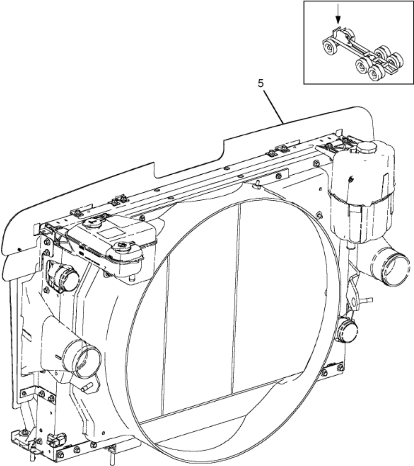
Figure 0K2R7 RADIATOR ASM, CAC
