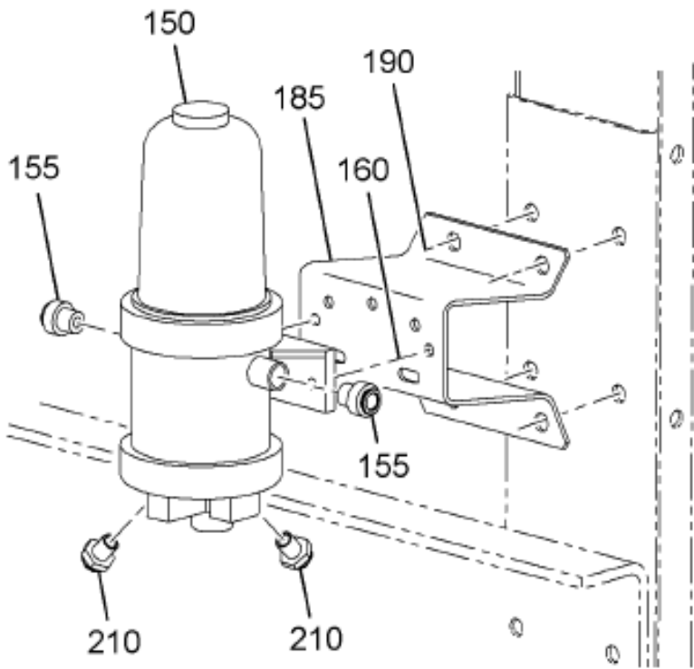
Figure 0LL11 FUEL WATER/SEPARATOR INSTL
