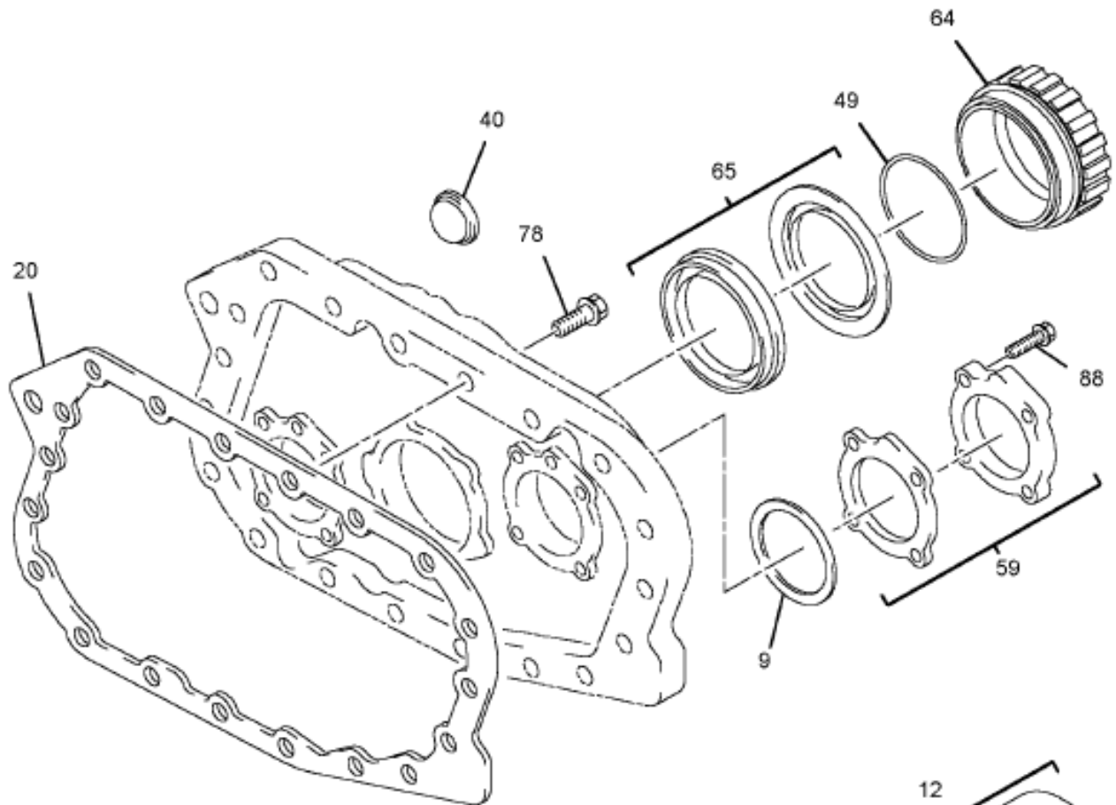
AUXILIARY CASE ASSEMBLY
