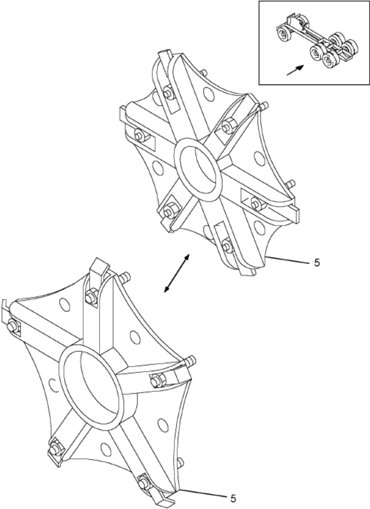
Figure 06LX1 HUB ASM, FRT WHEEL; DISC, W/DRUM
