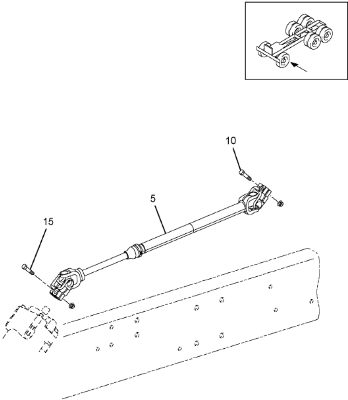
Figure 06SPX SHAFT, POWER STEERING;; INTERMEDIATE
