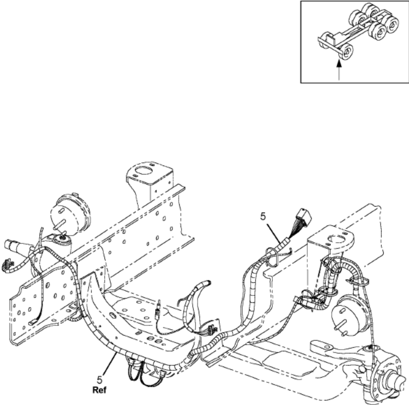
Figure 0F64M HARNESS, FORWARD CHASSIS; COMMON EFFECTS
