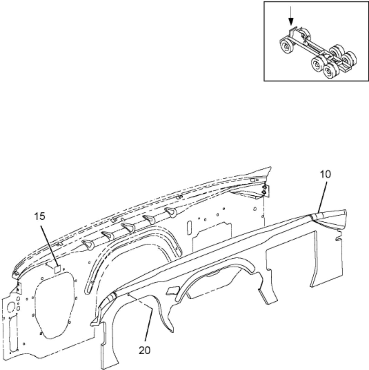
INSULATION, DASH PANEL Figure 06SV4
