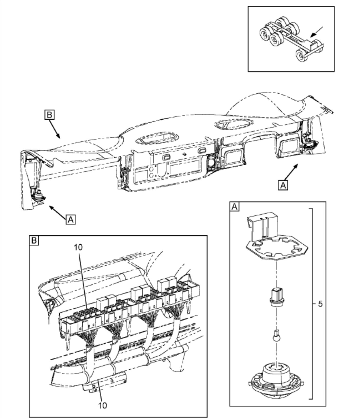
Figure 08-P30-0003-A0 INSTRUMENT PANEL MODULE; COURTESY & DOME LIGHT WIRING
