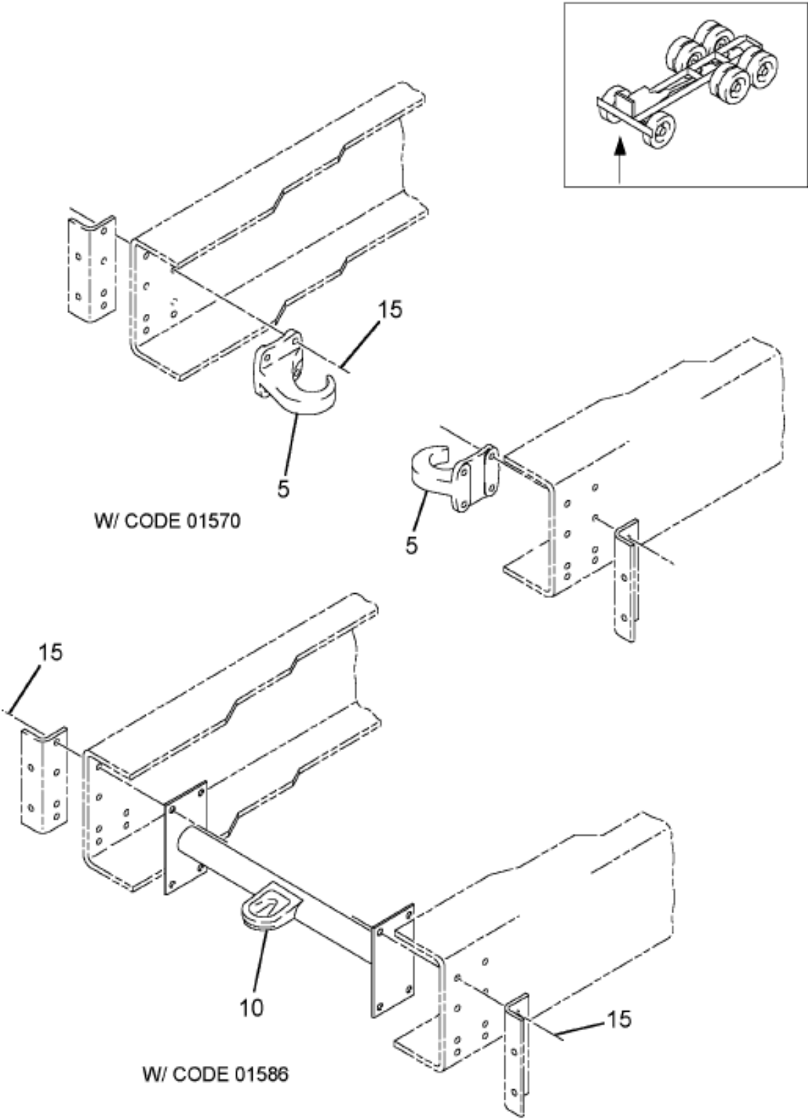
https://truckmanualshub.com/ Figure 07VQC TOW HOOK / LOOP & MTG; FRONT
