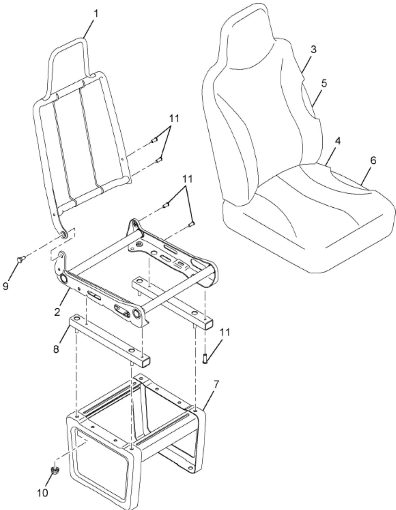
Figure 3575620C92 SEAT, PASS 1/3 HI BCK VINYL
