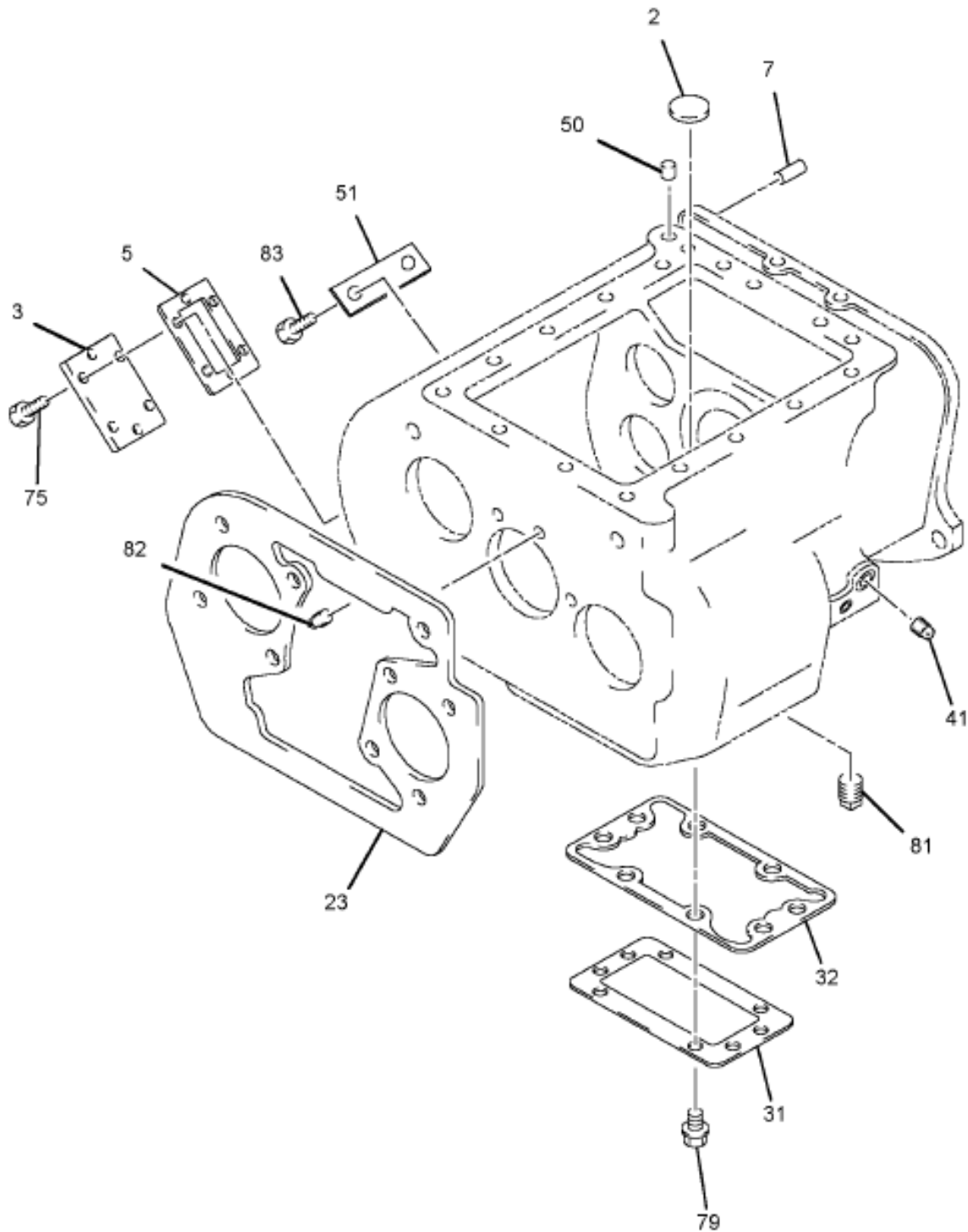
MAIN HOUSING ASSEMBLY
