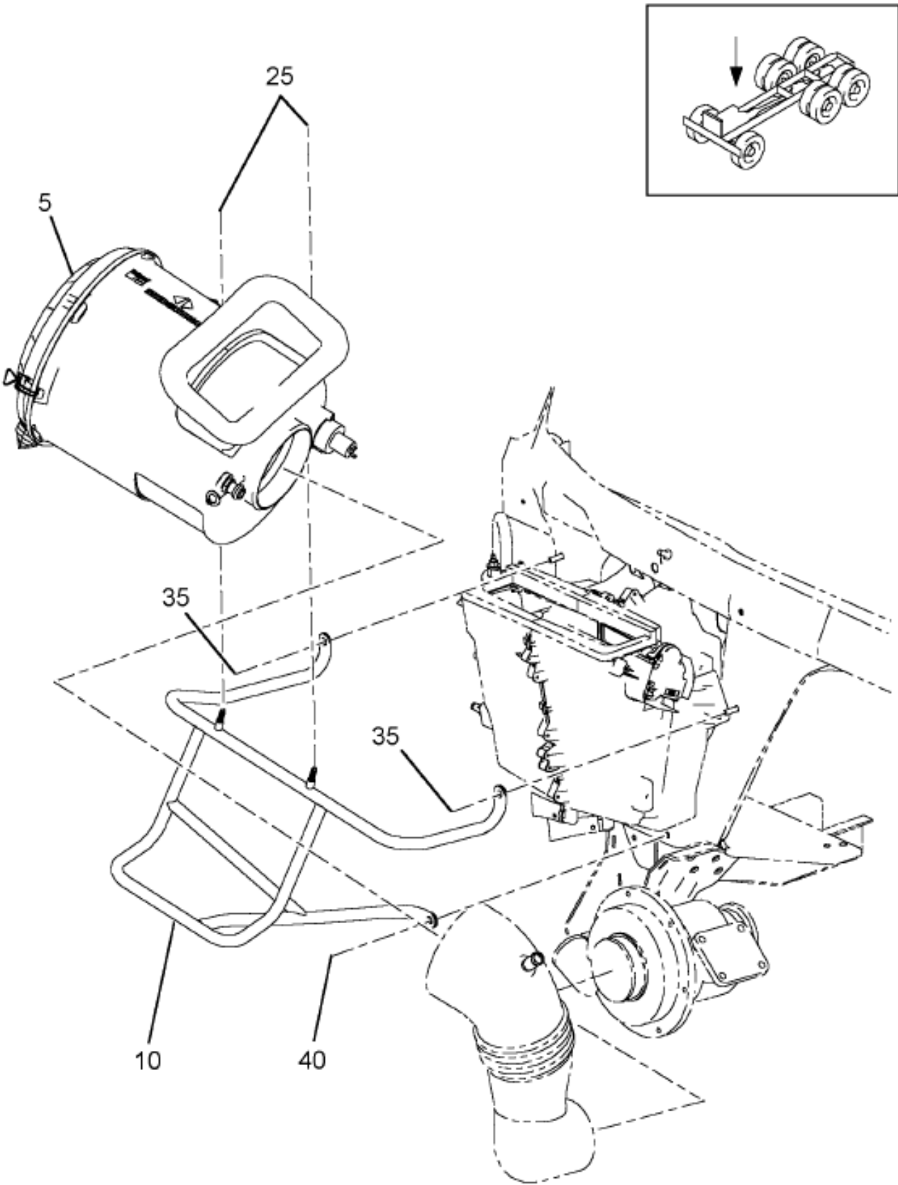
https://truckmanualshub.com/ Figure 0L3H6 AIR CLEANER & MTG
