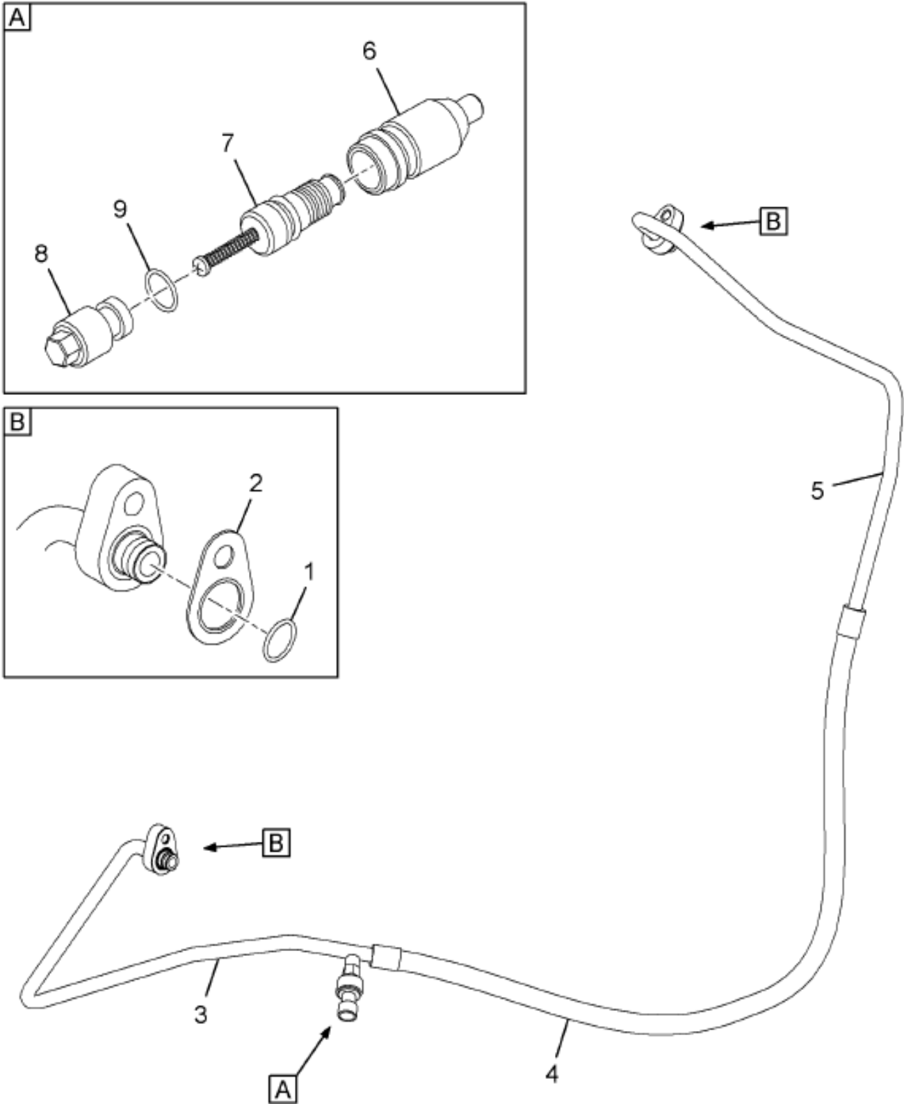
https://ruelmanualshub.com/ Figure 3561084C94 HOSE, A/C COND TO EVAP
