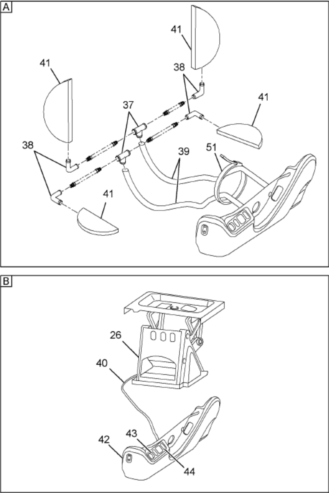
https://truckmanualshub.com/ Figure 3558490C92 SEAT, DRS HI AIR VN W/ARMREST
