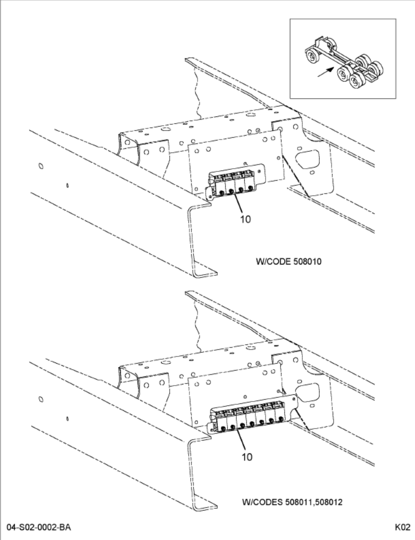
Figure 0CB2X VALVE, AIR SOLENOID; AIR HORN
