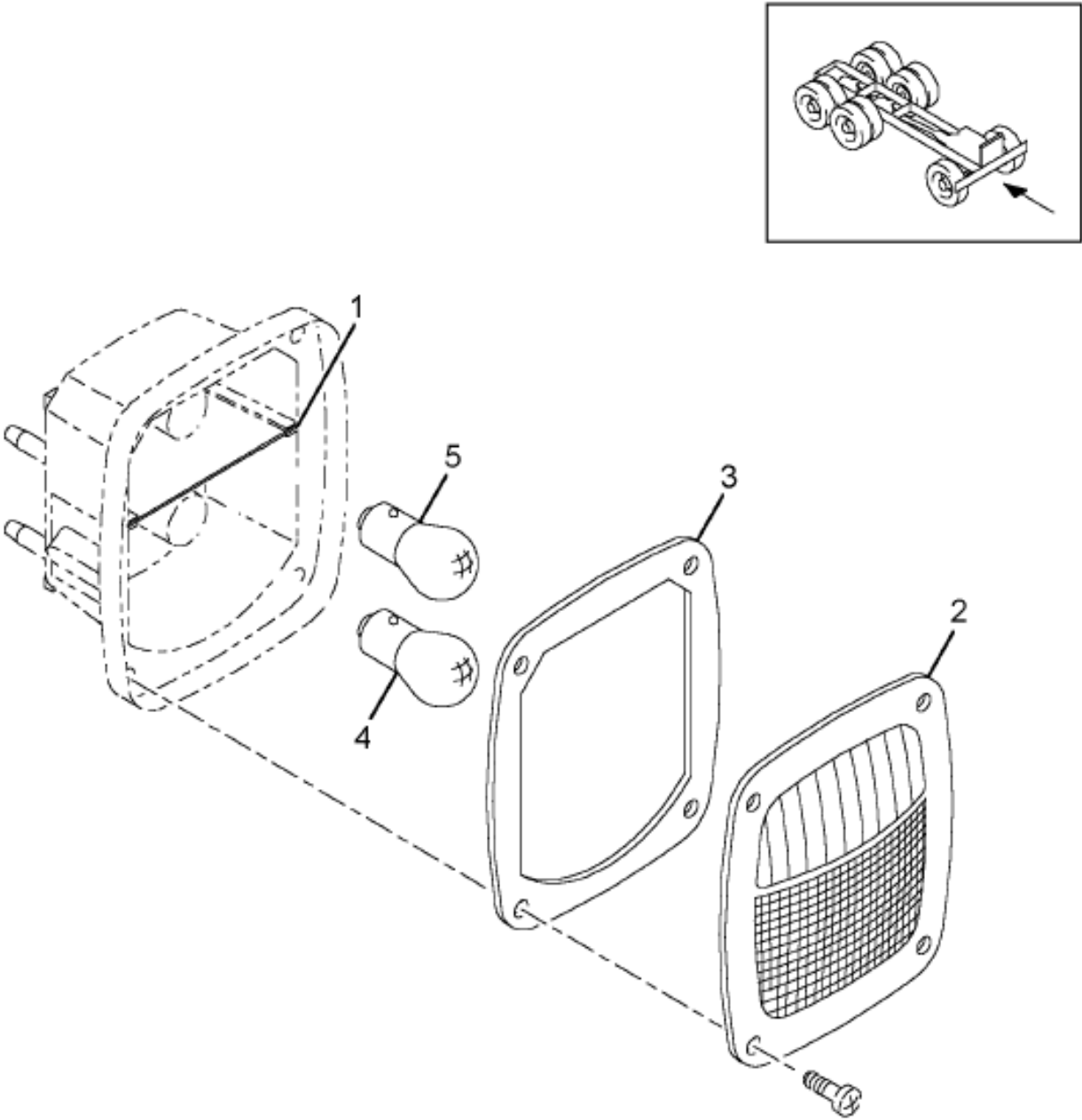
Figure 1661282C91 LIGHT, ASSY STOP TAIL TURN WITH
