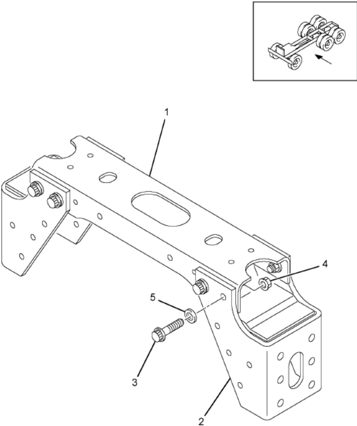
Figure 3567192C93 CROSSMEMBER, CAB REAR SUPT ASSY
