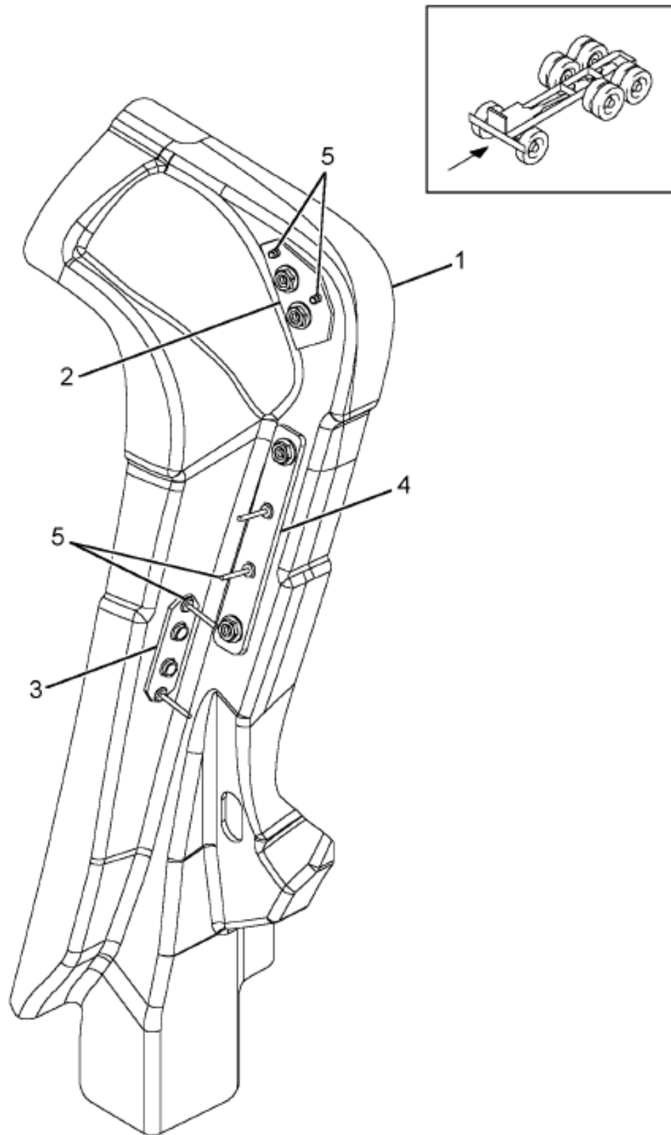
Figure 3556253C2 REINFORCEMENT, HOOD RH FRONT AS
