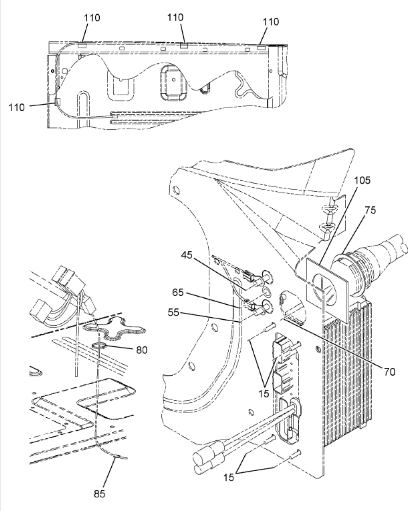
Figure 06TRV INSTRUMENT PANEL HARDWARE INSTL; CONTROL MODULE
