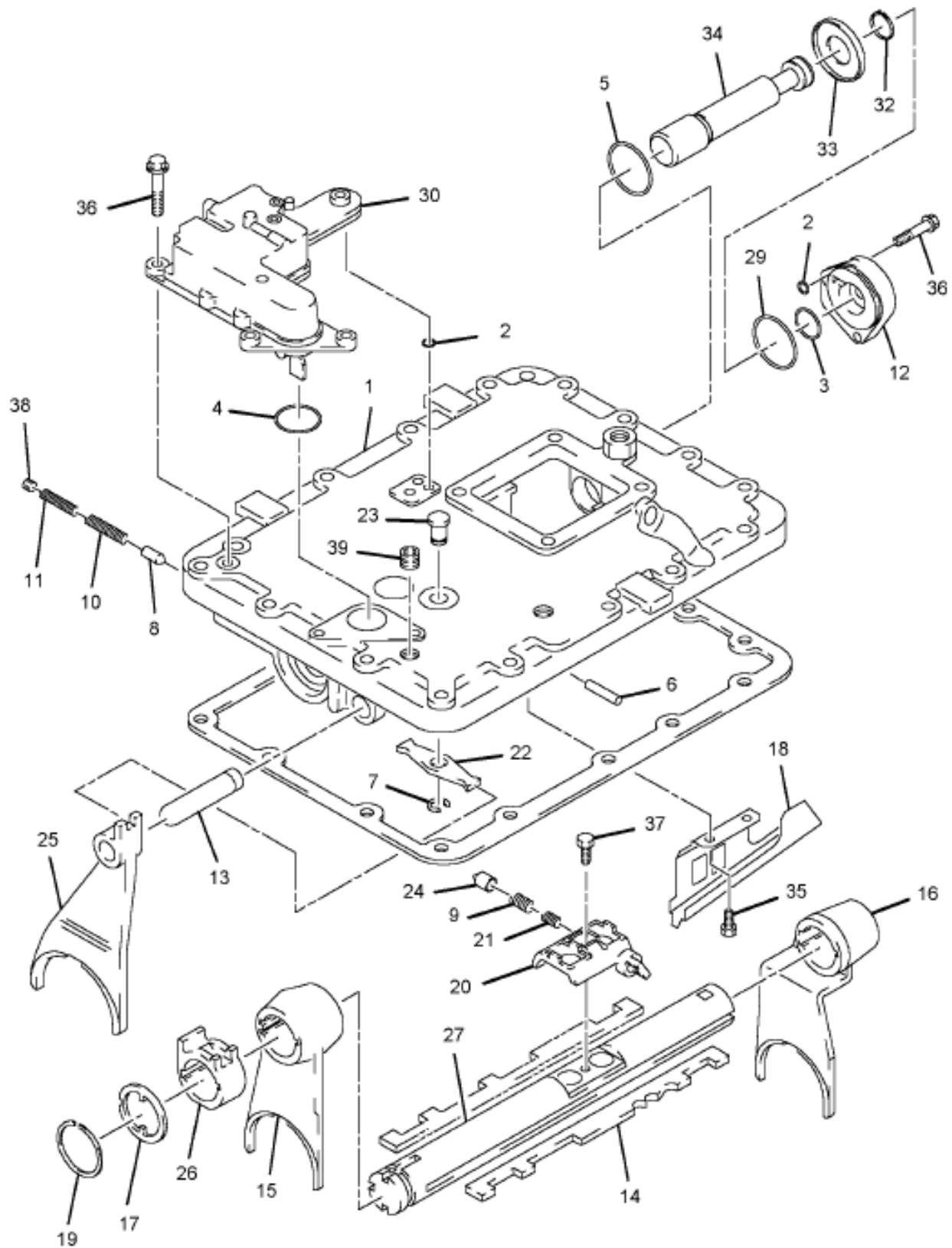
BAR HOUSING ASSEMBLY
