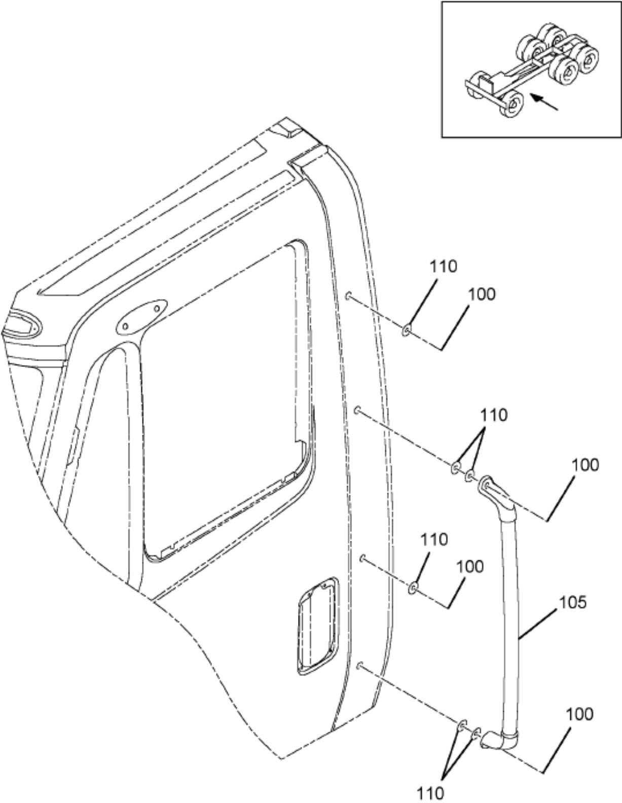
Figure 0HZNT GRAB HANDLES, CAB ACCESS
