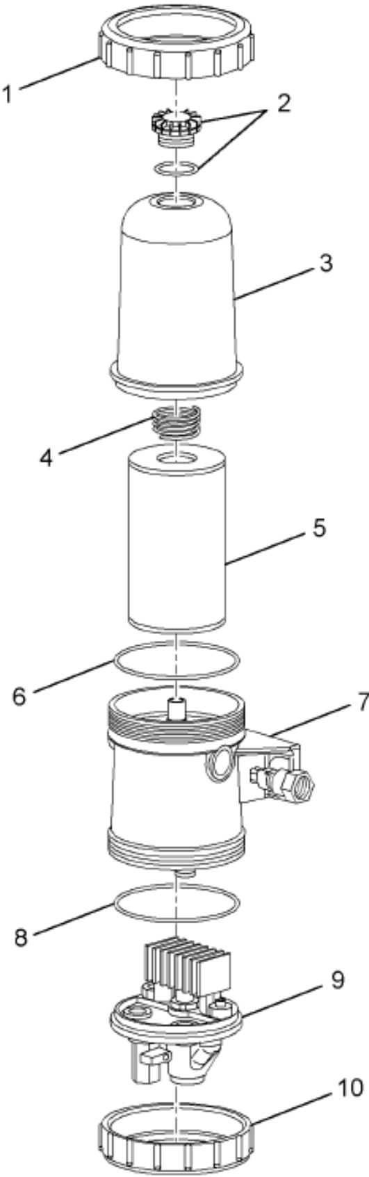
https://trucksmanualshub.com/ Figure 3588508C92 FILTER, FUEL *DAVCO 382 W/1-14 S
