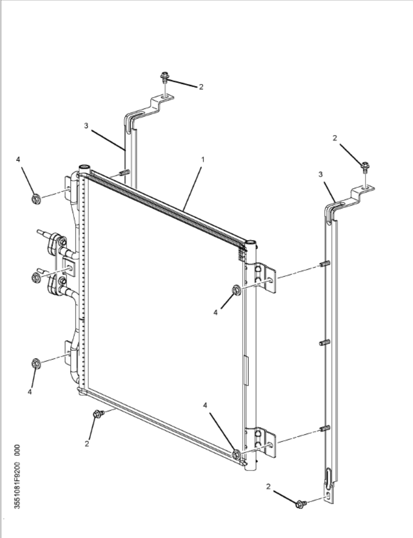
https://www.manualshub.com/ Figure 3560074F92 CONDENSER, AIR COND MODULE
