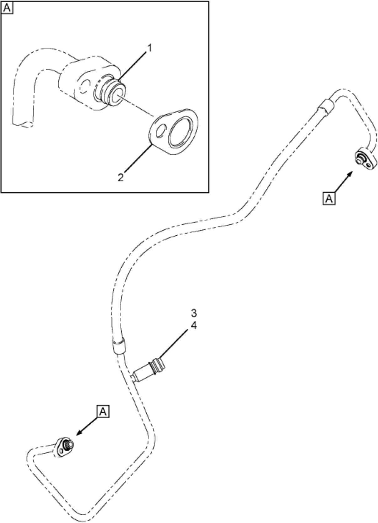
https://truckmanualshub.com/ Figure 3548042C1 TUBE, A/C EVAP TO ACCM W/O VLV
