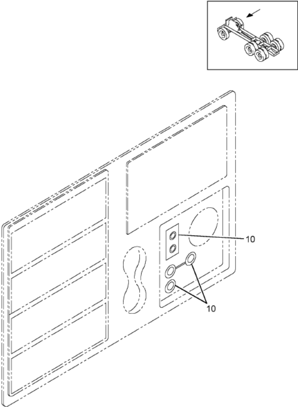
Figure 6DBN1 INSTRUMENT PANEL MODULE; CIGAR LIGHTER/POWER SOURCES
