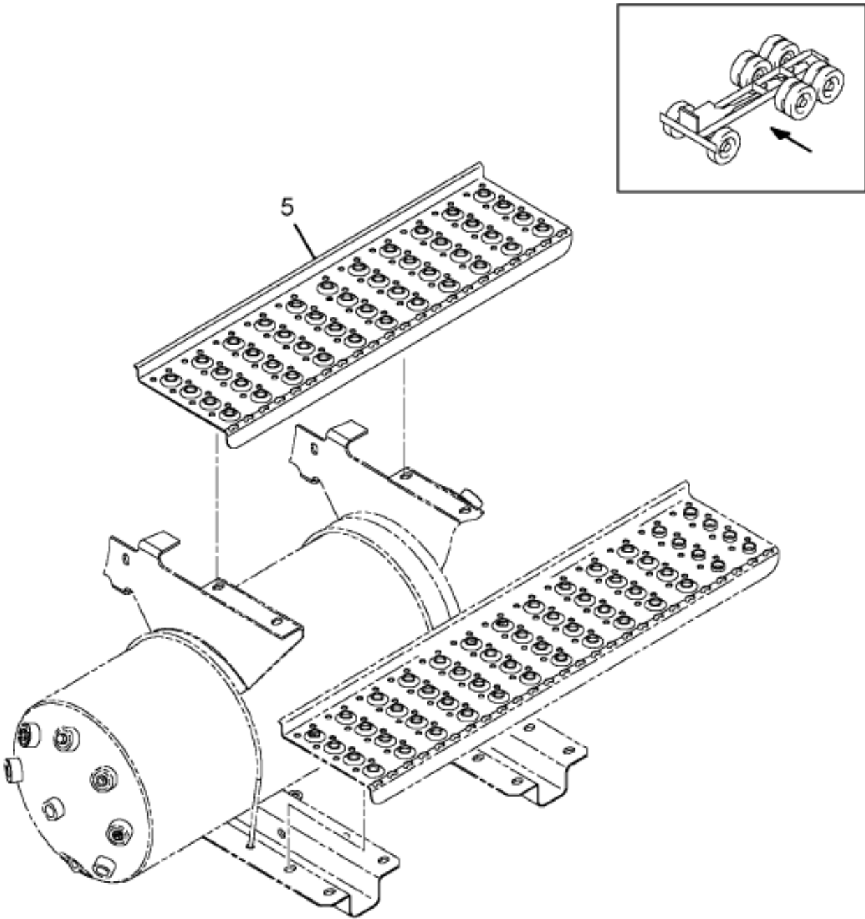
https://truckmanualshub.com/ Figure 0HK1X STEPS; AIR TANKS MODULE
