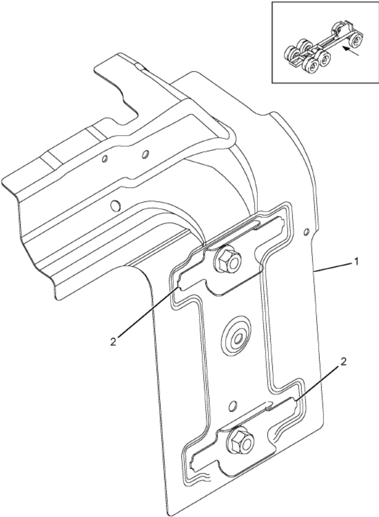
Figure 3562417C1 HEADER, DOOR OPENING RR CRNR RH
