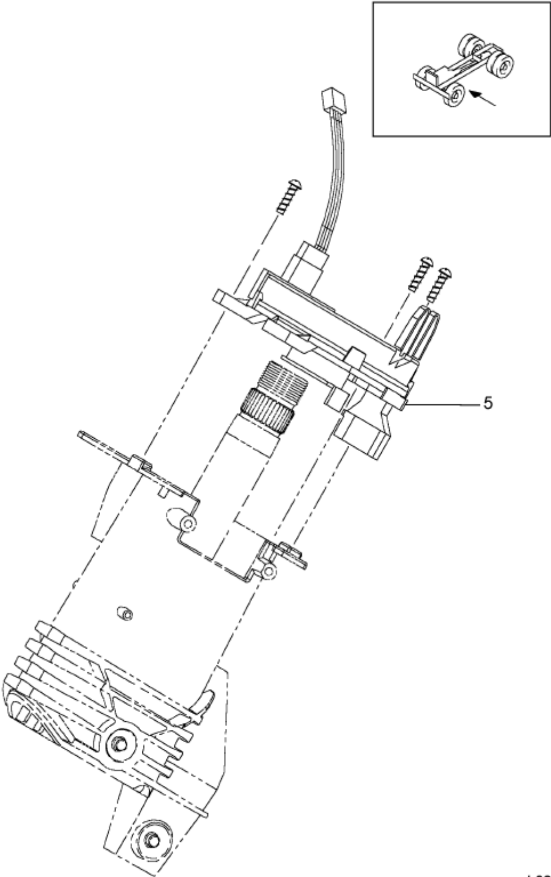
Figure 6DCJY DCM; CLOCK SPRING, ELECTRICAL
