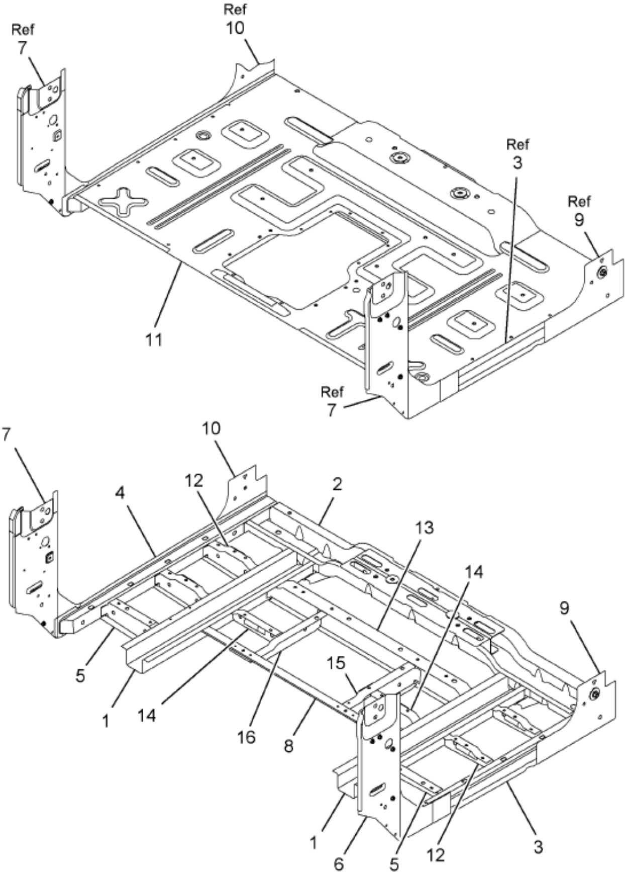
Figure 3547272C95 UNDERBODY, ASSY CONV BIG BORE
