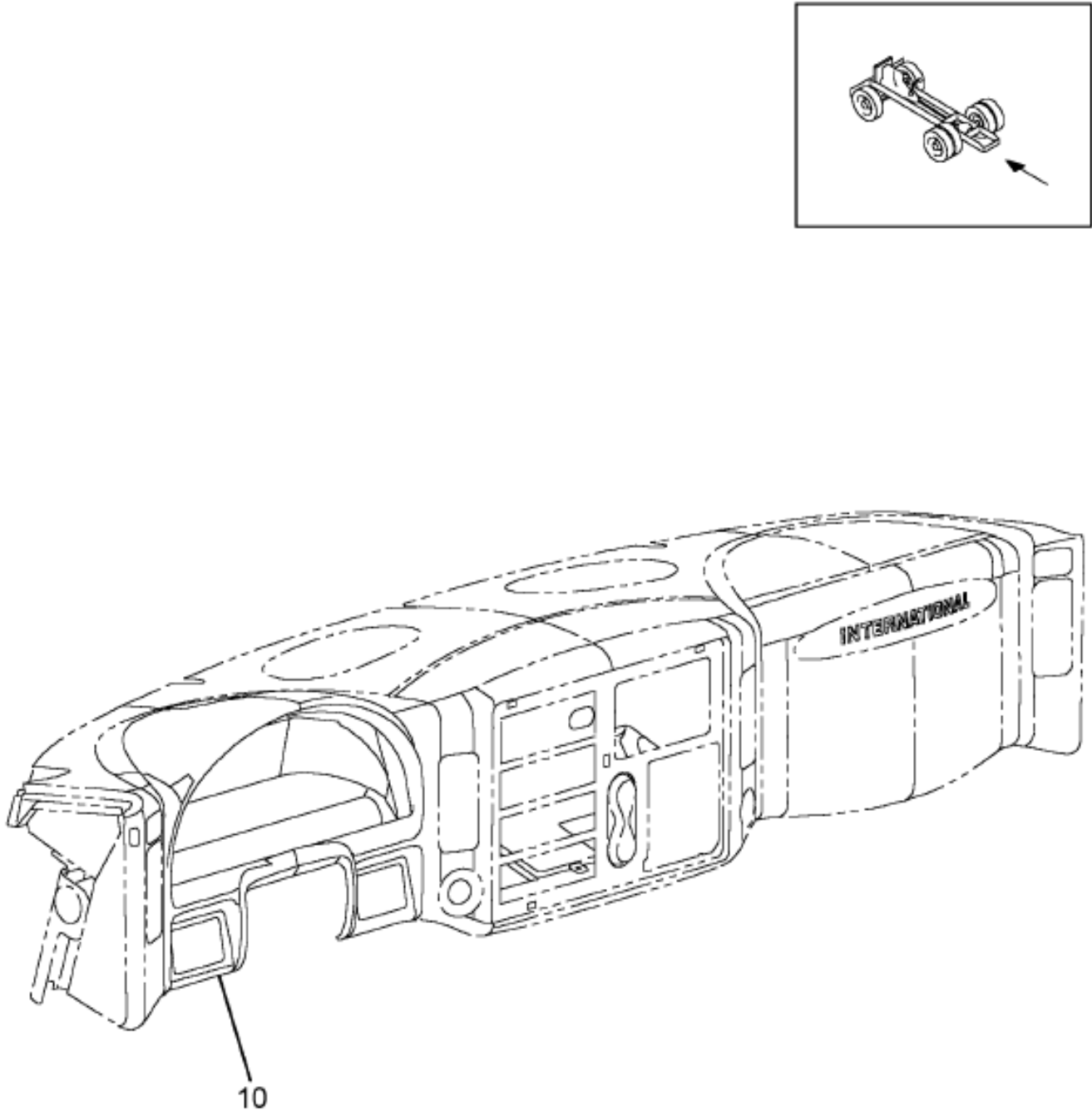
Figure 06JV1 INSTRUMENT PANEL CLOSEOUT; LEFT EFFECTS
