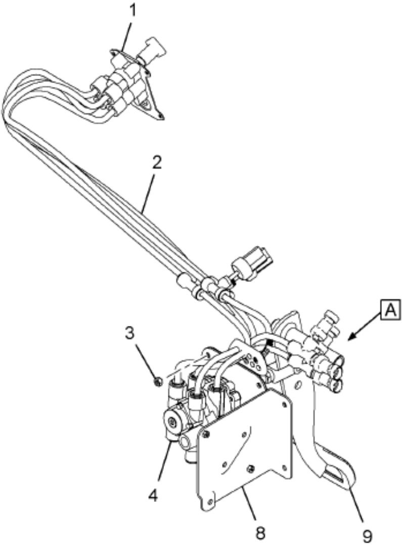
https://truckmanualshub.com/ Figure 3541516F93 BRAKE, DCM*TRUCK AIR BRK VLV
