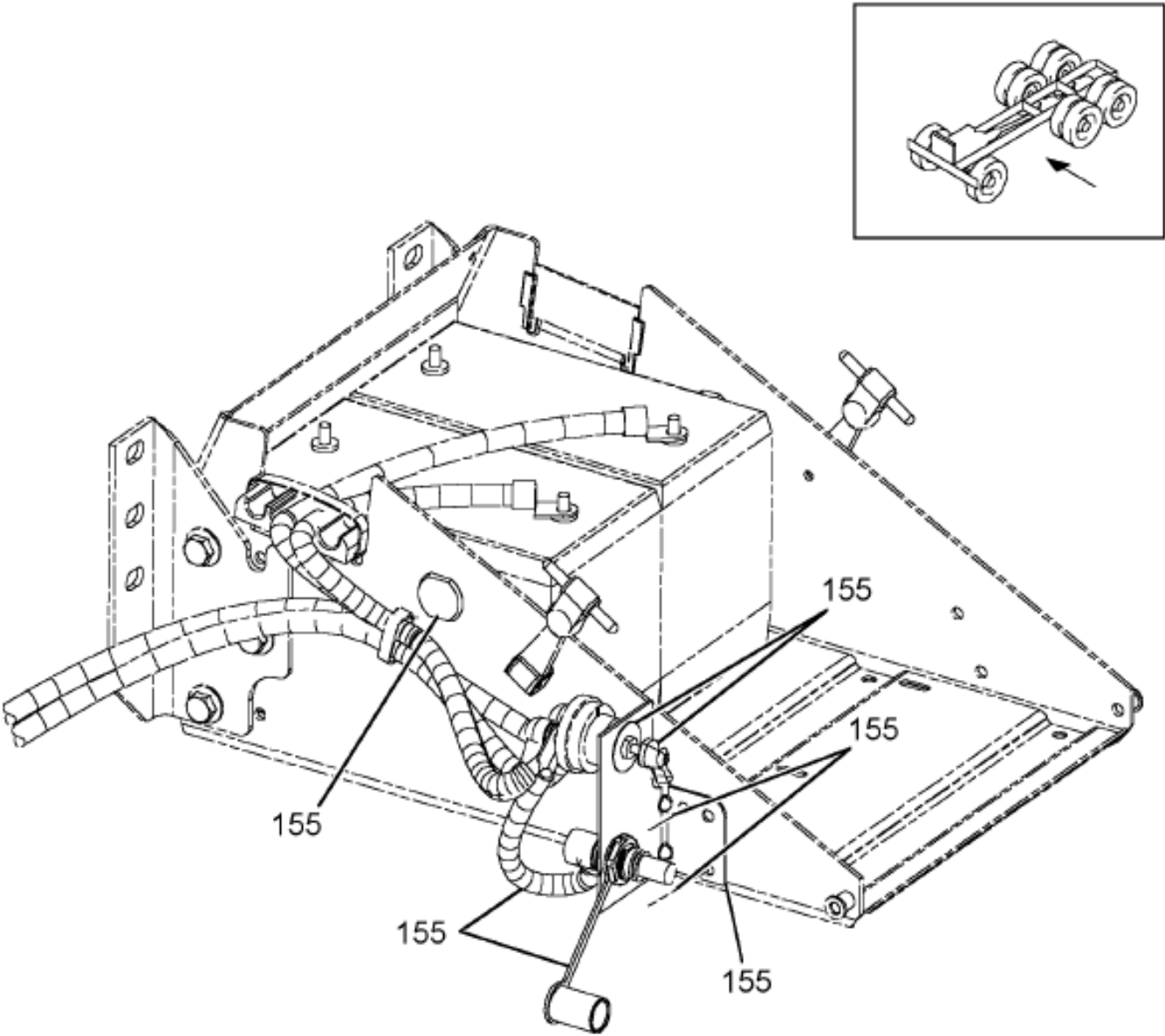
Figure 0L03Z JUMP START STUD & DISCONNECT SWITCH
