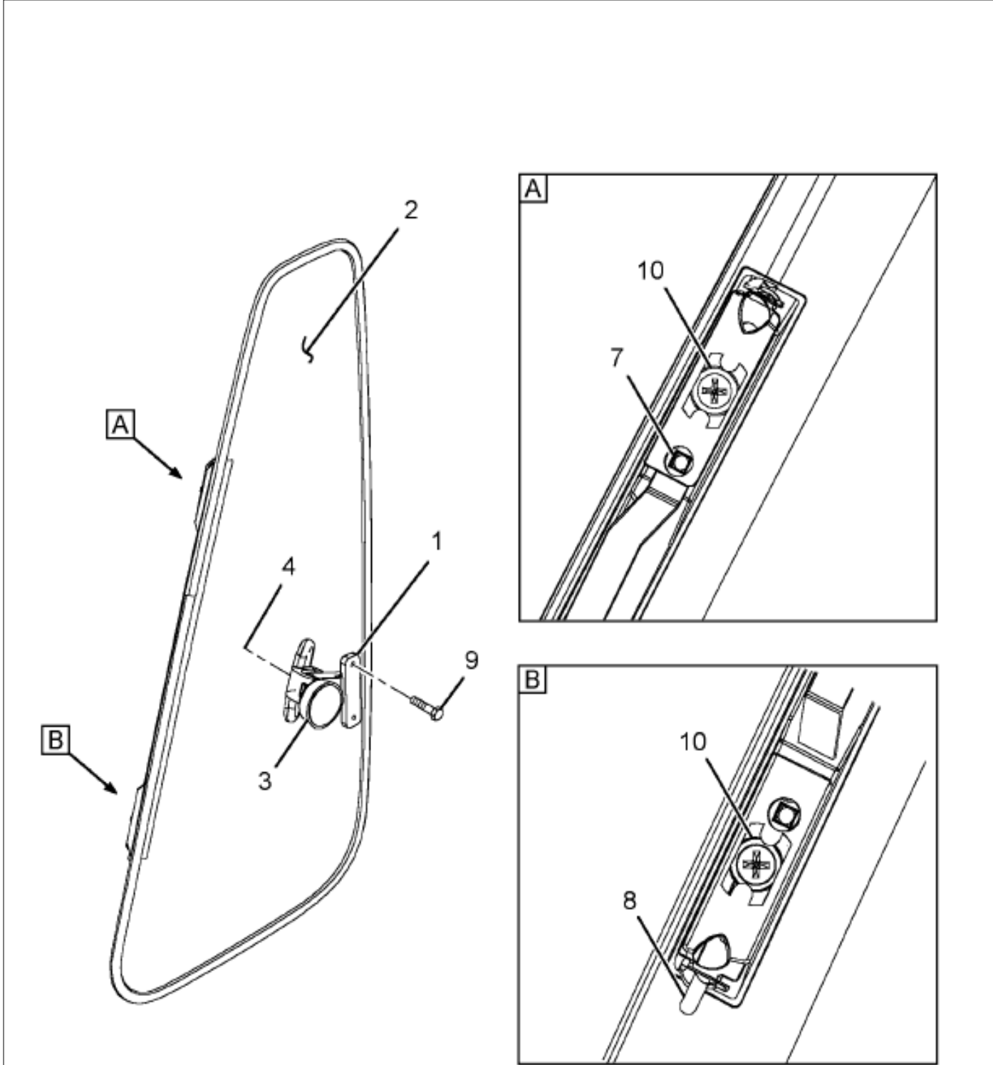
Figure 3567240C92 WINDOW, VENT LH
