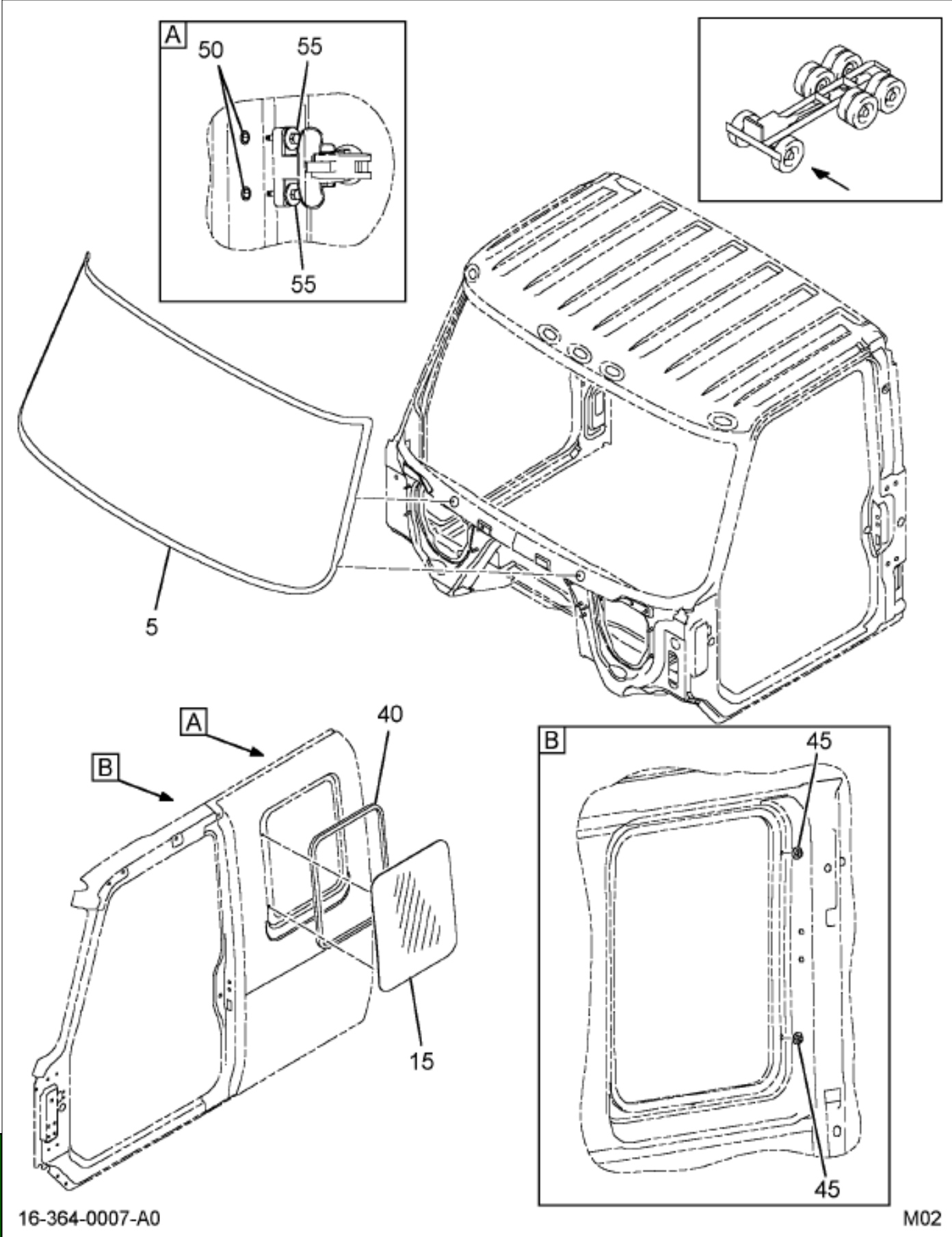
Figure 06MXR WINDSHIELD INSTL; W/REAR SIDE QTR WINDOW
