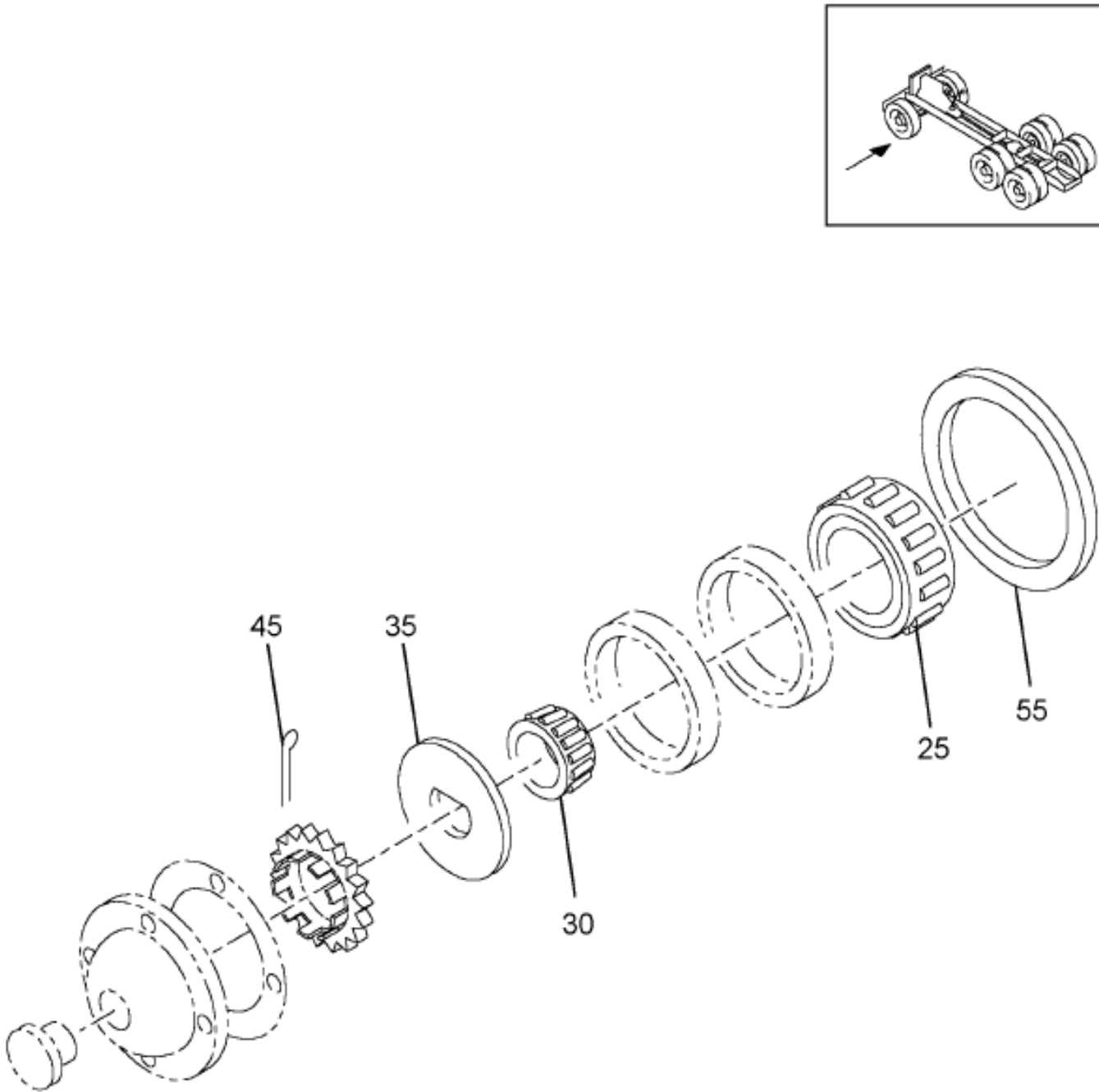
Figure 07SZV SEALS & BEARINGS; WHEELS, FRONT AXLE
