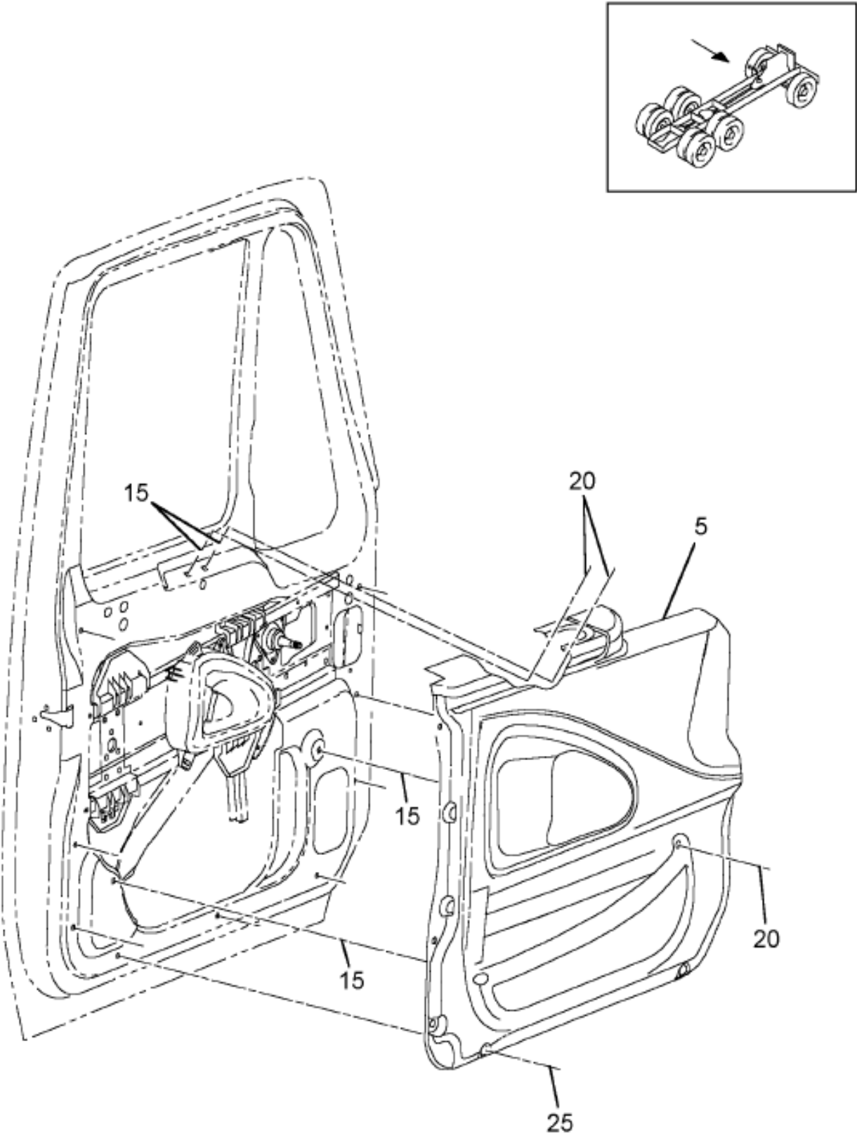
Figure 0JC0G PANEL, DOOR TRIM LEFT
