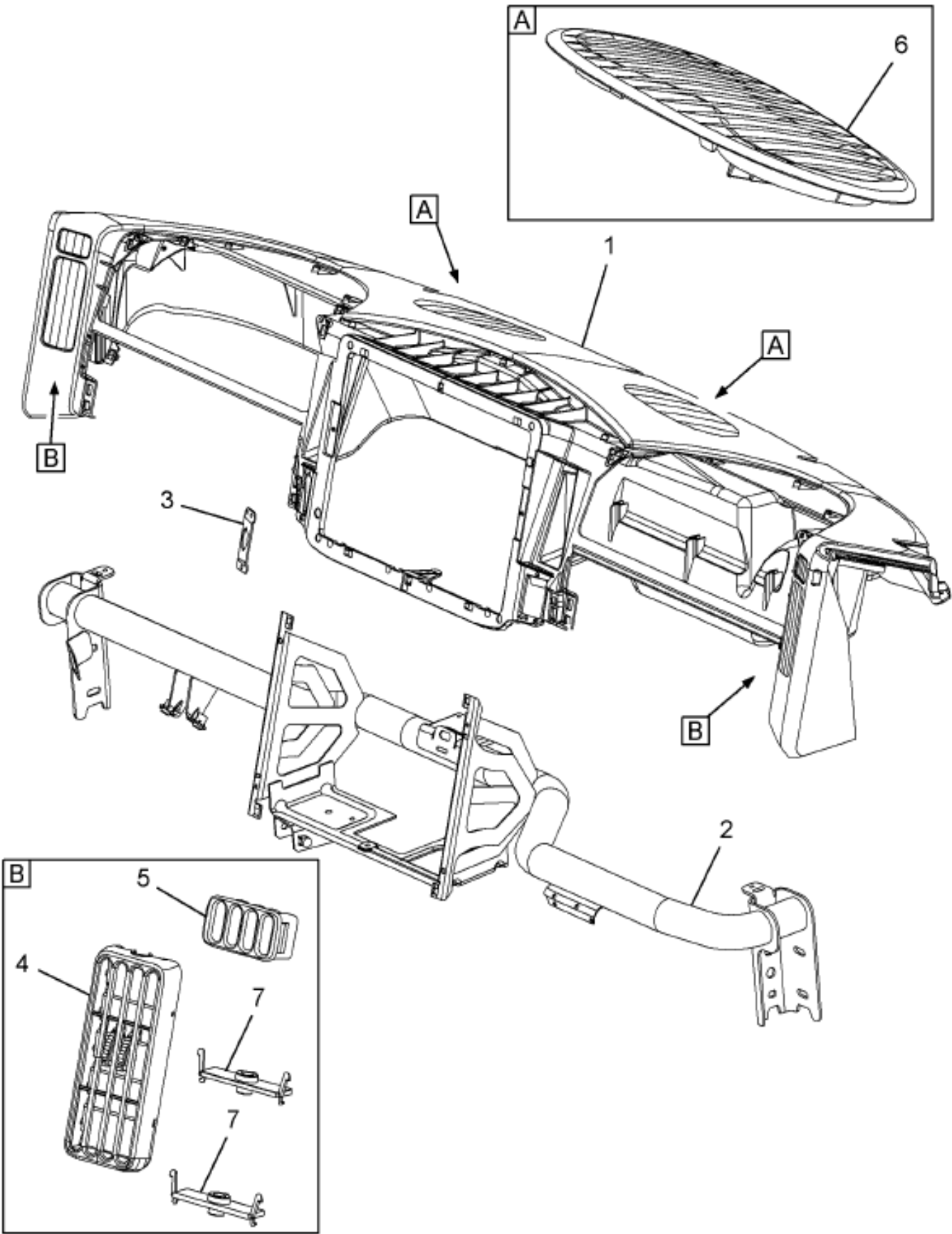
https://truckmanualshub.com/ Figure 3511018F93 INST PANEL MAIN CARRIER LHD
