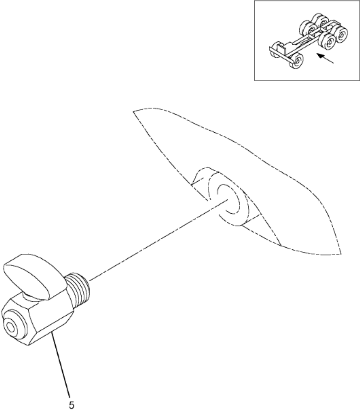
Figure 0FLMS DRAIN VALVES, AIR TANKS
