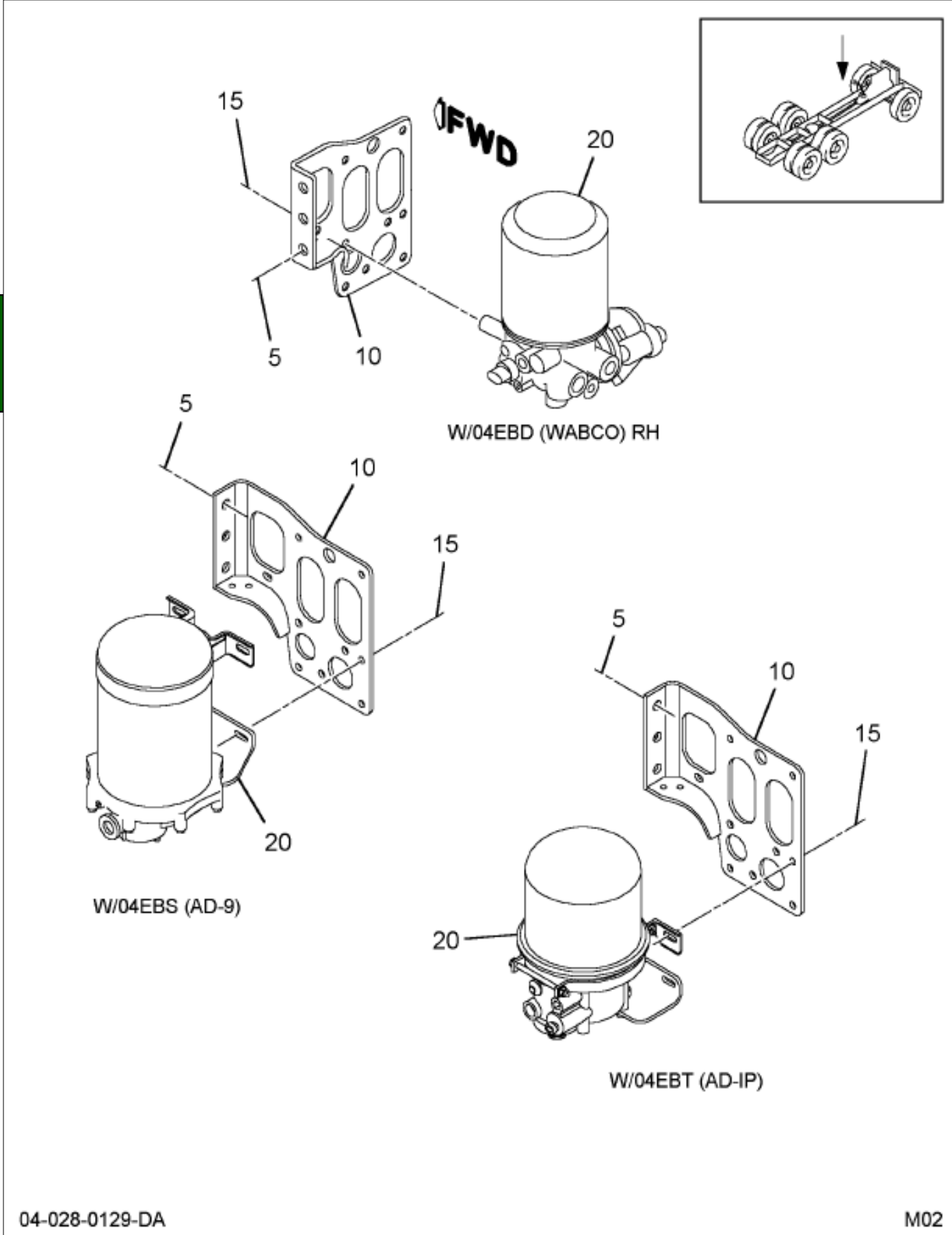
https://truckmanualshub.com/ Figure 0HZW3 AIR DRYER & MTG
