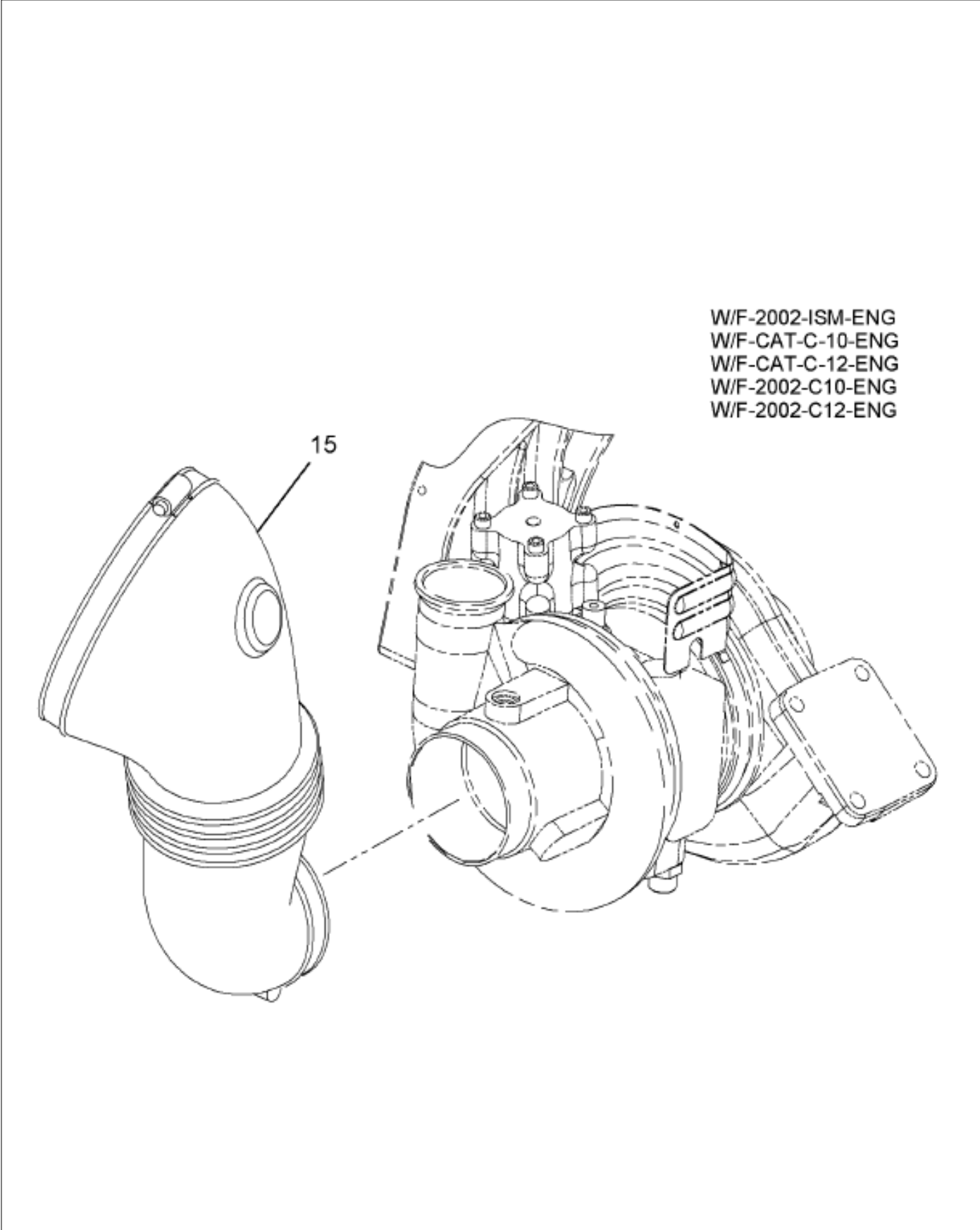
Figure 0F4N3 AIR CLEANER PIPING INSTL; (CAT ISM, C10/C12 ENGS)
