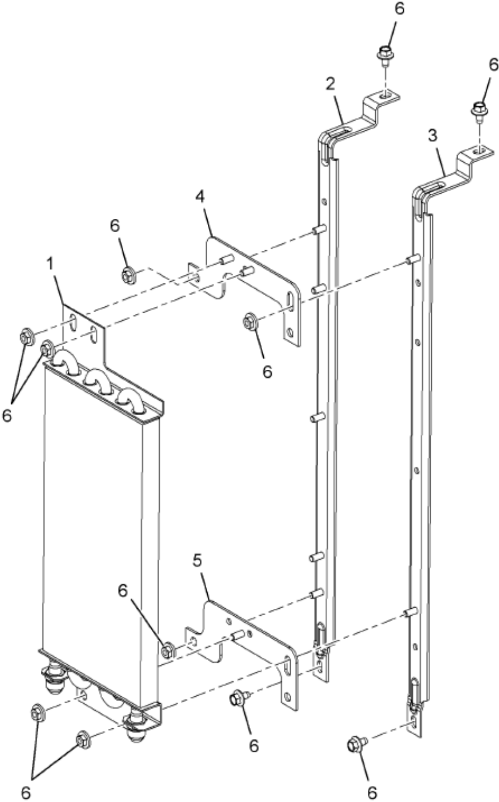
Figure 2508810C92 COOLER, OIL TRANS
