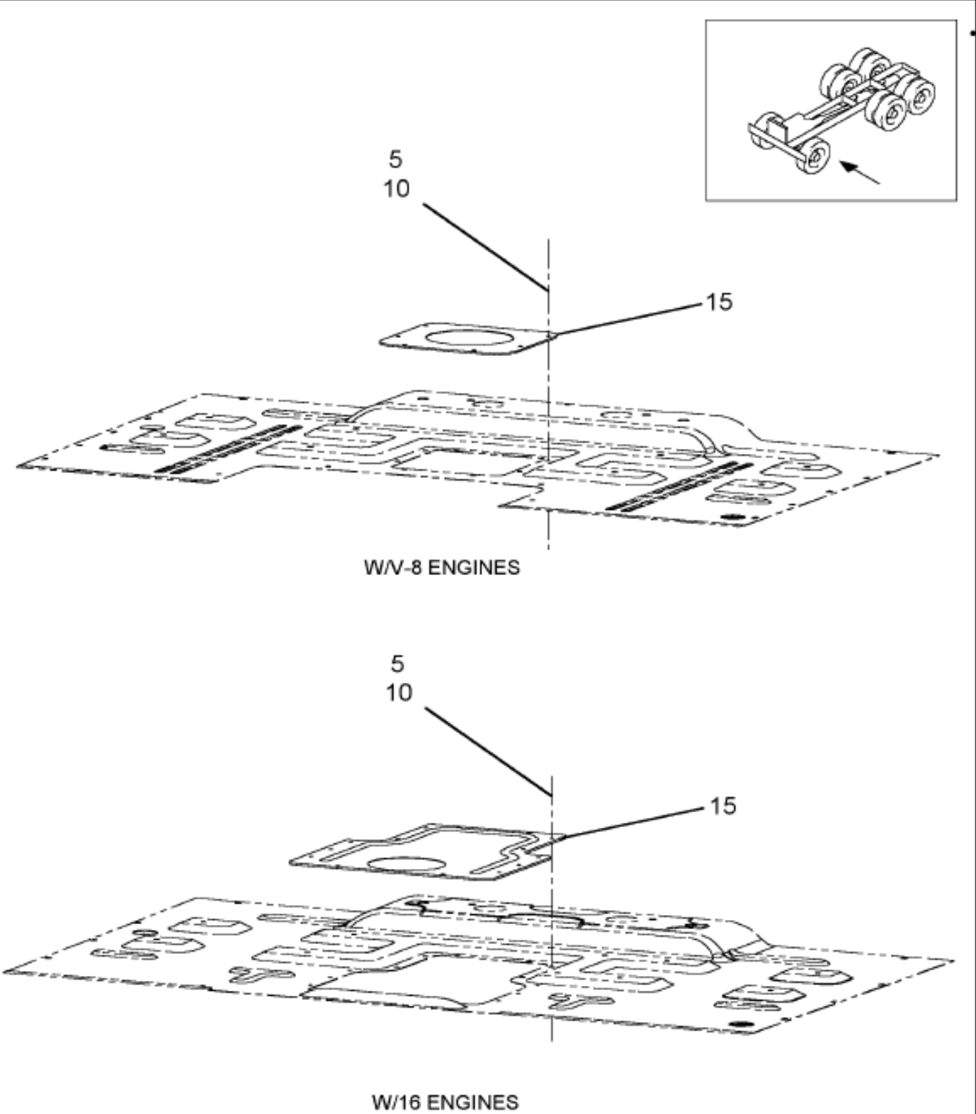
https://truckmanualshub.com/ Figure 0G4M9 TRANSMISSION COVER
