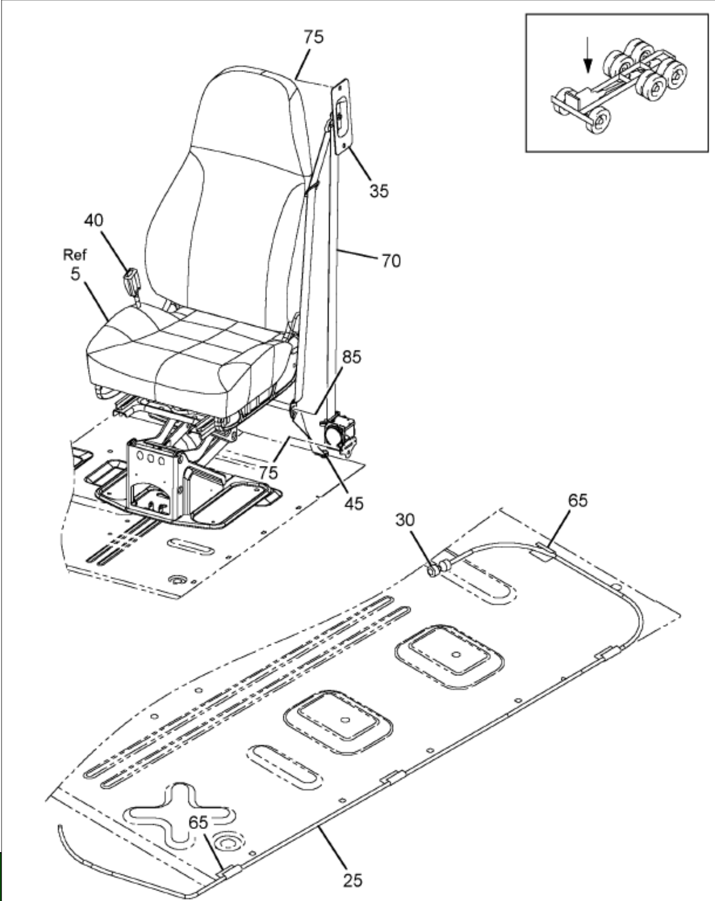
https://truckmanualshub.com/ Figure 0FVYN SEAT, DRIVER; W/ BELT; NATIONAL
