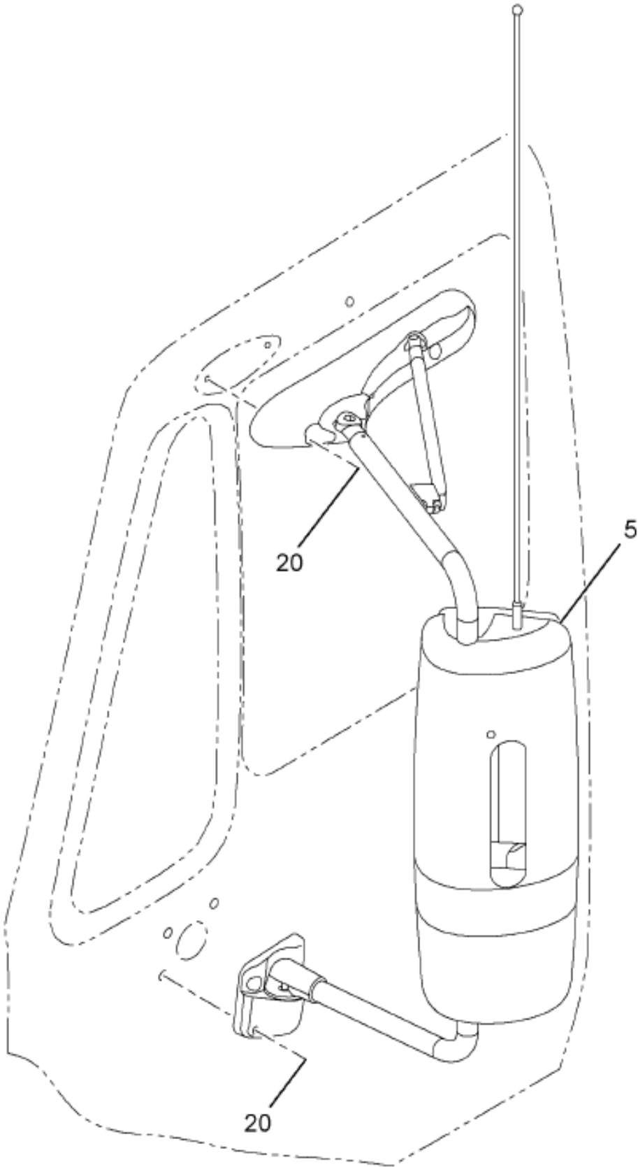
https://truckmanualshub.com/ Figure 06VP9 MIRROR ASM & MTG, REAR VIEW
