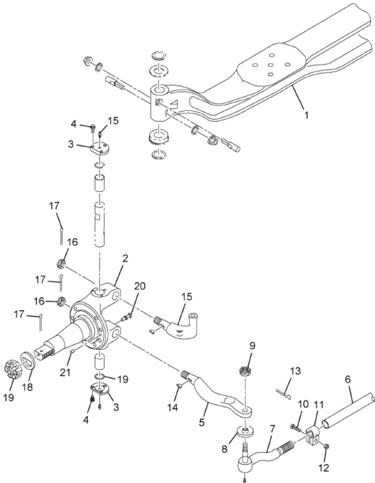
Figure 3567353C91 AXLE, ASSY FRT AIR 02AEW 20K
