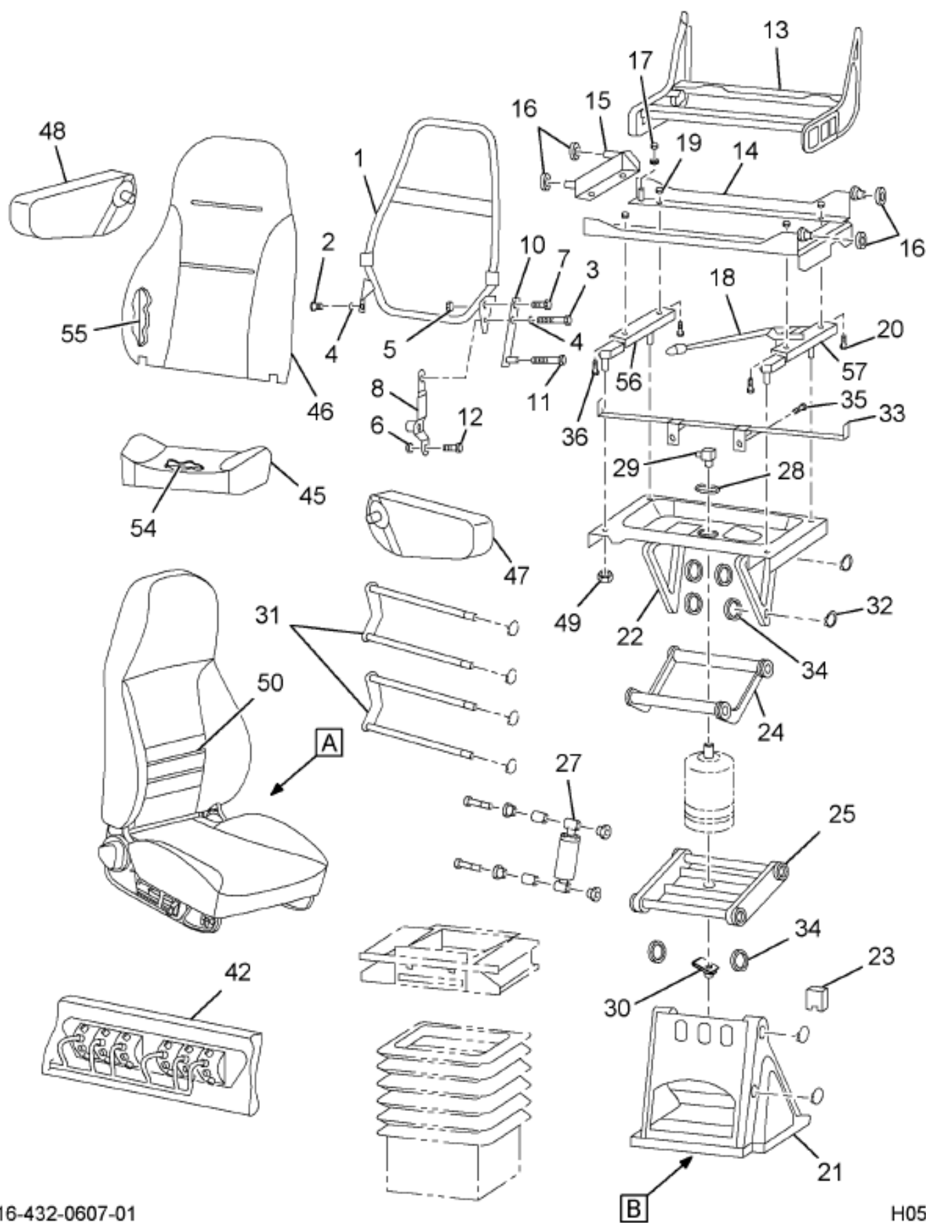
Figure 3558490C92 SEAT, DRS HI AIR VN W/ARMREST
