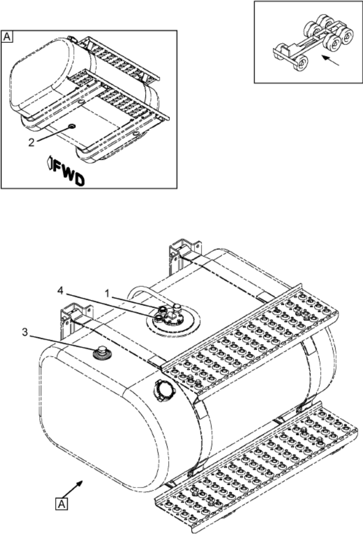
Figure 3548119F92 TUBE, FUEL TANK INLET OR OUTLET
