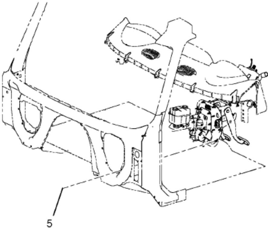
https://truckmanualshub.com/ Figure 06QS3 DCM MOUNTING HARDWARE
