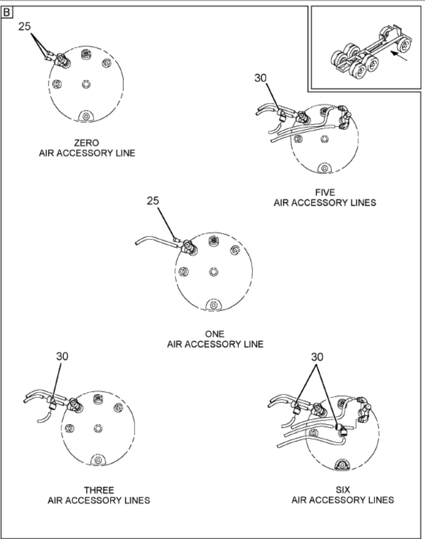
Figure 6HC2S AIR TANK TUBING
