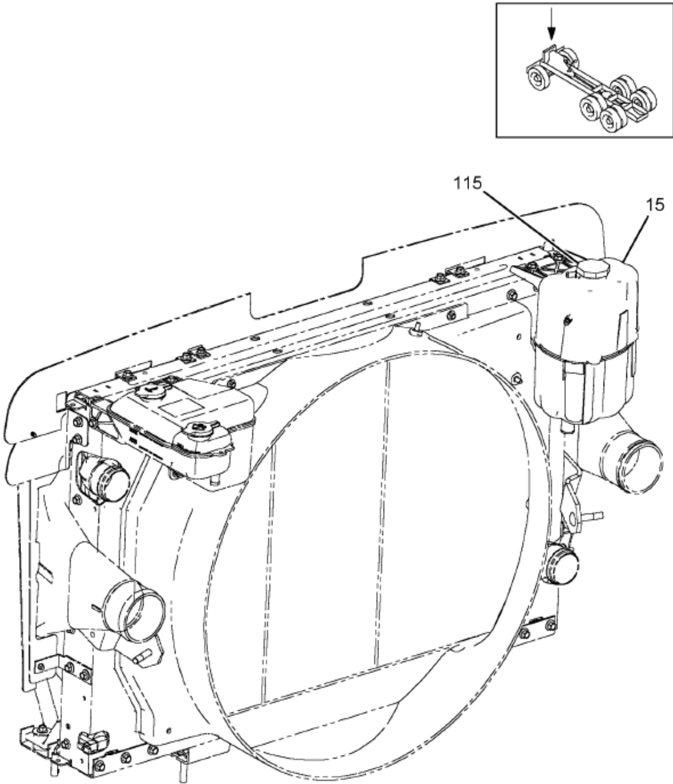
https://truckmanualshub.com/ Figure 0K2V9 SURGE TANK & MTG, DEAERATION
