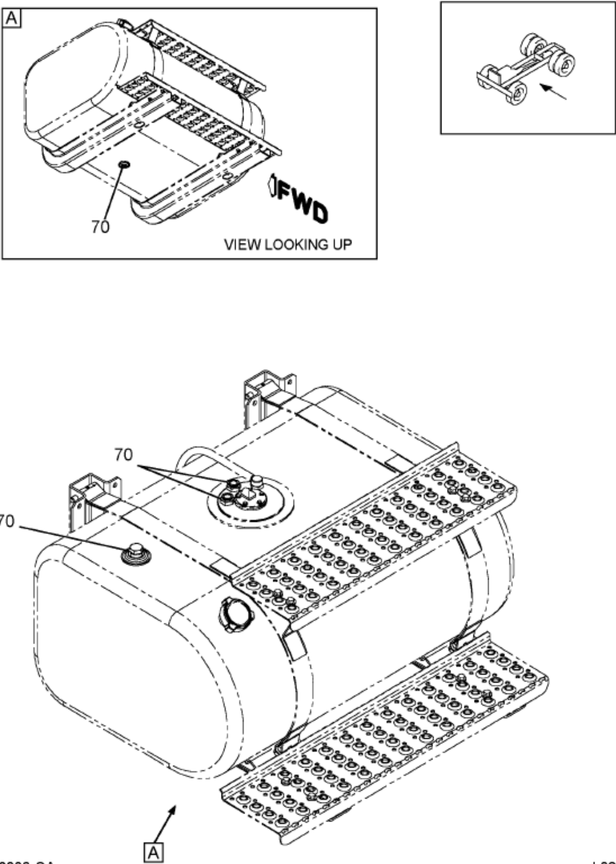
FUEL TANK DRAW TUBES, MODULE; LEFT SIDE (ABR #14)
