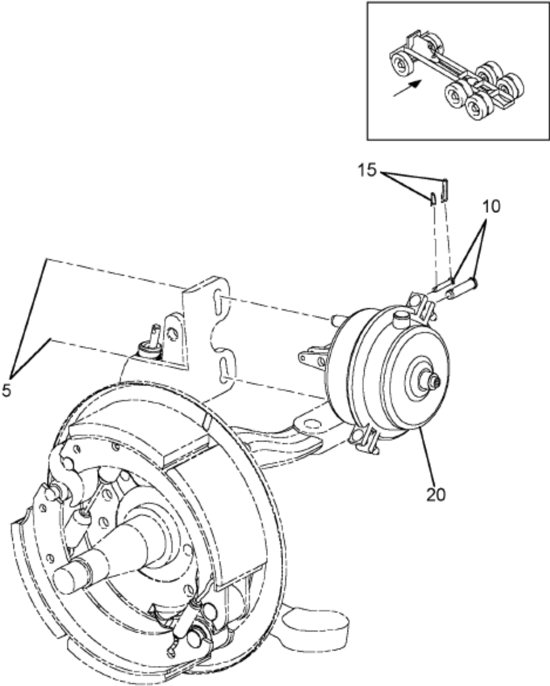
Figure 0DN3J BRAKE CHAMBER, FRONT; 24", LONGSTROKE
