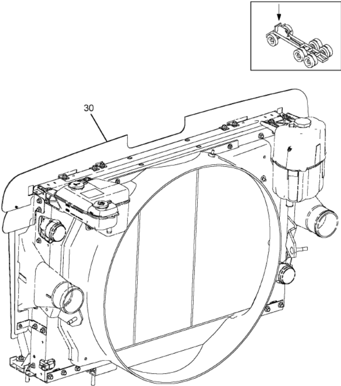
Figure 0K2VM AIR RECIRCULATION SEALS; COOLING PACKAGE
