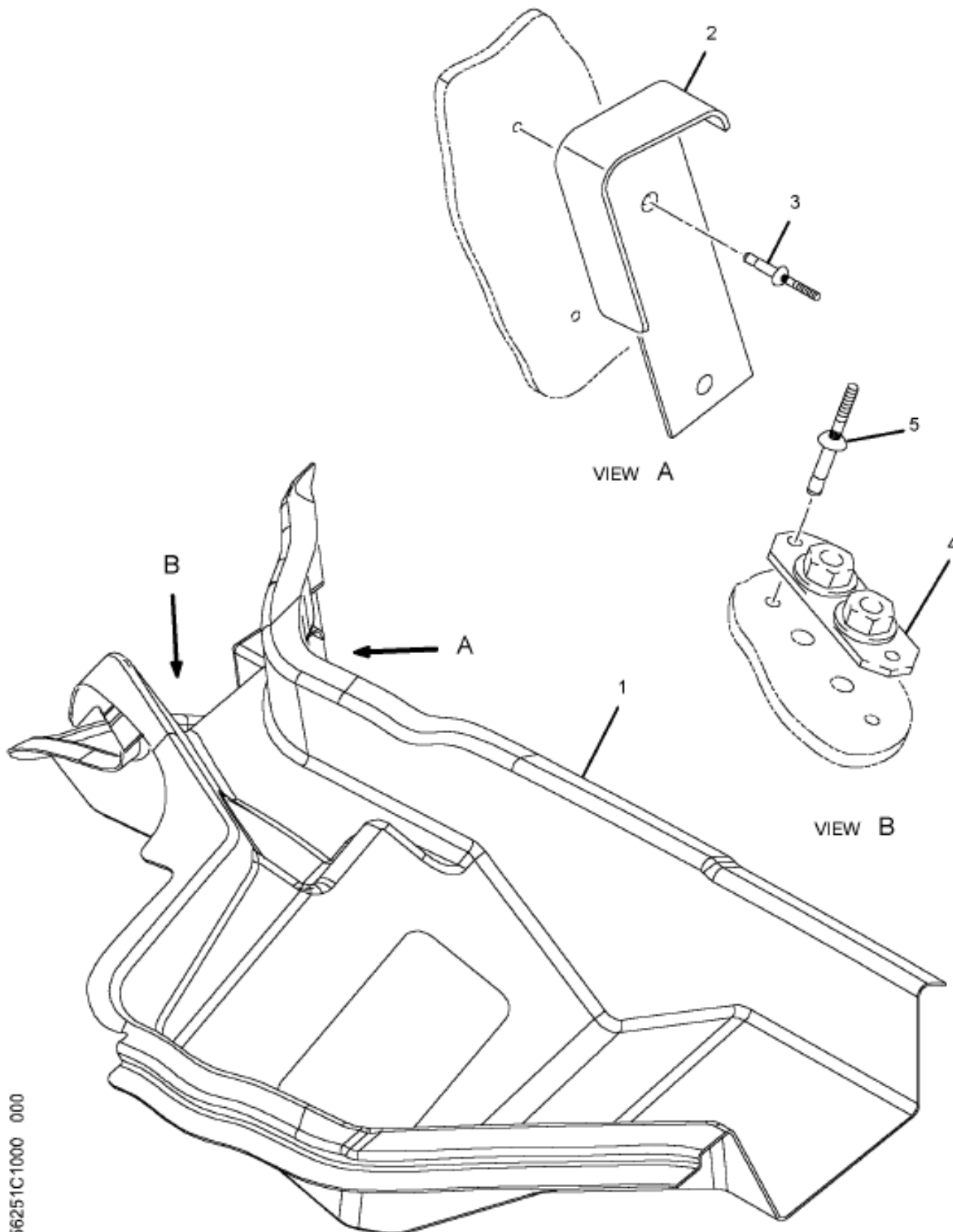
Figure 3556251C2 REINFORCEMENT, HOOD ASSY RH
