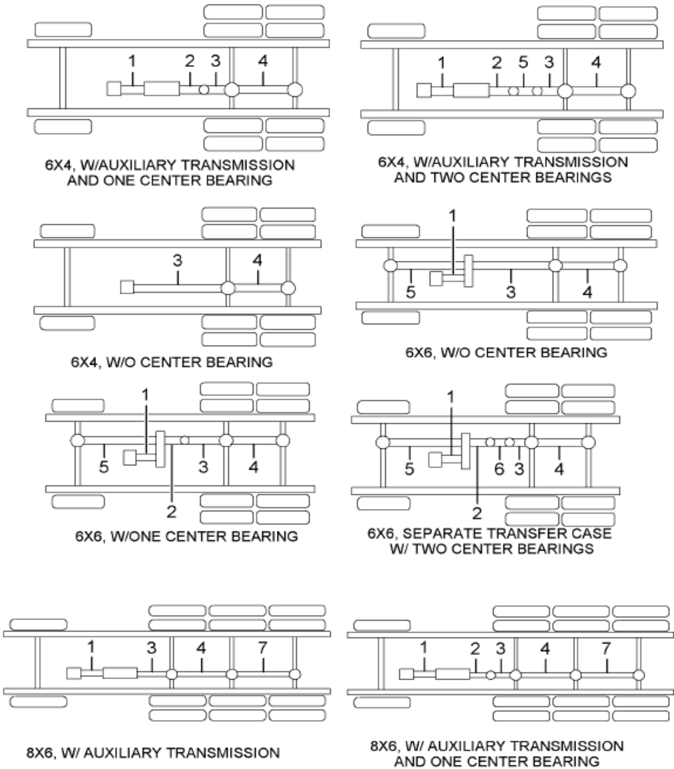
Figure 429DTHXXX DRIVESHAFT ASSY, 1810 SERIES M
