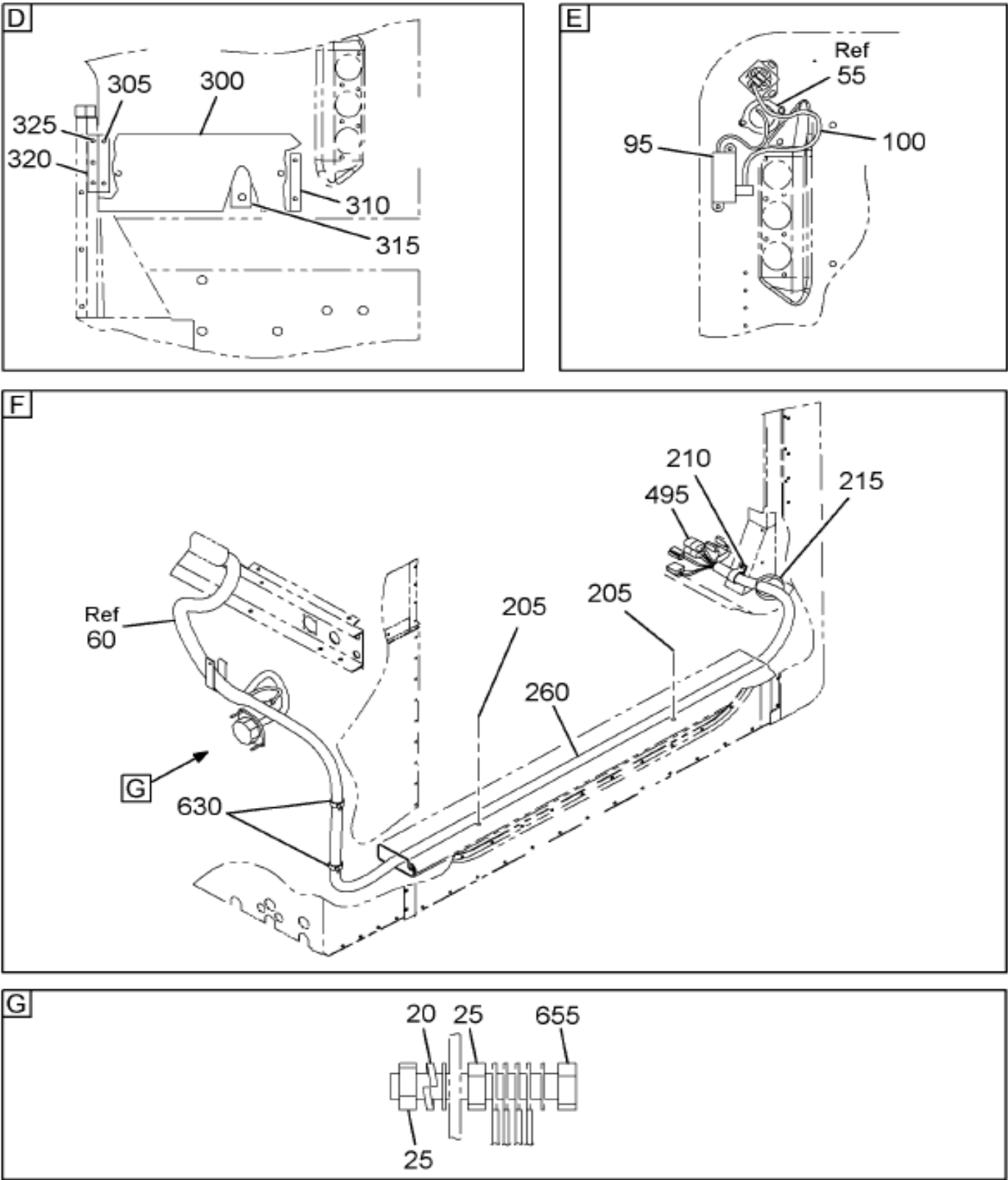
https://truckmanualshub.com/ Figure 0NQG9 MAIN CAB WIRING W/TRUCK, GLIDERS, TRIM...
