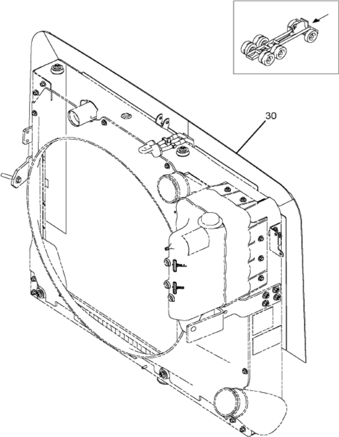
https://www.manualshub.com/ Figure 0NV9J AIR RECIRCULATION SEALS (ABR #6)
