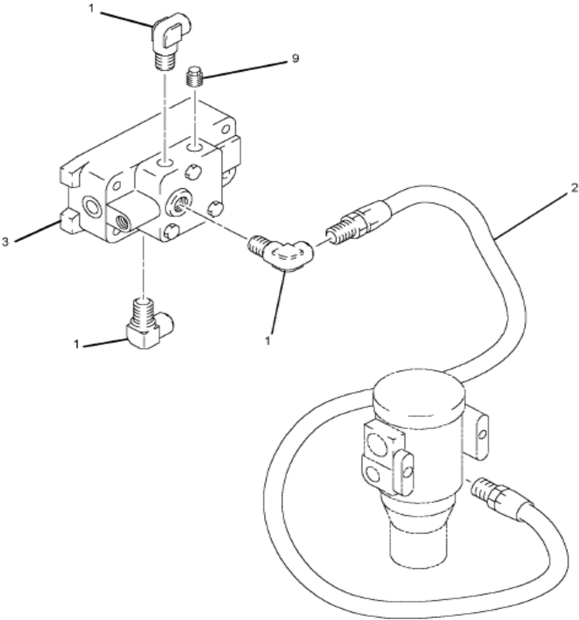
SLAVE VALE ASSEMBLY
