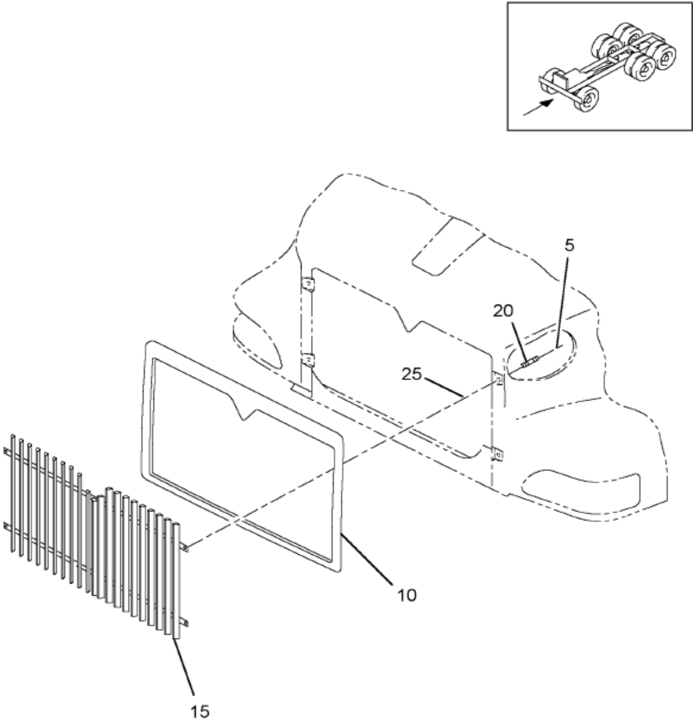
Figure 02L73 GRILLE INSTL; FRONT
