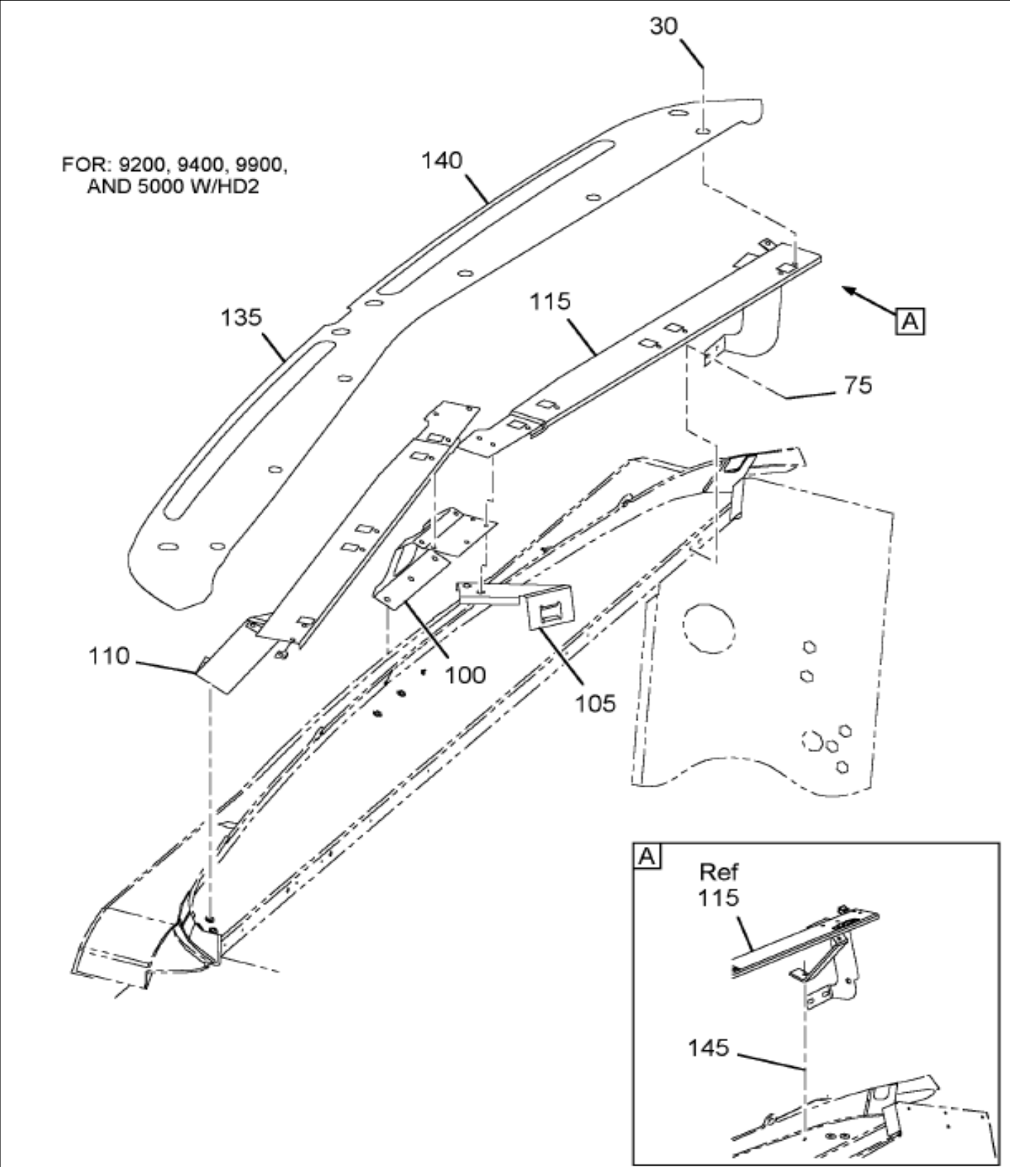
Figure 0GWWW INSTRUMENT PANEL INSTL
