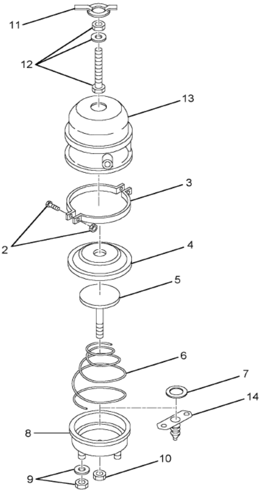
Figure 1688941C91 CHAMBER, BRAKE
