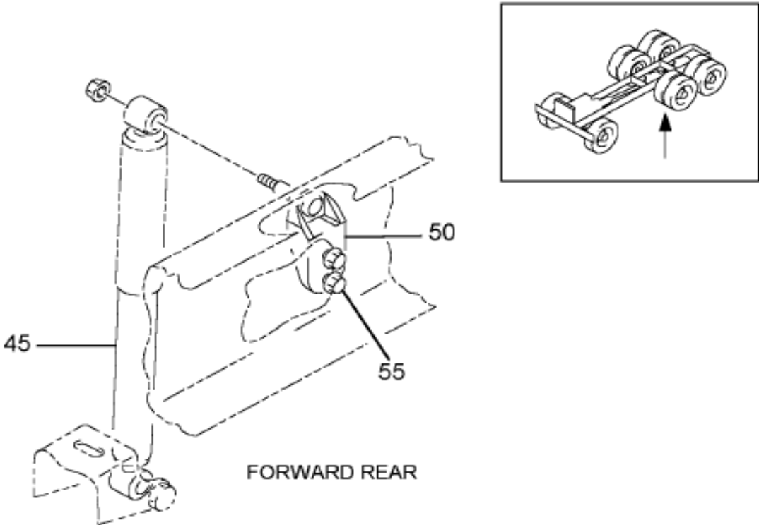
https://truckmanualshub.com/ Figure 02/25 SHOCK ABSORBER & MTG
