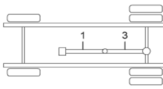
4X2, W/ ONE CENTER BEARING
