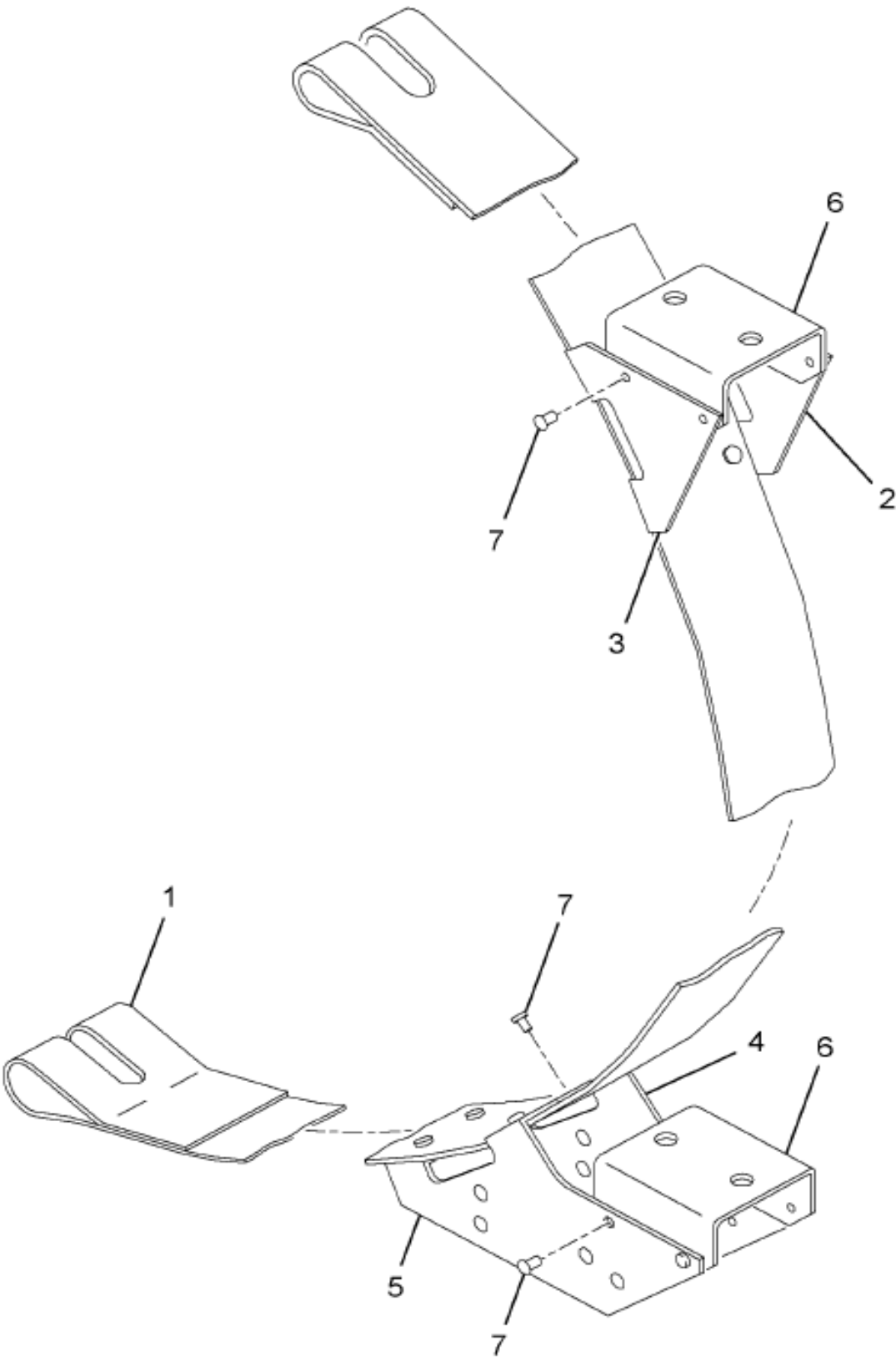
Figure 3566134C1 STRAP, FUEL TANK MTG*
