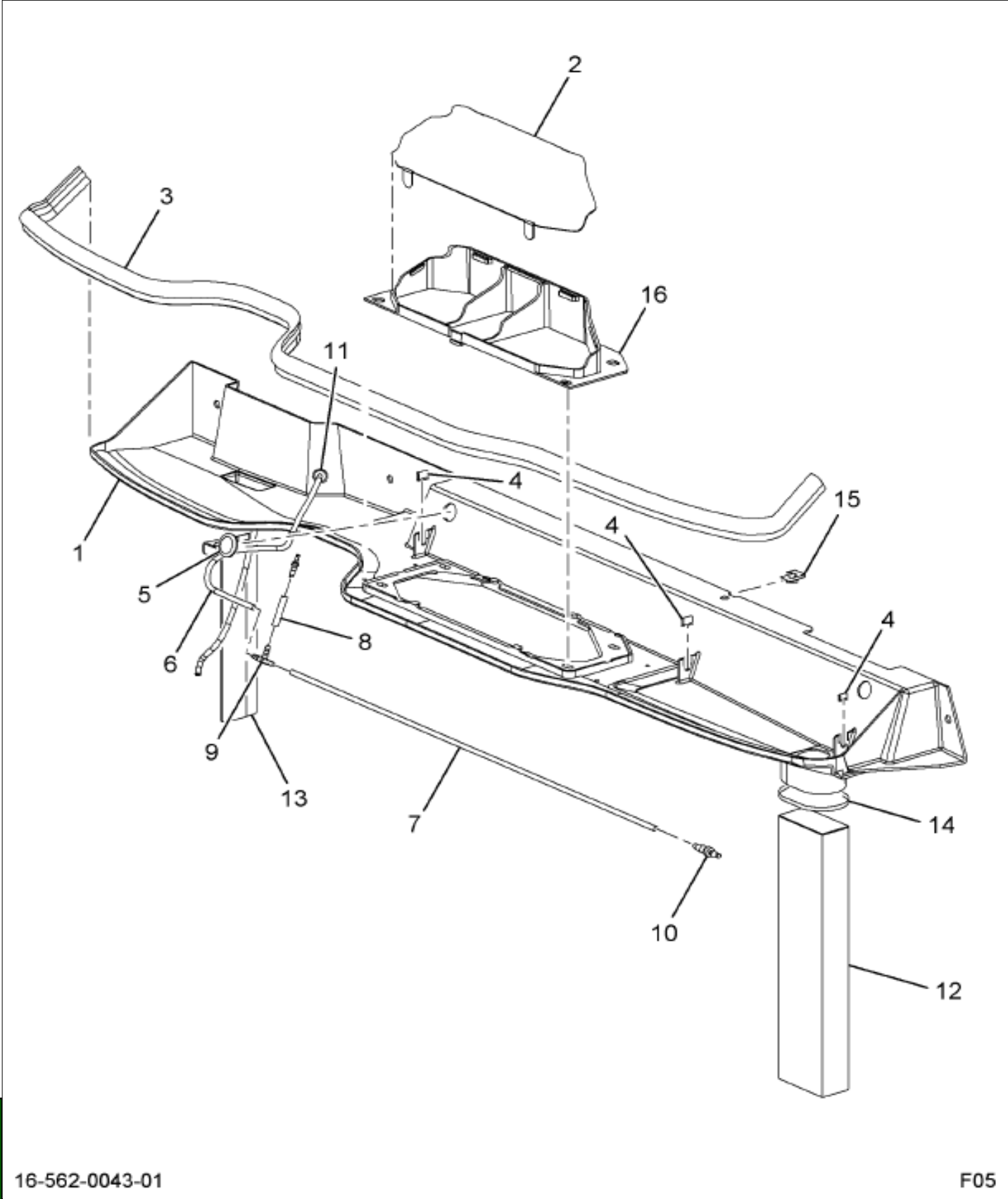
Figure 3571812C92 BAFFLE,ASM MTR CVR COWL TRAY
