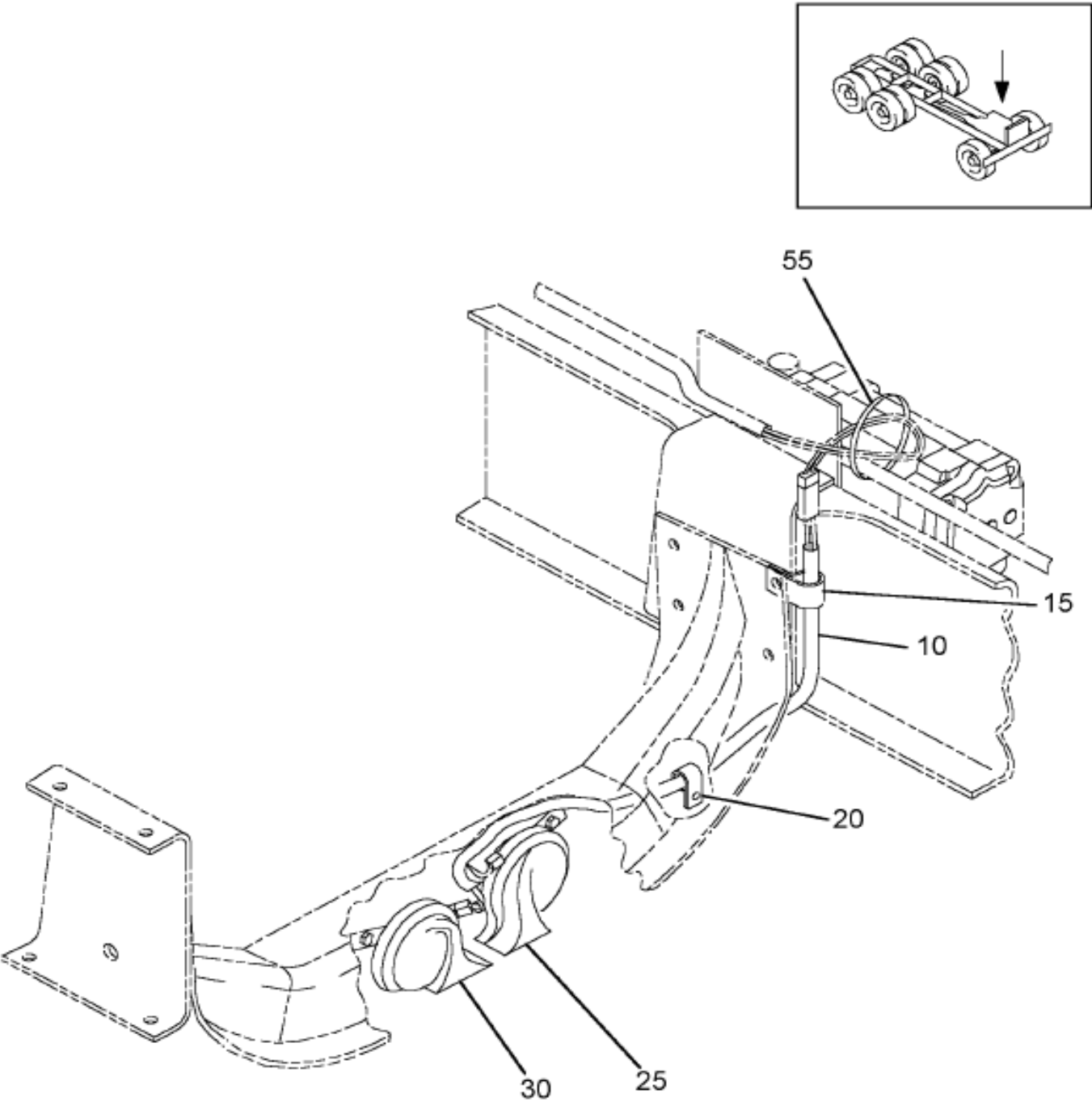
https://truckmanualshub.com/ Figure 0HTFW ELECTRIC HORN WIRING
