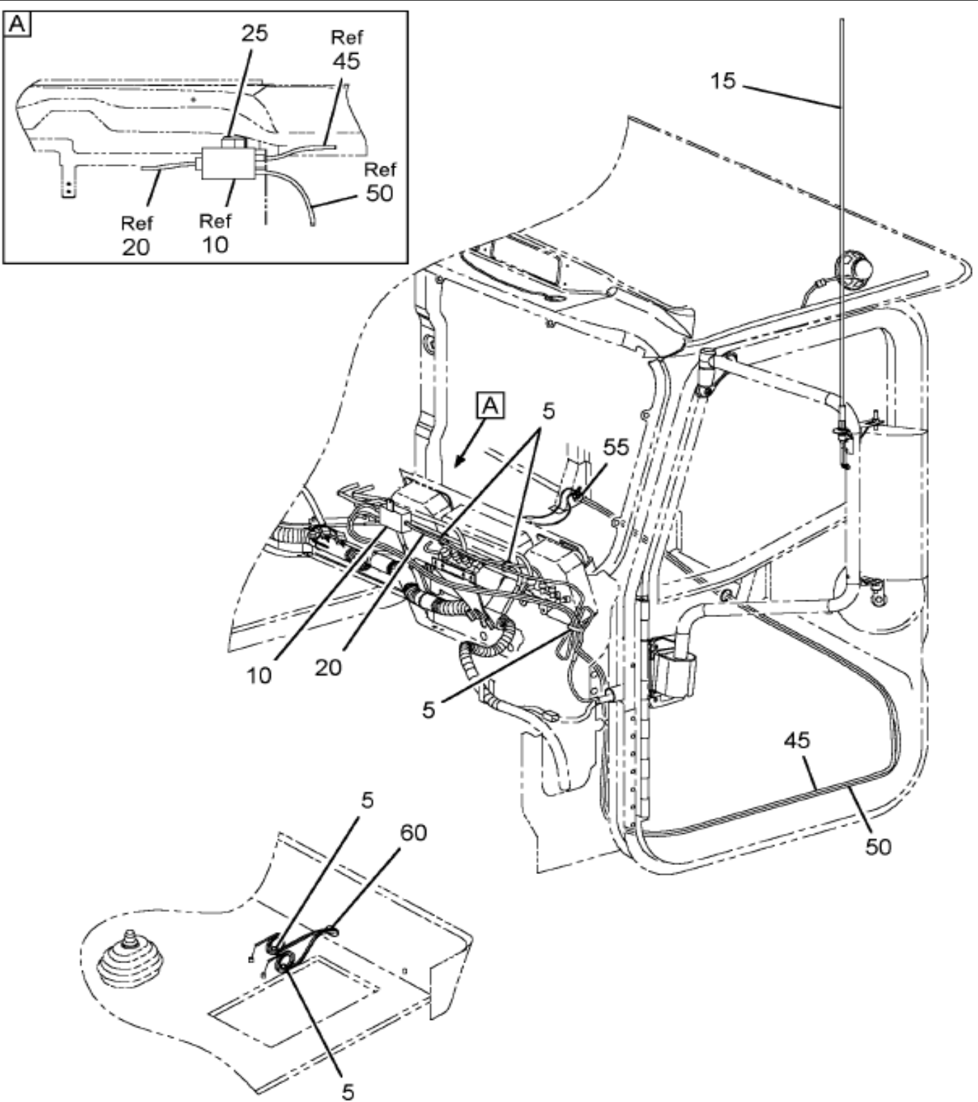
https://truckmanualshub.com/ Figure 05MW0 CB ANTENNA CABLE INSTL
