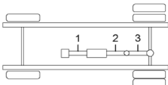
4X2, W/ AUXILIARY TRANSMISSION AND ONE CENTER BEARING
