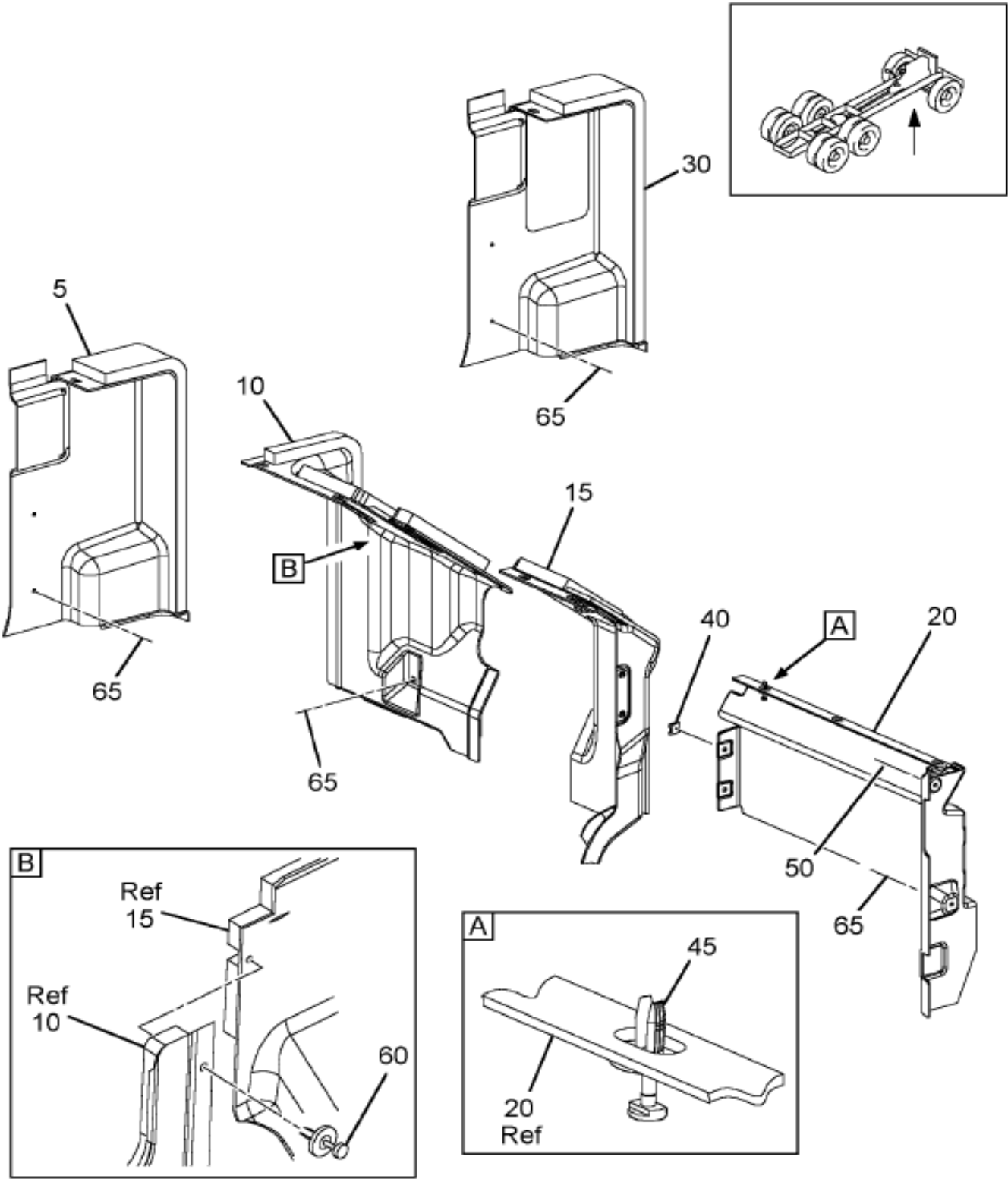
https://truckmanualshub.com/ Figure 0GW9Q DASH INSULATOR PANEL INSTL
