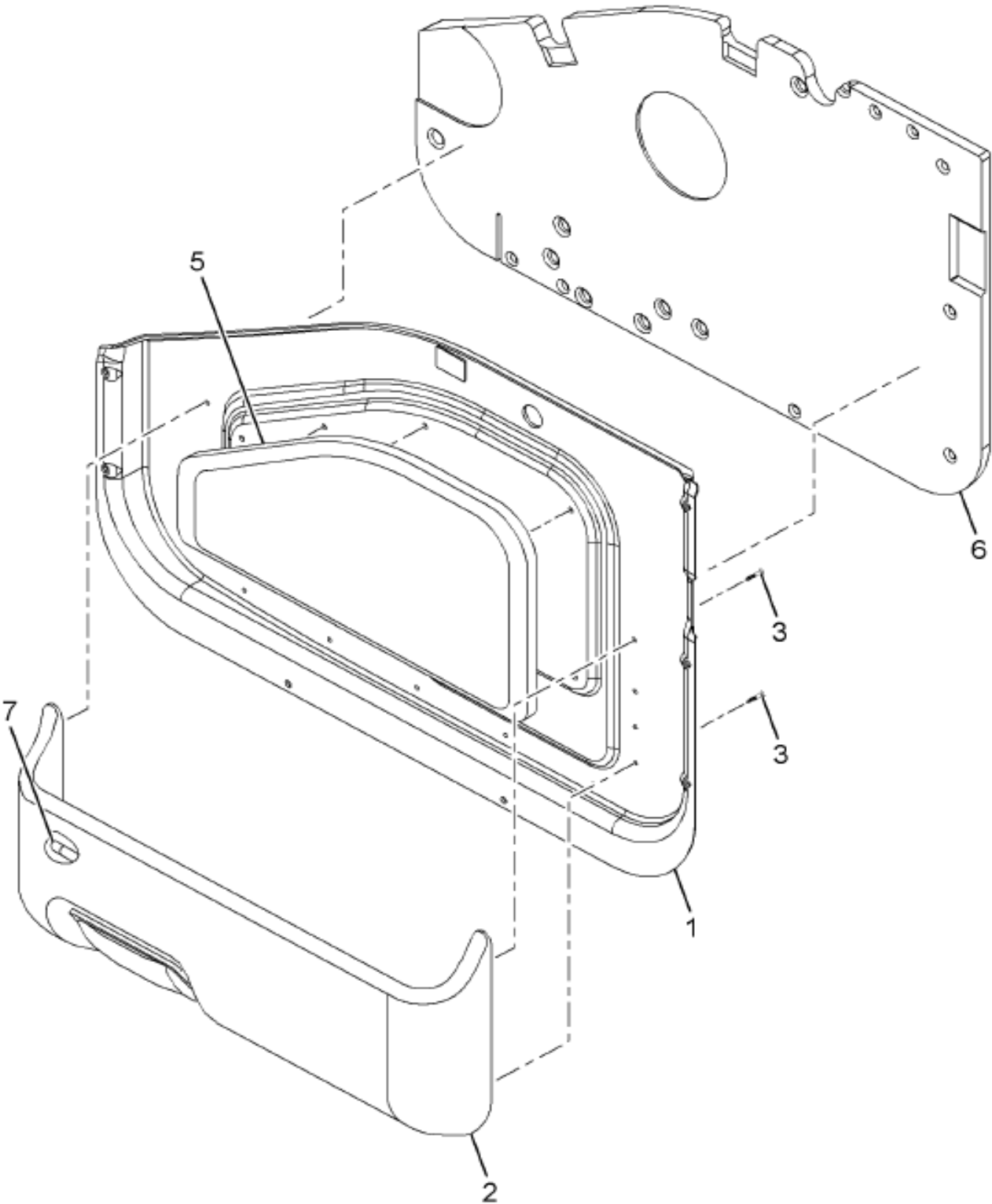
https://truckmanualshub.com/ Figure 3579489C92 PANEL, ASY-LWR LH DARK TAN-DOOR
