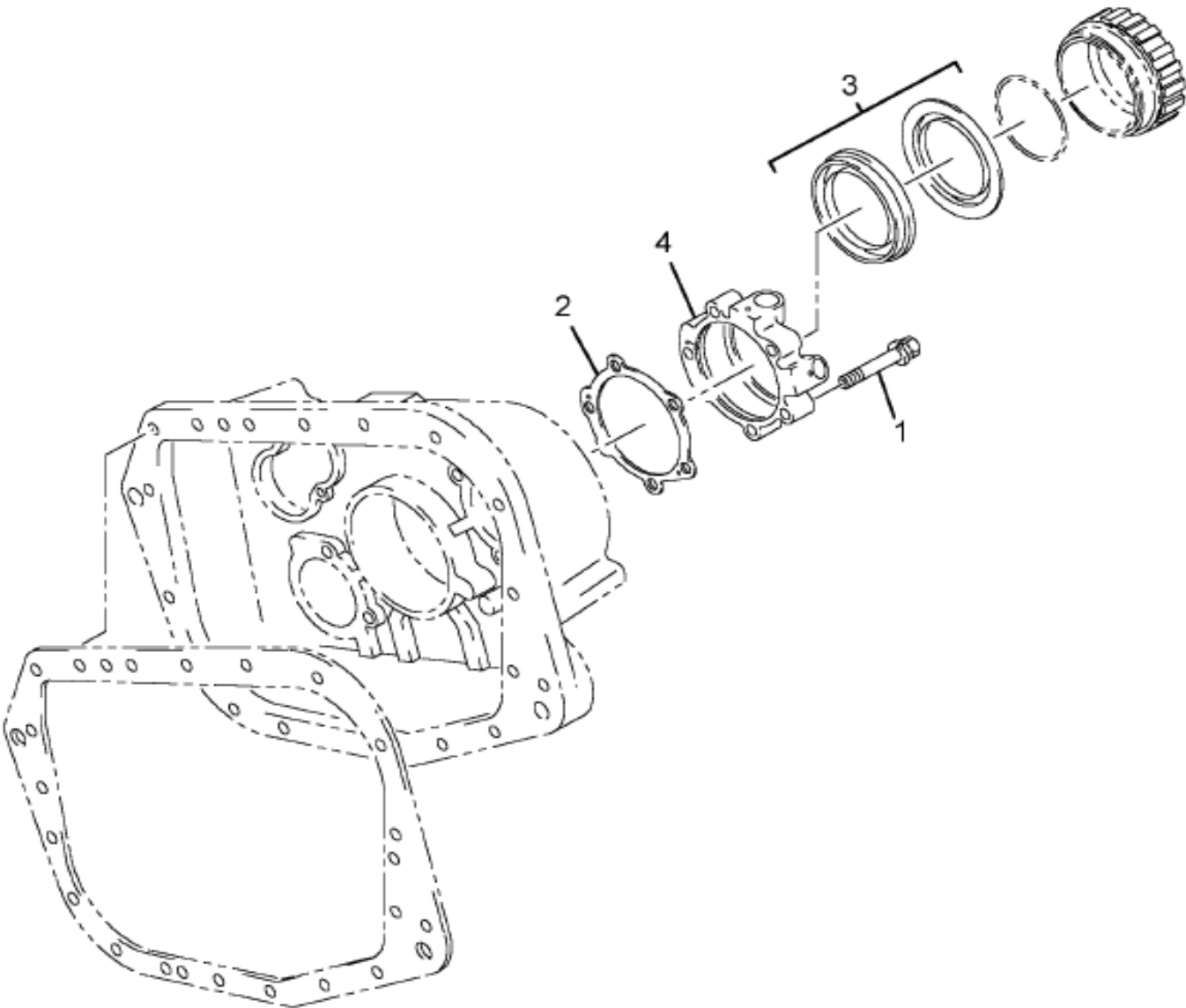
AUXILIARY HOUSING ASSEMBLY
