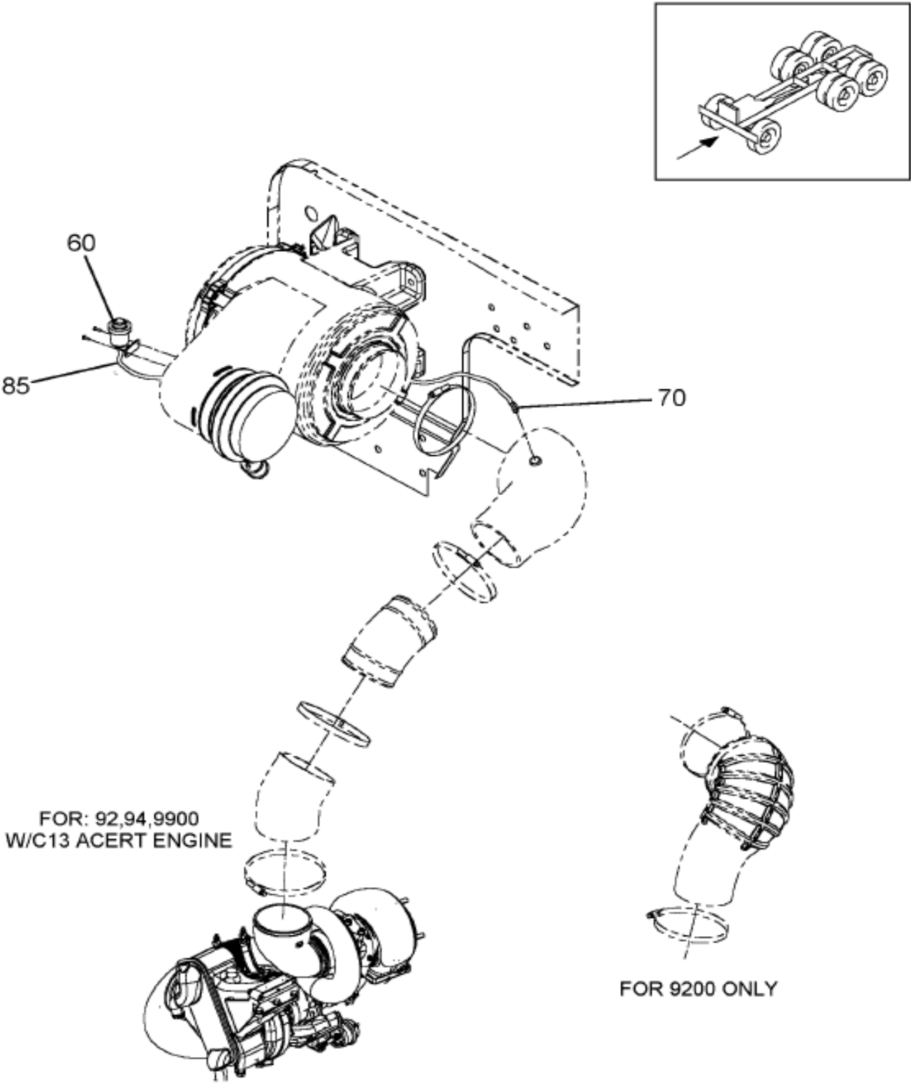
Figure 0MV9H AIR RESTRICTION GAUGE INSTL
