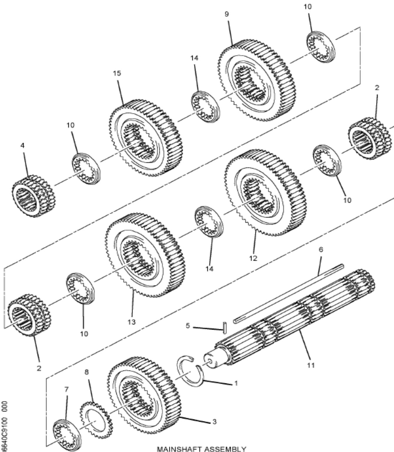
https://truckmanualshub.com/ Figure 2506640C91 SHAFT, ASSY TRANS MAIN
