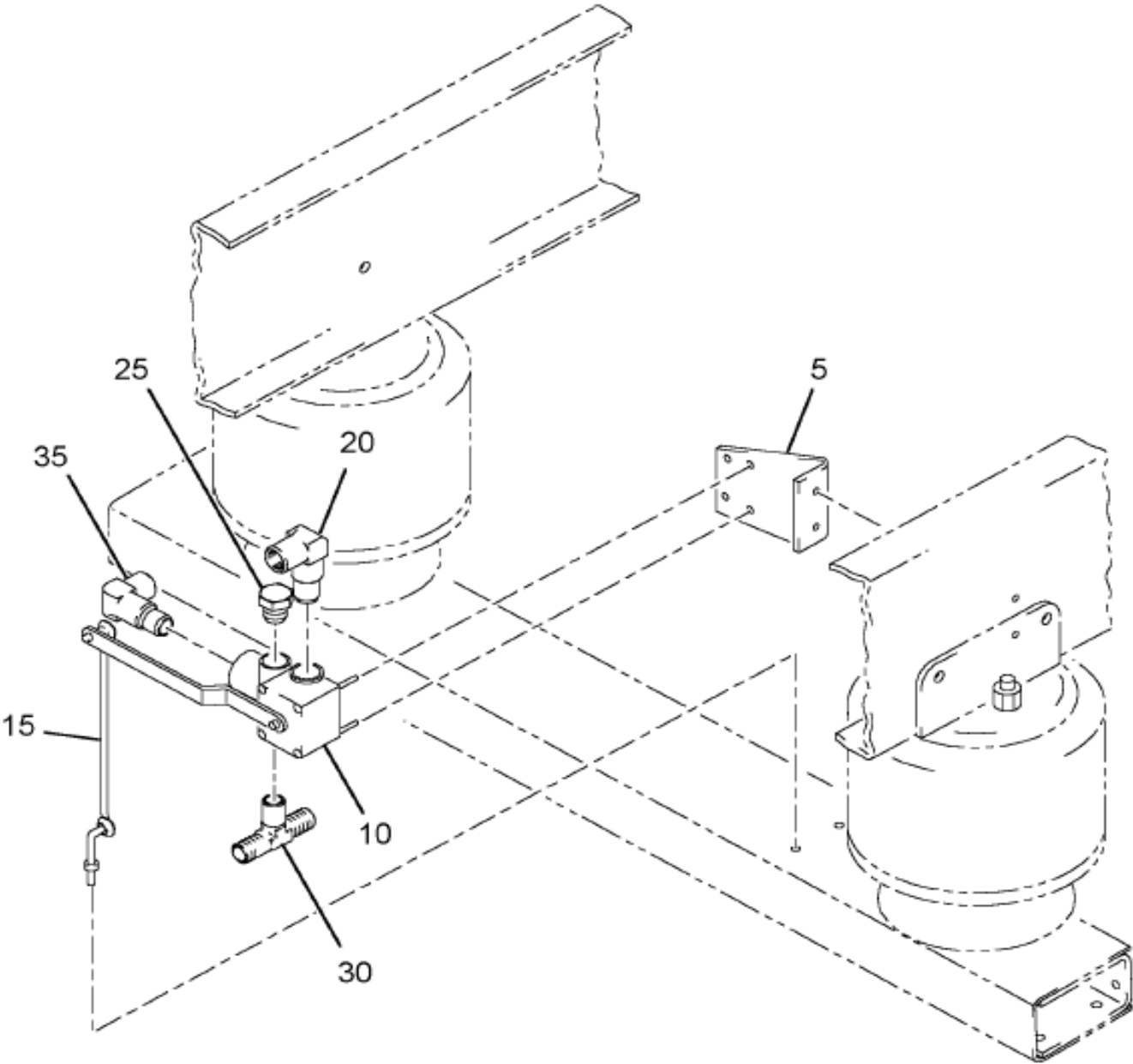
INTERNATIONAL SUSPENSION SINGLE HEIGHT CON VALVE W/14673, 14693, 14694, 14TAN
