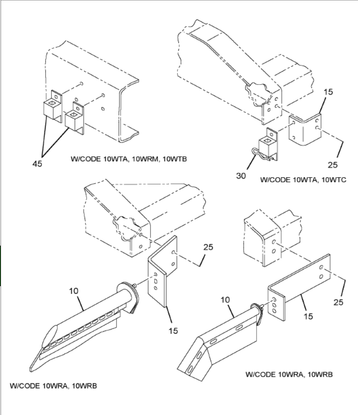
https://www.manualshub.com/ Figure 04P9C MUD FLAP SUPPORT & MTG, REAR
