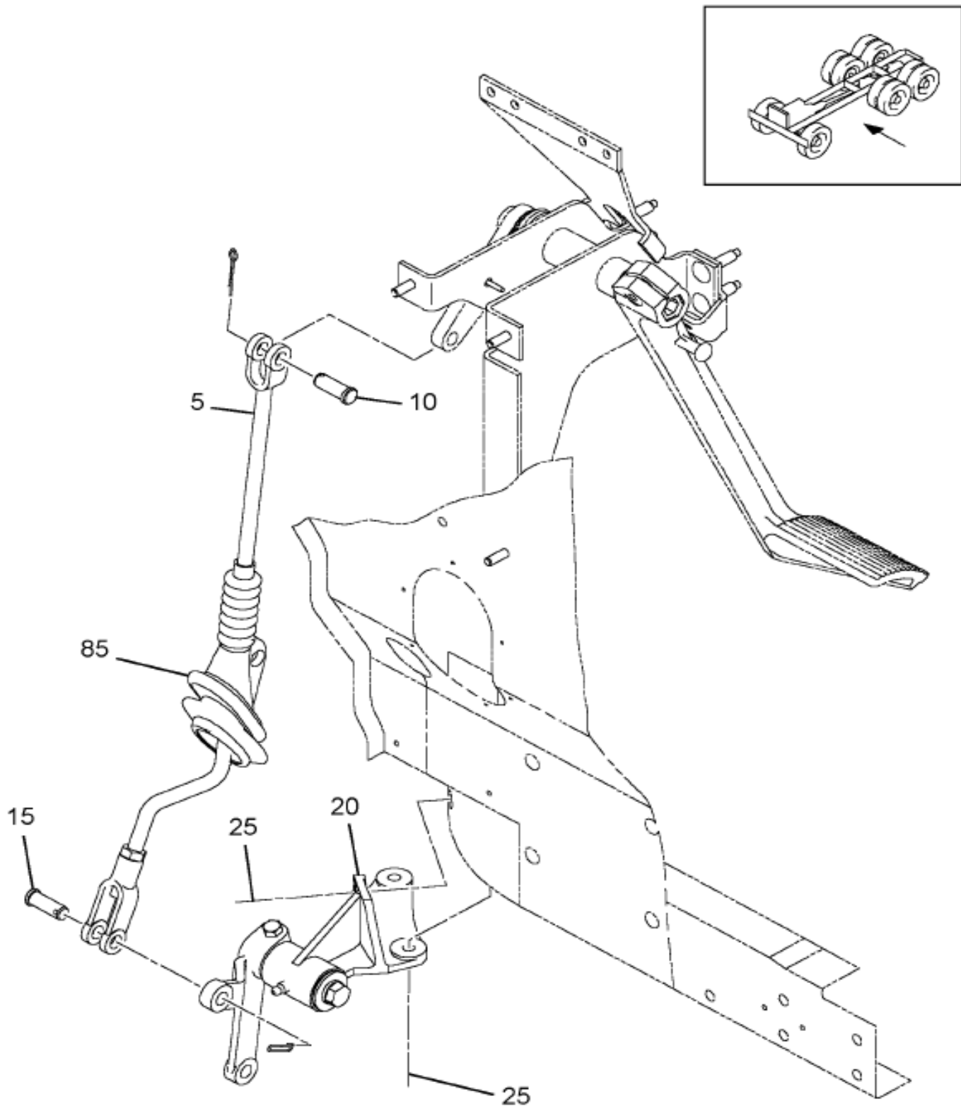
https://truckmanualshub.com/ Figure 00TH CLUTCH CONTROL, UPPER
