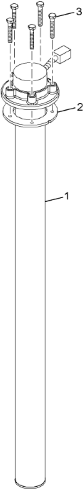
https://truckmanualshub.com/ Figure 3596382C91 GAUGE, FUEL SENDER, 26" DEEP TA
