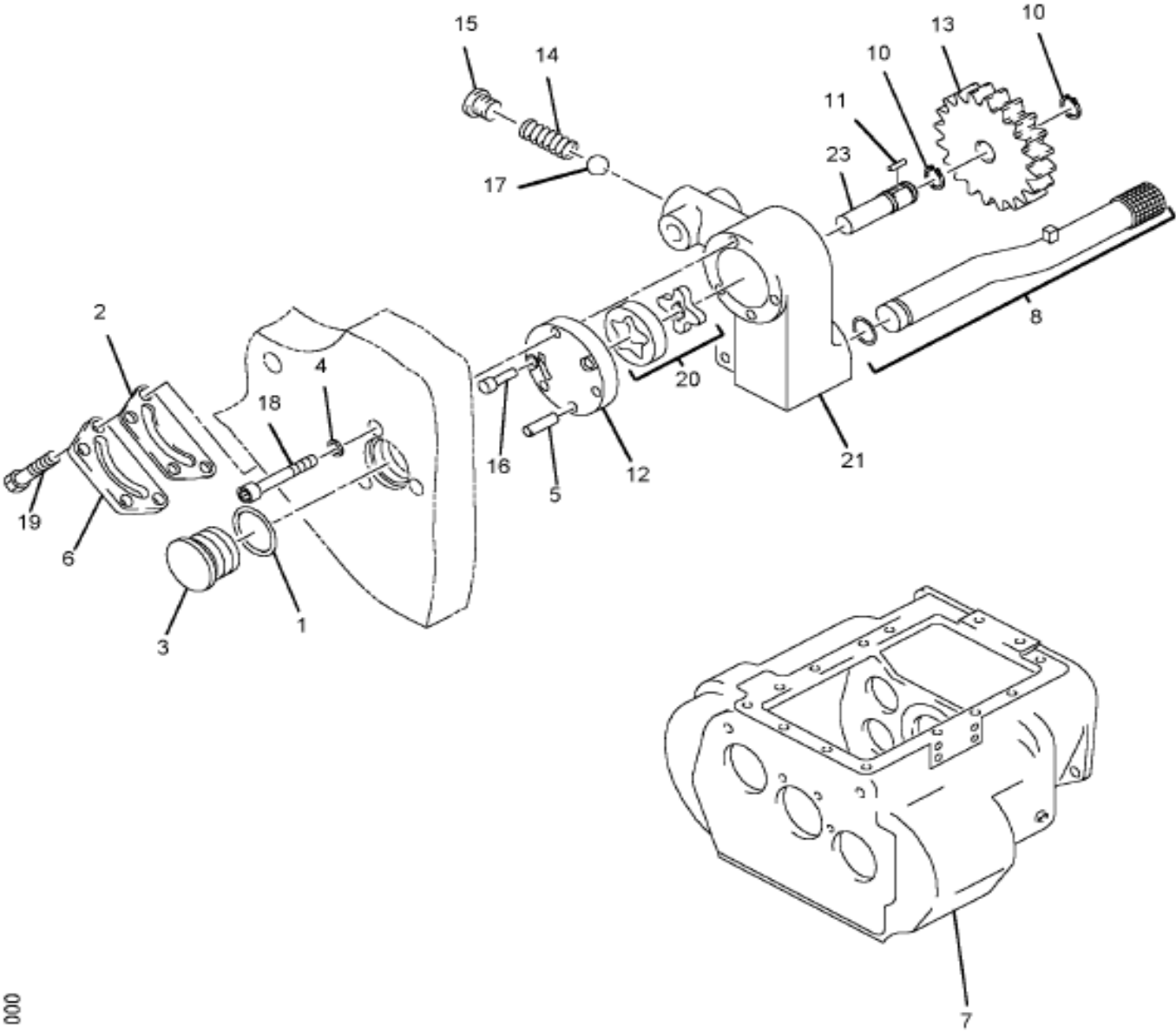
INTEGRAL OIL PUMP ASSEMBLY
