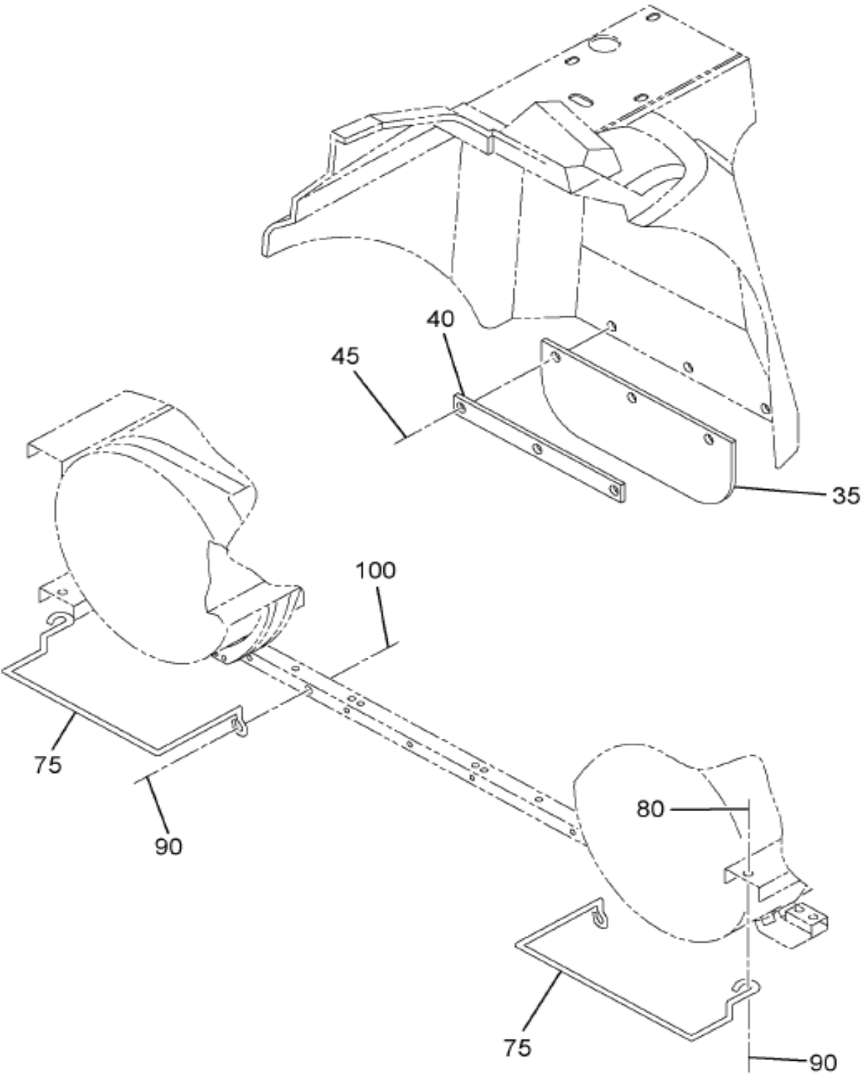
https://manualshub.com/ Figure 02MSC MUD GUARD INSTL, W/SPLASH FENDER
