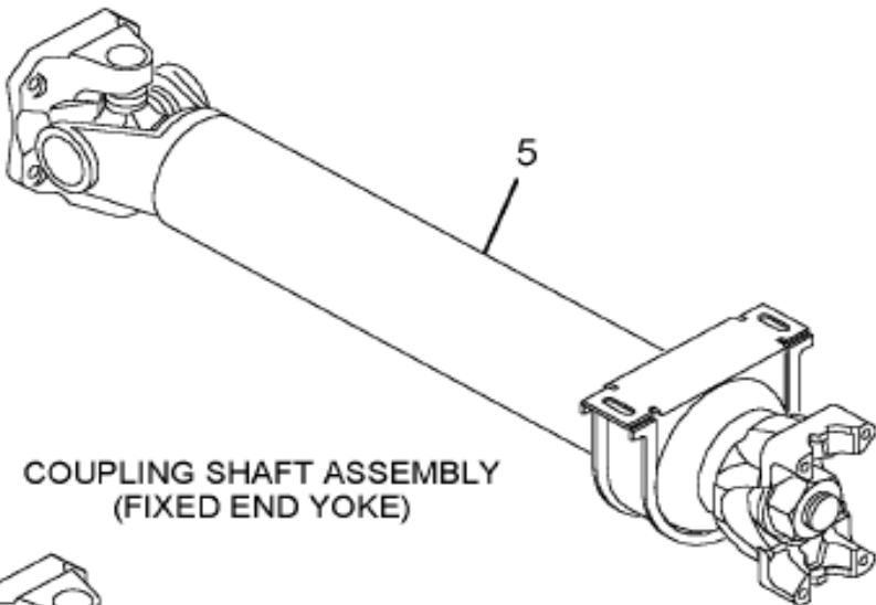
SHORT COUPLED DRIVESHAFT
