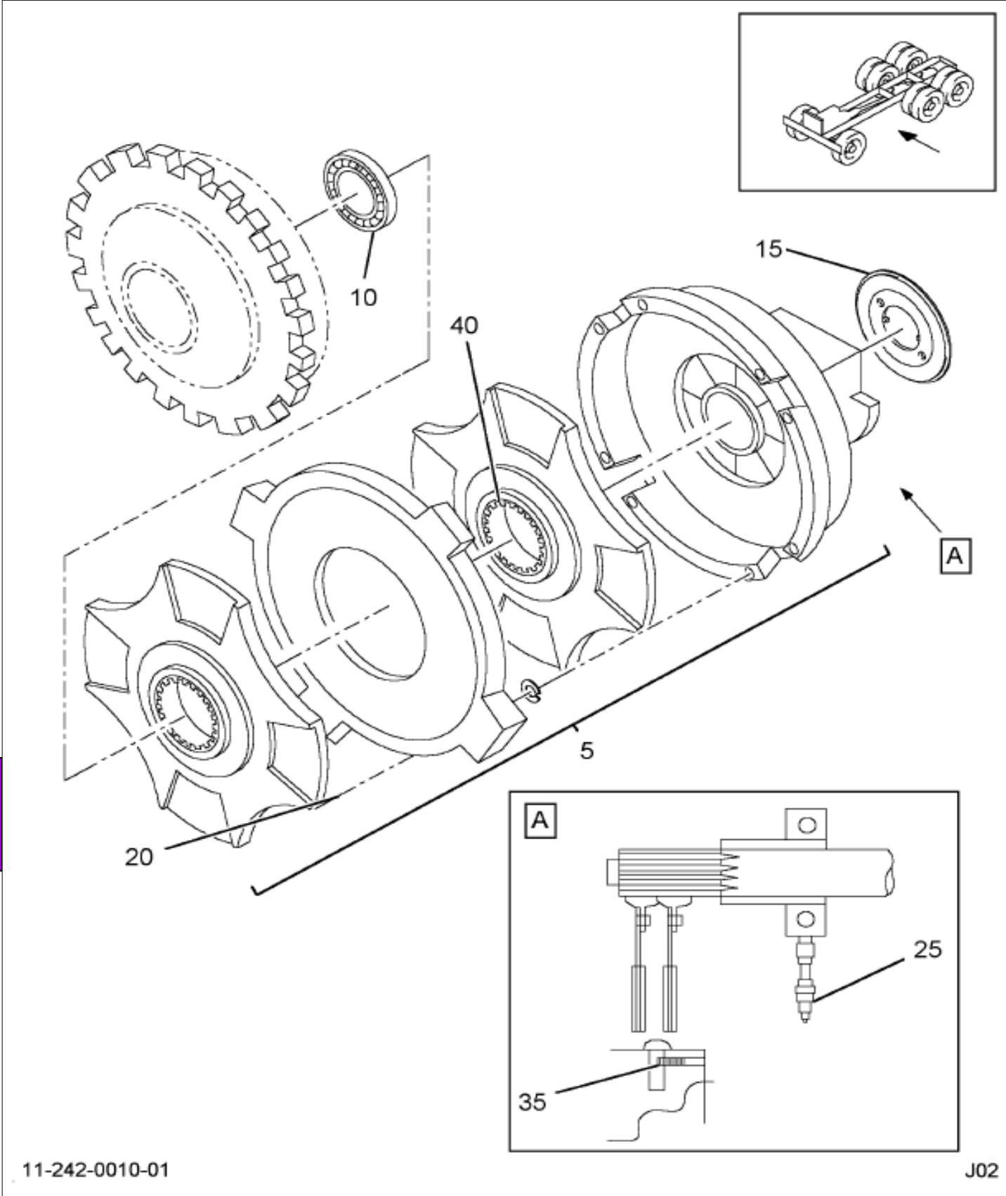
https://workmanualshub.com/ Figure 00V19 CLUTCH INSTL; SPICER
