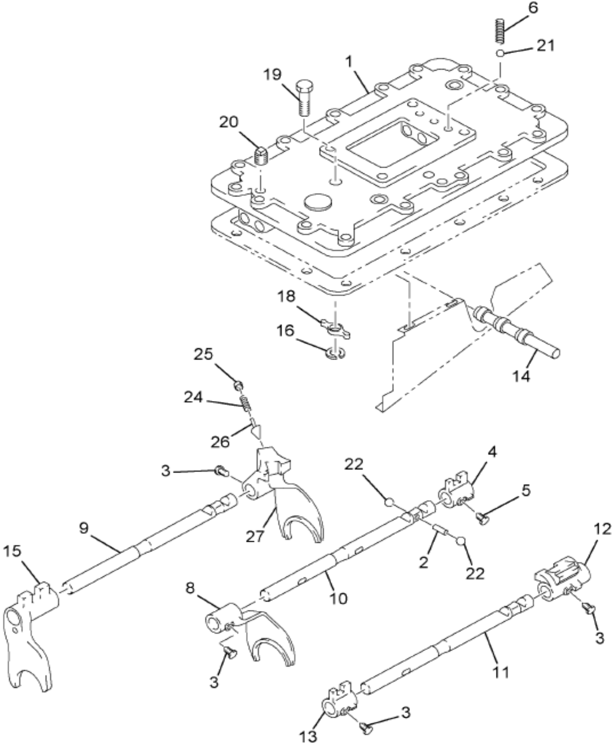
SHIFT BAR HOUSING ASSEMBLY
