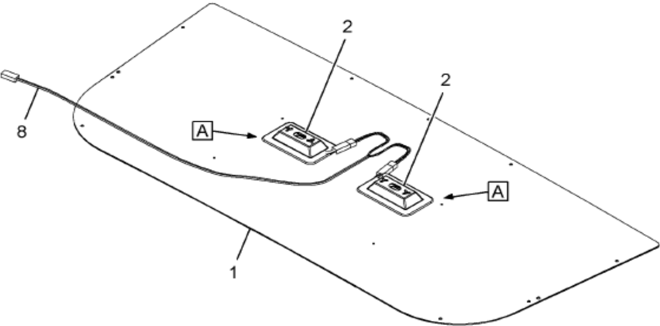
https://truckmanualshub.com/ Figure 3570329C91 LINING,HD RF TRM MED TAN DYCAB
