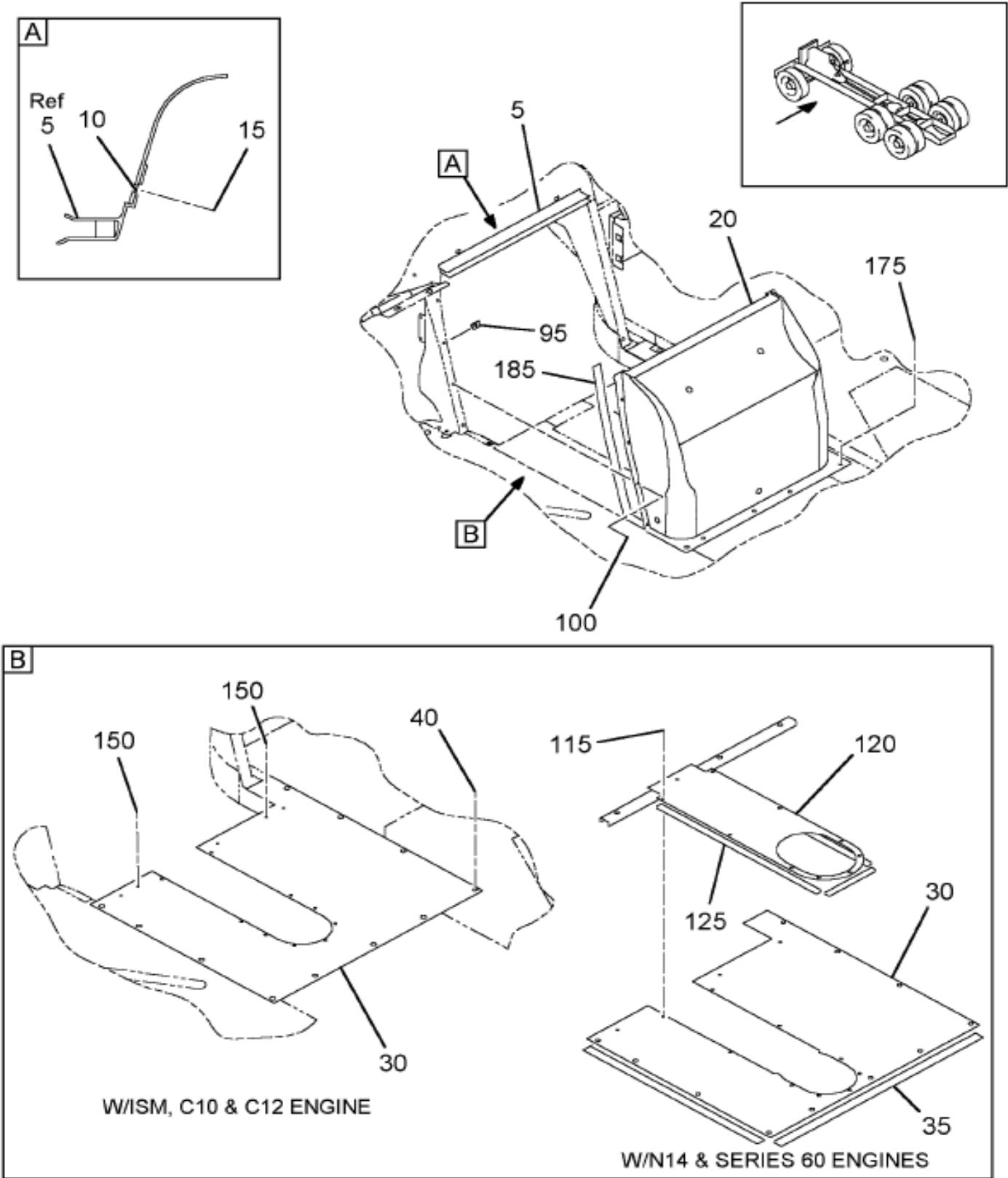
Figure 0HB3W COVER INSTL, ENGINE & TRANS
