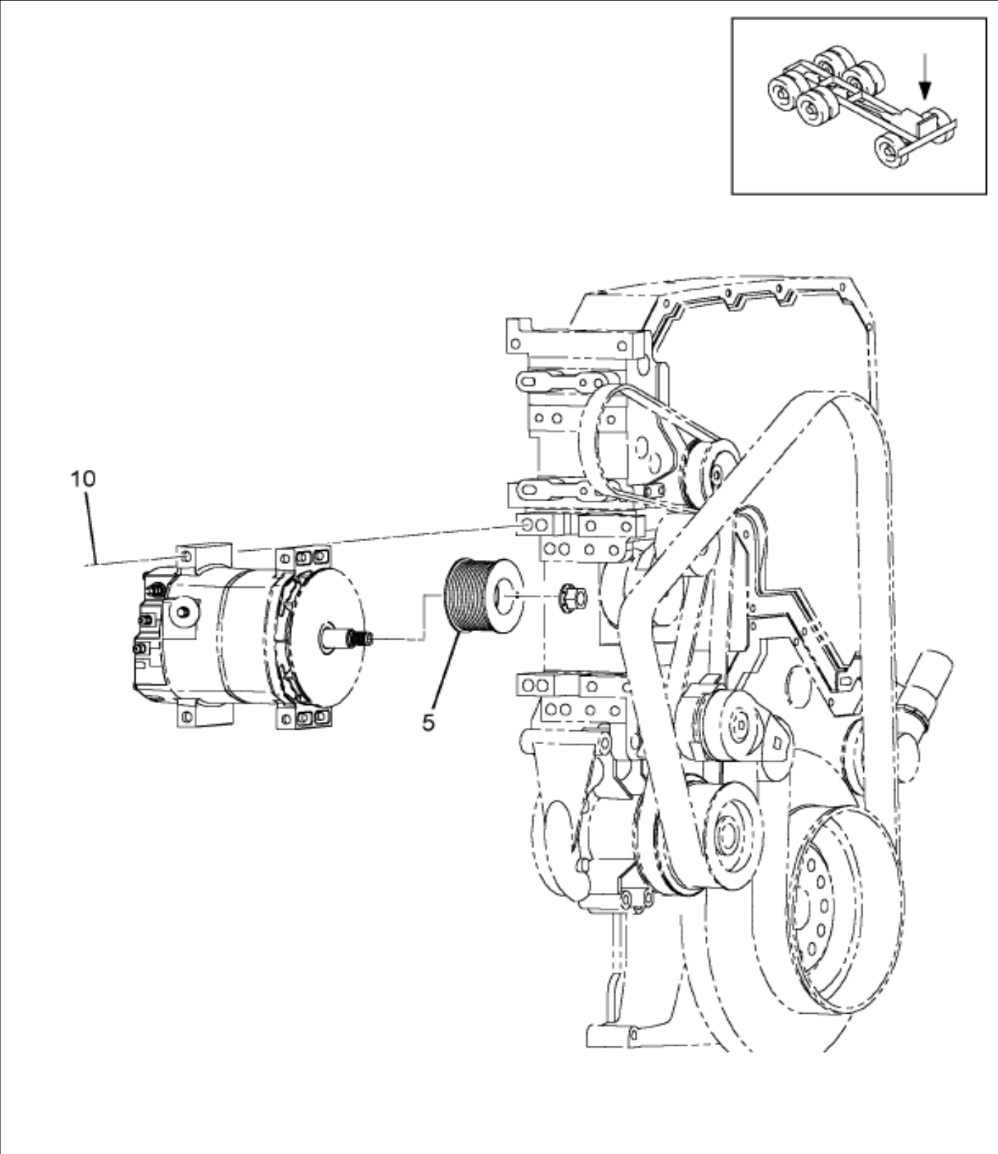
Figure 08-664-0018-BA ALTERNATOR PULLEY & MTG; W/CUM ISX ENG
