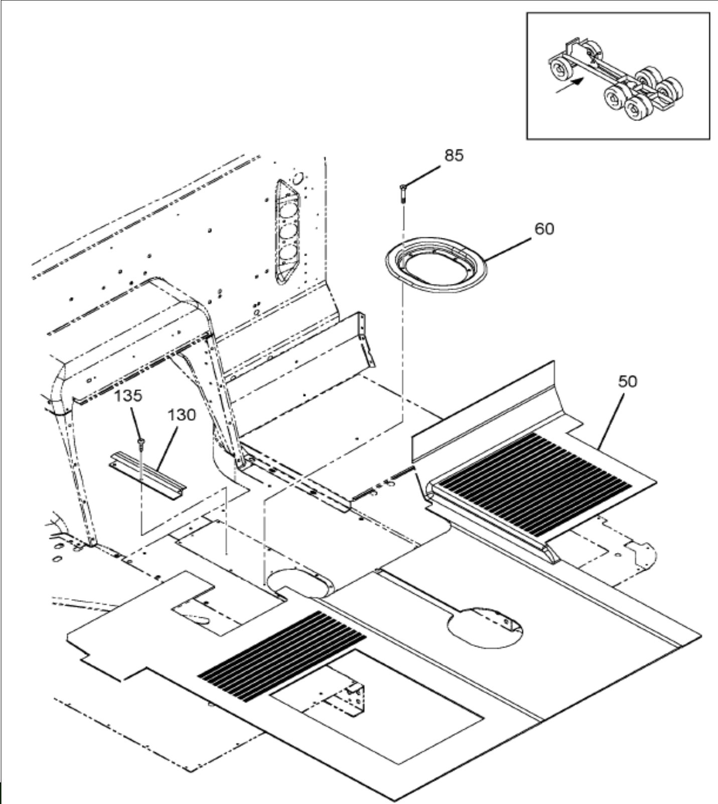
https://www.manualshub.com/ Figure 0HB62 FLOOR MAT INSTL
