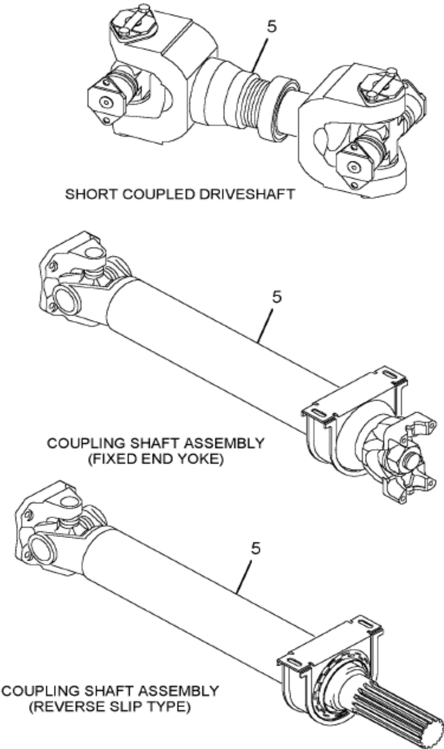
https://truckmanualshub.com/ Figure 01ZDG PROP SHAFT 1710 SERIES
