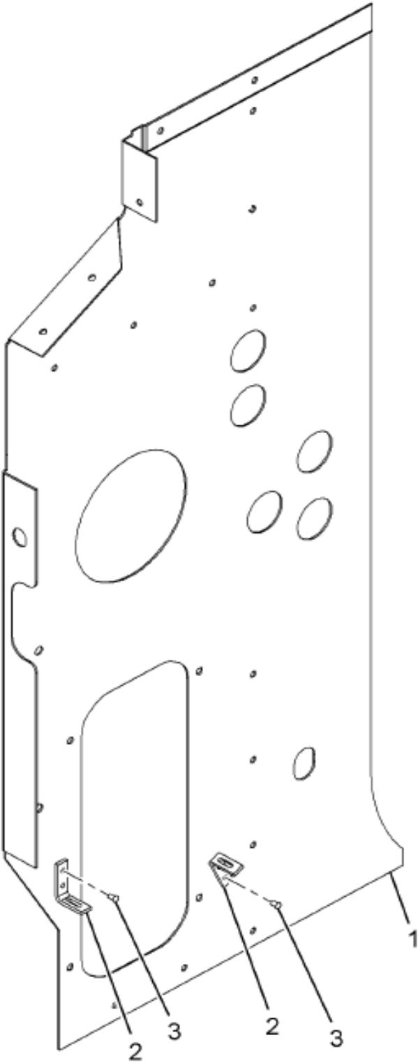
Figure 3527990C3 PANEL, COWL INR RH W/ DUCT OPNG
