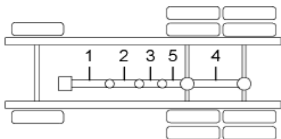
6X4, W/THREE CENTER BEARINGS
