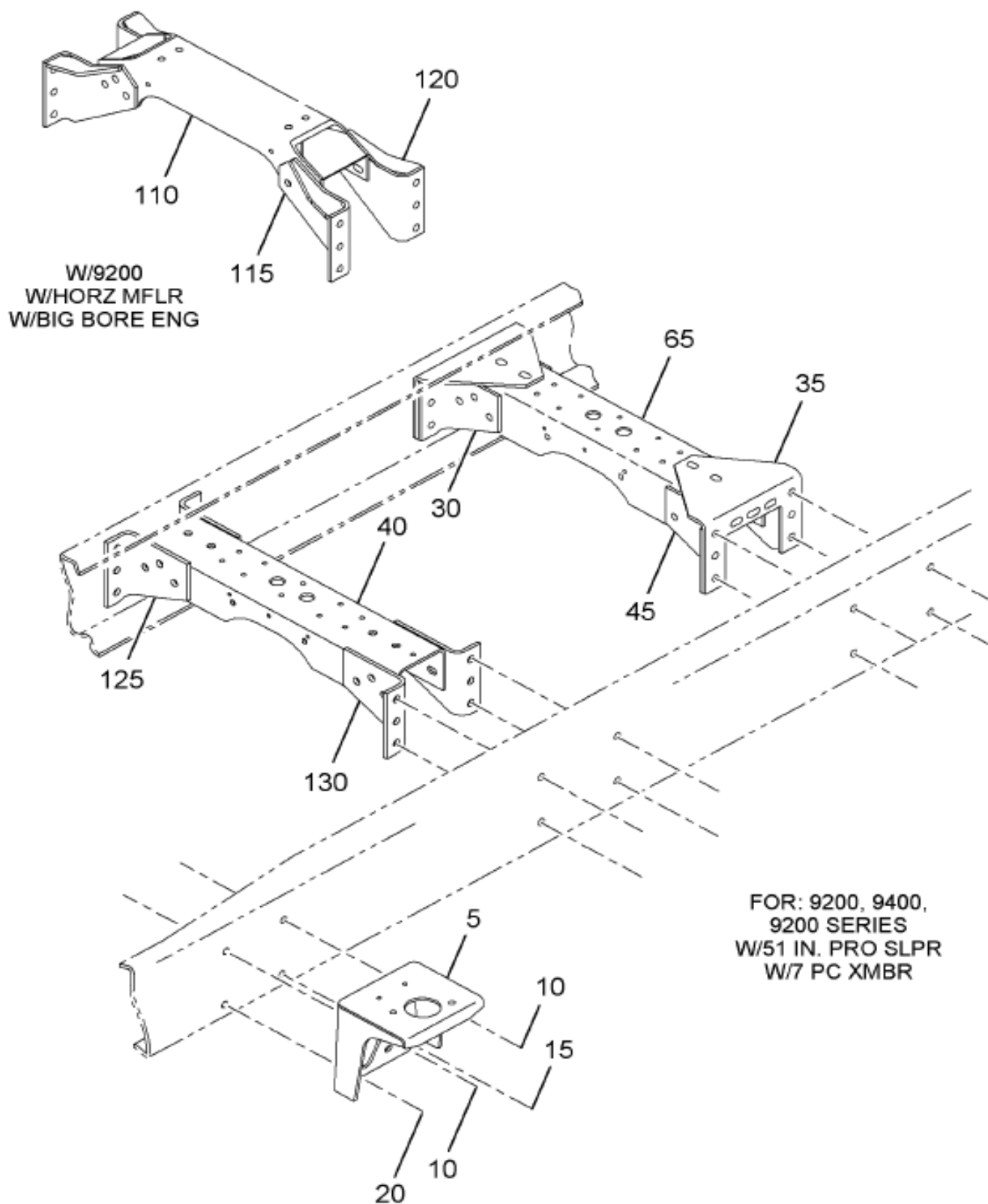
Figure 00B9Q CAB MTG
