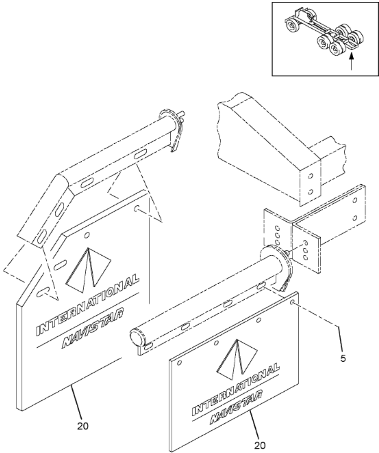
https://truckmanualshub.com/ Figure 04QLY MUD FLAP INSTL; REAR
