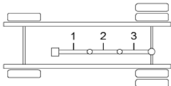
4X2, W/ TWO CENTER BEARINGS
