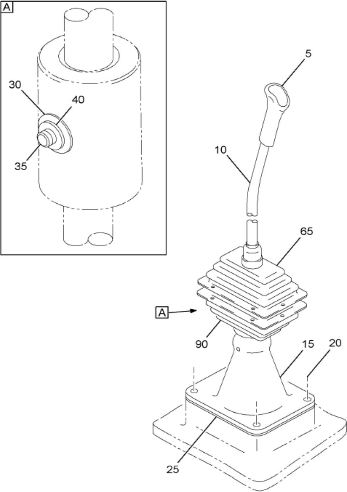
https://trucksmanualshub.com/ Figure 02G6J CNTRL ASM, TRANS SHIFT
