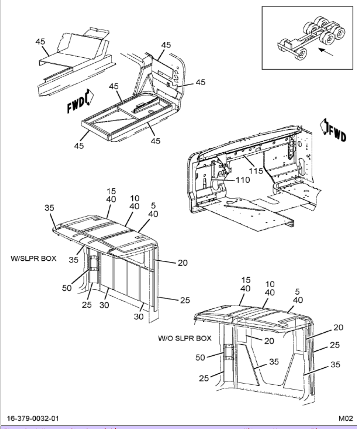
Figure 052ZR INSULATOR INSTL, CAB
