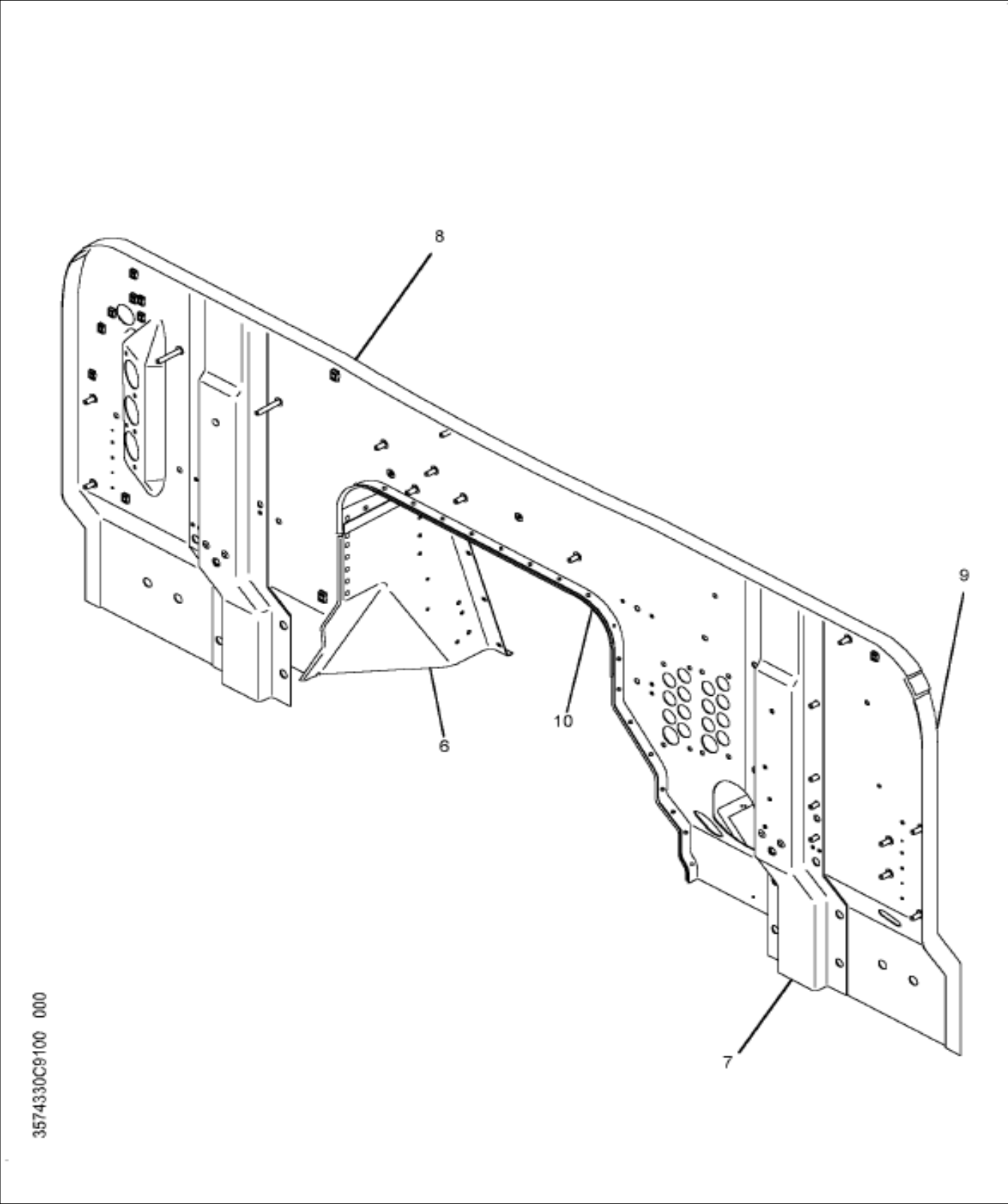
https://truckmanualshub.com/ Figure 3574330C91 PANEL, DASH ASSY COMPLETE
