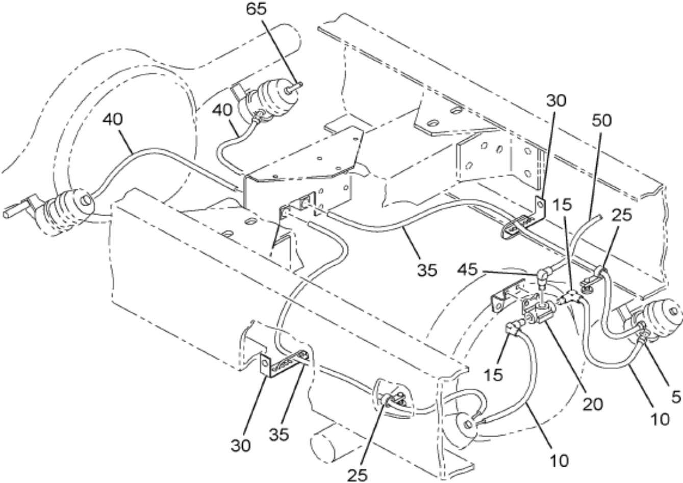
W/HEND AIR SUSP W/REYCO SUSP W/CODES 04AZC, 04AZD, 04AZK
