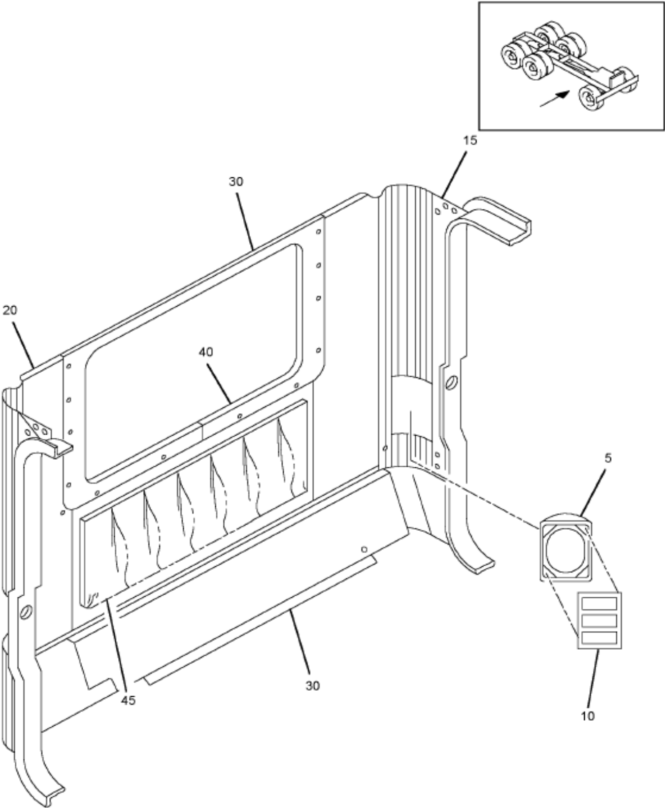
https://truckmanualshub.com/ Figure 0HC14 BACK PANEL & TRIM; DAY CAB
