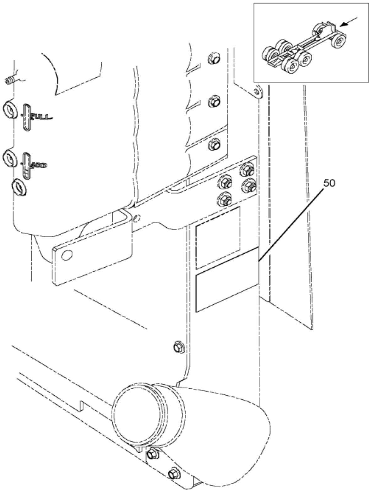
Figure 01V97 PRODUCT GRAPHIC; FAN DRIVE
