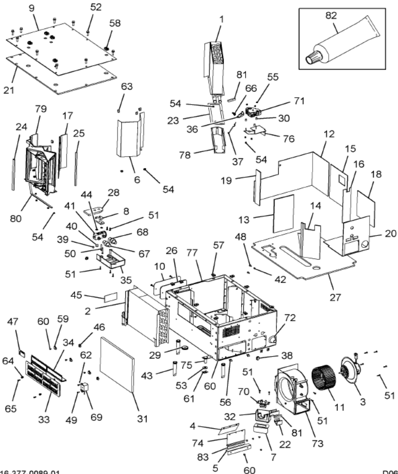
Figure 3517455C95 HEATER, A/C DAY CAB
