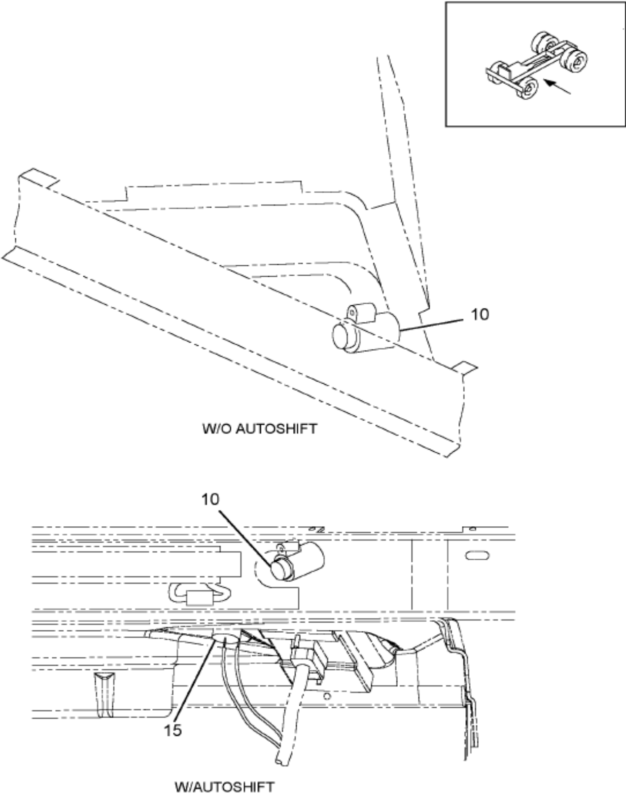
Figure 02QDC LIGHTER INSTL; CIGARETTE
