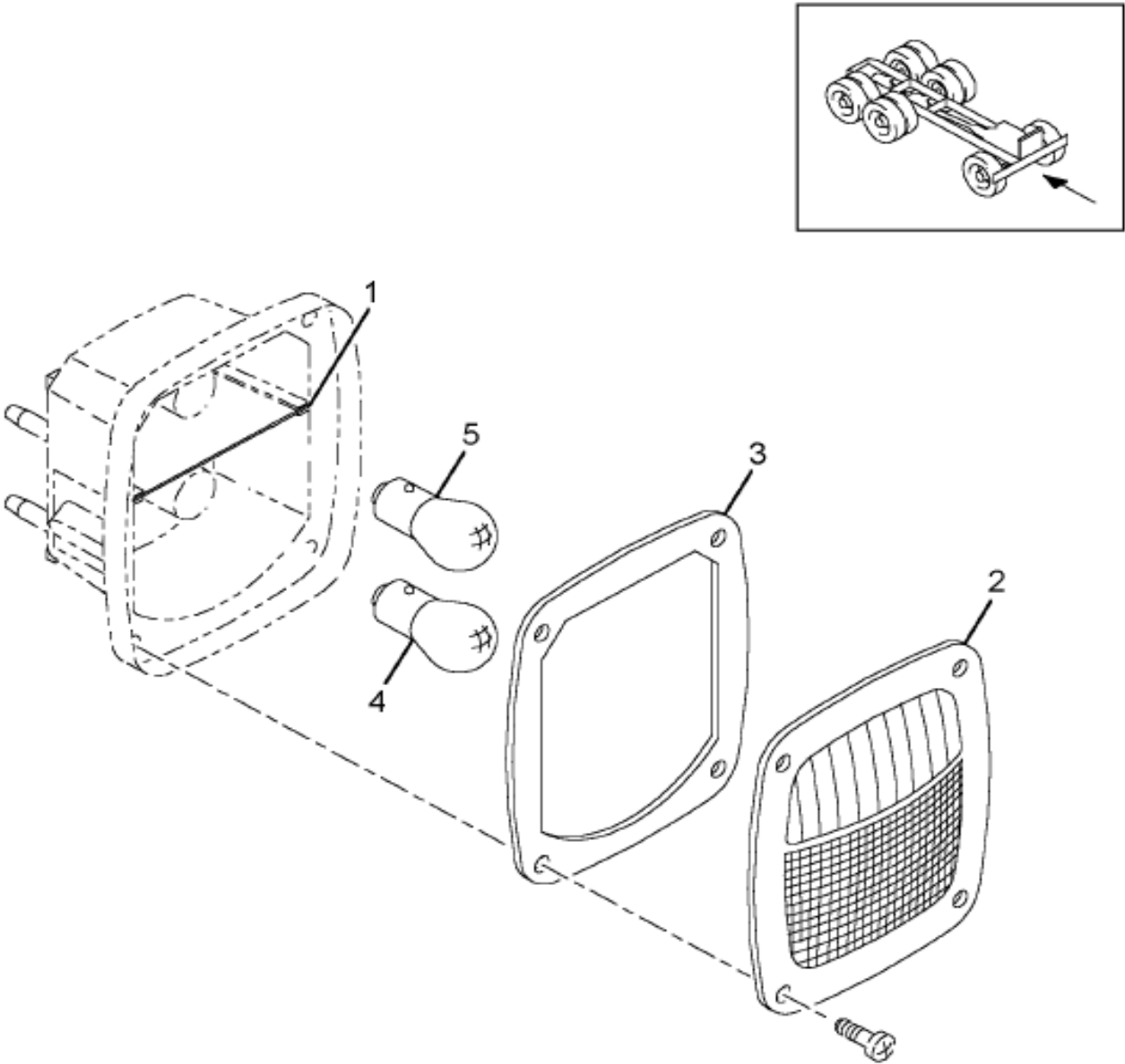
Figure 1661262C91 LIGHT, ASSY STOP TAIL TURN WITH
