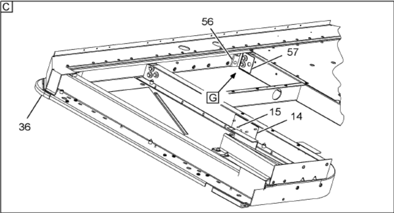
Figure 3547334C96 UNDERBODY, ASM DAYCAB
