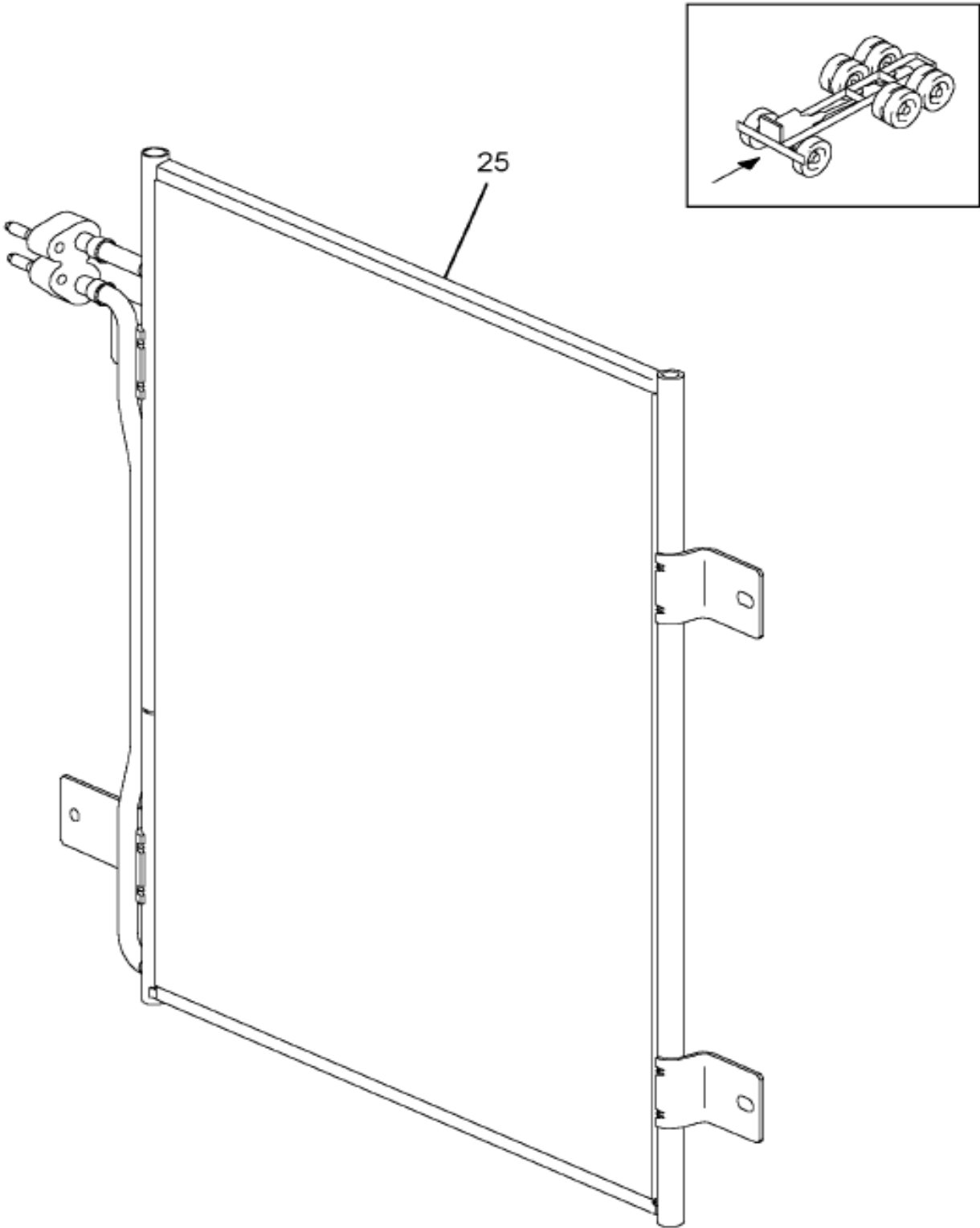
https://www.manualshub.com/ Figure 0NV93 A/C CONDENSER (ABR #5)
