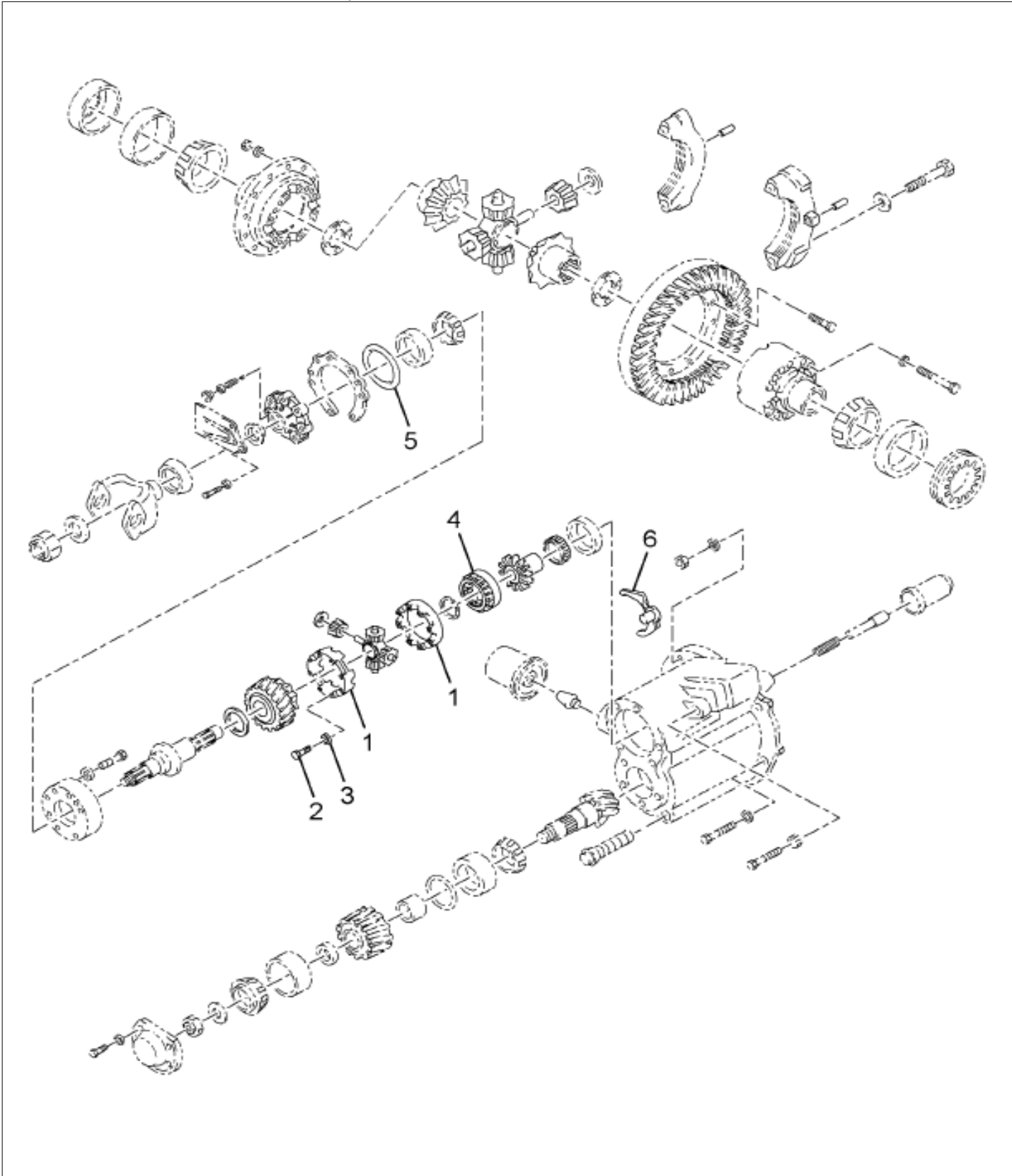
https://bookman.alshub.com/ Figure 1670270C91 KIT, I.A.D. DIFF CASE W/COLLAR
