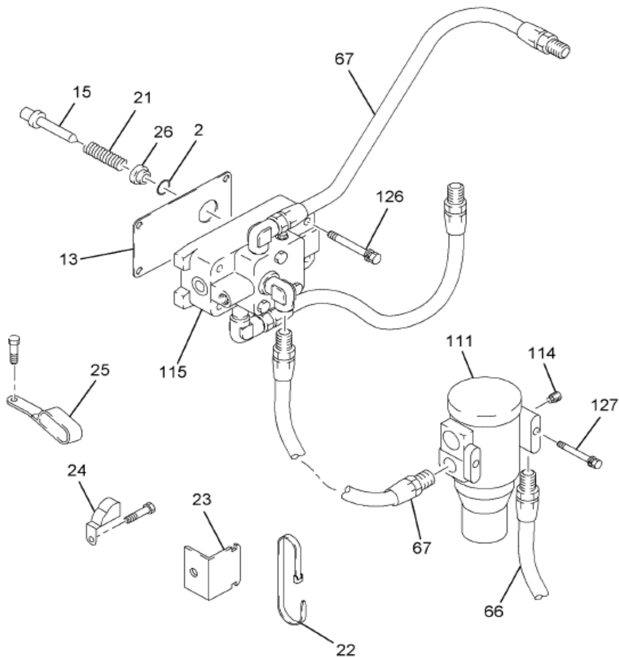
SLAVE VALVE AND AIR FILTER/REGULATOR ASSEMBLY
