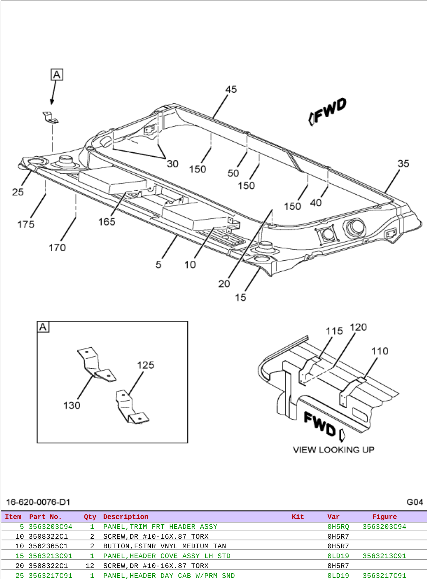
https://www.manualshub.com/ Figure 0H5R7 HEADER PANEL INSTL
