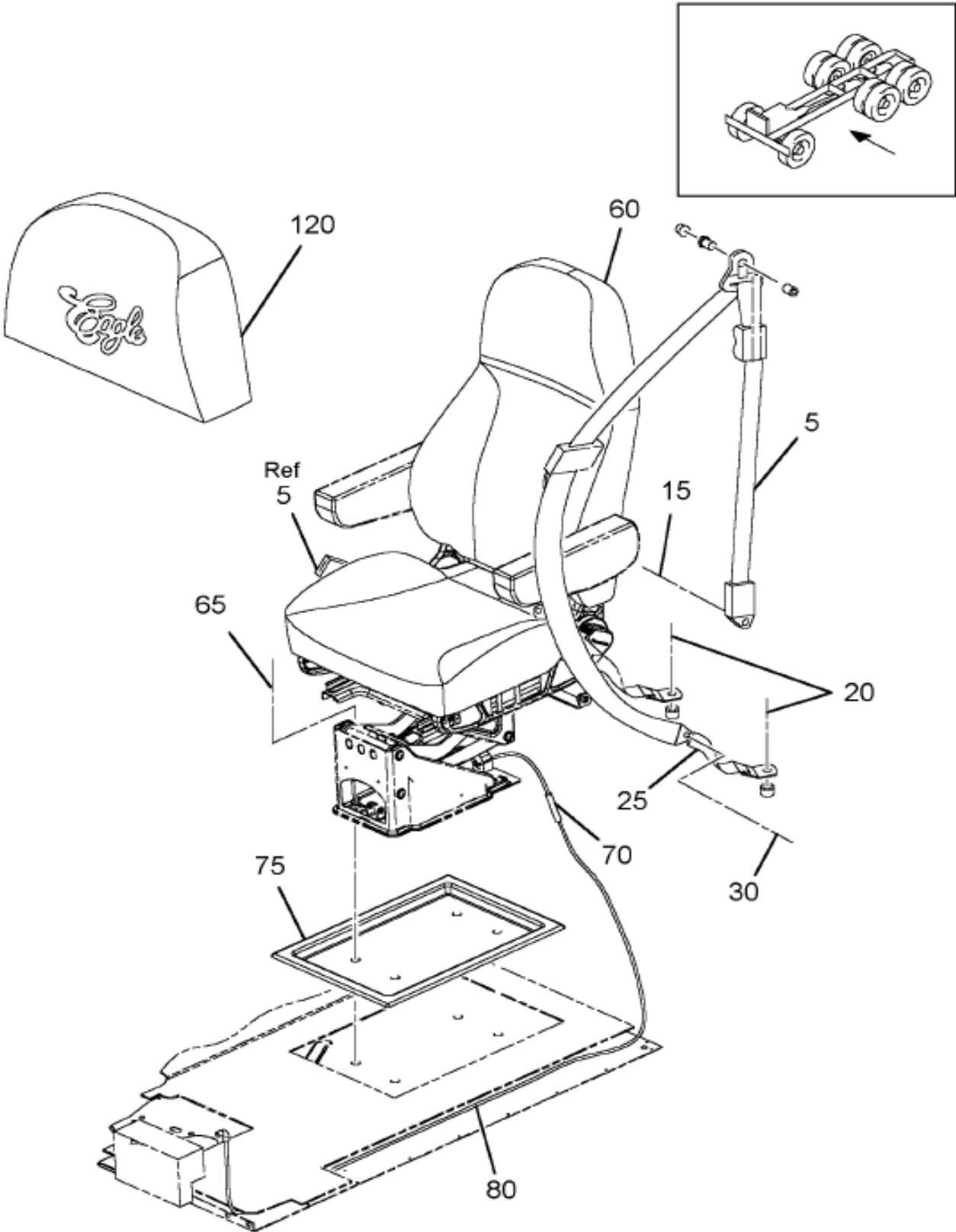
Figure 0H3R2 DRIVER SEAT; W/BELT, NATIONAL LEVEL 2
