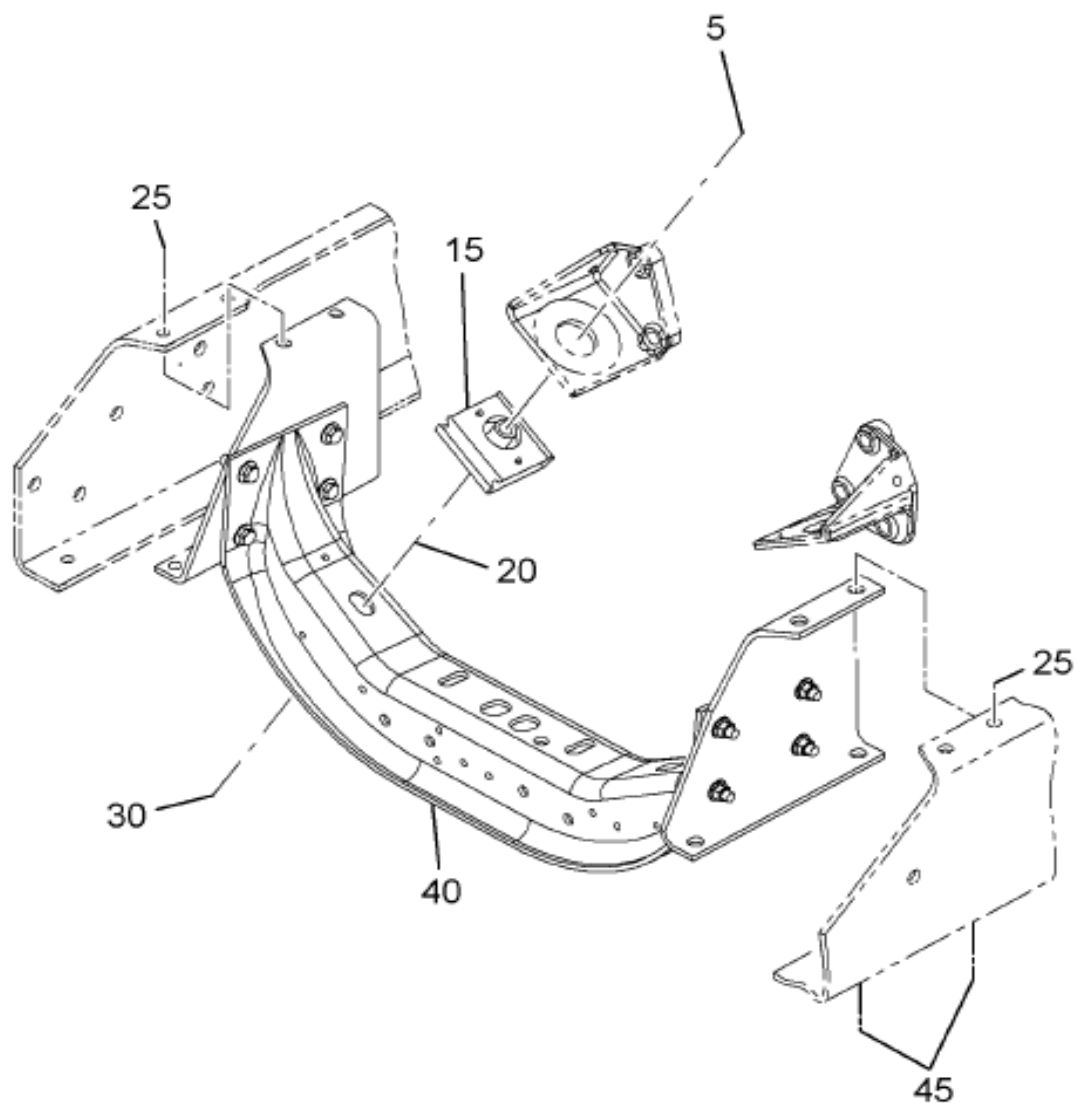
FRONT ENGINE MOUNT FOR M9920, M9930, OR M9940 WITH ISM OR C12 ENGINE
