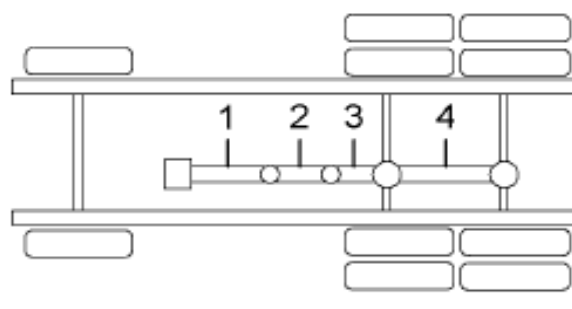
6X4, W/TWO CENTER BEARINGS
