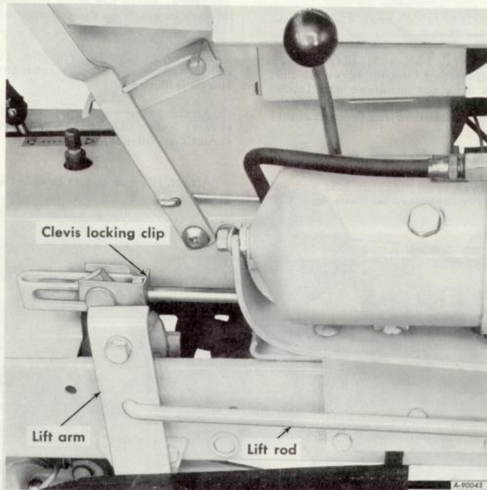
Illust. 11 Hydraulic lift arm attachment
