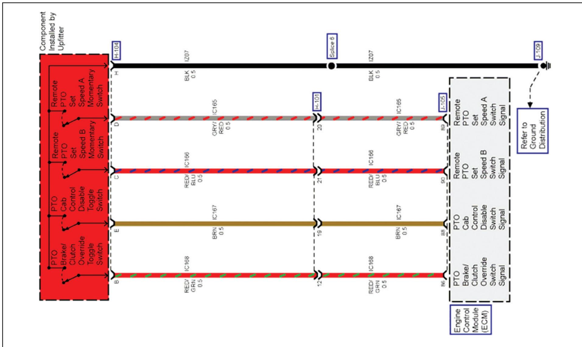
Brake clutch override, IP disable, Set a and b switches Illustration #9
