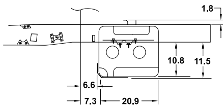
Side View In Frame Tank
