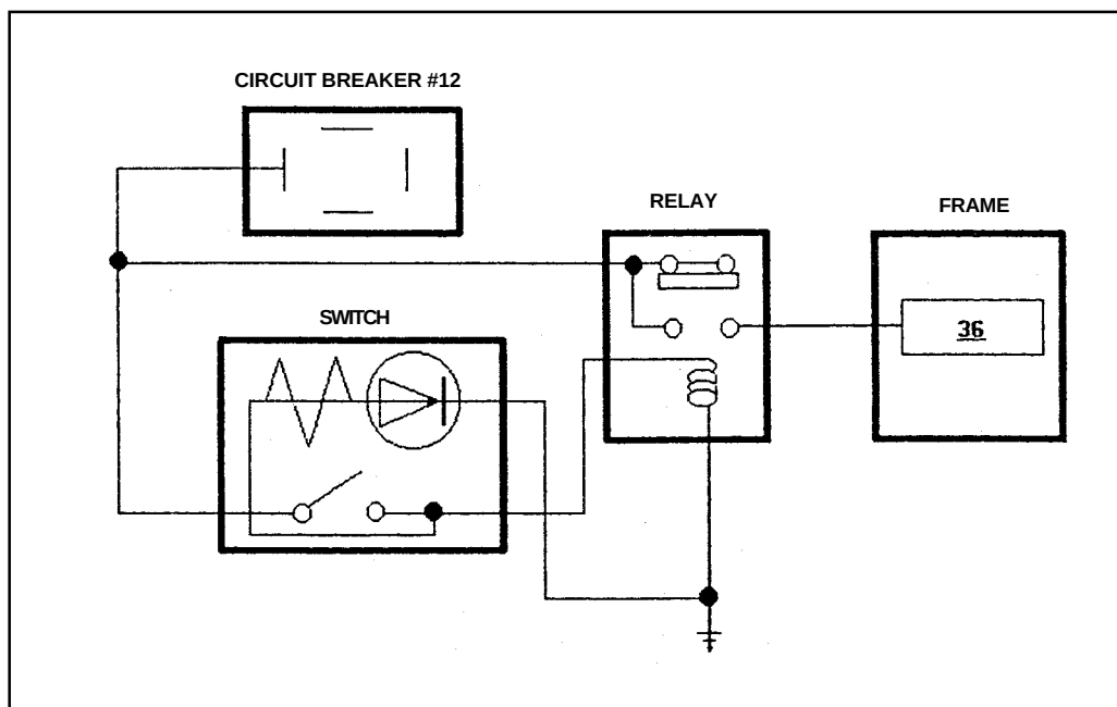
Rear Body Light Switch Wiring Diagram
