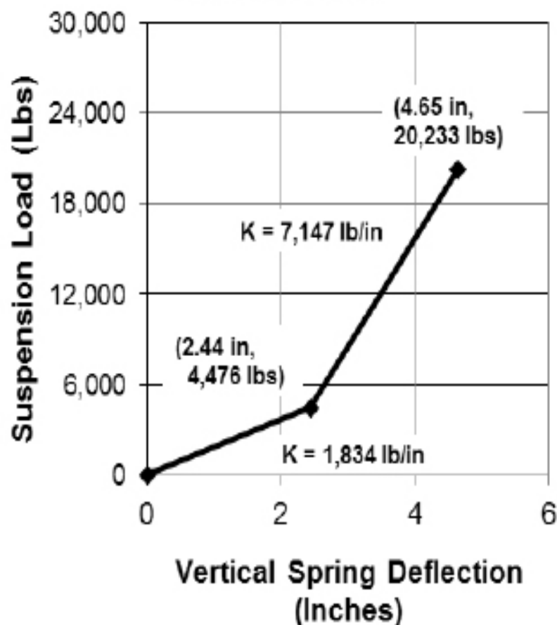
Rear Suspension Load vs. Deflection (Per Axle) 12,000 lb GVWR
