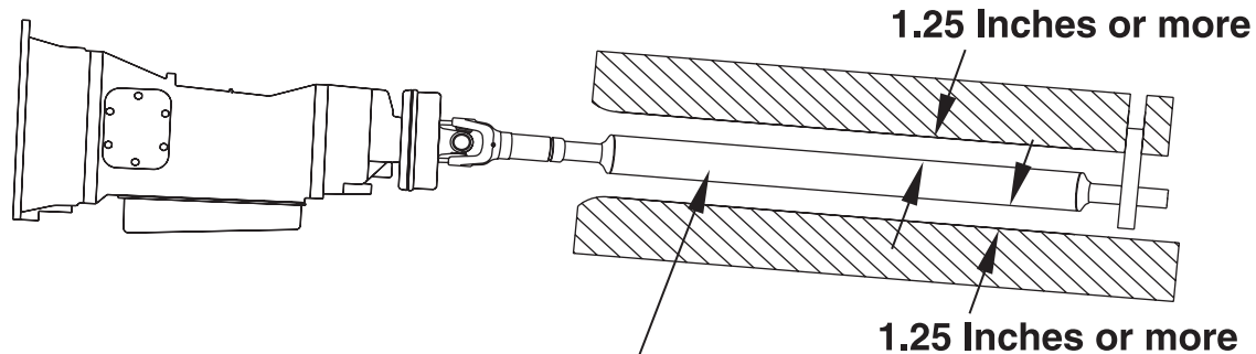
Front Propeller Shaft
