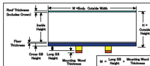
Calculator 1: Completed Vehicle Frontal Area From Body Inside Height
