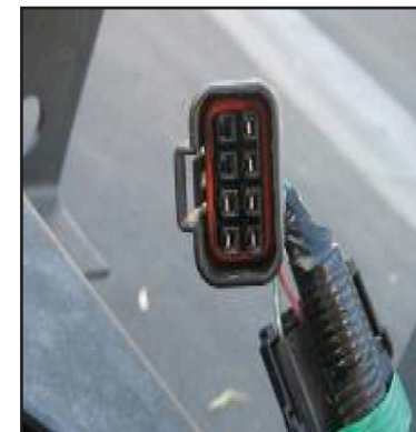
Chassis harness side part number 897364-5300
