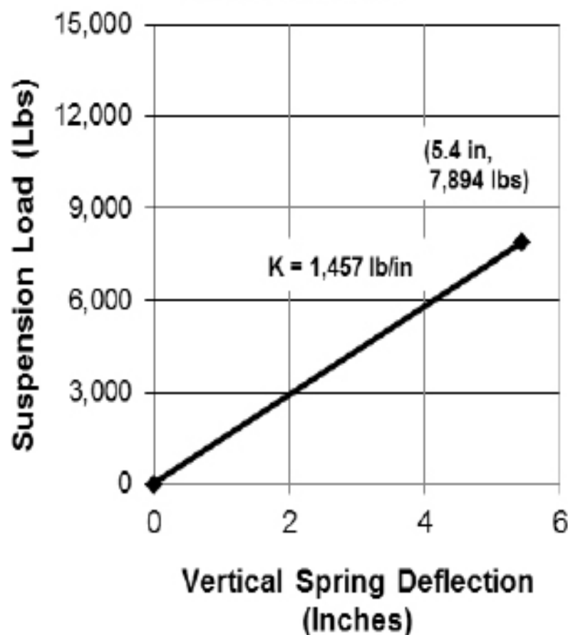
Front Suspension Load vs. Deflection (Per Axle) 12,000 lb GVWR
