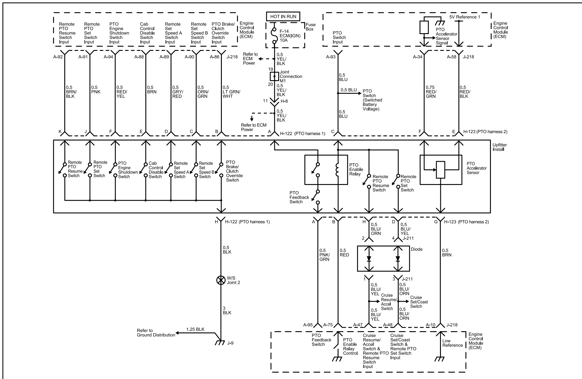
PTO Harness 1 and 2 Diagram Illustration #9
