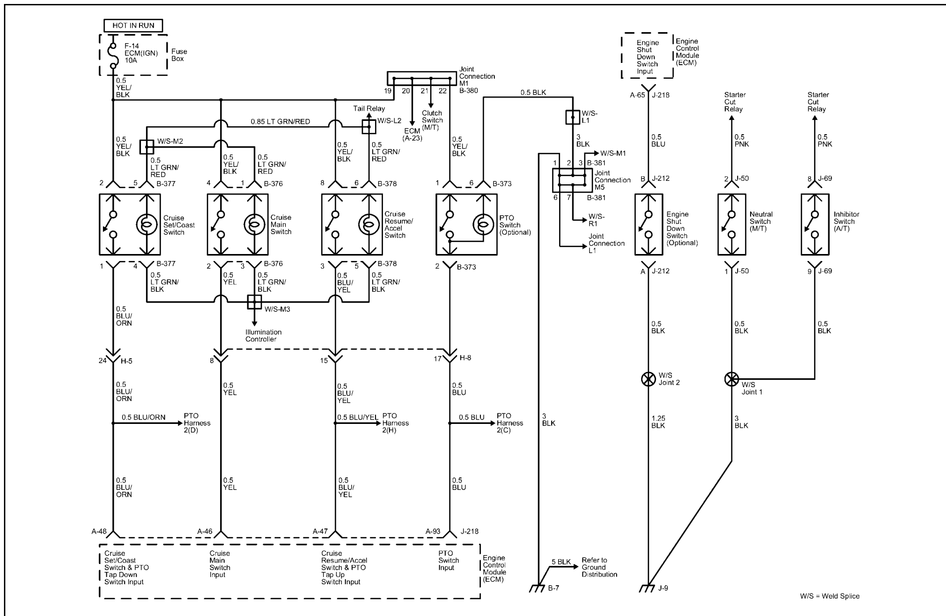
PTO Switch Wiring Diagram Illustration #8
