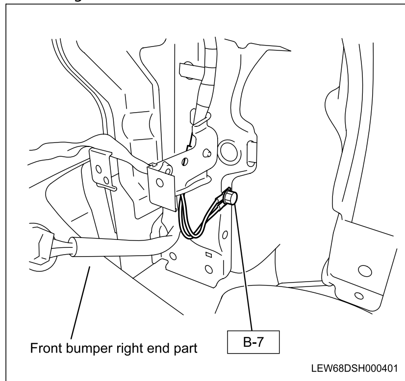
B-7 Headlight Bracket–RH
