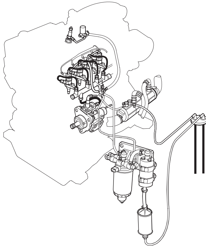
CIRCUIT FOR COMMON RAIL SYSTEM (CPI)
