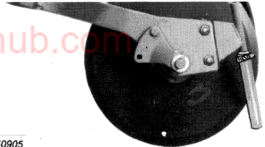
Opener W/Liquid Fertilizer Extension
