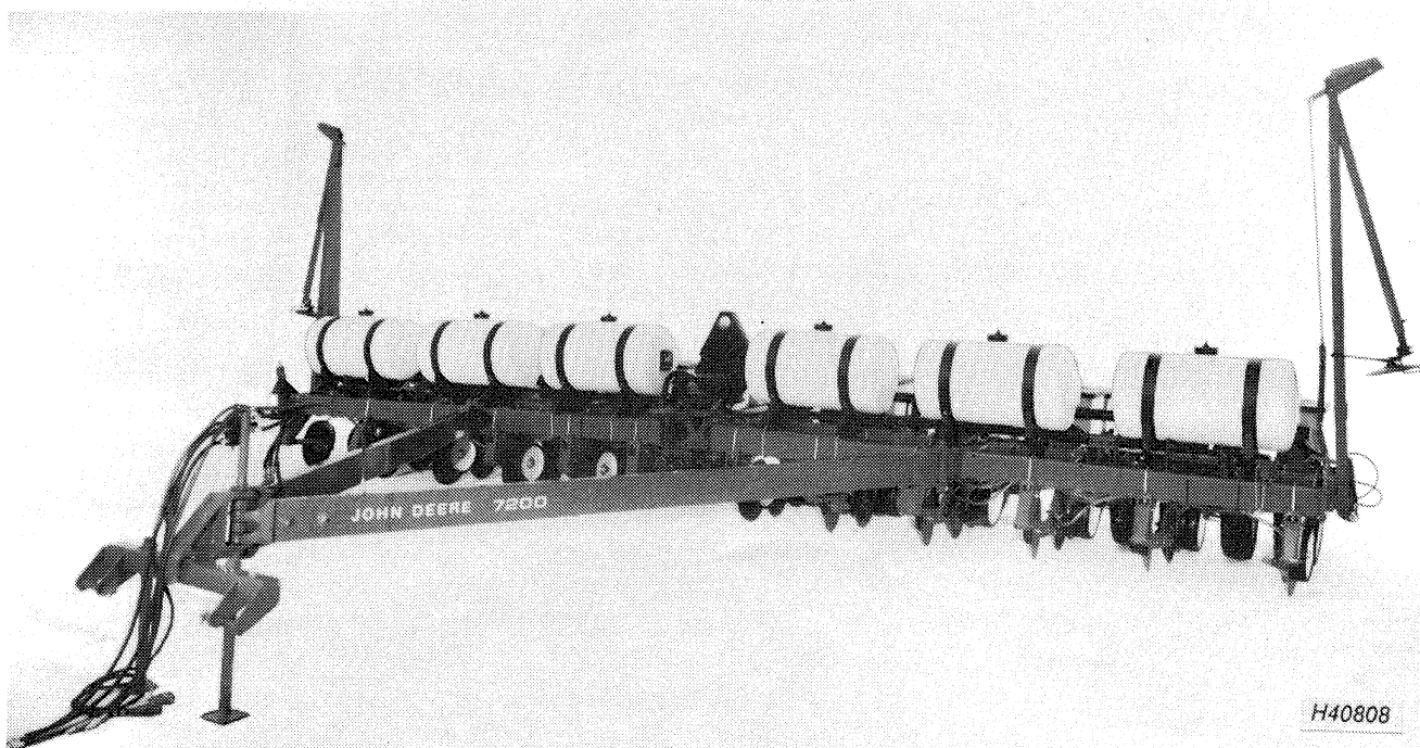
7200 Flex-Fold 12-Row Narrow Drawn Max-Emerge Planter with Vacuum Seed Metering System
