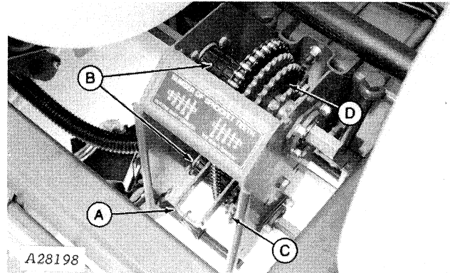
A—Chain Tightener B—Rubber Spacers
