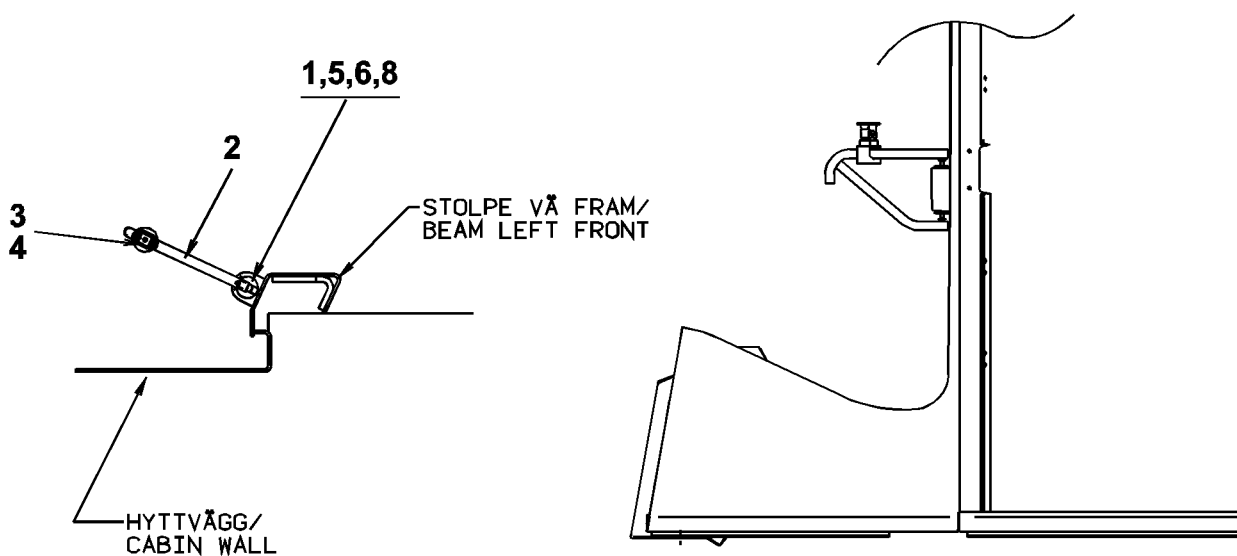
ALTERNATIVT SPEGLVÄNT PLACERAD / ALTERNATIVE MIRROR-INVERTED LOCATING
