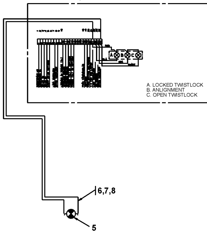
REVOLVING BEACON, ONCE
