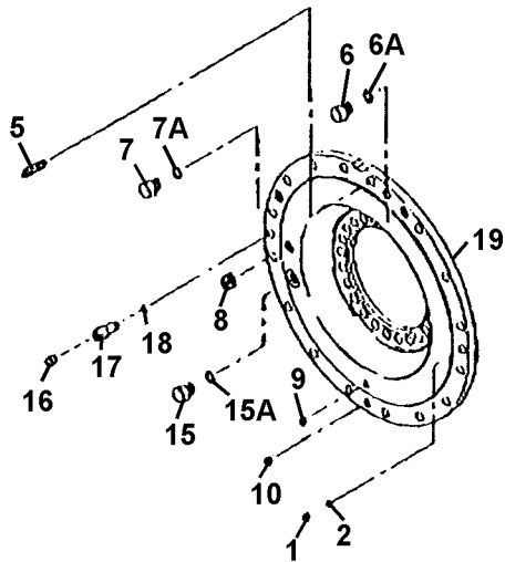
BRAKE COVER- LESS TEMP. SENSOR BRACKET
