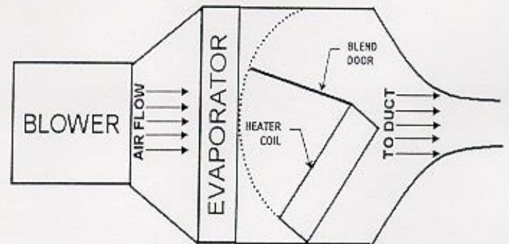
Blend Air System
