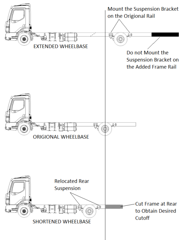
Figure 6-1 Wheelbase Customization
