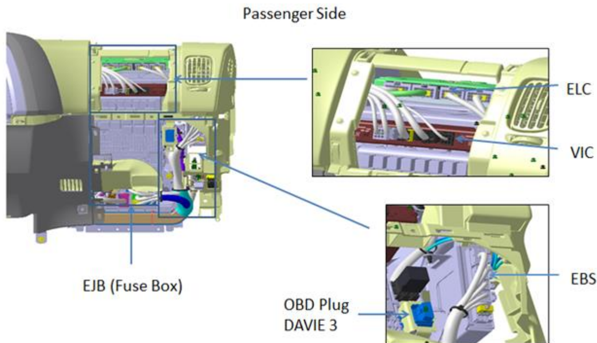
Figure 7-4 Contollers
