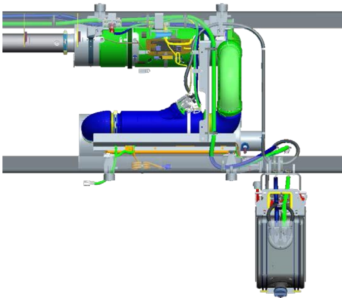
Horizontal Exhaust
