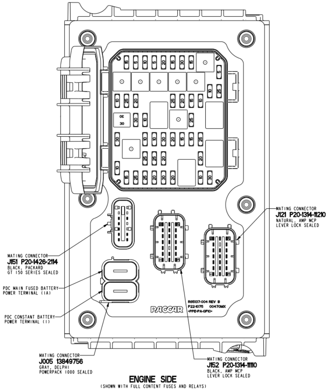
Figure 79 Engine Side Power Distribution Center
