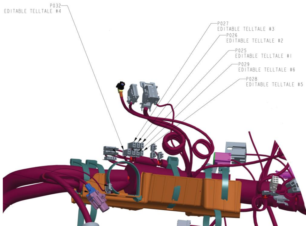
Figure 110 Body Builder Telltale Connections
