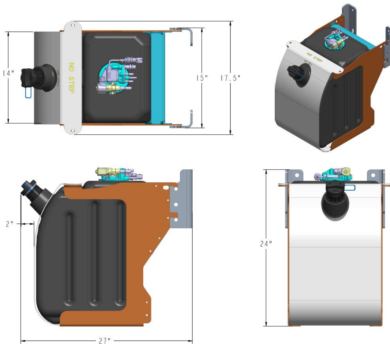
Figure 31 Large DEF Tank Dimensions
