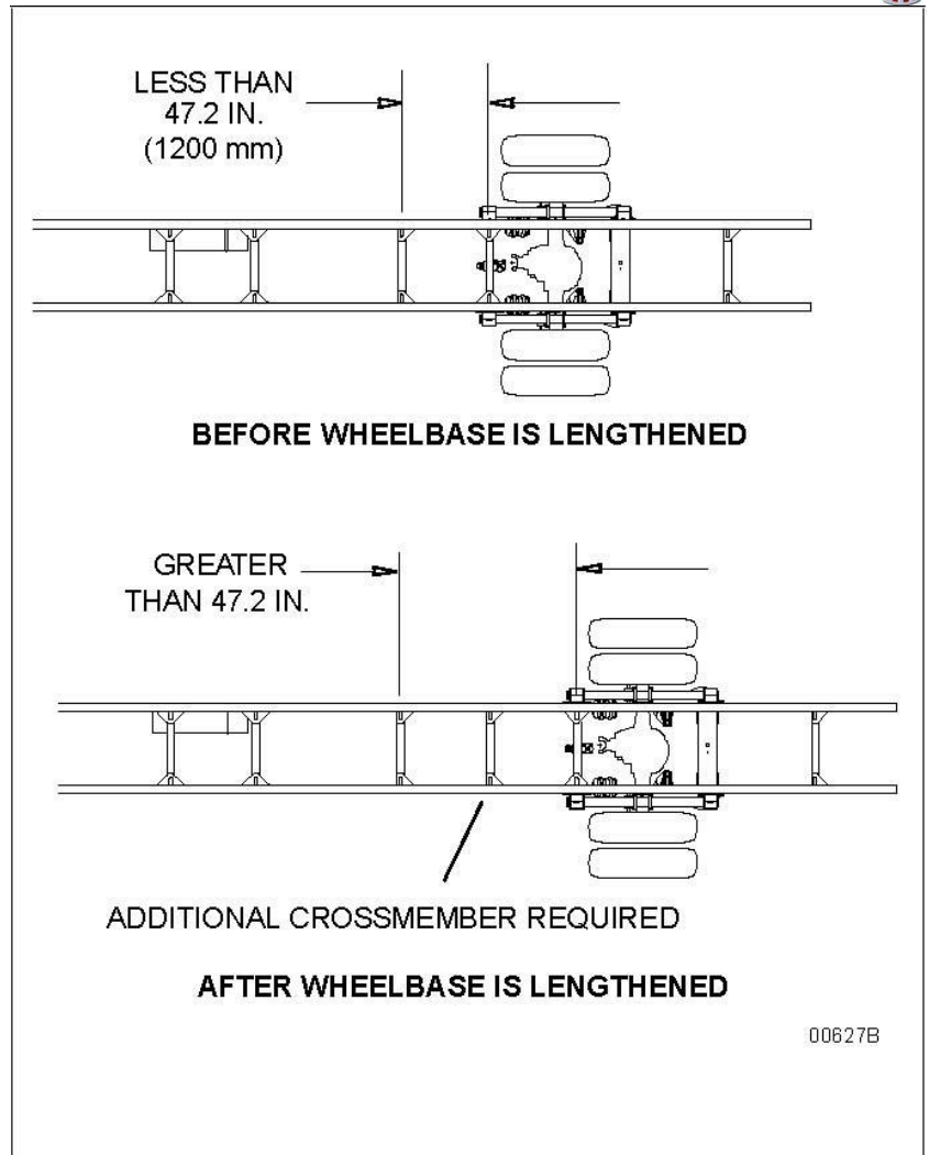
Figure 57 Crossmember Spacing Requirements
