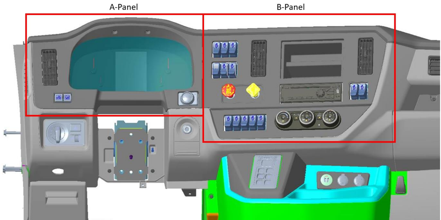
Figure 95 Dash Layout
