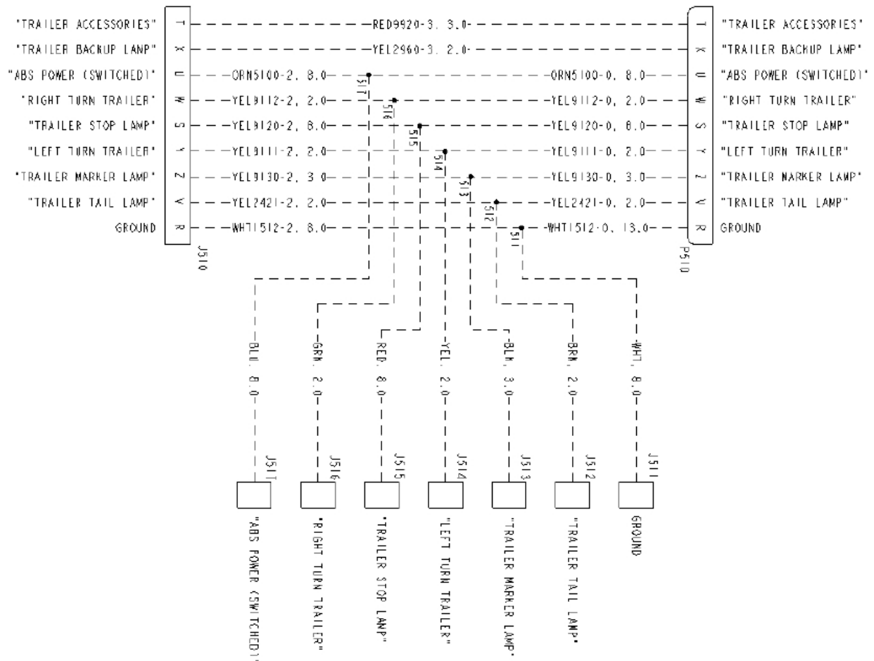
Figure 103 Junction Box BOC or EOF
