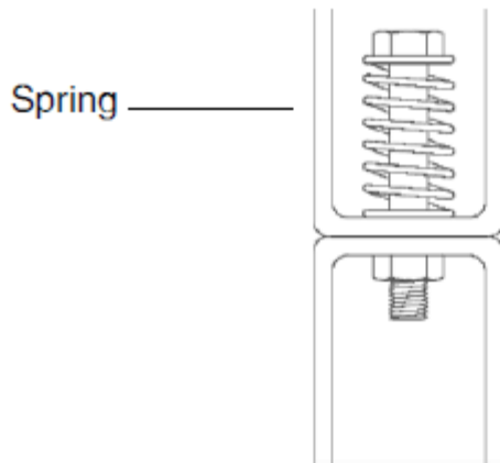
Figure 48 Mounting Brackets with Spring
