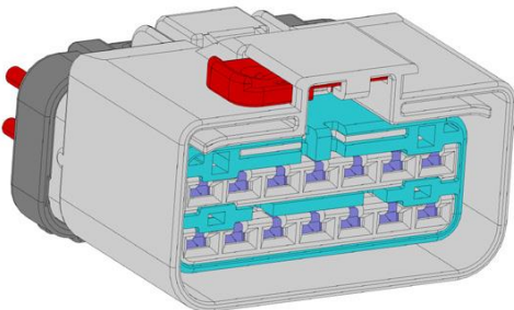
Figure 63 RP 1226 Connector
