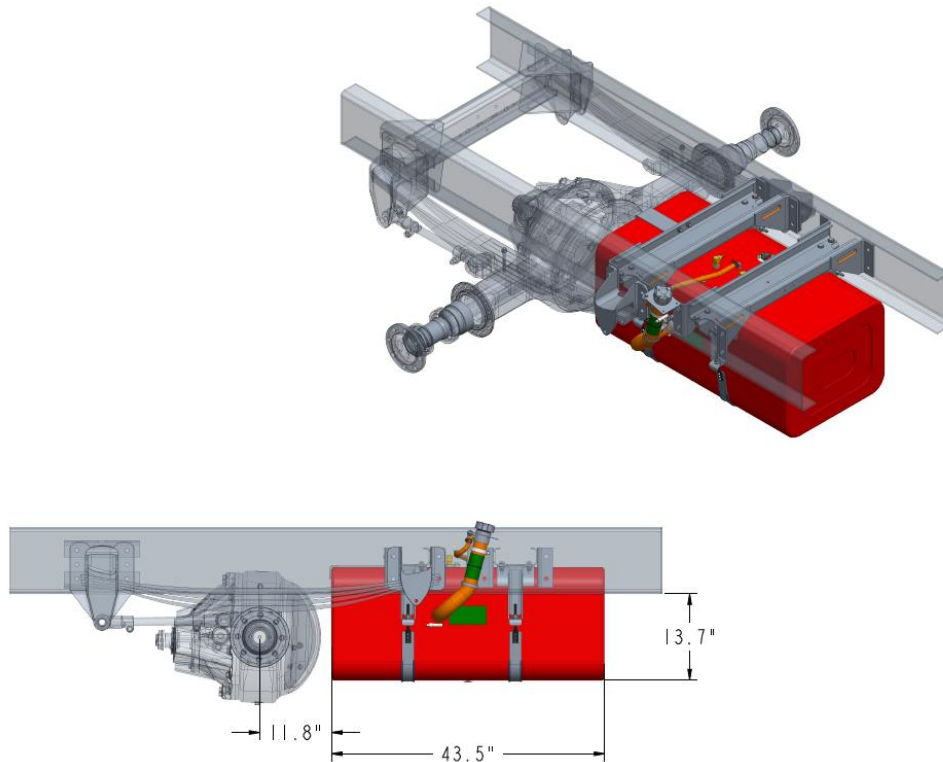
Figure 35 In-Frame Fuel Tank - 70 Gallon – With Dimensions
