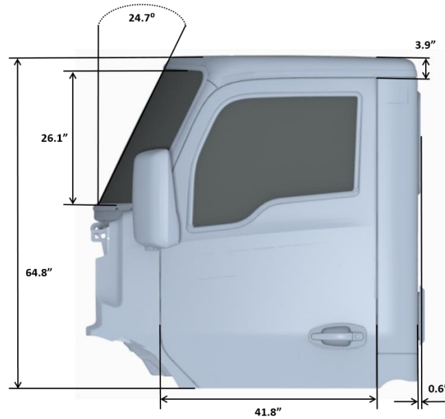
Figure 11 Cab Dimensions 2.1m Medium Duty
