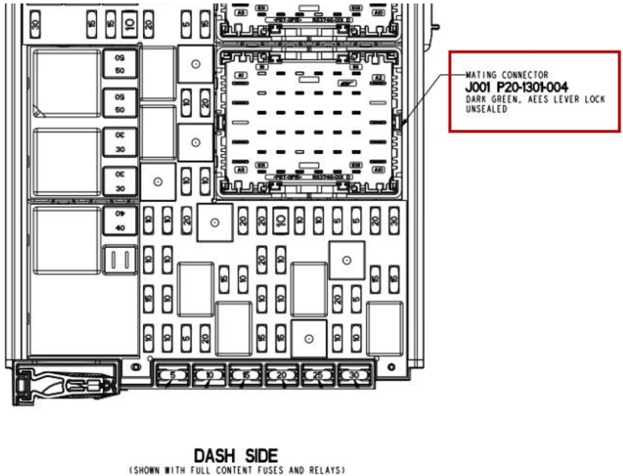
Figure 100 Spare Circuit Location on Power Distribution Center (Dash-Side, P001)
