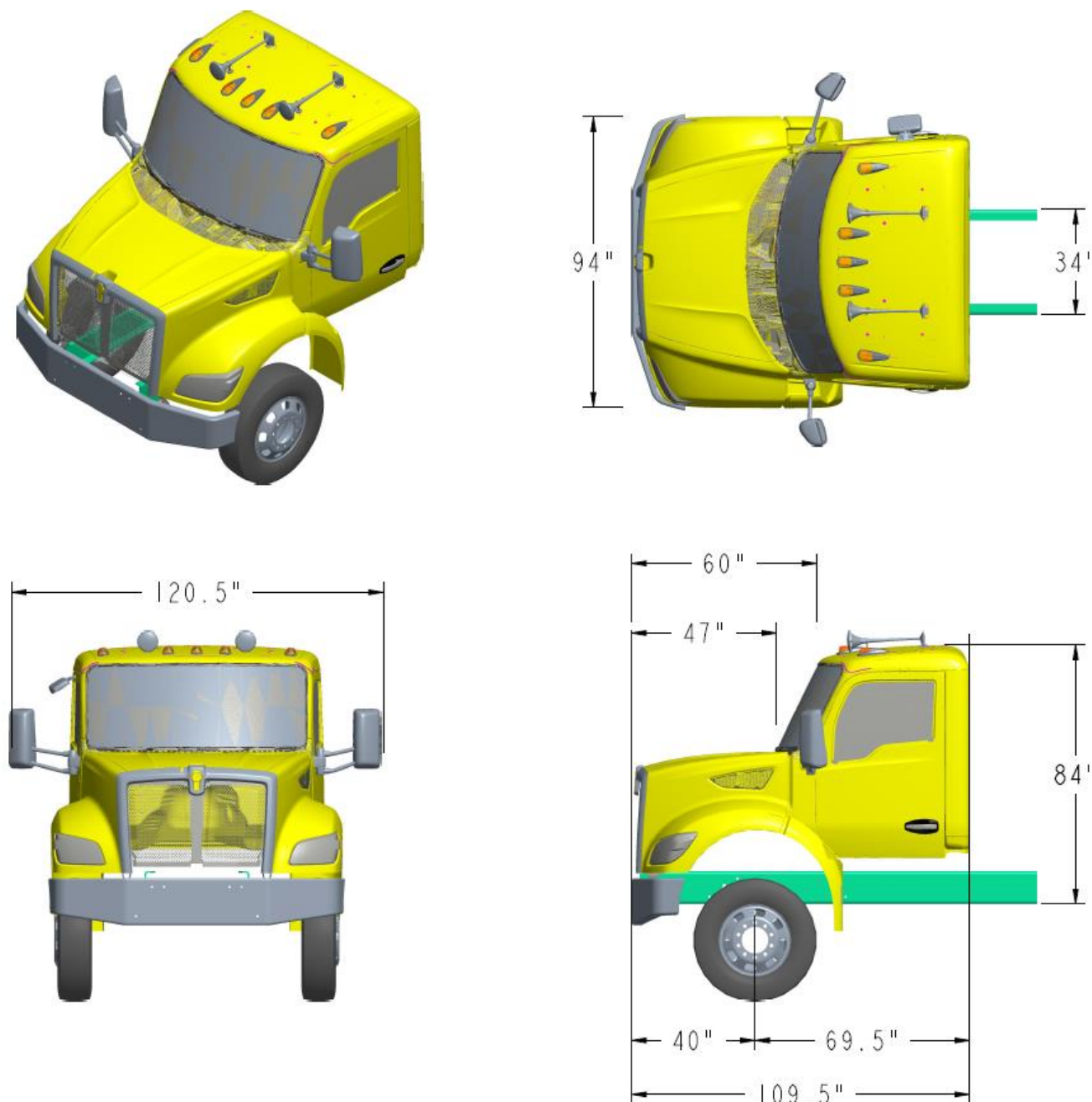
Figure 9 VH (109.5" BBC) - With Raised Roof - Overall Dimensions
