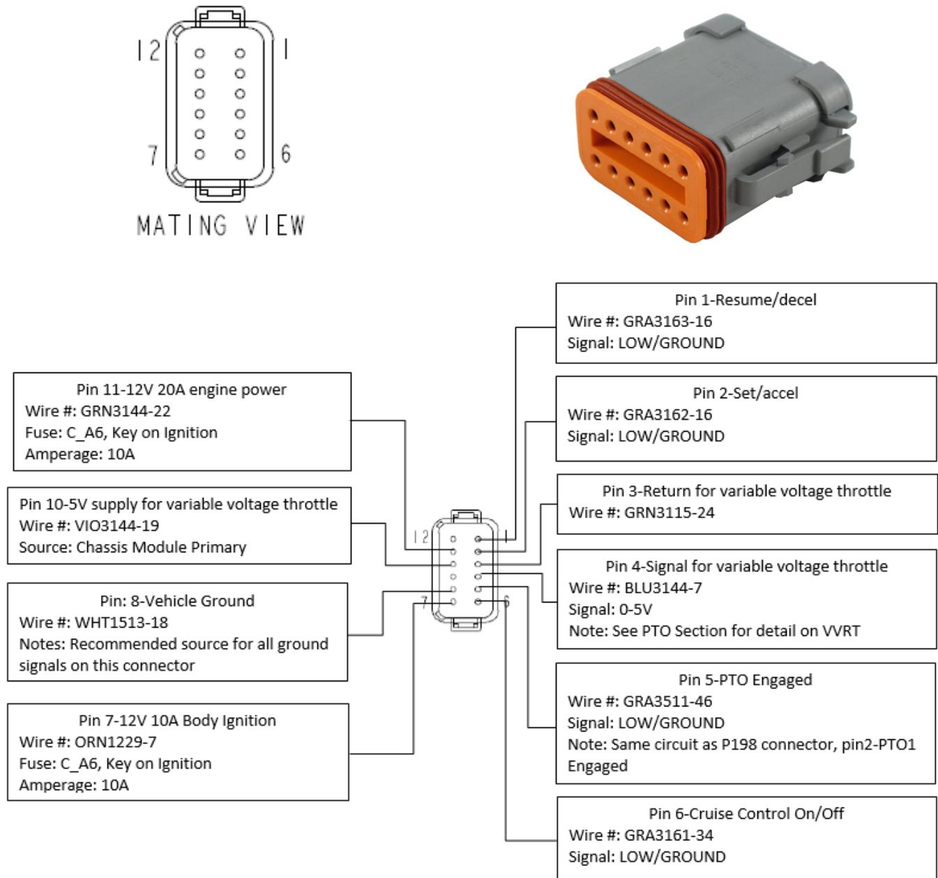
Figure 75 Engine Harness 12 Pin Connector and Pinout Details
