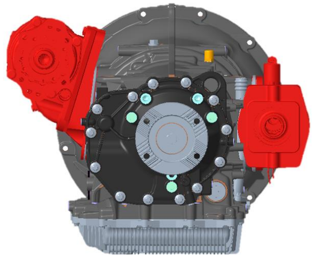
Figure 113 PACCAR 8-Speed Automatic Transmission PTO Locations
