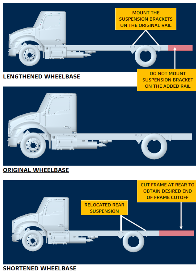
Figure 56 Wheelbase Customization
