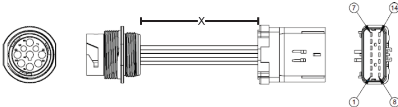
Figure 65 RP1226 to 9 Pin Jumper
