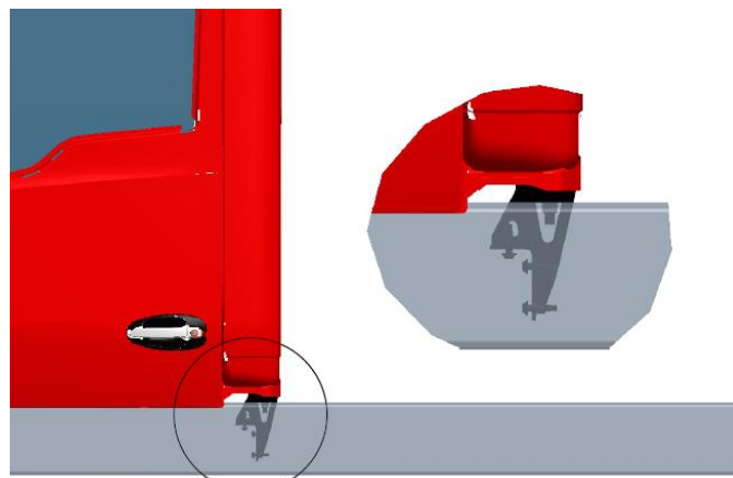
Figure 15 Cab Rigid Suspension
