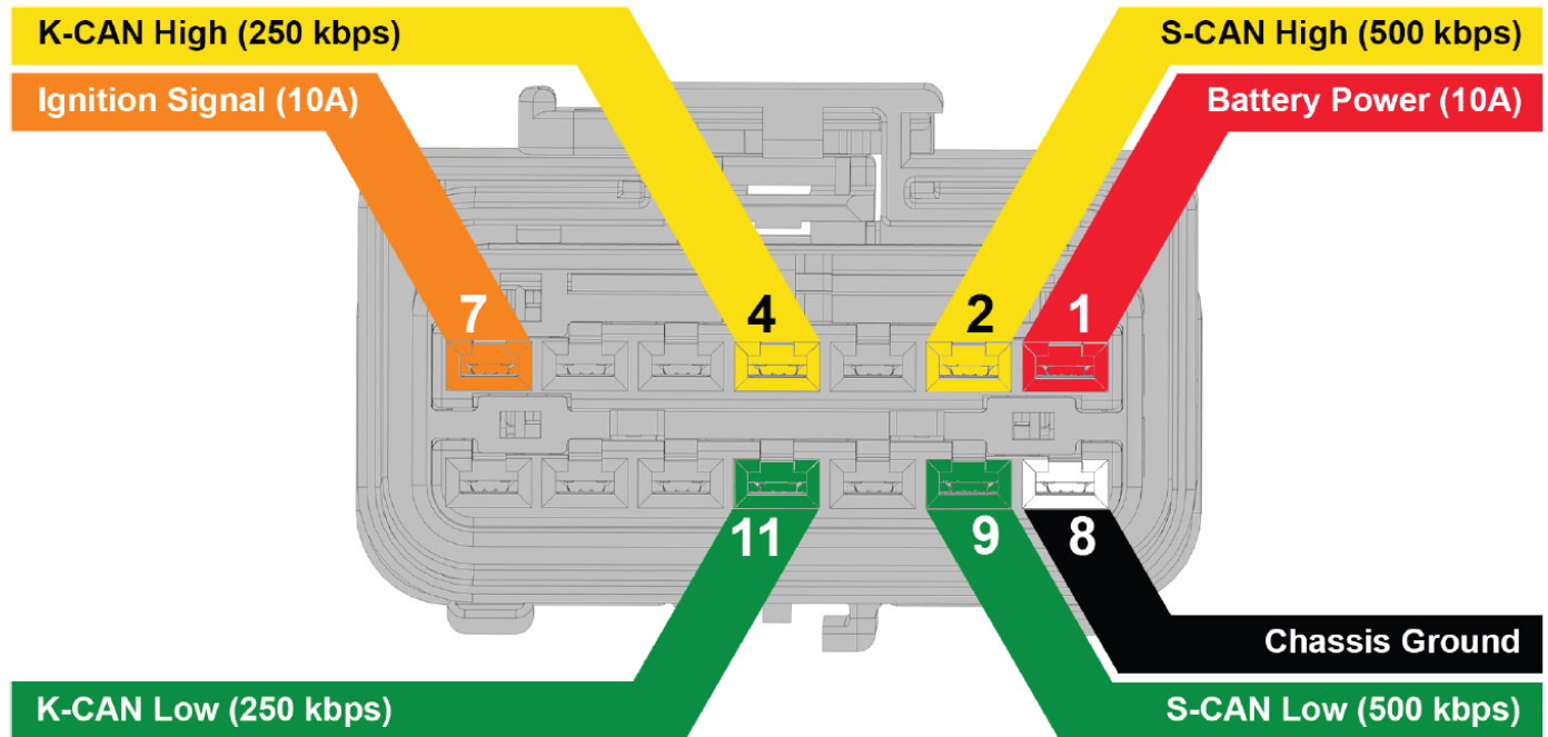
Figure 62 RP1226 Visual Pinout
