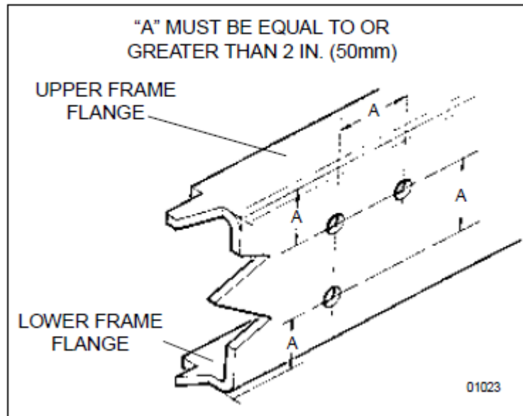
Figure 50 Frame Hole Location Guidelines for Frame Rail and Bracket
