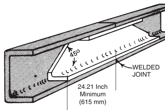
FIGURE 7-2. Frame Insert
