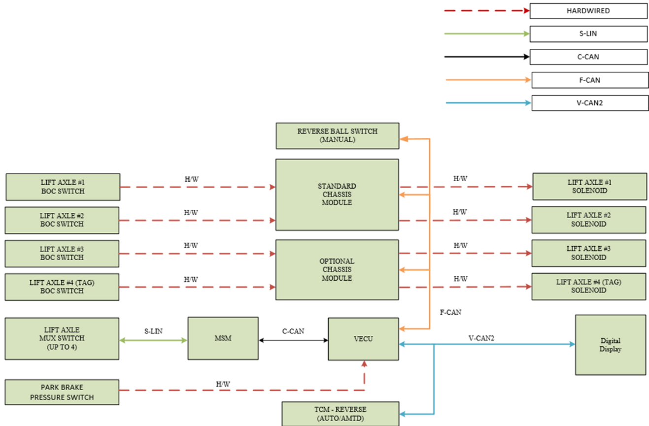
Figure 106 Lift Axle Diagram
