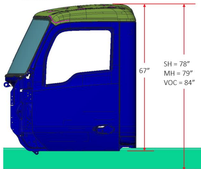
Figure 12 Low Roof and Raised Roof Cab Height 2.1m Medium Duty
